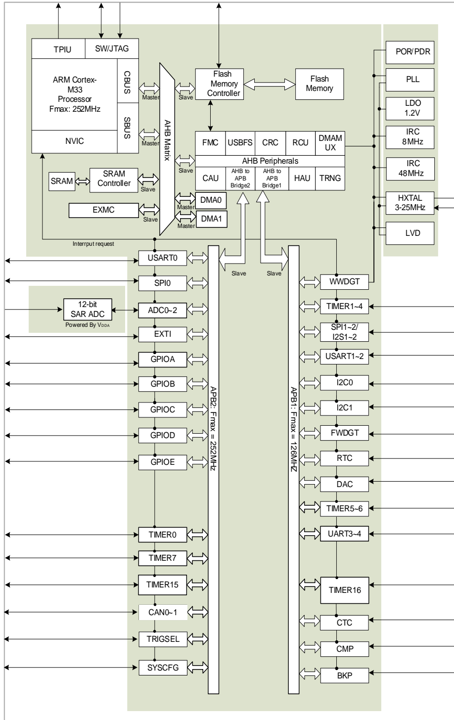
Figure 2-1. GD32F503xx block diagram
