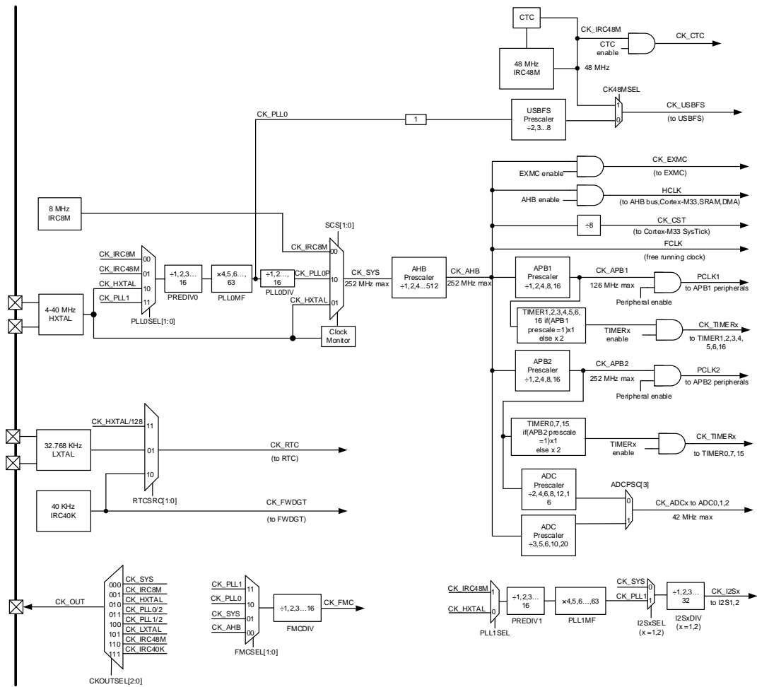
Figure 2-9. GD32F503xx clock tree
