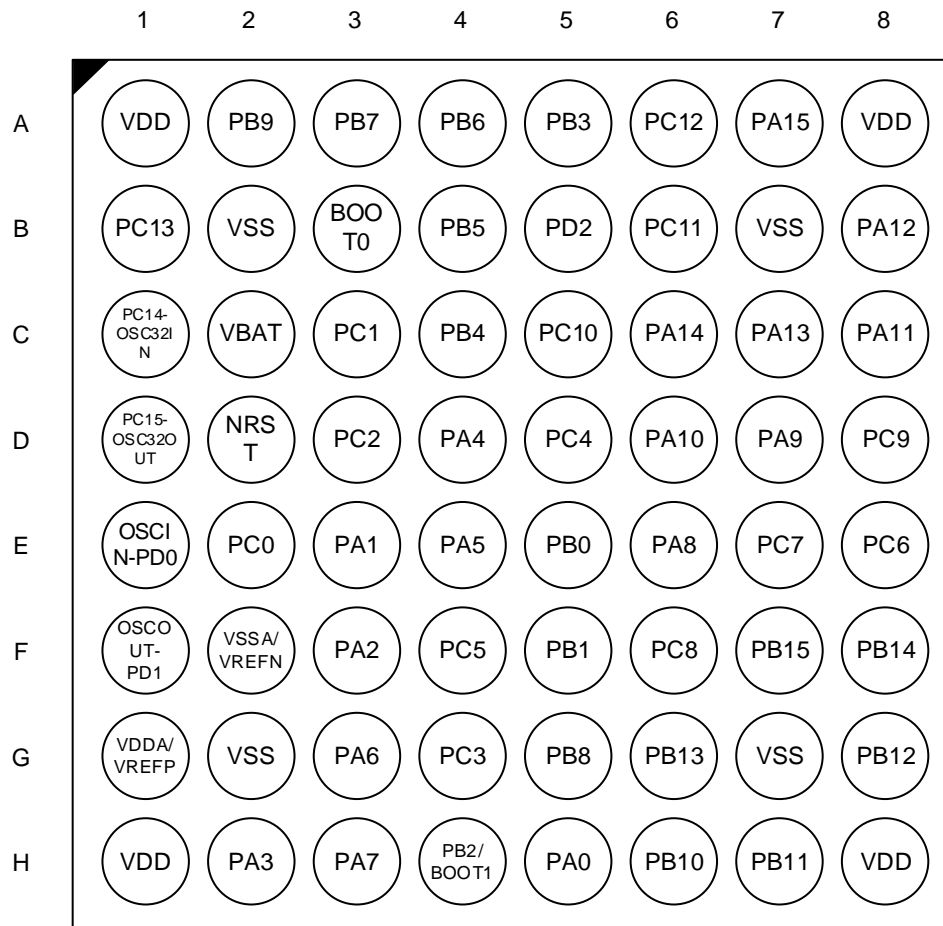
Figure 2-5. GD32F503Rx BGA64 pinouts
