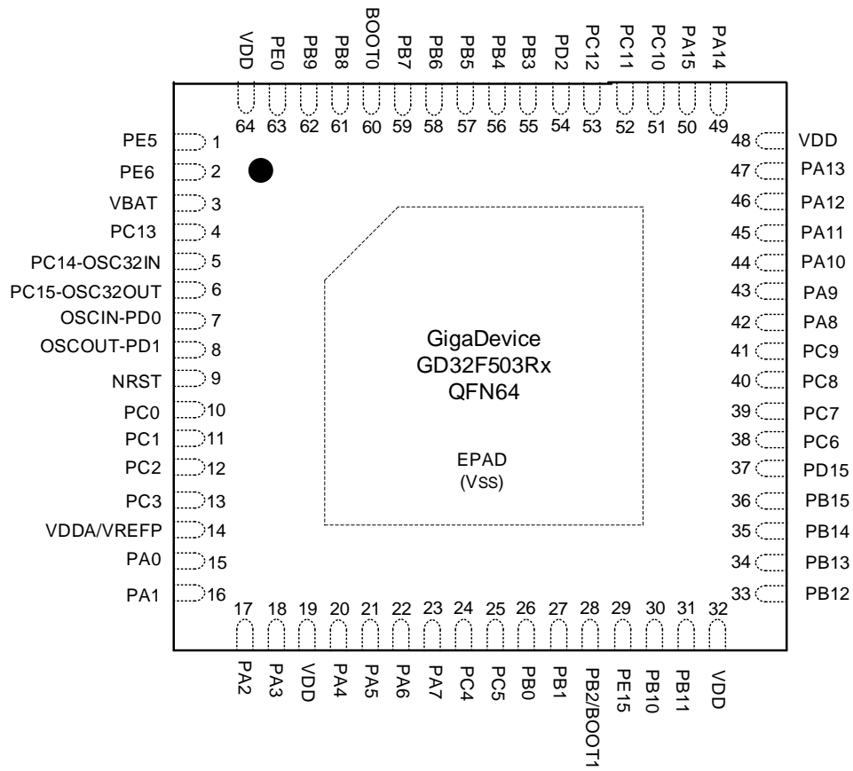
Figure 2-4. GD32F503Rx QFN64 pinouts
