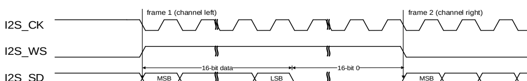
Figure 25-30. MSB justified standard timing diagram (DTLEN=00, CHLEN=1, CKPL=1)
