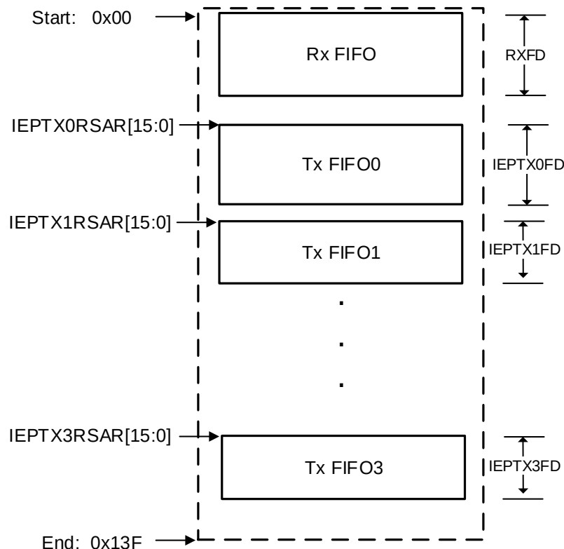
Figure 29-6. Device mode FIFO space in SRAM
