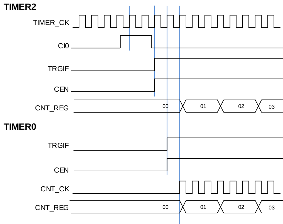
Figure 12-45. Trigger TIMER0 and TIMER2 by the CI0 signal of TIMER2
