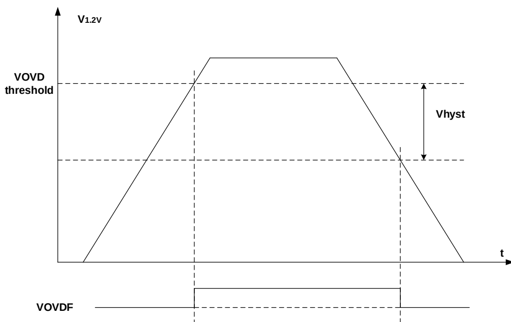
Figure 7-5. waveform of VOVD
