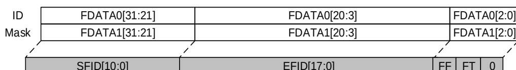
Figure 27-7. 32-bit mask mode filter
