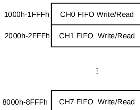
Figure 29-5. Host mode FIFO access register map
