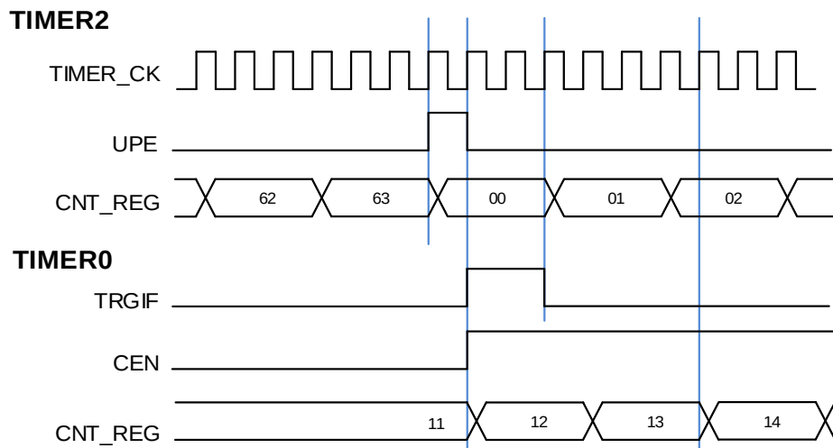
Figure 13-42. Trigger mode of TIMER0 controlled by update signal of TIMER2
