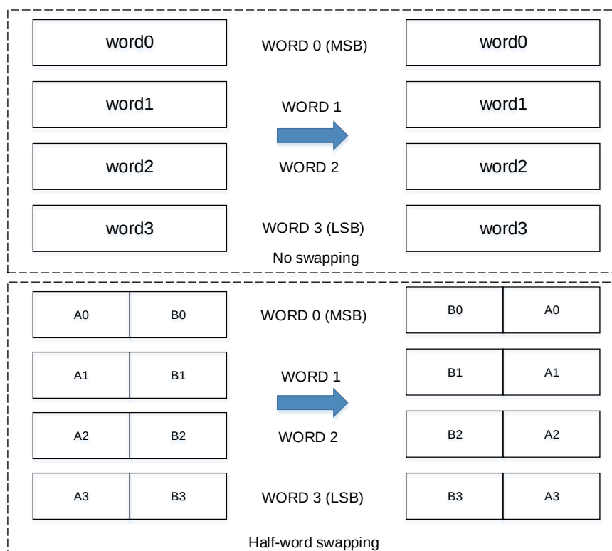
Figure 19-1. DATAM No swapping and Half-word swapping
