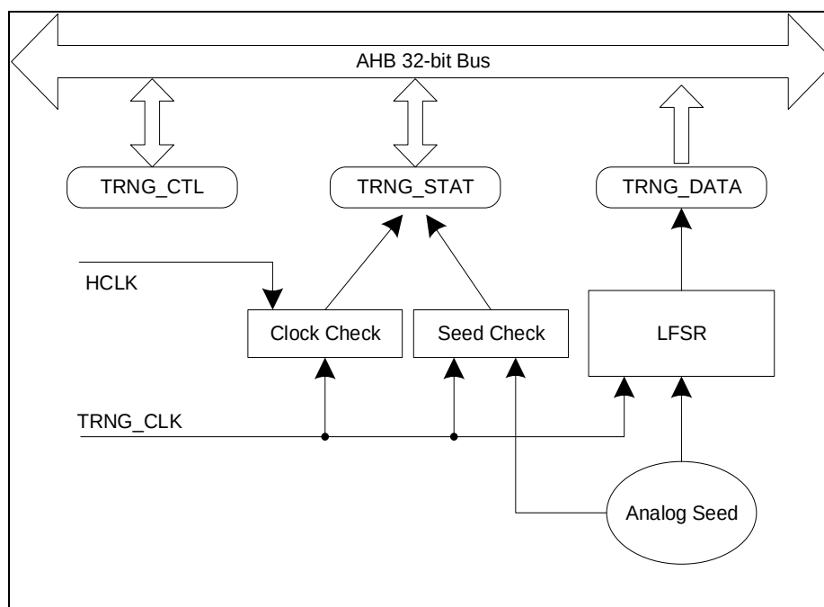
Figure 18-1. TRNG block diagram
