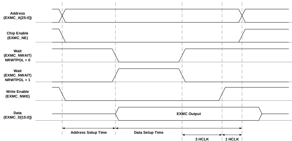
Figure 28-9. Write access timing diagram under async-wait signal assertion
