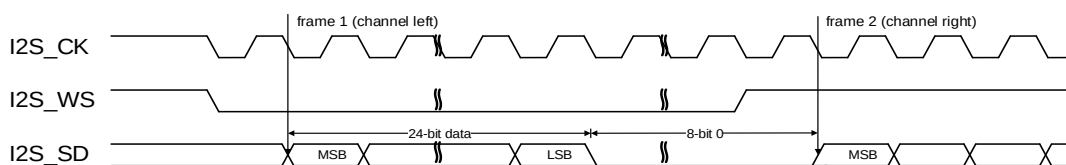
Figure 25-20. I2S Philips standard timing diagram (DTLEN=01, CHLEN=1, CKPL=1)
