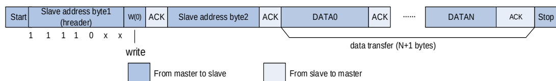
Figure 26-4. I2C communication flow with 10-bit address (Master Transmit)
