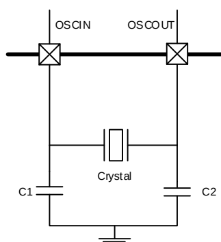
Figure 9-5. HXTAL clock source
