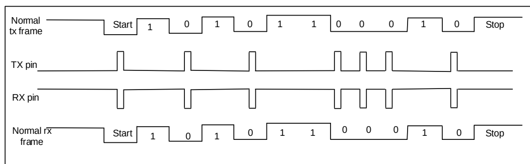
Figure 24-14. IrDA data modulation
