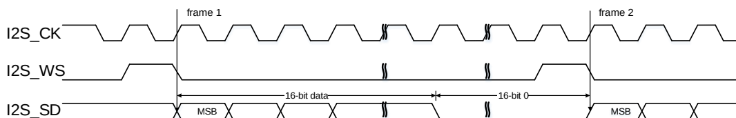
Figure 25-42. PCM standard short frame synchronization mode timing diagram (DTLEN=00, CHLEN=1, CKPL=1)
