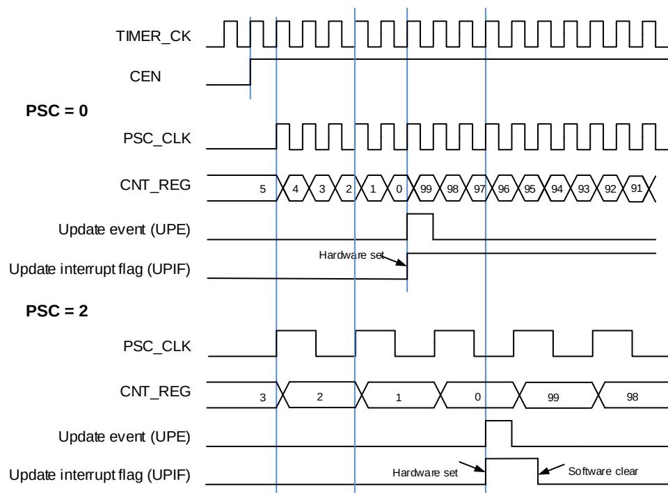
Figure 13-6. Timing diagram of down counting mode, \text{PSC}=0/2
