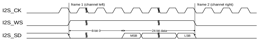
Figure 25-31. LSB justified standard timing diagram (DTLEN=01, CHLEN=1, CKPL=0)
