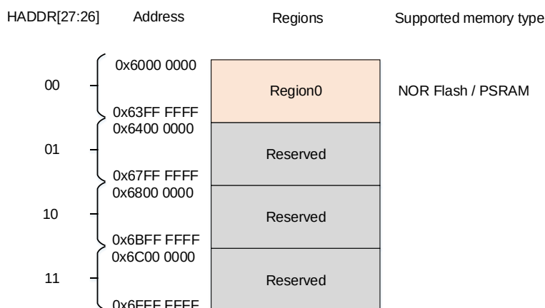
Figure 28-3. Four regions of bank0 address mapping
