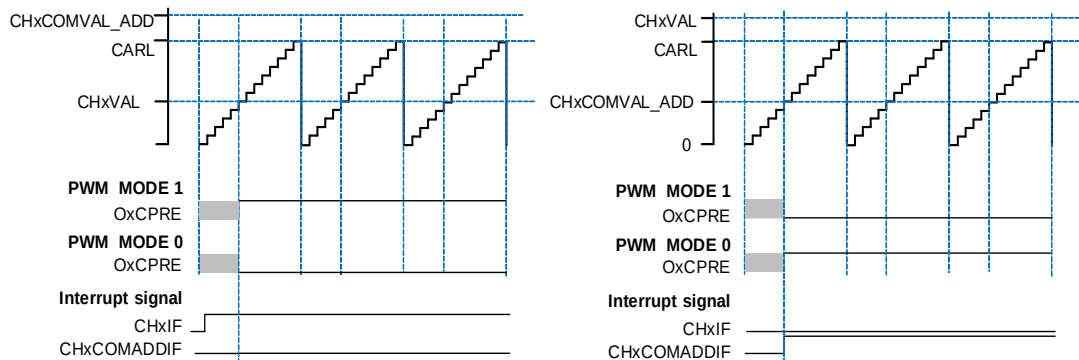
Figure 13-20. Channel x output PWM with CHxVAL or CHxCOMVAL_ADD exceeds CARL
