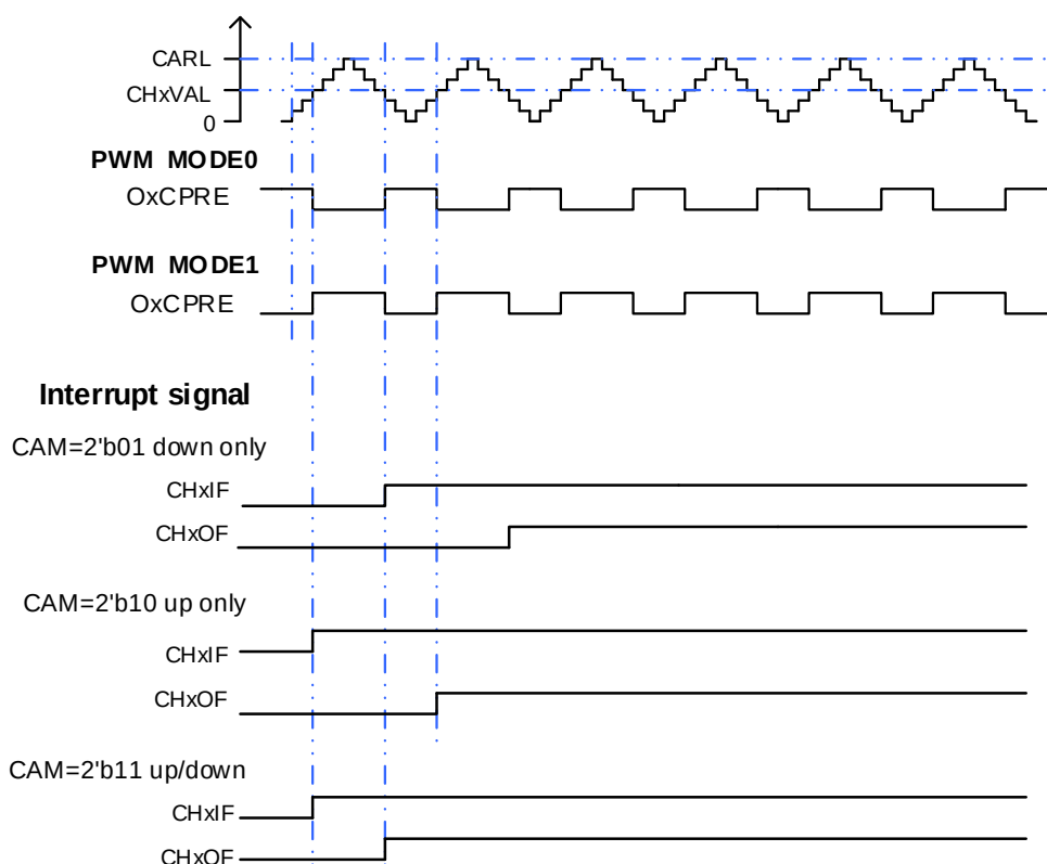
Figure 13-88. Timing diagram of CAPWM
