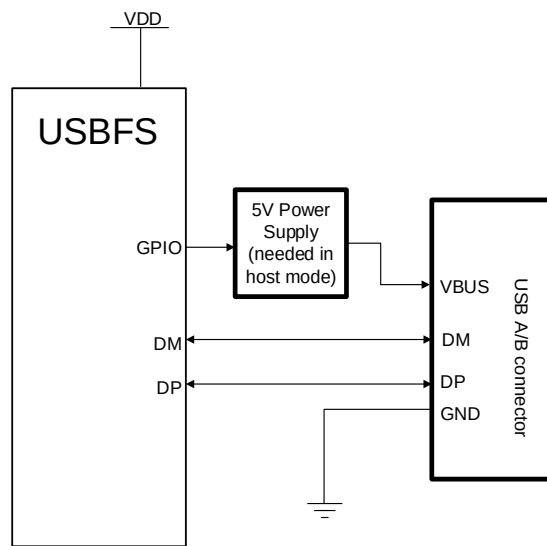
Figure 29-2. Connection with host or device mode
