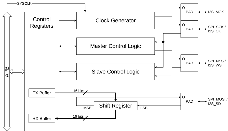
Figure 25-14. Block diagram of I2S
