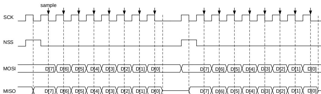
Figure 24-8. Timing diagram of TI master mode with discontinuous transfer
