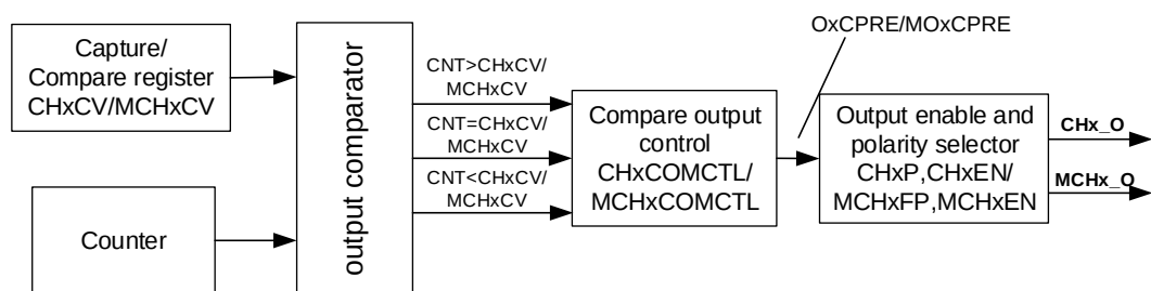
Figure 13-84. Output compare logic (when MCHxMSEL = 2'11, x=0)
