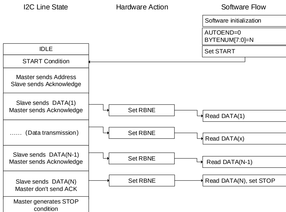
Figure 25-20. Programming model for master receiving ( N \leq 255 )
