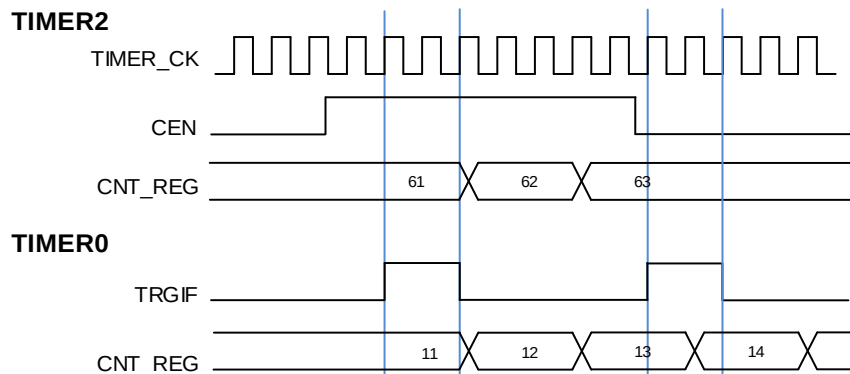
Figure 13-41. Trigger mode of TIMER0 controlled by enable signal of TIMER2
