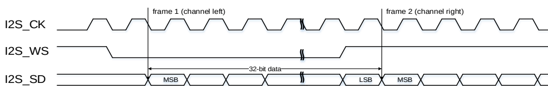
Figure 25-17. I2S Philips standard timing diagram (DTLEN=10, CHLEN=1, CKPL=0)
