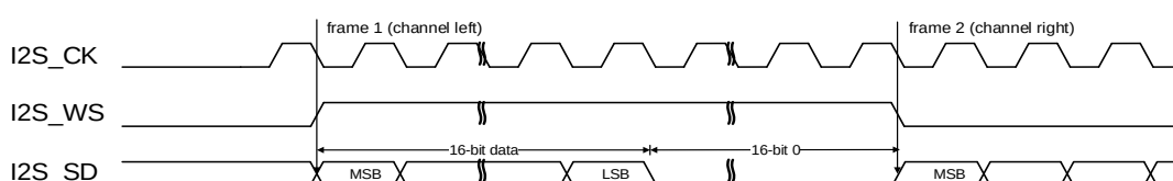
Figure 25-29. MSB justified standard timing diagram (DTLEN=00, CHLEN=1, CKPL=0)
