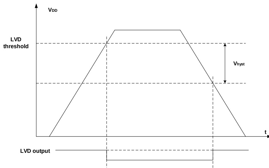
Figure 7-3. Waveform of the LVD threshold
