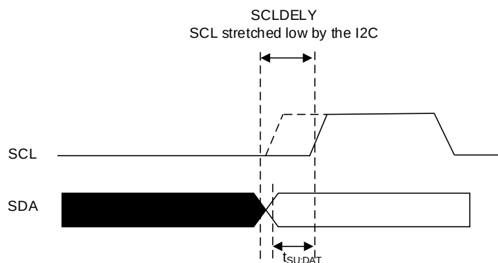
Figure 26-10. Data setup time
