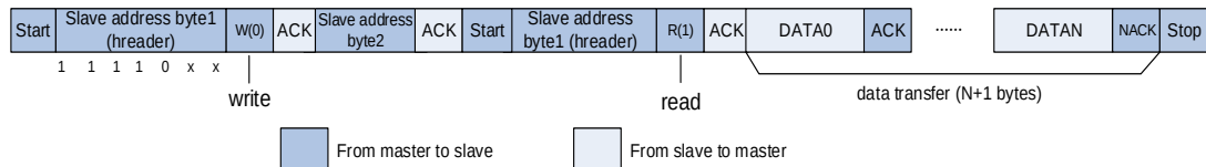
Figure 26-8. I2C communication flow with 10-bit address (Master Receive when HEAD10R=1)
