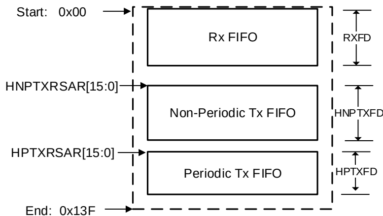
Figure 29-4. HOST mode FIFO space in SRAM
