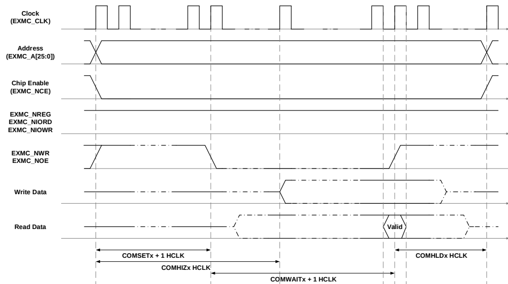
Figure 28-12. Access timing of common memory space of NAND flash Controller
