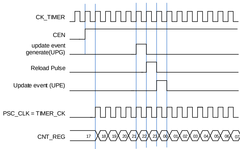
Figure 13-71. Normal mode, internal clock divided by 1
