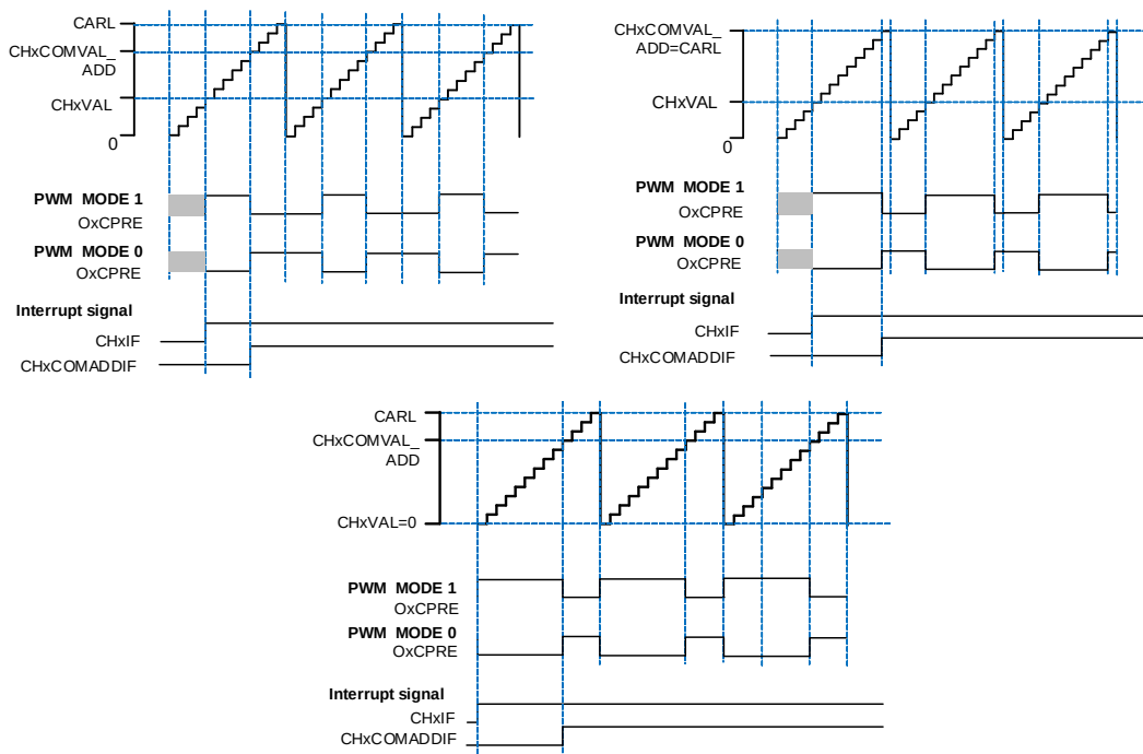
Figure 12-17. Channel x output PWM with ( CHxVAL < CHxCOMVAL\_ADD )
