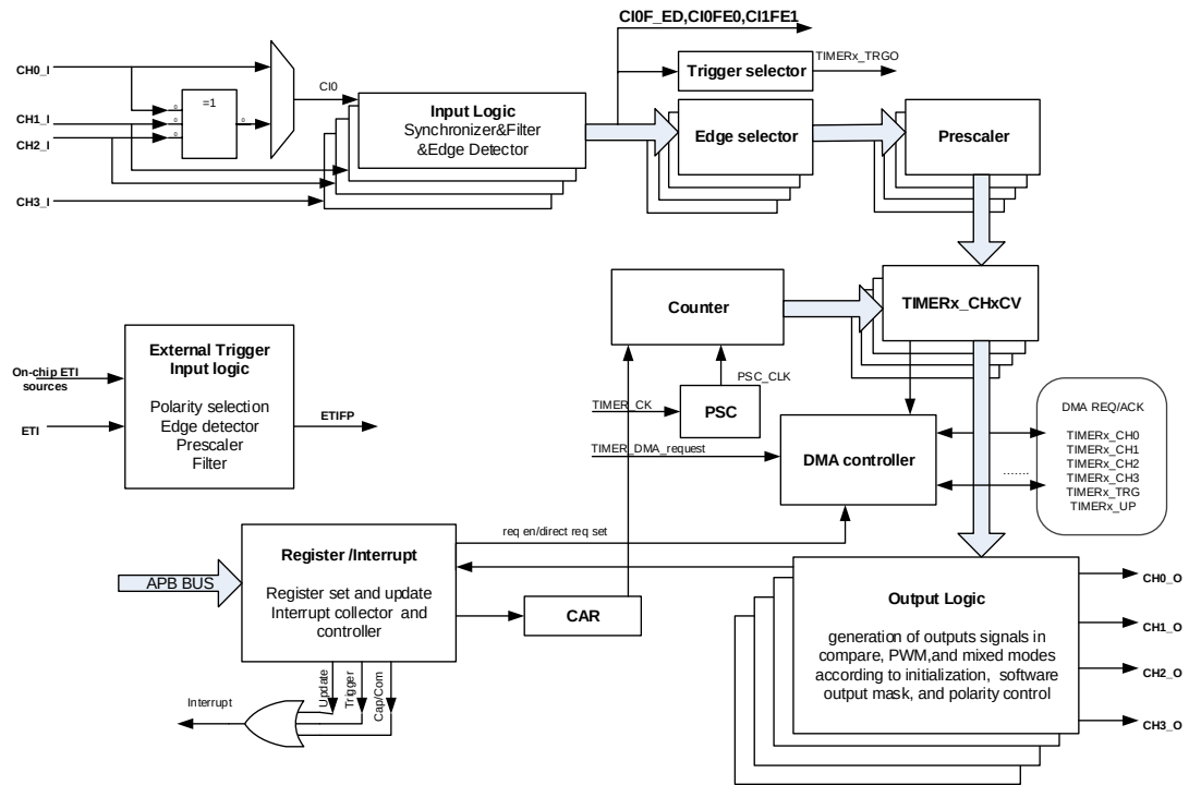
Figure 13-48. General Level 0 timer block diagram
