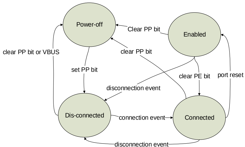
Figure 29-3. State transition diagram of host port
