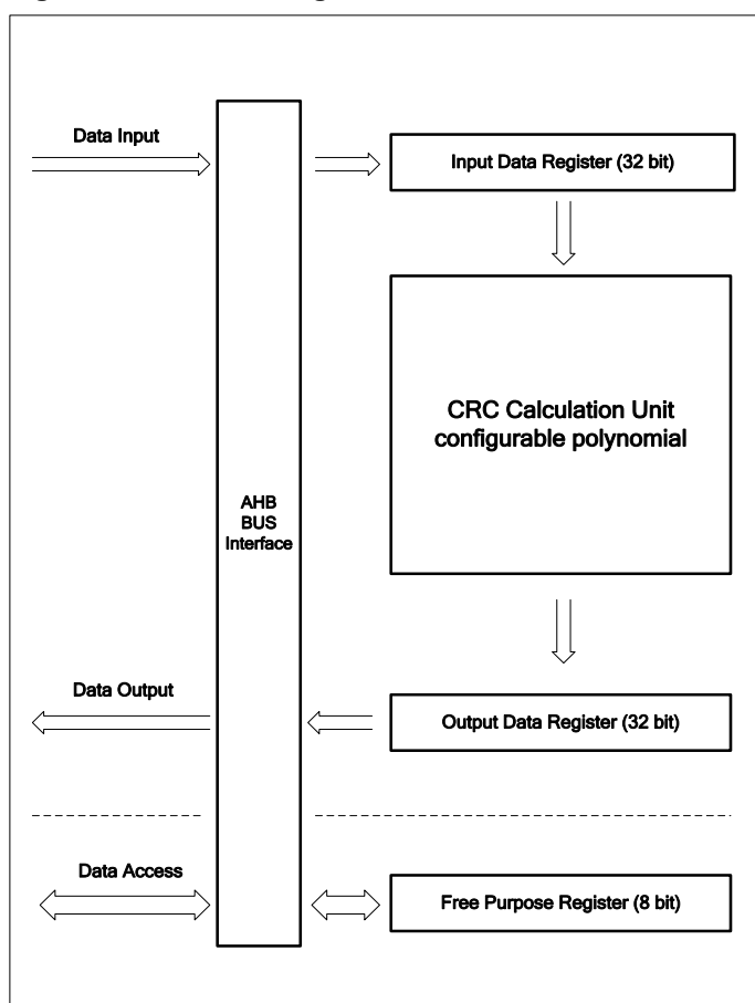
Figure 17-1. Block diagram of CRC calculation unit
