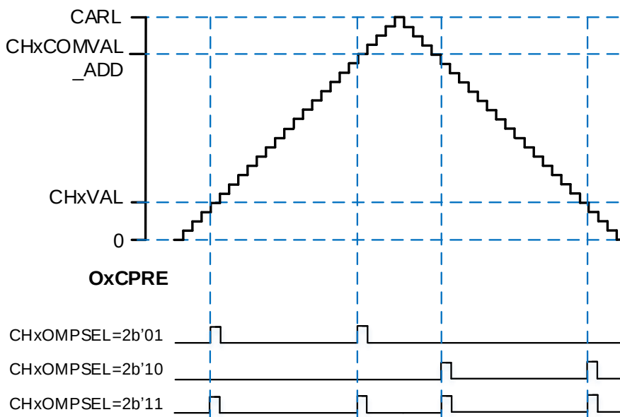
Figure 13-95. CHx_O output with a pulse in center-aligned mode (CHxOMPSEL≠2'b00)
