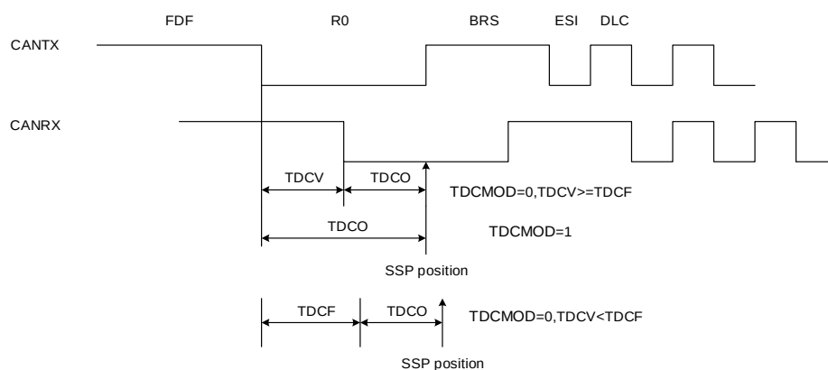
Figure 27-12. Transmitter Delay Measurement
