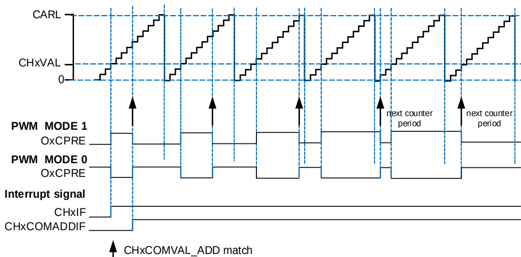
Figure 13-93. Channel x output PWM duty cycle changing with CHxCOMVAL_ADD
