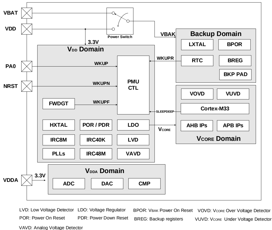
Figure 7-1. Power supply overview
