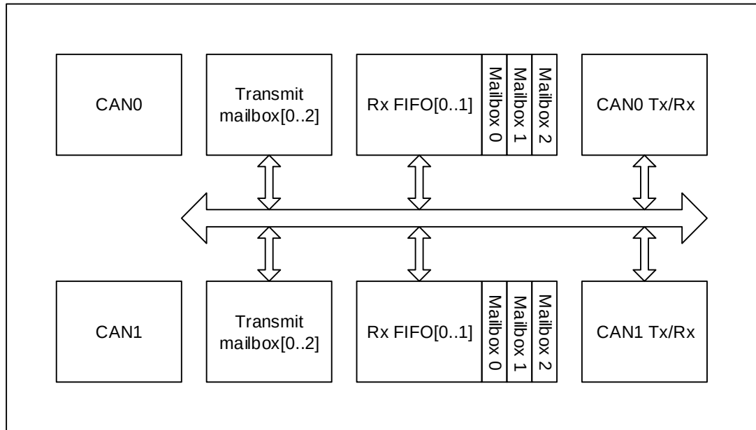
Figure 27-1. CAN module block diagram
