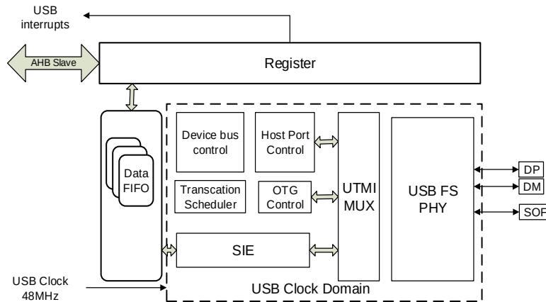
Figure 29-1. USBFS block diagram
