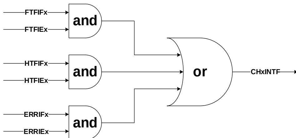
Figure 4-3. DMA interrupt logic
