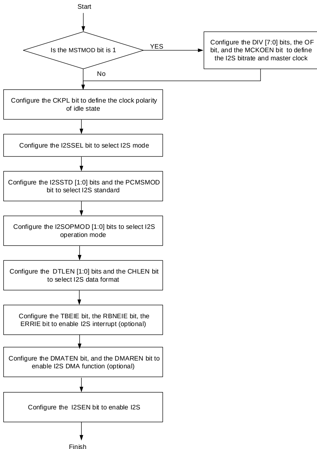
Figure 25-52. I2S initialization sequence
