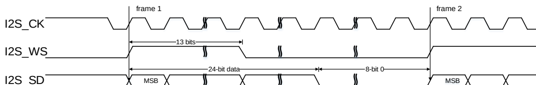
Figure 25-48. PCM standard long frame synchronization mode timing diagram (DTLEN=01, CHLEN=1, CKPL=1)
