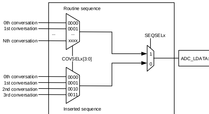
Figure 21-9. Data latch
