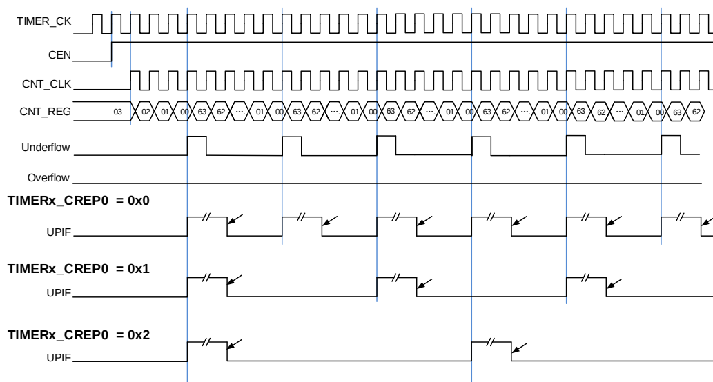
Figure 13-80. Repetition counter timing diagram of down counting mode
