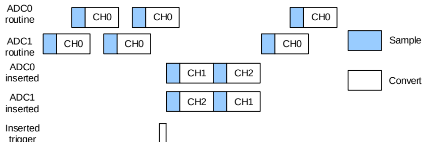
Figure 21-24. Follow-up single channel with inserted sequence CH1, CH2
