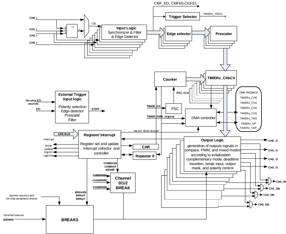
Figure 13-1. Advanced timer block diagram
