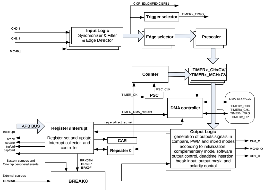
Figure 13-70. General level3 timer block diagram
