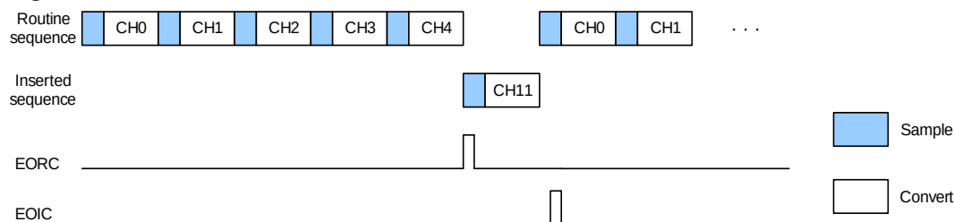
Figure 21-7. Auto-insertion, CNT = 1
