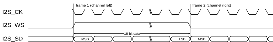
Figure 25-24. MSB justified standard timing diagram (DTLEN=00, CHLEN=0, CKPL=1)
