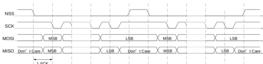
Figure 25-11. Timing diagram of NSS pulse with continuous transmit
