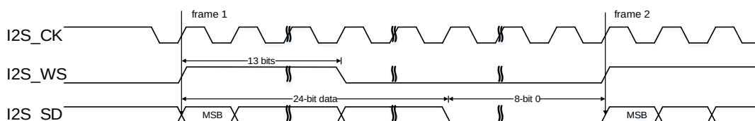
Figure 24-48. PCM standard long frame synchronization mode timing diagram (DTLEN=01, CHLEN=1, CKPL=1)
