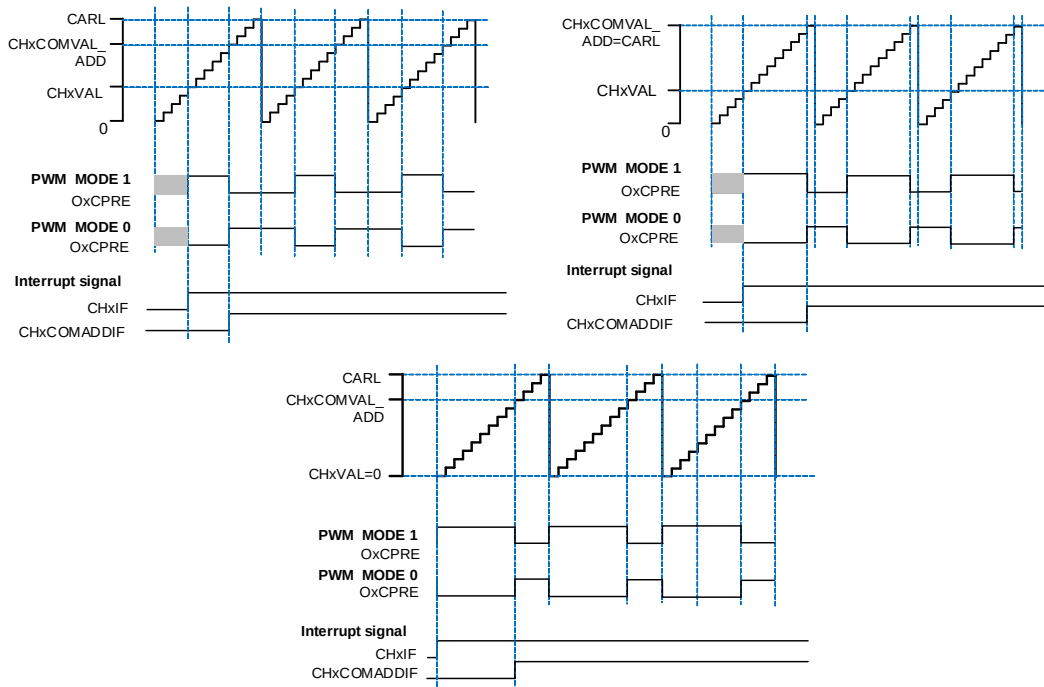
Figure 13-17. Channel x output PWM with ( CHxVAL < CHxCOMVAL\_ADD )
