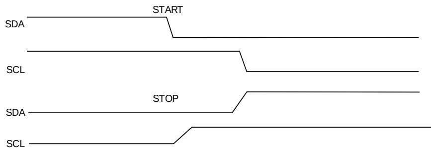
Figure 25-3. START and STOP signal
