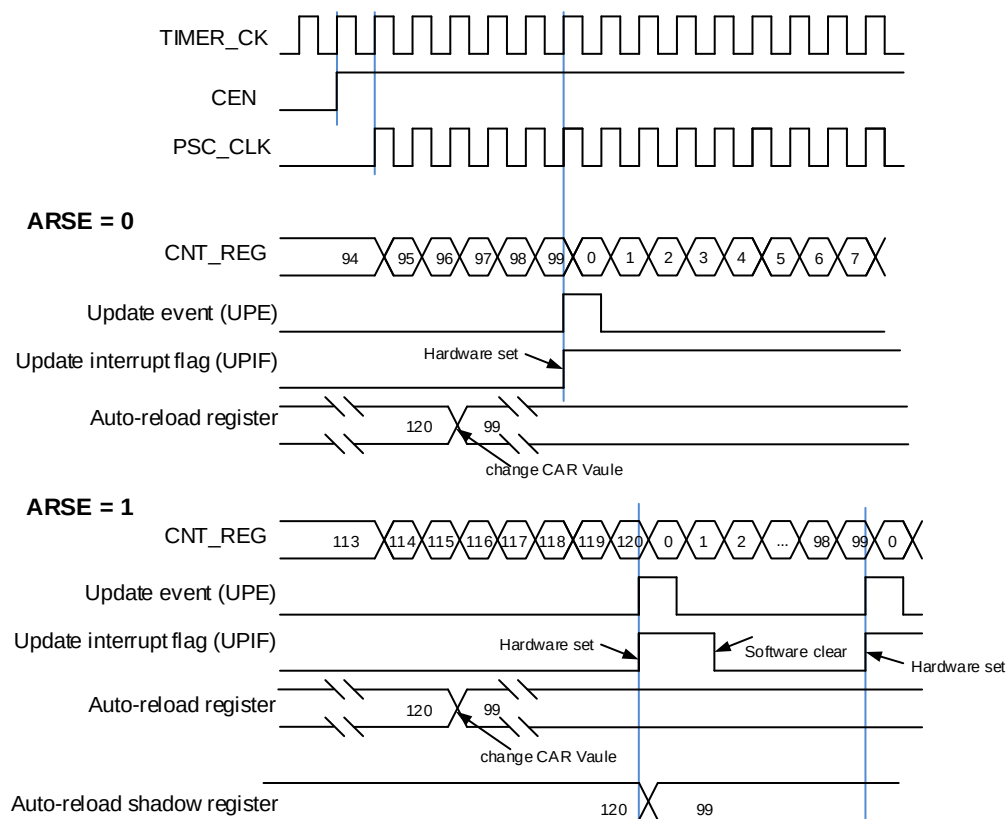
Figure 13-107. Timing chart of up counting mode, change TIMERx_CAR ongoing
