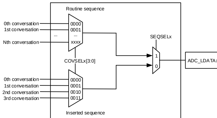
Figure 21-9. Data latch
