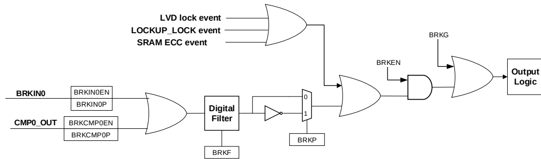
Figure 12-30. BREAK function logic diagram
