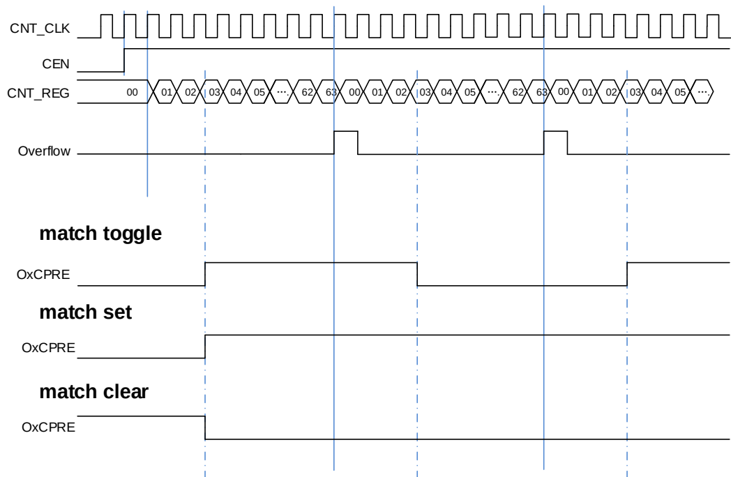
Figure 13-86. Output-compare in three modes
