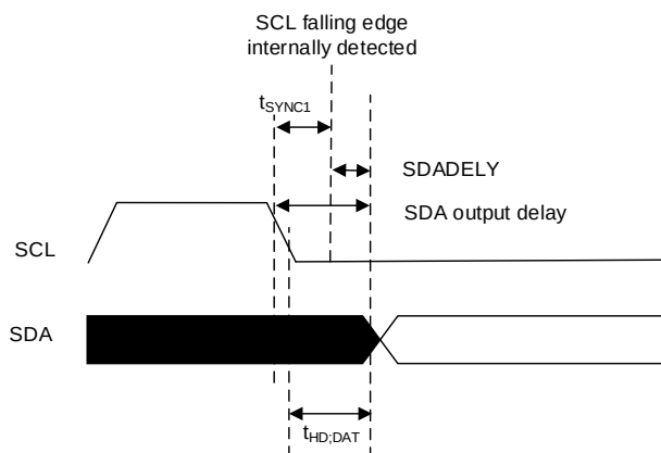
Figure 26-9. Data hold time
