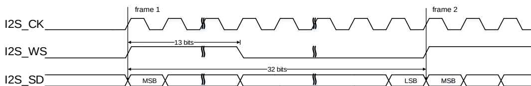
Figure 25-46. PCM standard long frame synchronization mode timing diagram (DTLEN=10, CHLEN=1, CKPL=1)
