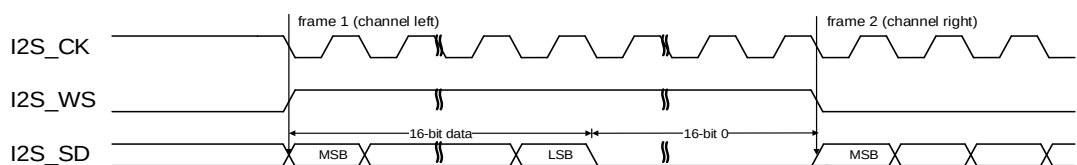
Figure 24-30. MSB justified standard timing diagram (DTLEN=00, CHLEN=1, CKPL=1)
