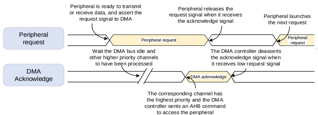
Figure 4-2. Handshake mechanism
