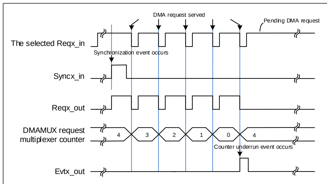
Figure 5-2. Synchronization mode
