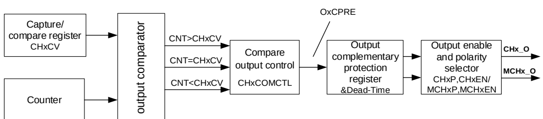
Figure 13-84. Output compare logic (when MCHxMSEL = 2'11, x=0)
