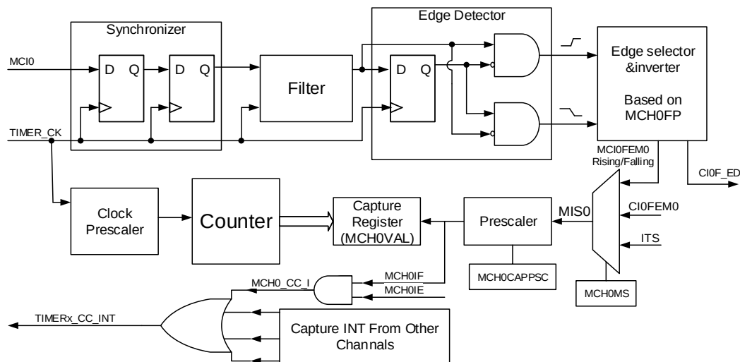
Figure 13-82. Input capture logic for multi mode channel 0
