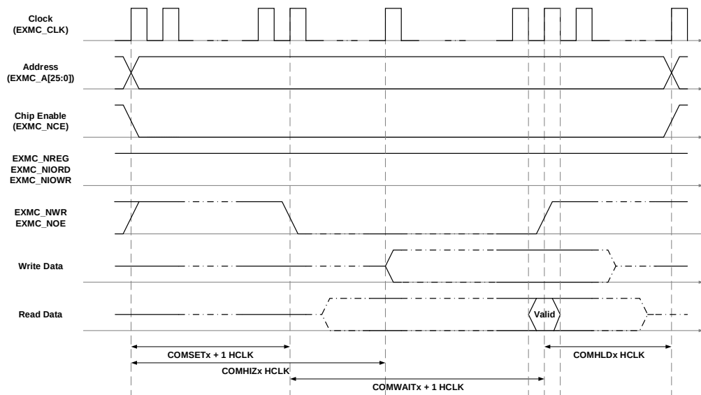
Figure 27-12. Access timing of common memory space of NAND flash Controller
