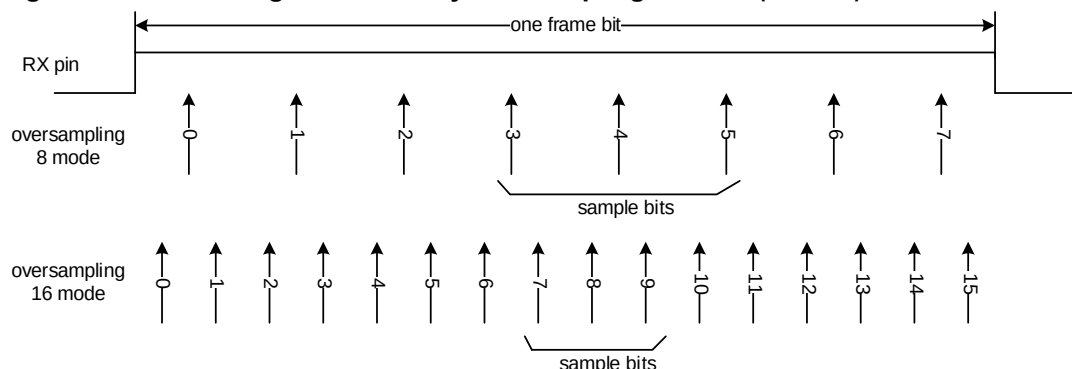
Figure 24-4. Receiving a frame bit by oversampling method (OSB=0)
