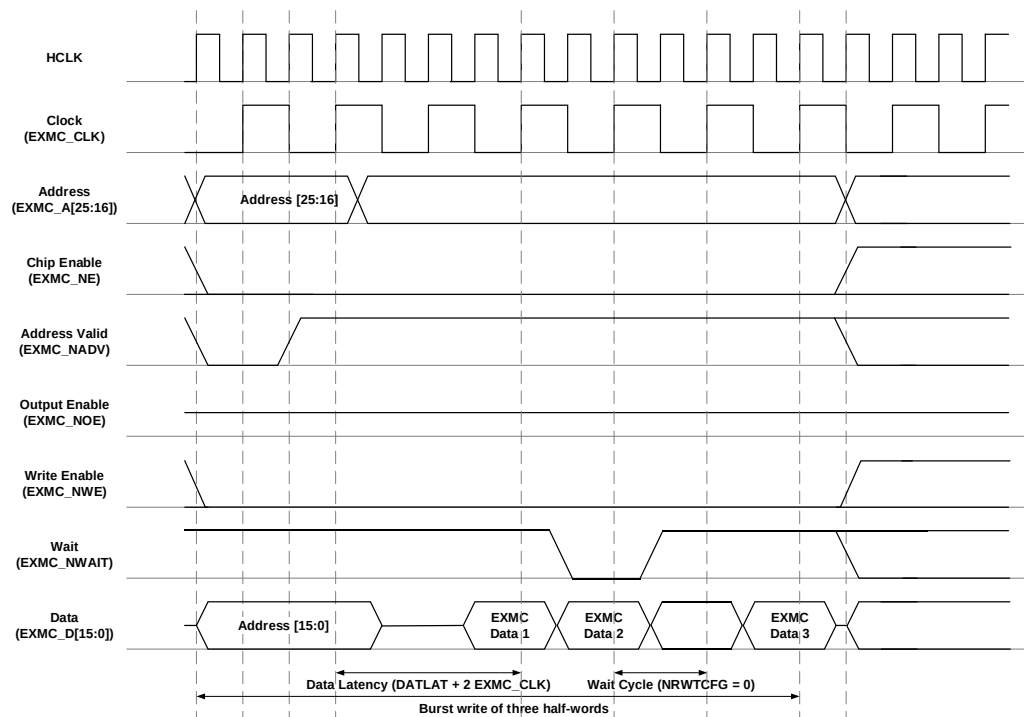
Figure 28-11. Write timing of synchronous multiplexed burst mode
