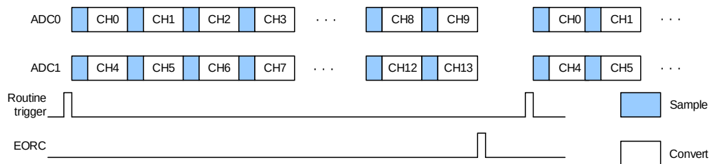
Figure 21-16. Routine parallel mode on 10 channels
