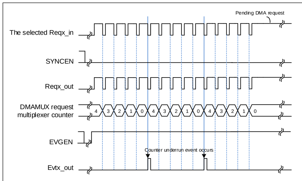
Figure 4-3. Event generation
