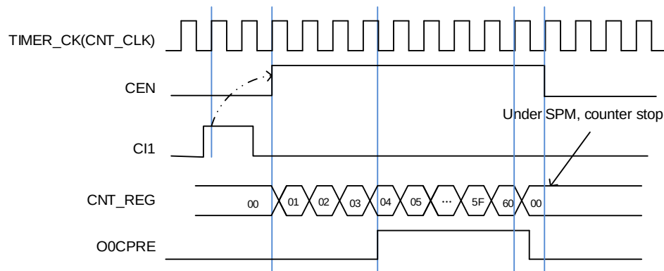
Figure 13-102. Single pulse mode TIMERx_CHxCV = 0x04 TIMERx_CAR=0x60
