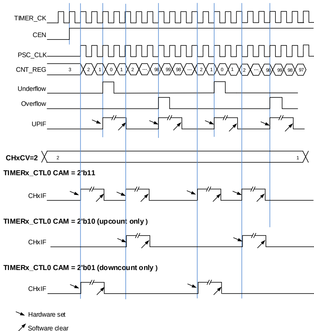
Figure 13-77. Timing diagram of center-aligned counting mode
