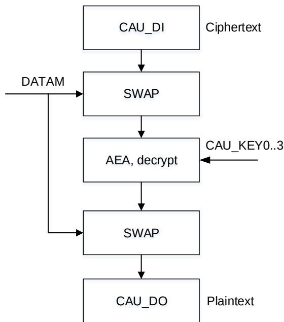
Figure 19-5. AES ECB decryption
