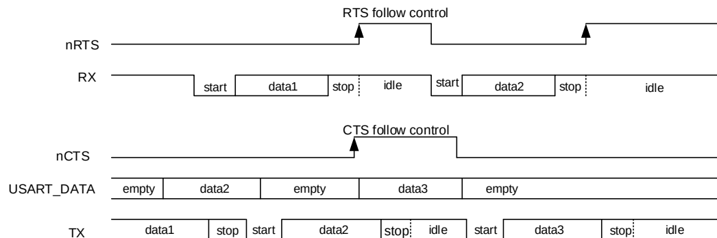
Figure 23-8. Hardware flow control
