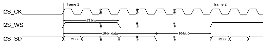
Figure 25-49. PCM standard long frame synchronization mode timing diagram (DTLEN=00, CHLEN=1, CKPL=0)
