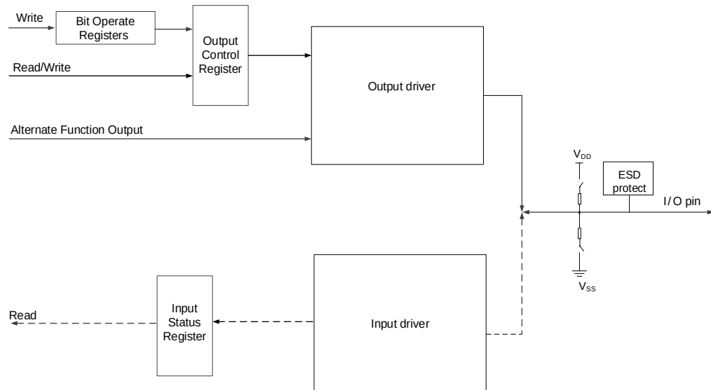
Figure 11-3. Basic structure of Output configuration
