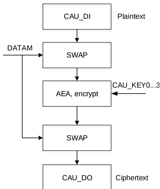
Figure 19-4. AES ECB encryption
