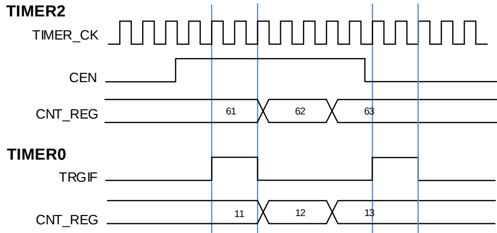
Figure 13-43. Pause mode of TIMER0 controlled by enable signal of TIMER2
