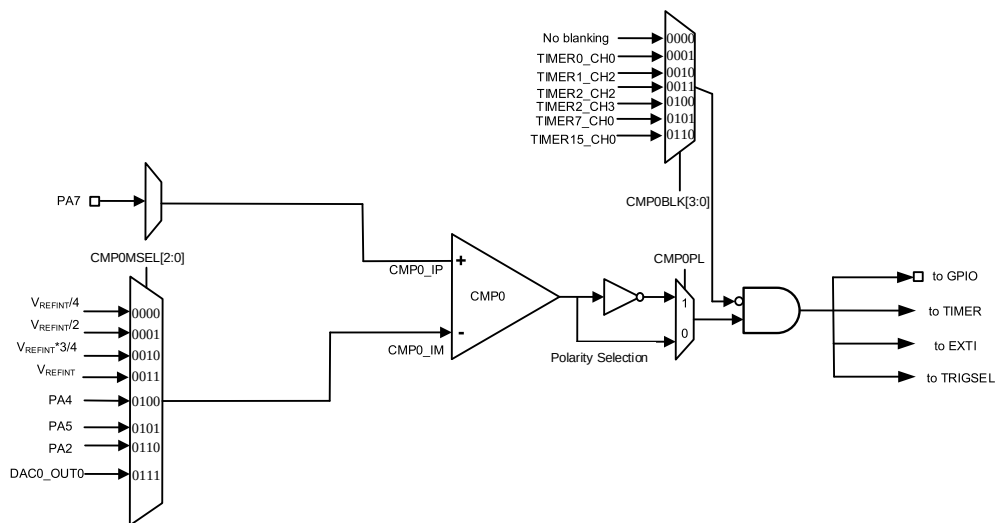
Figure 23-1. CMP block diagram
