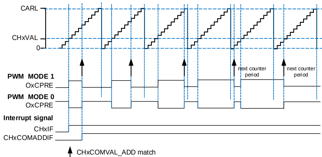
Figure 13-21. Channel x output PWM duty cycle changing with CHxCOMVAL_ADD
