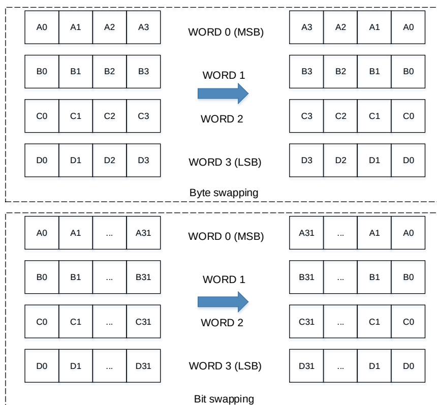
Figure 19-2. DATAM Byte swapping and Bit swapping
