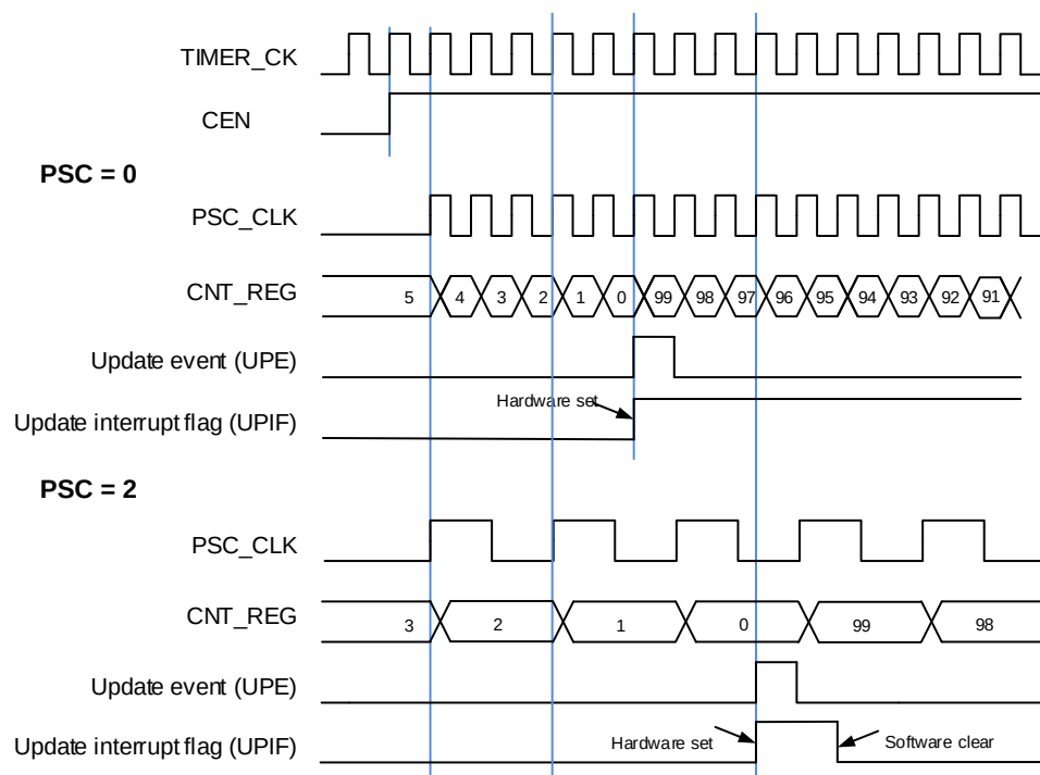
Figure 13-75. Timing diagram of down counting mode, \text{PSC}=0/2
