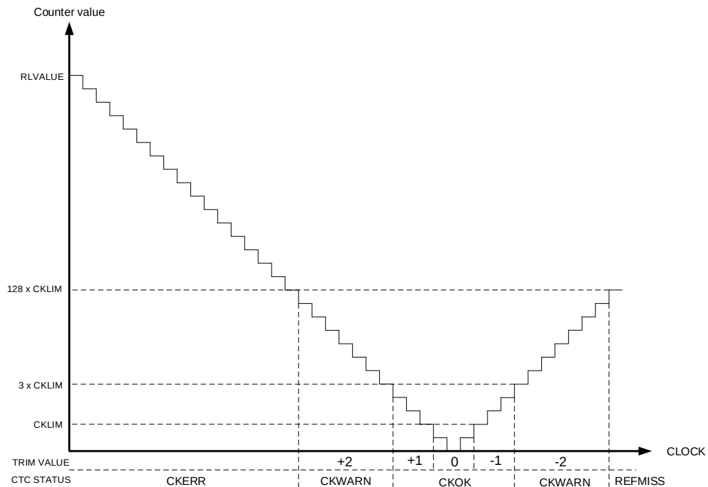
Figure 10-2. CTC trim counter
