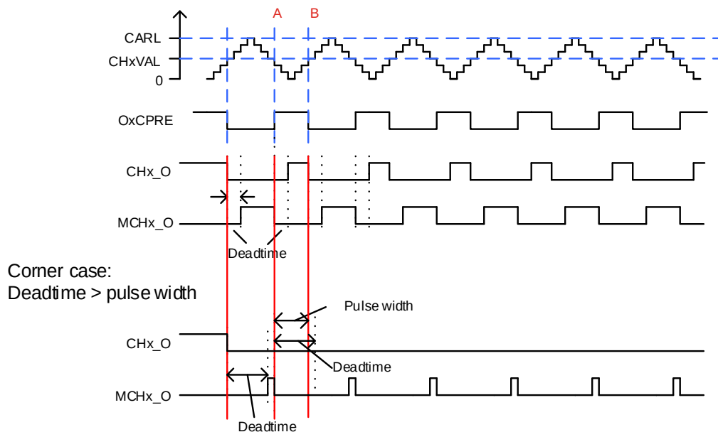
Figure 13-96. Complementary output with dead-time insertion
