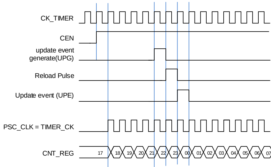
Figure 13-2. Normal mode, internal clock divided by 1
