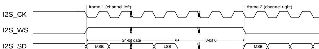
Figure 25-28. MSB justified standard timing diagram (DTLEN=01, CHLEN=1, CKPL=1)
