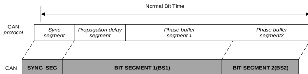
Figure 27-11. The bit time
