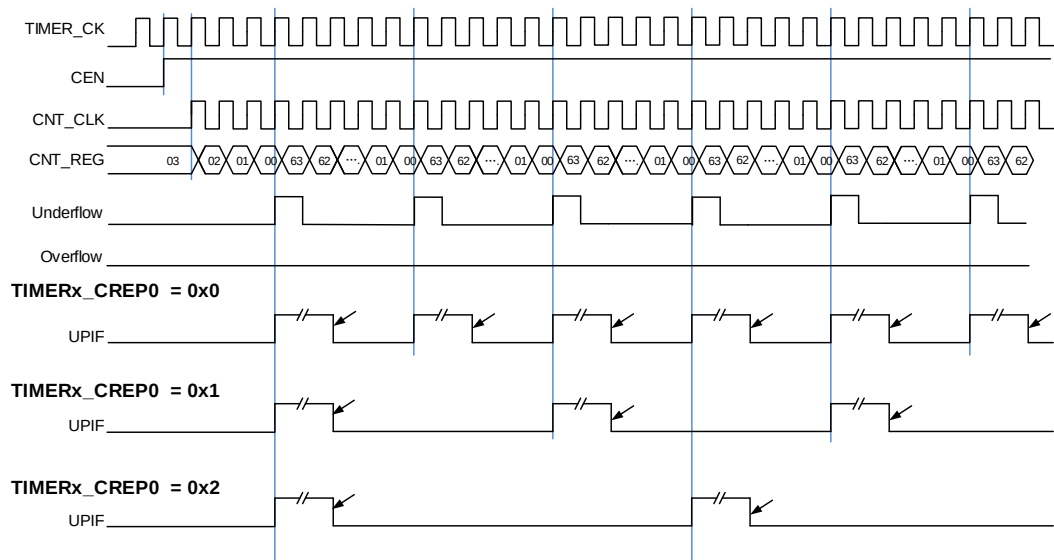
Figure 13-11. Repetition counter timing diagram of down counting mode
