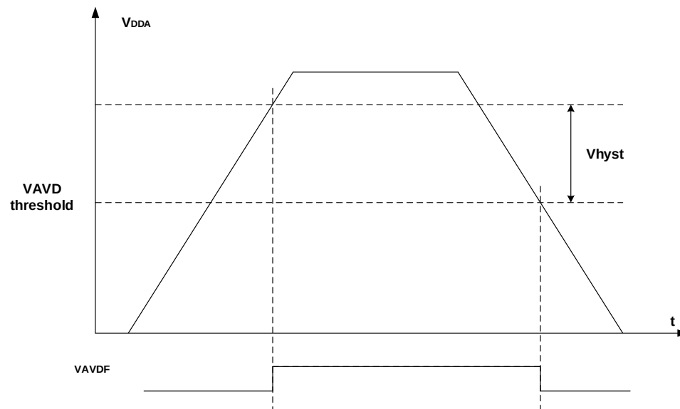
Figure 7-4. Waveform of the VAVD threshold
