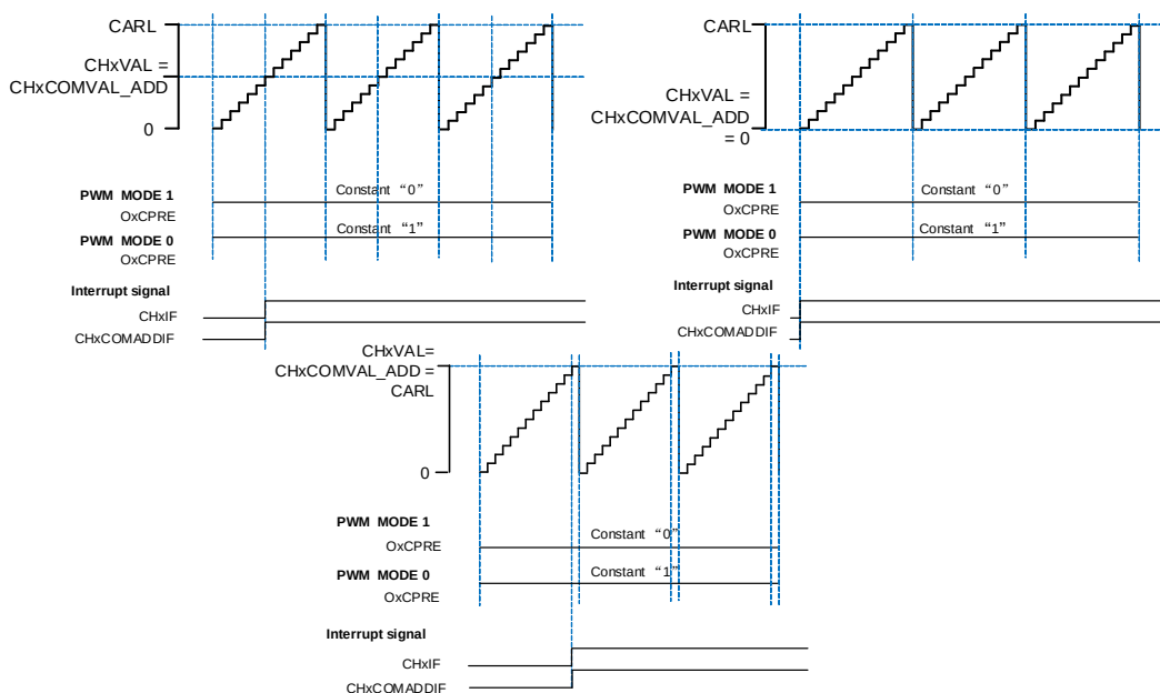
Figure 13-90. Channel x output PWM with ( CHxVAL = CHxCOMVAL\_ADD )
