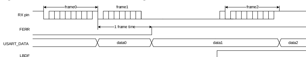
Figure 24-10. Break frame occurs during a frame
