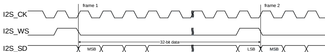
Figure 25-38. PCM standard short frame synchronization mode timing diagram (DTLEN=10, CHLEN=1, CKPL=1)
