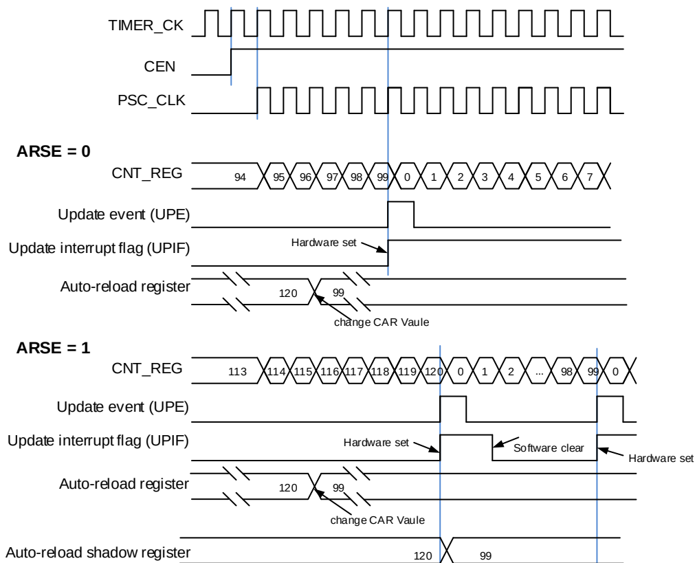
Figure 12-52. Timing chart of up counting, change TIMERx_CAR ongoing
