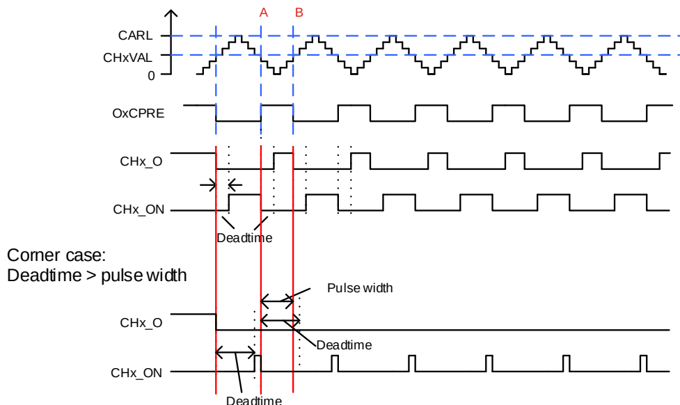
Figure 13-28. Complementary output with dead time insertion
