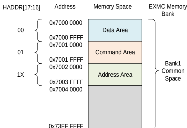
Figure 28-5. Diagram of bank1 common space
