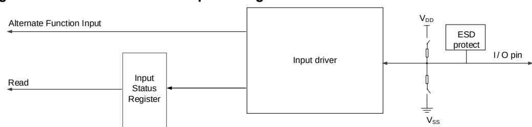
Figure 11-2. Basic structure of Input configuration
