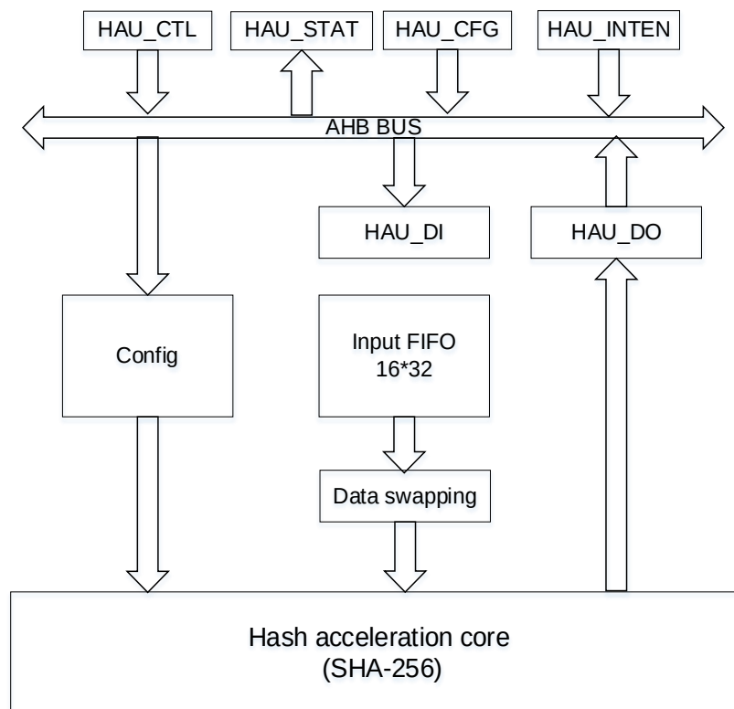
Figure 20-3. HAU block diagram
