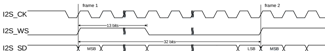
Figure 25-46. PCM standard long frame synchronization mode timing diagram (DTLEN=10, CHLEN=1, CKPL=1)
