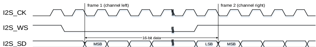
Figure 25-15. I2S Philips standard timing diagram (DTLEN=00, CHLEN=0, CKPL=0)
