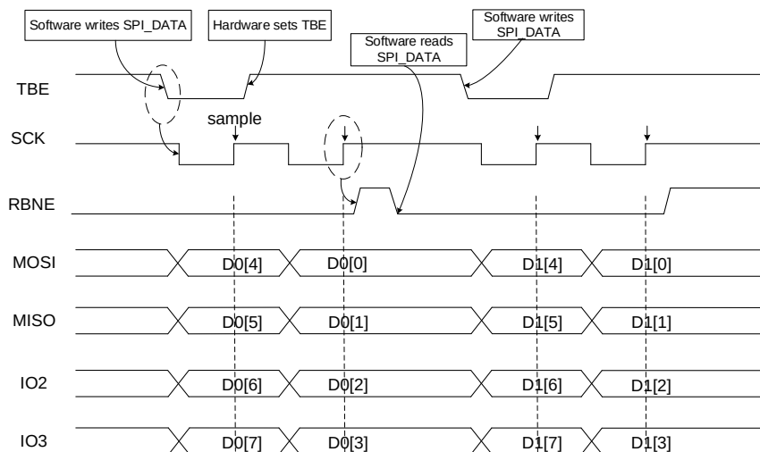
Figure 25-13. Timing diagram of quad read operation in Quad-SPI mode
