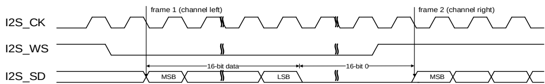
Figure 24-21. I2S Philips standard timing diagram (DTLEN=00, CHLEN=1, CKPL=0)
