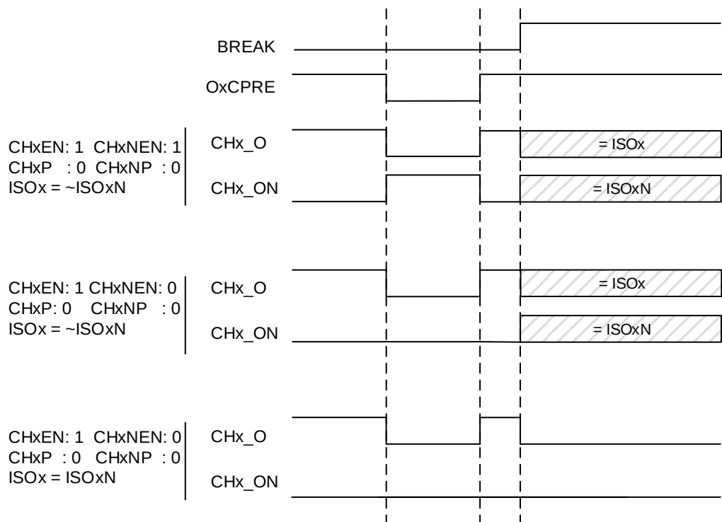
Figure 13-31. Output behavior of the channel in response to BREAK (the break input high active and IOS=1)
