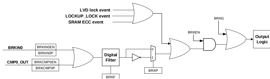
Figure 13-97. BREAK function logic diagram
