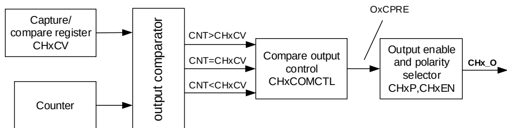
Figure 13-57. Output compare logic (x=0,1,2,3)
