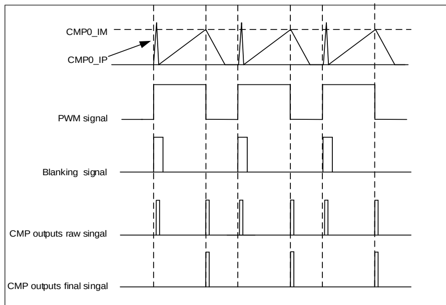
Figure 23-3. The CMP outputs signal blanking
