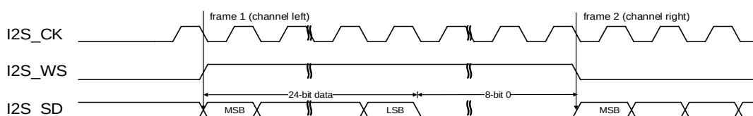
Figure 25-27. MSB justified standard timing diagram (DTLEN=01, CHLEN=1, CKPL=0)
