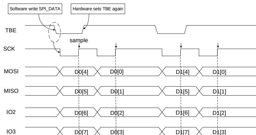
Figure 25-12. Timing diagram of quad write operation in Quad-SPI mode
