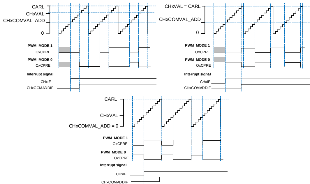
Figure 13-91. Channel x output PWM with (CHxVAL > CHxCOMVAL_ADD)
