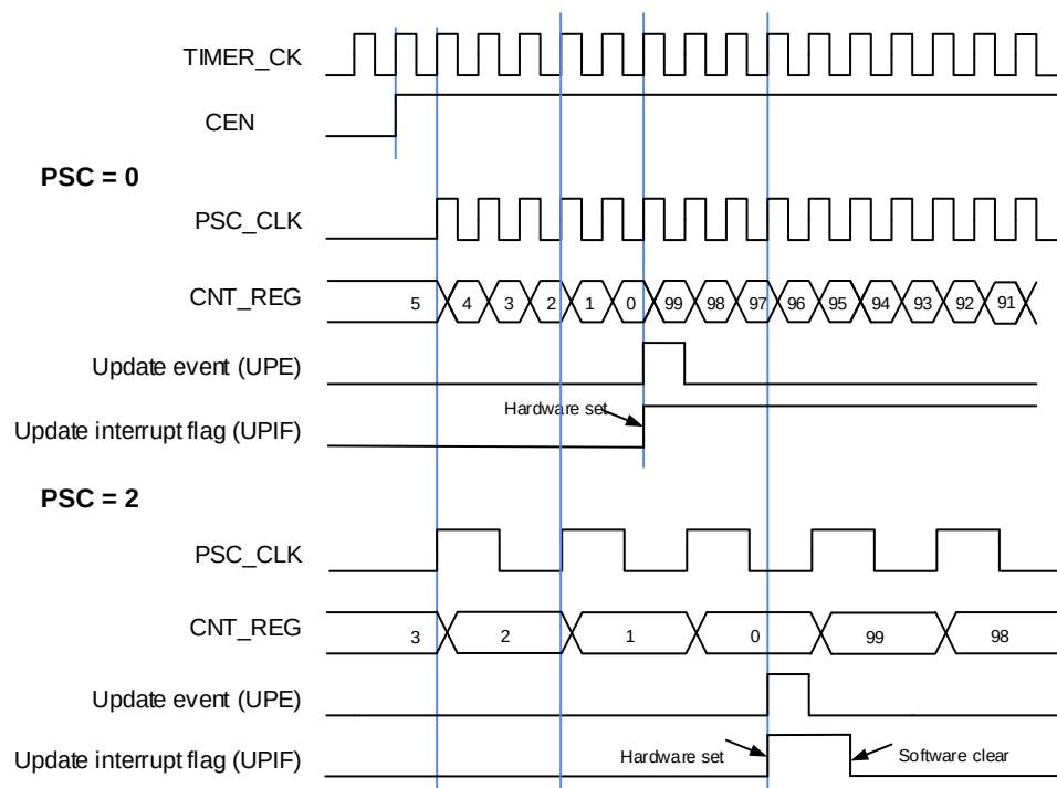
Figure 12-75. Timing diagram of down counting mode, \text{PSC}=0/2
