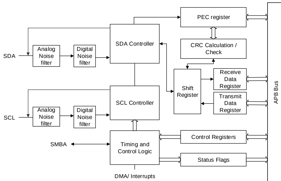
Figure 26-1. I2C module block diagram
