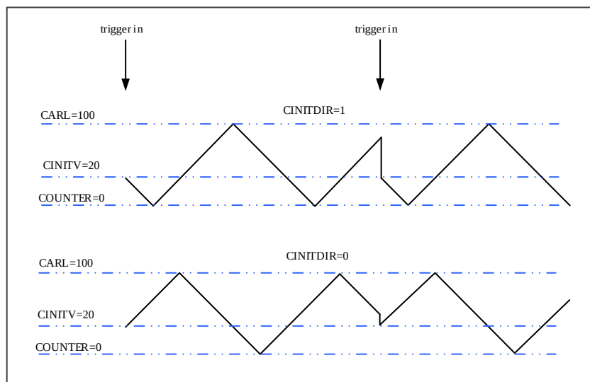
Figure 13-47. Counting direction in CINITDIR is 0 or 1
