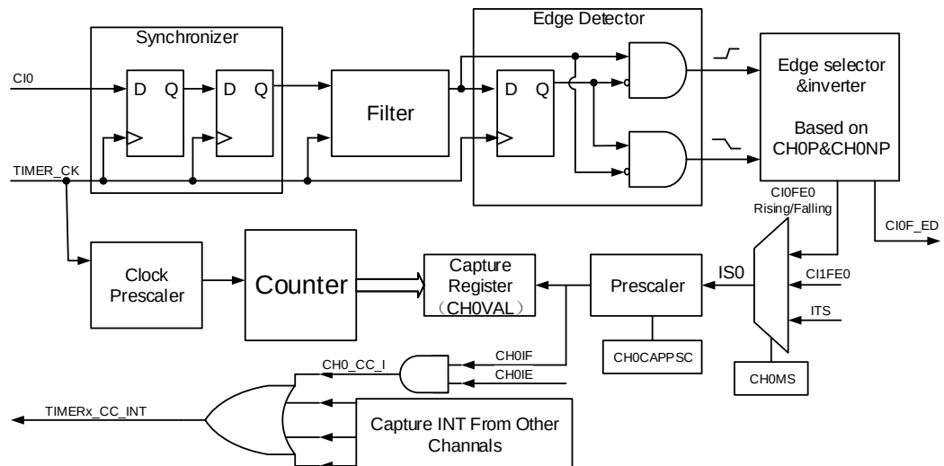
Figure 13-12. Input capture logic for channel 0
