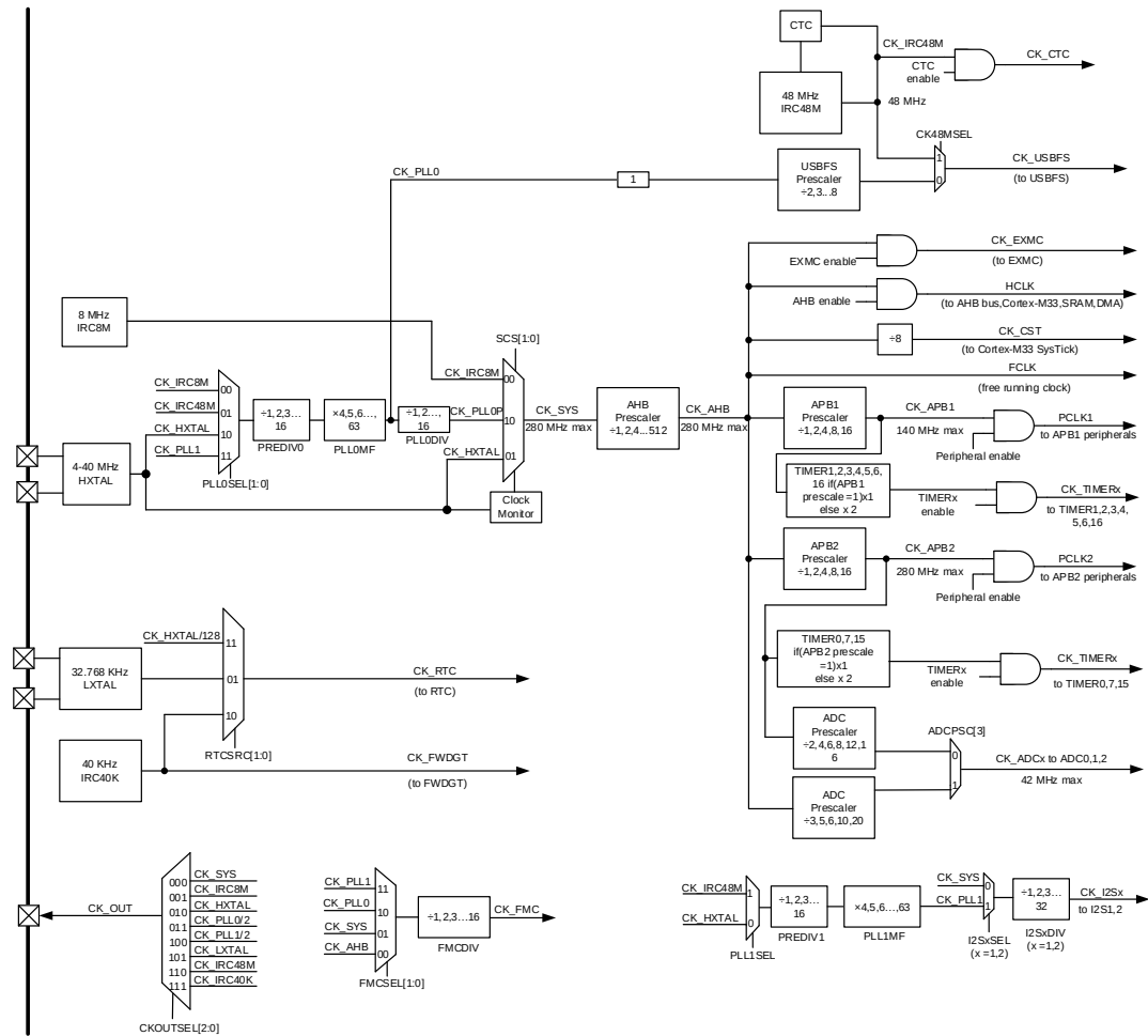
Figure 8-3. Clock tree (for GD32F505xx)
