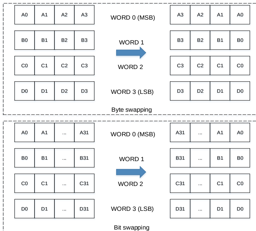
Figure 20-2. DATAM Byte swapping and Bit swapping
