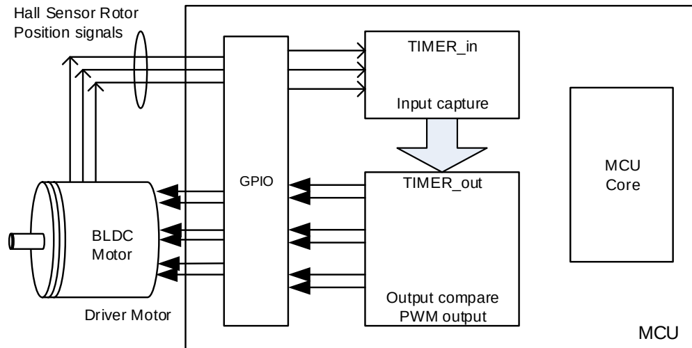
Figure 13-35. Hall sensor is used for BLDC motor
