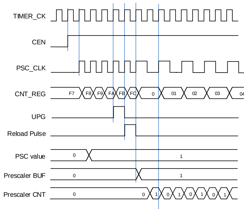
Figure 13-3. Counter timing diagram with prescaler division change from 1 to 2
