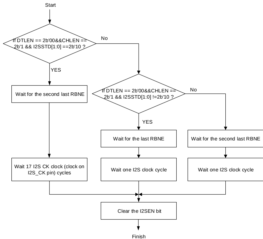
Figure 25-53. I2S master reception disabling sequence
