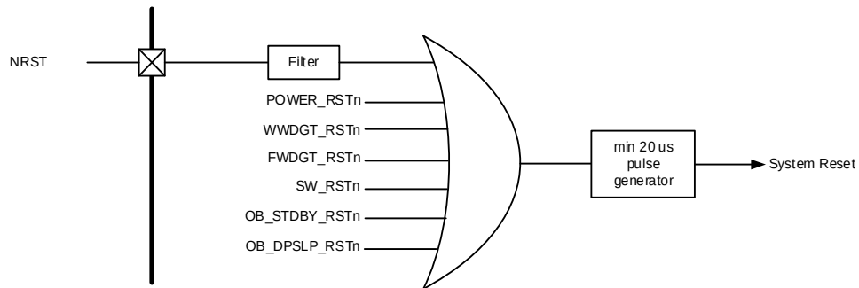
Figure 9-1. The system reset circuit
