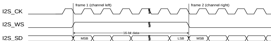
Figure 25-23. MSB justified standard timing diagram (DTLEN=00, CHLEN=0, CKPL=0)
