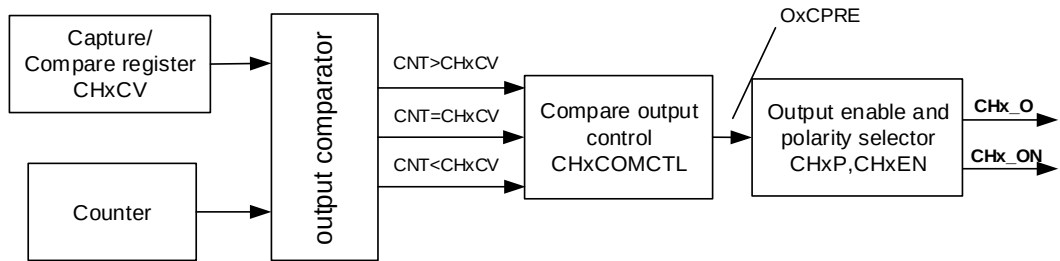
Figure 13-13. Output compare logic
