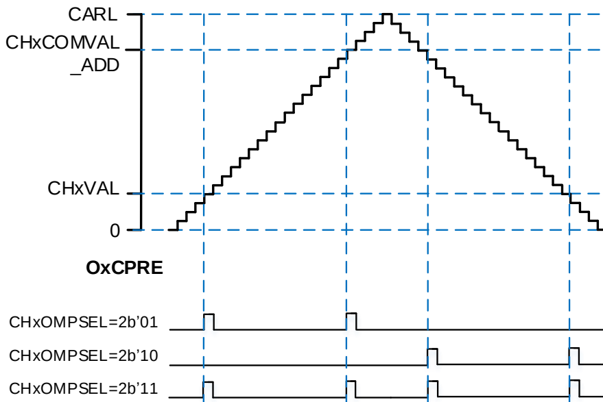
Figure 13-27. CHx_O output with a pulse in center-aligned mode (CHxOMPSEL≠2'b00)
