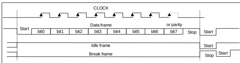
Figure 24-2. USART character frame (8 bits data and 1 stop bit)
