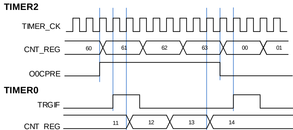
Figure 13-44. Pause mode of TIMER0 controlled by O0CPRE signal of TIMER2
