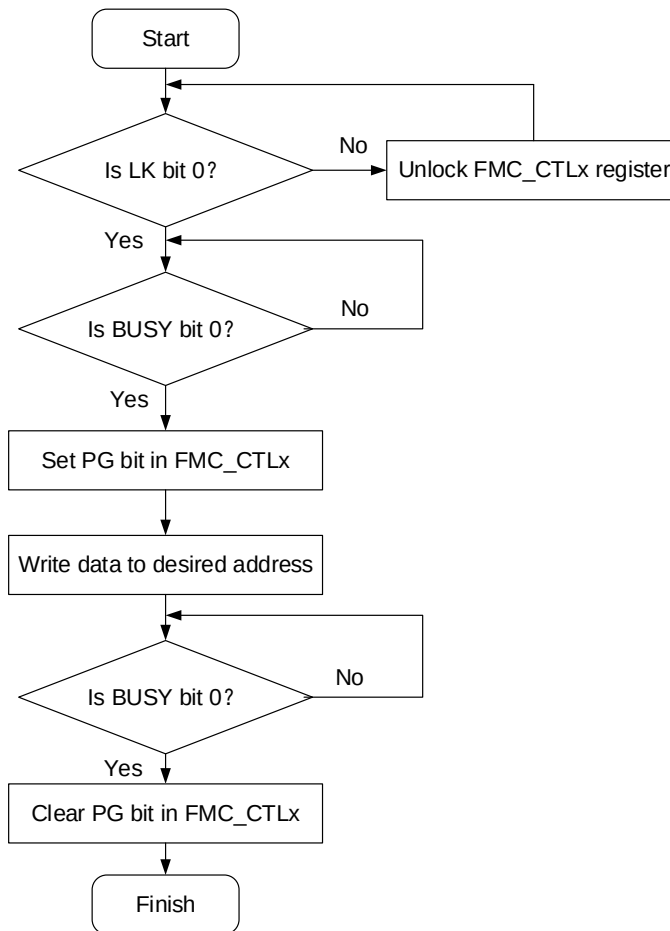
Figure 6-3. Process of word program operation
