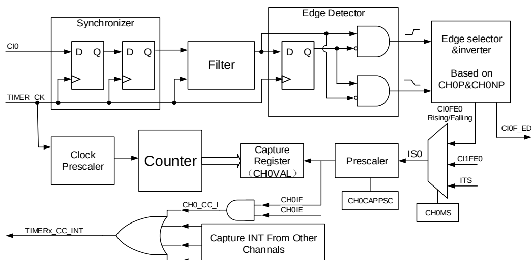
Figure 13-56. Input capture logic
