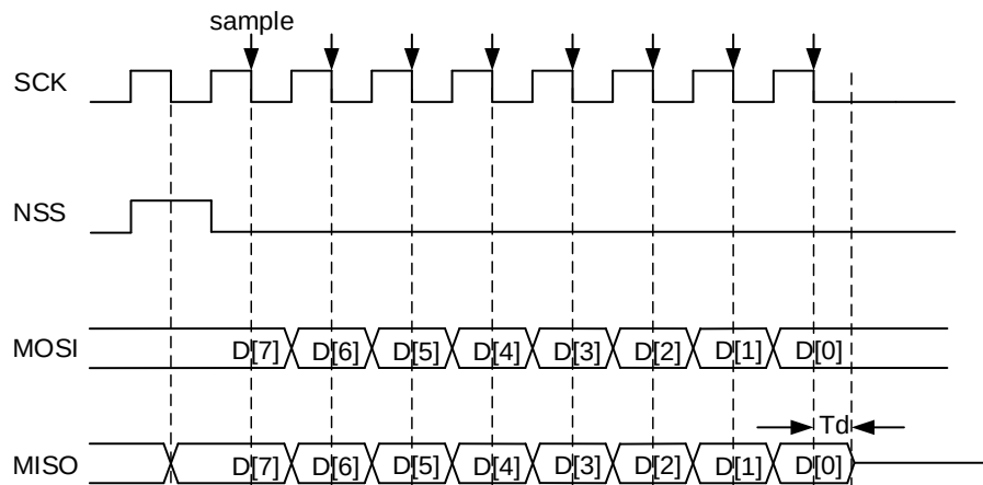
Figure 25-10. Timing diagram of TI slave mode
