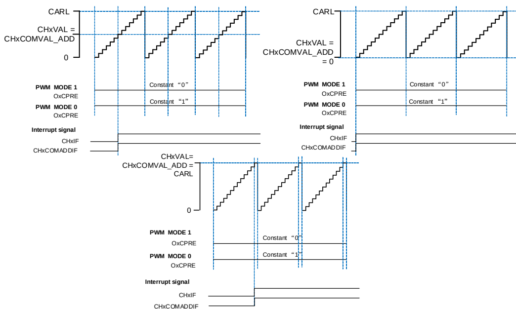
Figure 13-18. Channel x output PWM with ( CHxVAL = CHxCOMVAL\_ADD )
