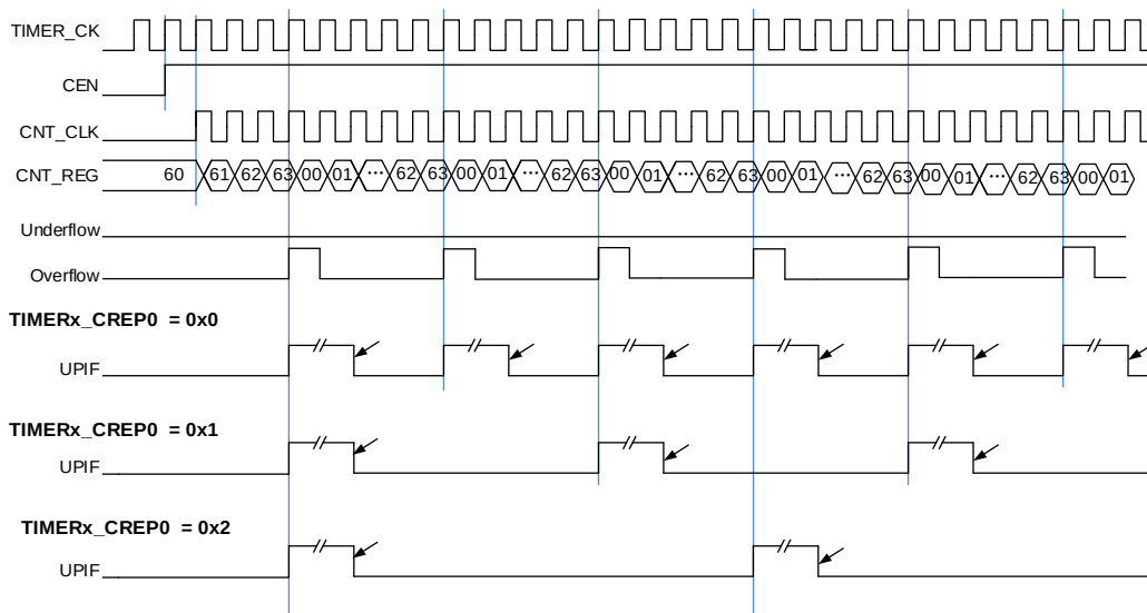
Figure 13-79. Repetition counter timing diagram of up counting mode
