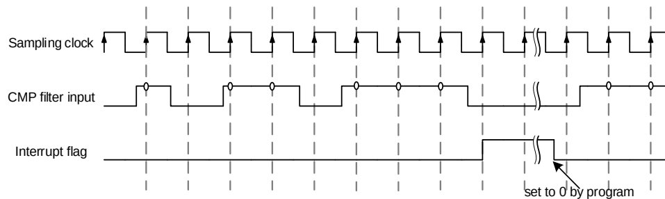
Figure 23-4. CMP noise filter and interrupt operation
