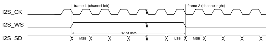
Figure 25-25. MSB justified standard timing diagram (DTLEN=10, CHLEN=1, CKPL=0)
