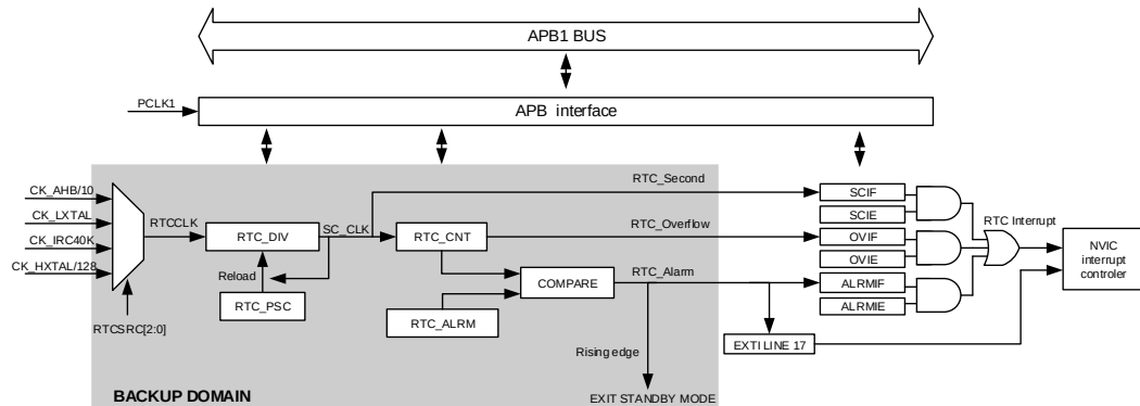
Figure 13-1. Block diagram of RTC
