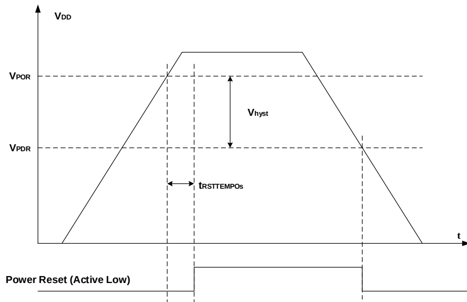
Figure 7-2. Waveform of the POR/PDR
