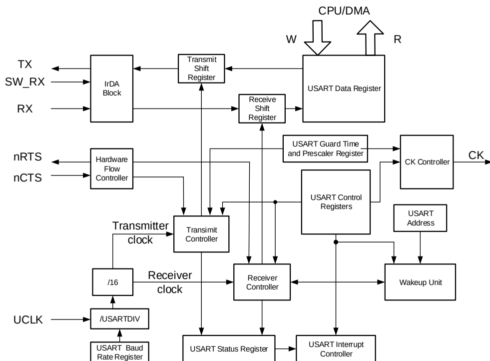
Figure 24-1. USART module block diagram
