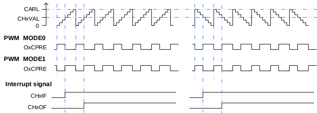
Figure 13-60. Timing chart of CAPWM
