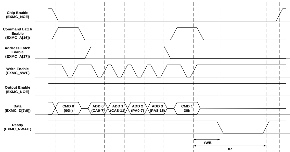
Figure 28-13. Access to none "NCE don't care" NAND Flash
