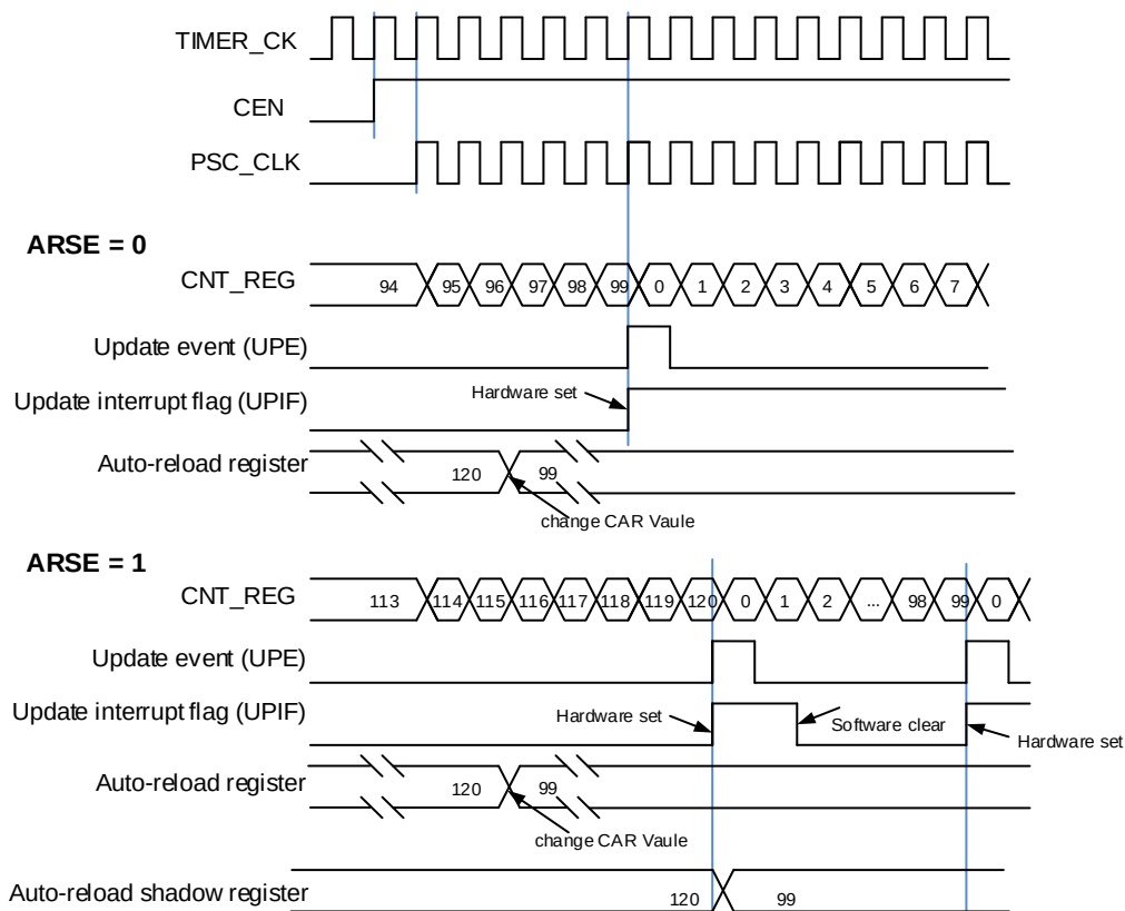
Figure 13-52. Timing chart of up counting, change TIMEx_CAR ongoing
