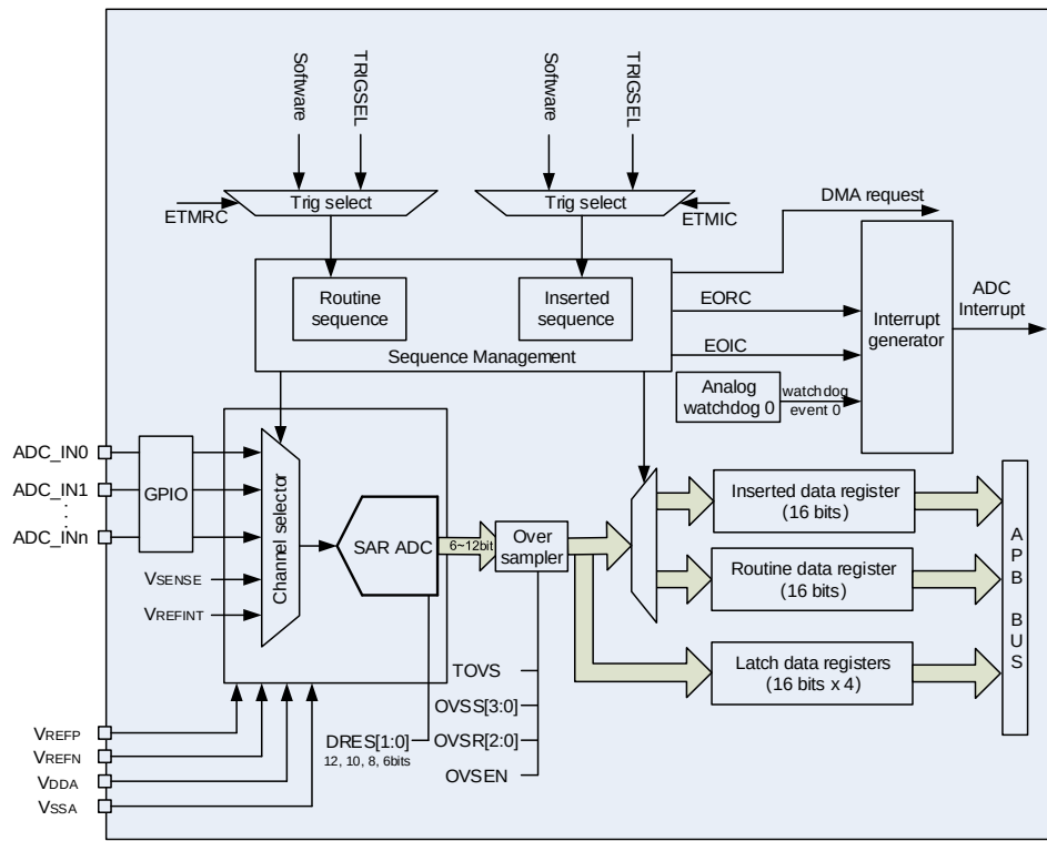
Figure 21-1. ADC module block diagram
