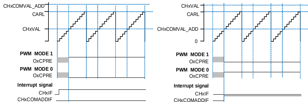
Figure 13-92. Channel x output PWM with CHxVAL or CHxCOMVAL_ADD exceeds CARL
