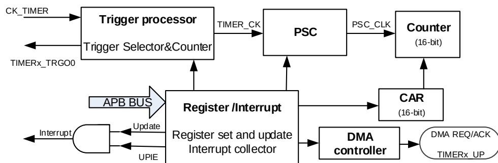
Figure 13-103. Basic timer block diagram
