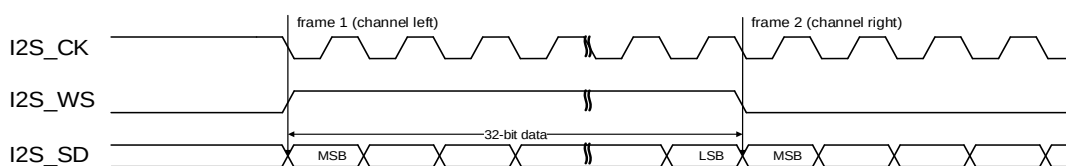
Figure 25-26. MSB justified standard timing diagram (DTLEN=10, CHLEN=1, CKPL=1)
