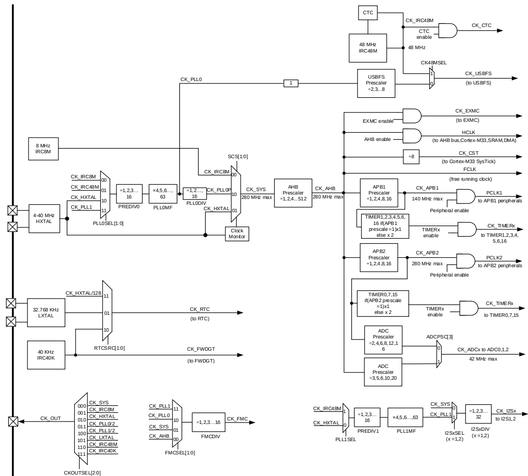
Figure 9-4. Clock tree (for GD32F505xx)
