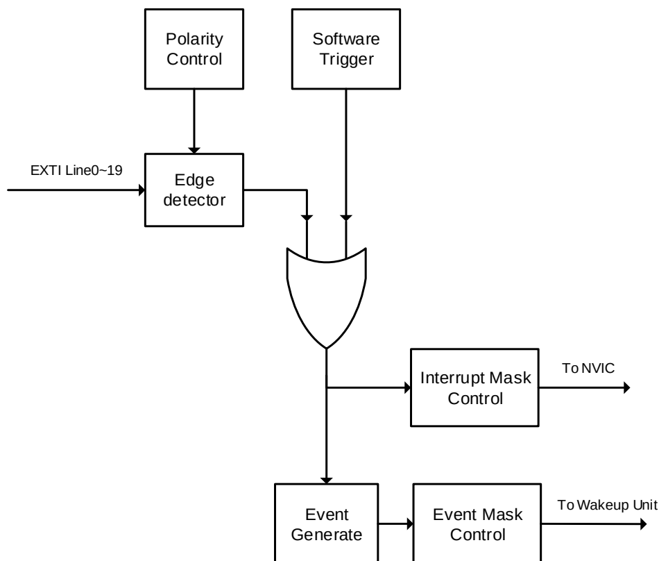
Figure 3-1. Block diagram of EXTI
