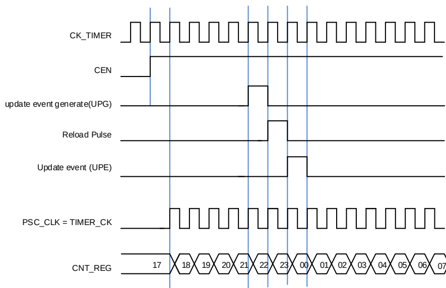
Figure 13-49. Normal mode, internal clock divided by 1
