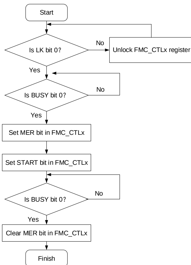
Figure 6-2. Process of mass erase operation
