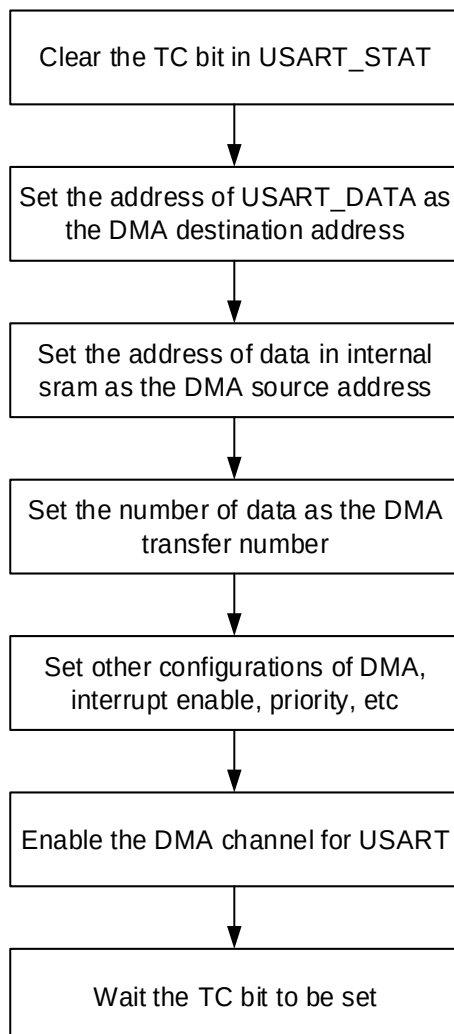
Figure 24-5. Configuration step when using DMA for USART transmission
