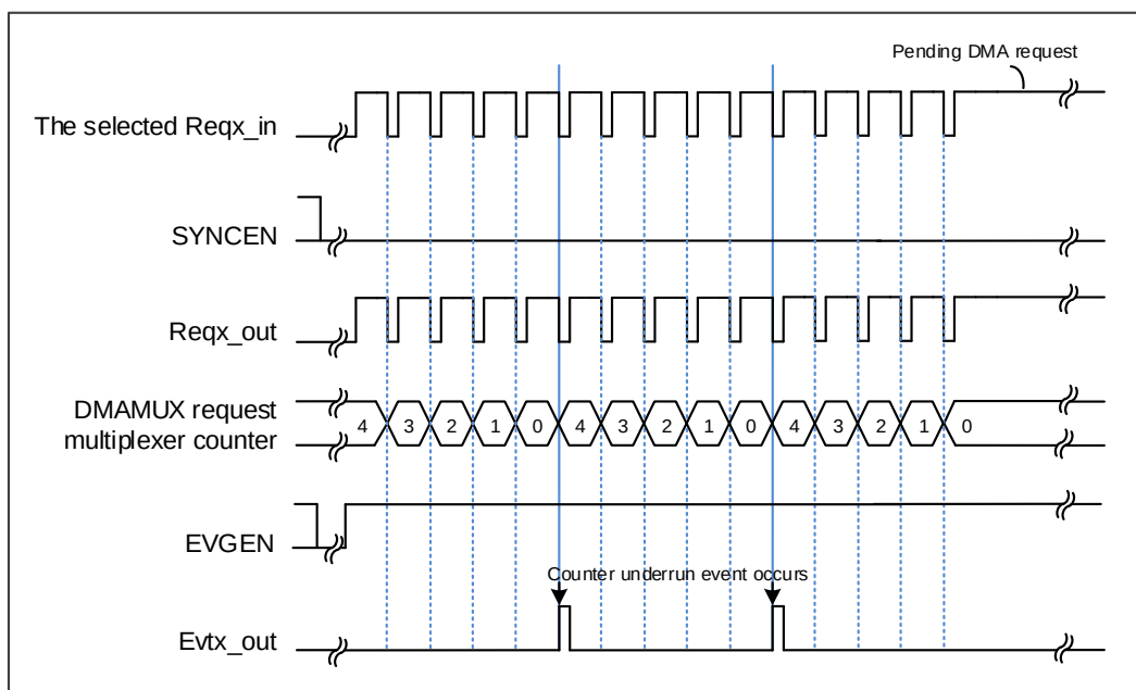
Figure 5-3. Event generation
