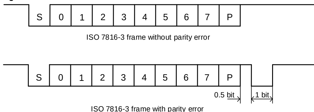
Figure 24-15. ISO7816-3 frame format
