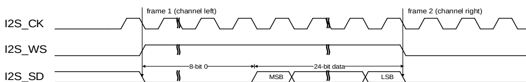
Figure 24-31. LSB justified standard timing diagram (DTLEN=01, CHLEN=1, CKPL=0)
