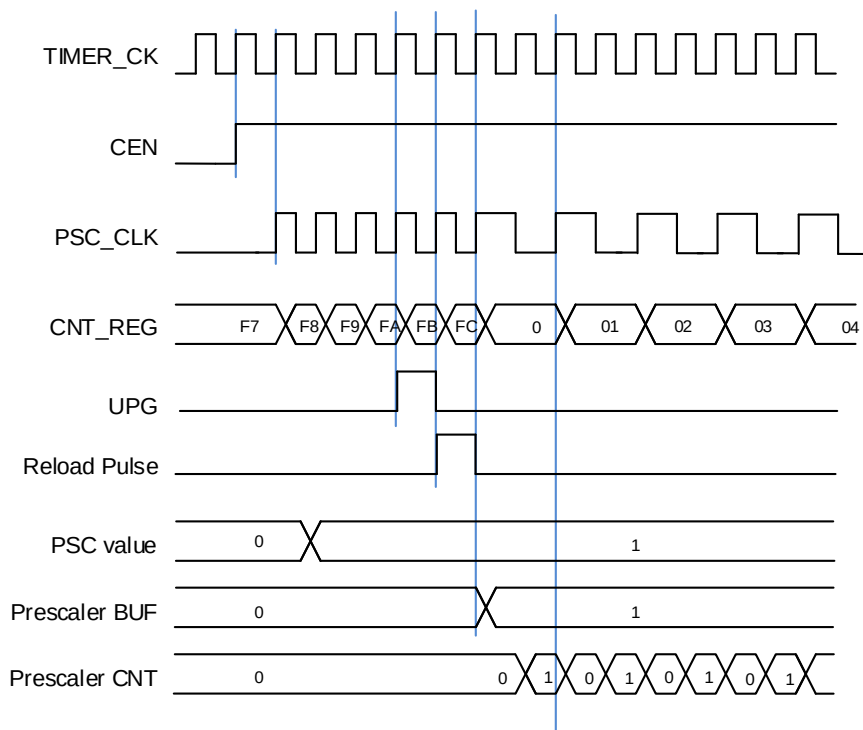
Figure 13-105. Counter timing diagram with prescaler division change from 1 to 2
