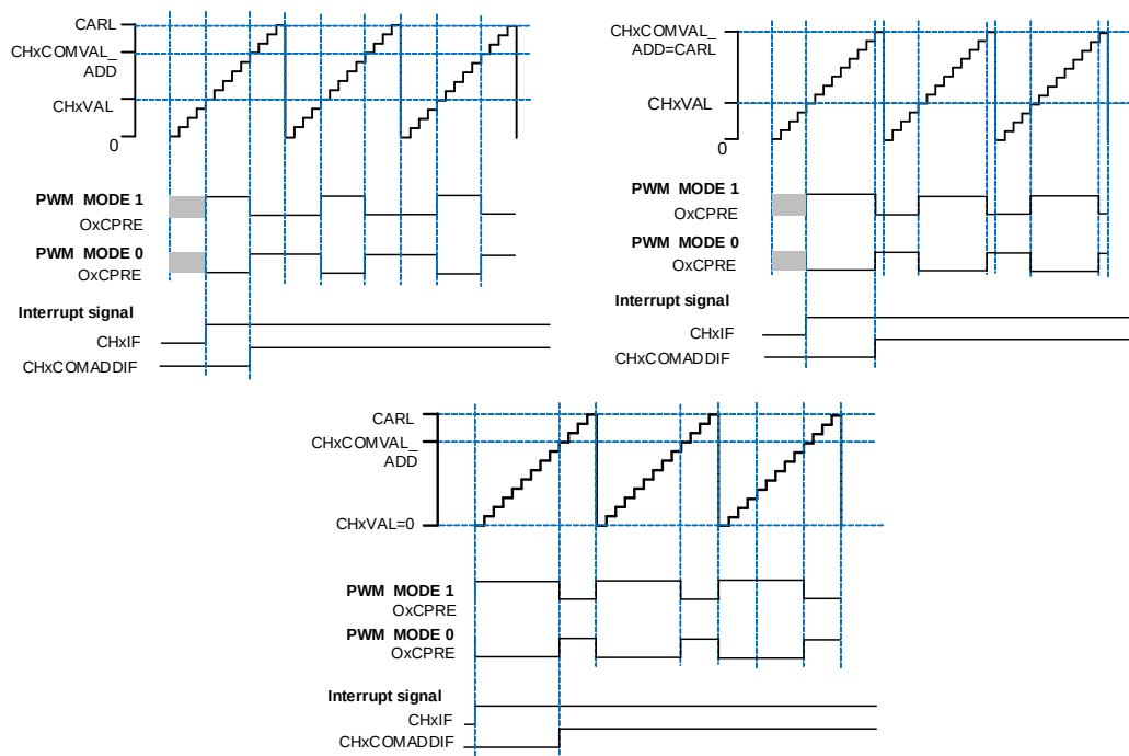
Figure 13-89. Channel x output PWM with ( CHxVAL < CHxCOMVAL\_ADD )
