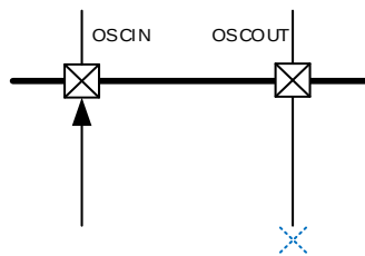
Figure 9-6. HXTAL clock source in bypass mode
