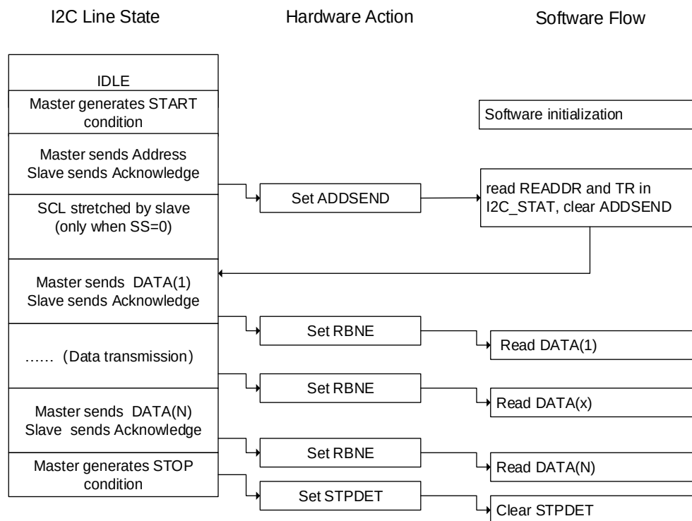
Figure 26-16. Programming model for slave receiving
