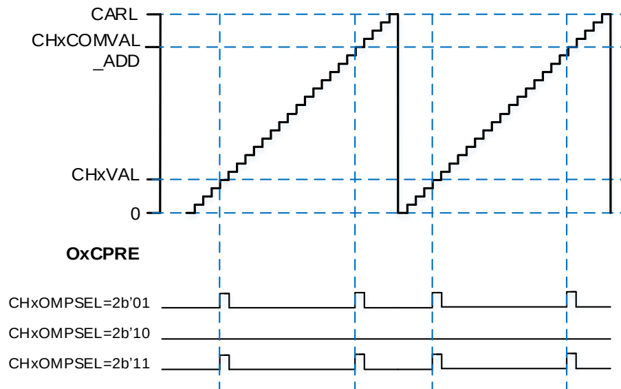
Figure 13-26. CHx_O output with a pulse in edge-aligned mode (CHxOMPSEL≠2'b00)
