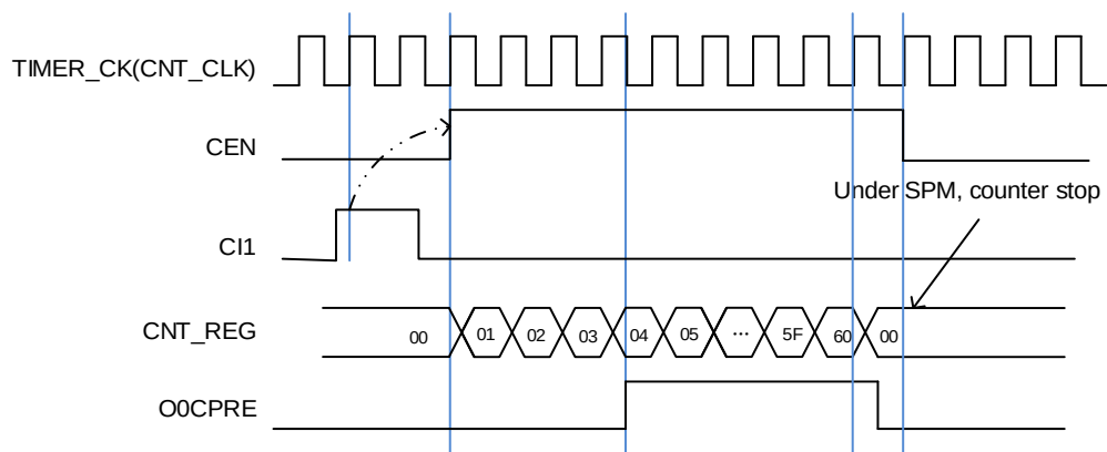
Figure 13-40. Single pulse mode TIMERx\_CHxCV=0x04 , TIMERx\_CAR=0x60
