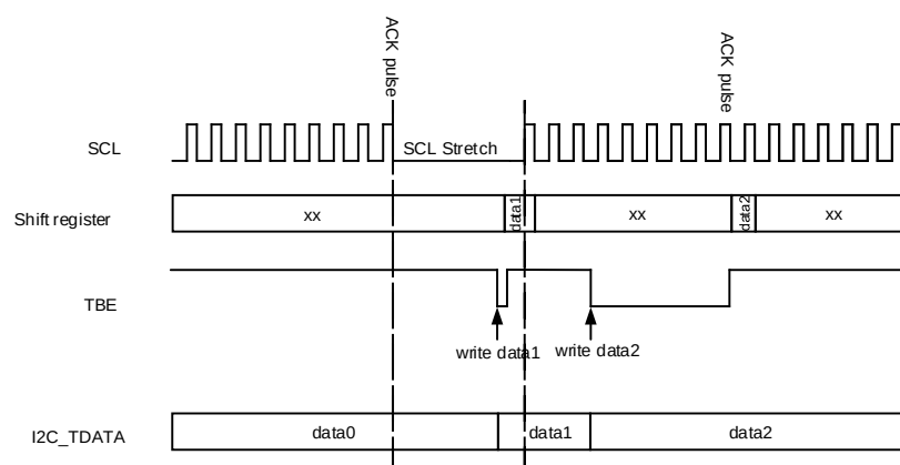
Figure 26-11. Data transmission
