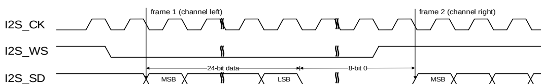
Figure 25-19. I2S Philips standard timing diagram (DTLEN=01, CHLEN=1, CKPL=0)
