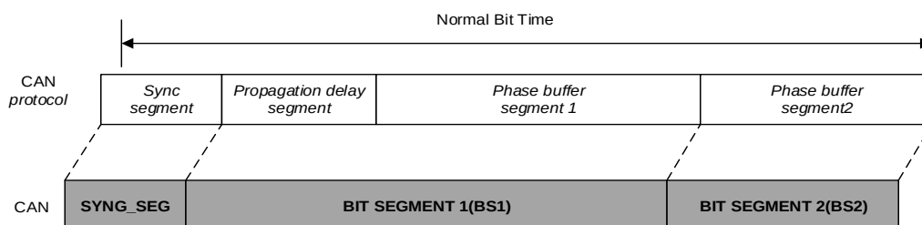
Figure 26-11. The bit time
