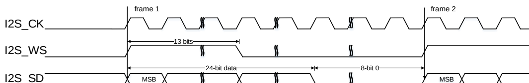
Figure 25-47. PCM standard long frame synchronization mode timing diagram (DTLEN=01, CHLEN=1, CKPL=0)
