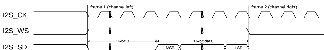
Figure 24-34. LSB justified standard timing diagram (DTLEN=00, CHLEN=1, CKPL=1)
