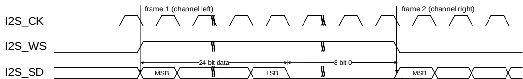
Figure 24-27. MSB justified standard timing diagram (DTLEN=01, CHLEN=1, CKPL=0)
