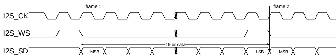
Figure 25-36. PCM standard short frame synchronization mode timing diagram (DTLEN=00, CHLEN=0, CKPL=1)
