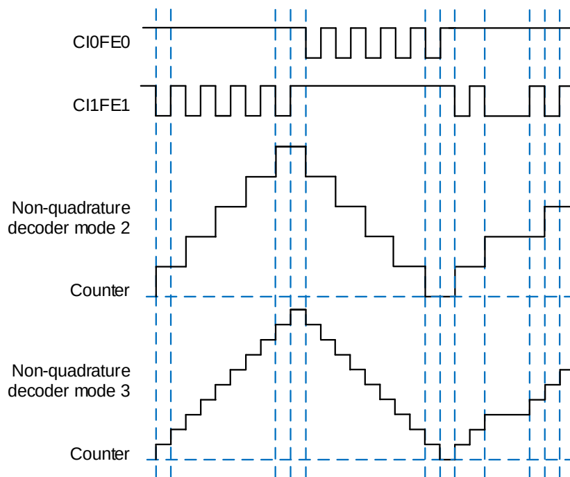
Figure 13-65. Example of counter operation in non-quadrature decoder mode 2 / 3 (CH0P / CH1P=0)
