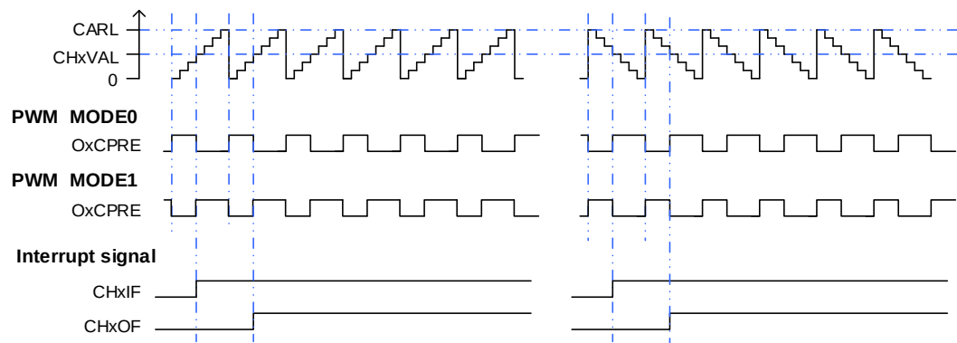
Figure 13-16. Timing diagram of CAPWM
