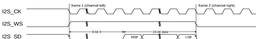
Figure 24-32. LSB justified standard timing diagram (DTLEN=01, CHLEN=1, CKPL=1)
