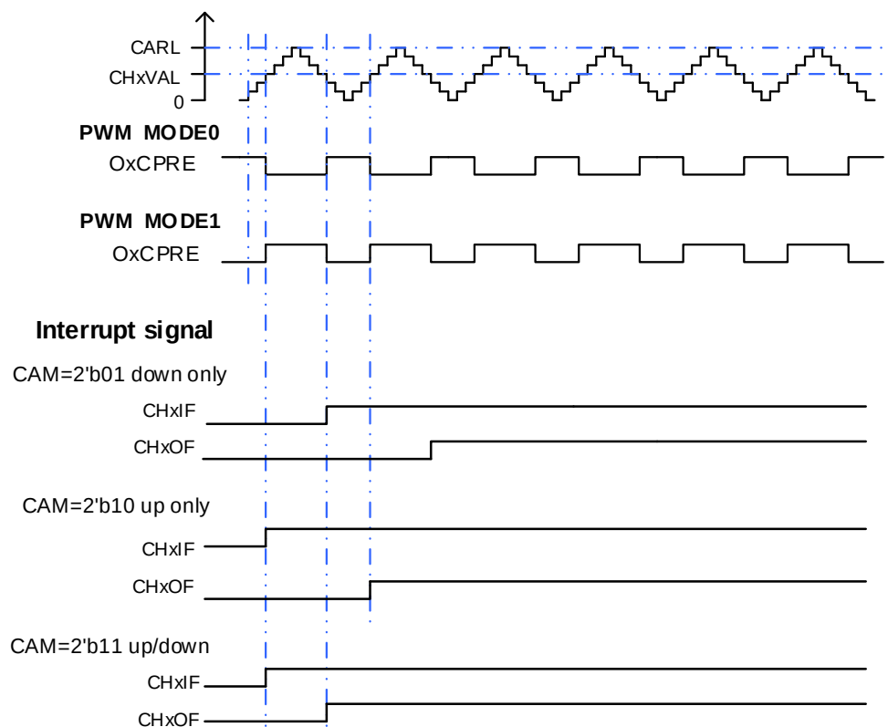
Figure 13-16. Timing diagram of CAPWM
