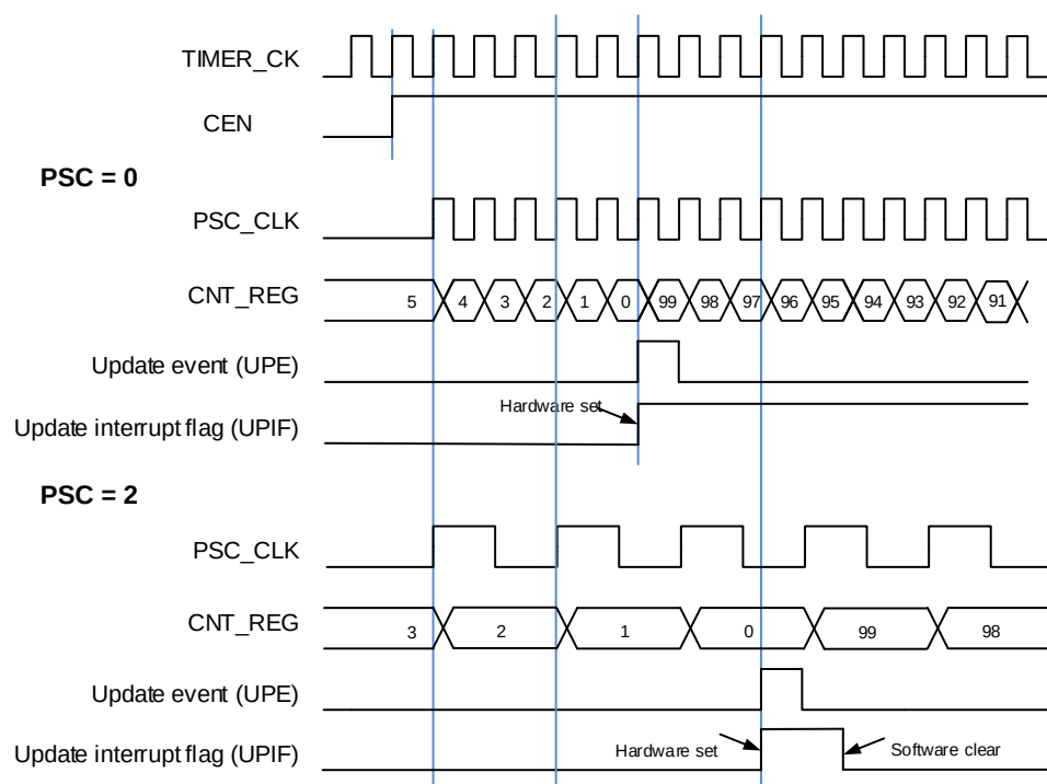
Figure 13-53. Timing chart of down counting mode, PSC=0/2
