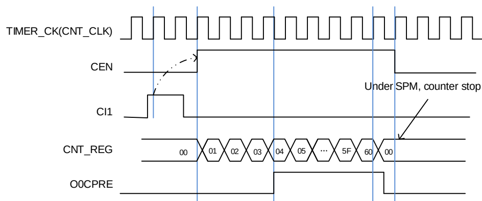
Figure 13-69. Single pulse mode TIMERx_CHxCV = 0x04 , TIMERx_CAR=0x60
