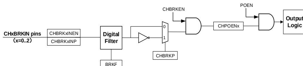
Figure 13-32. Channel break function logic diagram
