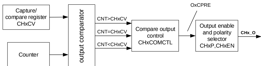
Figure 13-85. Output compare logic (x=1)
