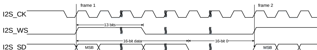
Figure 25-50. PCM standard long frame synchronization mode timing diagram (DTLEN=00, CHLEN=1, CKPL=1)
