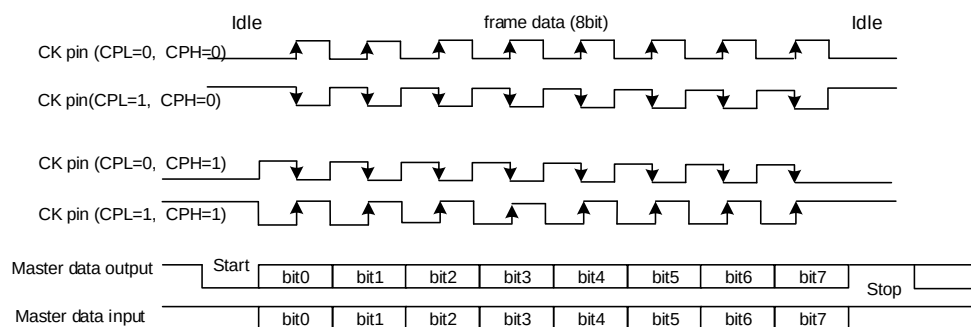
Figure 24-12. 8-bit format USART synchronous waveform (CLEN=1)
