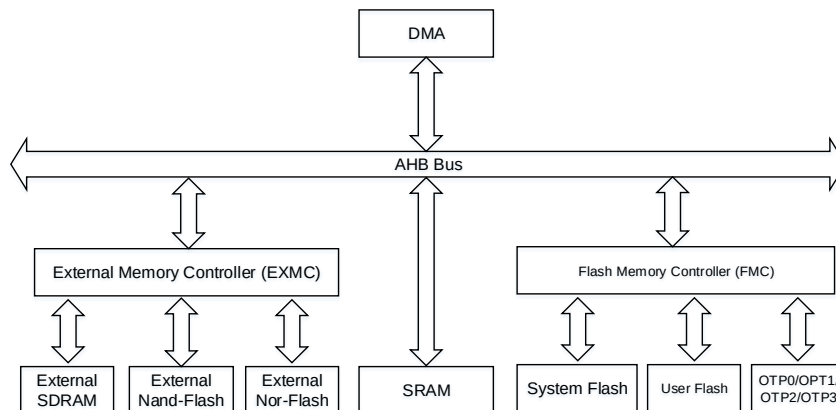
Figure 2-1. GD32F50x memory access architecture
