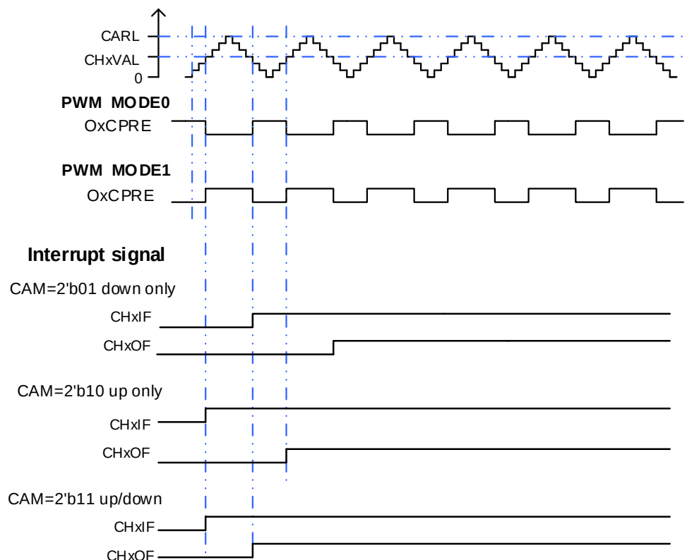
Figure 13-60. Timing chart of CAPWM
