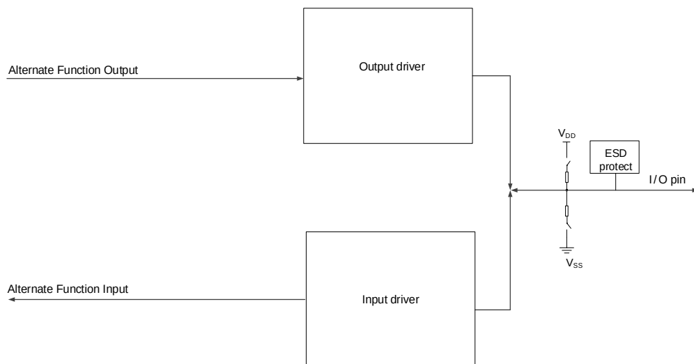
Figure 11-5. Basic structure of Alternate function configuration
