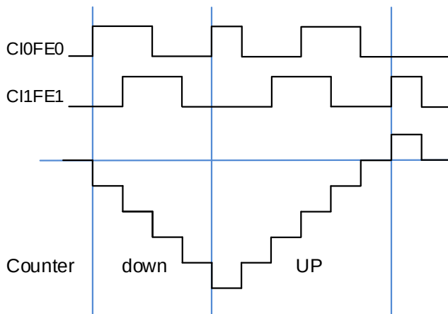
Figure 13-62. Example of decoder interface mode with CI0FE0 polarity inverted
