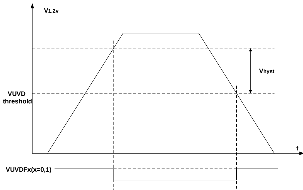
Figure 7-6. waveform of VUVD
