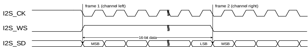
Figure 24-24. MSB justified standard timing diagram (DTLEN=00, CHLEN=0, CKPL=1)
