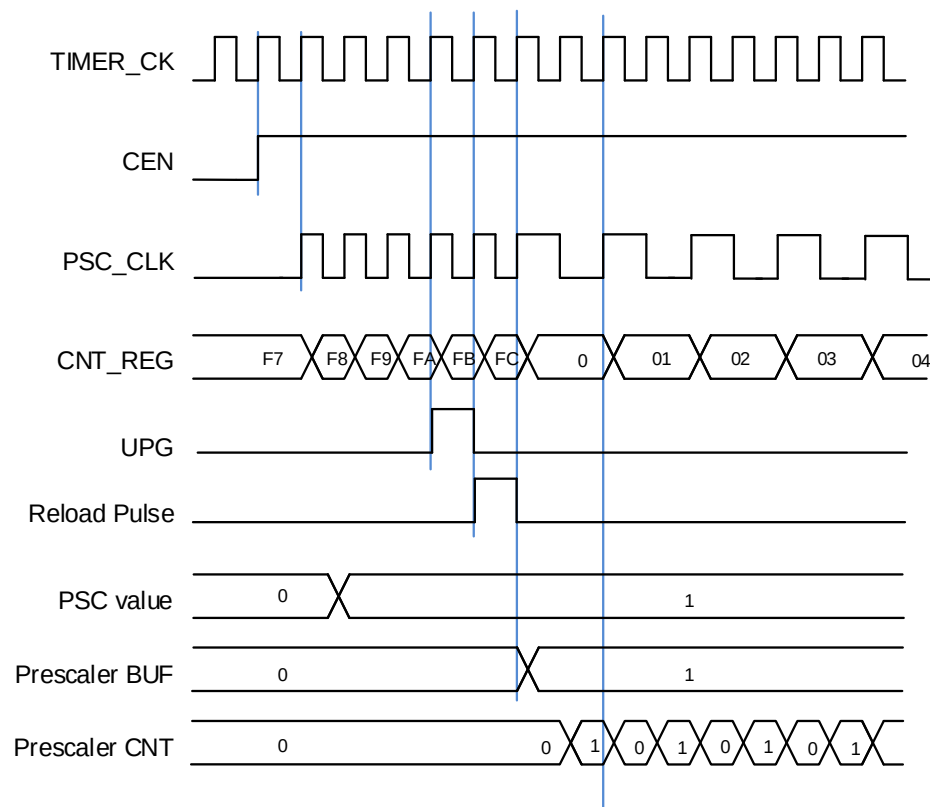
Figure 13-72. Counter timing diagram with prescaler division change from 1 to 2
