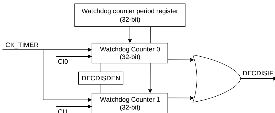
Figure 13-63. Quadrature decoder signal disconnection detection block diagram
