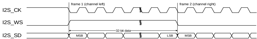
Figure 24-26. MSB justified standard timing diagram (DTLEN=10, CHLEN=1, CKPL=1)
