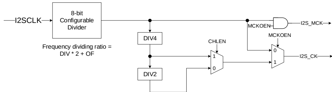
Figure 25-51. Block diagram of I2S clock generator
