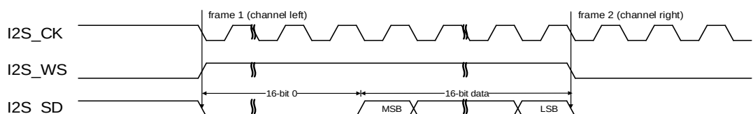
Figure 25-34. LSB justified standard timing diagram (DTLEN=00, CHLEN=1, CKPL=1)
