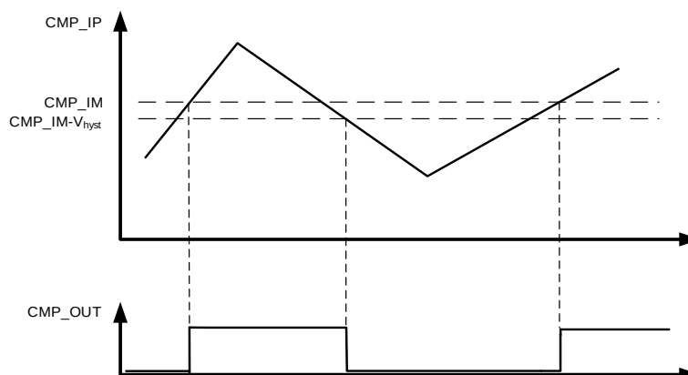
Figure 20-2. CMP hysteresis
