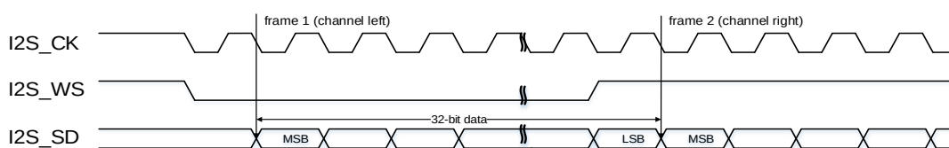
Figure 25-18. I2S Philips standard timing diagram (DTLEN=10, CHLEN=1, CKPL=1)
