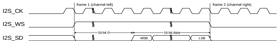
Figure 25-33. LSB justified standard timing diagram (DTLEN=00, CHLEN=1, CKPL=0)
