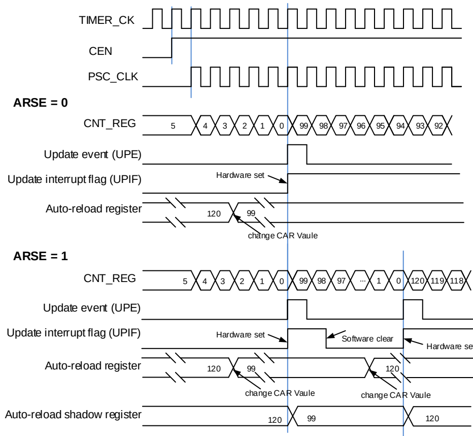
Figure 13-54. Timing chart of down counting mode, change TIMERx_CAR ongoing
