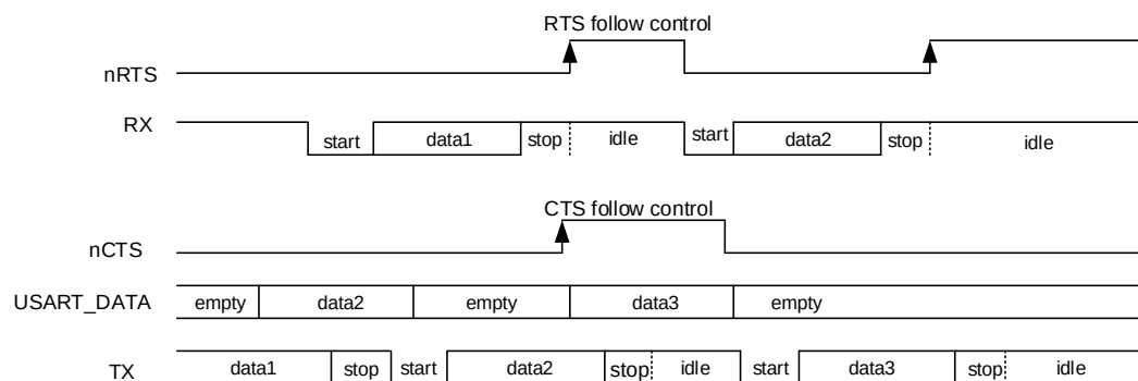
Figure 24-8. Hardware flow control
