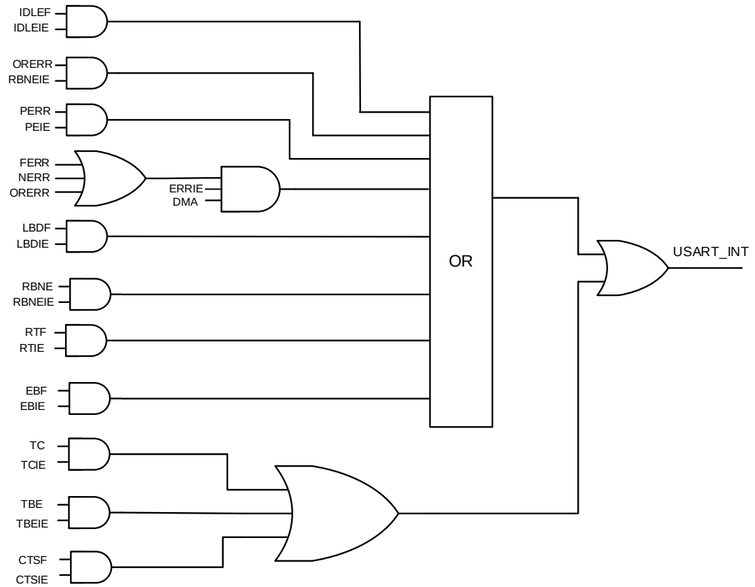
Figure 24-16. USART interrupt mapping diagram
