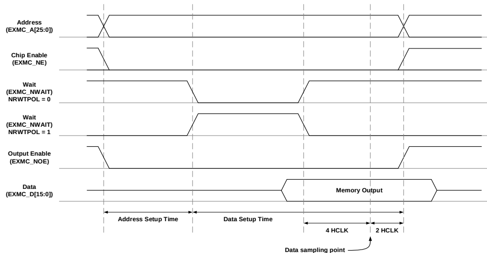
Figure 28-8. Read access timing diagram under async-wait signal assertion
