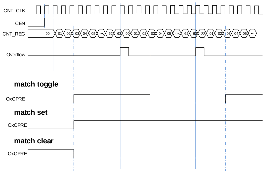
Figure 13-14. Output-compare in three modes
