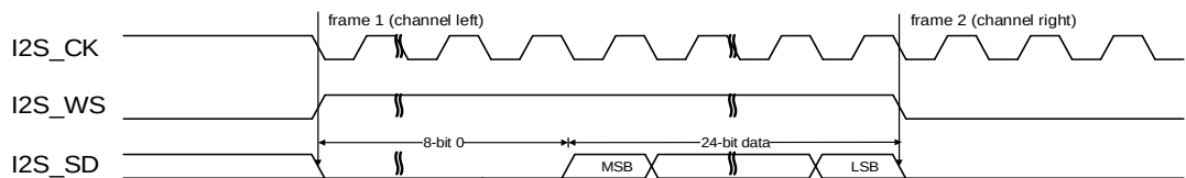
Figure 25-32. LSB justified standard timing diagram (DTLEN=01, CHLEN=1, CKPL=1)
