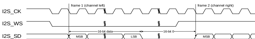
Figure 25-22. I2S Philips standard timing diagram (DTLEN=00, CHLEN=1, CKPL=1)
