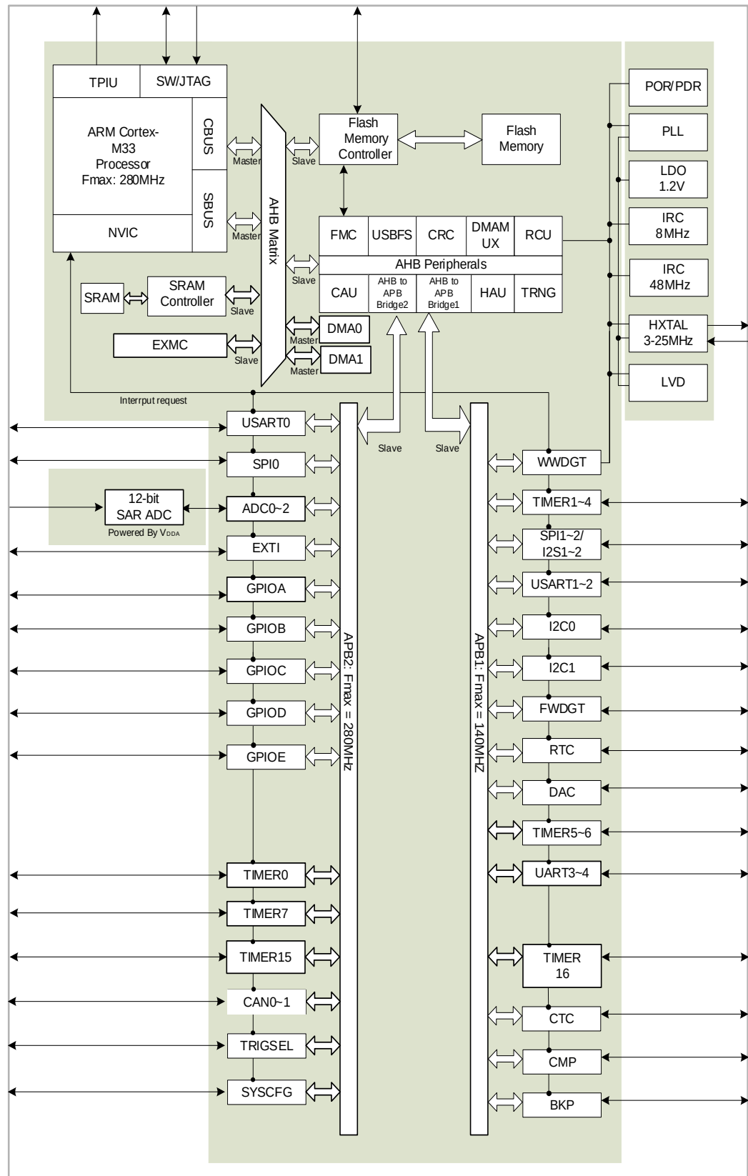
Figure 1-2. GD32F50x series system architecture
