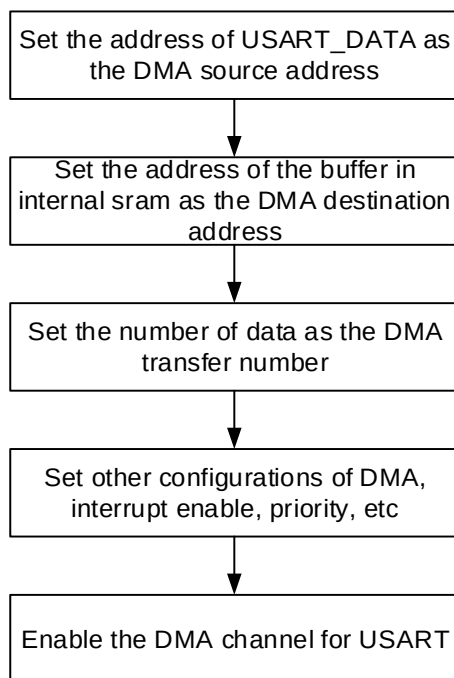
Figure 24-6. Configuration steps when using DMA for USART reception
