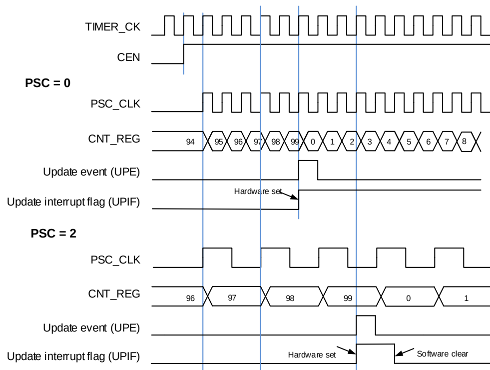
Figure 13-106. Timing chart of up counting mode, PSC=0/2
