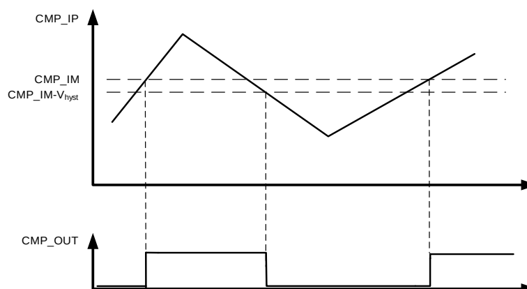
Figure 23-2. CMP hysteresis
