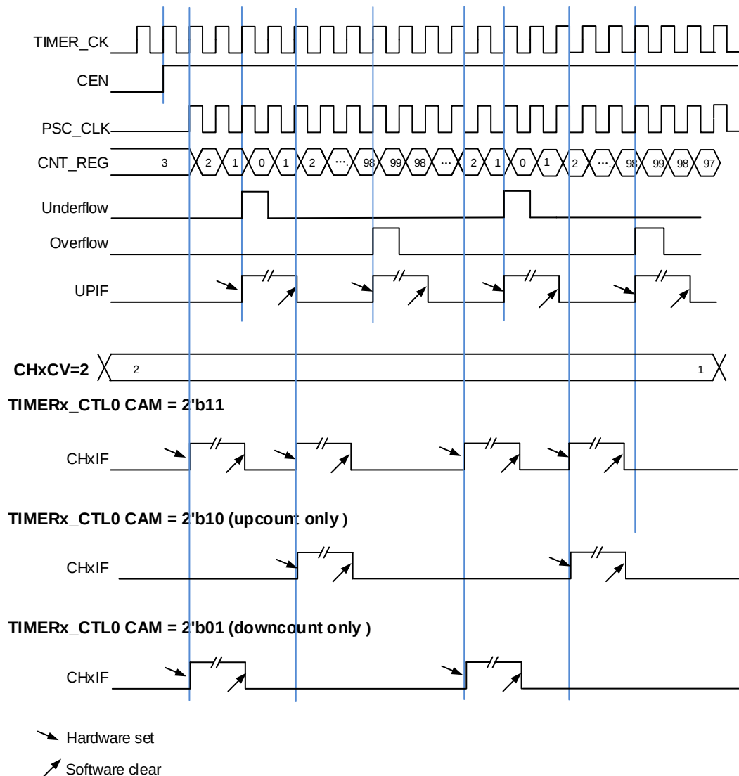
Figure 13-55. Timing chart of center-aligned counting mode
