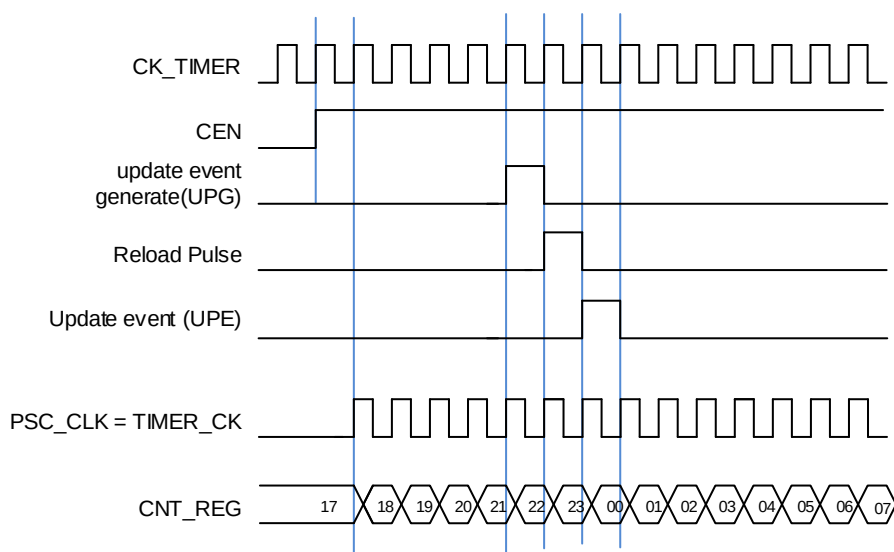
Figure 13-104. Normal mode, internal clock divided by 1
