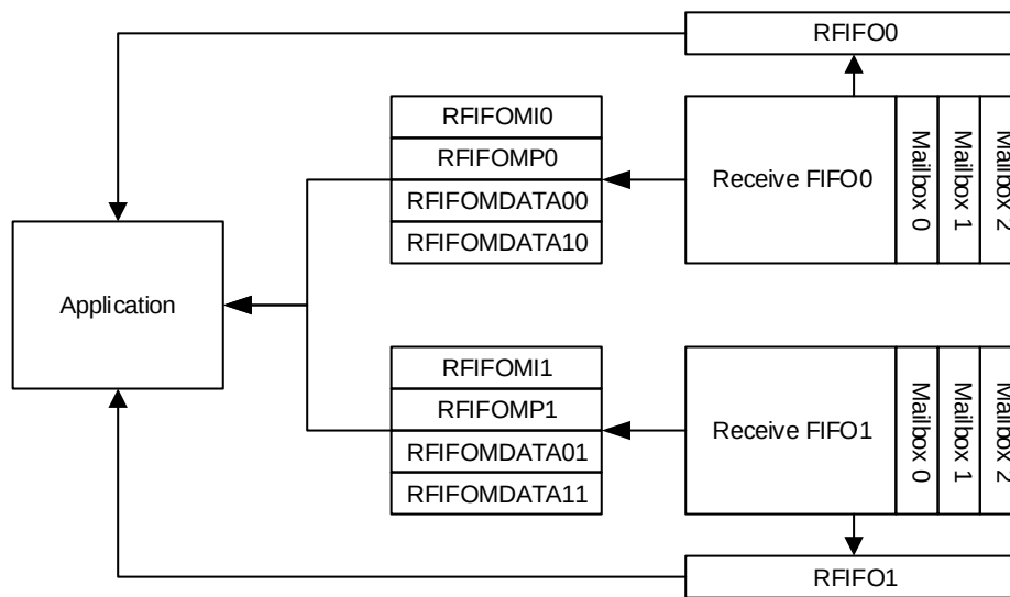
Figure 27-4. Reception register
