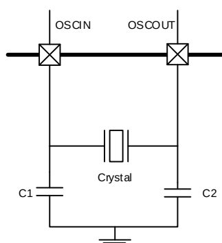
Figure 8-4. HXTAL clock source
