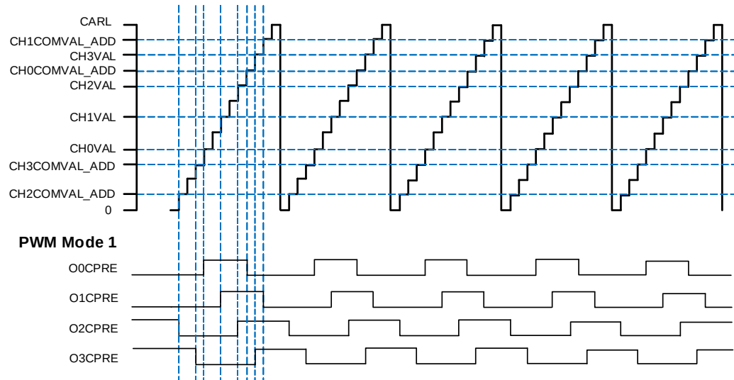
Figure 13-22. Four Channels outputs in Composite PWM mode
