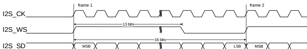
Figure 25-43. PCM standard long frame synchronization mode timing diagram (DTLEN=00, CHLEN=0, CKPL=0)
