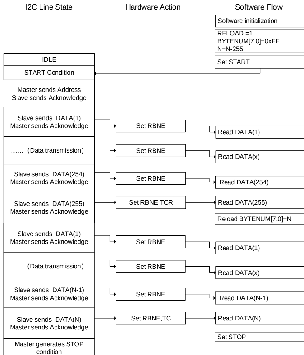
Figure 26-21. Programming model for master receiving (N>255)
