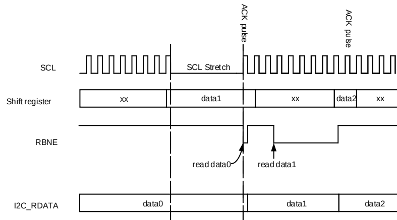
Figure 26-12. Data reception
