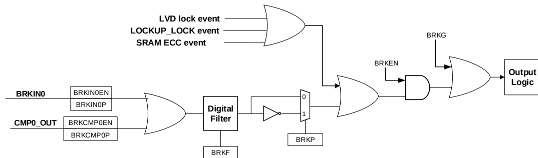
Figure 13-30. BREAK function logic diagram
