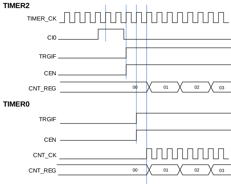
Figure 13-45. Trigger TIMER0 and TIMER2 by the CI0 signal of TIMER2
