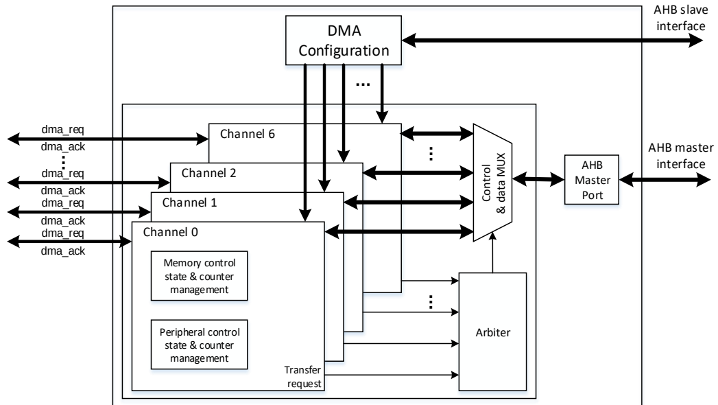
Figure 4-1. Block diagram of DMA
