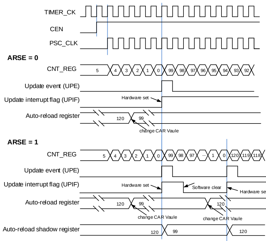
Figure 13-7. Timing diagram of down counting mode, change TIMERx_CAR ongoing
