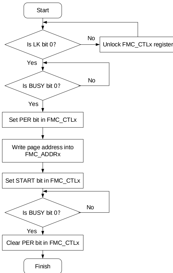
Figure 6-1. Process of page erase operation
