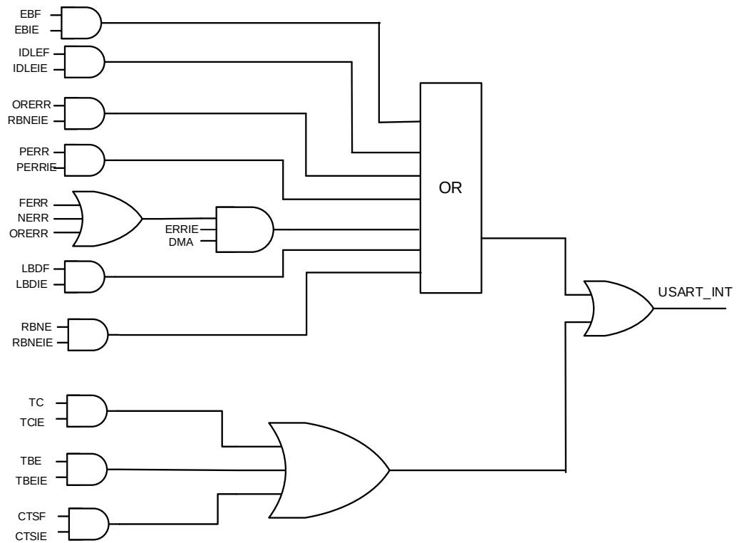
Figure 23-16. USART interrupt mapping diagram
