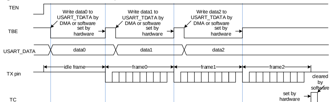
Figure 24-3. USART transmit procedure
