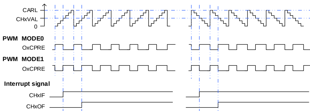
Figure 13-88. Timing diagram of CAPWM
