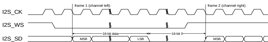
Figure 25-21. I2S Philips standard timing diagram (DTLEN=00, CHLEN=1, CKPL=0)
