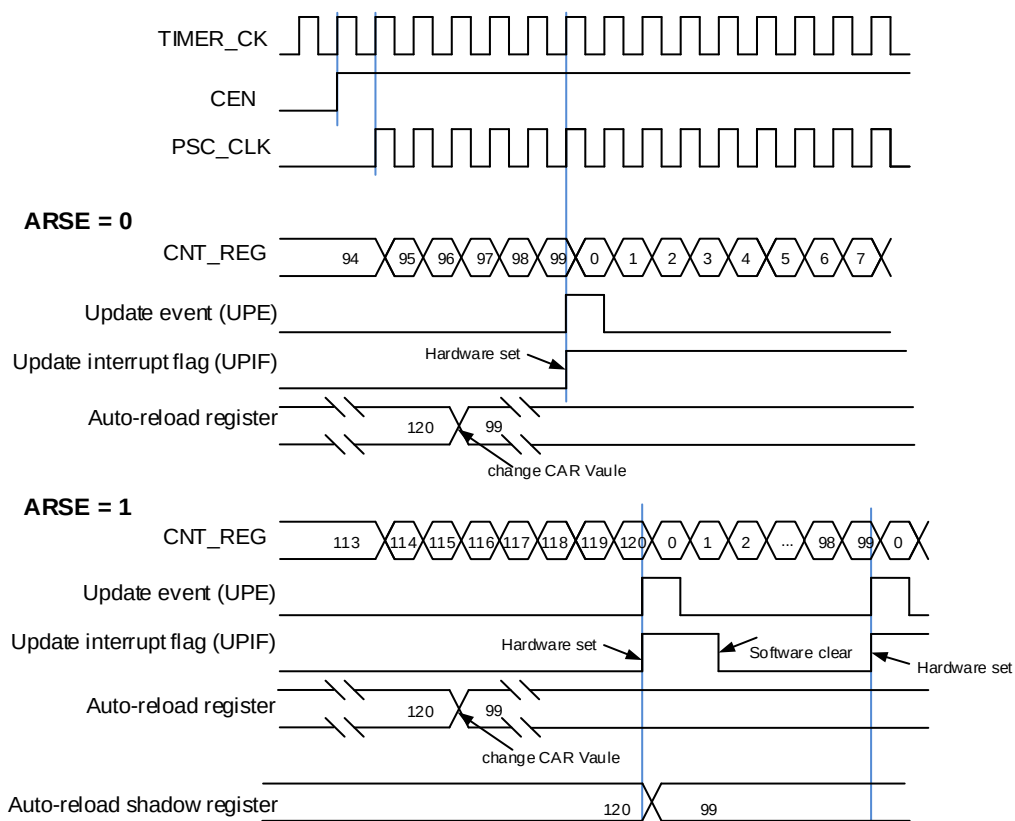
Figure 13-5. Timing diagram of up counting mode, change TIMERx\_CAR ongoing
