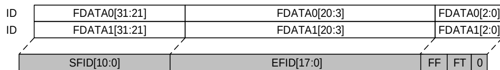
Figure 27-9. 32-bit list mode filter
