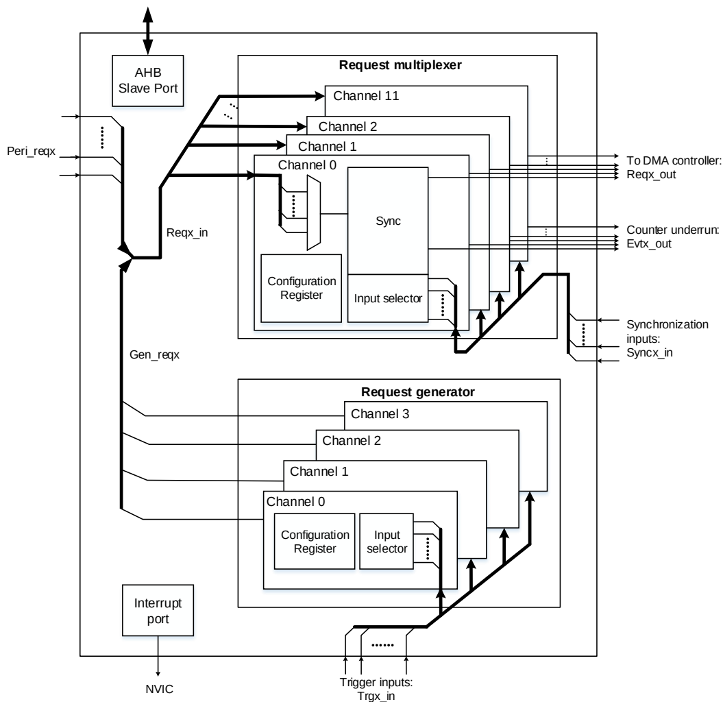
Figure 5-1. Block diagram of DMAMUX
