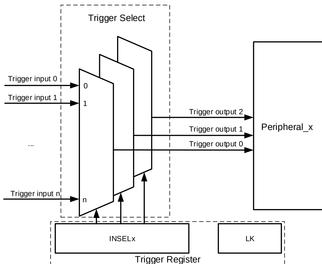
Figure 12-1. TRIGSEL main composition example
