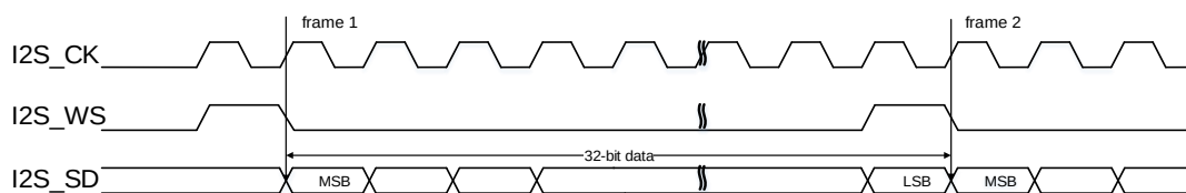
Figure 25-37. PCM standard short frame synchronization mode timing diagram (DTLEN=10, CHLEN=1, CKPL=0)
