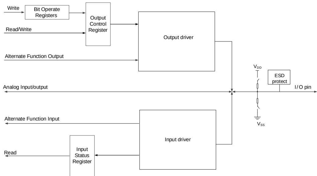
Figure 11-1. Basic structure of a standard I/O port bit
