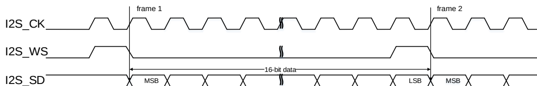
Figure 25-35. PCM standard short frame synchronization mode timing diagram (DTLEN=00, CHLEN=0, CKPL=0)
