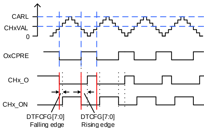
Figure 13-29. Complementary output with different dead time(DTDIFEN=1)
