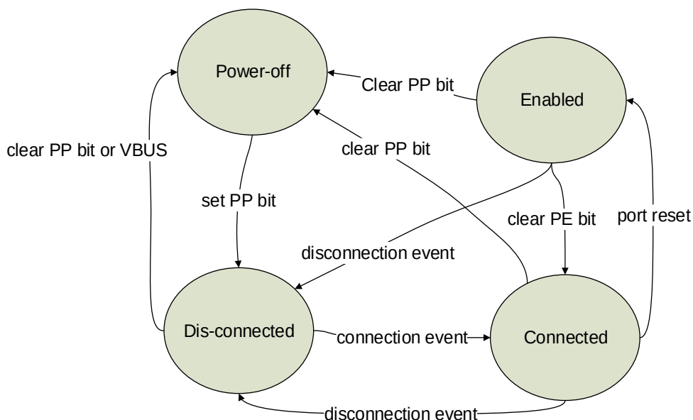
Figure 28-3. State transition diagram of host port
