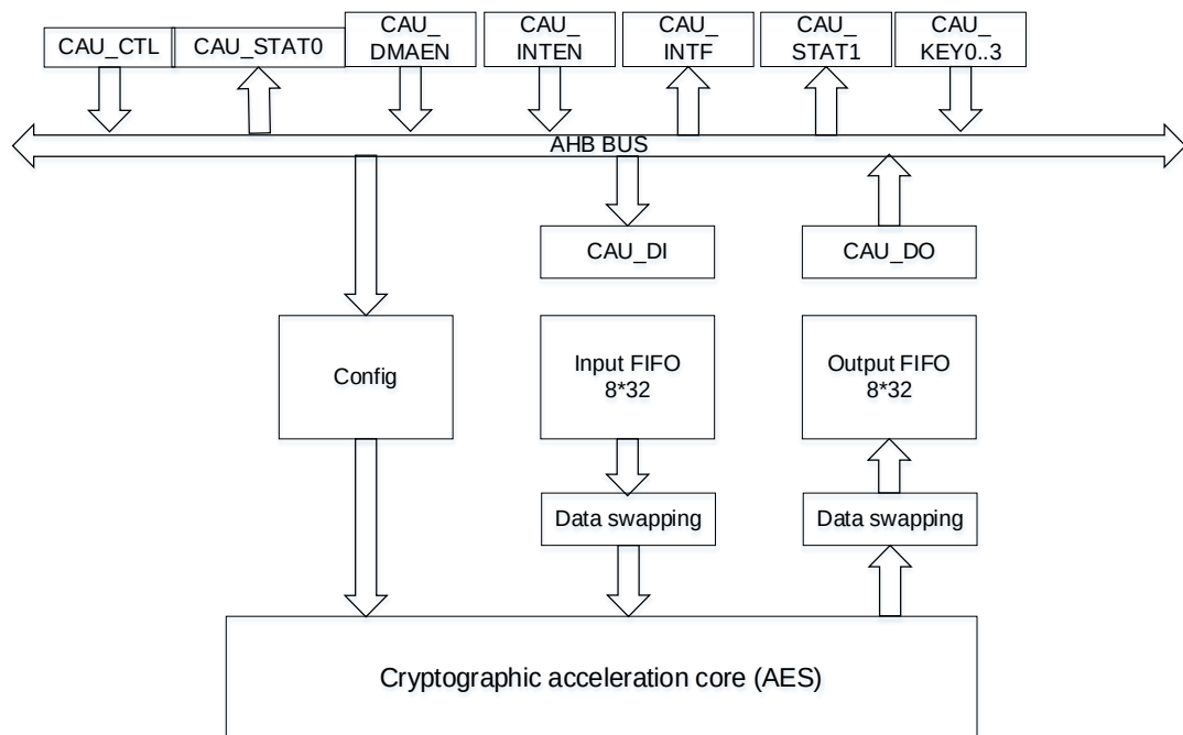
Figure 19-3. CAU diagram
