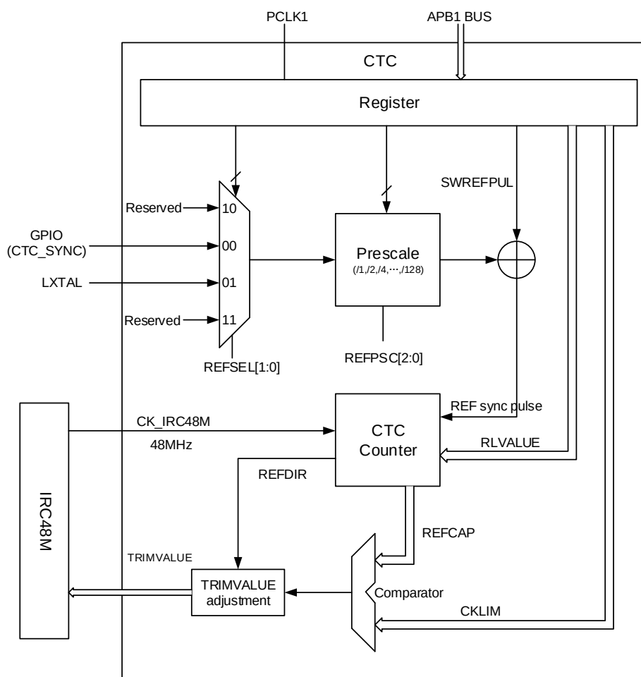
Figure 10-1. CTC overview
