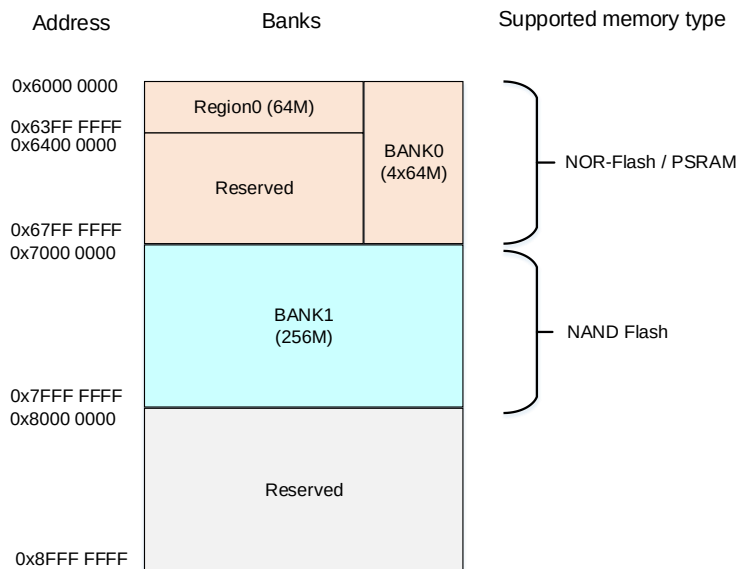
Figure 28-2. EXMC memory banks
