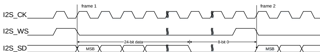
Figure 25-39. PCM standard short frame synchronization mode timing diagram (DTLEN=01, CHLEN=1, CKPL=0)
