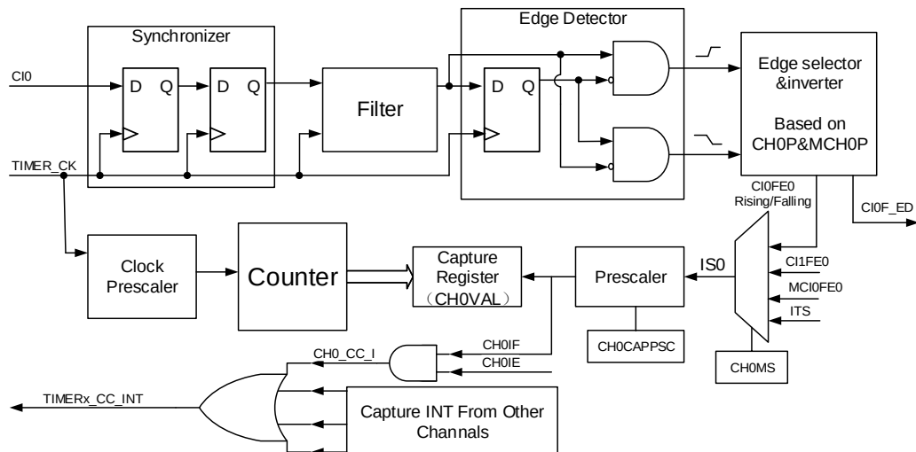
Figure 13-81. Input capture logic for channel 0
