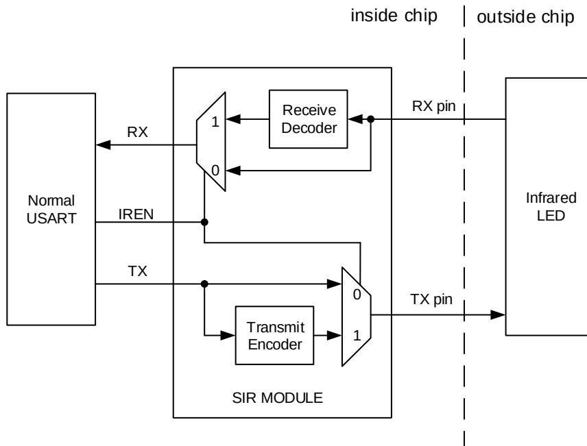
Figure 24-13. IrDA SIR ENDEC module
