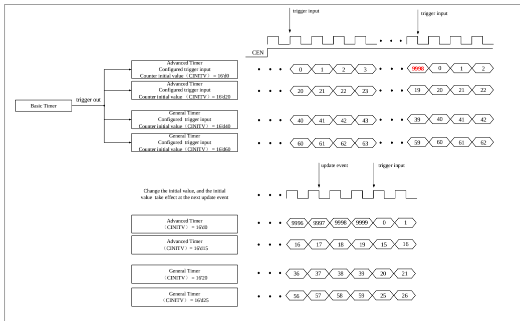
Figure 13-46. Triggering four timers by trigger out of basic timer
