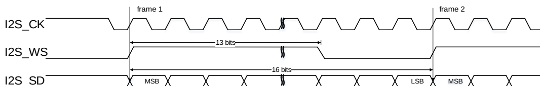
Figure 25-44. PCM standard long frame synchronization mode timing diagram (DTLEN=00, CHLEN=0, CKPL=1)
