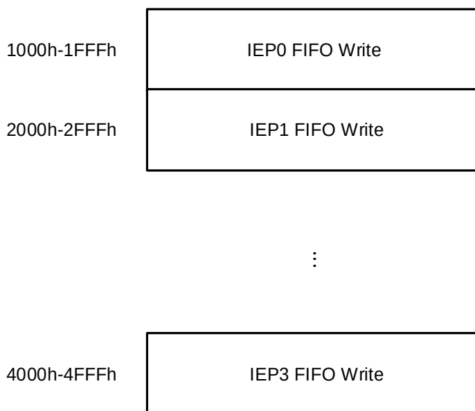
Figure 29-7. Device mode FIFO access register map
