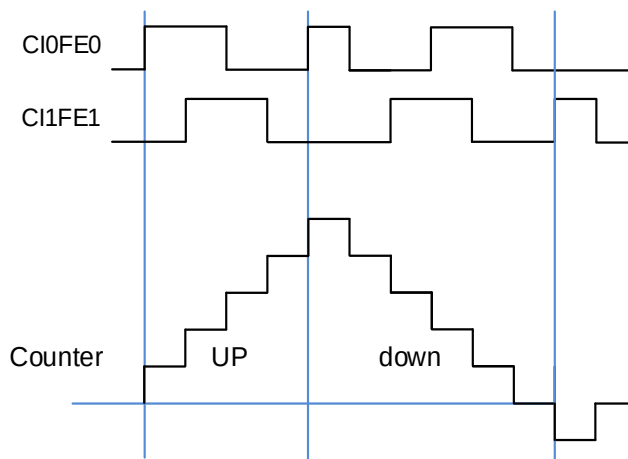
Figure 13-33. Example of counter operation in quadrature decoder interface mode
