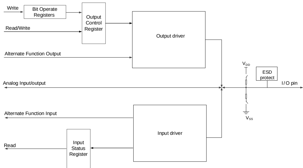
Figure 10-1. Basic structure of a standard I/O port bit
