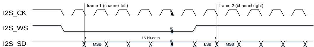
Figure 25-16. I2S Philips standard timing diagram (DTLEN=00, CHLEN=0, CKPL=1)
