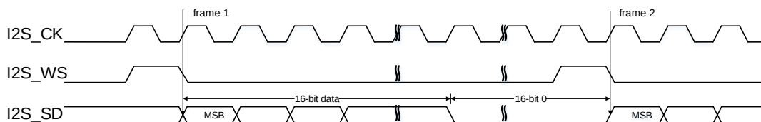
Figure 25-41. PCM standard short frame synchronization mode timing diagram (DTLEN=00, CHLEN=1, CKPL=0)
