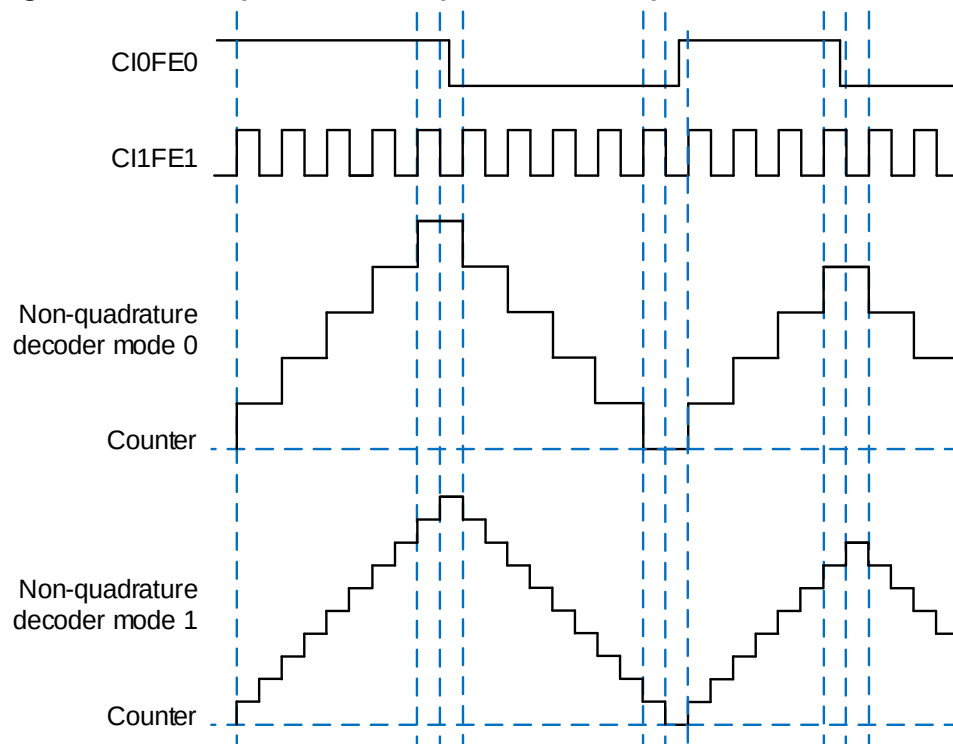
Figure 13-64. Example of counter operation in non-quadrature mode 0 / 1 with CH1P=0
