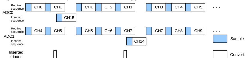
Figure 21-22. Routine parallel & inserted trigger rotation mode: SYNCM = 4'b0010
