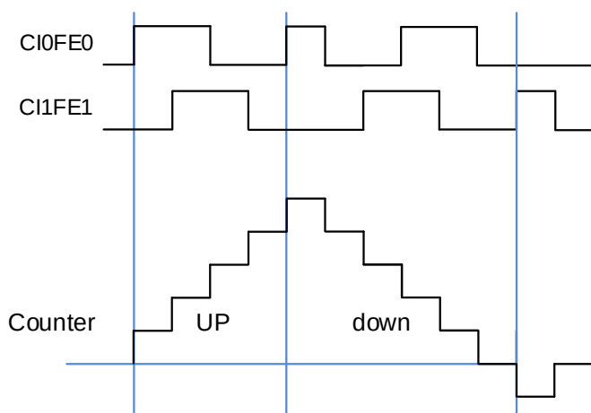
Figure 13-61. Example of counter operation in decoder interface mode
