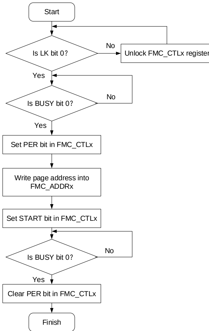
Figure 5-1. Process of page erase operation
