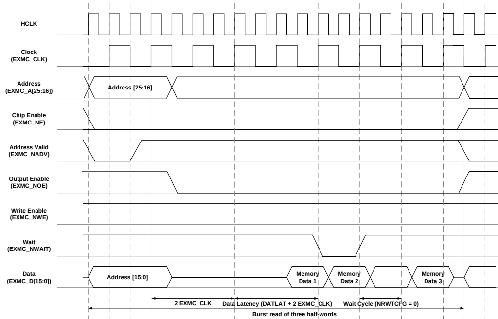
Figure 28-10. Read timing of synchronous multiplexed burst mode
