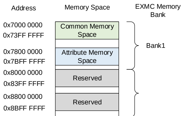
Figure 28-4. NAND address mapping
