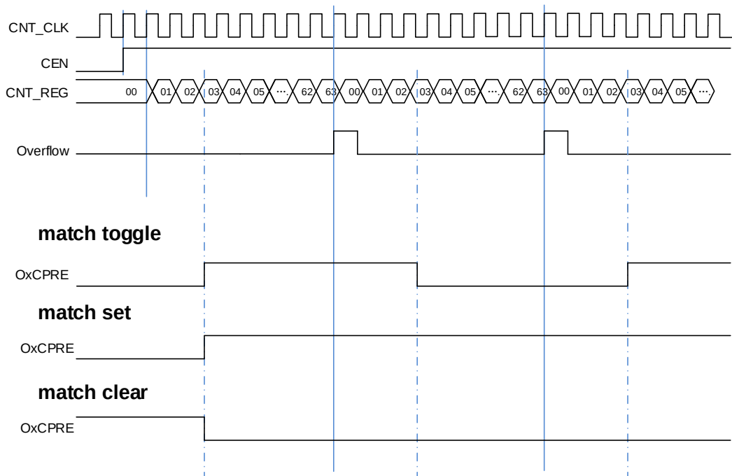
Figure 13-58. Output-compare under three modes
