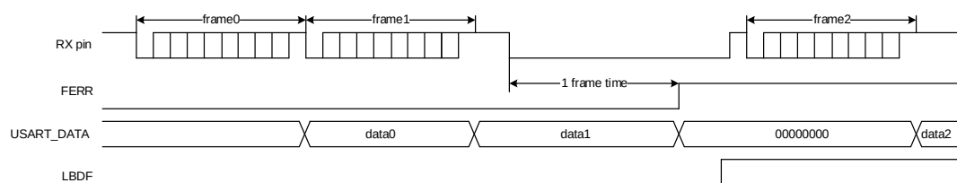
Figure 24-9. Break frame occurs during idle state
