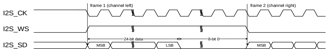
Figure 24-28. MSB justified standard timing diagram (DTLEN=01, CHLEN=1, CKPL=1)
