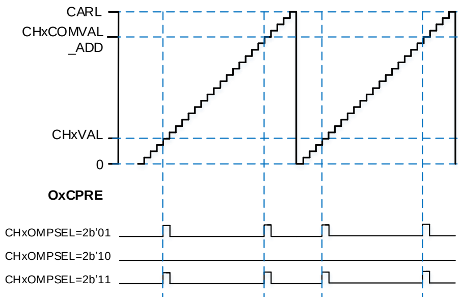
Figure 13-94. CHx_O output with a pulse in edge-aligned mode (CHxOMPSEL≠2'b00)
