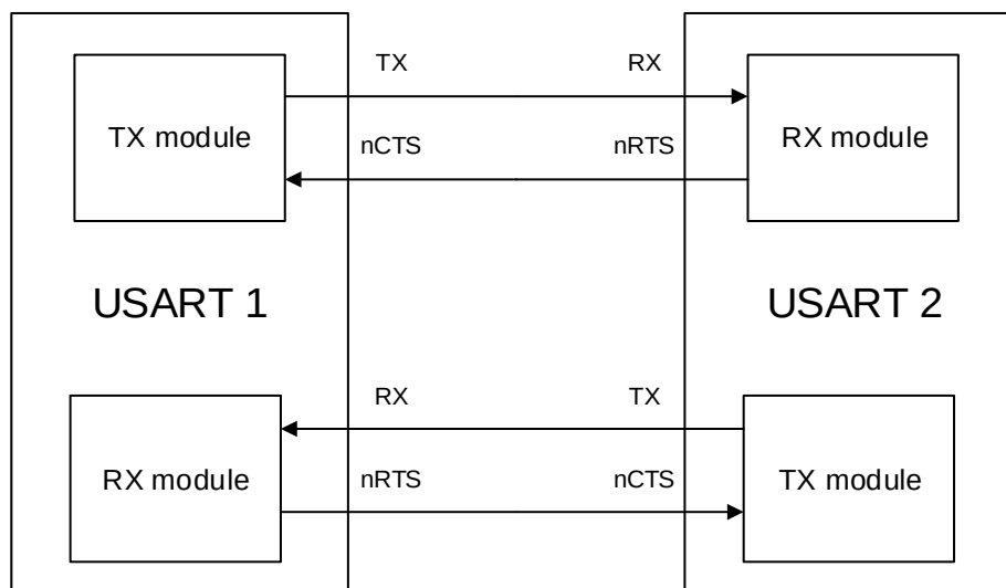
Figure 24-7. Hardware flow control between two USARTs
