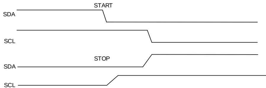
Figure 26-3. START and STOP signal
