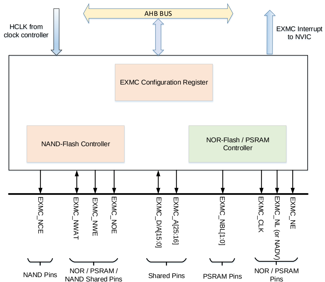
Figure 28-1. The EXMC block diagram
