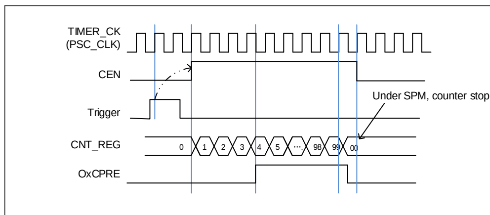
图 14-60. 单脉冲模式, TIMERx_CHxCV = 4 TIMERx_CAR=99
