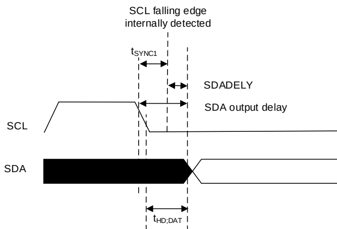
Figure 28-9. Data hold time
