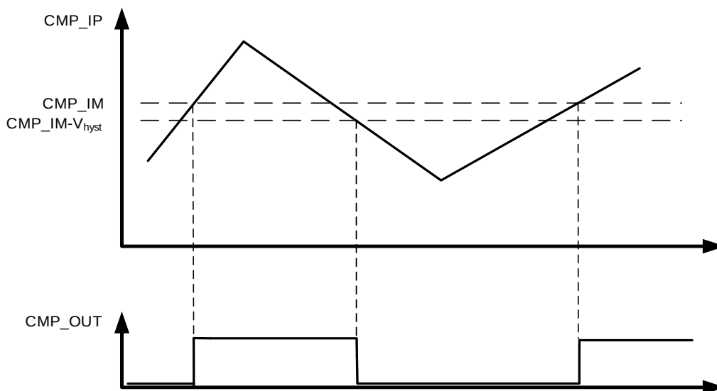
Figure 19-2. CMP hysteresis
