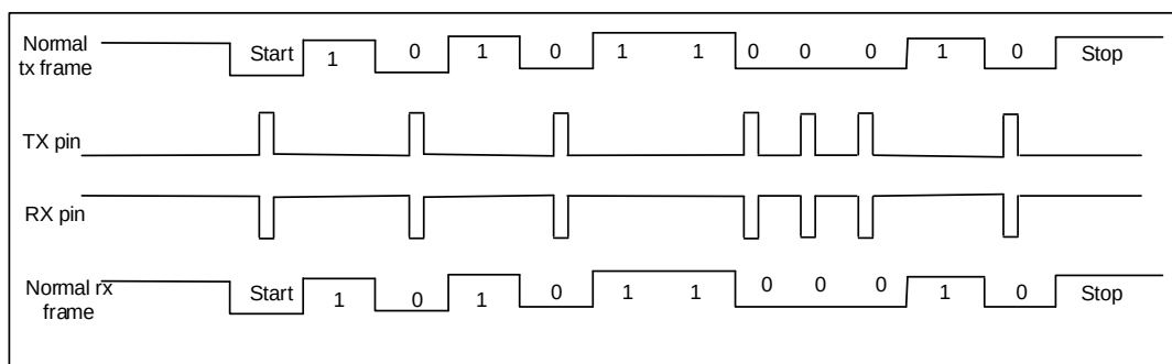
Figure 27-14. IrDA data modulation
