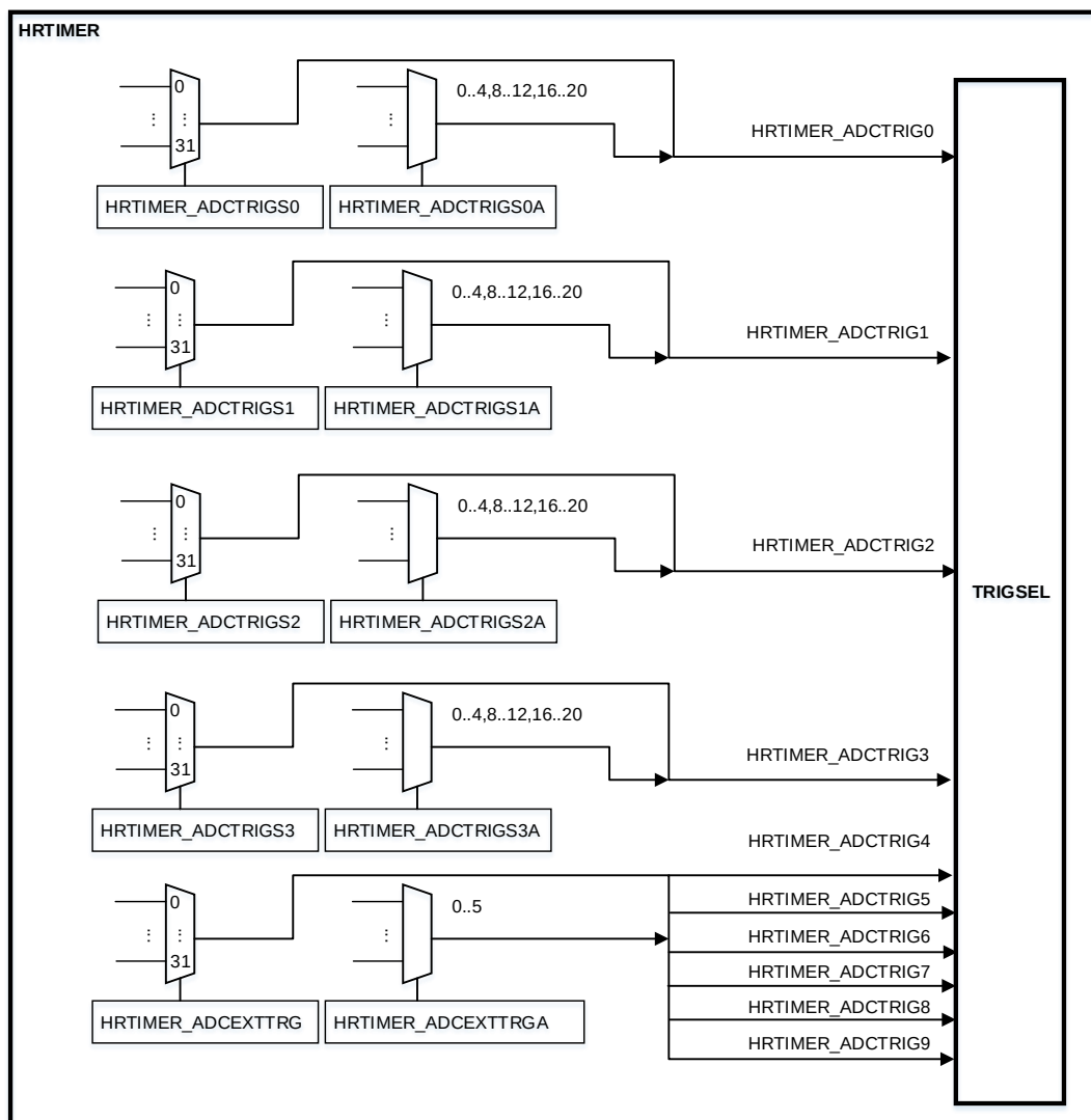
Figure 25-54. Trigger to ADC selection overview
