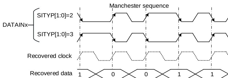
Figure 34-3. The sequence diagram of Manchester data transmission
