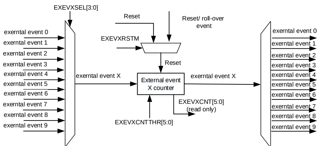
Figure 25-43. External event X counter
