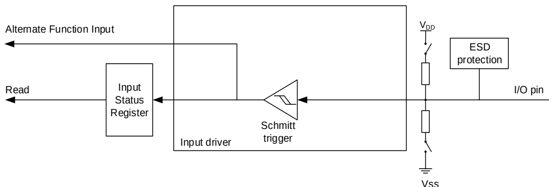
Figure 7-2. Input configuration
