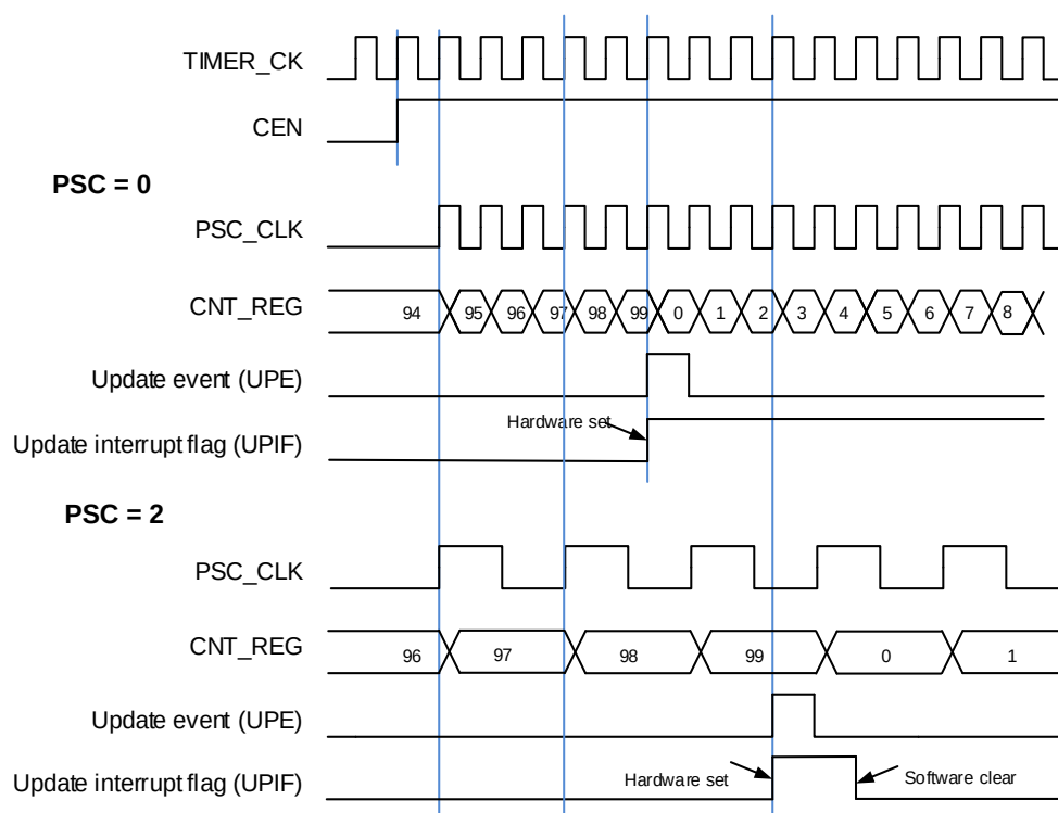
Figure 23-4. Timing diagram of up counting mode, PSC=0 / 2
