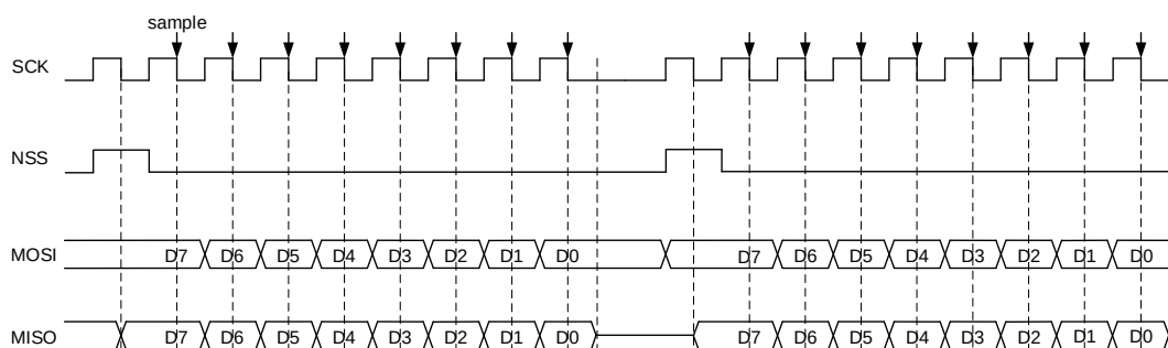
Figure 30-10. Timing diagram of TI master mode with discontinuous transfer
