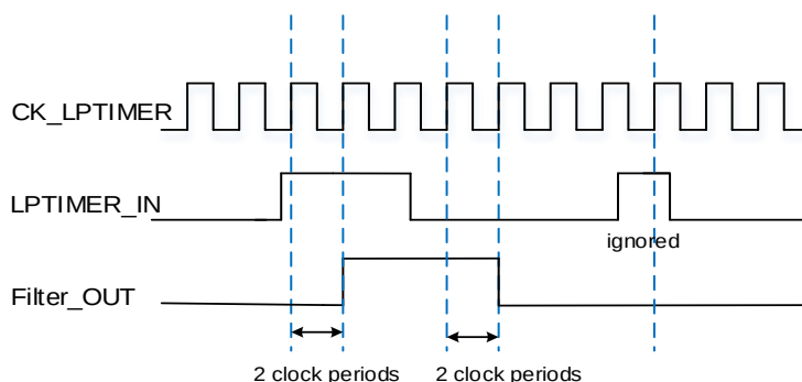
Figure 24-4. Input filter timing diagram (ECKFLT=2'b01)
