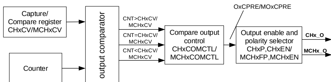
Figure 23-101. Output compare logic (when MCHxMSEL = 2'b11, x=0)
