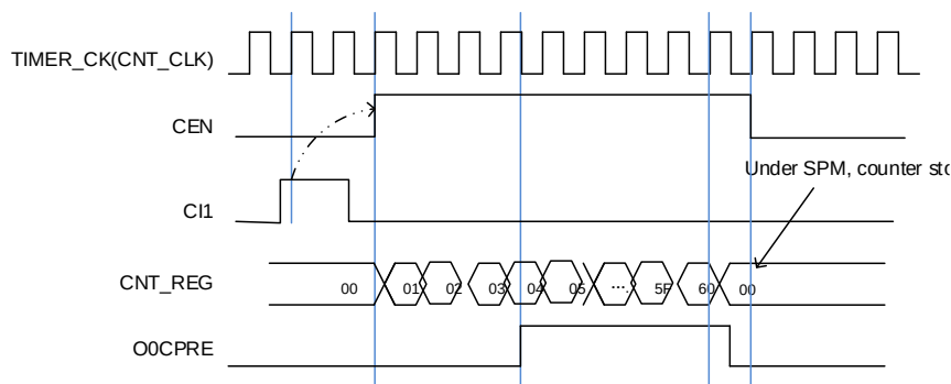
Figure 23-140. Single pulse mode TIMERx_CHxCV = 0x04 TIMERx_CAR=0x60
