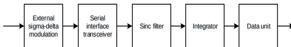
Figure 34-7. HPDF module external input data processing flow
