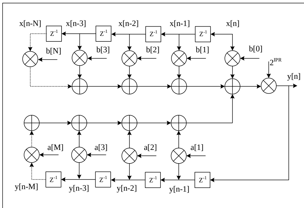
Figure 35-8 The structure of IIR filter
