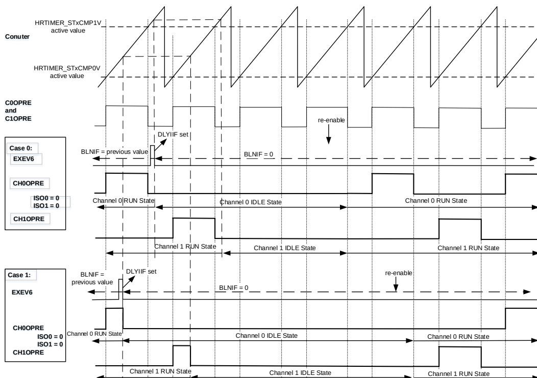
Figure 25-38. Balanced IDLE with ISO0 = 0 and ISO1 = 0
