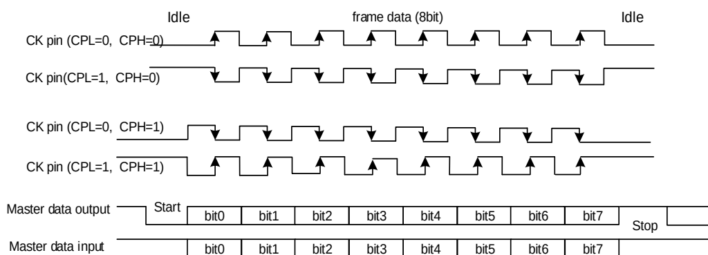
Figure 27-12. 8-bit format USART synchronous waveform (CLEN = 1)
