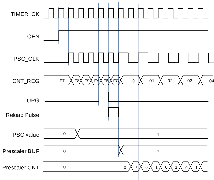
Figure 23-125. Counter timing diagram with prescaler division change from 1 to 2
