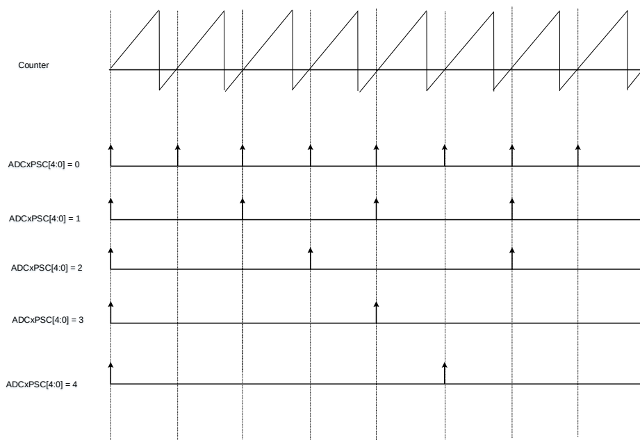
Figure 25-55. ADC trigger division in up counting mode
