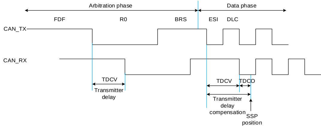
Figure 29-2. Transmitter delay
