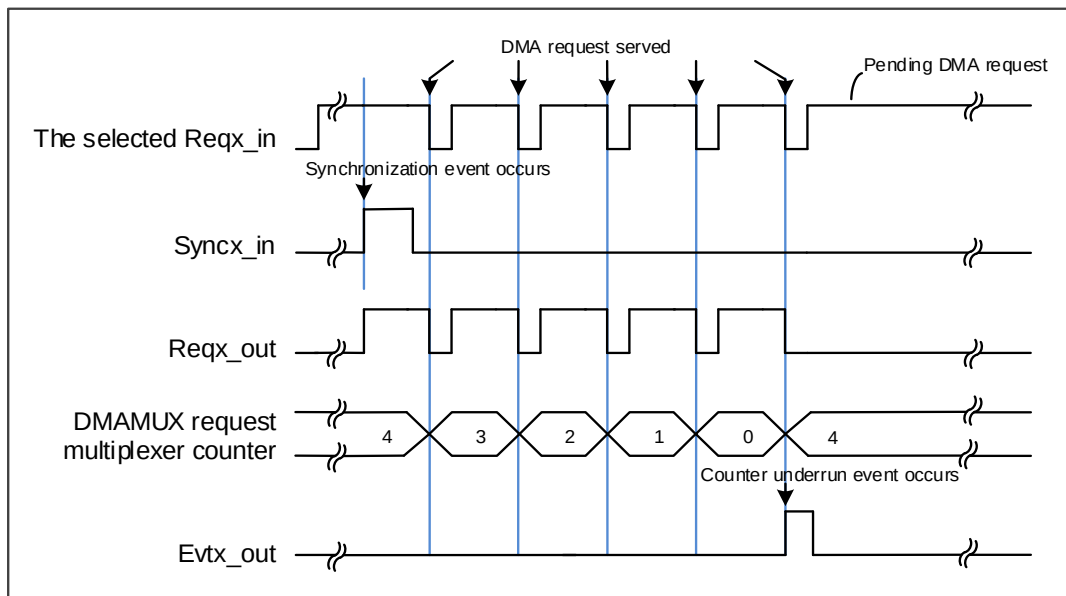
Figure 9-2. Synchronization mode
