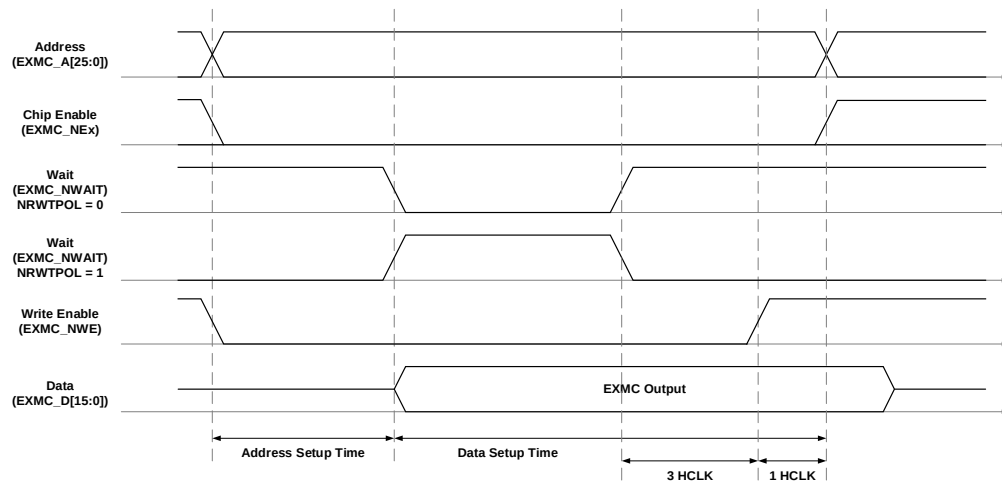
Figure 33-18. Write access timing diagram under async-wait signal assertion
