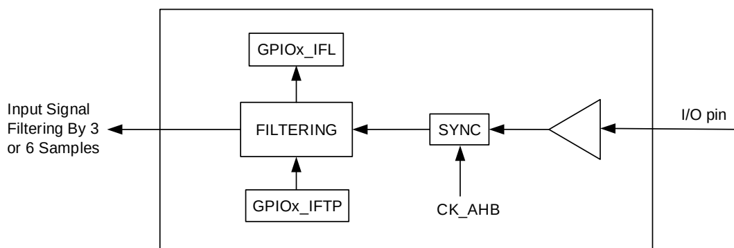
Figure 7-6. Filtering using the sampling window
