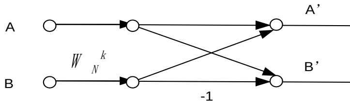
Figure 15-3. 8 points DIT FFT flow digram
