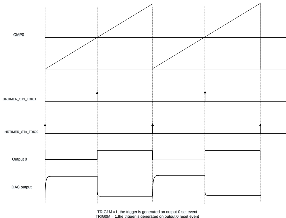
Figure 25-59. Trigger to DAC when TRIG0M = 1 and TRIG1M = 1
