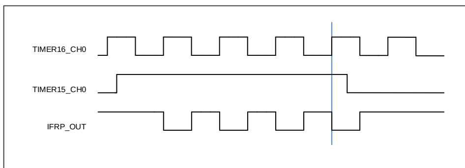
Figure 26-3. IFRP output timechart 3
