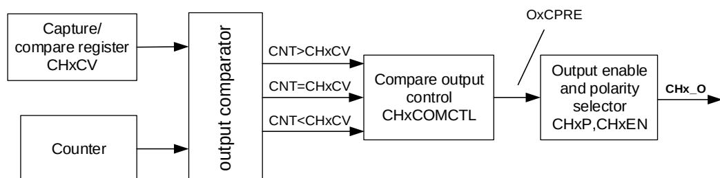
Figure 23-102. Output compare logic (x=1)
