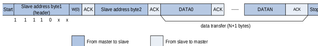
Figure 28-4. I2C communication flow with 10-bit address (Master Transmit)
