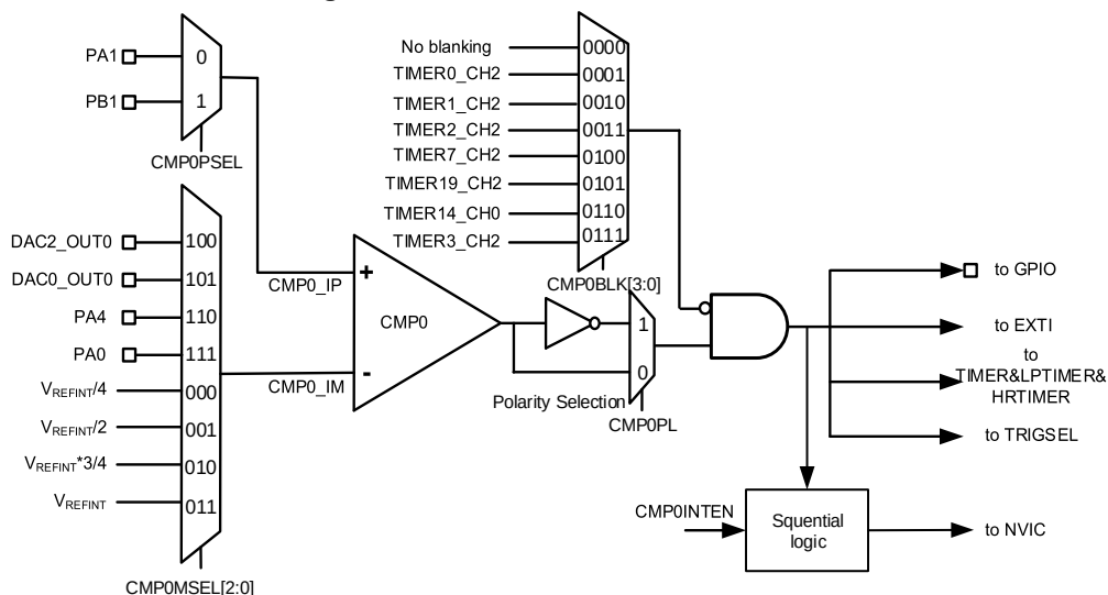
Figure 19-1. CMP block diagram
