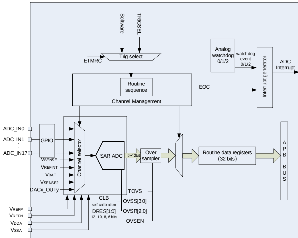
Figure 17-1. ADC module block diagram
