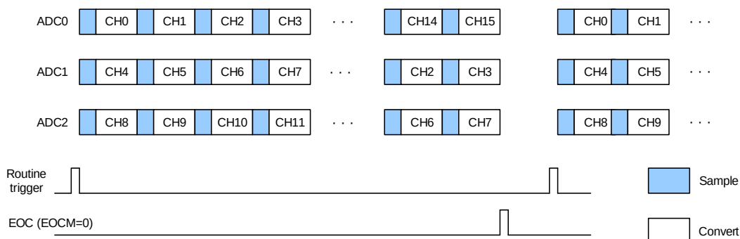
Figure 17-13. Routine parallel mode on 16 channels
