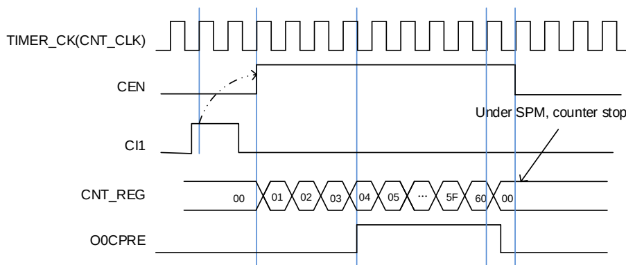
Figure 23-121. Single pulse mode TIMERx\_CHxCV = 0x04 TIMERx\_CAR=0x60
