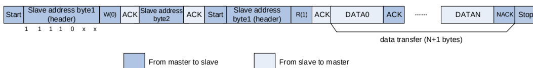
Figure 28-7. I2C communication flow with 10-bit address (Master Receive when HEAD10R=0)
