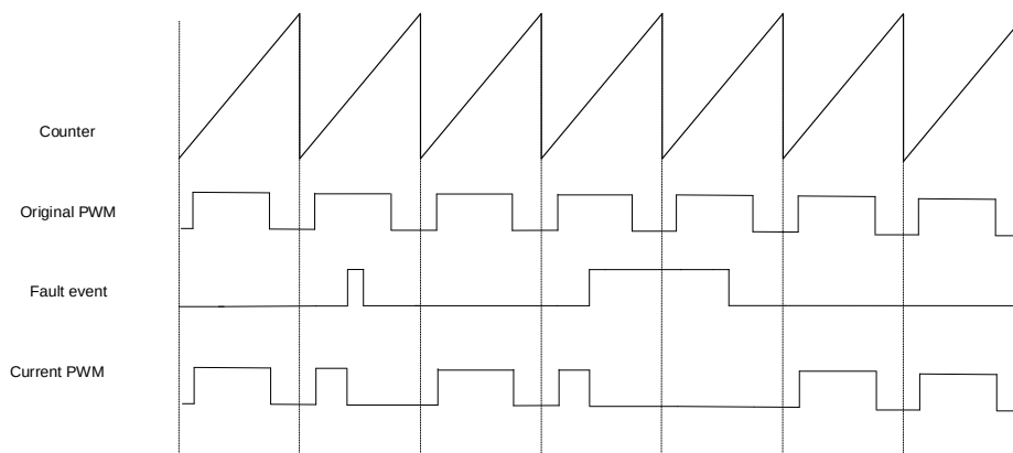
Figure 25-53. Fault automatic resume when FLT x RST bit is 1 and FLTAR = 1
