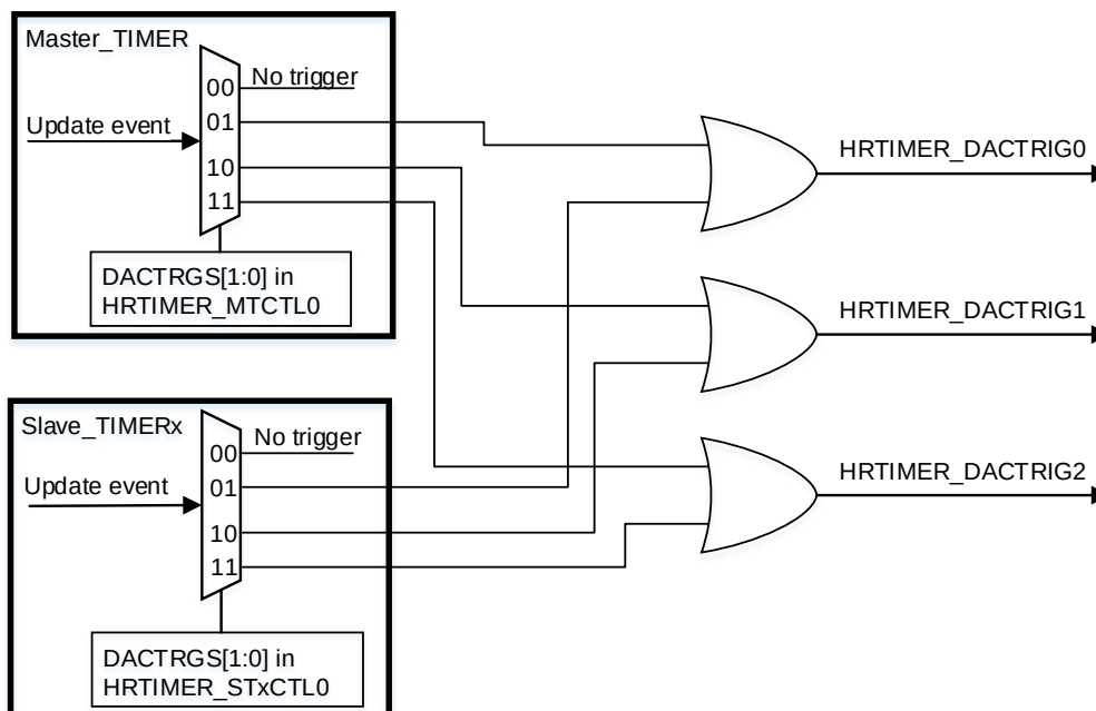
Figure 25-57. Trigger to DAC selection overview
