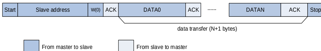
Figure 28-5. I2C communication flow with 7-bit address (Master Transmit)
