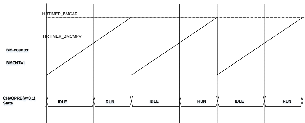
Figure 25-45. Bunch mode timing chart
