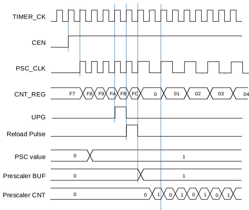
Figure 23-143. Counter timing diagram with prescaler division change from 1 to 2
