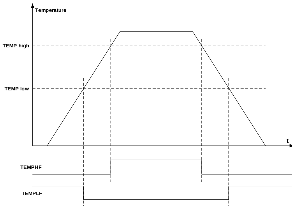
Figure 3-4. Temperature thresholds
