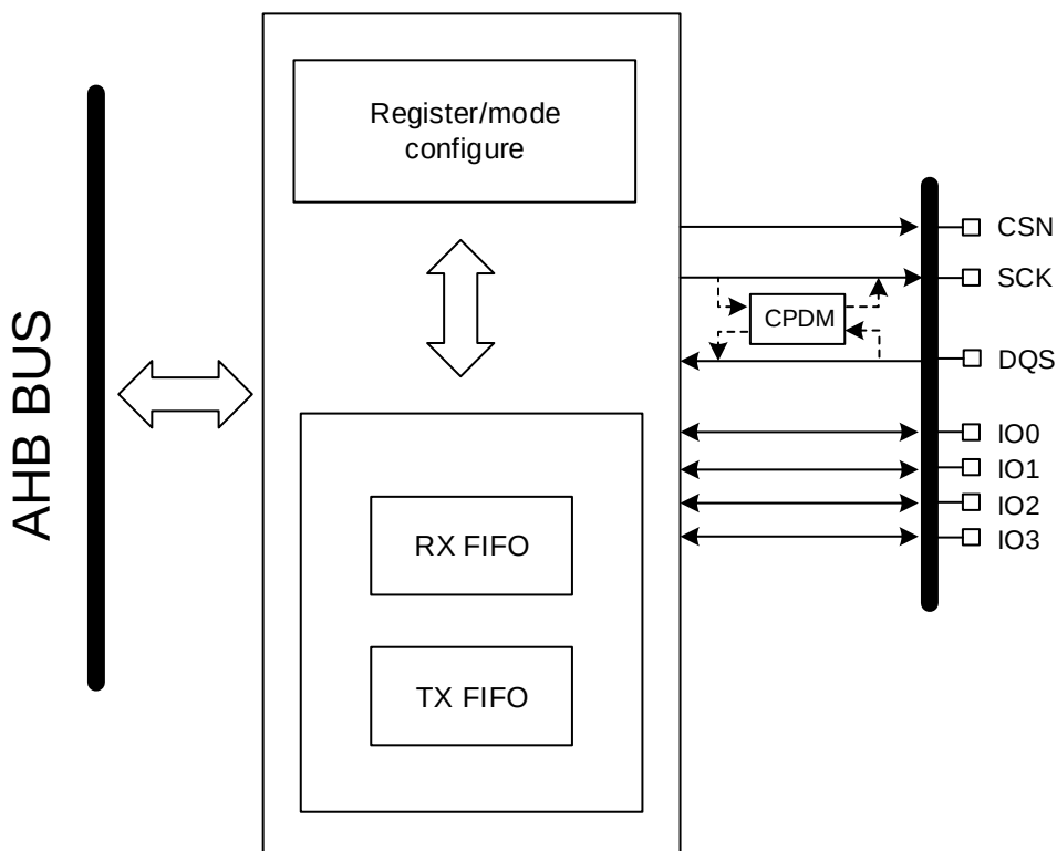
Figure 31-1 QSPI diagram
