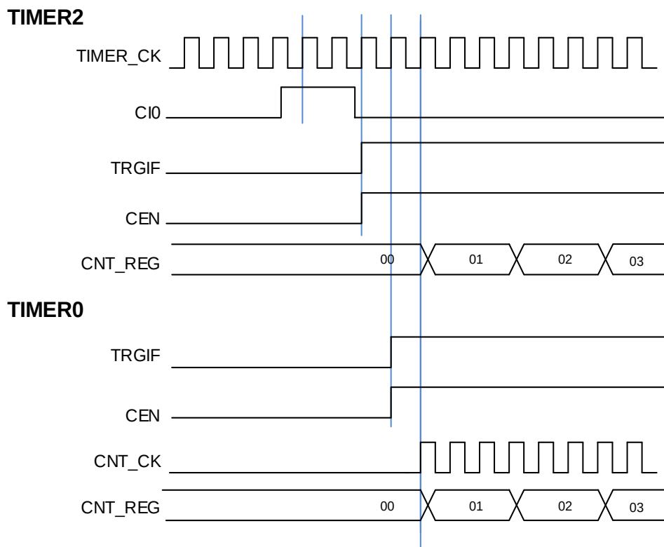
Figure 23-60. Trigger TIMER0 and TIMER2 by the CIO signal of TIMER2
