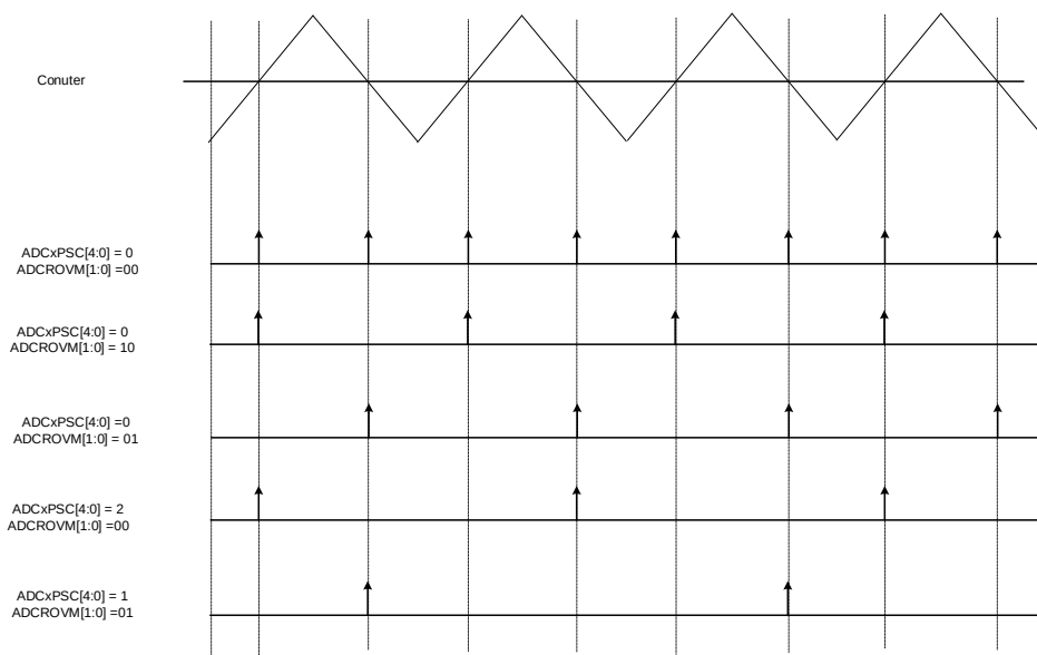
Figure 25-56. ADC trigger division in center aligned mode
