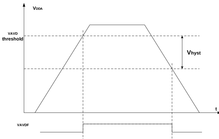
Figure 3-8. Waveform of the VAVD threshold
