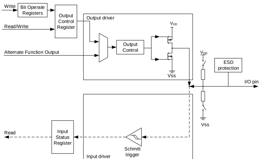
Figure 7-3. Output configuration
