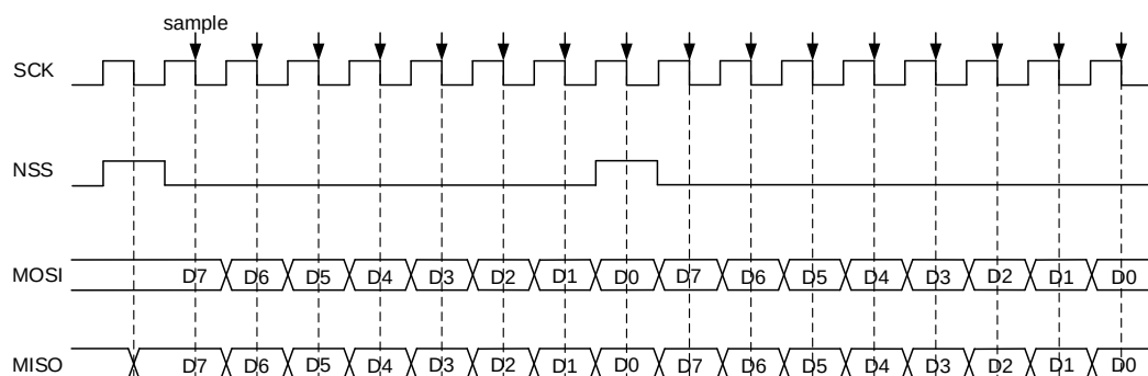
Figure 30-11. Timing diagram of TI master mode with continuous transfer
