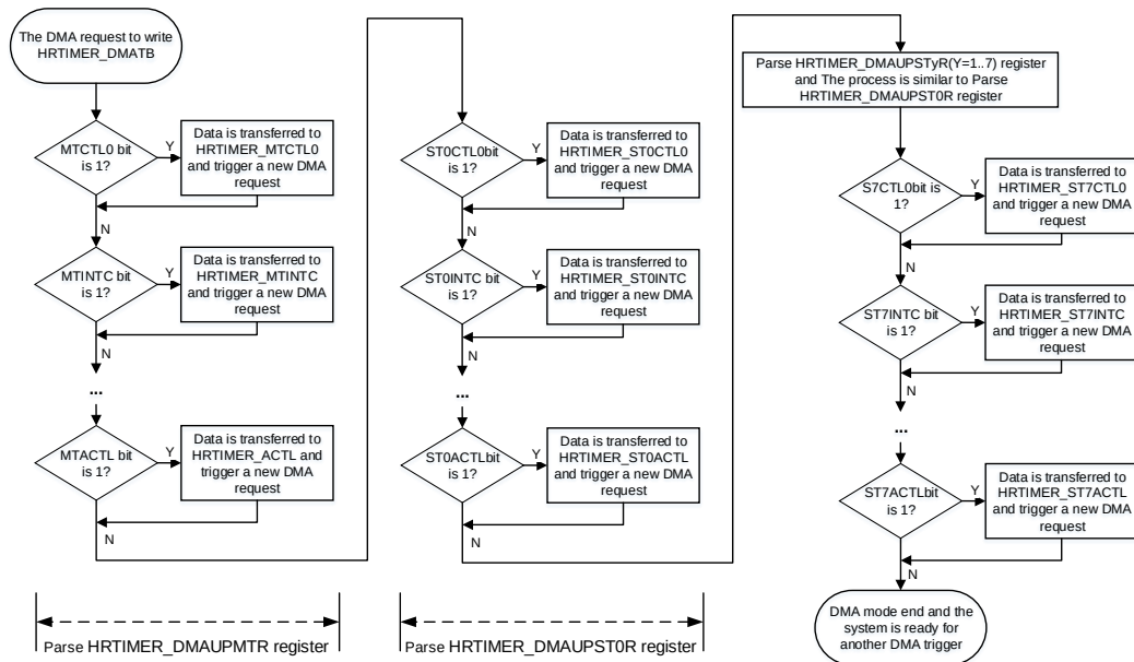
Figure 25-60. DMA mode operation flowchart
