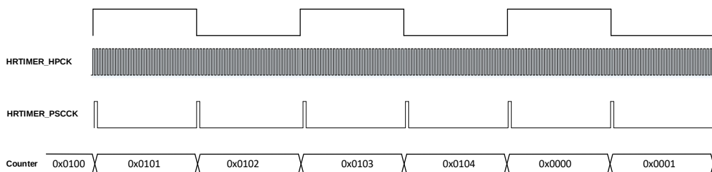
Figure 25-3. Counter clock when divided by 16
