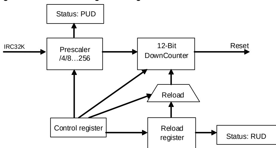
Figure 21-1. Free watchdog block diagram
