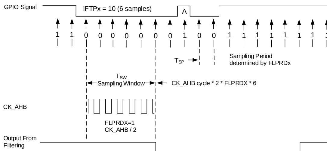
Figure 7-7. Input filtering clock cycle
