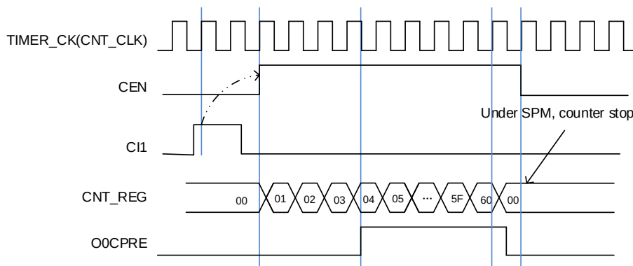
Figure 23-90. Single pulse mode TIMERx\_CHxCV = 0x04 , TIMERx\_CAR=0x60
