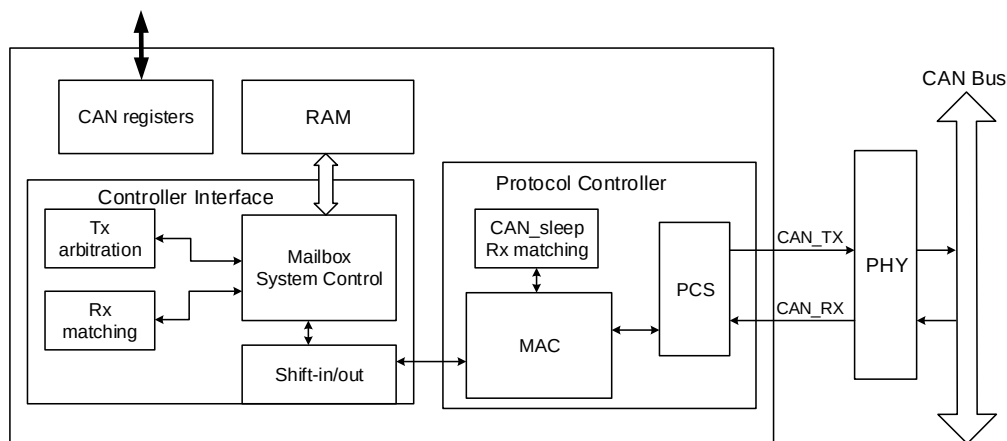
Figure 29-1. CAN module block diagram
