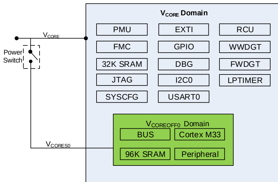
Figure 3-2. V CORE domain supply overview
