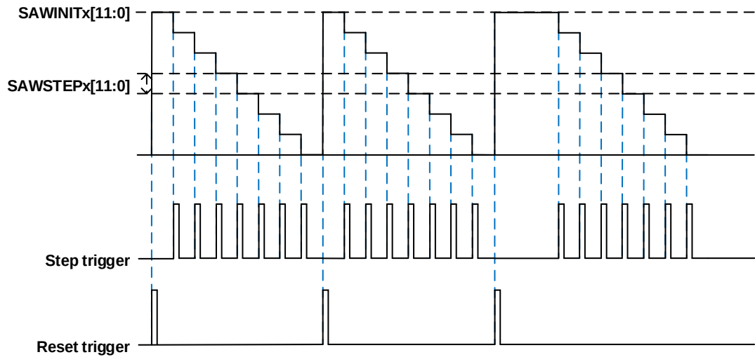
Figure 18-5. DAC sawtooth wave (SAWDIRx = 0)
