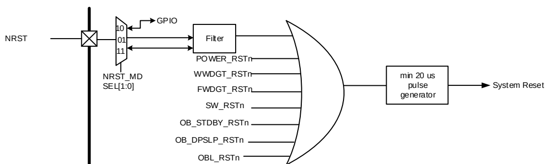
Figure 4-1. The system reset circuit
