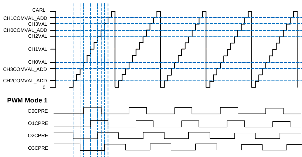
Figure 23-26. Four Channels outputs in Composite PWM mode
