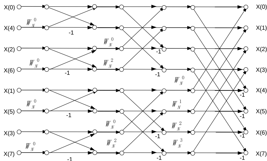
Figure 15-2 8 point DIT FFT flow diagram
