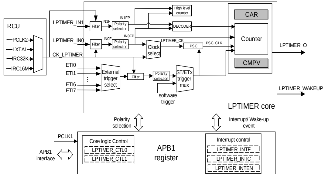
Figure 24-1. LPTIMER block diagram
