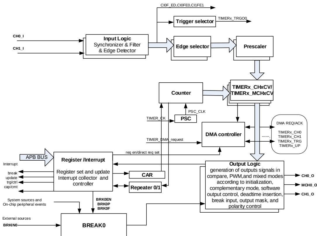
Figure 23-92. General level3 timer block diagram
