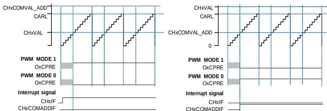
Figure 23-24. Channel x output PWM with CHxVAL or CHxCOMVAL_ADD exceeds CARL
