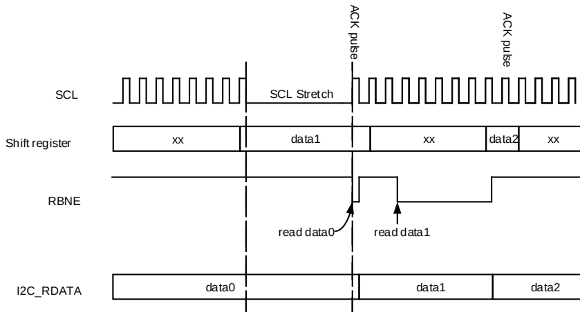
Figure 28-12. Data reception
