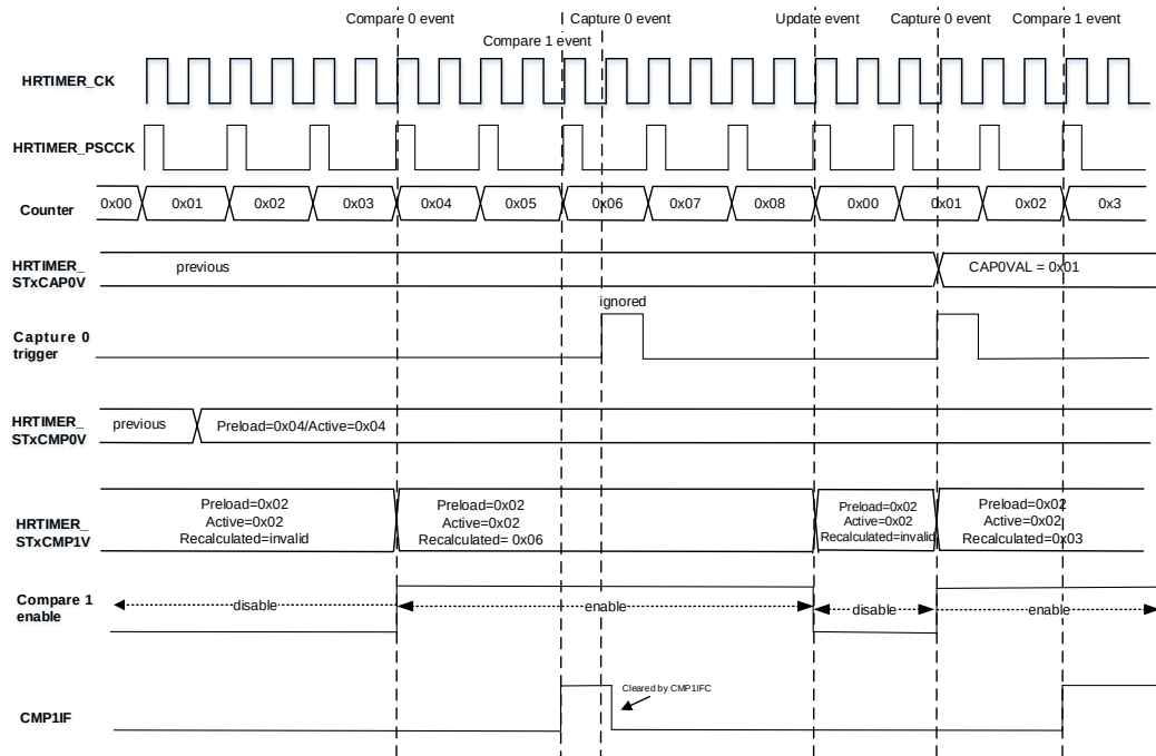
Figure 25-15. Compare 1 delayed mode 1
