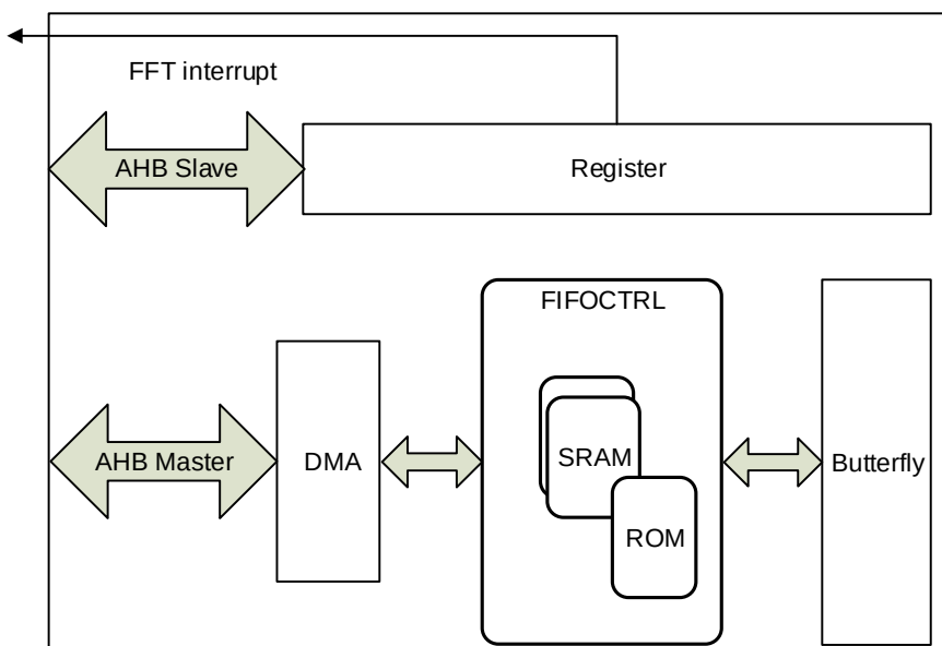
Figure 15-1. FFT module block diagram
