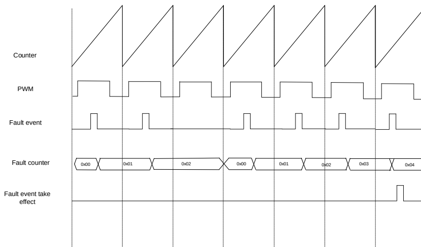
Figure 25-52. Fault counter when FLTxBLKS bit is 1, FLTRECCTL bit is 1 and FLTxCNT[3:0] = 0x03
