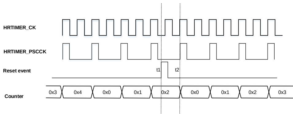
Figure 25-9 Reset event resynchronization when prescaling ratio is 64
