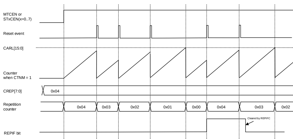
Figure 25-6. Repetition counter behavior in continuous mode
