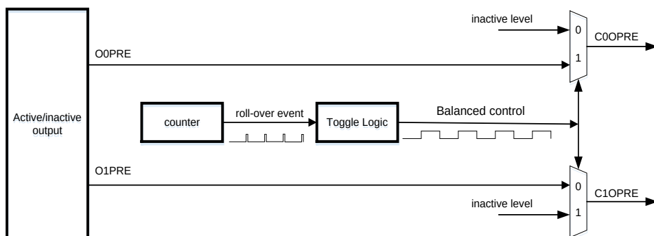
Figure 25-32. Structure chart in balanced mode
