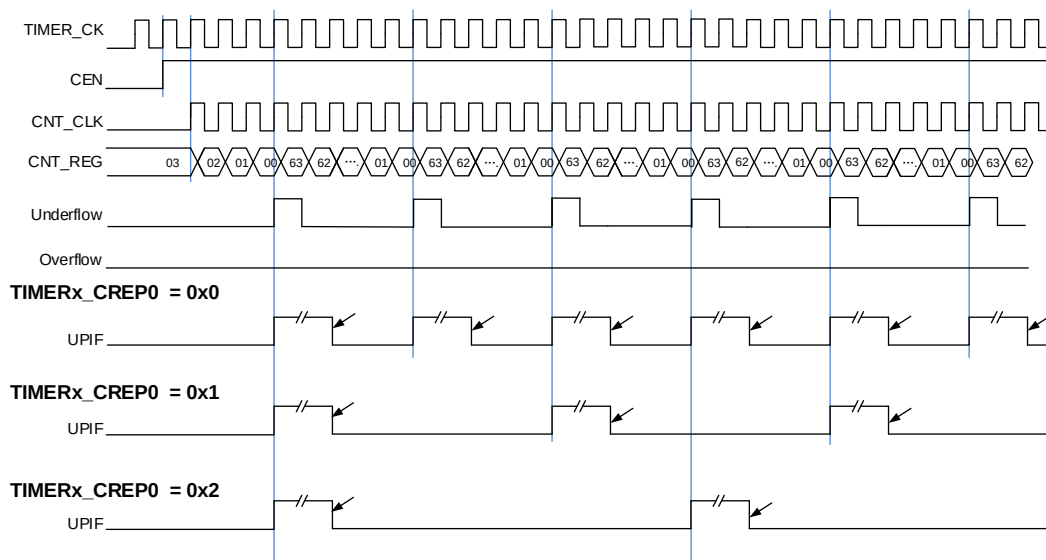
Figure 23-11. Repetition counter timing diagram of down counting mode
