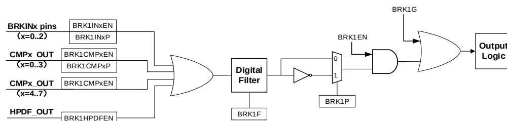
Figure 23-32. BREAK1 function logic diagram
