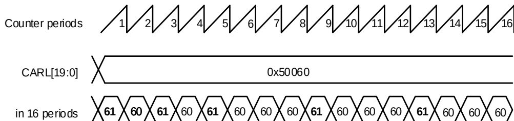
Figure 23-147. Adjustment mode schematic diagram
