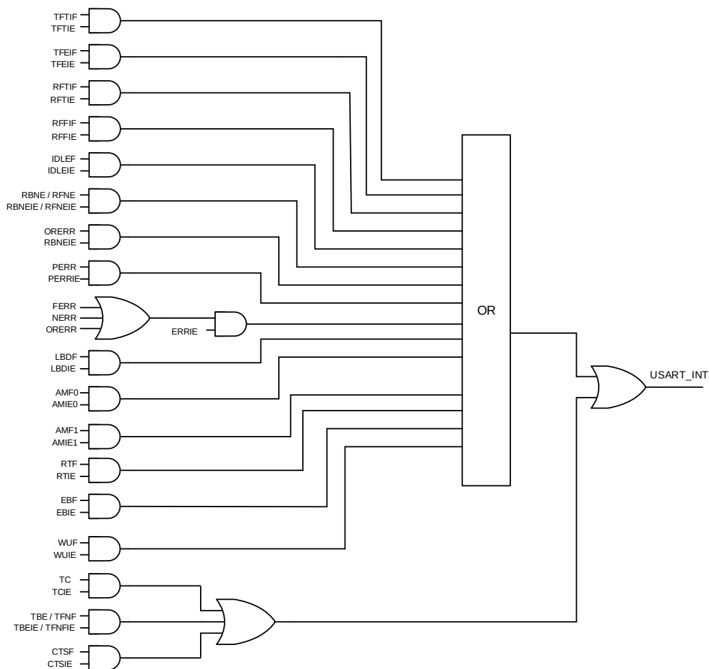
Figure 27-18. USART interrupt mapping diagram
