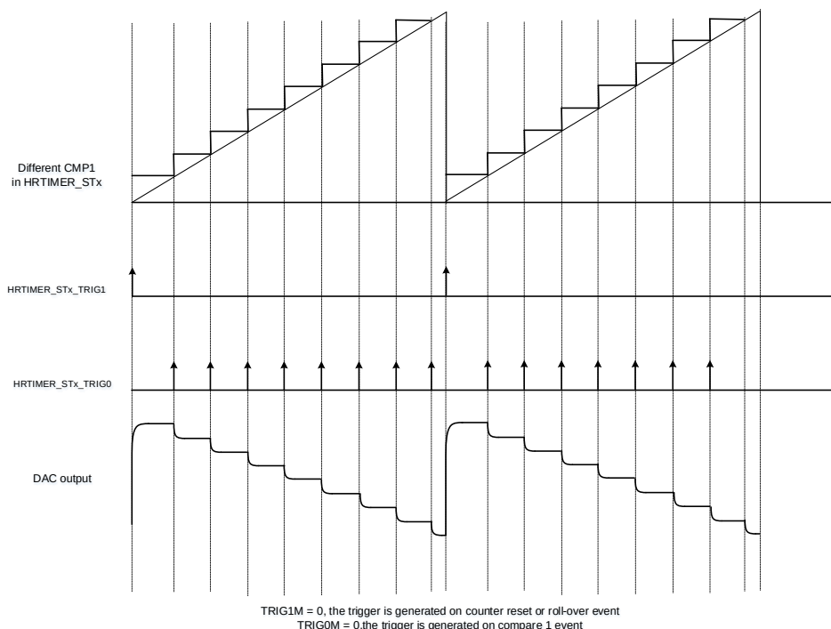
Figure 25-58. Trigger to DAC when TRIG0M = 0 and TRIG1M = 0
