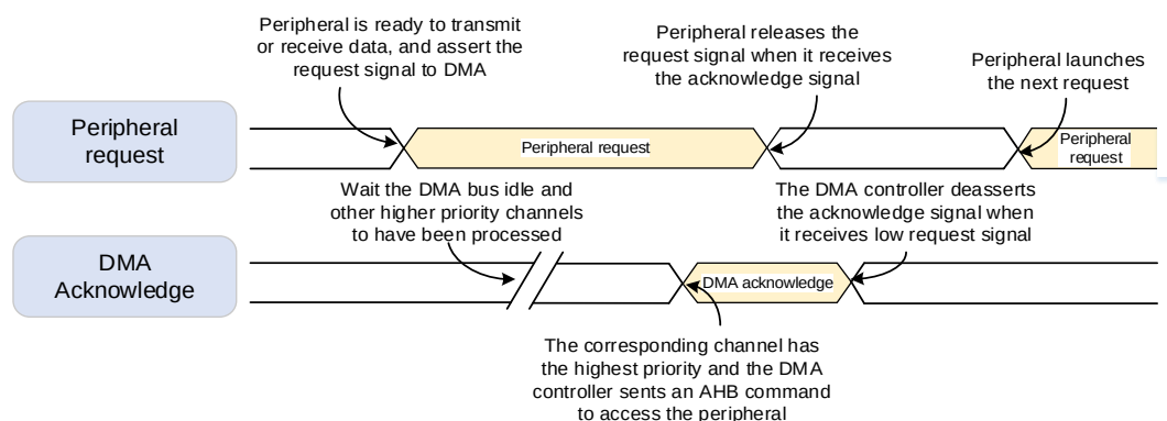
Figure 8-2. Handshake mechanism
