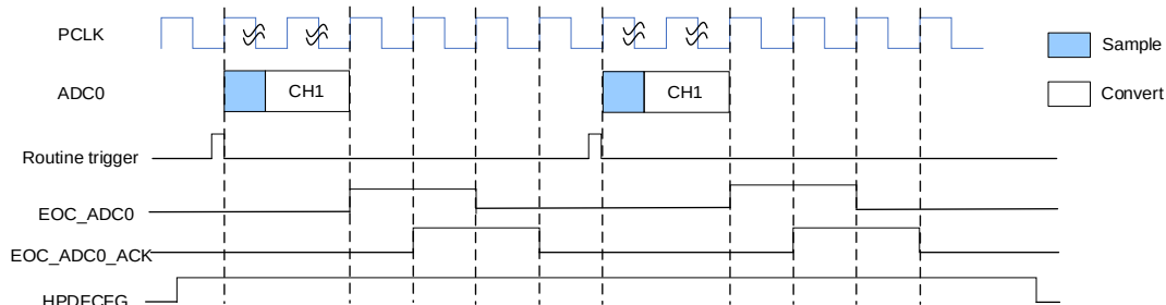
Figure 17-9. Schematic diagram of handshake signal between HPDF and ADC module
