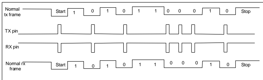
Figure 20-28. IrDA data modulation
