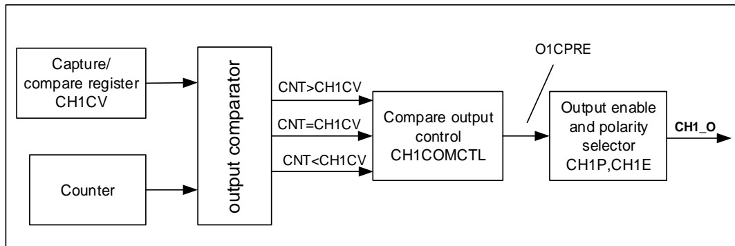
Figure 18-75. Channel output compare principle (CH1_O)
