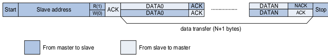
Figure 21-7. I2C communication flow with 10-bit address (Master Transmit)
