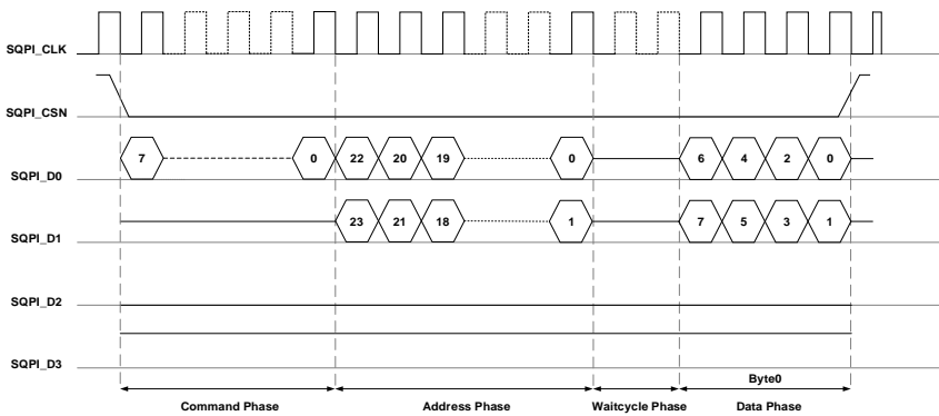
Figure 23-10. SQPI SDD Mode Timing
