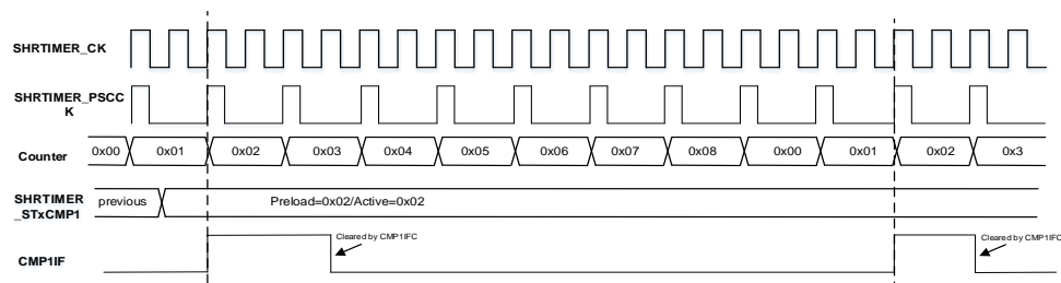
Figure 19-12. Compare 1 behavior with STxCAR=0x8, STxCMP1V=0x02
