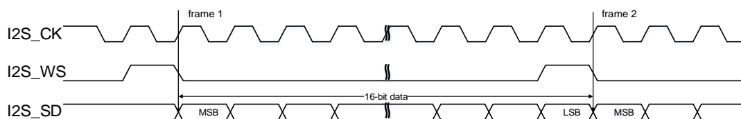
Figure 22-37. PCM standard short frame synchronization mode timing diagram
