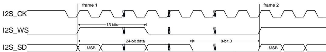
Figure 22-49. PCM standard long frame synchronization mode timing diagram (DTLEN=00, CHLEN=1, CKPL=0)
