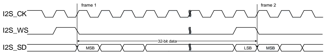
Figure 22-39. PCM standard short frame synchronization mode timing diagram (DTLEN=01, CHLEN=1, CKPL=0)
