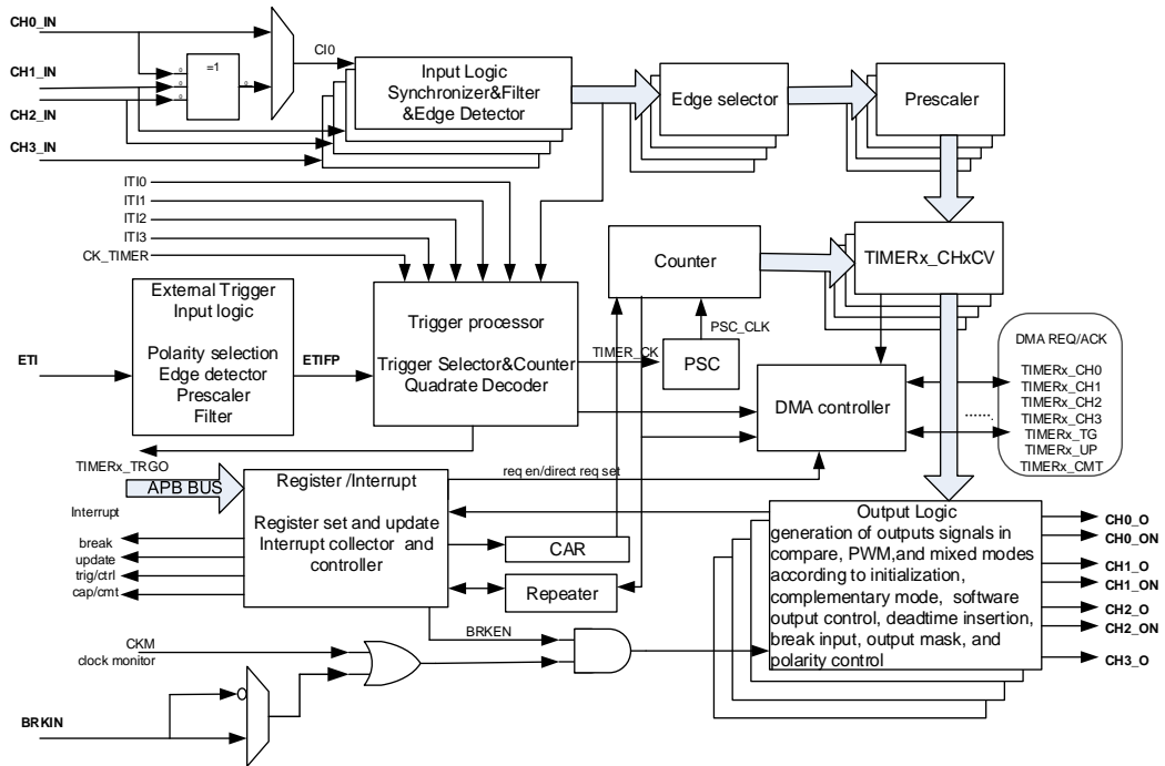
Figure 18-1. Advanced timer block diagram
