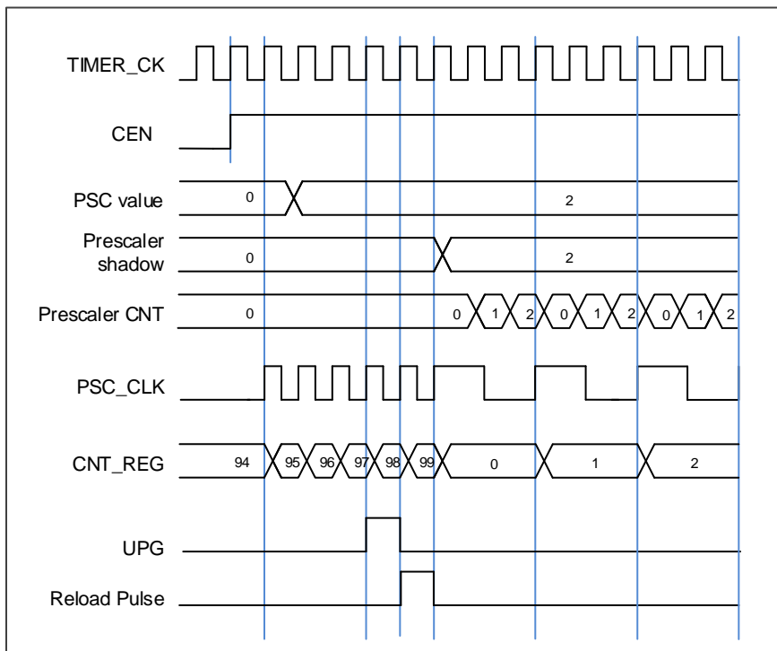
Figure 18-99. Timing chart of PSC value change from 0 to 2
