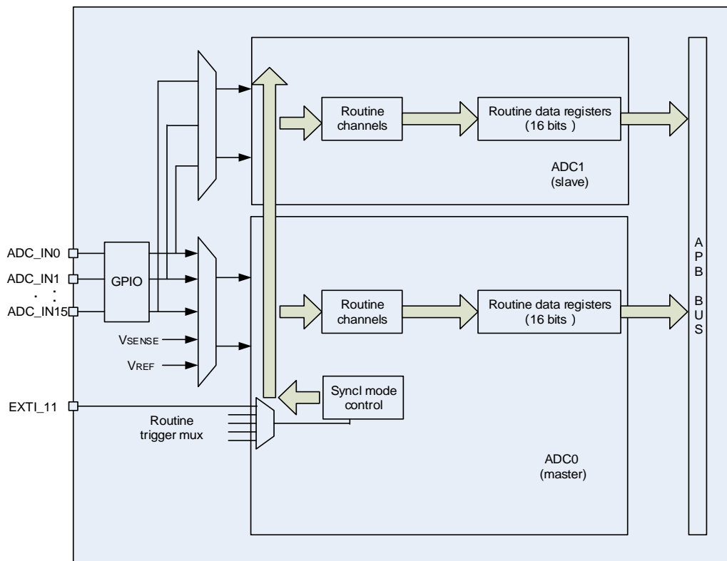
Figure 13-12. ADC sync block diagram
