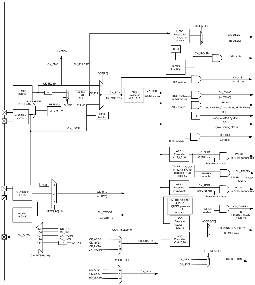
Figure 5-2. Clock tree
