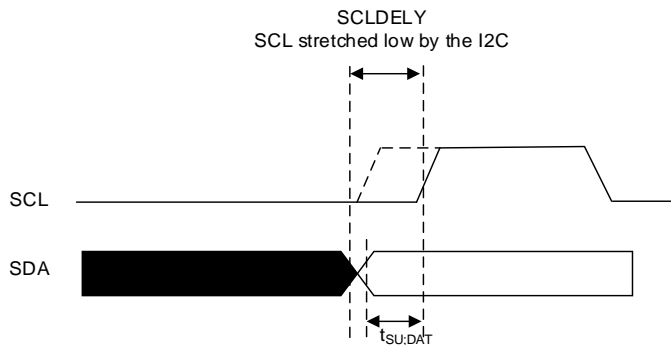
Figure 21-23. Data setup time
