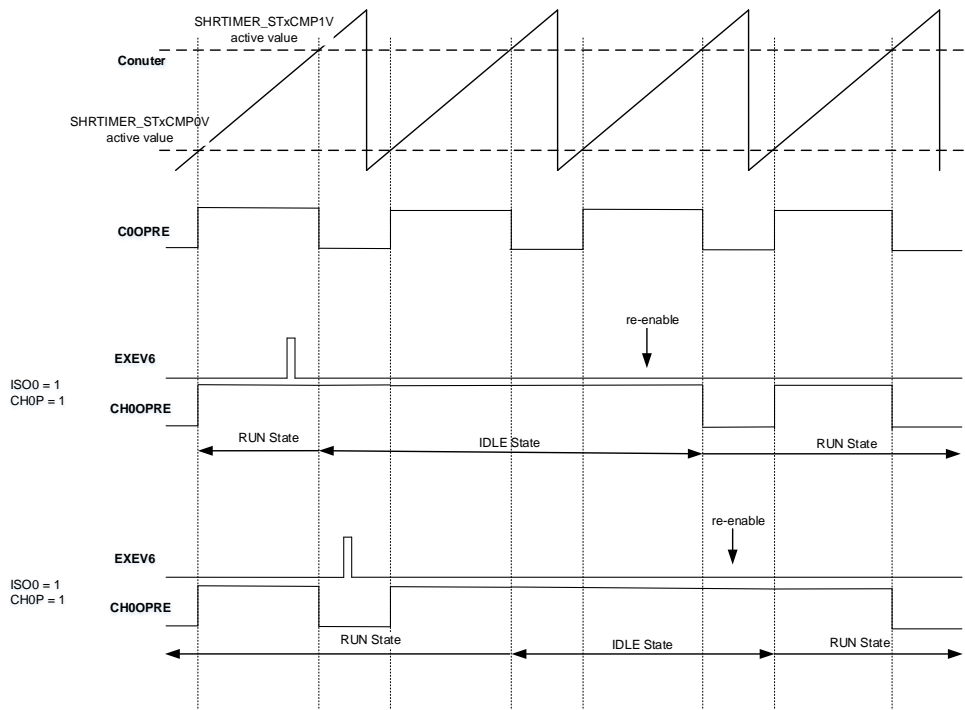
Figure 19-33. ISO0 = 1 and CHOP = 1 in delayed IDLE
