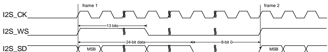
Figure 22-48. PCM standard long frame synchronization mode timing diagram
