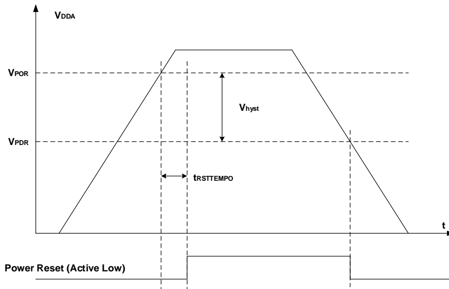
Figure 4-4. Waveform of the POR / PDR
