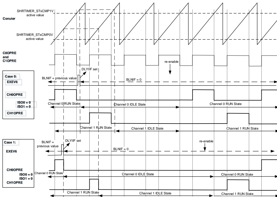
Figure 19-34. Balanced IDLE with ISO0 = 0 and ISO1 = 0
