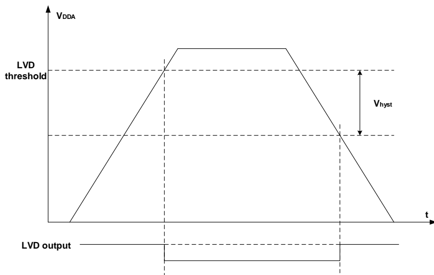
Figure 4-5. Waveform of the LVD threshold
