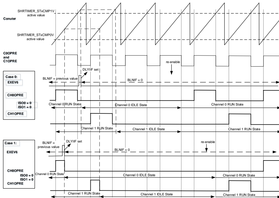
Figure 19-34. Balanced IDEL with ISO0 = 0 and ISO1 = 0
