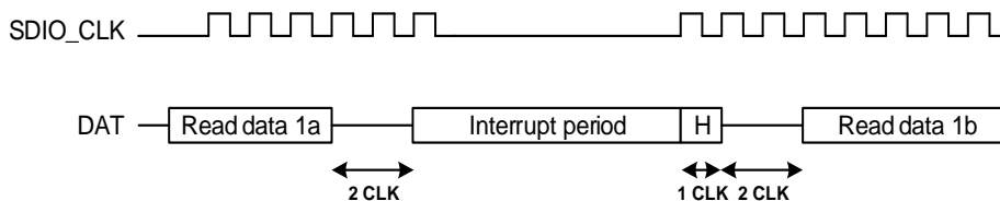
Figure 24-12. Read wait control by stopping SDIO_CLK
