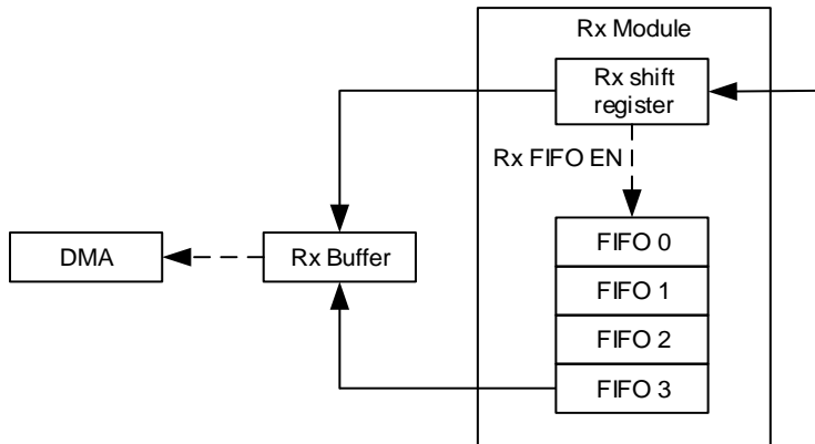
Figure 20-30. USART receive FIFO structure
