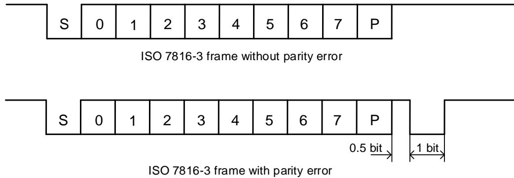
Figure 20-15. ISO7816-3 frame format
