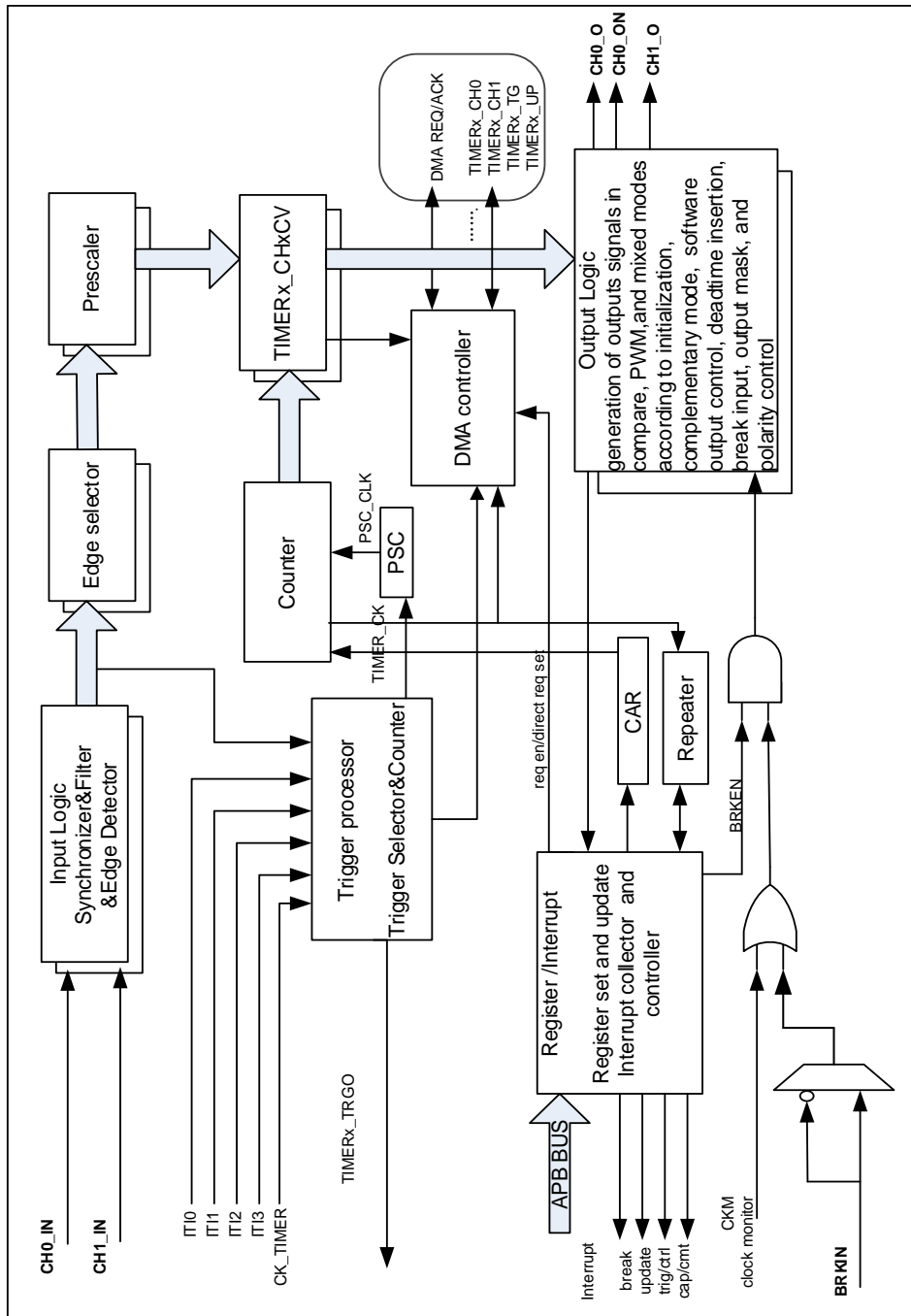
Figure 18-67. General level3 timer block diagram
