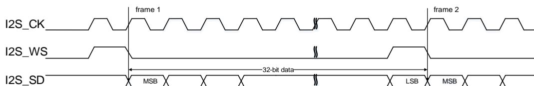
Figure 22-38. PCM standard short frame synchronization mode timing diagram
