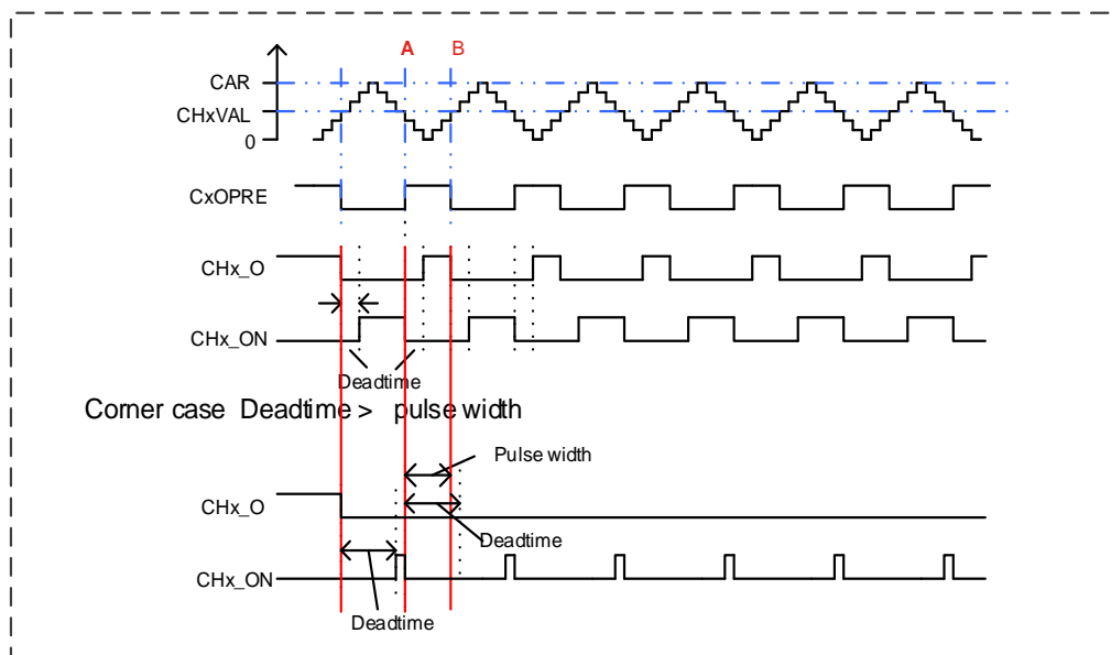
Figure 18-78. Complementary output with dead-time insertion
