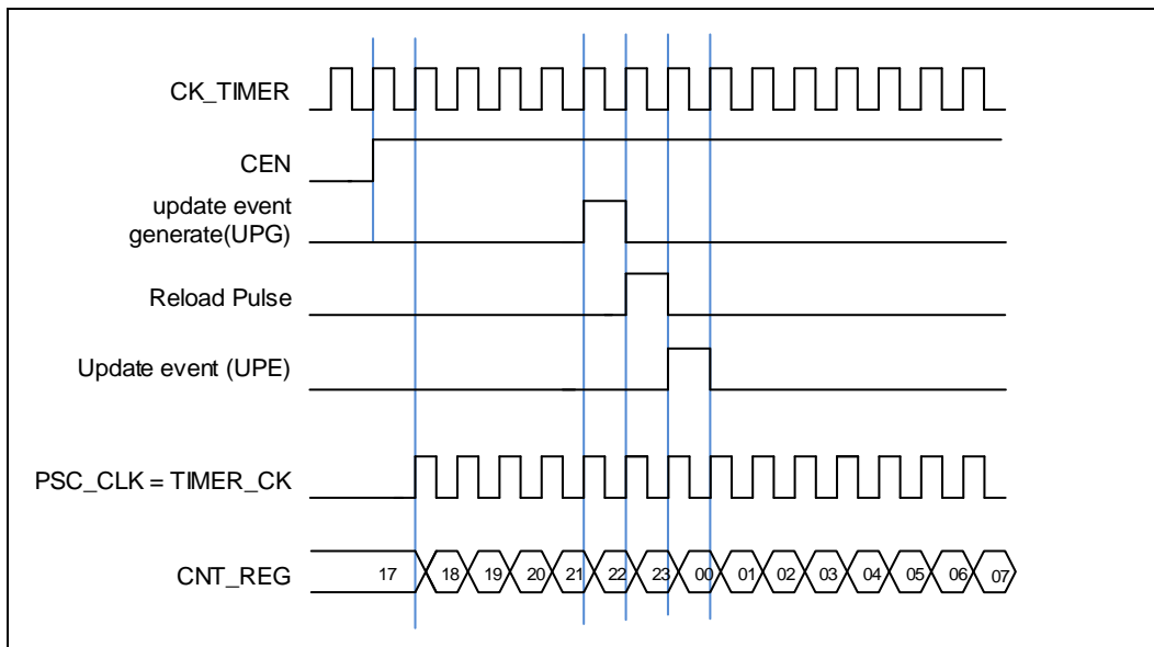
Figure 18-98. Timing chart of internal clock divided by 1
