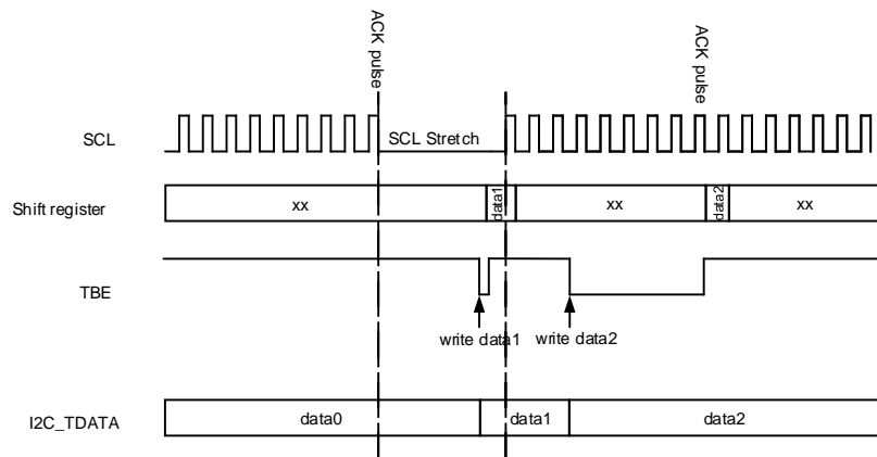
Figure 21-24. Data transmission
