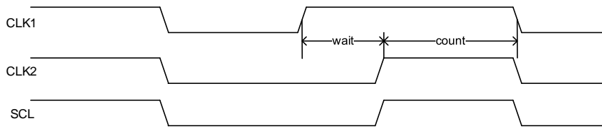
Figure 21-4. Clock synchronization
