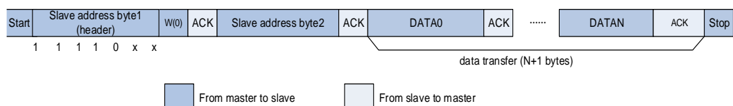
Figure 21-17. I2C communication flow with 10-bit address (Master Transmit)
