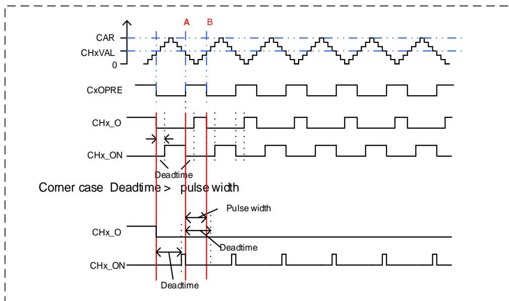
Figure 18-94. Complementary output with dead-time insertion
