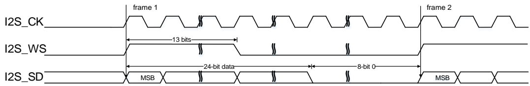
Figure 22-48. PCM standard long frame synchronization mode timing diagram (DTLEN=01, CHLEN=1, CKPL=1)
