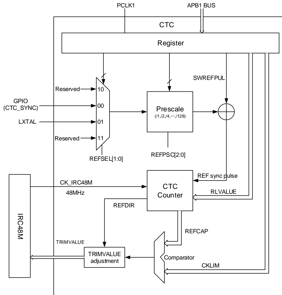
Figure 6-1. CTC overview
