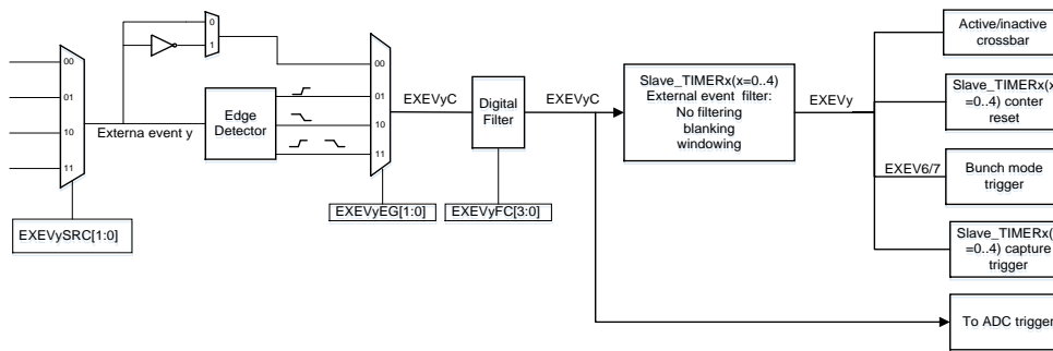
Figure 19-44. Extern event y(y=5..9) processed diagram
