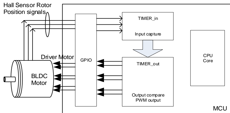
Figure 18-22. Hall sensor is used to BLDC motor
