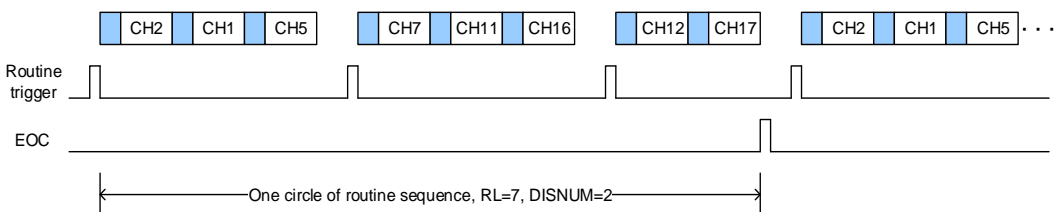
Figure 13-7. Discontinuous operation mode
