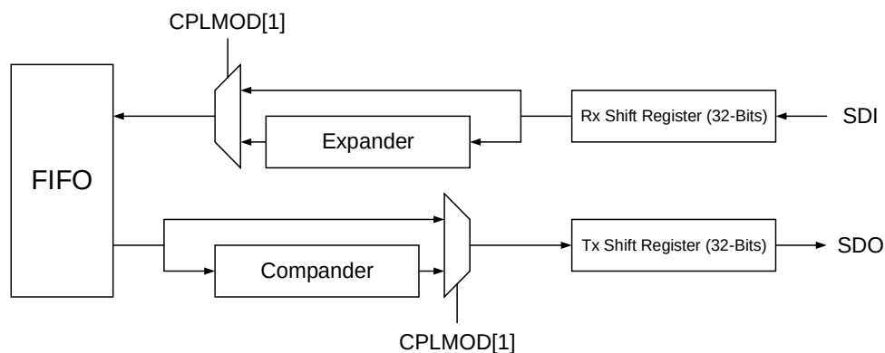
Figure 26-17 Compander data path
