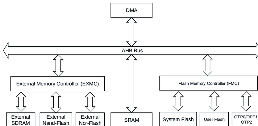
Figure 2-1. GD32F527xx memory access architecture
