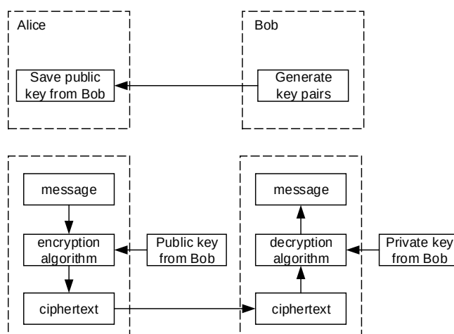
Figure 11-2. Flow chart of RSA algorithm
