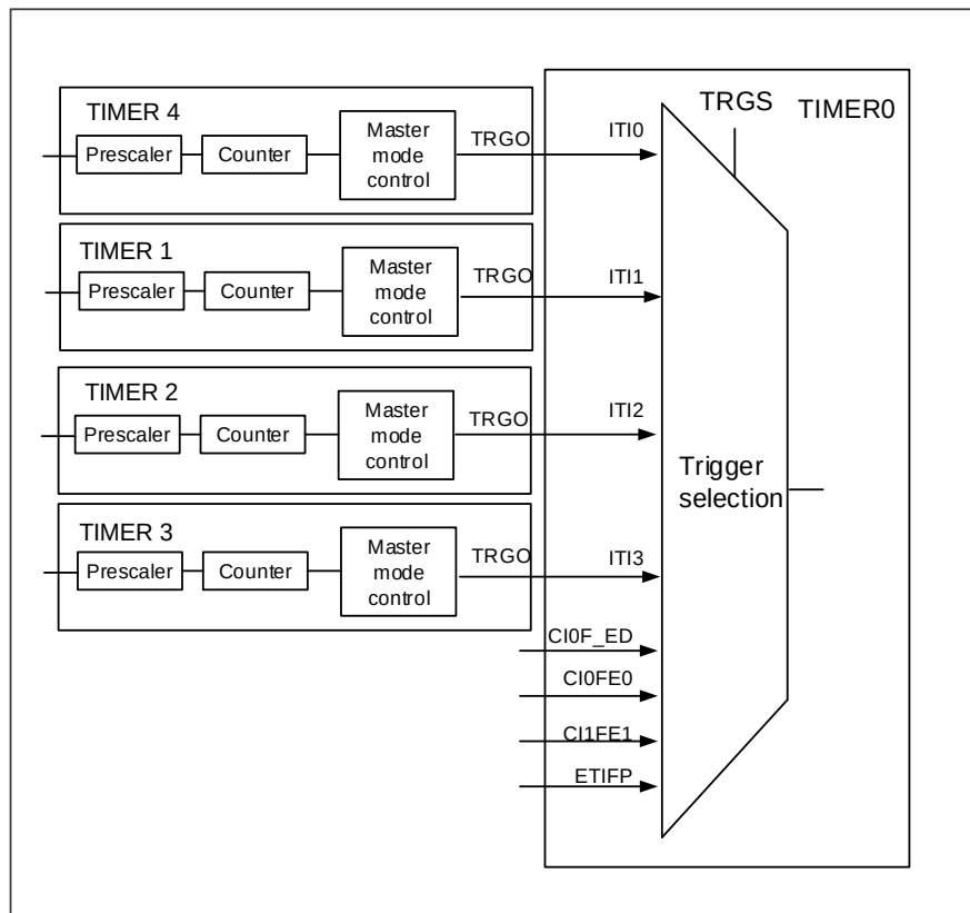
Figure 22-32. Timer0 master/slave mode timer example
