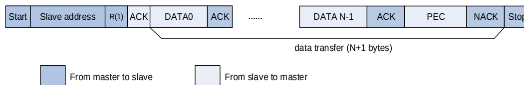
Figure 24-36. SMBus master receiver and slave transmitter communication flow
