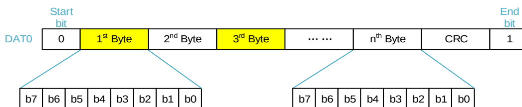
Figure 29-9. 1-bit data bus width
