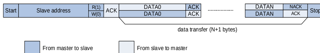
Figure 24-6. I2C communication flow with 7-bit address
