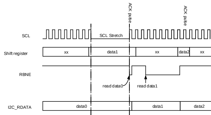
Figure 24-25. Data reception
