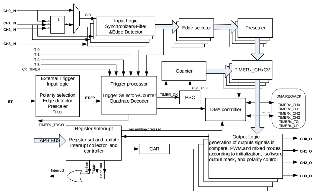
Figure 22-34. General Level 0 timer block diagram
