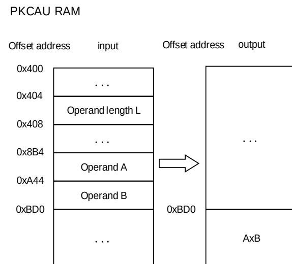
Figure 11-7. Arithmetic multiplication
