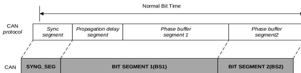
Figure 31-11. The bit time
