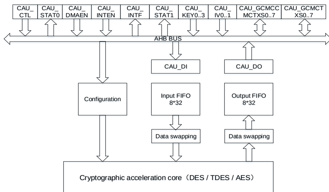
Figure 13-3. CAU diagram
