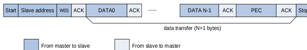
Figure 24-35. SMBus master transmitter and slave receiver communication flow
