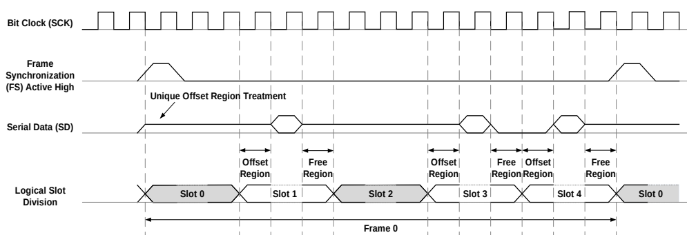
Figure 26-11 SD output management
