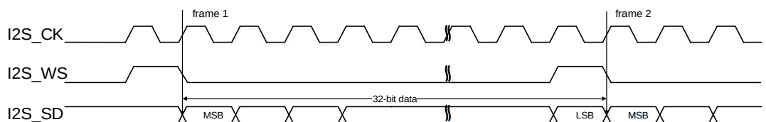
Figure 25-36. PCM standard short frame synchronization mode timing diagram (DTLEN=10, CHLEN=1, CKPL=0)
