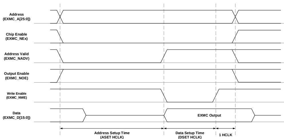
Figure 30-12. Mode 2 write access
