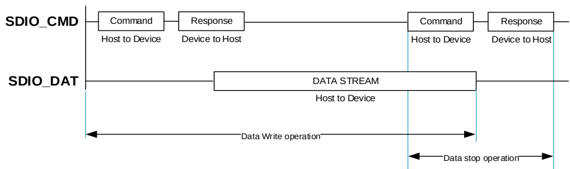
Figure 29-5. SDIO sequential write operation
