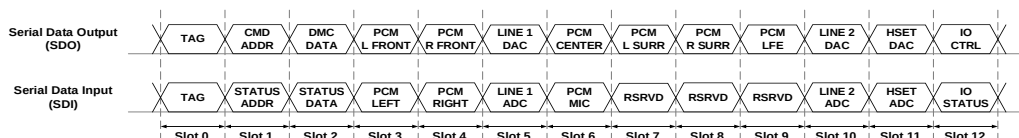
Figure 26-14 AC'97 tag definition
