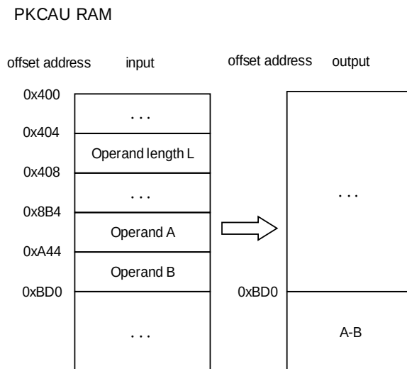
Figure 11-6. Arithmetic subtraction
