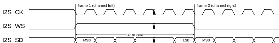
Figure 25-25. MSB justified standard timing diagram (DTLEN=10, CHLEN=1, CKPL=1)
