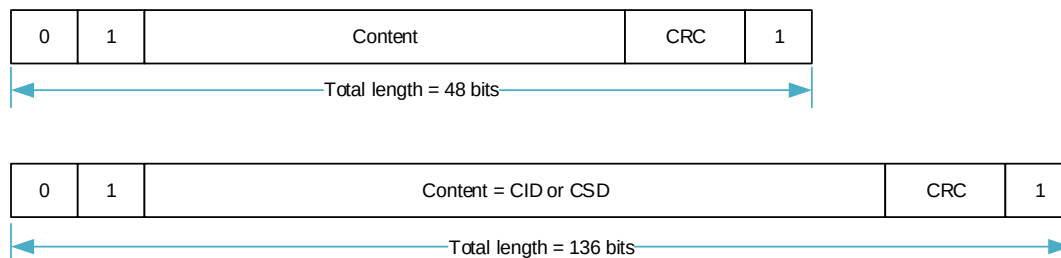
Figure 29-8. Response Token Format
