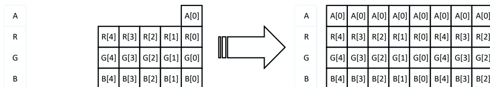
Figure 15-4. Pixel extension from 'ARGB1555' or 'ARGB4444' to 'ARGB8888'
