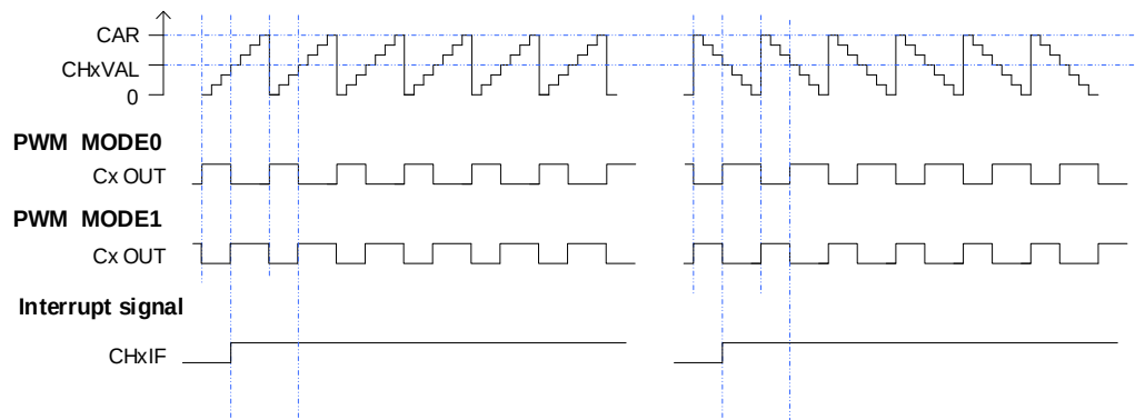
Figure 22-45. CAPWM timechart
