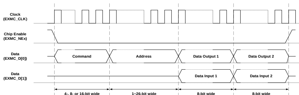
Figure 30-24. SPI-PSRAM access
