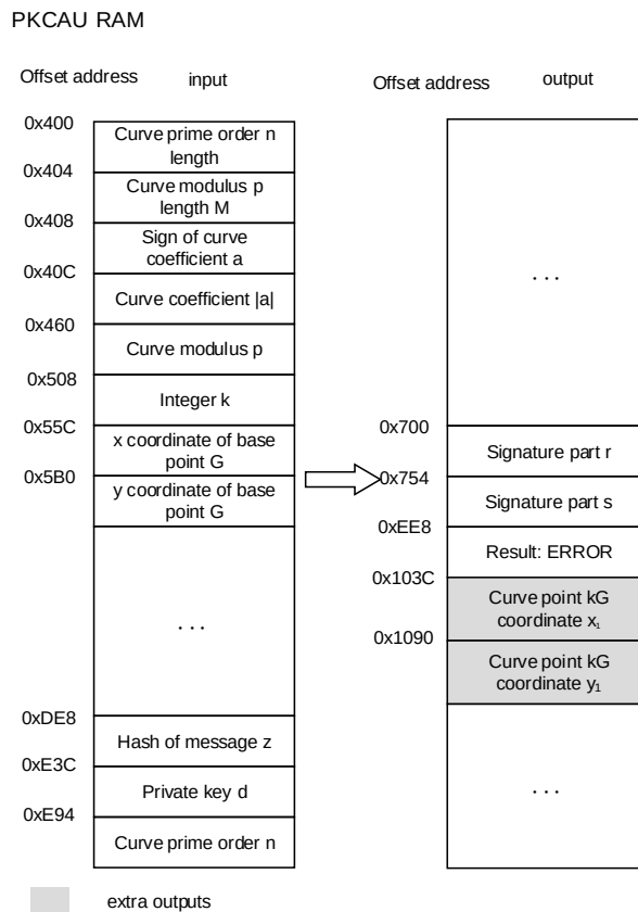
Figure 11-22. ECDSA sign
