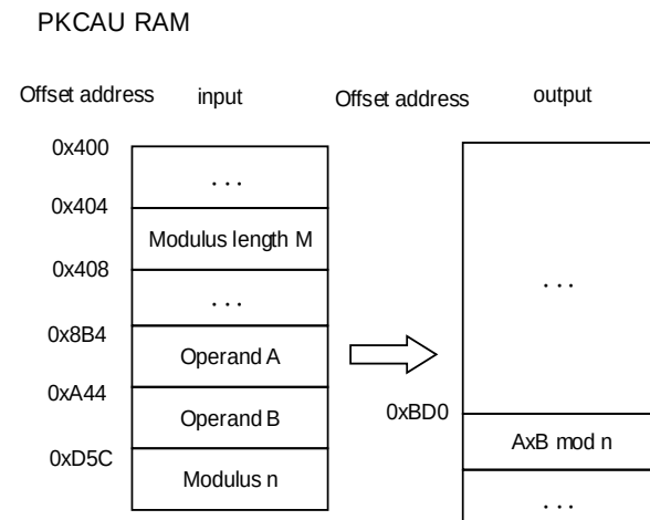
Figure 11-14. Montgomery multiplication
