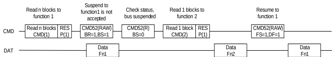
Figure 29-14. Function2 read cycle inserted during function1 multiple read cycle
