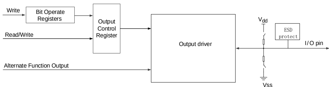
Figure 8-3. Basic structure of Output configuration
