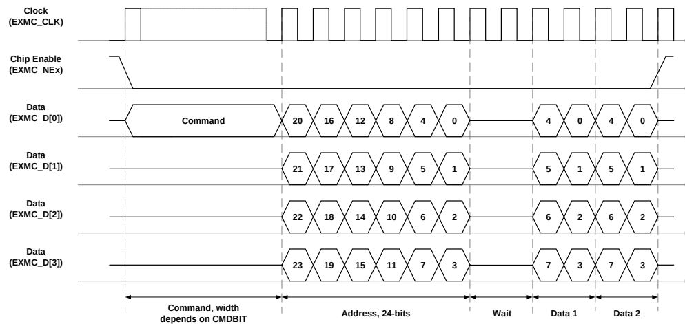
Figure 30-25. SQPI-PSRAM access
