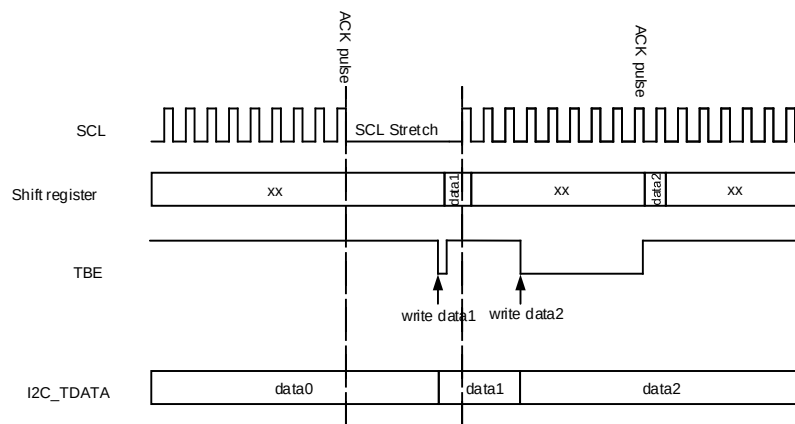
Figure 24-24. Data transmission
