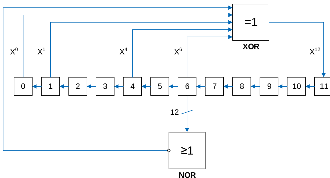
Figure 19-2. DAC LFSR algorithm
