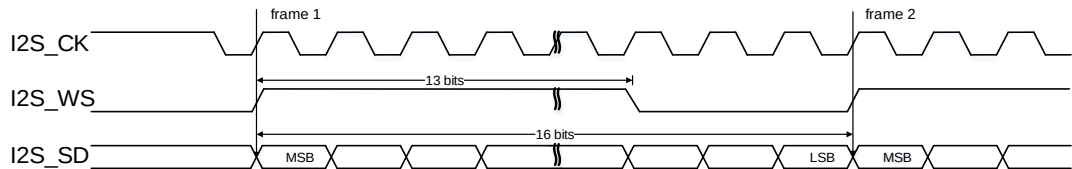
Figure25-43. PCM standard long frame synchronization mode timing diagram (DTLEN=00, CHLEN=0, CKPL=1)
