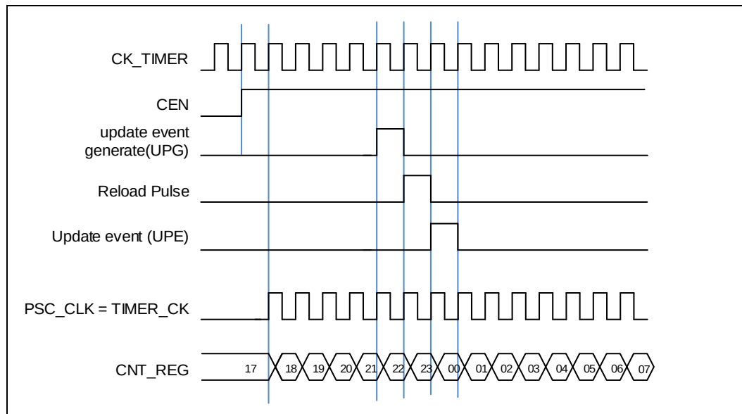
Figure 22-35. Timing chart of internal clock divided by 1
