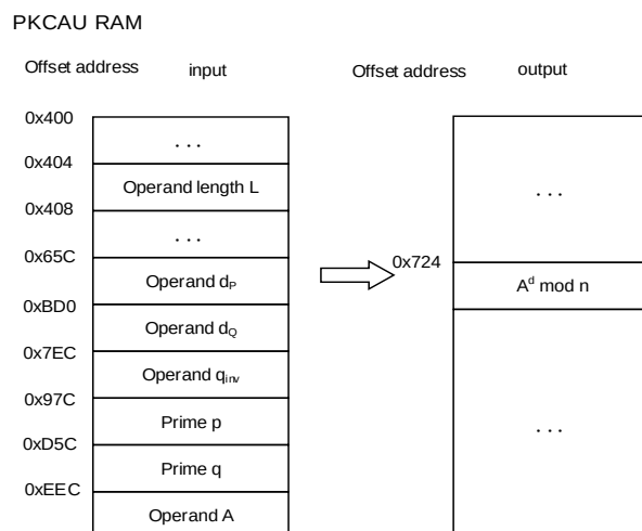
Figure 11-18. RSA CRT exponentiation
