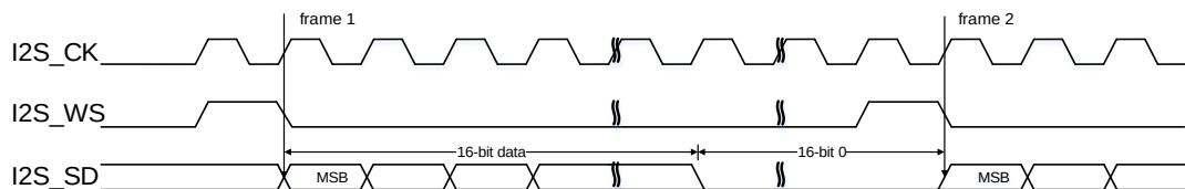
Figure 25-40. PCM standard short frame synchronization mode timing diagram (DTLEN=00, CHLEN=1, CKPL=0)
