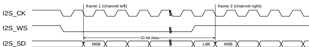
Figure 25-17. I2S Philips standard timing diagram (DTLEN=10, CHLEN=1, CKPL=1)
