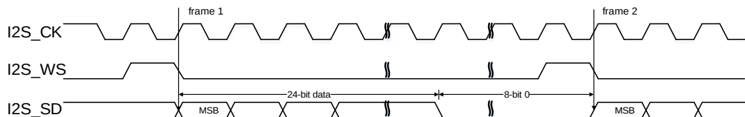
Figure25-39. PCM standard short frame synchronization mode timing diagram (DTLEN=01, CHLEN=1, CKPL=1)
