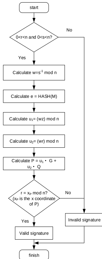
Figure 11-4. Flow chart of ECDSA verification
