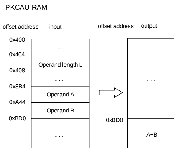
Figure 11-5. Arithmetic addition
