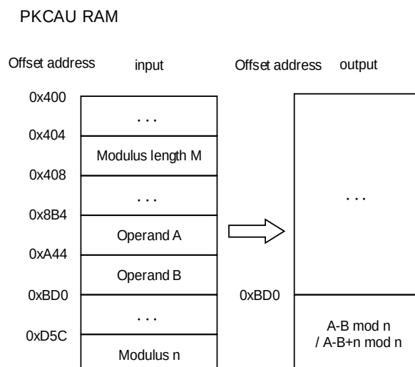
Figure 11-11. Modular subtraction
