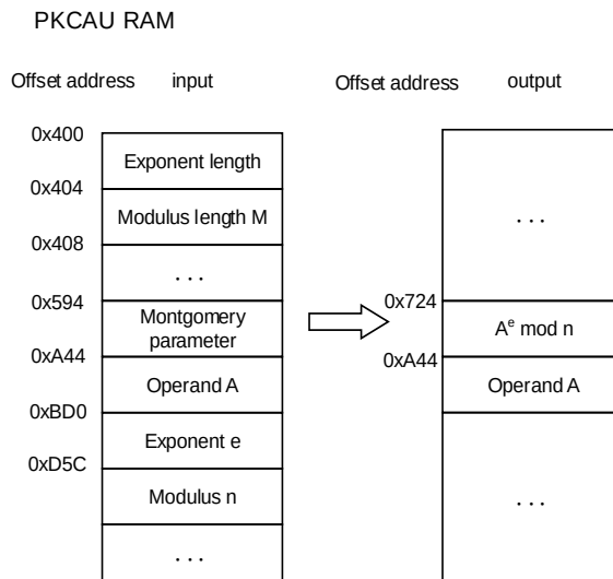
Figure 11-16. Modular exponentiation of fast mode
