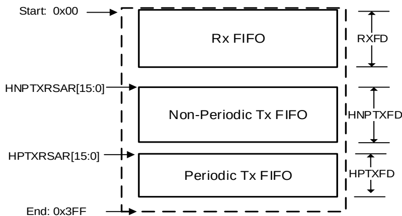
Figure 34-6. HOST mode FIFO space in SRAM
