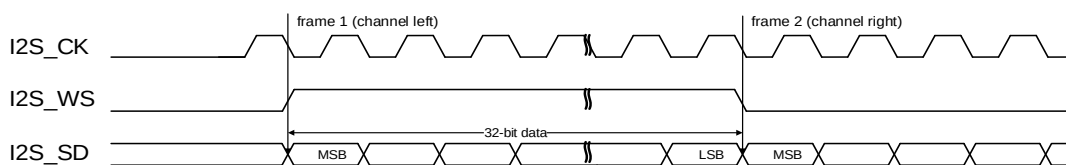
Figure 25-24. MSB justified standard timing diagram (DTLEN=10, CHLEN=1, CKPL=0)
