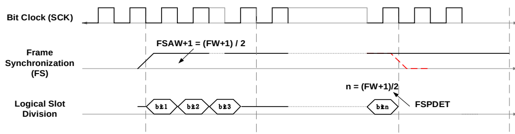
Figure 26-19 Frame synchronization postponed detection
