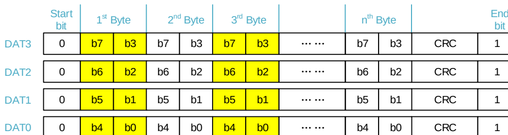
Figure 29-10. 4-bit data bus width
