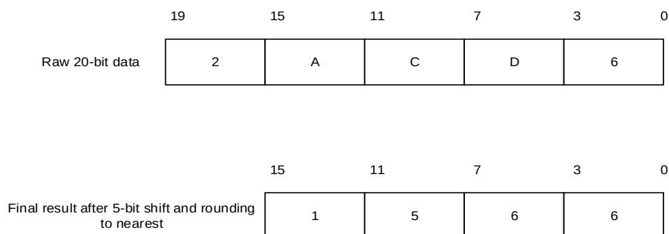
Figure 18-12. Numerical example with 5-bits shift and rounding
