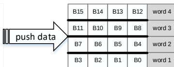
Figure 14-6. Data packing/unpacking when PWIDTH = '10'
