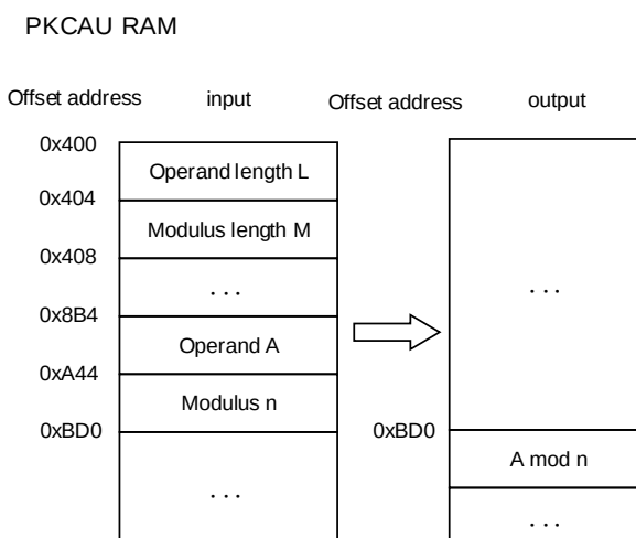
Figure 11-9. Modular reduction
