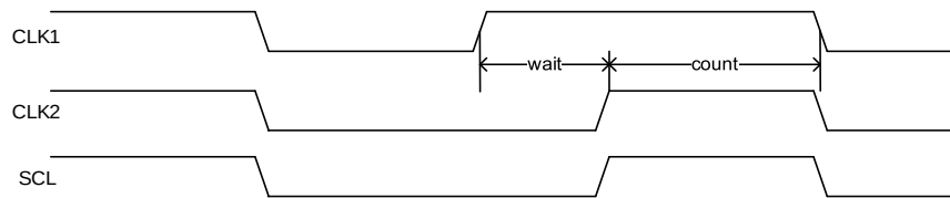
Figure 24-4. Clock synchronization
