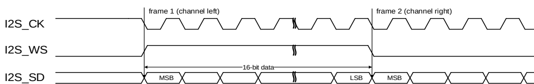
Figure 25-23. MSB justified standard timing diagram (DTLEN=00, CHLEN=0, CKPL=1)
