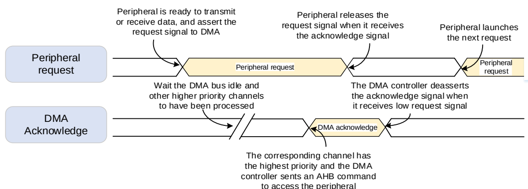
Figure 14-3. Handshake mechanism
