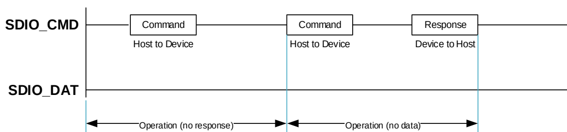
Figure 29-1. SDIO “no response” and “no data” operations
