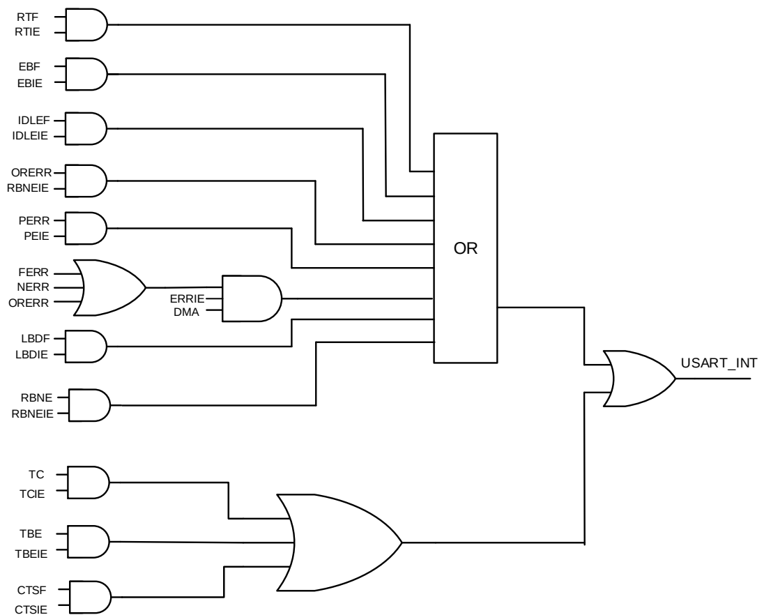
Figure 23-16. USART interrupt mapping diagram
