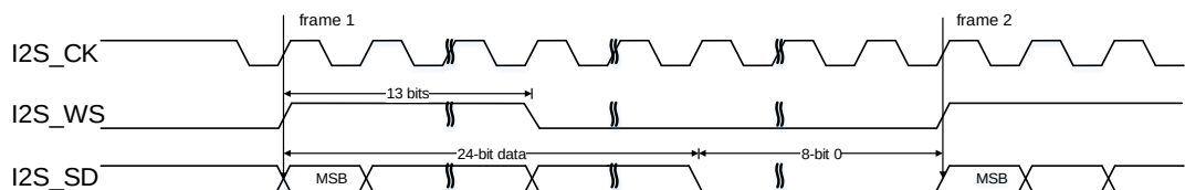
Figure 25-47. PCM standard long frame synchronization mode timing diagram (DTLEN=01, CHLEN=1, CKPL=1)
