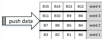
Figure 14-5. Data packing/unpacking when PWIDTH = '01'
