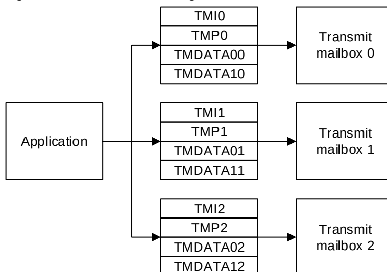
Figure 31-2. Transmission register
