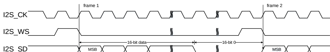
Figure 25-41. PCM standard short frame synchronization mode timing diagram (DTLEN=00, CHLEN=1, CKPL=1)
