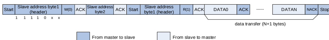
Figure 24-20. I2C communication flow with 10-bit address (Master Receive when HEAD10R=0)
