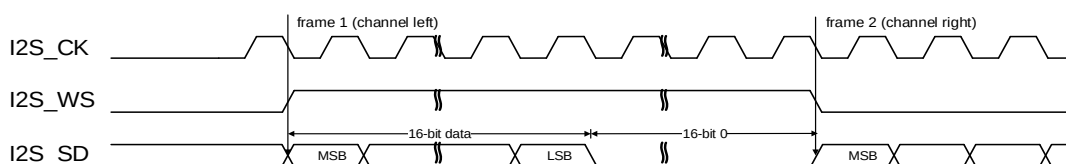
Figure 25-28. MSB justified standard timing diagram (DTLEN=00, CHLEN=1, CKPL=0)
