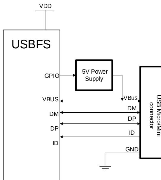
Figure 33-3. Connection with OTG mode
