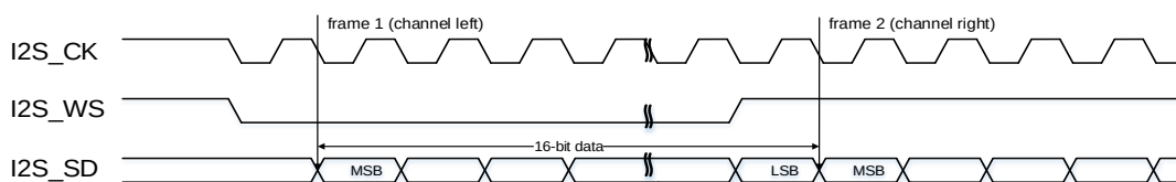
Figure 25-15. I2S Philips standard timing diagram (DTLEN=00, CHLEN=0, CKPL=1)
