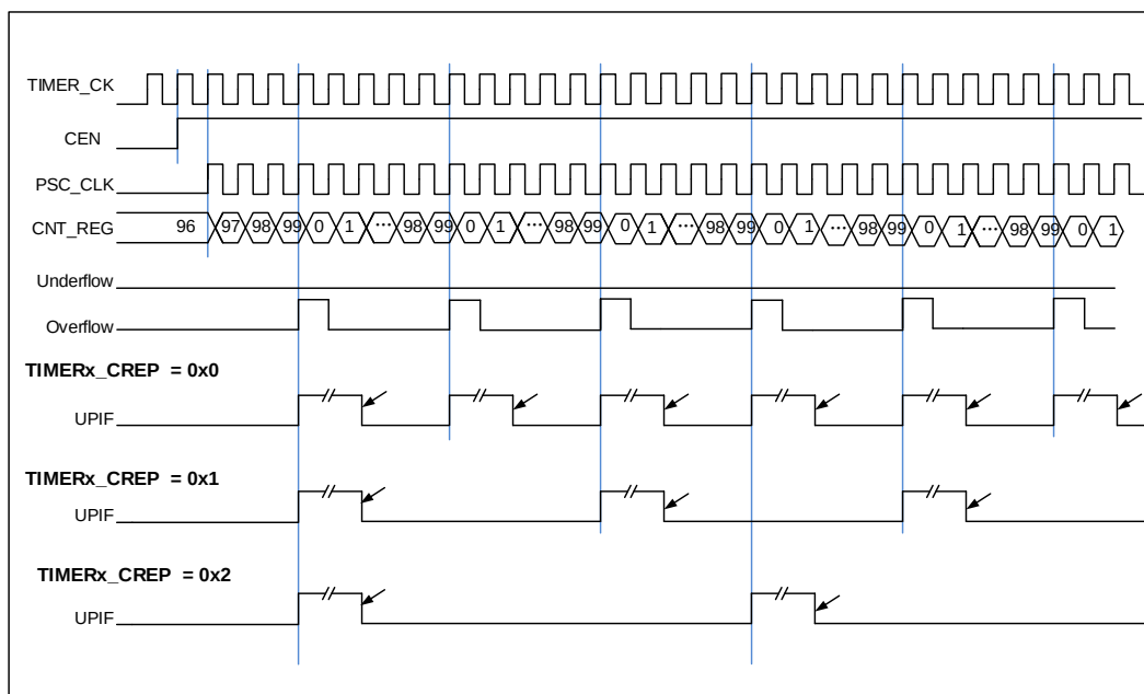
Figure 22-10. Repetition timechart for up-counter
