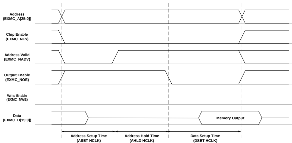
Figure 30-16. Mode D read access
