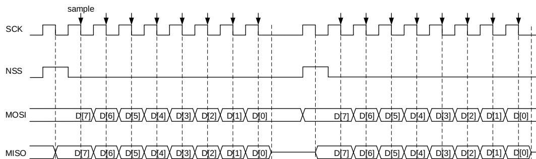
Figure 25-8. Timing diagram of TI master mode with discontinuous transfer
