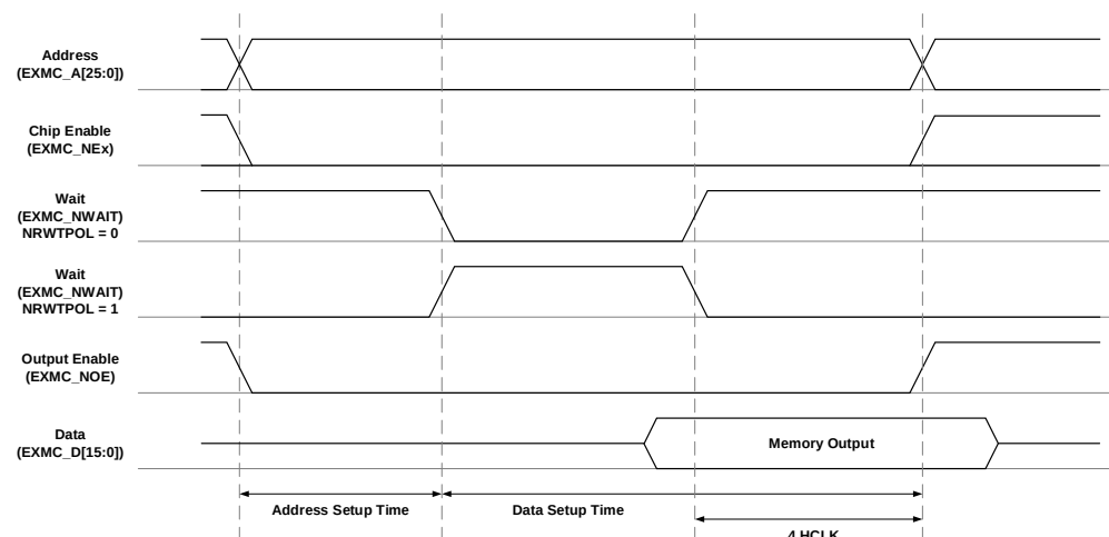
Figure 30-20. Read access timing diagram under async-wait signal assertion
