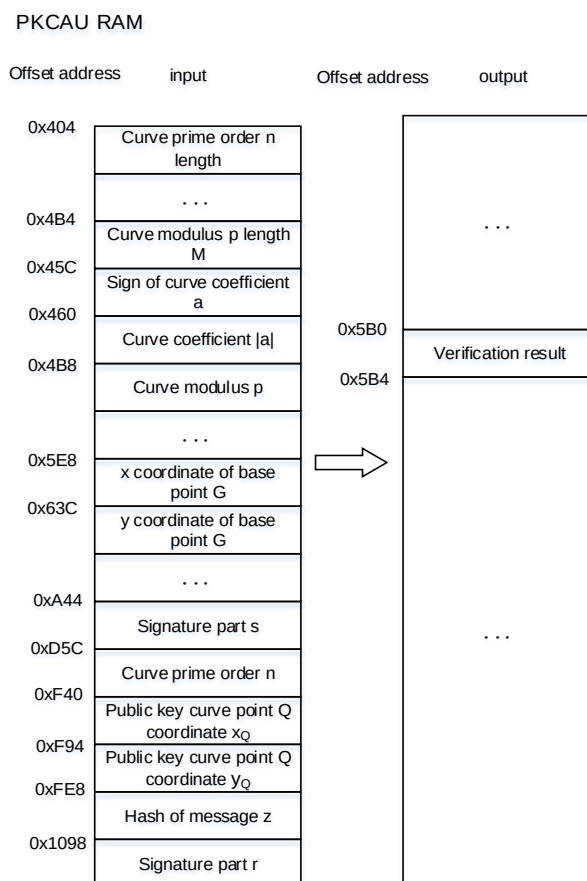
Figure 11-23. ECDSA verification
