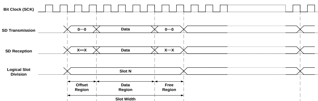
Figure 26-12 Data configuration
