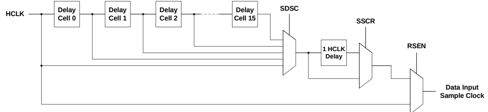
Figure 30-31. Data sampling clock delay chain
