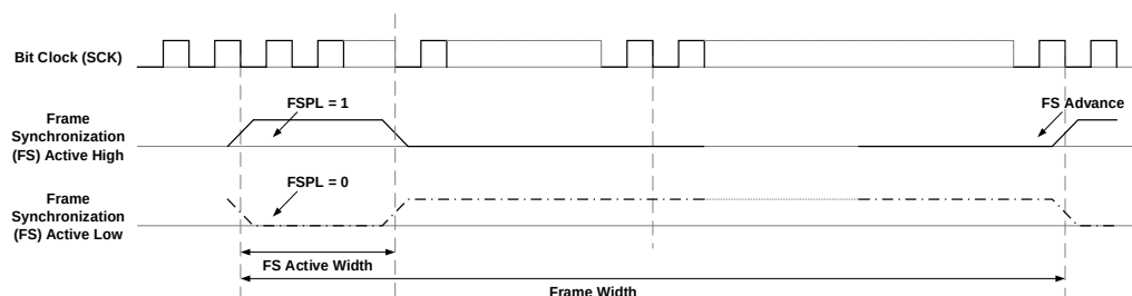
Figure 26-4 FS polarity
