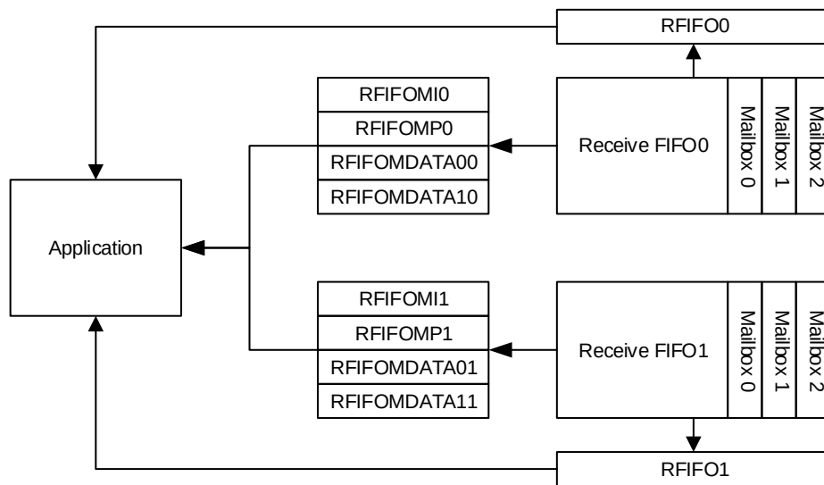
Figure 31-4. Reception register
