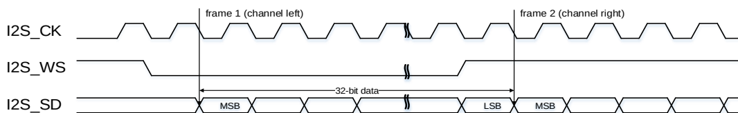
Figure 25-16. I2S Philips standard timing diagram (DTLEN=10, CHLEN=1, CKPL=0)
