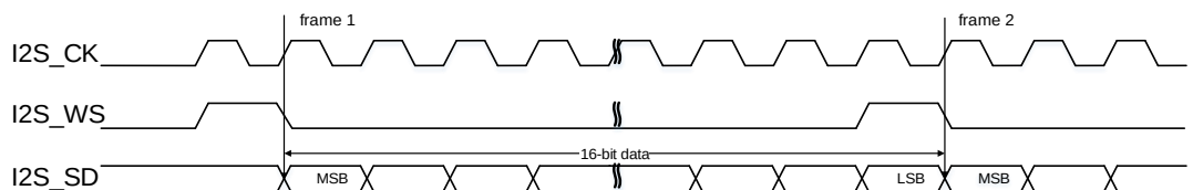
Figure 25-34. PCM standard short frame synchronization mode timing diagram (DTLEN=00, CHLEN=0, CKPL=0)
