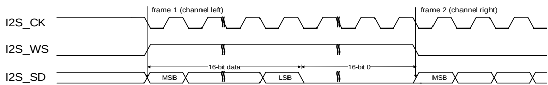
Figure 25-29. MSB justified standard timing diagram (DTLEN=00, CHLEN=1, CKPL=1)
