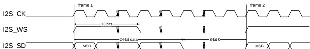
Figure 25-46. PCM standard long frame synchronization mode timing diagram (DTLEN=01, CHLEN=1, CKPL=0)
