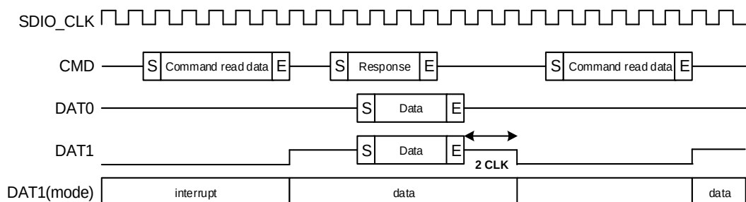
Figure 29-15. Read Interrupt cycle timing
