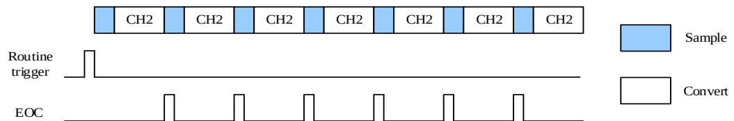
Figure 18-3. Continuous operation mode
