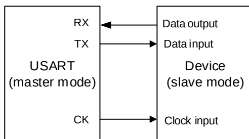
Figure 23-11. Example of USART in synchronous mode
