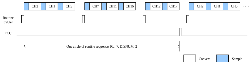
Figure 18-6. Discontinuous operation mode
