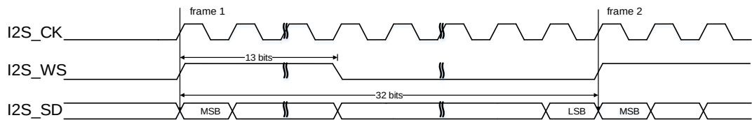
Figure 25-44. PCM standard long frame synchronization mode timing diagram (DTLEN=10, CHLEN=1, CKPL=0)
