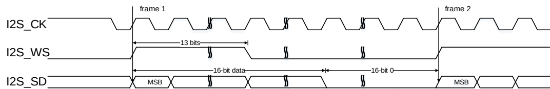
Figure 25-49. PCM standard long frame synchronization mode timing diagram (DTLEN=00, CHLEN=1, CKPL=1)
