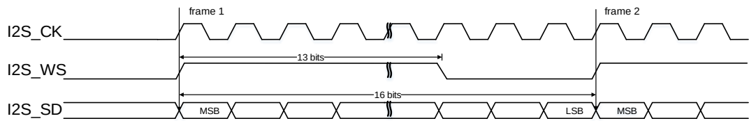
Figure25-43. PCM standard long frame synchronization mode timing diagram (DTLEN=00, CHLEN=0, CKPL=1)
