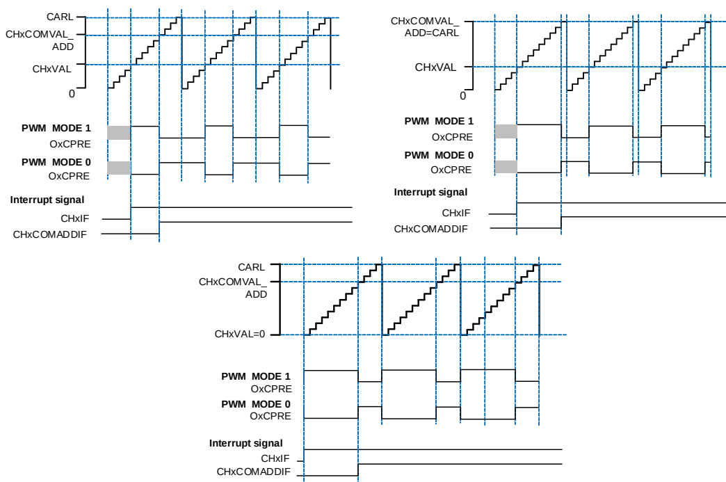
Figure 22-16. Channel x output PWM with (CHxVAL < CHxCOMVAL_ADD)
