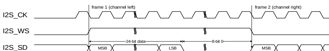
Figure 25-26. MSB justified standard timing diagram (DTLEN=01, CHLEN=1, CKPL=0)
