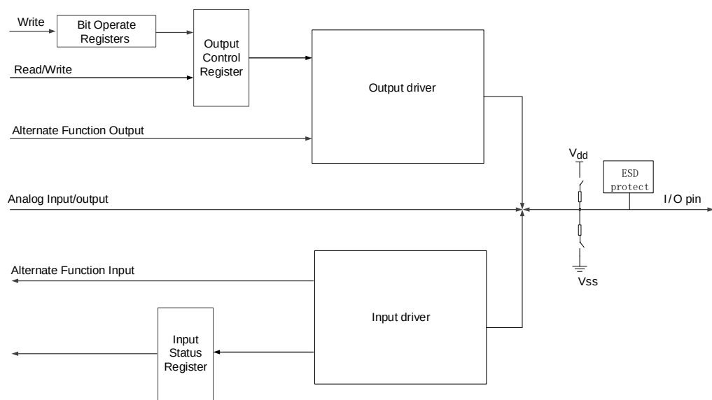
Figure 8-1. Basic structure of a standard I / O
