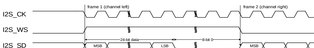
Figure 25-27. MSB justified standard timing diagram (DTLEN=01, CHLEN=1, CKPL=1)
