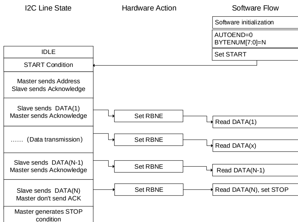
Figure 24-33. Programming model for master receiving ( N \leq 255 )
