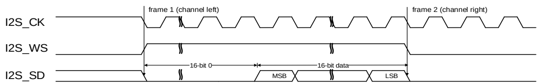
Figure 25-33. LSB justified standard timing diagram (DTLEN=00, CHLEN=1, CKPL=1)
