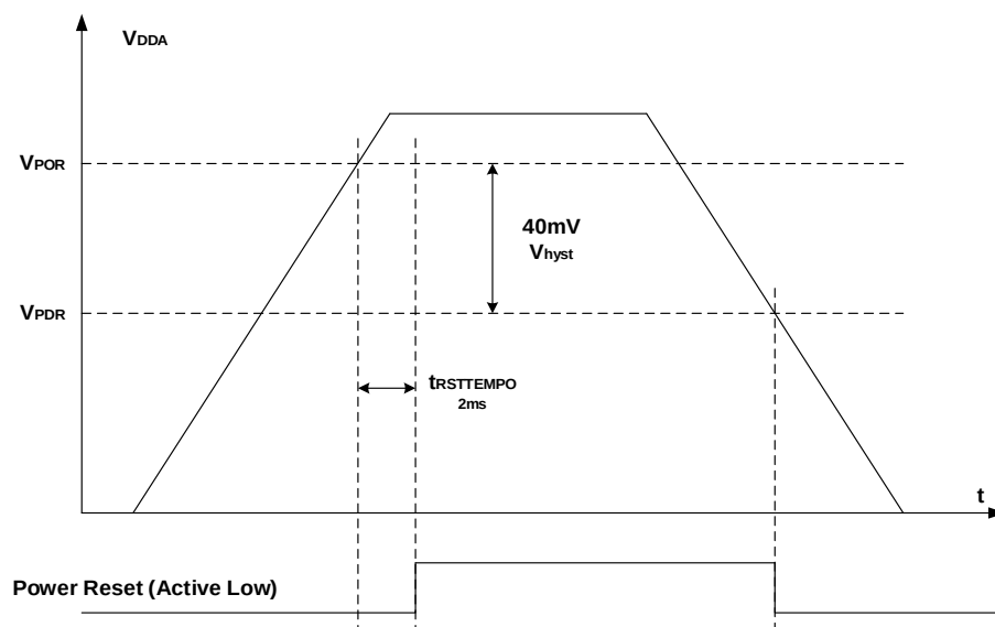
Figure 4-2. Waveform of the POR / PDR
