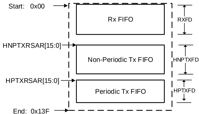
Figure 33-5. HOST mode FIFO space in SRAM
