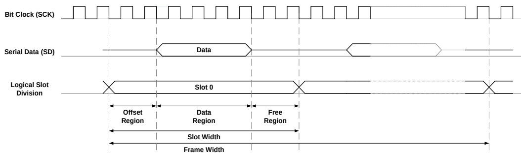
Figure 26-9 Slot partition convention
