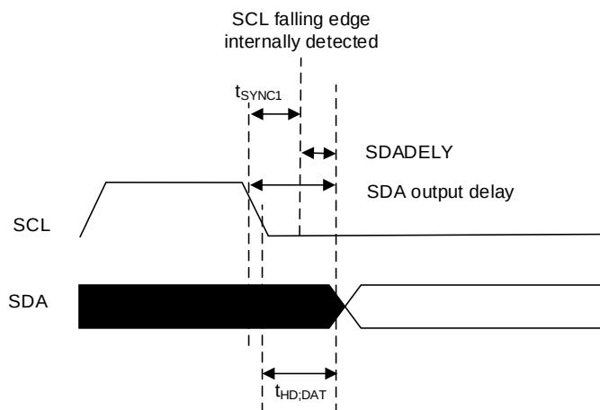
Figure 24-22. Data hold time
