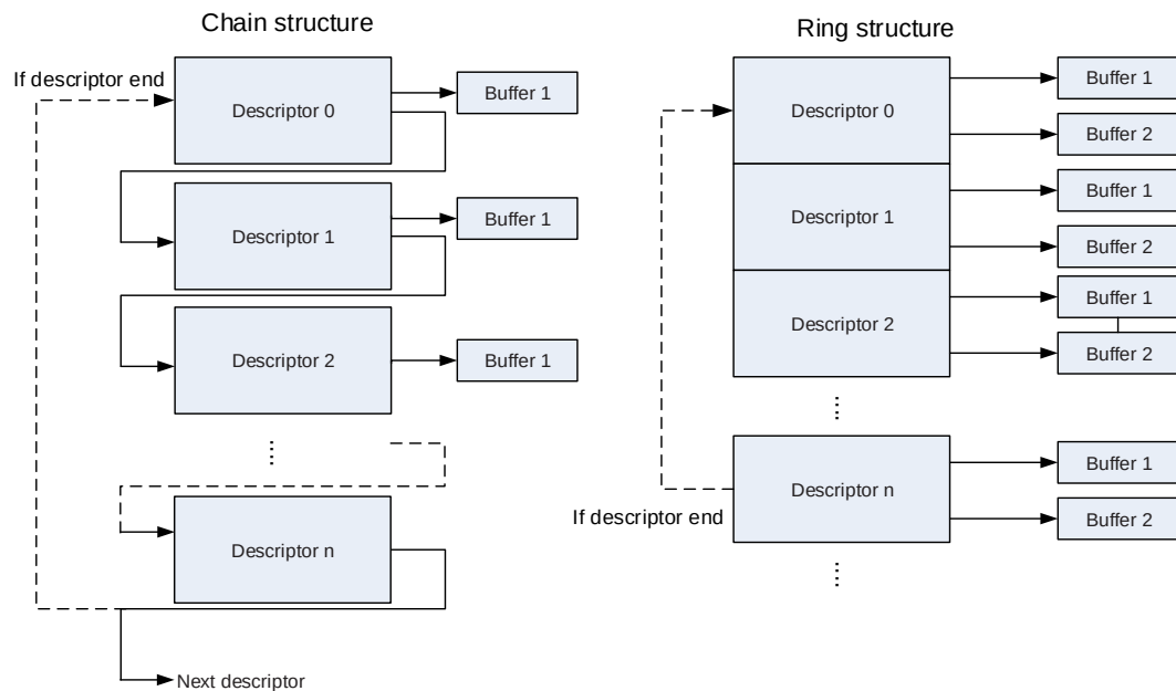
Figure 32-8. Descriptor ring and chain structure
