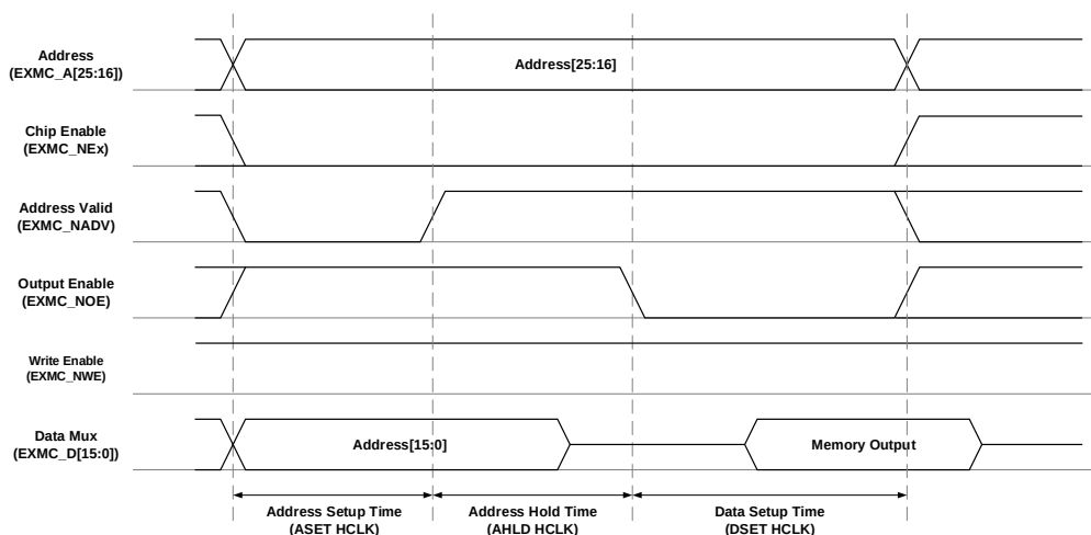
Figure 30-18. Multiplex mode read access
