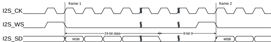
Figure 25-38. PCM standard short frame synchronization mode timing diagram (DTLEN=01, CHLEN=1, CKPL=0)
