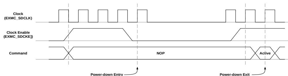
Figure 30-38. Process for power-down entry and exit
