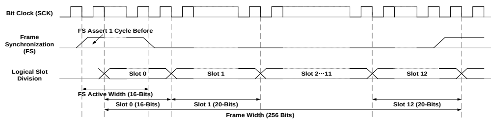
Figure 26-13 AC'97 slot partition
