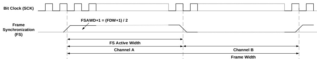
Figure 26-5 FS function
