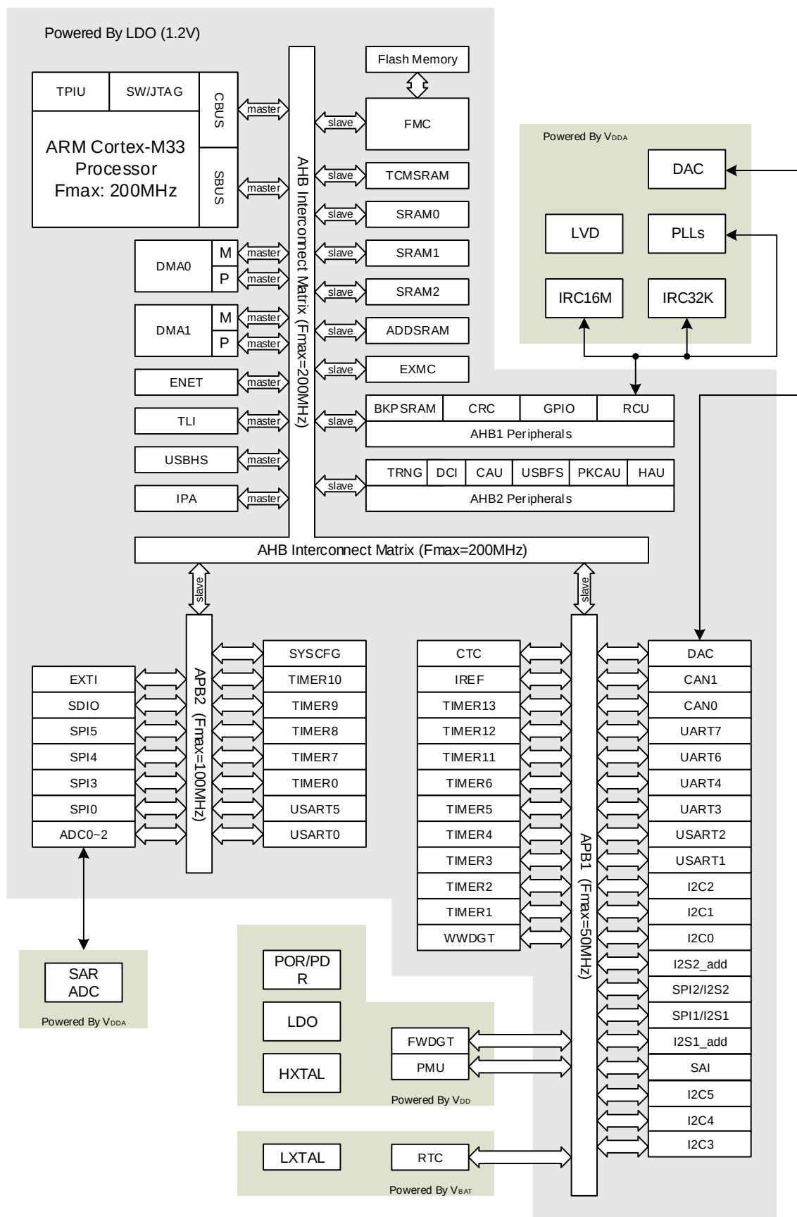
Figure 1-2. The system architecture of GD32F527xx devices
