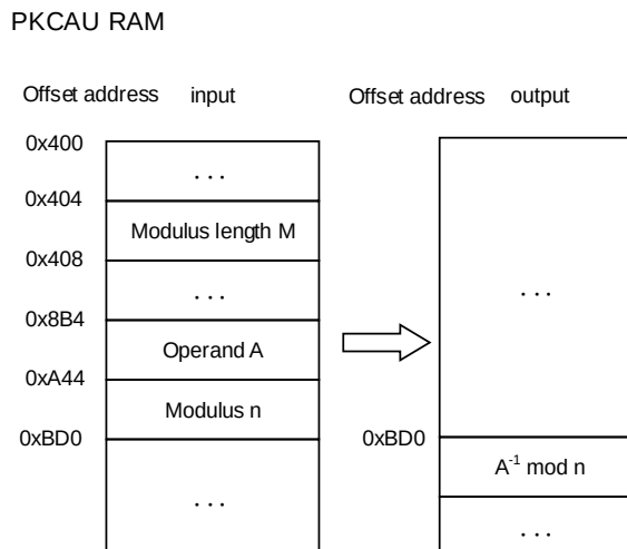
Figure 11-17. Modular inversion
