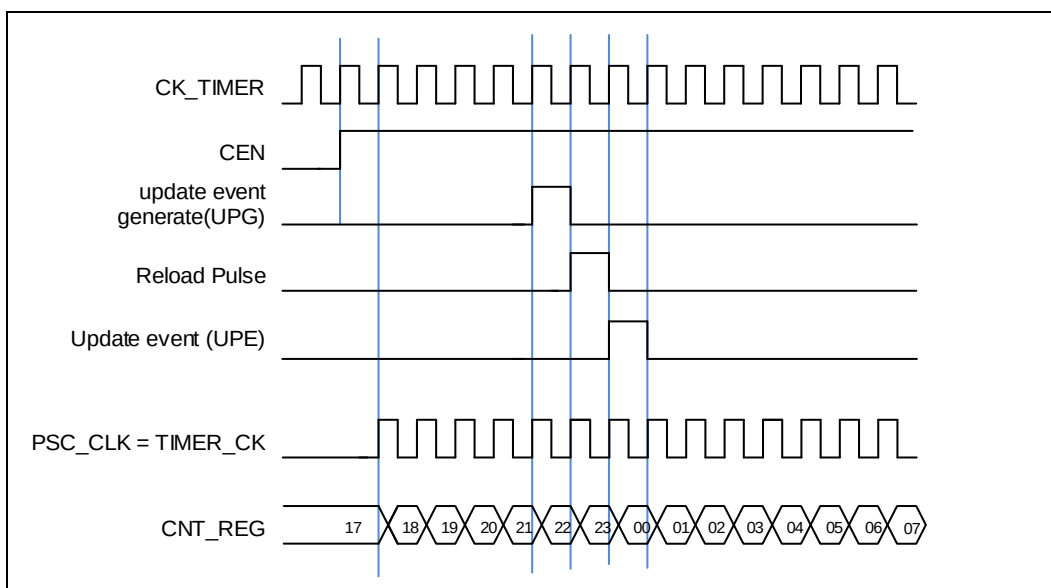
Figure 22-63. Timing chart of internal clock divided by 1
