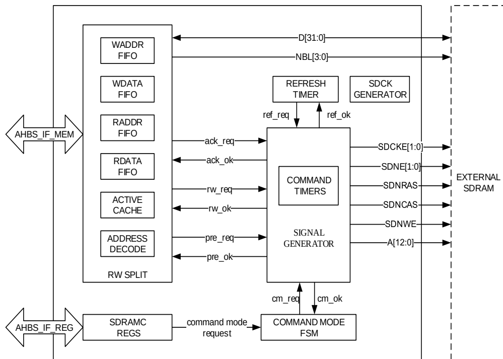
Figure 30-29. SDRAM controller block diagram
