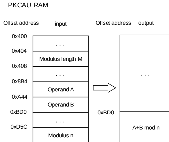
Figure 11-10. Modular addition
