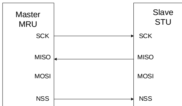
Figure 25-5. A typical simplex connection (Master: Receive, Slave: Transmit)
