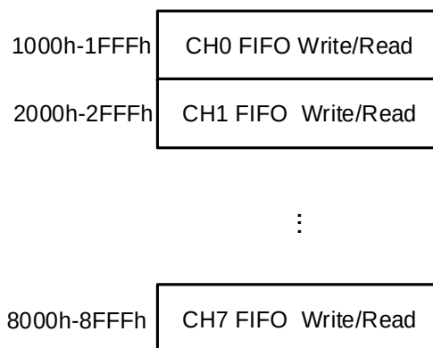
Figure 33-6. Host mode FIFO access register map
