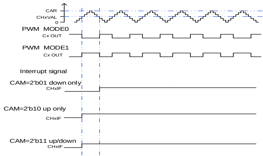
Figure 22-15. CAPWM timechart
