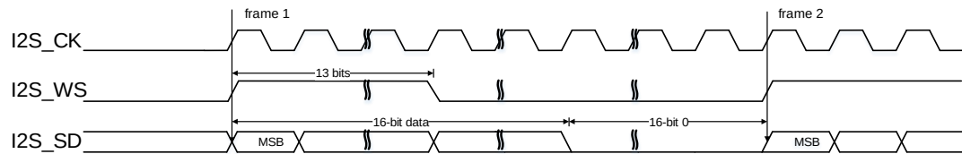
Figure 25-48. PCM standard long frame synchronization mode timing diagram (DTLEN=00, CHLEN=1, CKPL=0)
