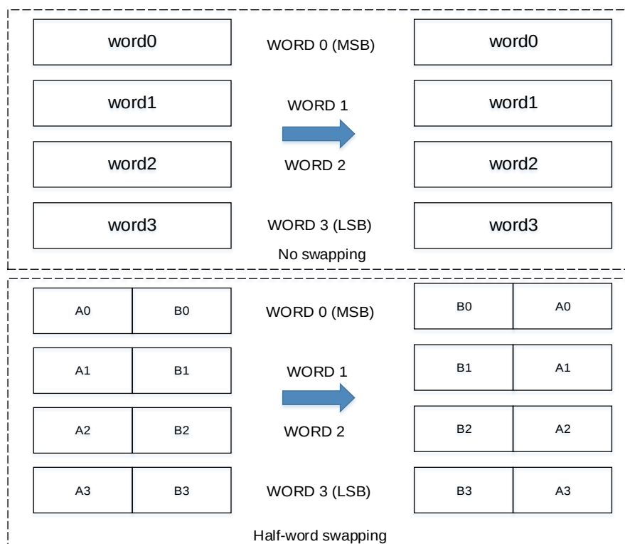
Figure 12-1. DATAM No swapping and Half-word swapping
