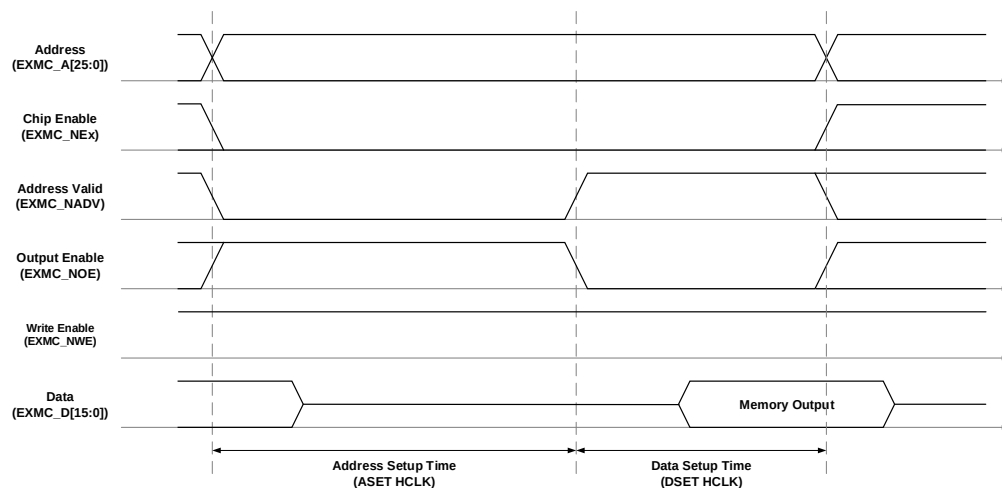
Figure 30-14. Mode C read access
