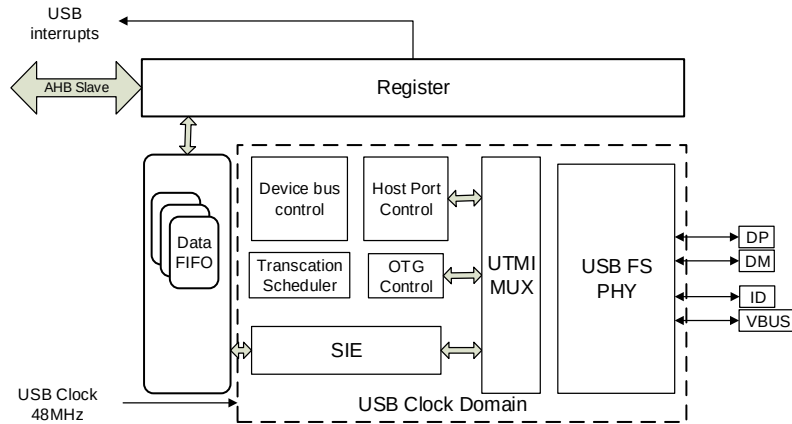
Figure 33-1. USBFS block diagram
