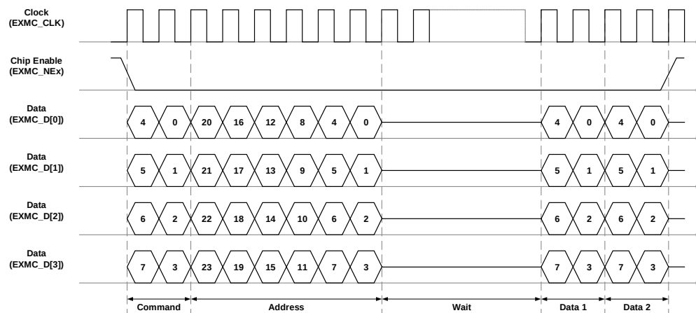
Figure 30-26. QPI-PSRAM access
