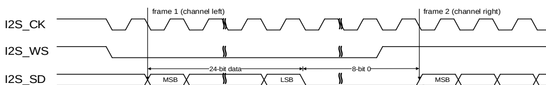
Figure 25-19. I2S Philips standard timing diagram (DTLEN=01, CHLEN=1, CKPL=1)
