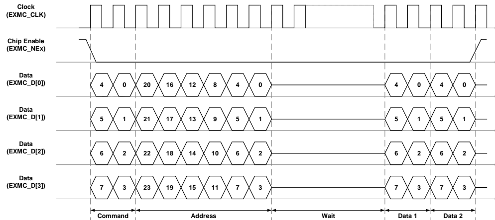
Figure 25-26. QPI-PSRAM access
