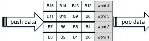
Figure 10-4. Data packing/unpacking when PWIDTH = ‘00’
