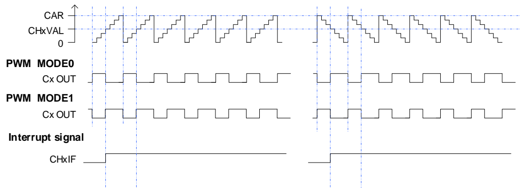
Figure 18-15. CAPWM timechart
