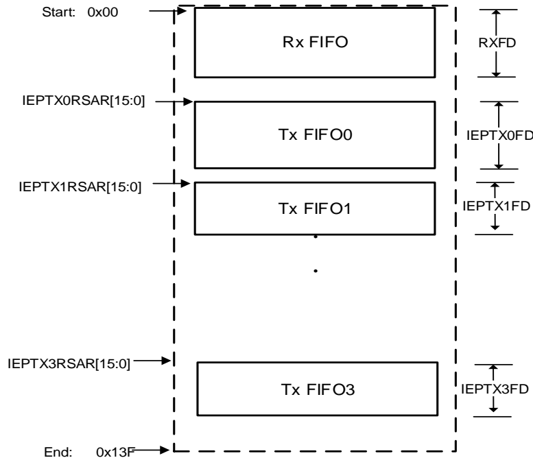
Figure 28-7. Device mode FIFO space in SRAM
