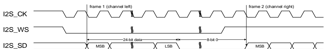
Figure 21-19. I2S Phillips standard timing diagram (DTLEN=01, CHLEN=1, CKPL=1)
