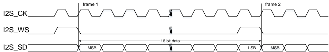
Figure 21-34. PCM standard short frame synchronization mode timing diagram (DTLEN=00, CHLEN=0, CKPL=0)
