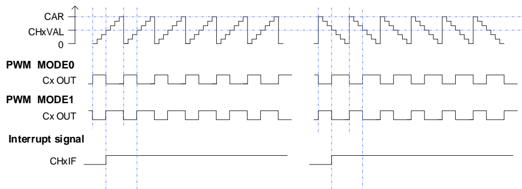
Figure 18-51. CAPWM timechart
