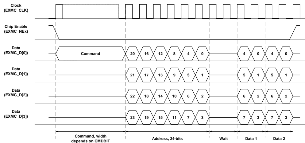
Figure 25-25. SQPI-PSRAM access
