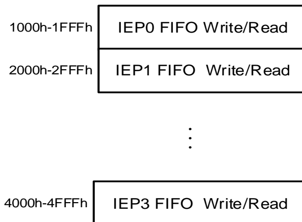
Figure 28-8. Device mode FIFO access register map
