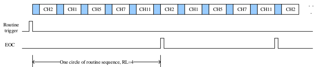
Figure 14-5. Scan operation mode, continuous enable
