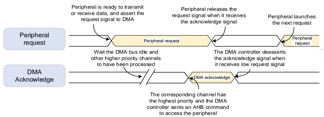
Figure 10-3. Handshake mechanism
