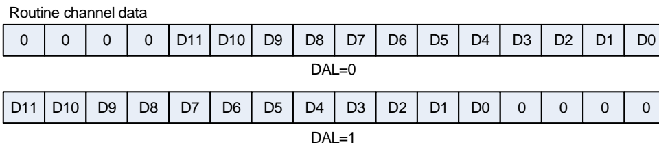
Figure 14-7. Data storage mode of 12-bit resolution
