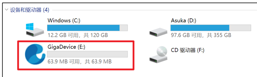
Figure 2-4. GDLINK folder
