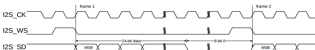
Figure 27-45. PCM standard short frame synchronization mode timing diagram (DTLEN = 01, CHLEN = 1, CKPL = 1)
