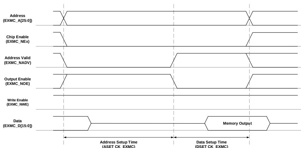
Figure 38-14. Mode C read access
