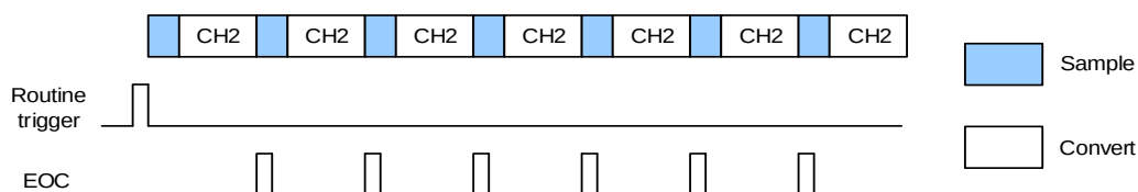
Figure 20-3. Continuous operation mode
