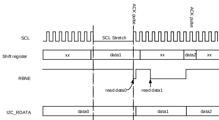
Figure 26-12. Data reception
