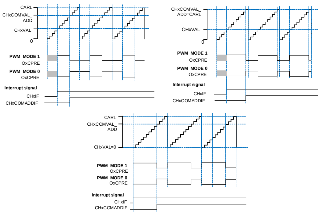
Figure 24-19. Channel x output PWM with ( CHxVAL < CHxCOMVAL\_ADD )
