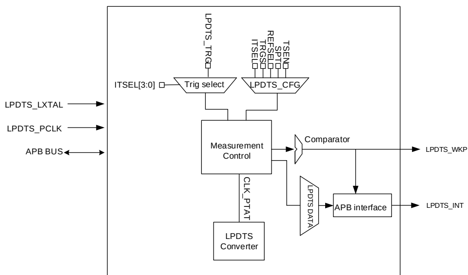
Figure 40-1. LPDTS block diagram
