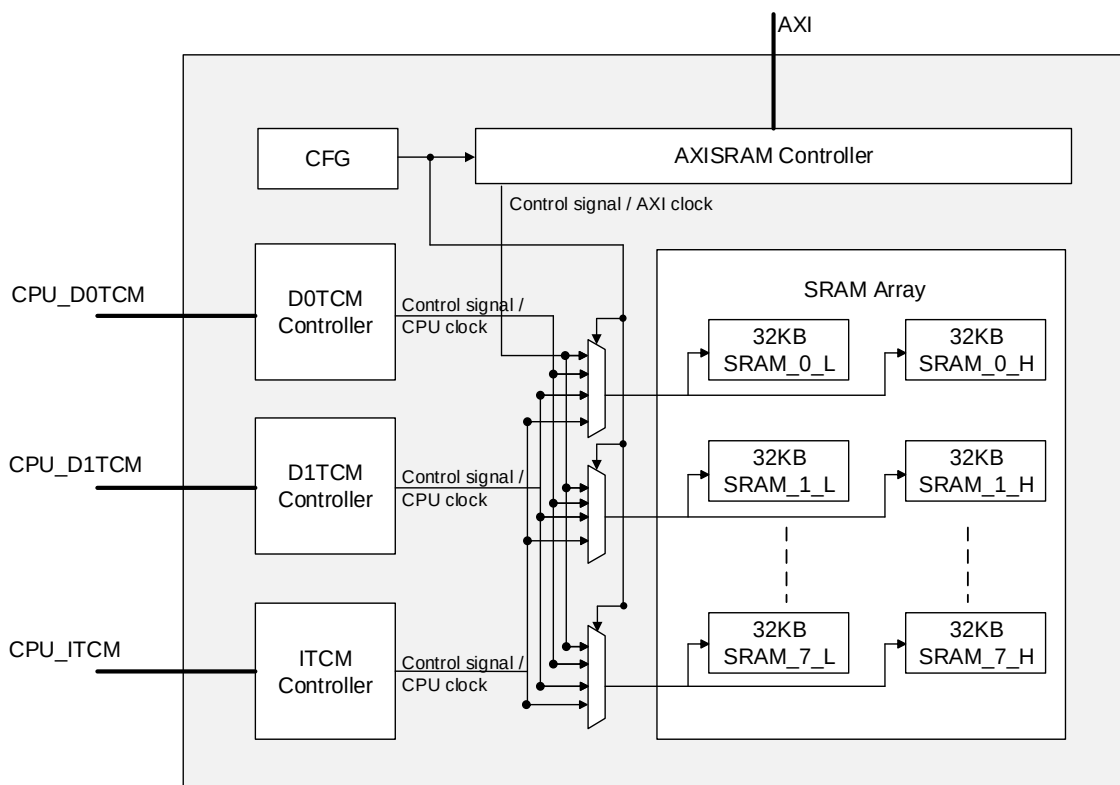
Figure 1-7. Block diagram of RAM shared by ITCM/DTCM/AXI SRAM
