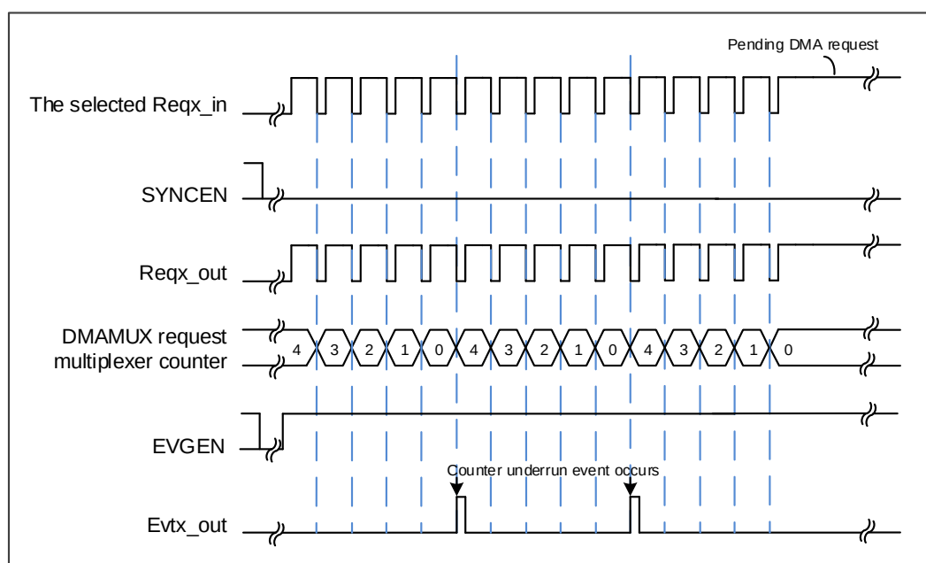
Figure 18-3. Event generation
