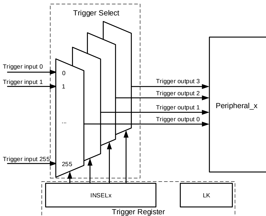
Figure 9-1. TRIGSEL main composition example
