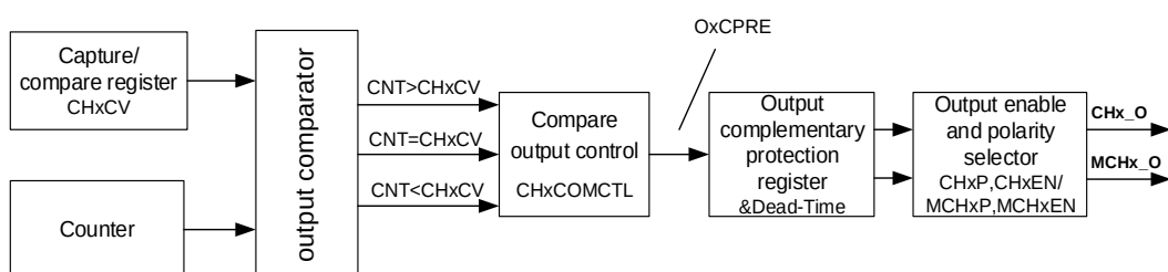
Figure 24-90. Output compare logic (when MCHxMSEL = 2'11, x=0)
