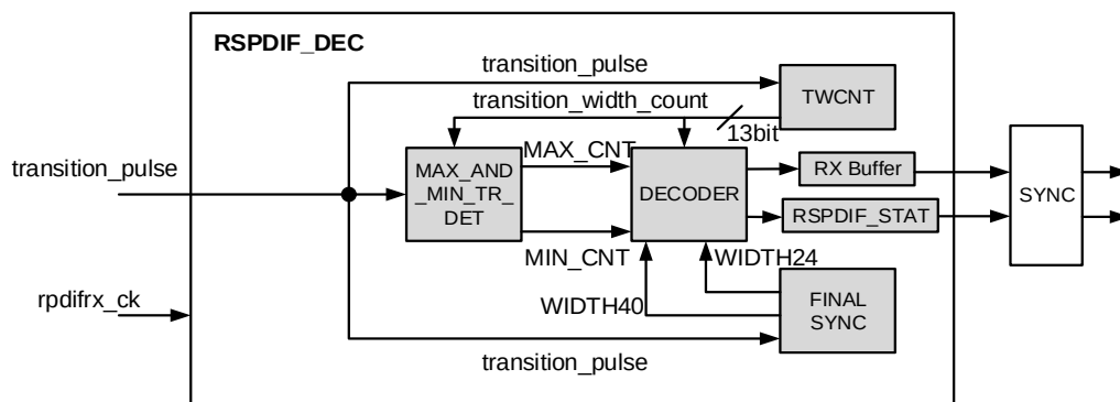
Figure 33-6. RSPDIF_DEC block
