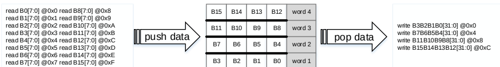
Figure 17-6. Data packing / unpacking
