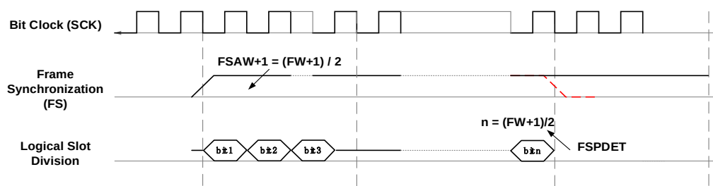
Figure 34-25 Frame synchronization postponed detection
