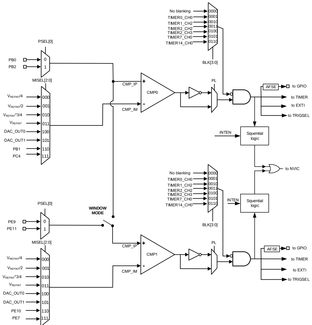
Figure 44-1. CMP block diagram
