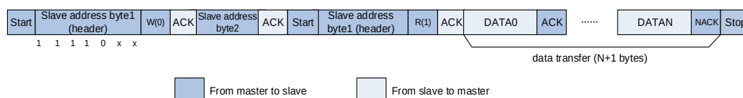
Figure 26-7. I2C communication flow with 10-bit address (Master Receive when HEAD10R=0)
