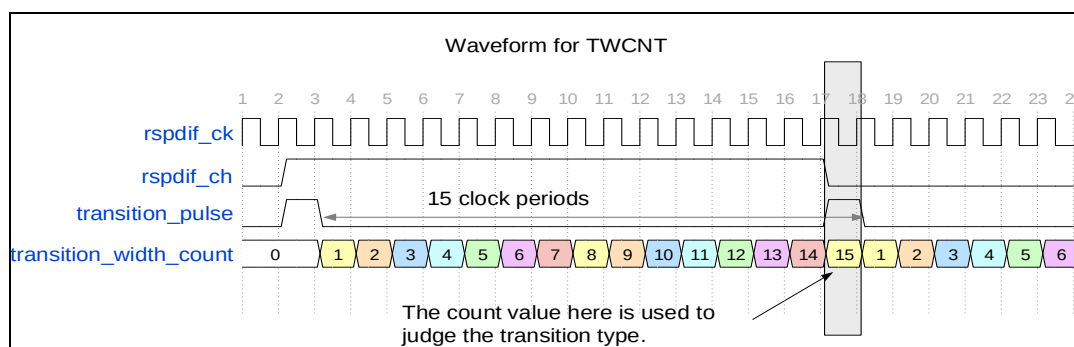
Figure 33-7. Waveforms of TWCNT
