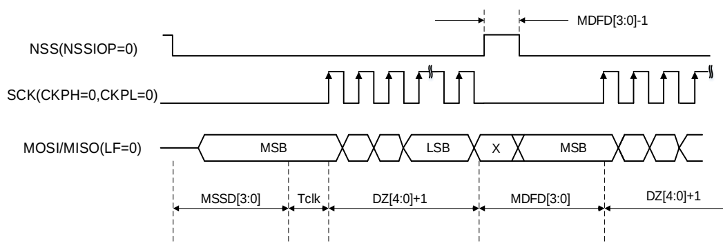
Figure 27-9. NSS interlaced pulses timing diagram ( MSSD[3:0] = 0011 (3 \times T_{clk}) , MDFD = 0011 (3 \times T_{clk}) )
