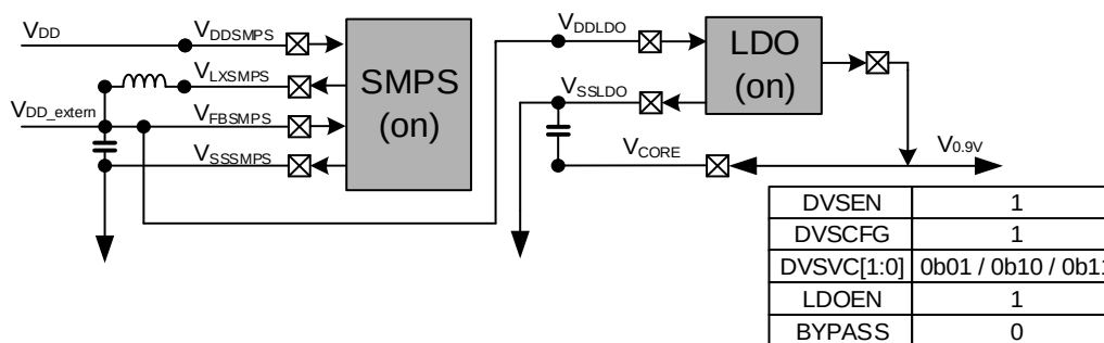
Figure 5-11. SMPS supplies for LDO and external, LDO supplies for 0.9V power domain
