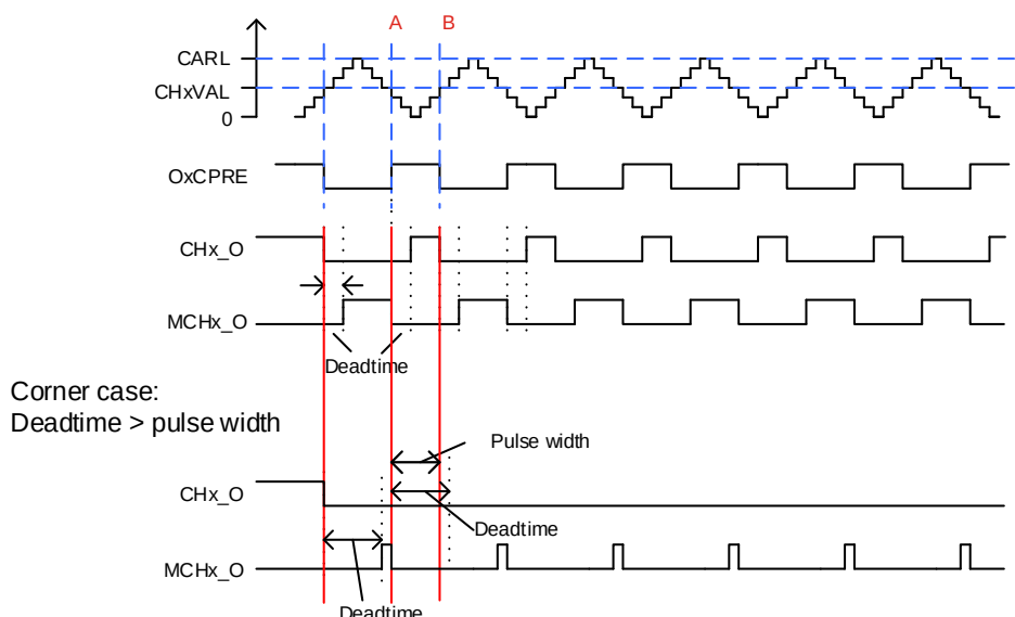
Figure 24-27. Complementary output with dead time insertion
