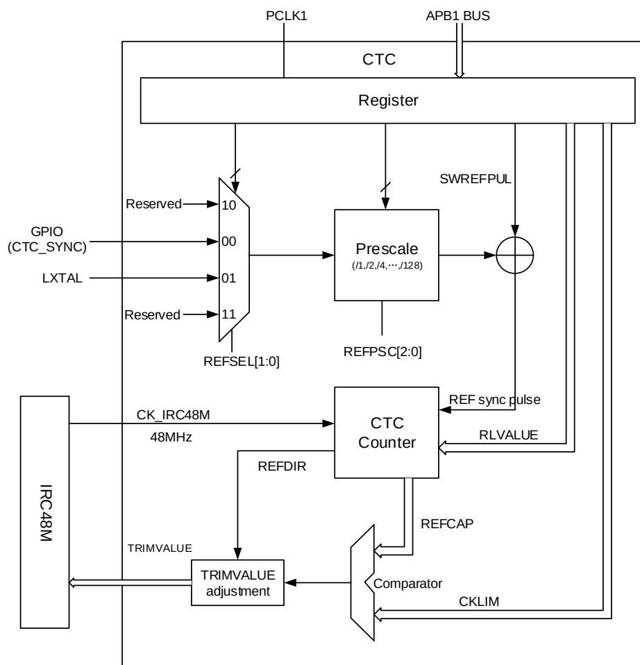
Figure 7-1. CTC overview
