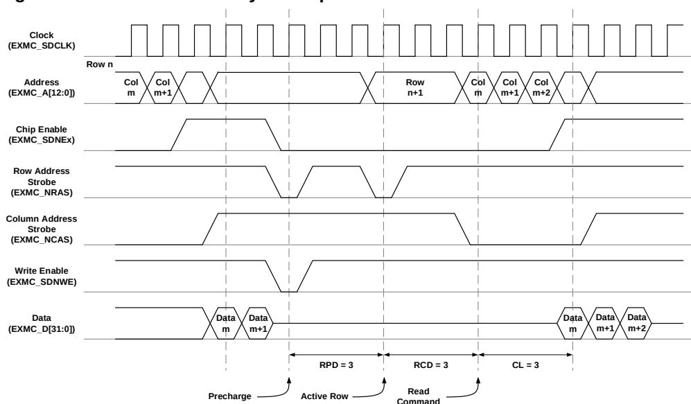
Figure 38-32. Cross boundary read operation
