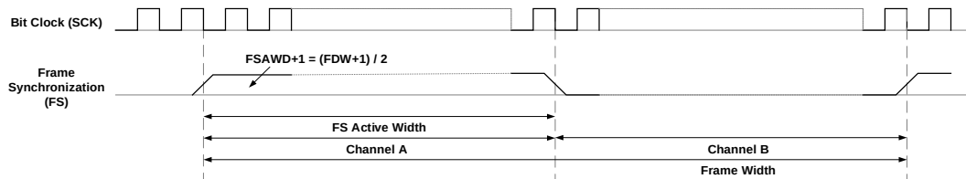
Figure 34-5 FS function
