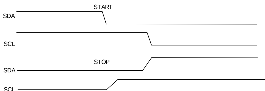
Figure 26-3. START and STOP condition
