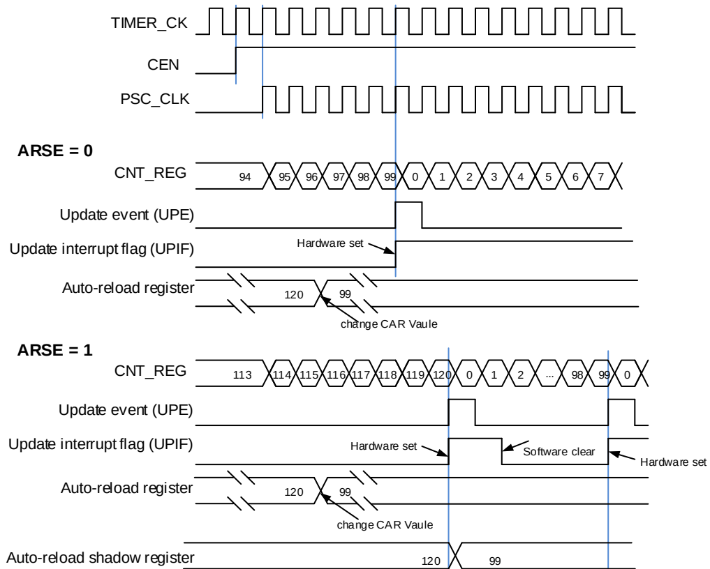
Figure 24-54. Timing chart of up counting, change TIMEx_CAR ongoing
