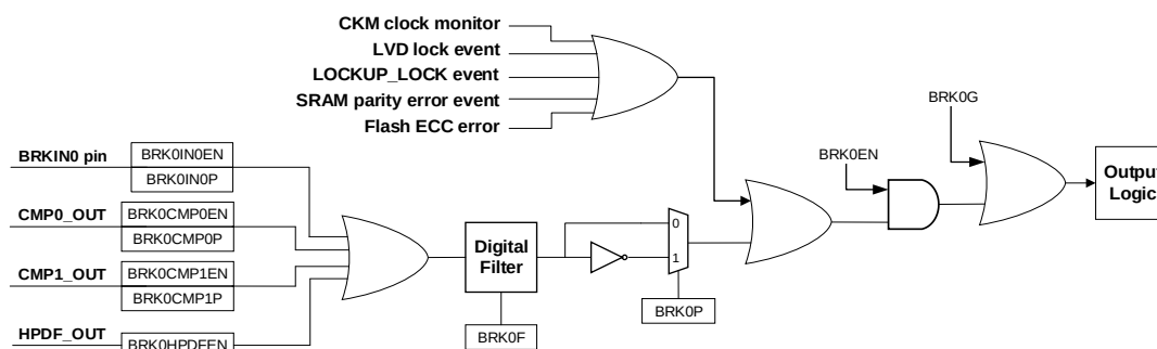
Figure 24-101. BREAK0 function logic diagram
