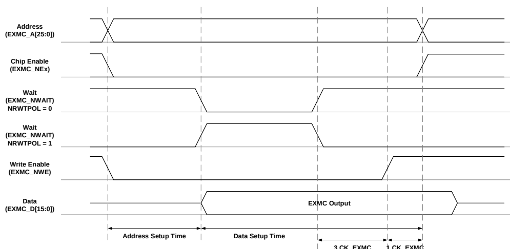
Figure 38-21. Write access timing diagram under async-wait signal assertion
