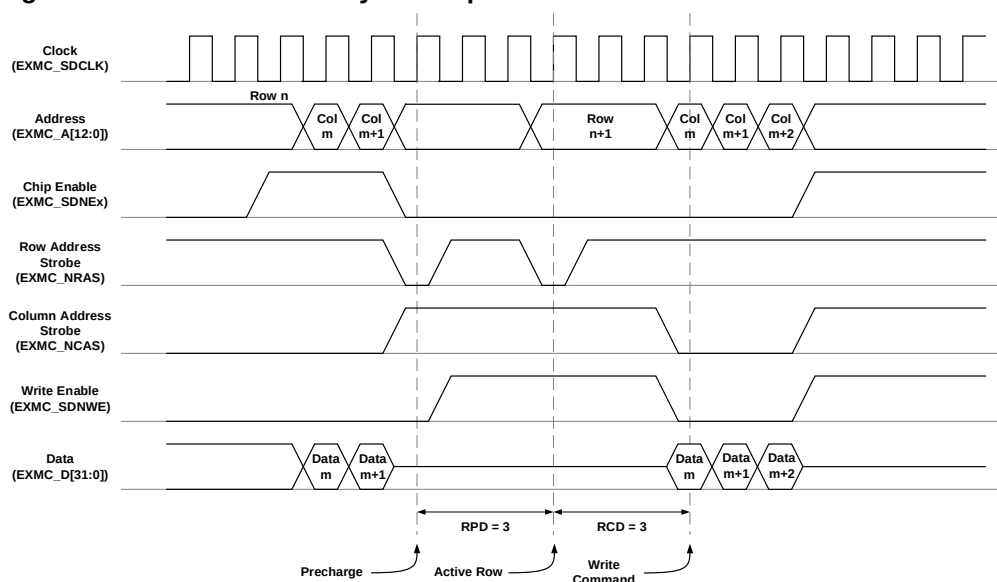
Figure 38-33. Cross boundary write operation
