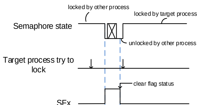
Figure 48-4. Second try lock success
