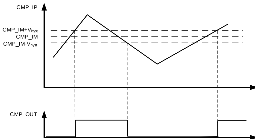
Figure 44-3. CMP hysteresis
