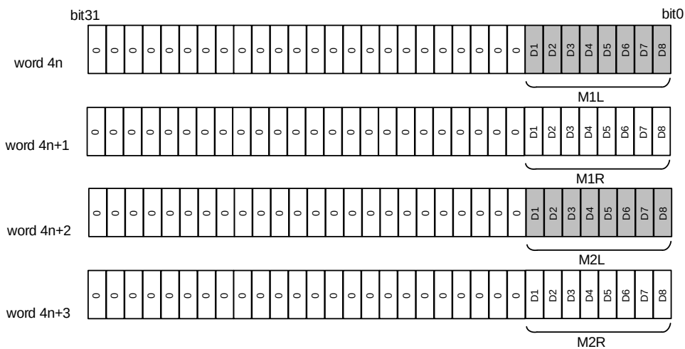
Figure 34-18. Dual microphones, under different slot widths, BxDATA register data format
