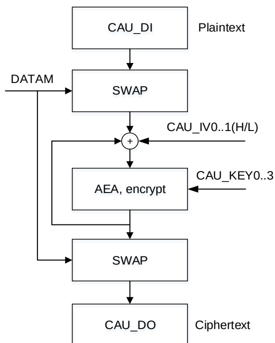
Figure 13-10. AES CBC encryption
