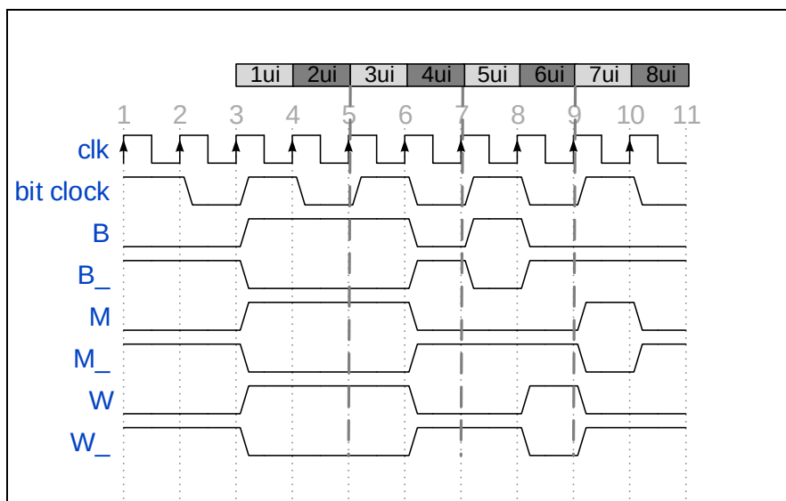
Figure 33-4. S/PDIF Preambles
