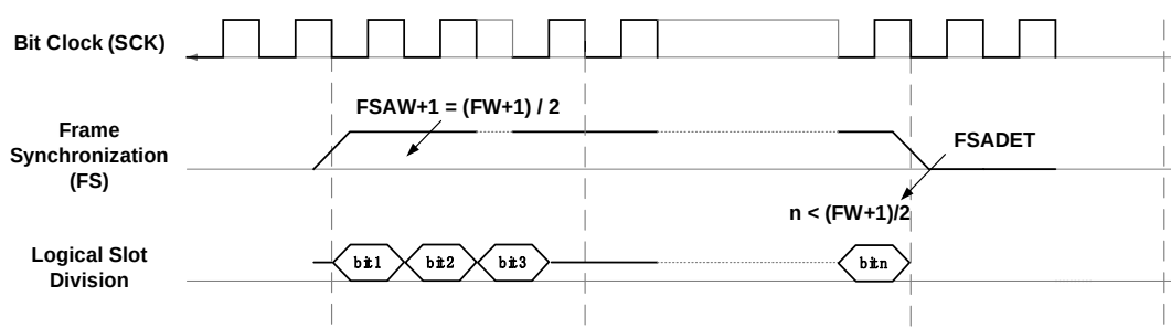
Figure 34-24 Frame synchronization advanced detection
