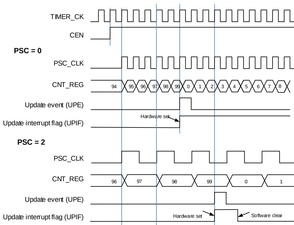
Figure 24-112. Timing diagram of up counting mode, \text{PSC}=0/2
