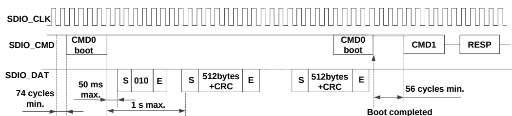
Figure 36-17. Alternative Boot operation timing
