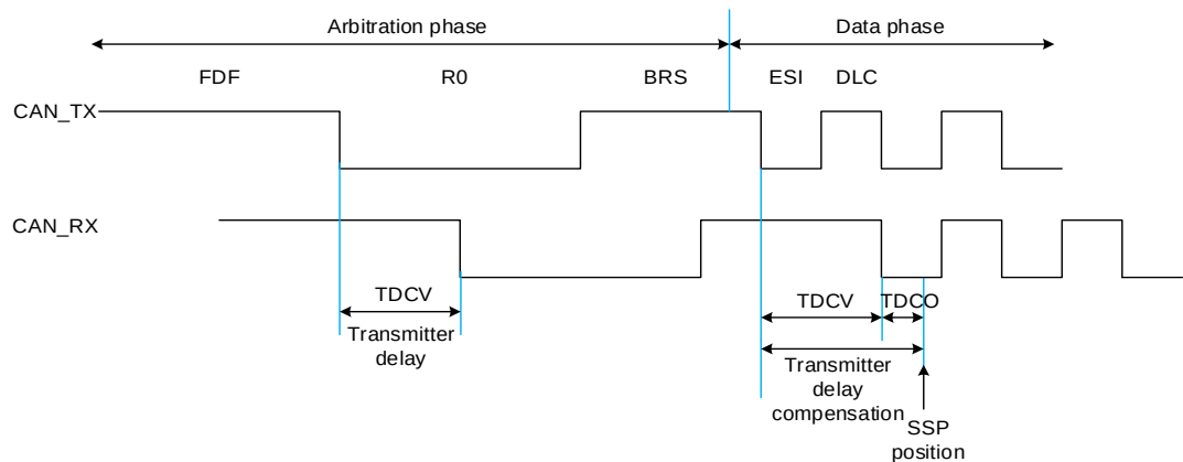
Figure 42-2. Transmitter delay
