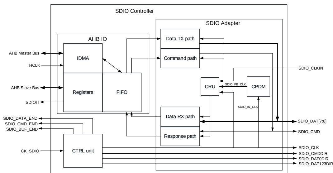
Figure 36-6. SDIO block diagram
