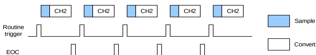
Figure 20-2. Single operation mode
