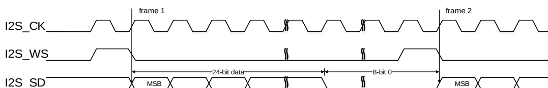
Figure 27-44. PCM standard short frame synchronization mode timing diagram (DTLEN = 01, CHLEN = 1, CKPL = 0)
