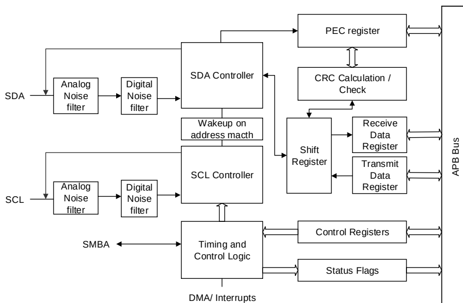
Figure 26-1. I2C module block diagram
