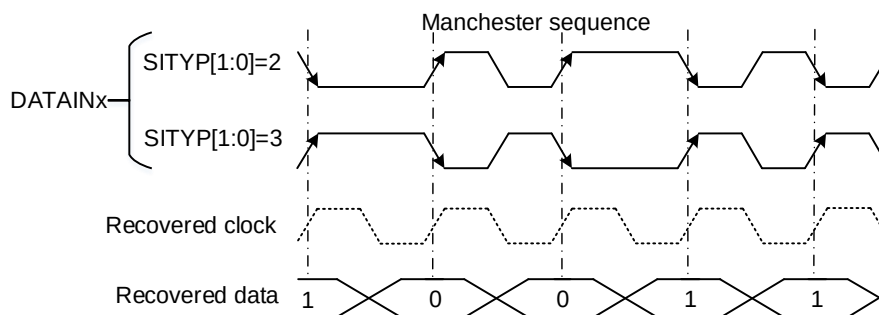
Figure 45-3. The sequence diagram of Manchester data transmission
