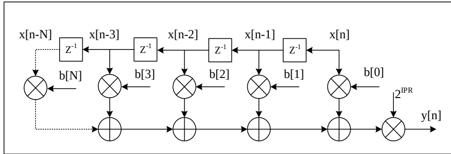
Figure 47-7 The structure of FIR filter function
