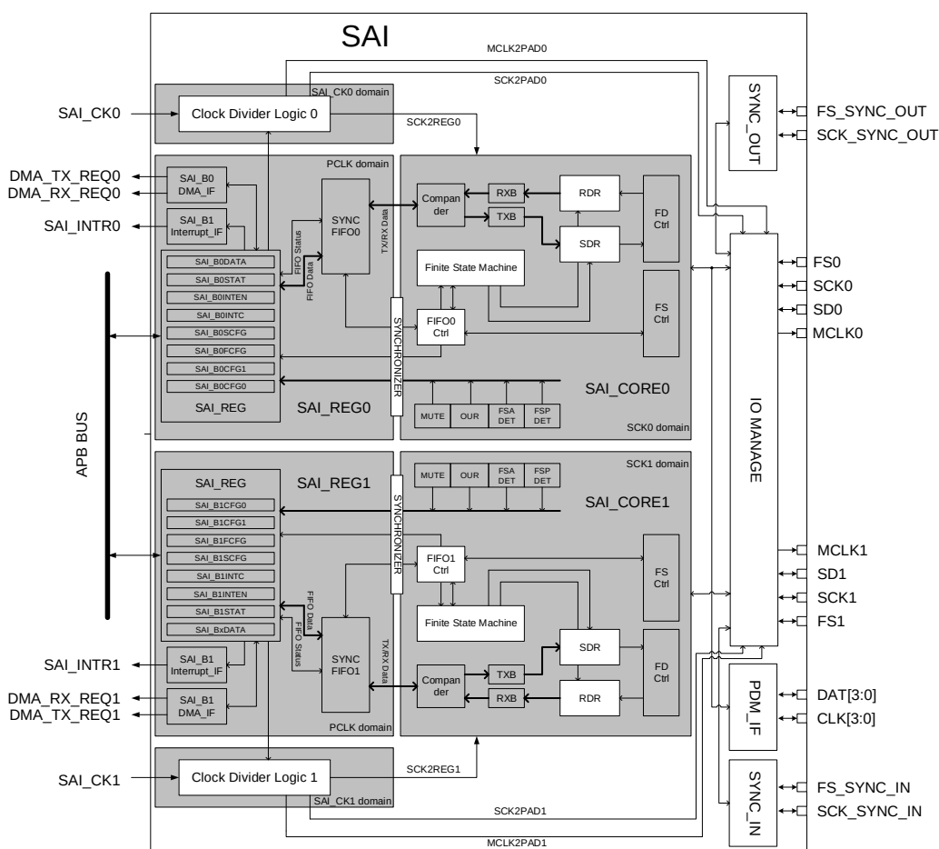
Figure 34-1. block diagram
