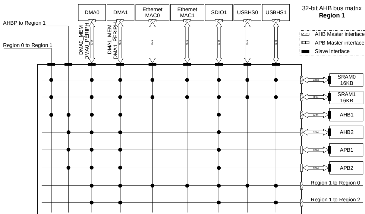
Figure 1-4. Bus matrix Region 1
