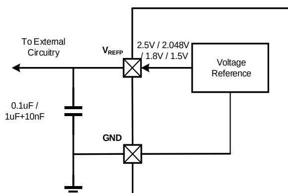
Figure 39-1. Precision reference connection
