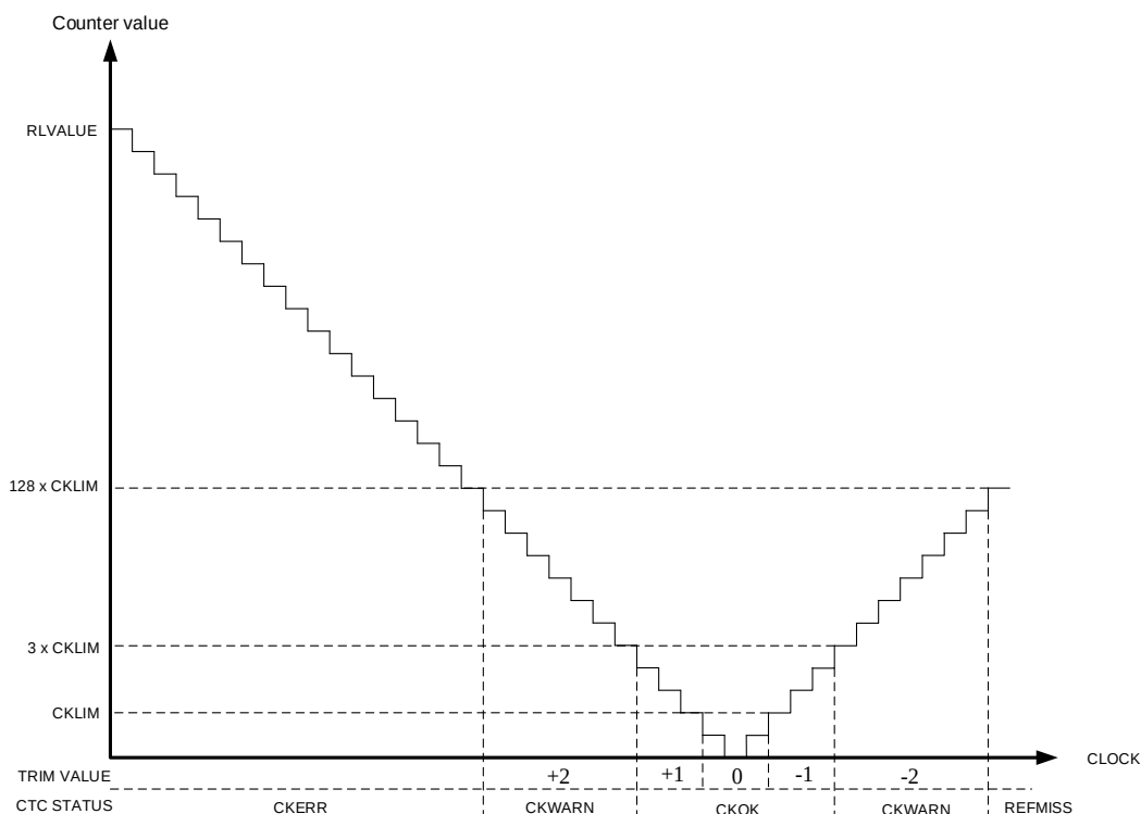
Figure 7-2. CTC trim counter
