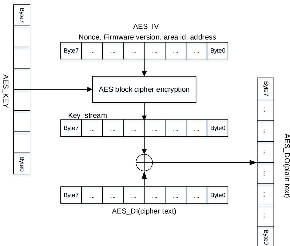
Figure 46-3. Decryption flow with AES-128 in CTR mode
