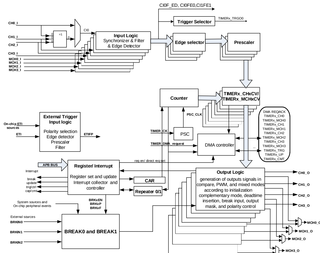
Figure 24-1. Advanced timer block diagram
