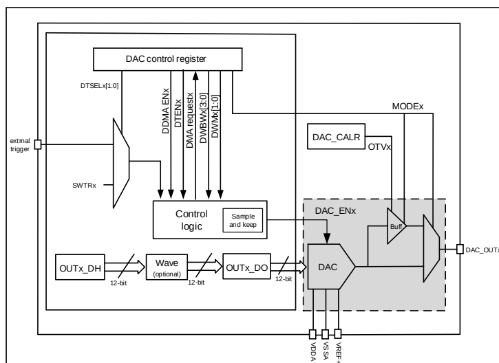
Figure 21-1. DAC block diagram
