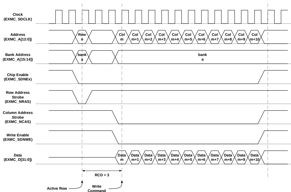
Figure 38-29. Burst write operation
