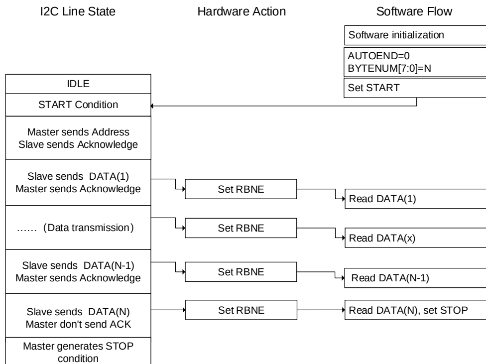
Figure 26-20. Programming model for master receiving ( N \leq 255 )
