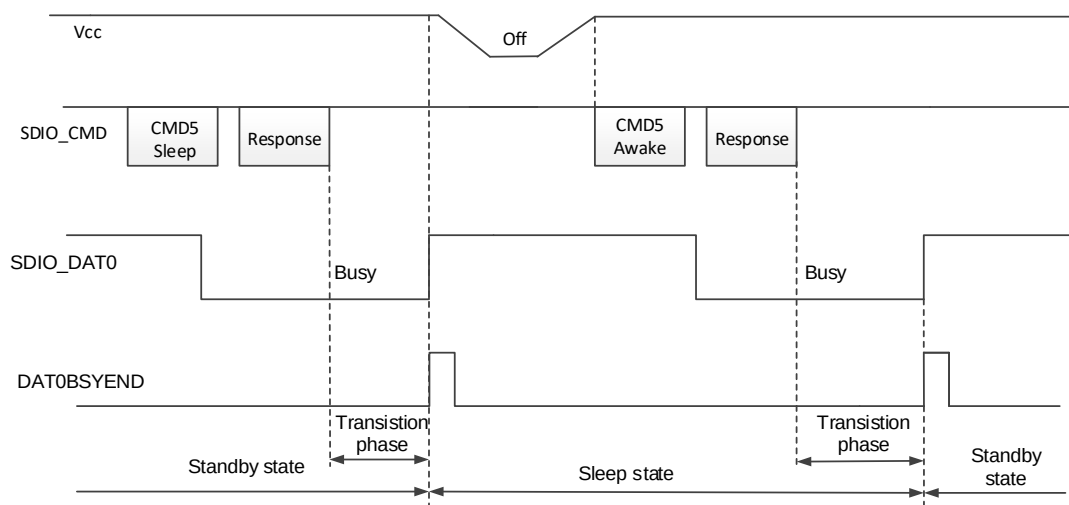
Figure 36-18. CMD5 timing
