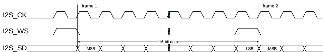
Figure 27-41. PCM standard short frame synchronization mode timing diagram (DTLEN = 00, CHLEN = 0, CKPL = 1)
