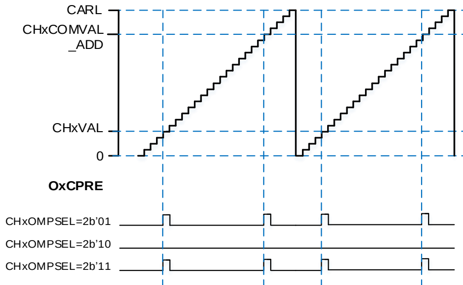
Figure 24-69. CHx_O output with a pulse in edge-aligned mode (CHxOMPSEL ≠ 2'b00)
