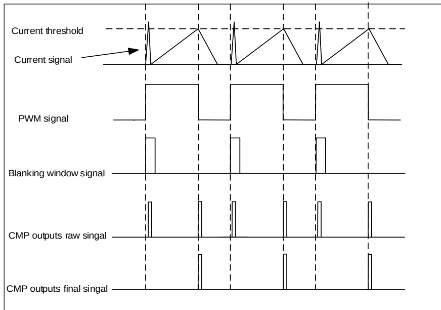
Figure 44-2. The CMP outputs signal blanking
