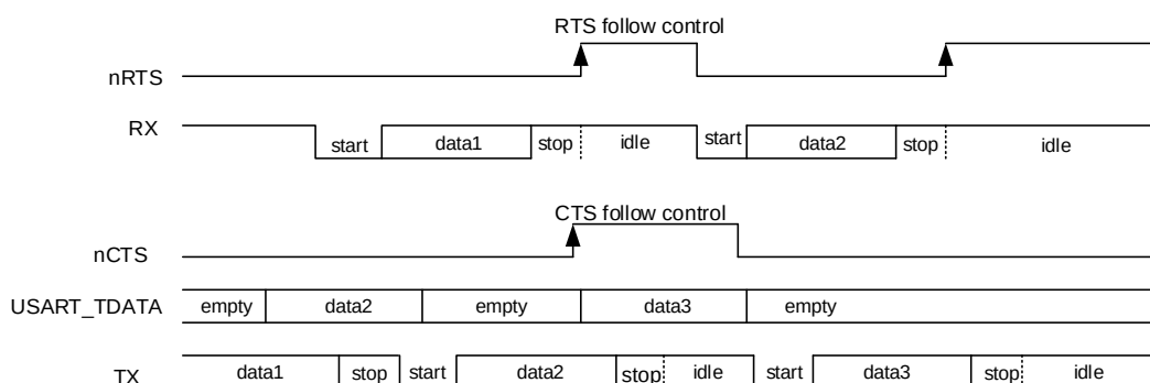
Figure 25-8. Hardware flow control
