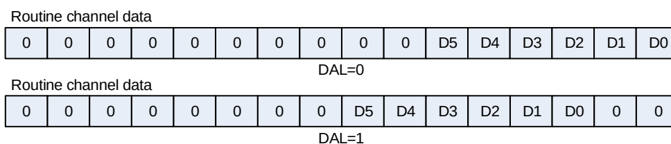
Figure 20-9. 6-bit data storage mode
