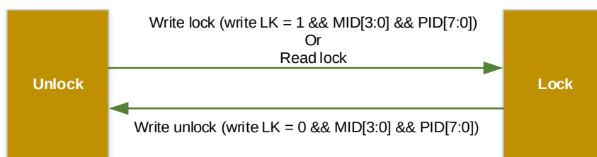
Figure 48-2. HWSEM state machine
