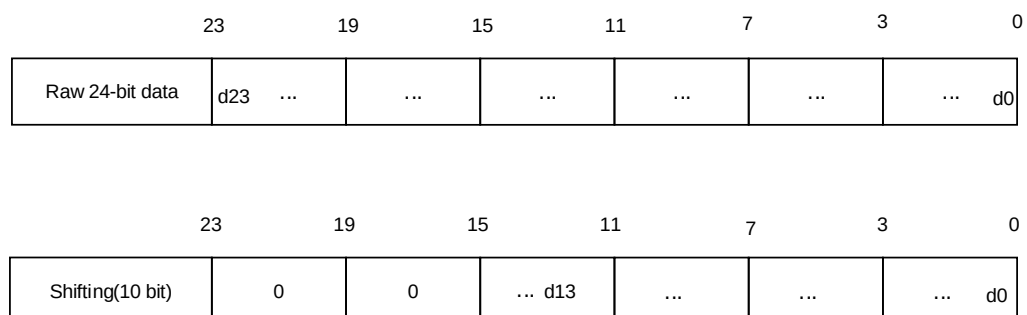
Figure 20-13. 14bit ADC oversampling with 10bits right shift
