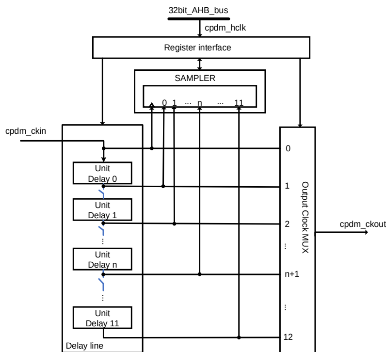
Figure 30-1. Schematic diagram of CPDM
