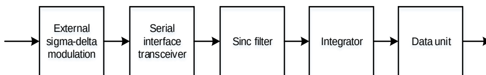
Figure 45-7. HPDF module external input data processing flow
