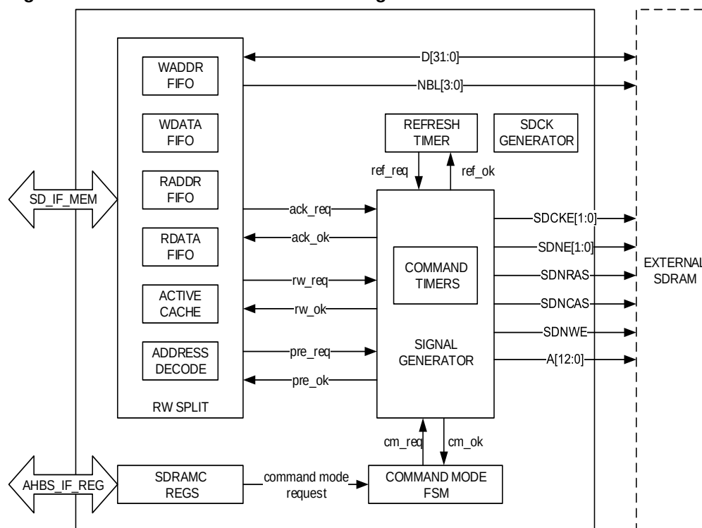
Figure 38-26. SDRAM controller block diagram
