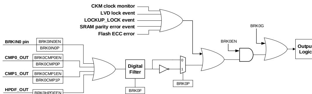
Figure 24-122. BREAK0 function logic diagram
