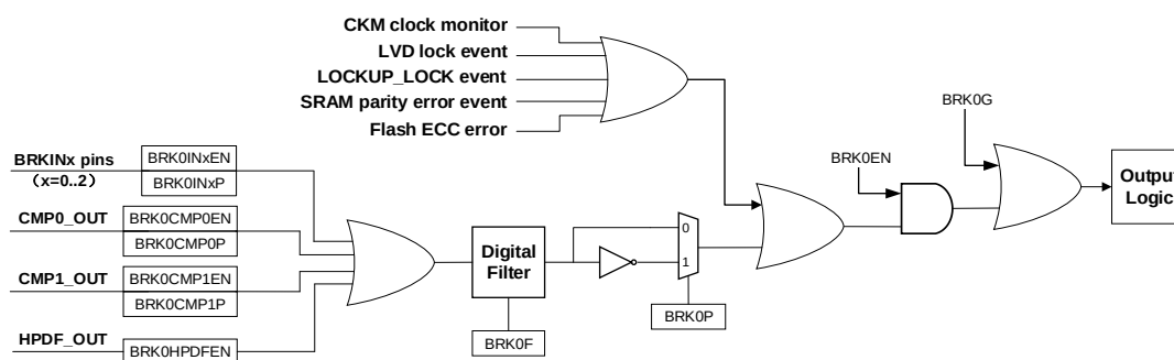
Figure 24-28. BREAK0 function logic diagram
