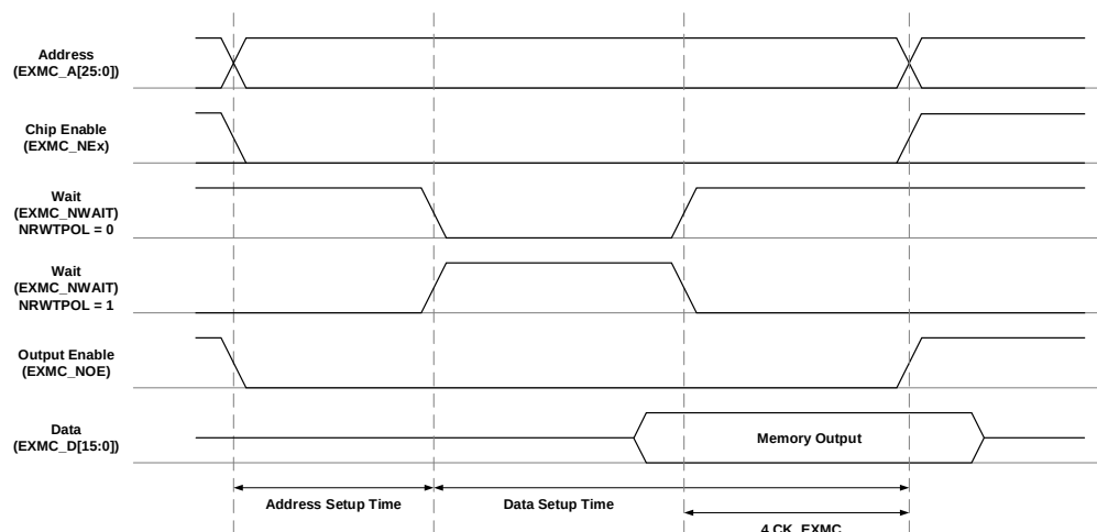
Figure 38-20. Read access timing diagram under async-wait signal assertion
