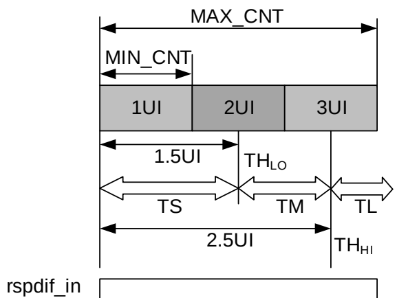
Figure 33-8. Threshold
