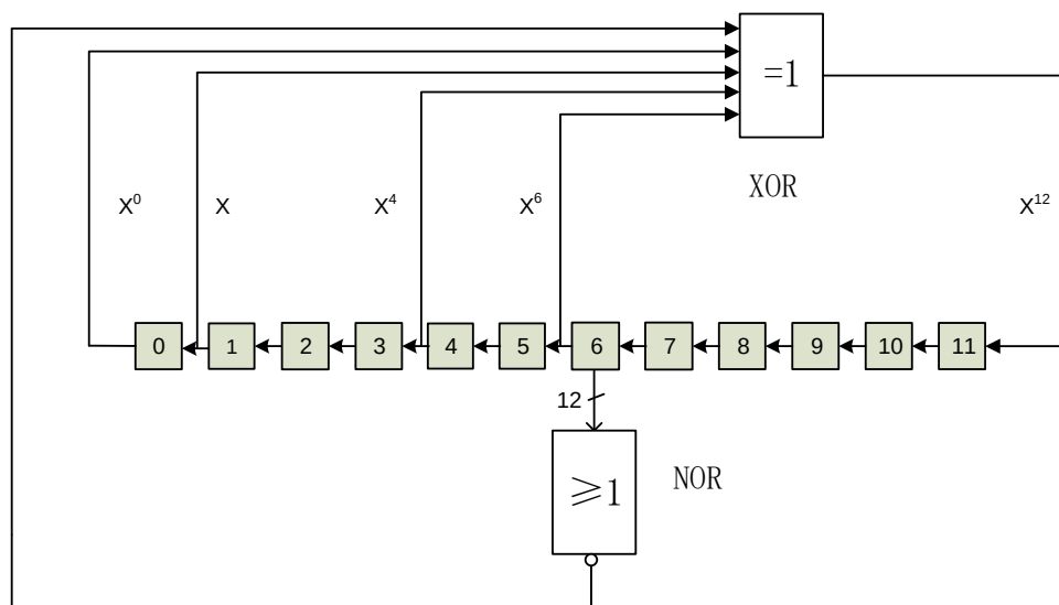
Figure 21-2. DAC LFSR algorithm
