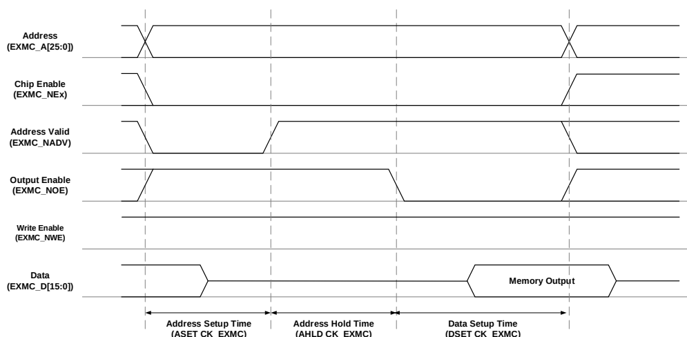
Figure 38-16. Mode D read access
