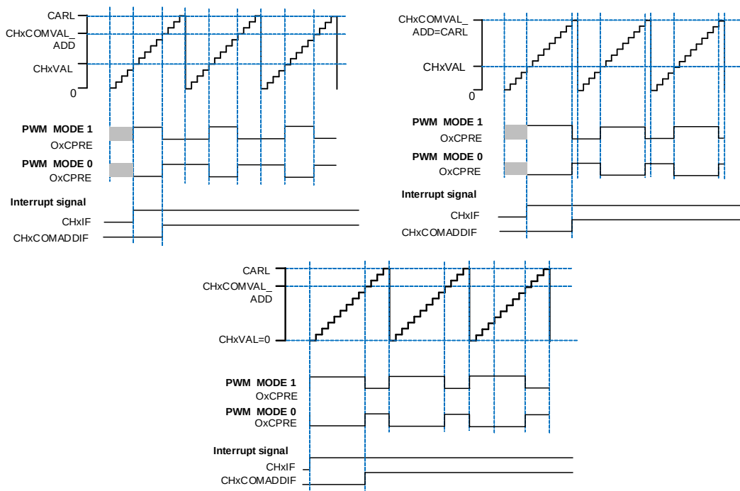
Figure 24-63. Channel x output PWM with (CHxVAL < CHxCOMVAL_ADD)
