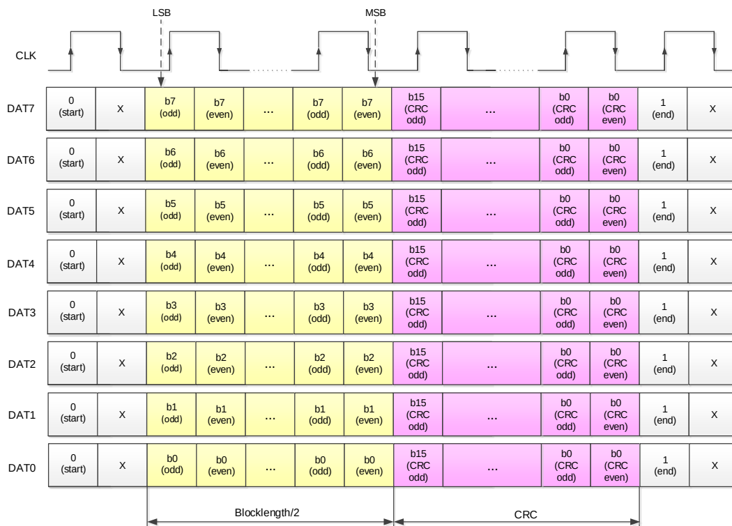
Figure 36-15. 8-bit data bus DDR
