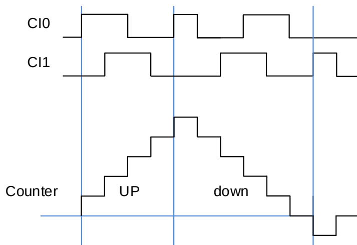
Figure 24-33. Example of counter operation in decoder interface mode
