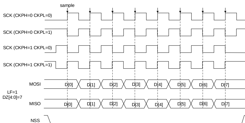
Figure 27-2. SPI timing diagram in normal mode
