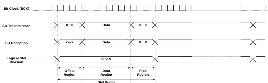
Figure 34-12 Data configuration
