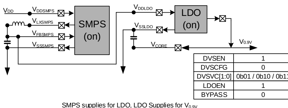
Figure 5-10. SMPS supplies for LDO, LDO supplies for 0.9V power domain
