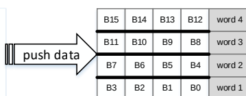
Figure 16-4. Data packing/unpacking when PWIDTH = '00'
