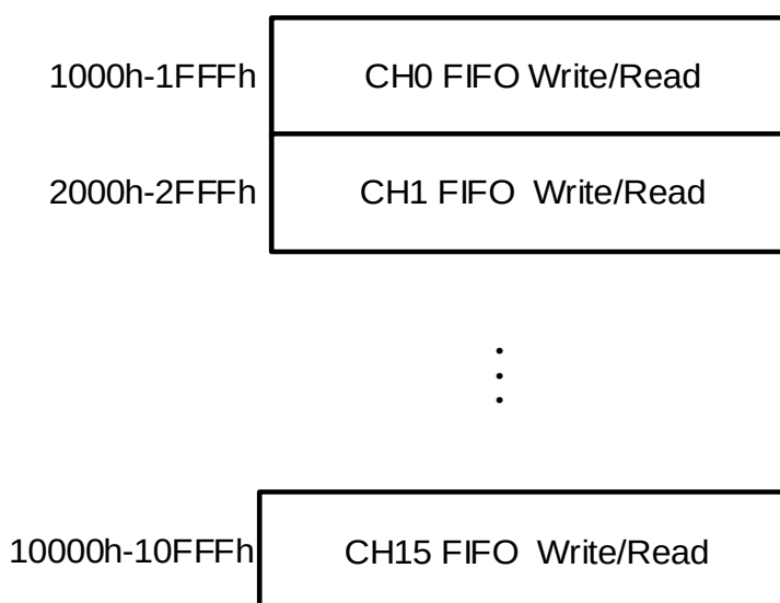
Figure 49-7. Host mode FIFO access register map
