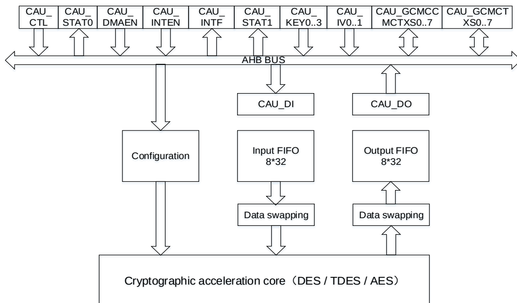
Figure 13-3. CAU diagram
