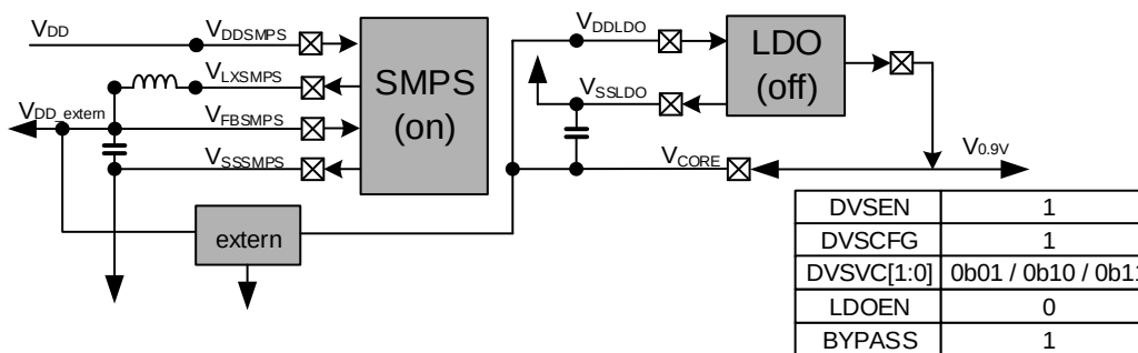
Figure 5-12. SMPS supplies for external, external supplies for 0.9V power domain
