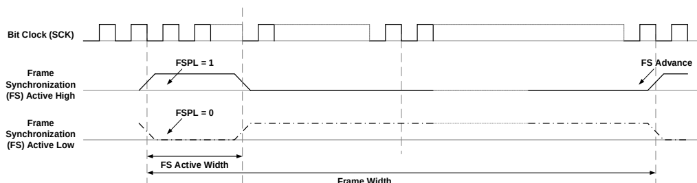
Figure 34-4 FS polarity
