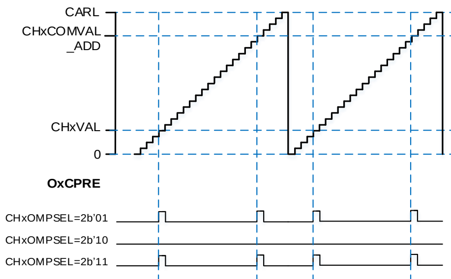
Figure 24-25. CHx_O output with a pulse in edge-aligned mode (CHxOMPSEL ≠ 2'b00)
