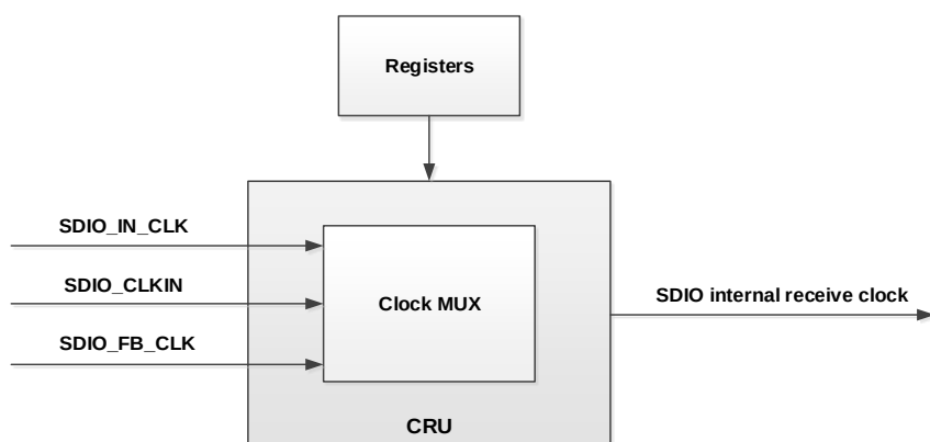
Figure 36-7. CRU unit
