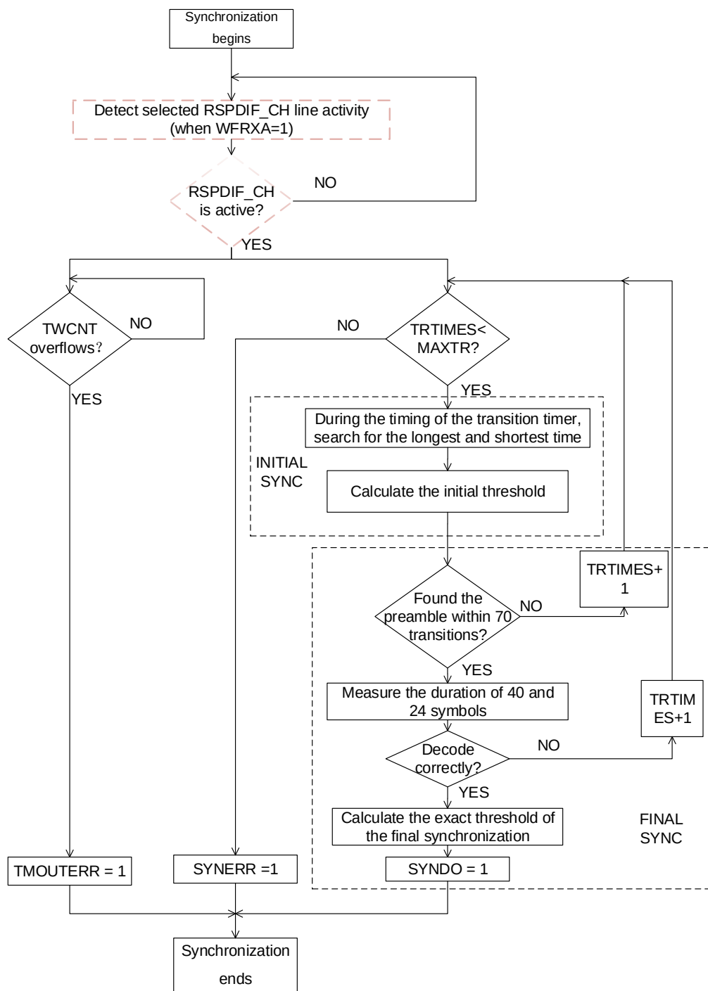
Figure 33-10. Synchronization process scheduling
