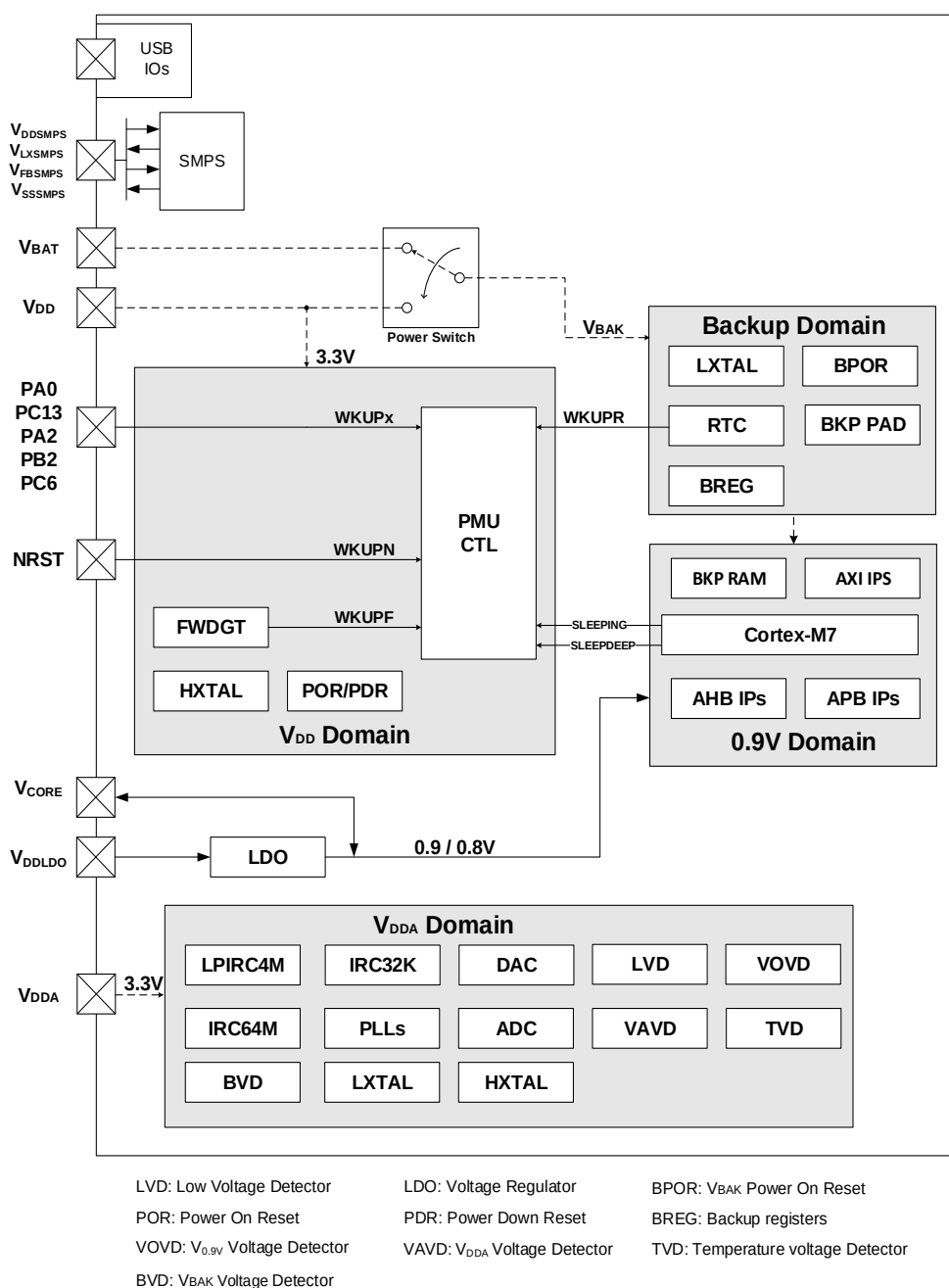
Figure 5-1. Power supply overview
