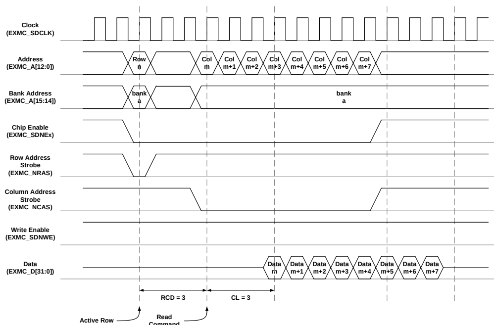
Figure 38-27. Burst read operation
