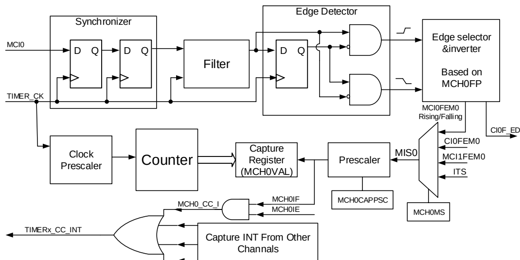
Figure 24-13. Input capture logic for multi mode channel 0
