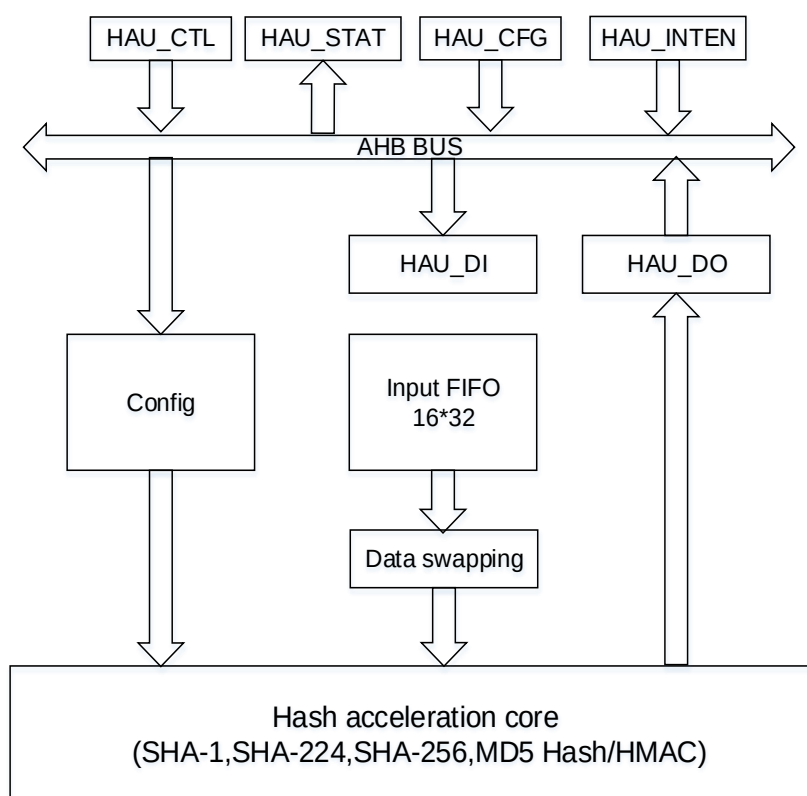
Figure 14-3. HAU block diagram
