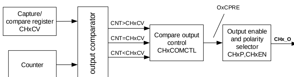
Figure 24-59. Output compare logic (x=0,1,2,3)
