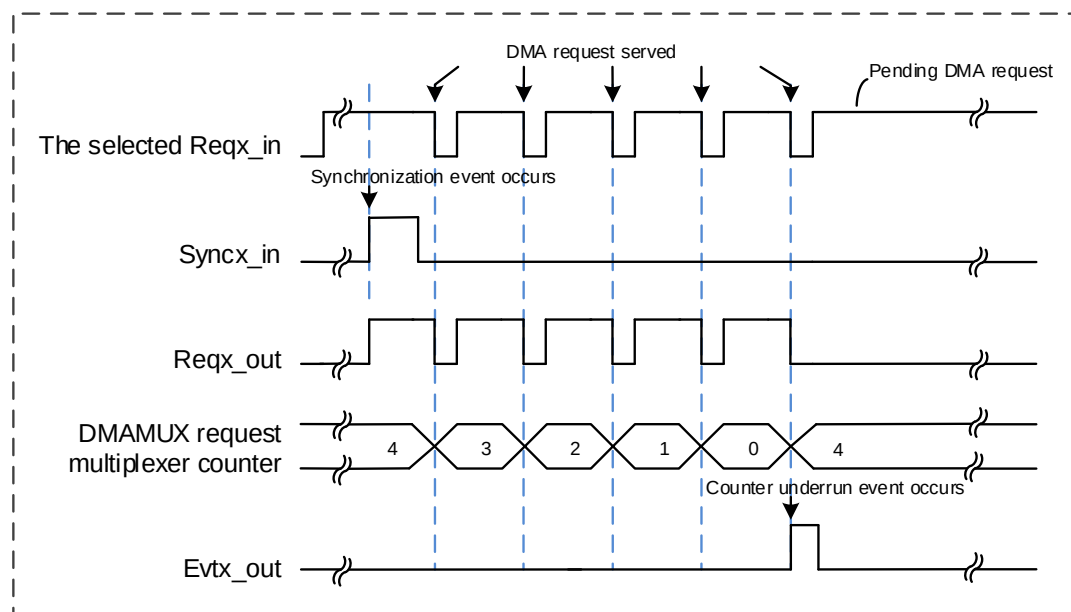
Figure 18-2. Synchronization mode
