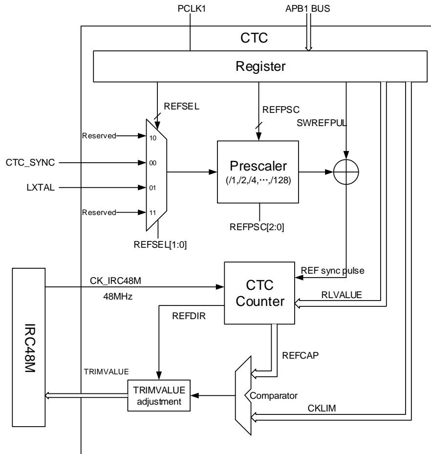
Figure 6-1. CTC overview
