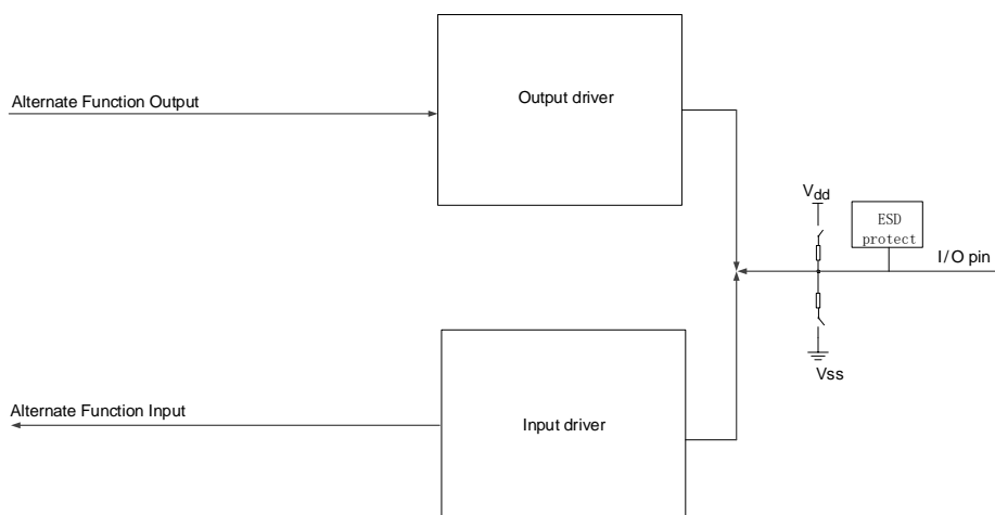
Figure 8-5. Basic structure of Alternate function configuration
