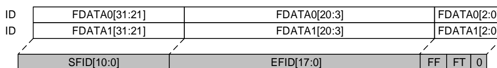
Figure 21-9. 32-bit list mode filter
