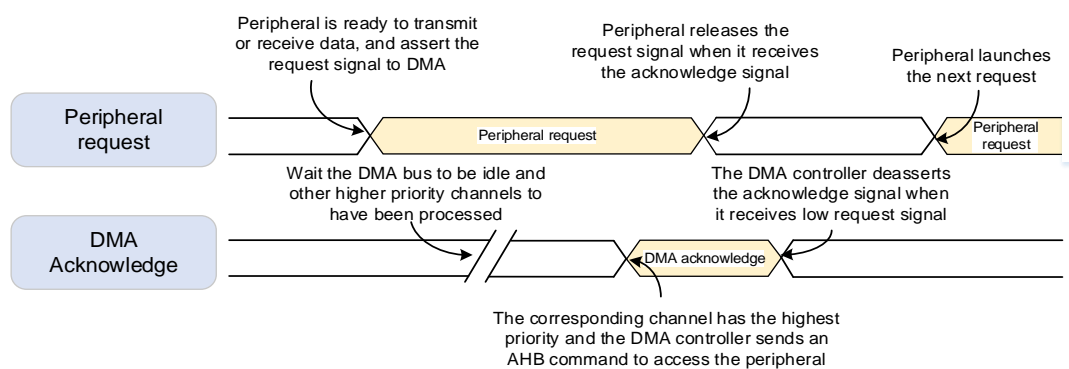
Figure 10-2. Handshake mechanism
