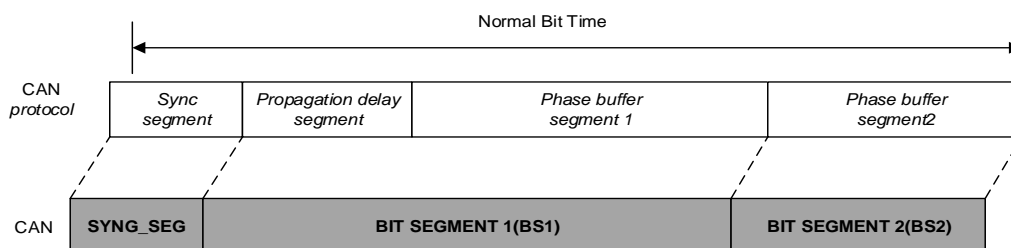
Figure 21-11. The bit time
