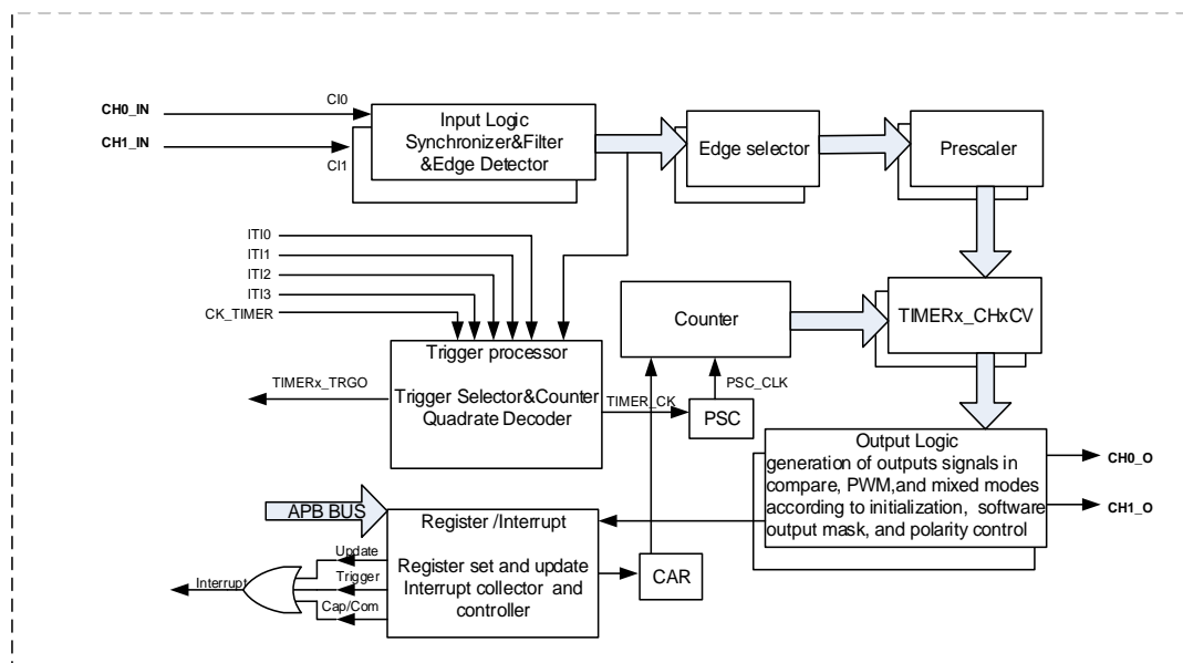
Figure 16-44. General level1 timer block diagram
