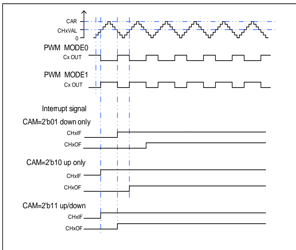
Figure 16-52. CAPWM timechart
