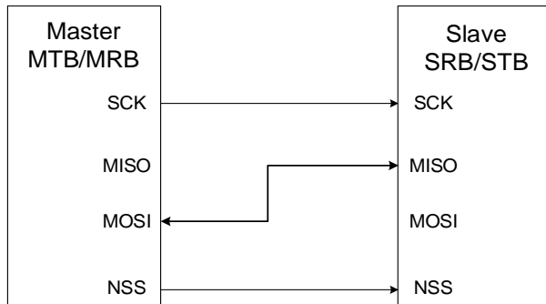
Figure 19-7. A typical bidirectional connection
