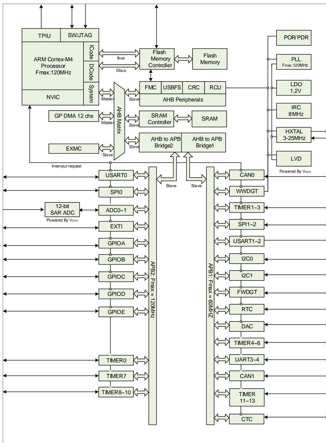
Figure 1-2. GD32C11x series system architecture
