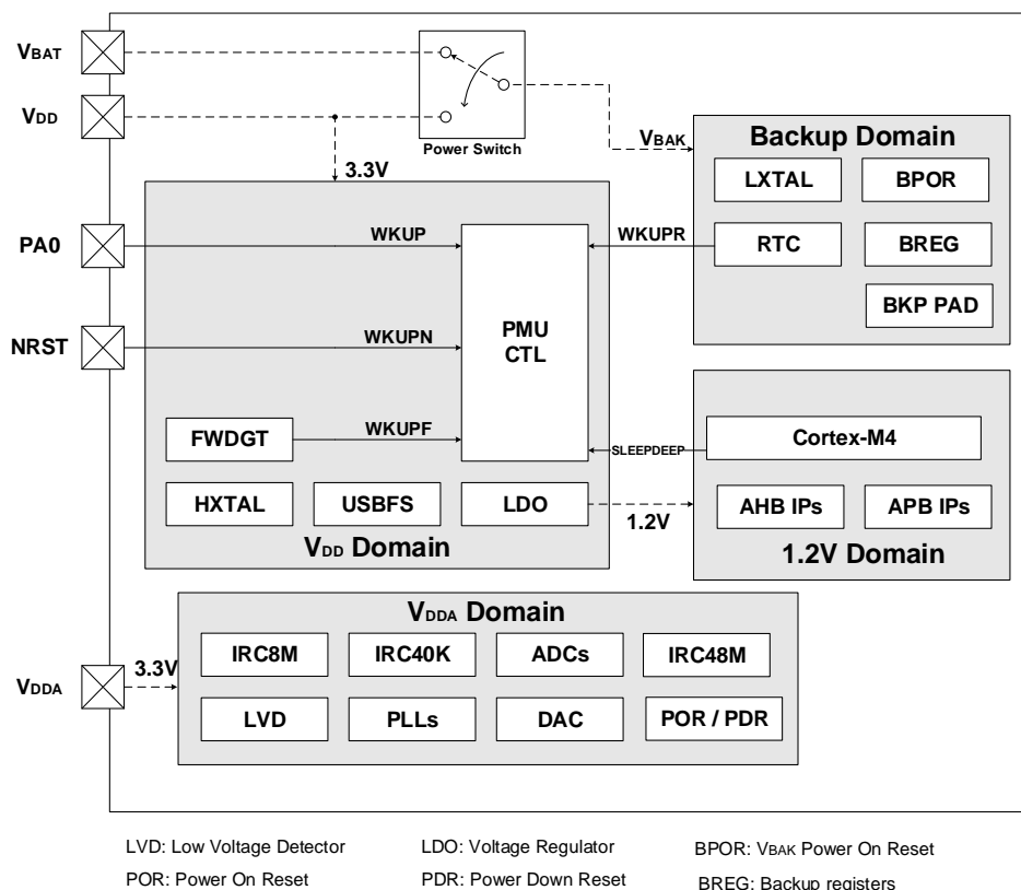
Figure 3-1. Power supply overview
