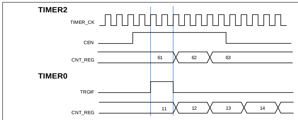
Figure 16-27. Triggering TIMER0 with enable signal of TIMER2
