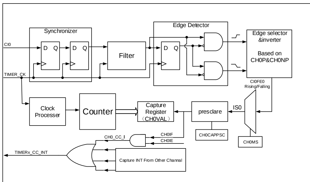
Figure 16-62. Channel input capture principle
