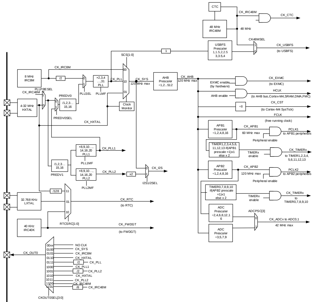
Figure 5-2. Clock tree
