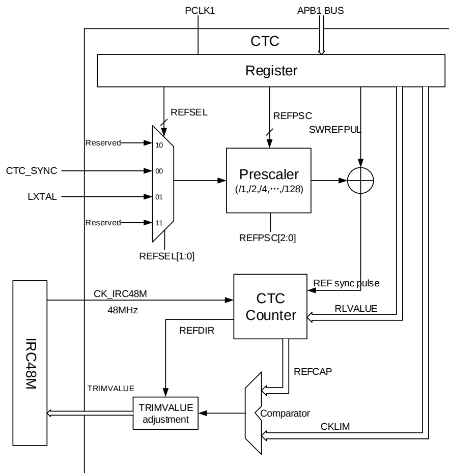
Figure 6-1. CTC overview
