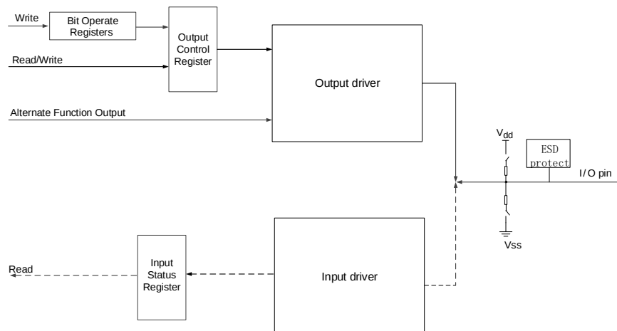
Figure 8-3. Basic structure of Output configuration
