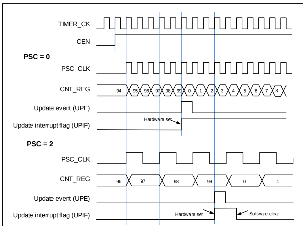
Figure 16-47. Timing chart of up counting mode, PSC=0/2
