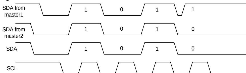
Figure 18-5. SDA line arbitration
