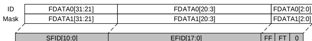
Figure 21-7. 32-bit mask mode filter
