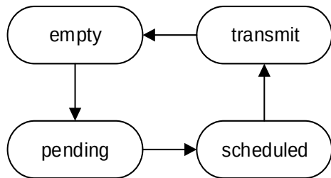
Figure 21-3. State of transmit mailbox
