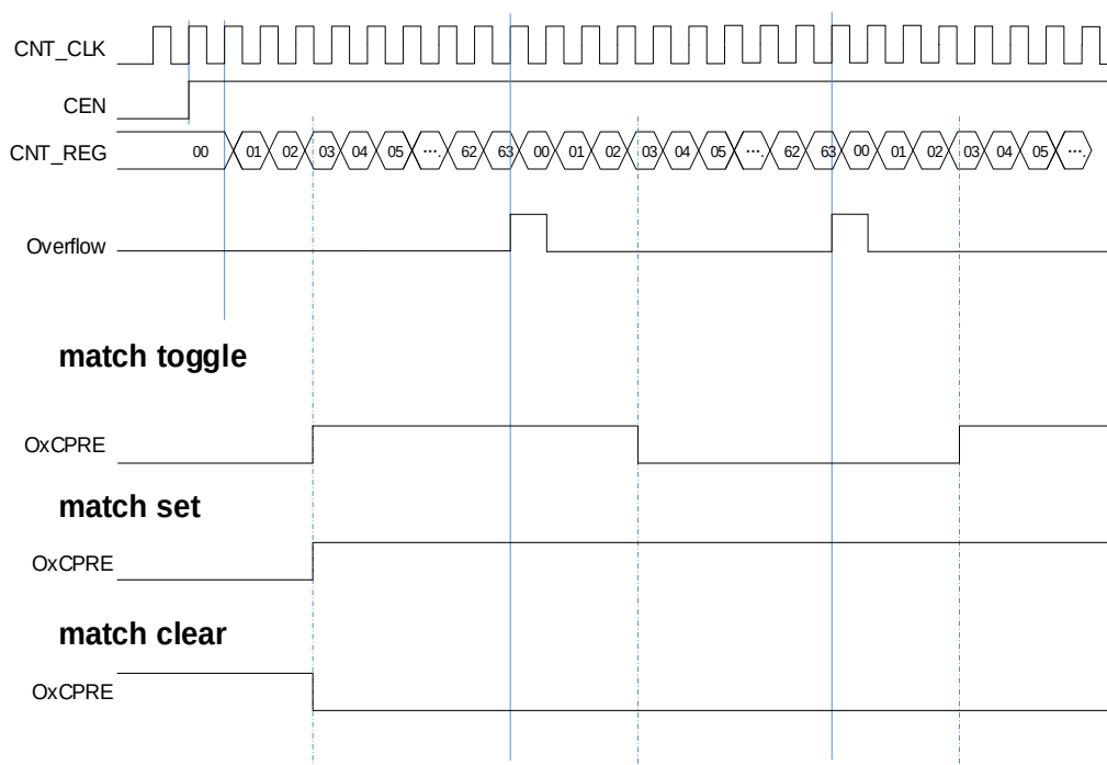
Figure 18-40. Output-compare in three modes
