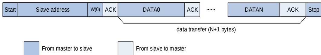
Figure 21-18. I2C communication flow with 7-bit address (Master Transmit)
