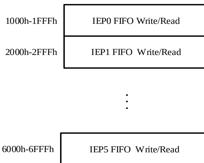
Figure 29-9. Device mode FIFO access register map
