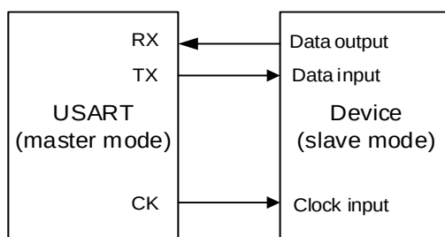
Figure 20-25. Example of USART in synchronous mode
