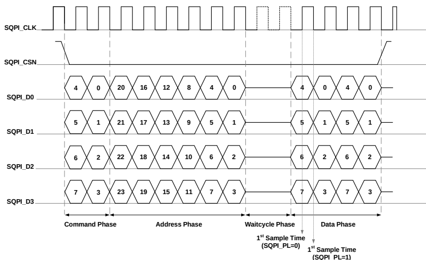
Figure 23-1. SQPI_PL Example
