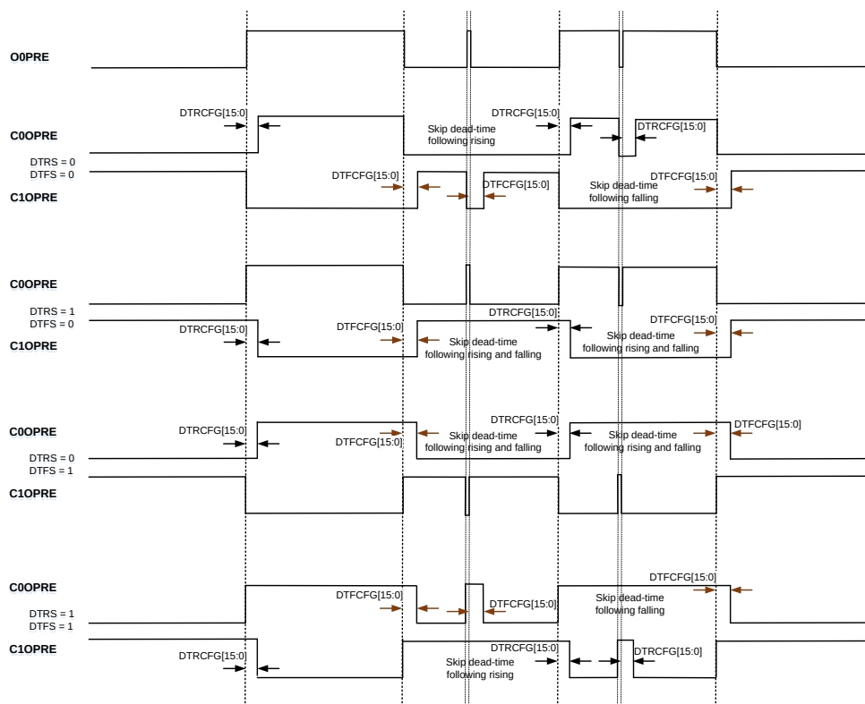
Figure 19-27. Complementary wave with pulse width less than dead-time
