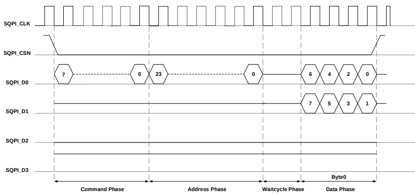
Figure 23-9. SQPI SSD Mode Timing
