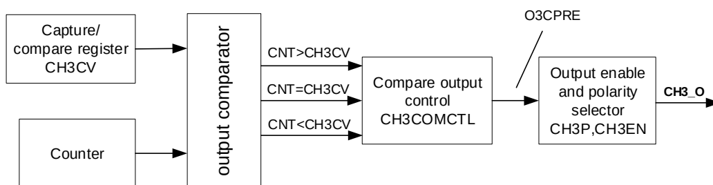
Figure 18-14. Channel output compare principle (CH3_O)
