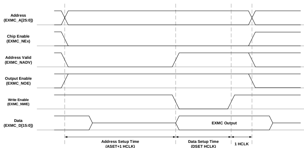
Figure 25-12. Mode B write access
