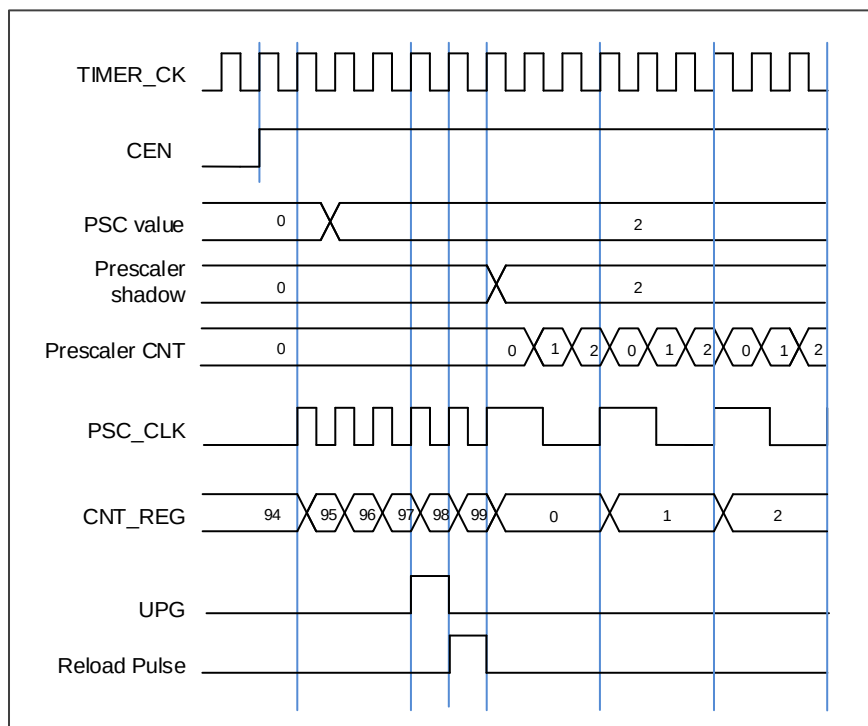
Figure 18-3. Timing chart of PSC value change from 0 to 2
