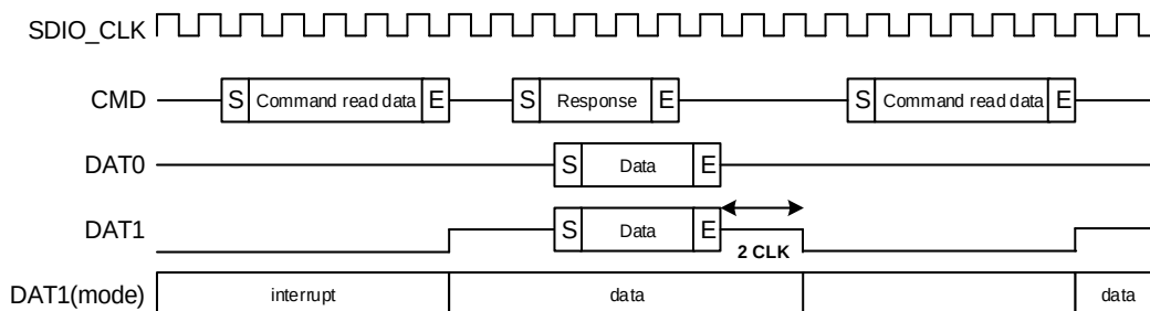
Figure 24-15. Read Interrupt cycle timing
