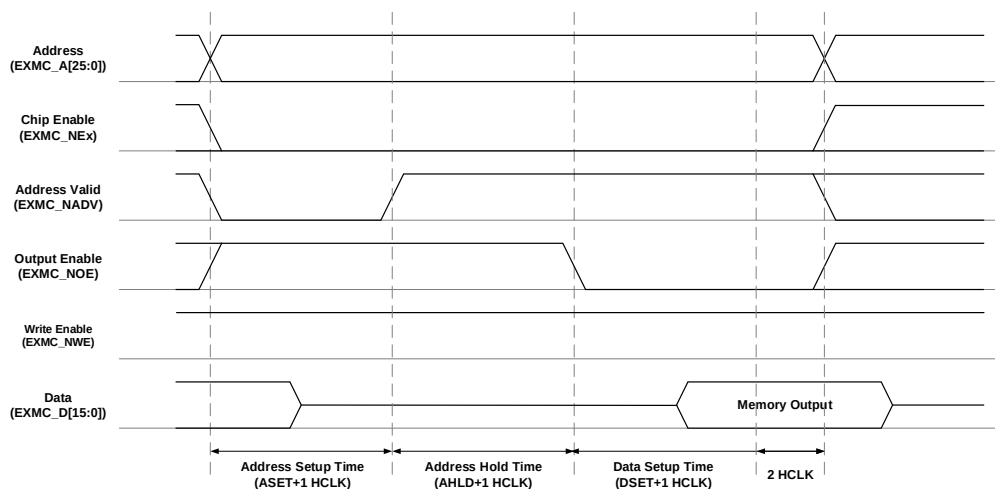
Figure 25-15. Mode D read access
