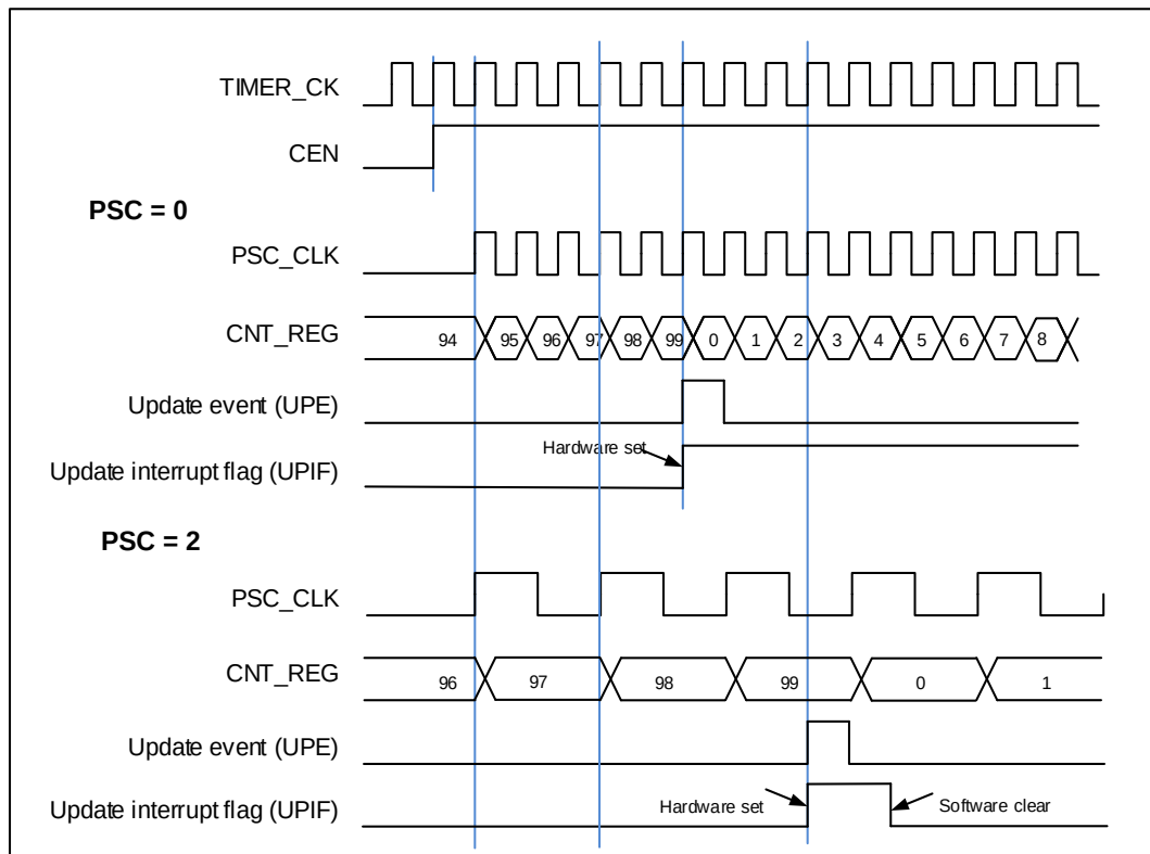
Figure 18-49. Timing chart of up counting mode, PSC=0/2
