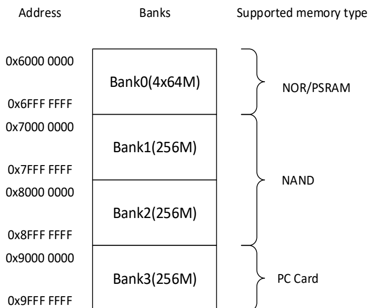
Figure 25-2. EXMC memory banks
