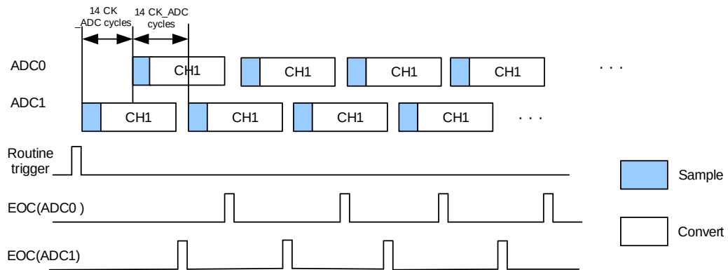
Figure 13-15. Routine follow-up slow mode on routine sequence channel
