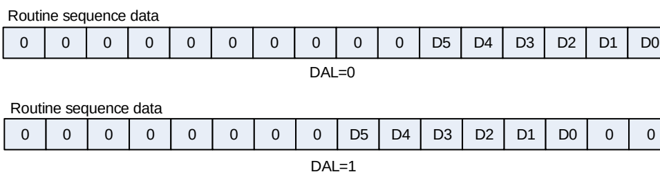
Figure 13-9. 6-bit data storage mode
