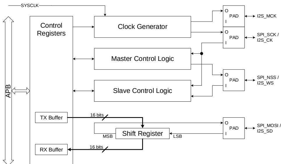
Figure 22-14. Block diagram of I2S
