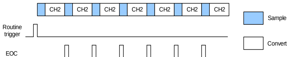
Figure 13-4. Continuous operation mode
