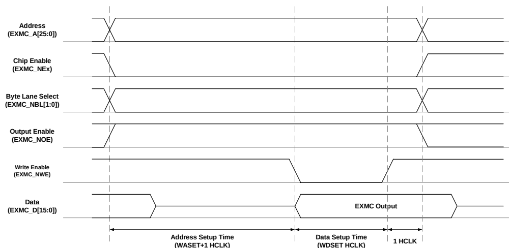
Figure 25-9. Mode A write access
