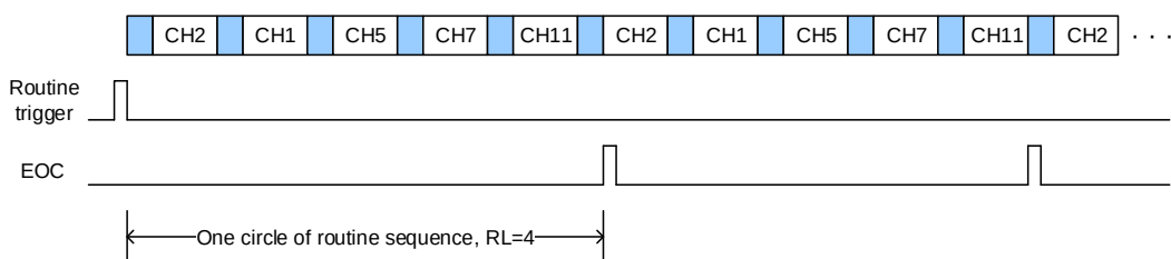
Figure 13-6. Scan operation mode, continuous operation mode enable
