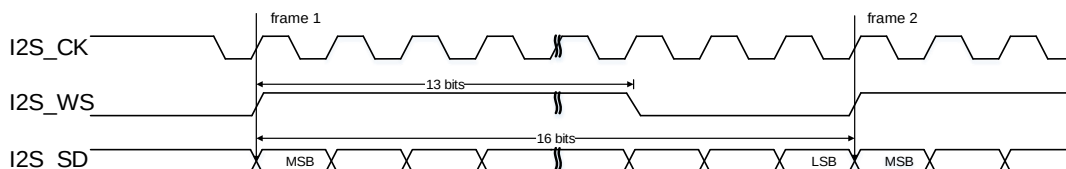
Figure22-44. PCM standard long frame synchronization mode timing diagram (DTLEN=00, CHLEN=0, CKPL=1)
