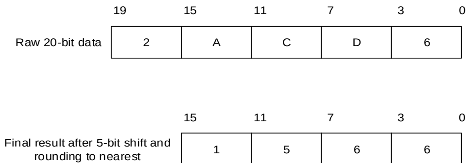
Figure 13-11. Numerical example with 5-bits shift and rounding
