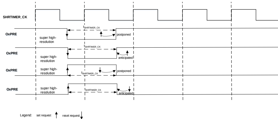
Figure 19-21. A pulse of 1 t_{SHRTMER\_CK} period
