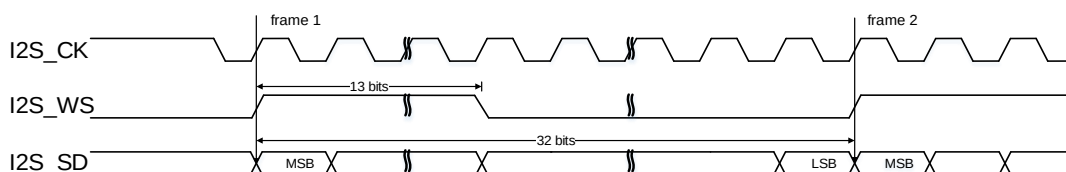
Figure 22-46. PCM standard long frame synchronization mode timing diagram (DTLEN=10, CHLEN=1, CKPL=1)
