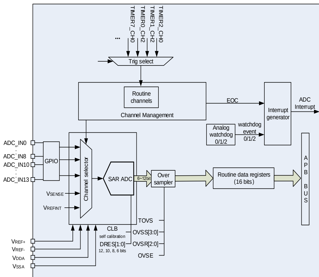
Figure 13-2. ADC module block diagram (for ADC2)
