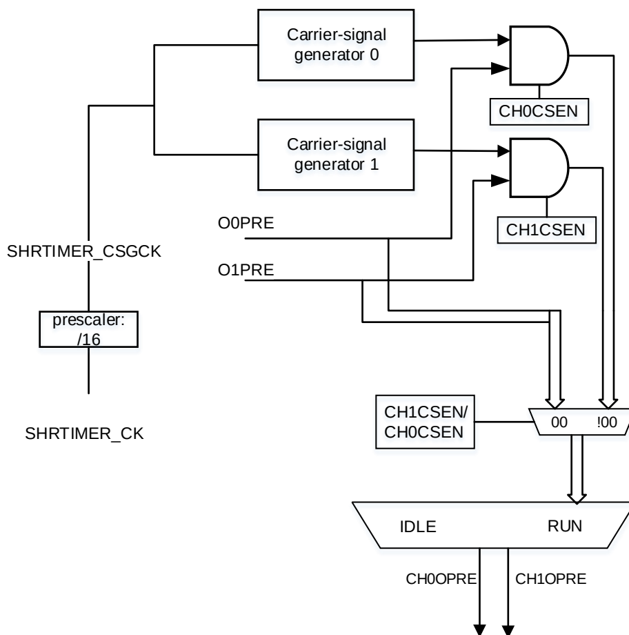
Figure 19-36. Carrier-signal structure diagram
