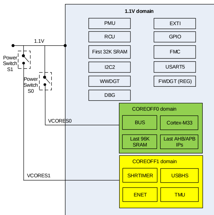
Figure 4-2. 1.1V domain supply overview
