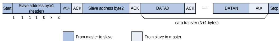
Figure 21-17. I2C communication flow with 10-bit address (Master Transmit)
