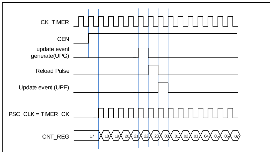
Figure 18-47. Timing chart of internal clock divided by 1
