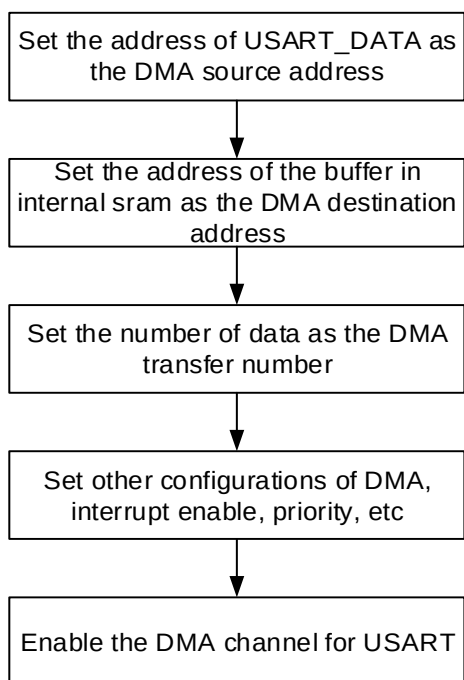
Figure 20-6. Configuration steps when using DMA for USART reception
