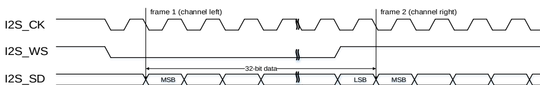
Figure 22-18. I2S Philips standard timing diagram (DTLEN=10, CHLEN=1, CKPL=1)
