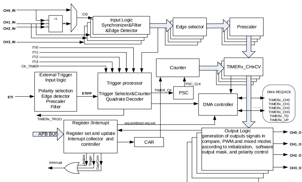
Figure 18-30. General Level 0 timer block diagram
