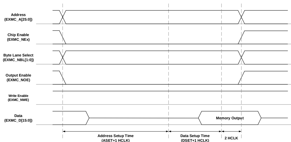
Figure 25-7. Mode 1 write access
