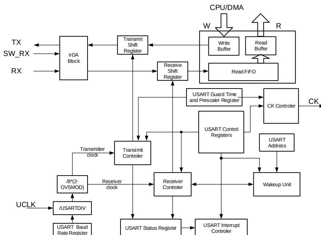
Figure 20-17. USART module block diagram
