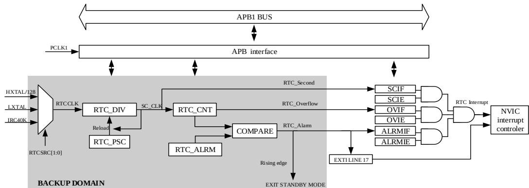
Figure 17-1. Block diagram of RTC
