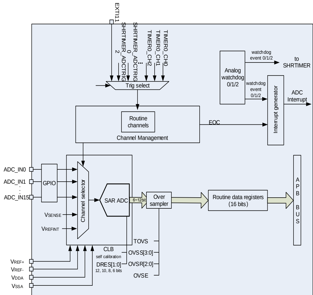
Figure 13-1. ADC module block diagram (for ADC0 and ADC1)
