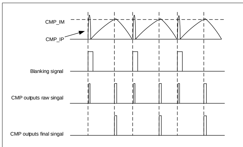
Figure 15-2. The CMP outputs signal blanking
