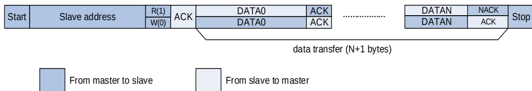
Figure 21-6. I2C communication flow with 7-bit address
