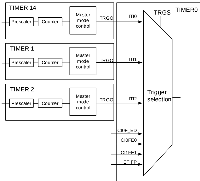
Figure 18-28. Timer0 master/slave mode example
