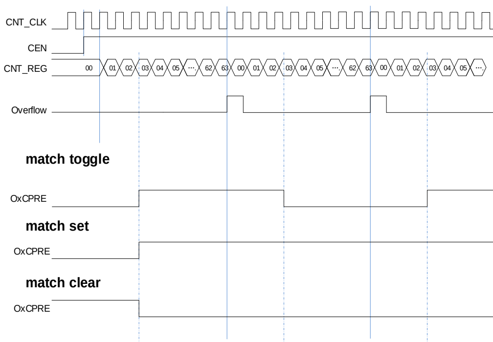
Figure 18-66. Output-compare under three modes
