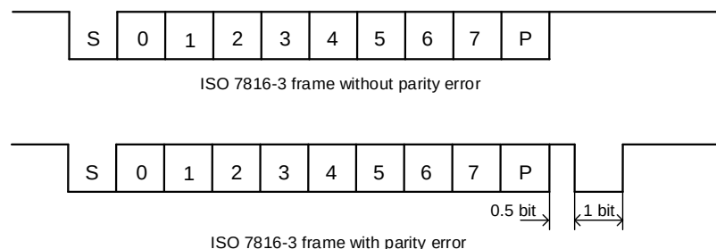
Figure 20-29. ISO7816-3 frame format
