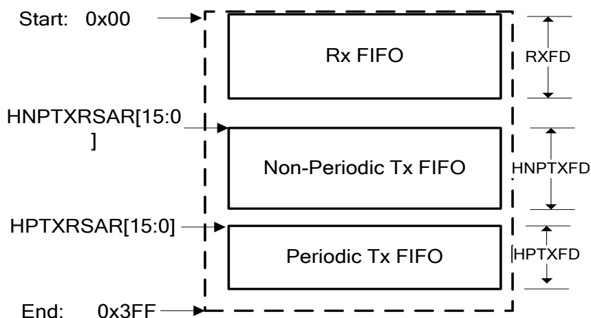
Figure 29-6. Host mode FIFO space in SRAM
