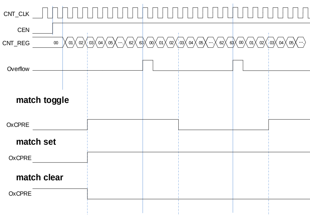
Figure 18-15. Output-compare in three modes
