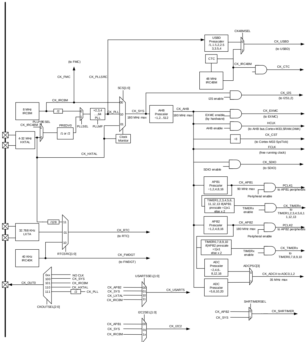
Figure 5-2. Clock tree
