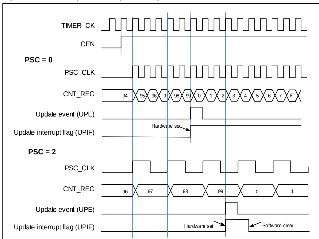
Figure 18-62. Timing chart of up counting mode, PSC=0/2
