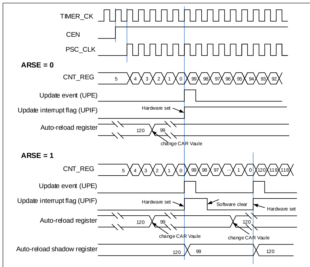
Figure 18-36. Timing chart of down counting mode, change TIMERx_CAR ongoing
