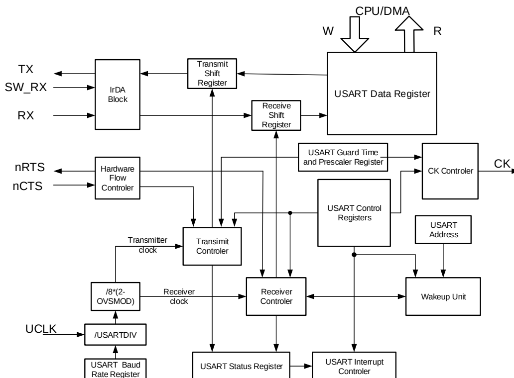
Figure 20-1. USART module block diagram
