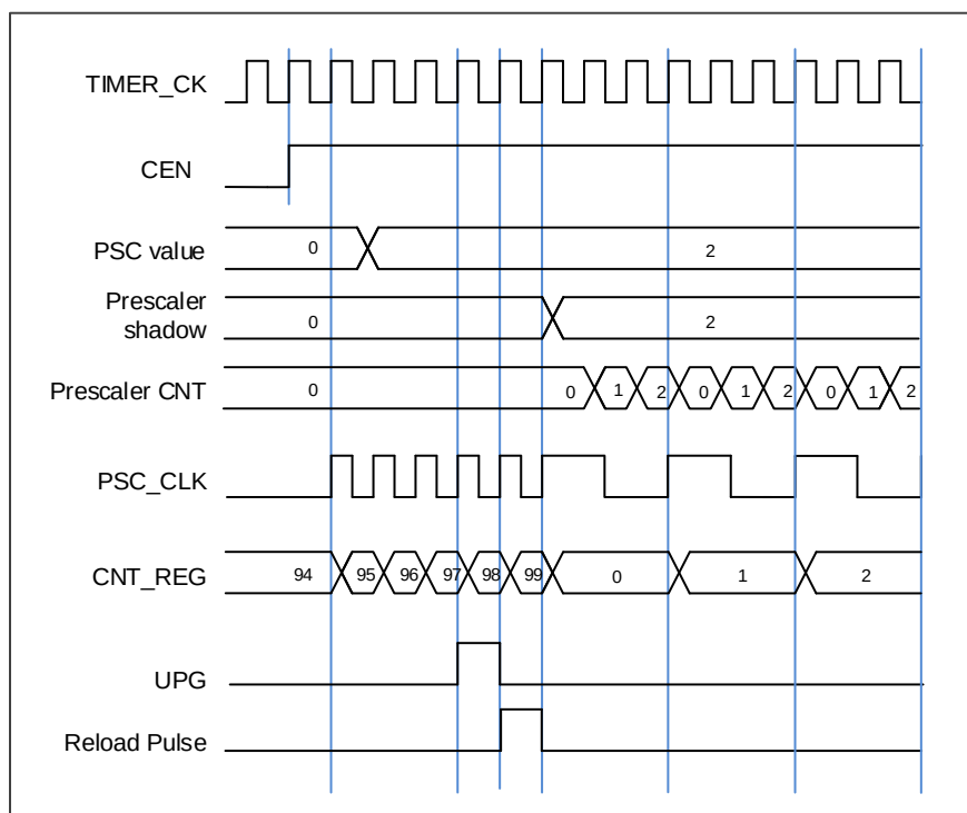
Figure 18-32. Timing chart of PSC value change from 0 to 2
