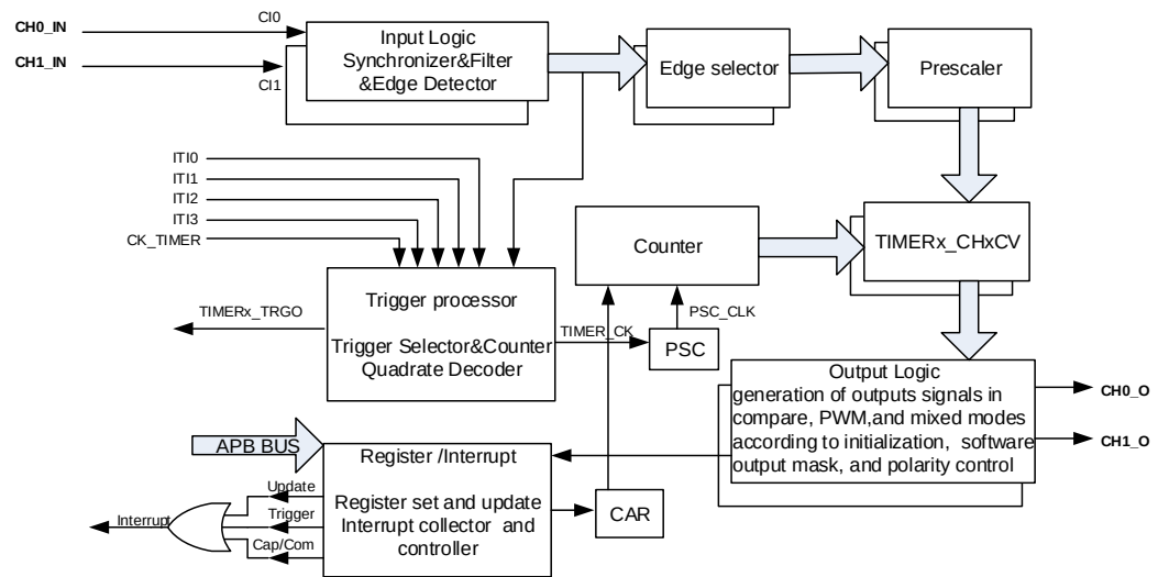
Figure 18-46. General level1 timer block diagram
