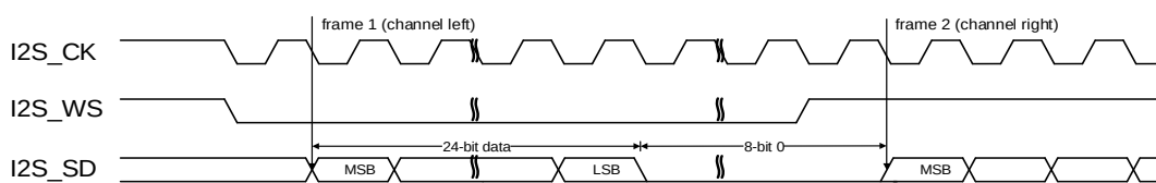
Figure 22-20. I2S Philips standard timing diagram (DTLEN=01, CHLEN=1, CKPL=1)
