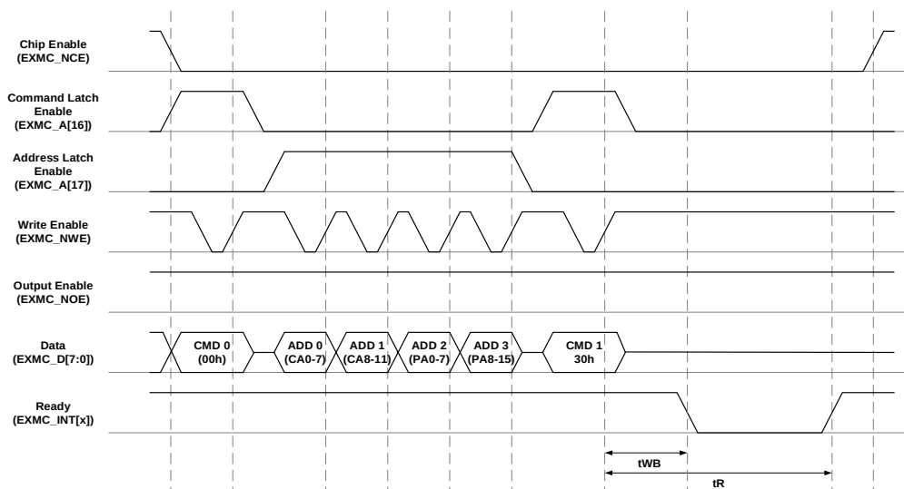
Figure 25-24. Access to none "NCE don't care" NAND Flash
