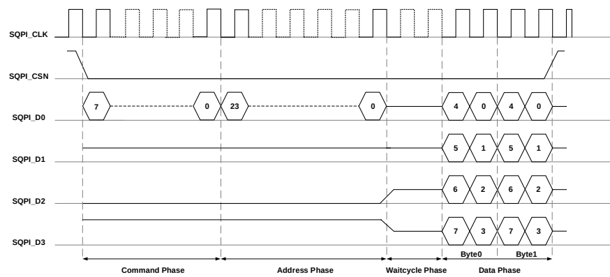
Figure 23-6. SQPI SSQ Mode Timing
