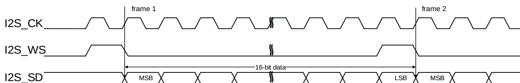
Figure 22-35. PCM standard short frame synchronization mode timing diagram (DTLEN=00, CHLEN=0, CKPL=0)
