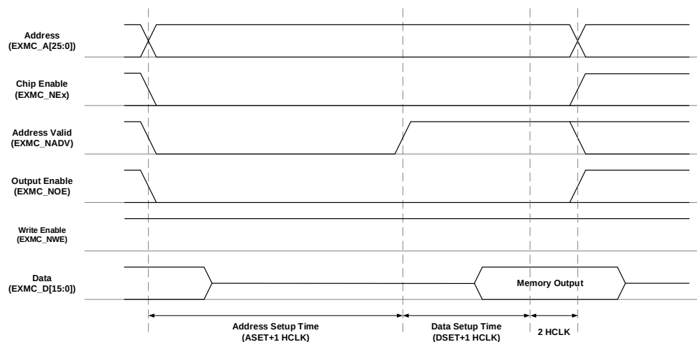
Figure 25-10. Mode 2/B read access
