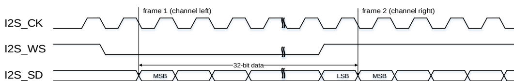
Figure 22-17. I2S Philips standard timing diagram (DTLEN=10, CHLEN=1, CKPL=0)
