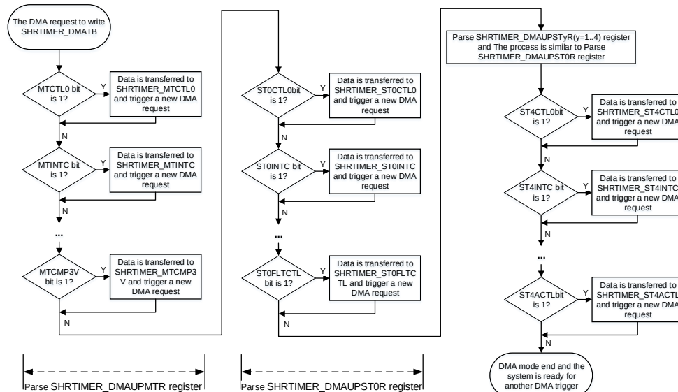
Figure 19-48. DMA mode operation flowchart
