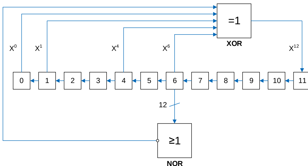
Figure 14-2. DAC LFSR algorithm
