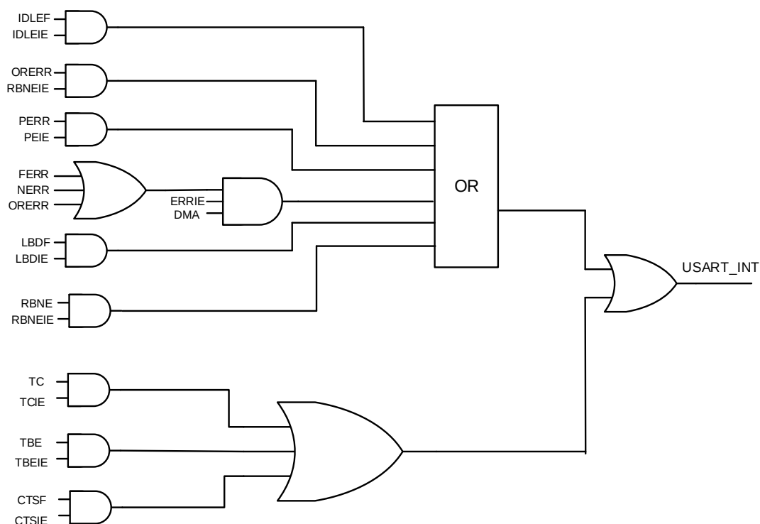
Figure 20-16. USART interrupt mapping diagram
