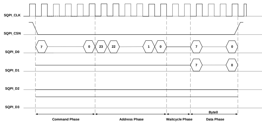
Figure 23-5. SQPI SSS Mode Timing (SPI)
