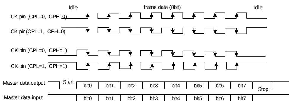
Figure 20-12. 8-bit format USART synchronous waveform (CLEN=1)
