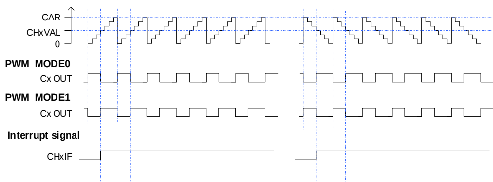
Figure 18-42. Timing chart of CAPWM
