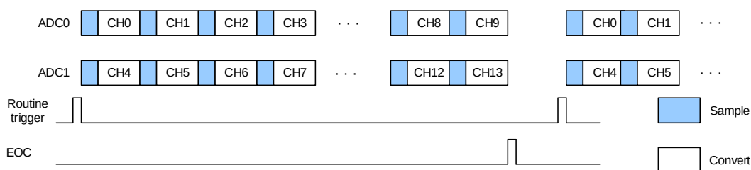
Figure 13-13. Routine parallel mode on 10 channels
