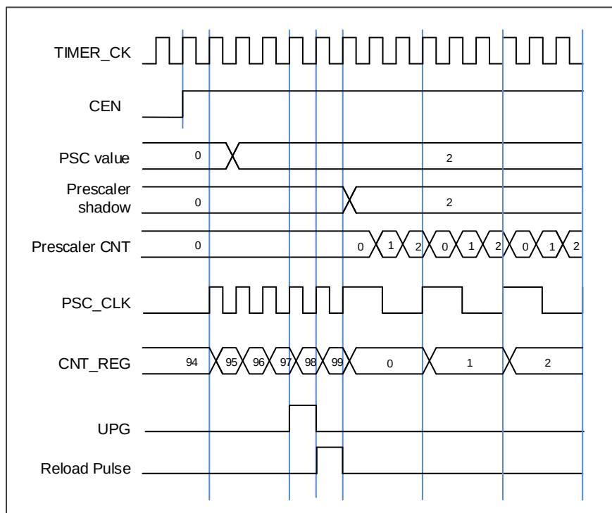
Figure 18-48. Timing chart of PSC value change from 0 to 2
