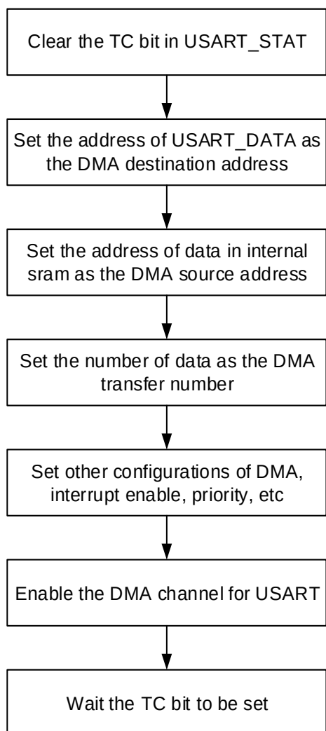
Figure 20-5. Configuration step when using DMA for USART transmission
