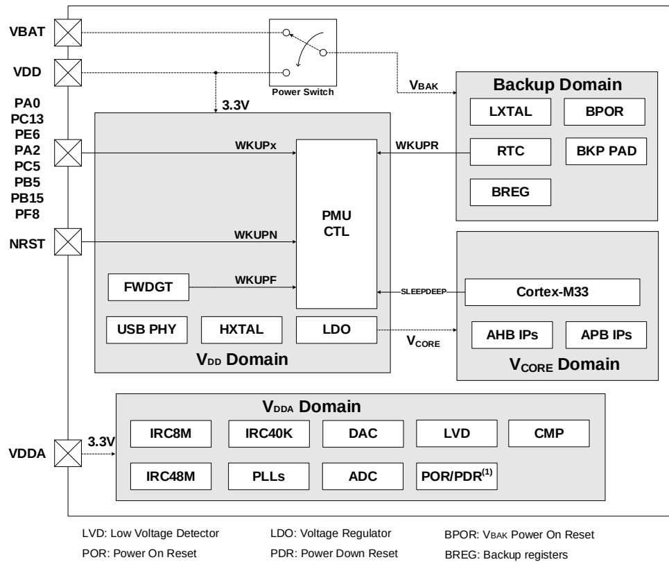
Figure 4-1. Power supply overview
