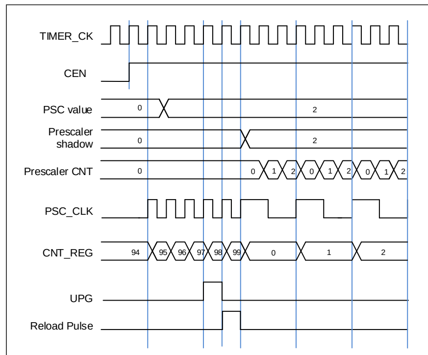
Figure 18-69. Timing chart of PSC value change from 0 to 2
