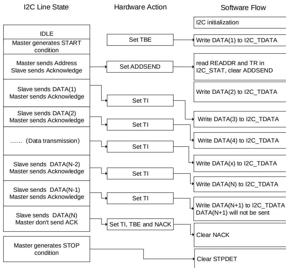
Figure 21-28. Programming model for slave transmitting when SS=1
