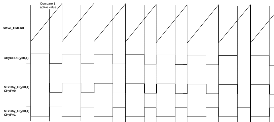
Figure 19-35. STxCHy_O wave with CHyP=0 or CHyP=1
