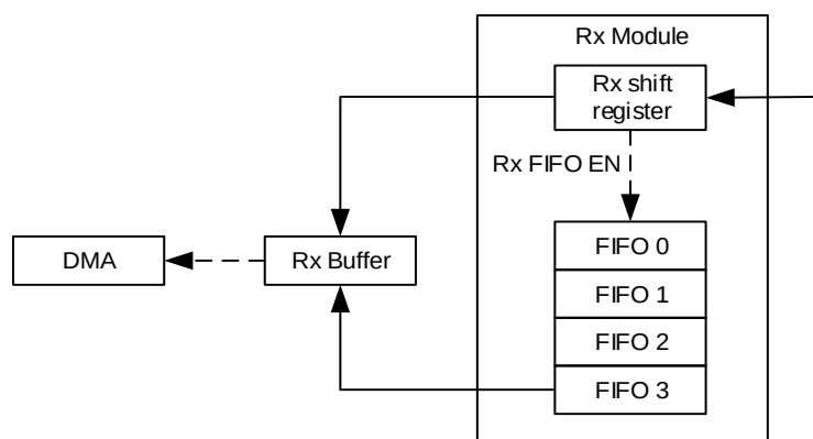
Figure 20-30. USART receive FIFO structure
