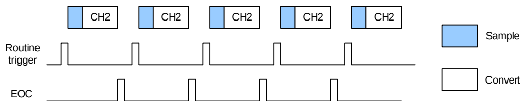
Figure 13-3. Single operation mode
