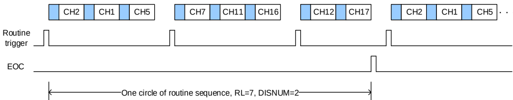
Figure 13-7. Discontinuous operation mode
