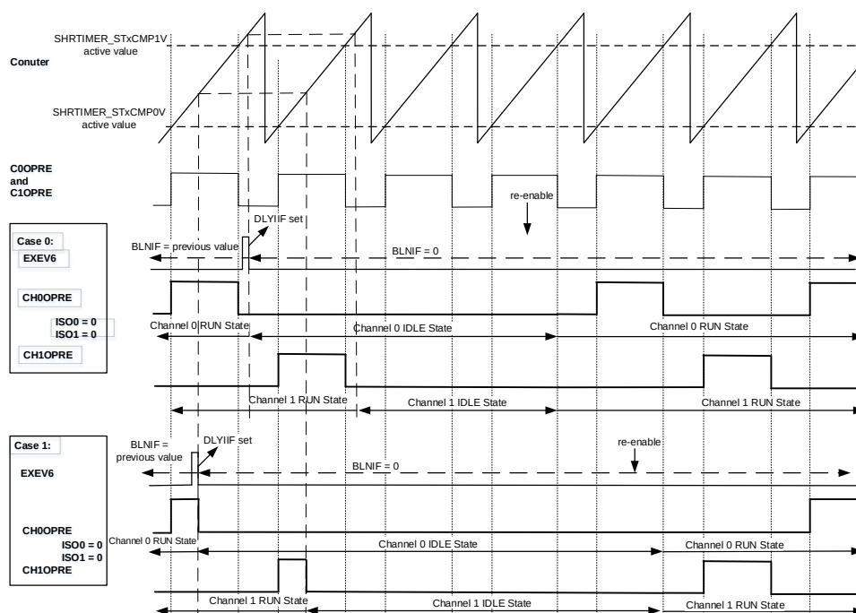
Figure 19-34. Balanced IDEL with ISO0 = 0 and ISO1 = 0
