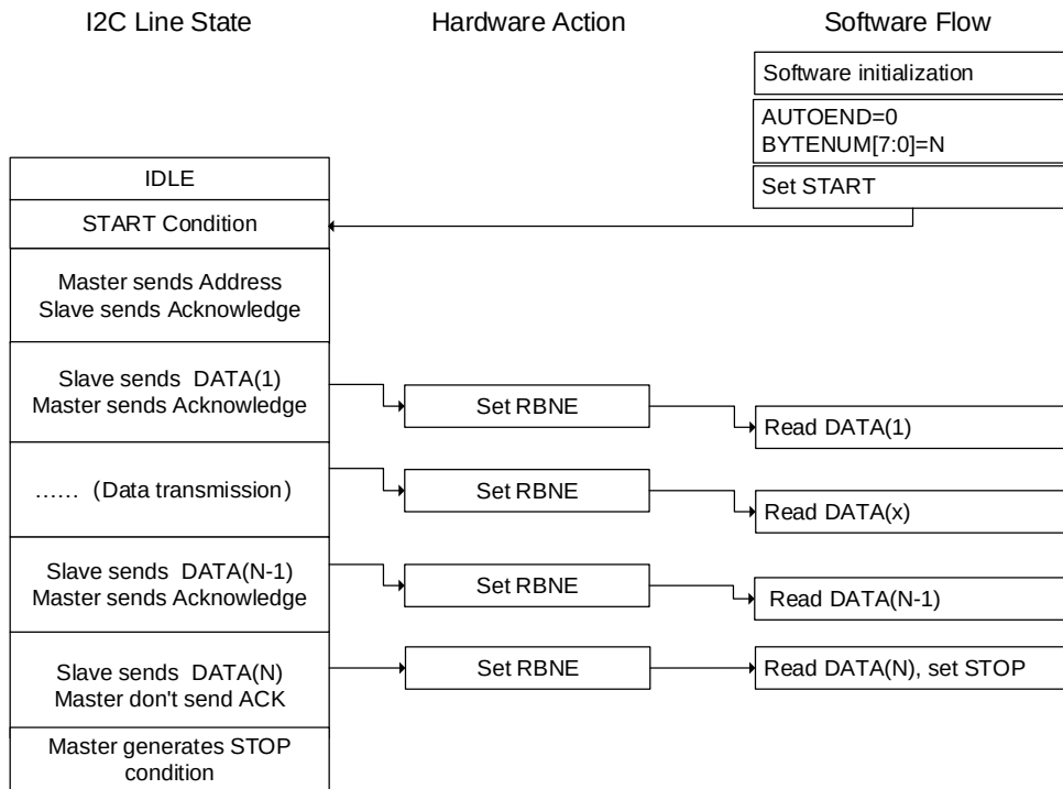
Figure 21-33. Programming model for master receiving ( N \leq 255 )
