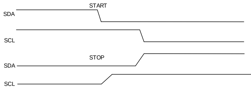
Figure 21-16. START and STOP signal
