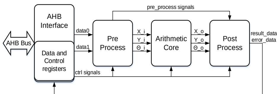
Figure 10-1. Block diagram of Trigonometric Math Unit
