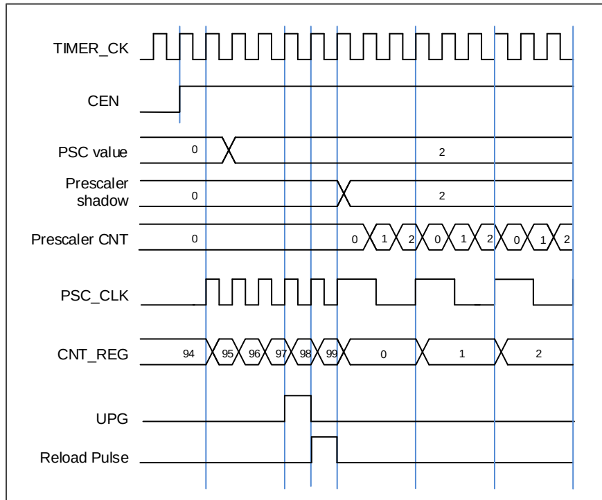
Figure 18-61. Timing chart of PSC value change from 0 to 2
