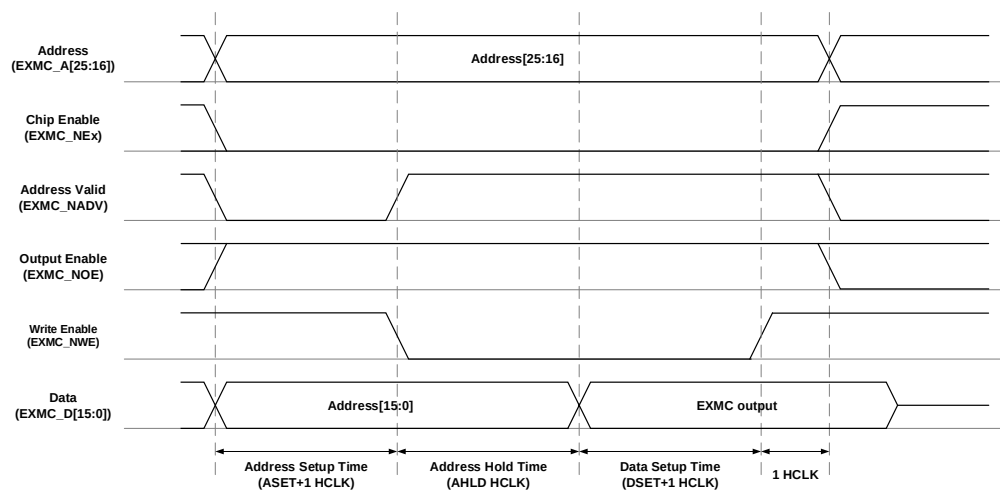
Figure 25-18. Multiplex mode write access
