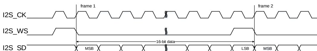
Figure 22-35. PCM standard short frame synchronization mode timing diagram (DTLEN=00, CHLEN=0, CKPL=0)
