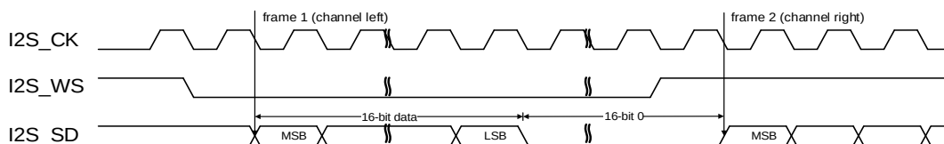
Figure 22-21. I2S Phillips standard timing diagram (DTLEN=00, CHLEN=1, CKPL=0)
