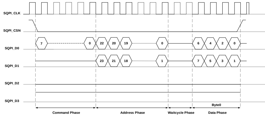
Figure 23-10. SQPI SDD Mode Timing
