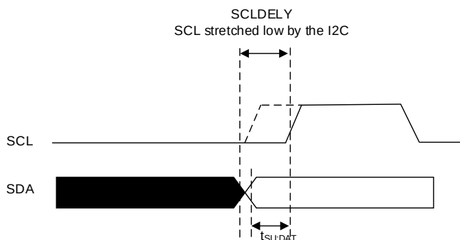
Figure 21-23. Data setup time
