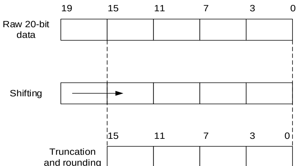
Figure 13-10. 20-bit to 16-bit result truncation
