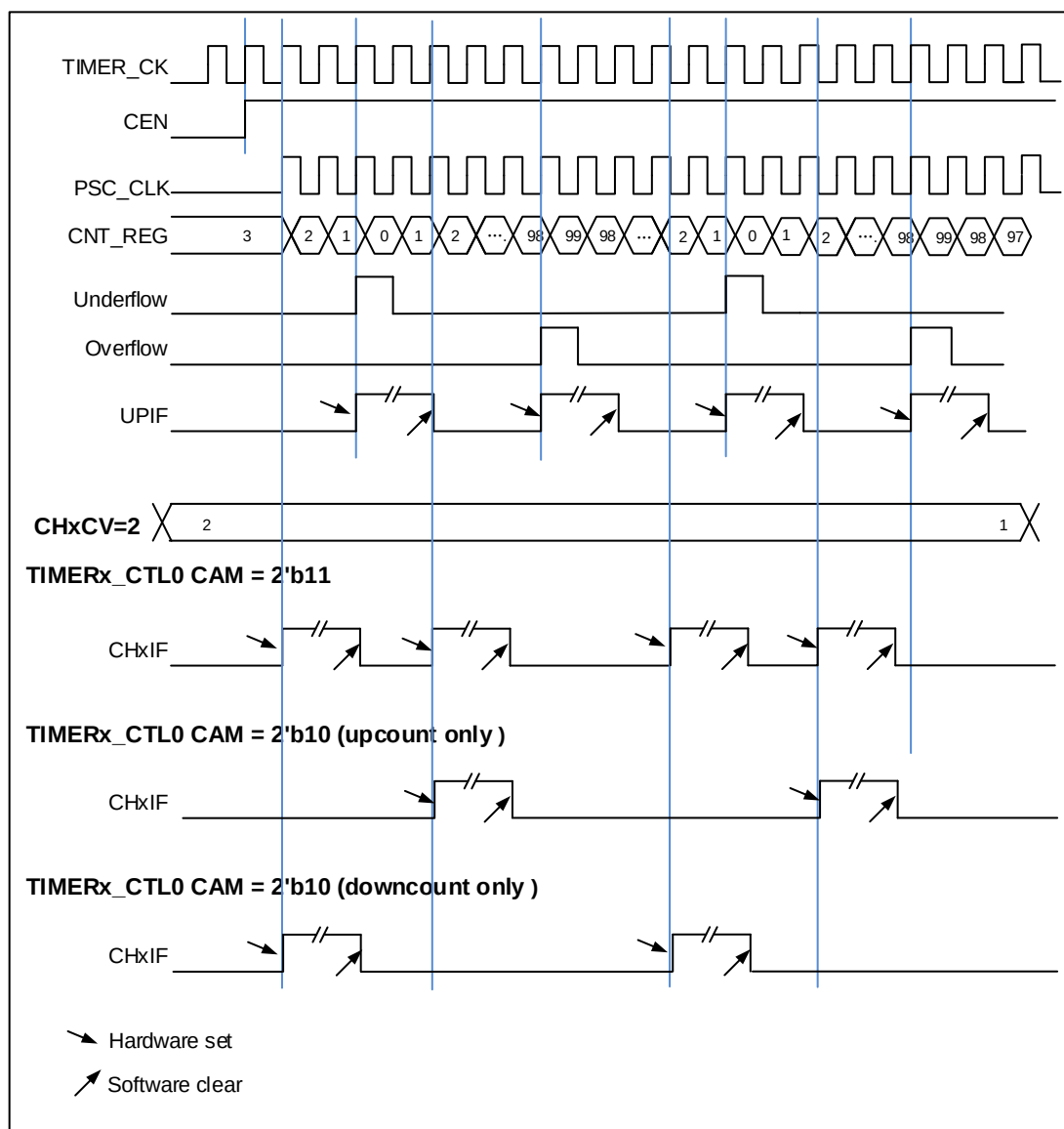
Figure 18-37. Timing chart of center-aligned counting mode
