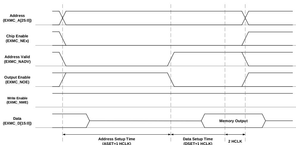
Figure 25-13. Mode C read access
