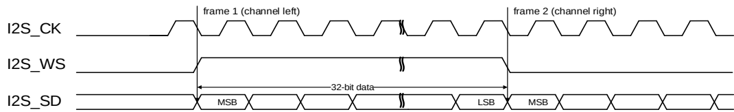
Figure 22-25. MSB justified standard timing diagram (DTLEN=10, CHLEN=1, CKPL=0)
