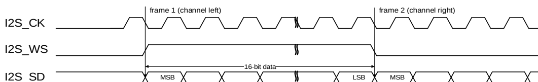
Figure 22-23. MSB justified standard timing diagram (DTLEN=00, CHLEN=0, CKPL=0)
