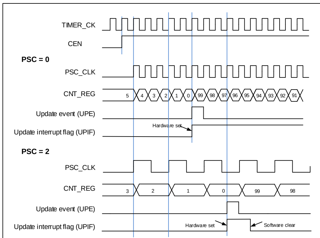
Figure 18-35. Timing chart of down counting mode, PSC=0/2
