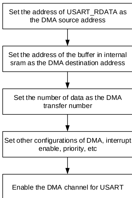
Figure 20-22. Configuration step when using DMA for USART reception
