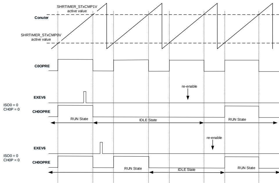
Figure 19-30. ISO0 = 0 and CHOP = 0 in delayed IDLE
