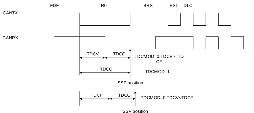
Figure 26-12. Transmitter Delay Measurement
