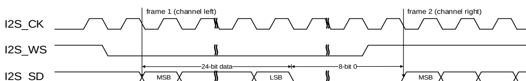
Figure 22-19. I2S Philips standard timing diagram (DTLEN=01, CHLEN=1, CKPL=0)
