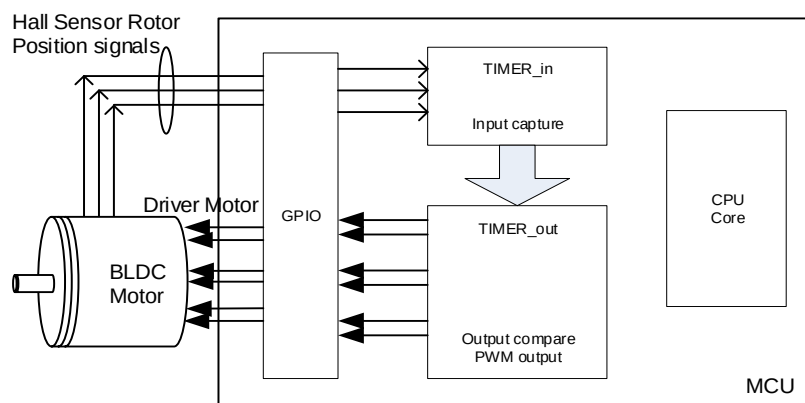
Figure 18-22. Hall sensor is used to BLDC motor
