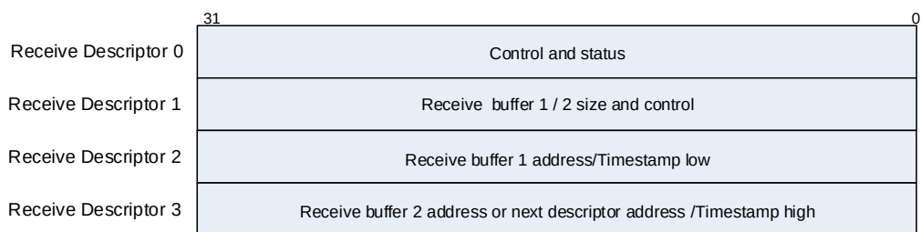
Figure 27-9. Receive descriptor in normal mode
