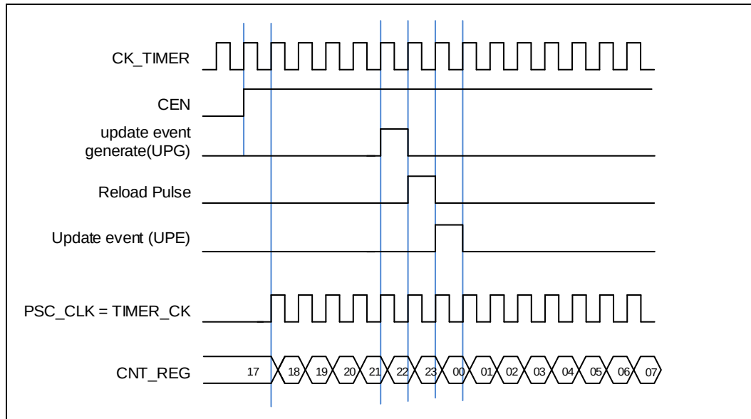
Figure 18-60. Timing chart of internal clock divided by 1
