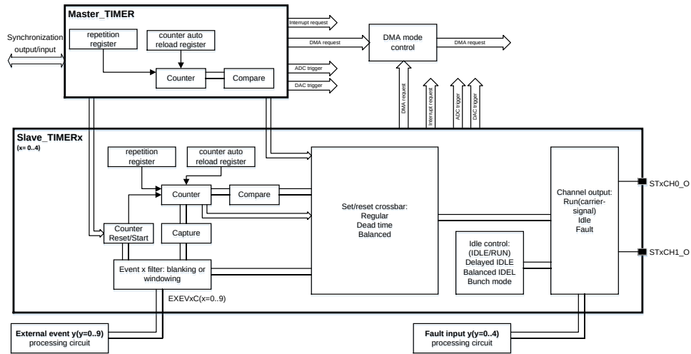
Figure 19-1. SHRTIMER block diagram
