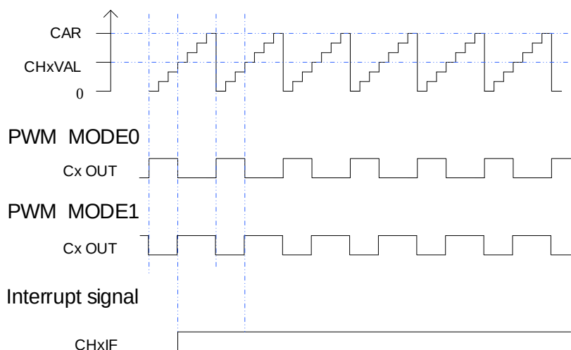
Figure 18-54. PWM mode timechart
