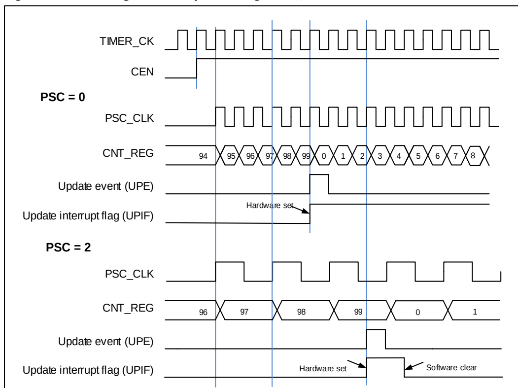
Figure 18-70. Timing chart of up counting mode, PSC=0/2
