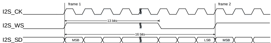
Figure 22-43. PCM standard long frame synchronization mode timing diagram (DTLEN=00, CHLEN=0, CKPL=0)
