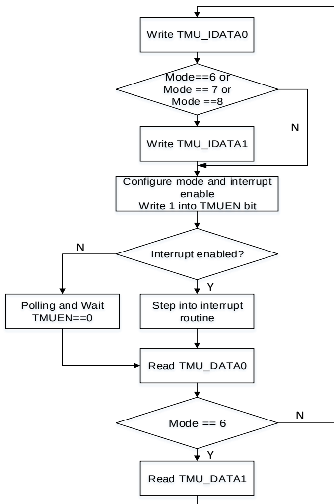
Figure 10-3. TMU program guideline
