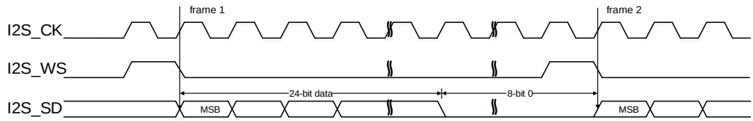
Figure22-40. PCM standard short frame synchronization mode timing diagram (DTLEN=01, CHLEN=1, CKPL=1)
