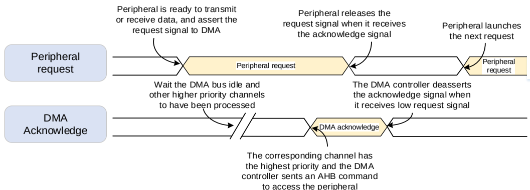
Figure 11-2. Handshake mechanism
