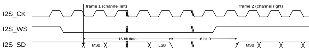
Figure 22-21. I2S Philips standard timing diagram (DTLEN=00, CHLEN=1, CKPL=0)
