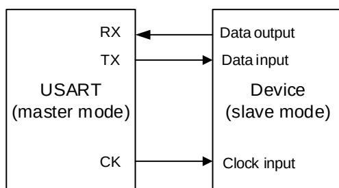
Figure 20-11. Example of USART in synchronous mode
