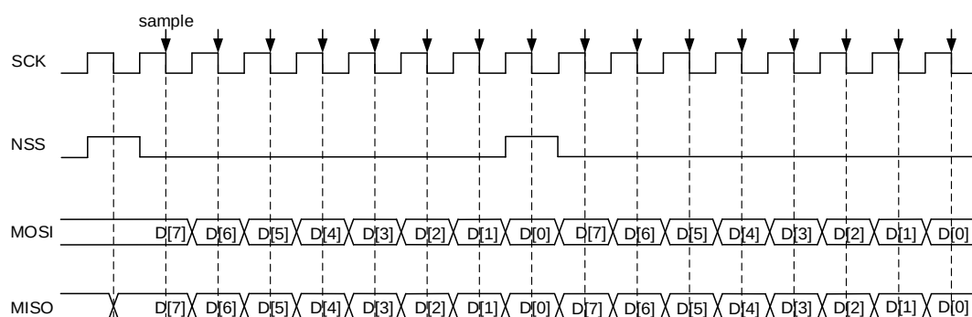
Figure 22-9. Timing diagram of TI master mode with continuous transfer
