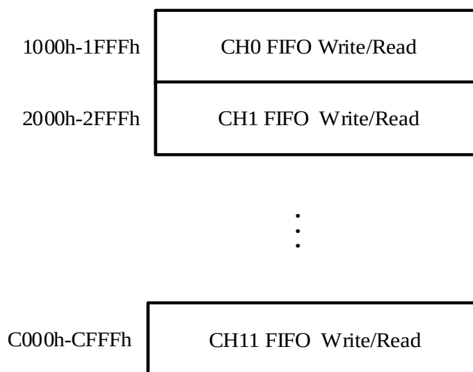
Figure 29-7. Host mode FIFO access register map
