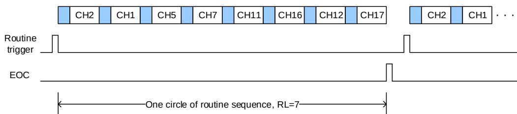
Figure 13-5. Scan operation mode, continuous operation mode disable
