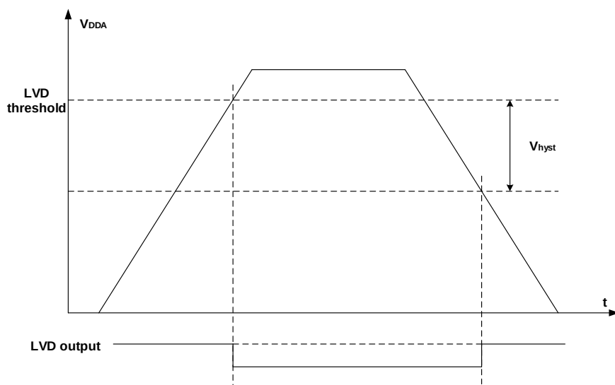
Figure 4-4. Waveform of the LVD threshold
