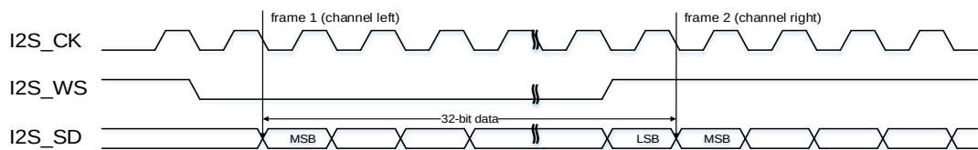
Figure 22-17. I2S Phillips standard timing diagram (DTLEN=10, CHLEN=1, CKPL=0)
