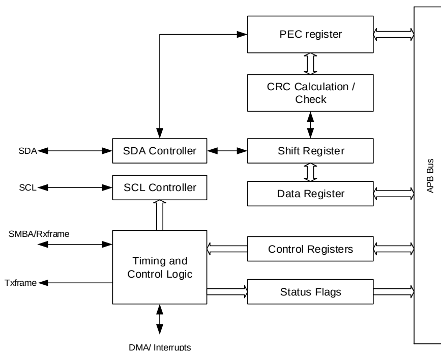
Figure 21-1. I2C module block diagram
