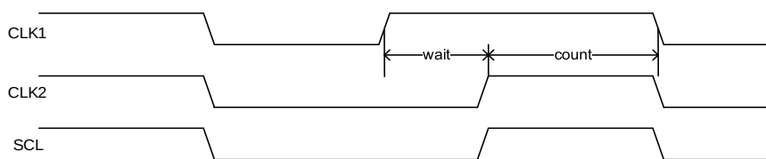
Figure 21-4. Clock synchronization
