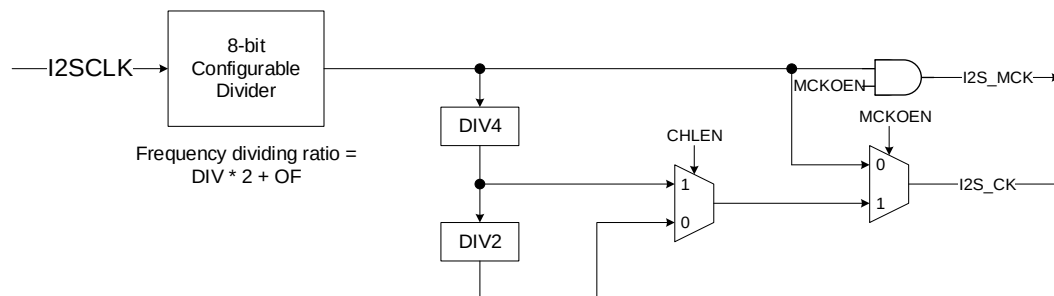
Figure 22-51. Block diagram of I2S clock generator
