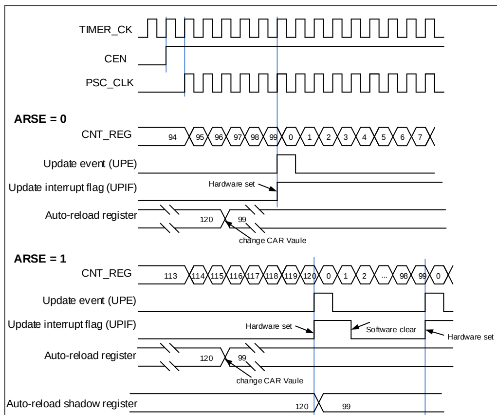
Figure 18-71. Timing chart of up counting mode, change TIMERx_CAR ongoing
