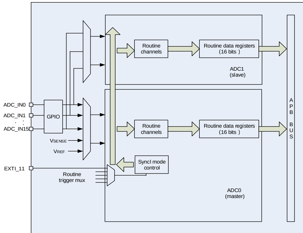
Figure 13-12. ADC sync block diagram
