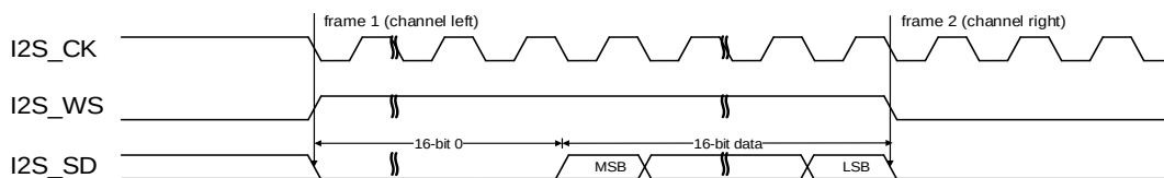
Figure 22-34. LSB justified standard timing diagram (DTLEN=00, CHLEN=1, CKPL=1)
