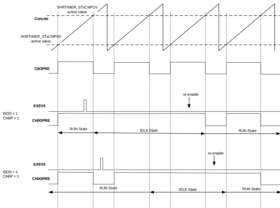
Figure 19-33. ISO0 = 1 and CHOP = 1 in delayed IDLE
