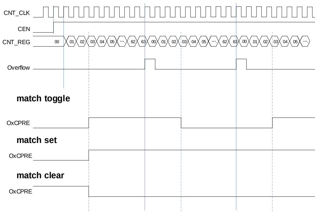
Figure 18-53. Output-compare under three modes
