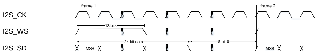
Figure 22-47. PCM standard long frame synchronization mode timing diagram (DTLEN=01, CHLEN=1, CKPL=0)
