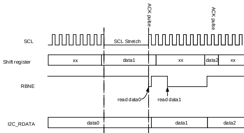
Figure 21-25. Data reception
