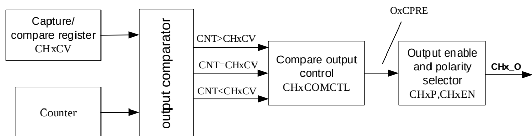
Figure 18-39. Channel output compare principle (x=0,1,2,3)
