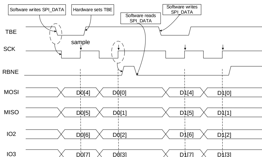
Figure 22-13. Timing diagram of read operation in Quad-SPI mode
