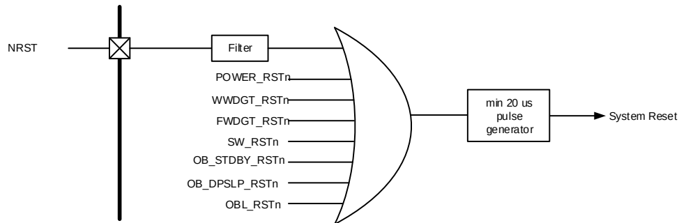
Figure 5-5. The system reset circuit
