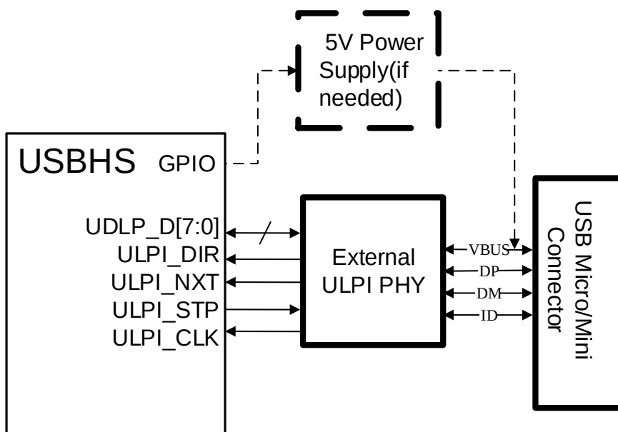
Figure 29-4. Connection using external ULPI PHY
