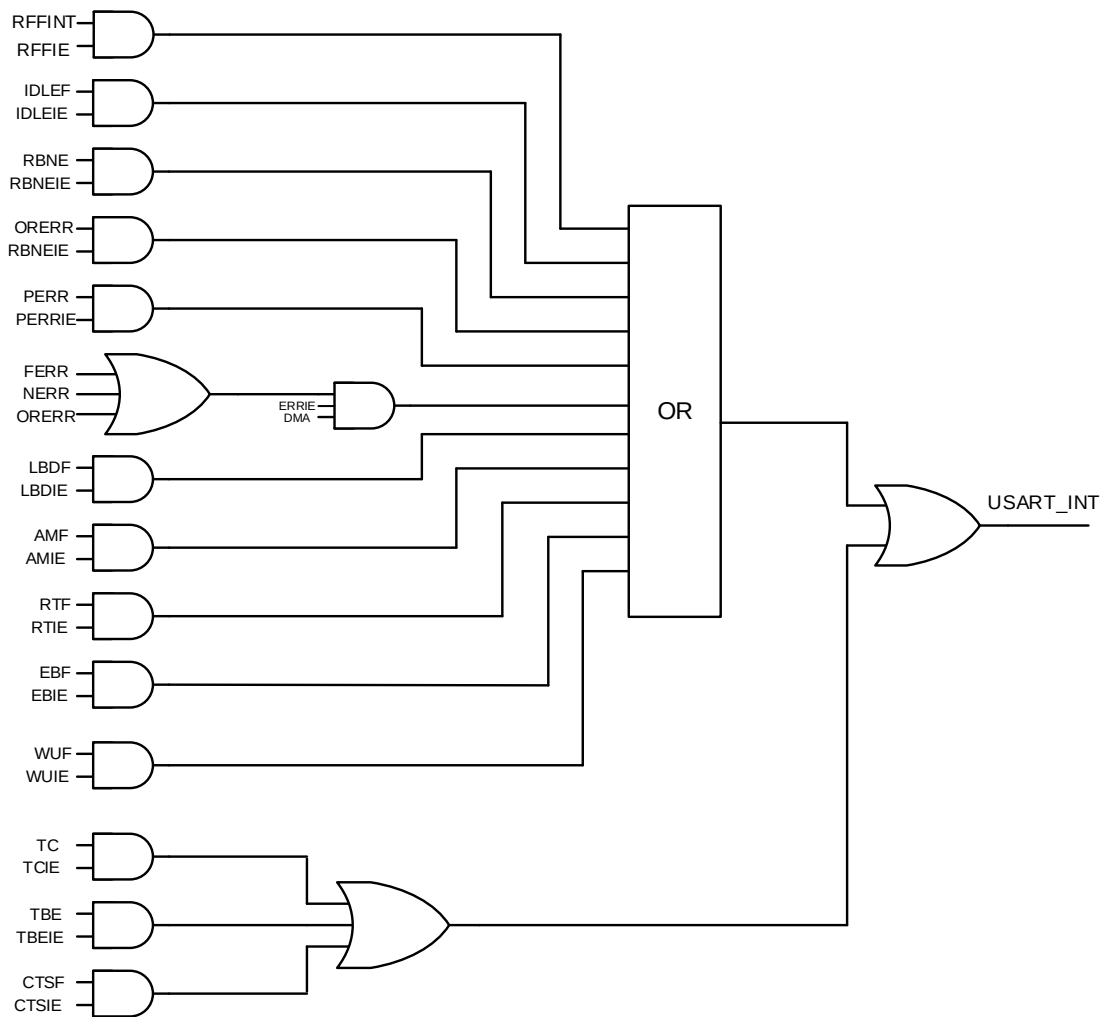
Figure 20-31. USART interrupt mapping diagram
