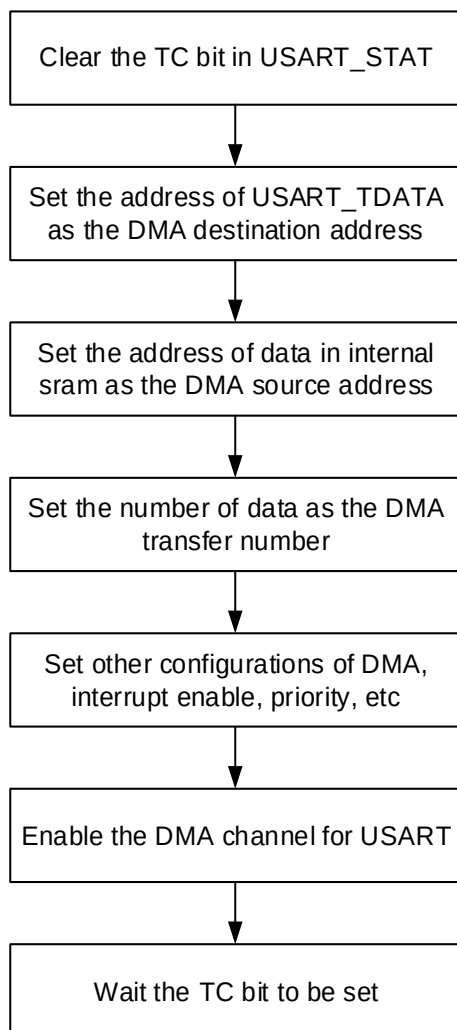
Figure 20-21. Configuration step when using DMA for USART transmission
