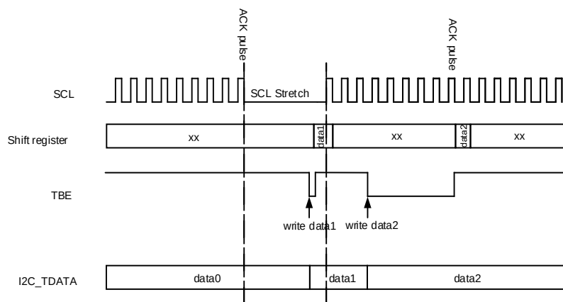
Figure 21-24. Data transmission
