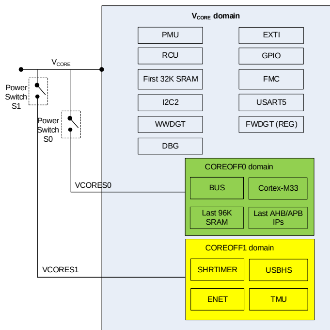
Figure 4-2. V CORE domain supply overview
