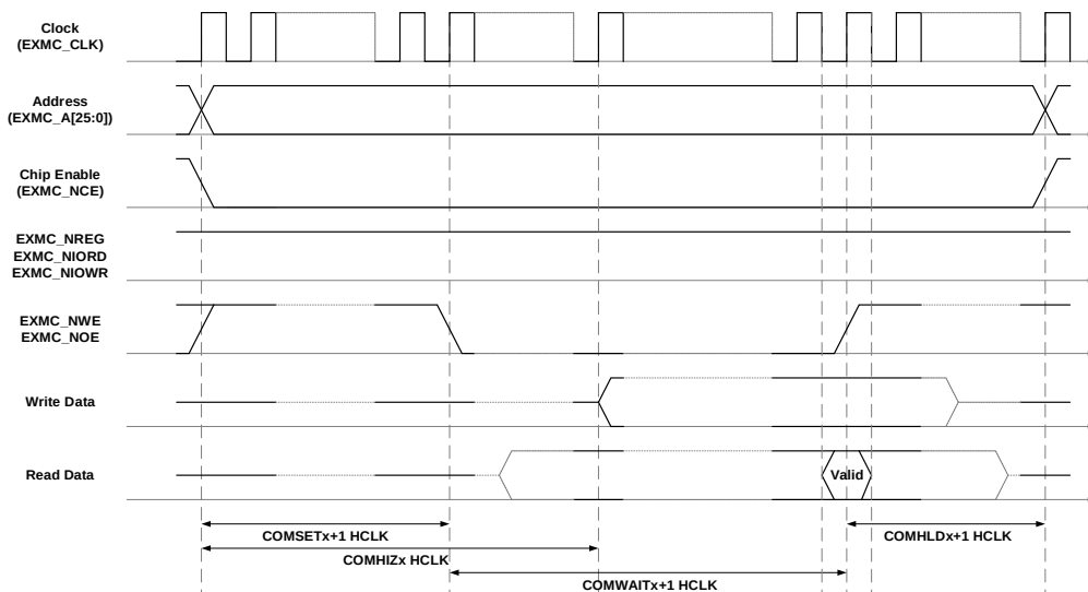
Figure 25-23. Access timing of common memory space of PC Card Controller
