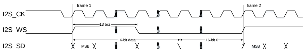
Figure 22-50. PCM standard long frame synchronization mode timing diagram (DTLEN=00, CHLEN=1, CKPL=1)
