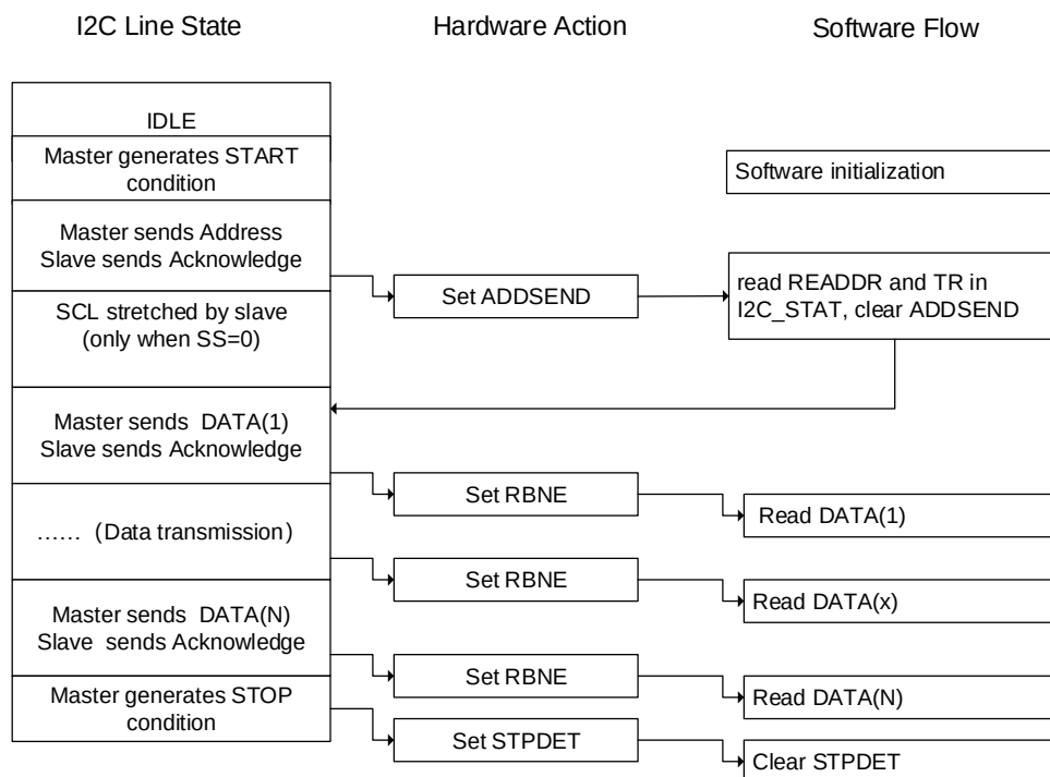
Figure 21-29. Programming model for slave receiving
