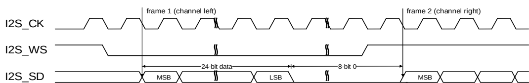
Figure 22-19. I2S Phillips standard timing diagram (DTLEN=01, CHLEN=1, CKPL=0)
