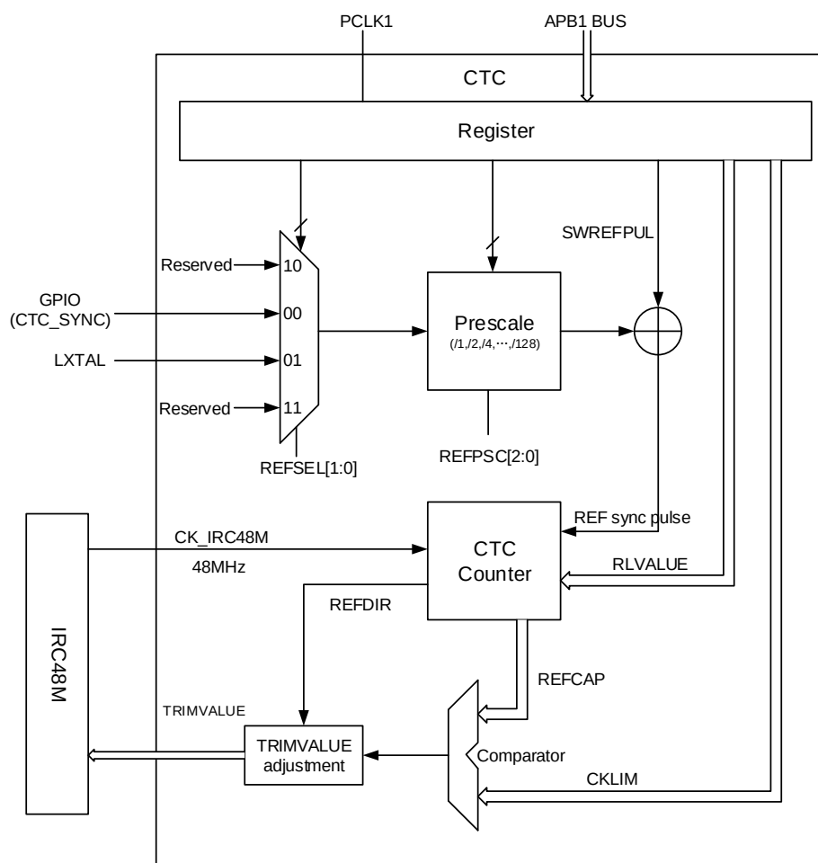
Figure 6-1. CTC overview
