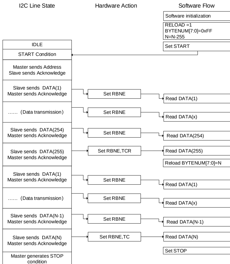
Figure 21-34. Programming model for master receiving (N>255)
