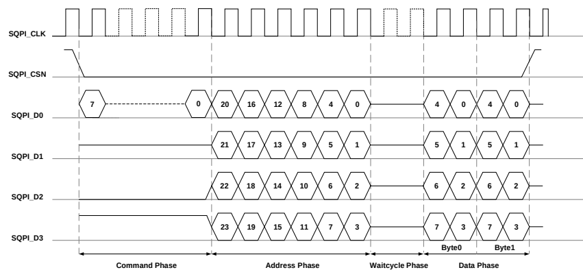
Figure 23-7. SQPI SQQ Mode Timing (SQPI)
