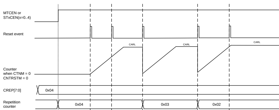
Figure 19-8. Repetition counter behavior in single pulse mode with CNTRSTM = 1
