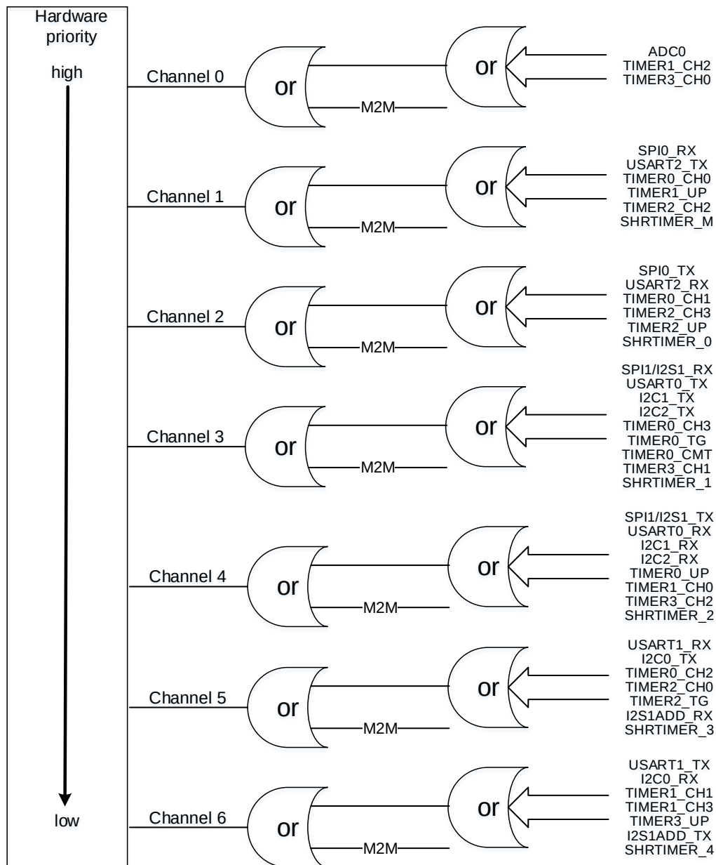
Figure 11-4. DMA0 request mapping
