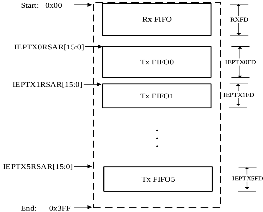
Figure 29-8. Device mode FIFO space in SRAM
