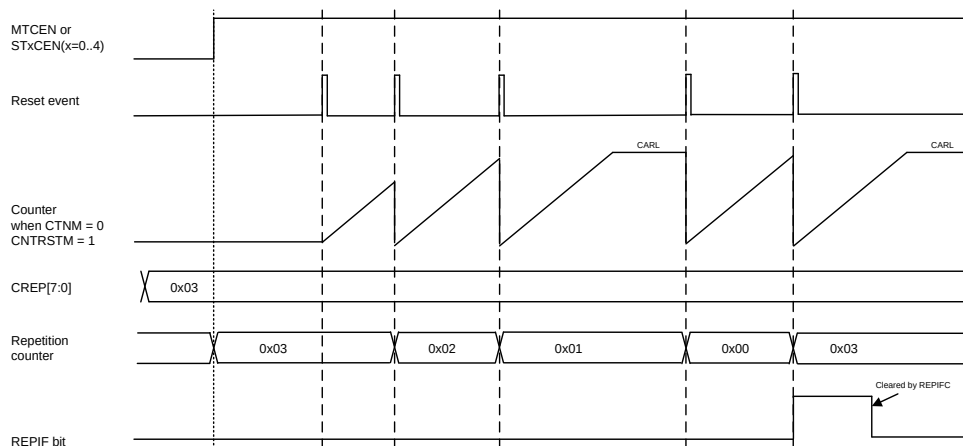
Figure 19-8. Repetition counter behavior in single pulse mode with CNTRSTM = 1
