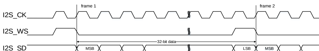
Figure 22-37. PCM standard short frame synchronization mode timing diagram (DTLEN=10, CHLEN=1, CKPL=0)
