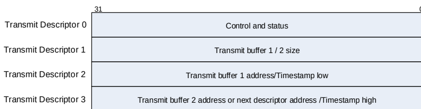
Figure 27-7. Transmit descriptor in normal mode
