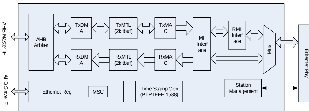
Figure 27-1. ENET module block diagram
