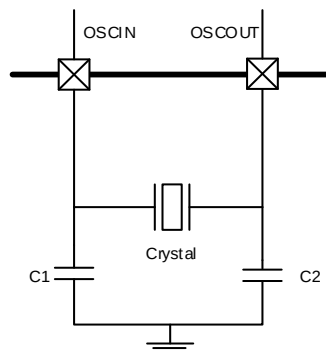
Figure 5-3. HXTAL clock source
