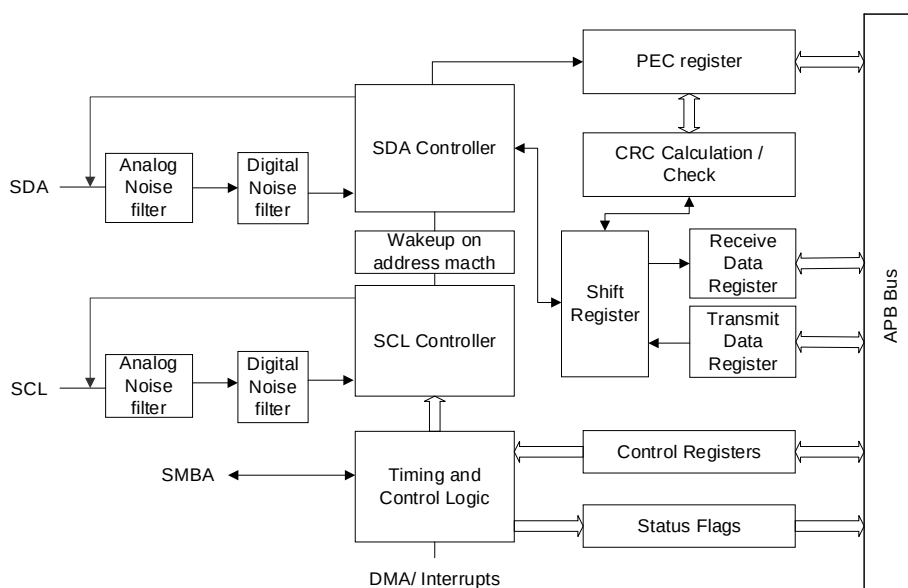
Figure 21-14. I2C module block diagram
