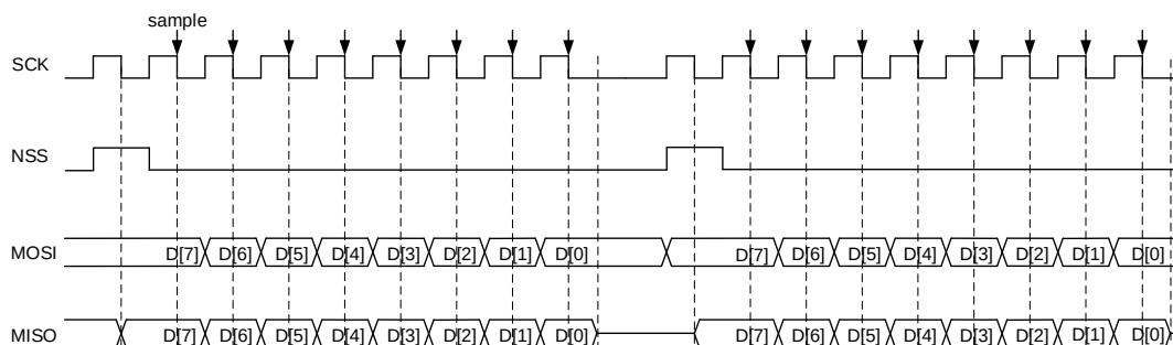
Figure 22-8. Timing diagram of TI master mode with discontinuous transfer
