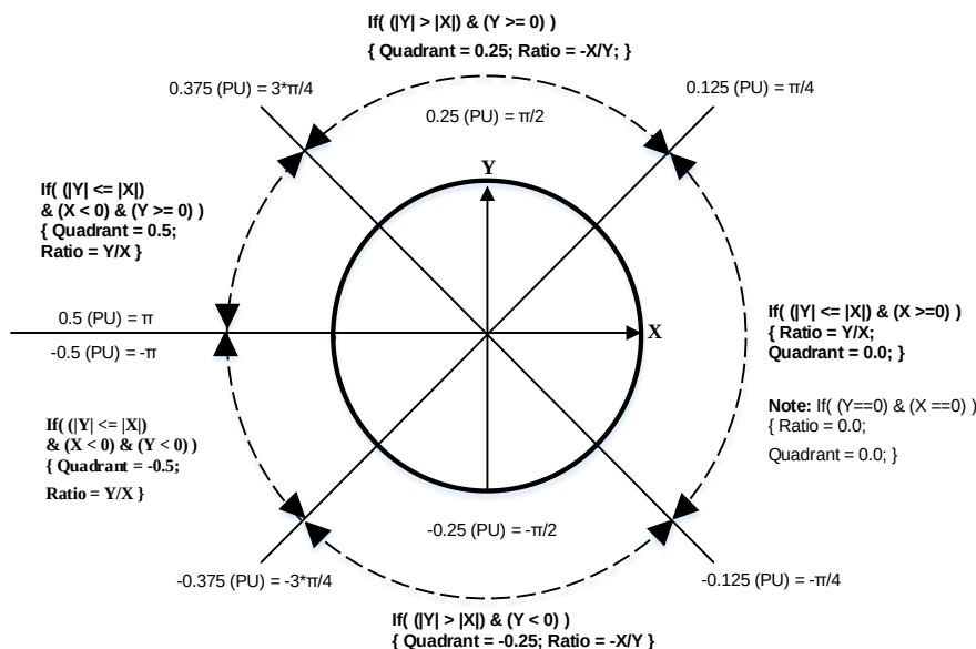
Figure 10-2. Calculation of R1 (Quadrant) and R0 (Ratio) Based on Y and X Values
