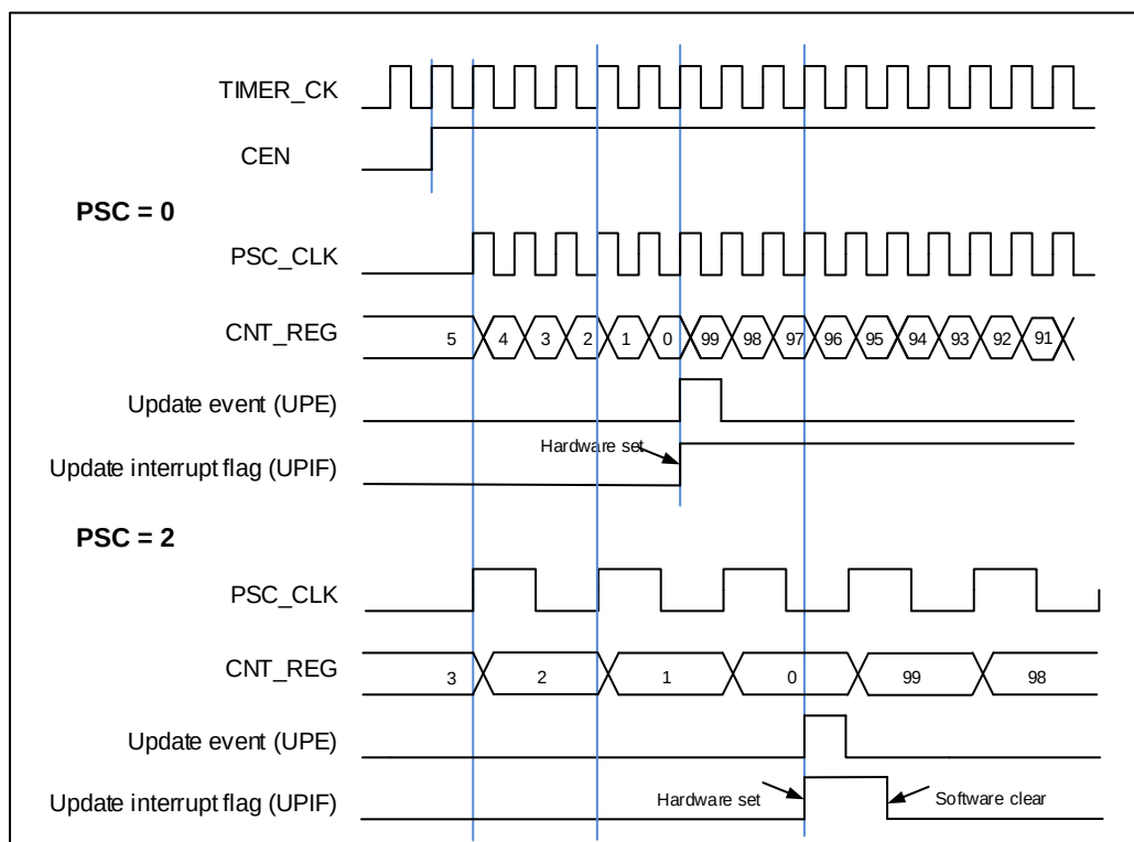
Figure 18-6. Timing chart of down counting mode, \text{PSC}=0/2
