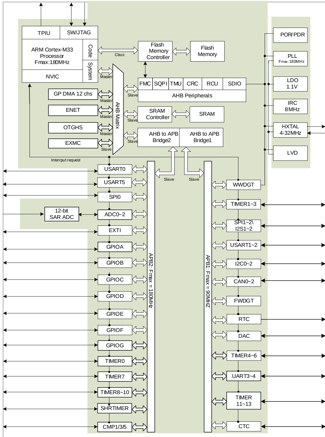
Figure 1-2. GD32E50x system architecture
