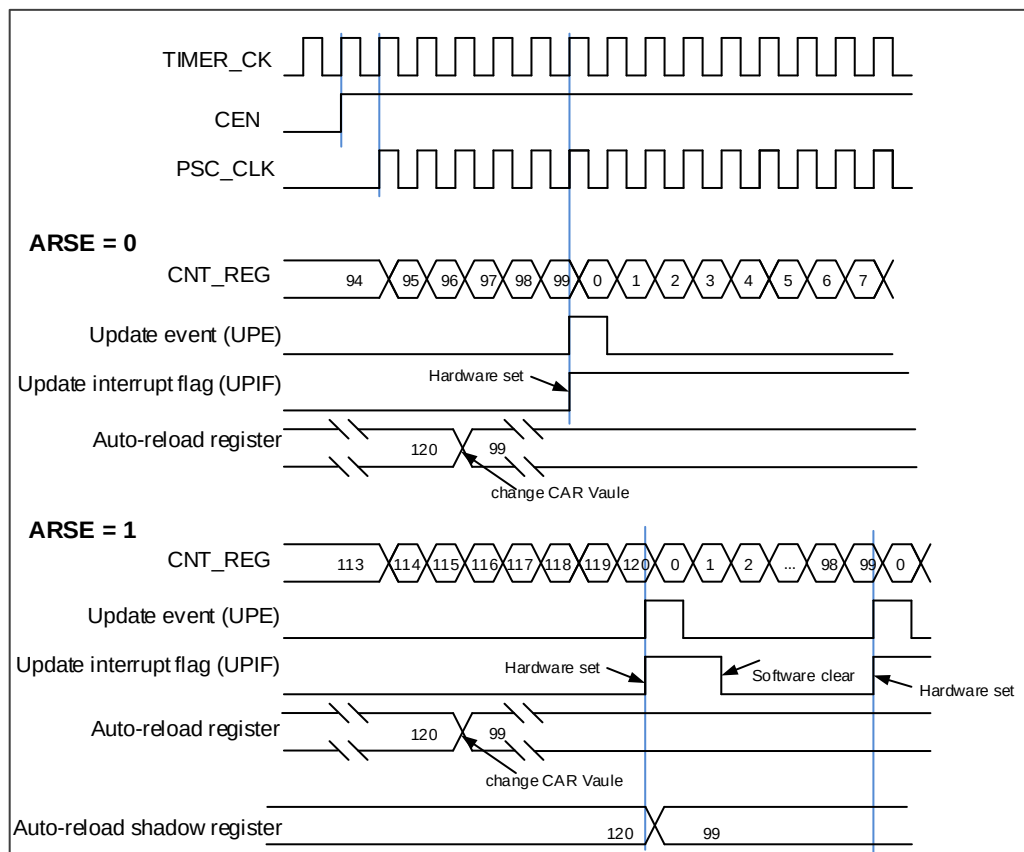
Figure 18-34. Timing chart of up counting mode, change TIMEx_CAR ongoing
