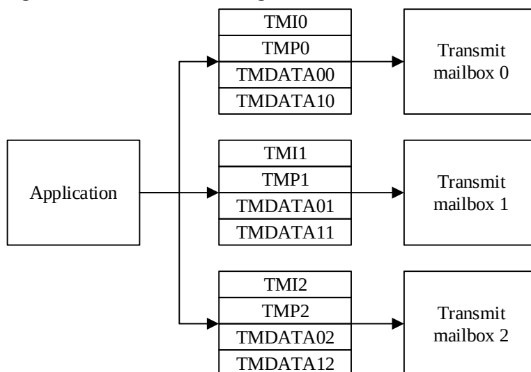
Figure 26-2. Transmission register
