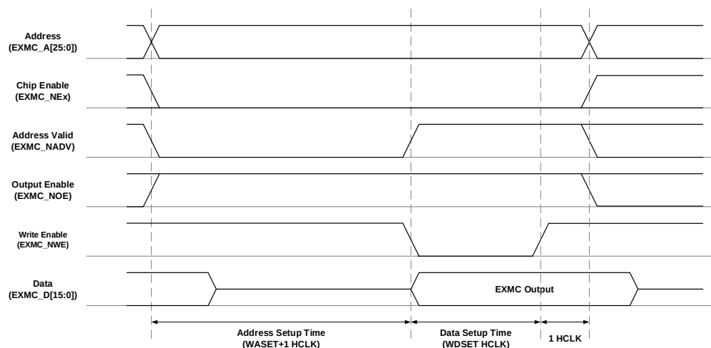
Figure 25-14. Mode C write access
