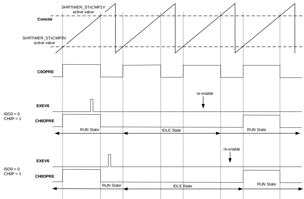
Figure 19-32. ISO0 = 0 and CHOP = 1 in delayed IDLE
