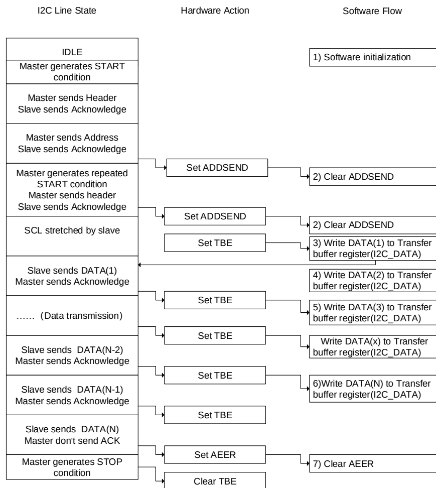
Figure 21-9. Programming model for slave transmitting (10-bit address mode)
