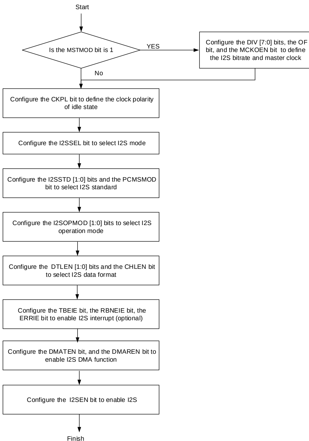
Figure 22-52. I2S initialization sequence
