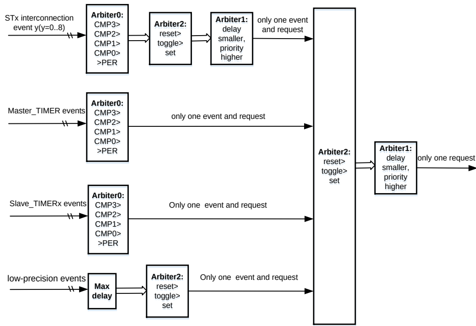
Figure 19-19. Arbitration mechanism during each t SHRTMER_CK period
