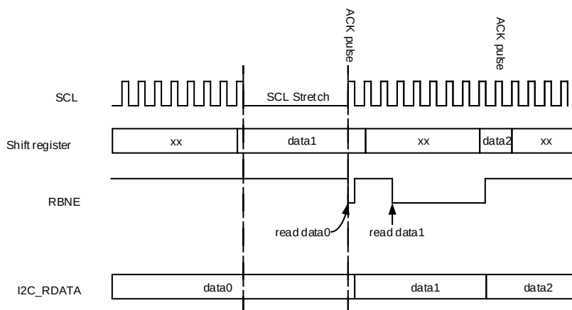
Figure 21-25. Data reception
