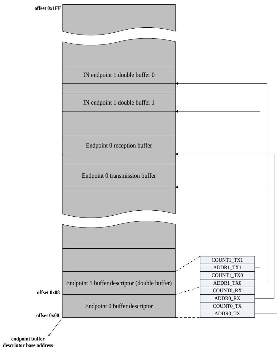
Figure 28-2. An example with buffer descriptor table usage (USBD_BADDR = 0)
