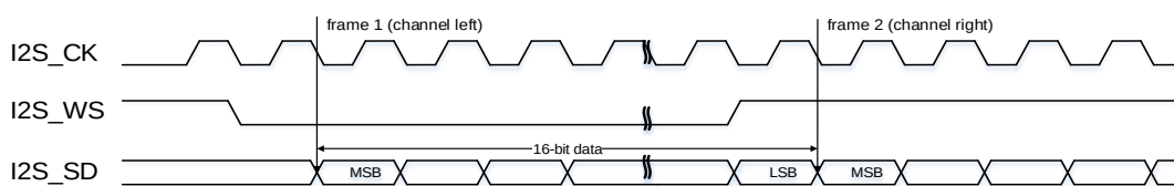
Figure 22-15. I2S Philips standard timing diagram (DTLEN=00, CHLEN=0, CKPL=0)
