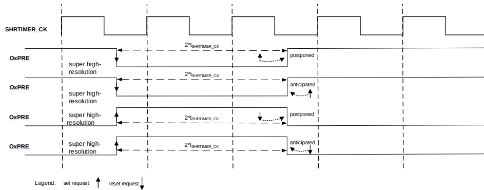
Figure 19-22. A pulse of 2 t_{SHRTMER\_CK} period
