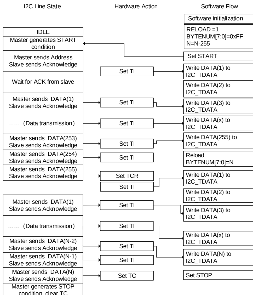
Figure 21-32. Programming model for master transmitting (N>255)
