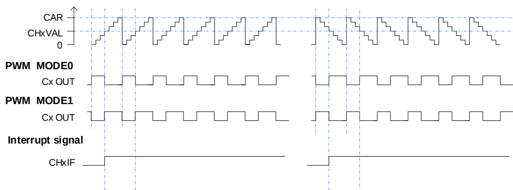
Figure 18-17. Timing chart of CAPWM
