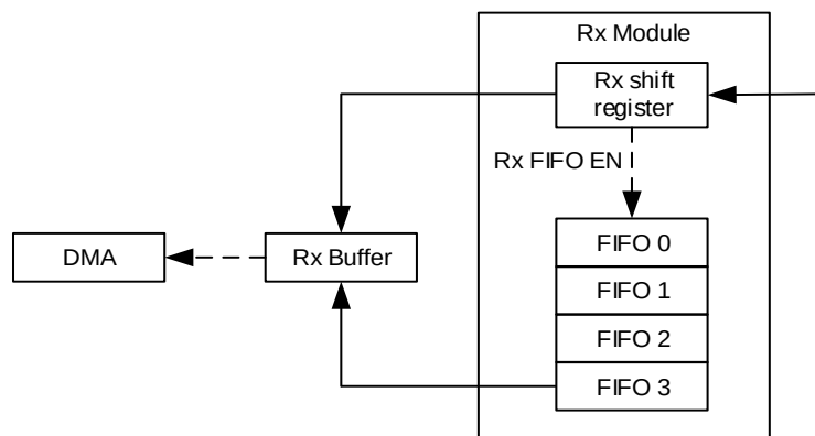
Figure 20-30. USART receive FIFO structure
