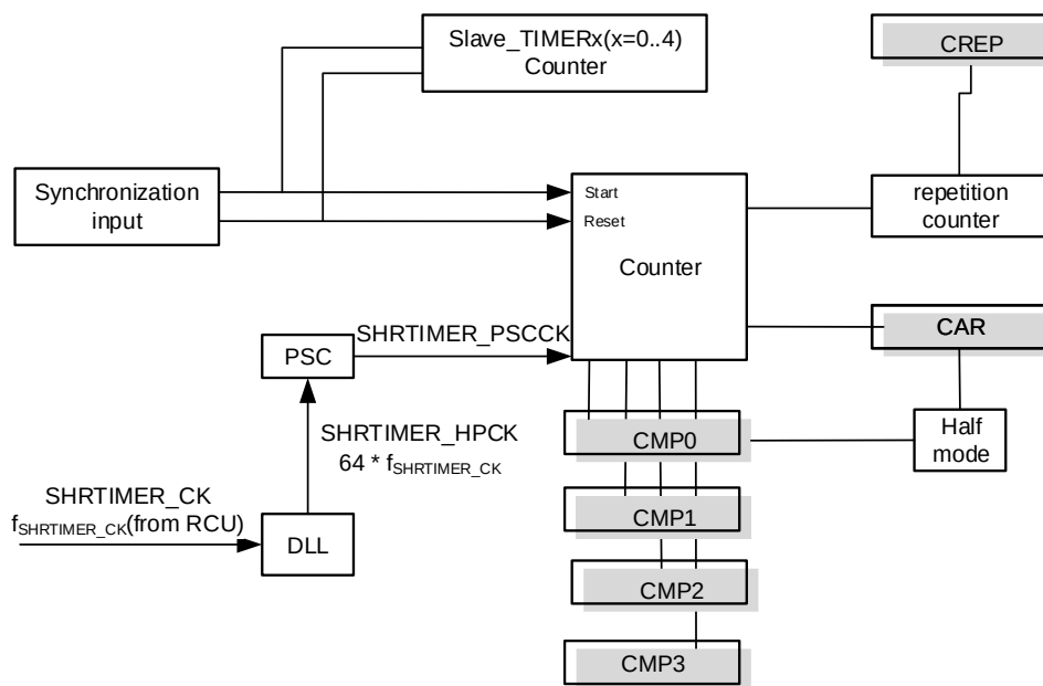
Figure 19-2. Master_TIMER diagram
