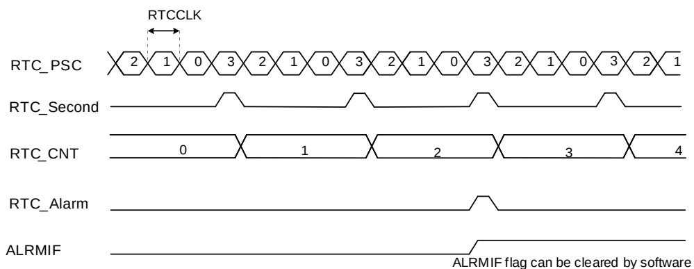
Figure 17-2. RTC second and alarm waveform example (RTC_PSC = 3, RTC_ALRM = 2)
