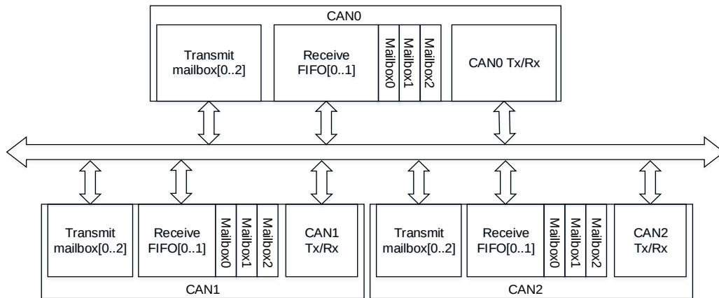
Figure 26-1. CAN module block diagram
