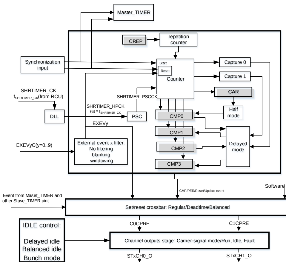
Figure 19-10. Slave_TIMERx diagram
