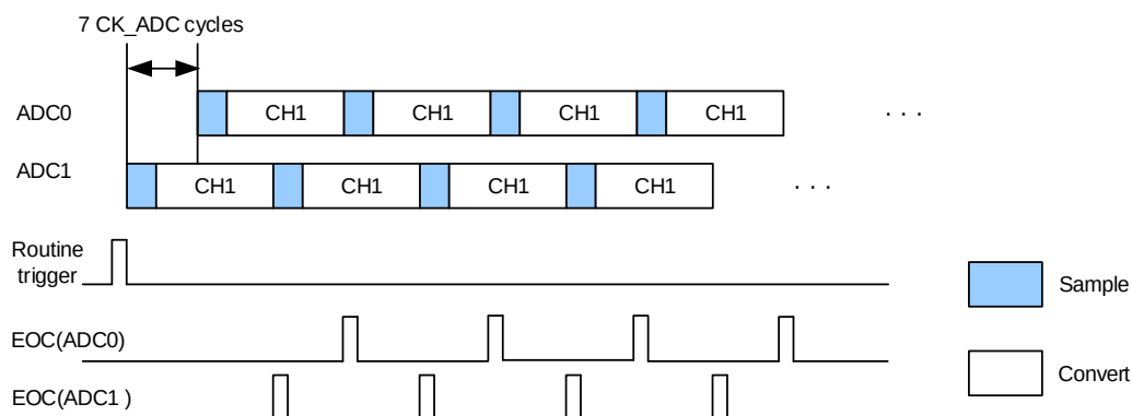
Figure 13-14. Routine follow-up fast mode on routine sequence (the CTN bit of the ADCs are set)
