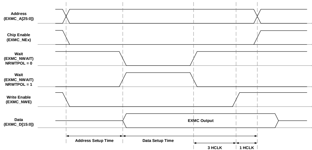
Figure 25-20. Write access timing diagram under async-wait signal assertion
