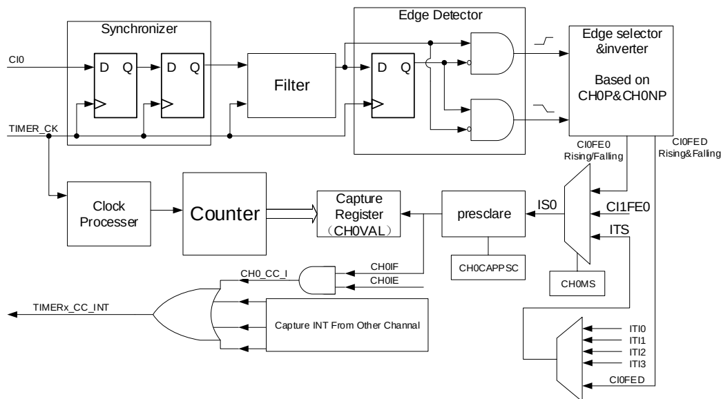
Figure 18-12. Channel Input capture principle
