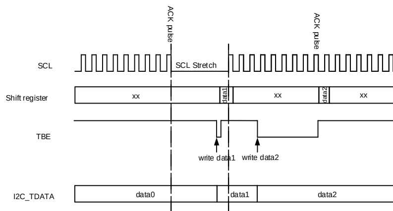
Figure 21-24. Data transmission
