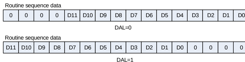
Figure 13-8. 12-bit data storage mode
