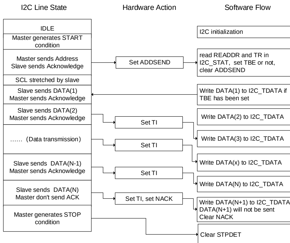
Figure 21-27. Programming model for slave transmitting when SS=0
