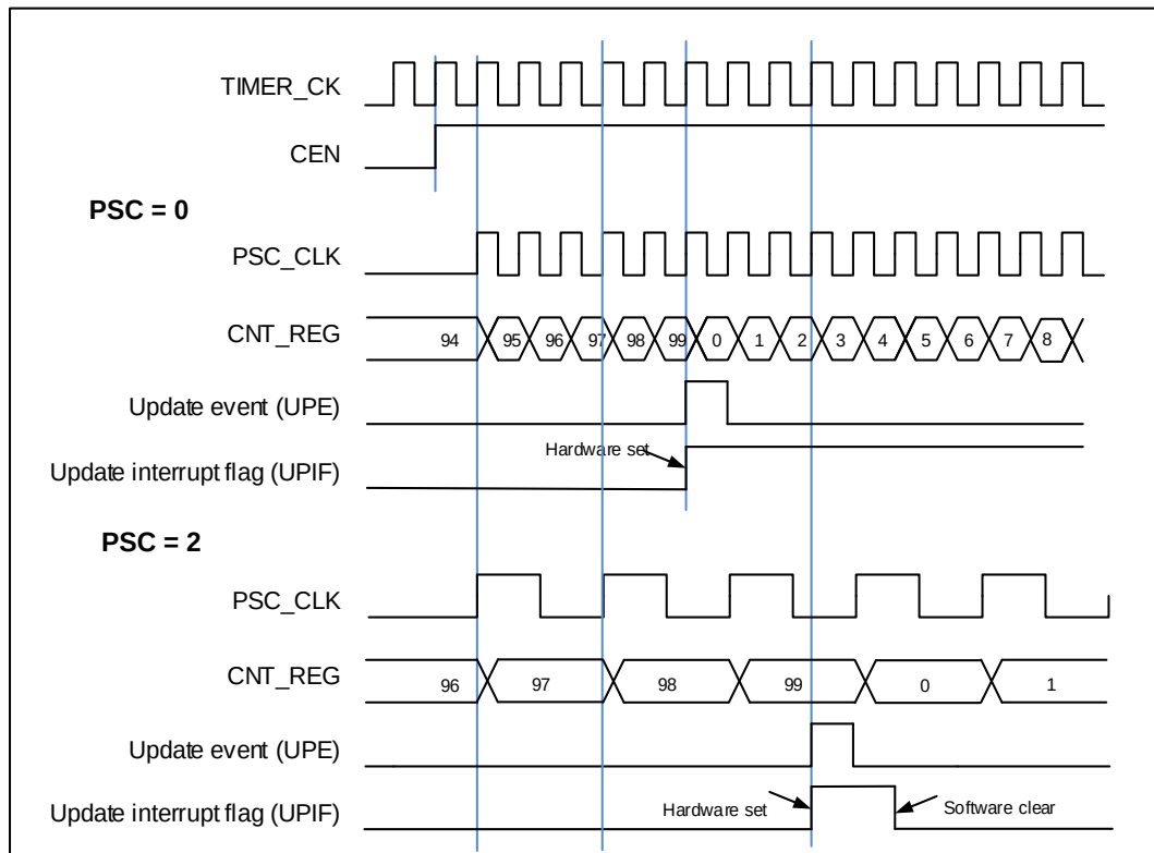
Figure 18-70. Timing chart of up counting mode, PSC=0/2
