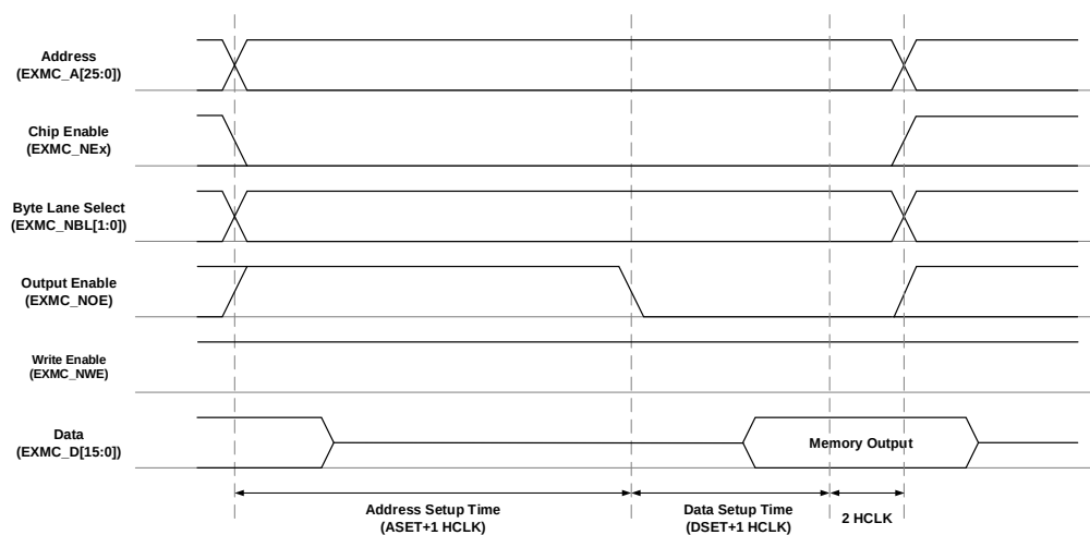
Figure 25-8. Mode A read access
