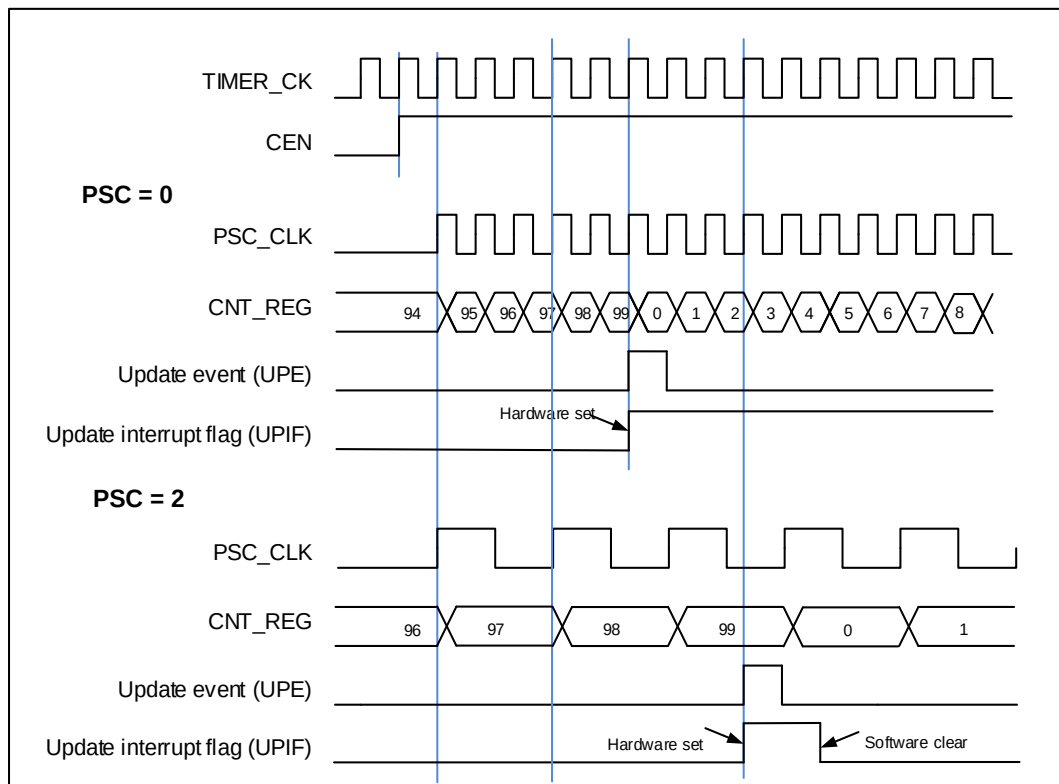
Figure 18-62. Timing chart of up counting mode, PSC=0/2
