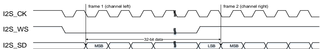
Figure 18-15. I2S Philips standard timing diagram (DTLEN=10, CHLEN=1, CKPL=1)
