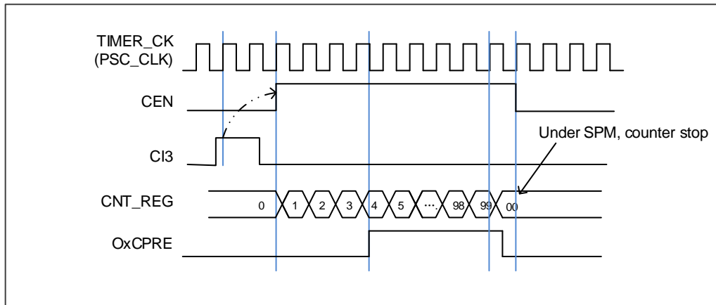
Figure 15-27. Single pulse mode, TIMERx\_CHxCV = 4 , TIMERx\_CAR=99
