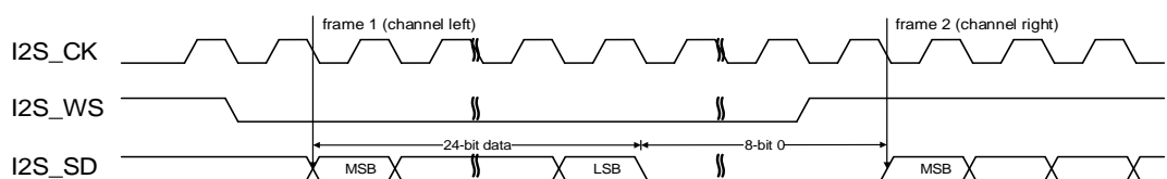
Figure 18-16. I2S Philips standard timing diagram (DTLEN=01, CHLEN=1, CKPL=0)
