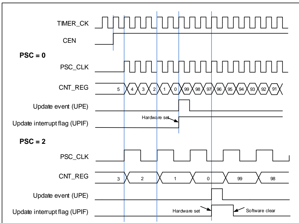
Figure 15-35. Timing chart of down counting mode, PSC=0/2
