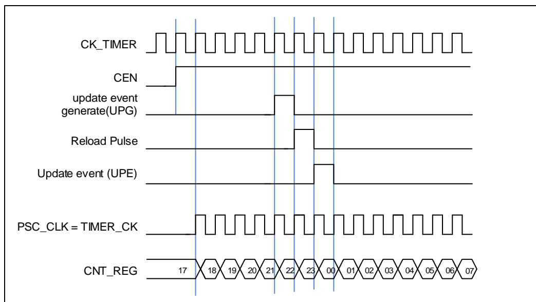
Figure 15-31. Timing chart of internal clock divided by 1
