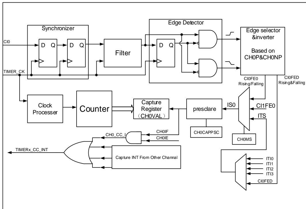
Figure 15-12. Channel input capture principle
