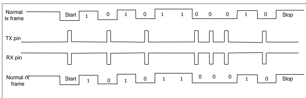
Figure 16-14. IrDA data modulation
