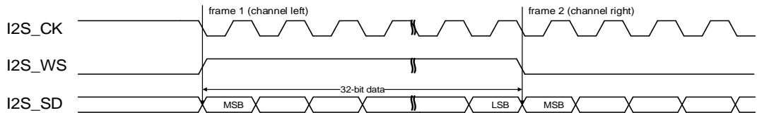
Figure 18-23. MSB justified standard timing diagram (DTLEN=10, CHLEN=1, CKPL=1)
