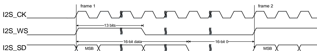
Figure 18-46. PCM standard long frame synchronization mode timing diagram (DTLEN=00, CHLEN=1, CKPL=0)
