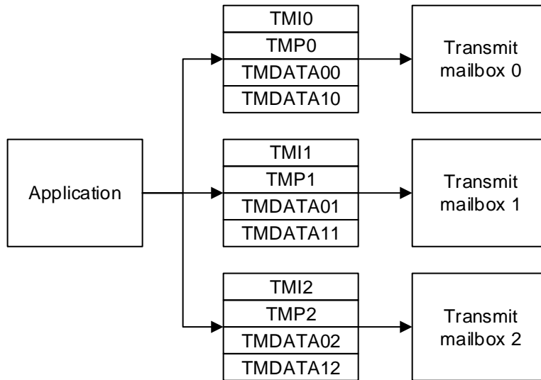
Figure 20-2. Transmission register
