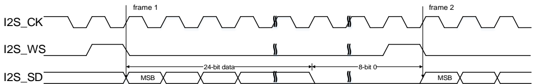
Figure 18-37. PCM standard short frame synchronization mode timing diagram (DTLEN=01, CHLEN=1, CKPL=1)
