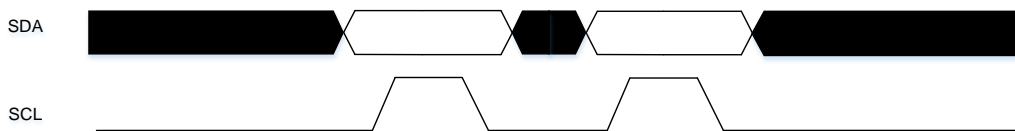
Figure 17-2. Data validation
