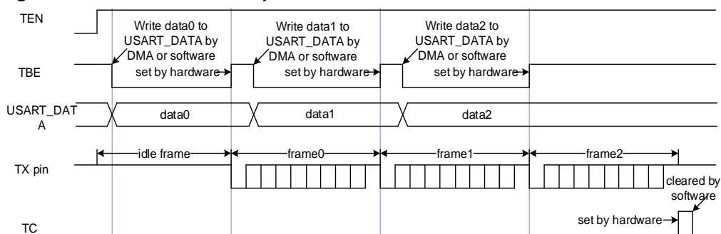
Figure 16-3. USART transmit procedure
