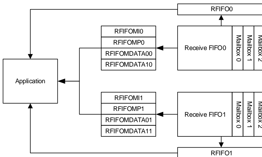
Figure 20-4. Reception register
