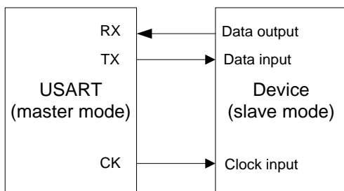
Figure 16-11. Example of USART in synchronous mode
