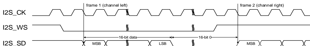
Figure 18-18. I2S Philips standard timing diagram (DTLEN=00, CHLEN=1, CKPL=0)
