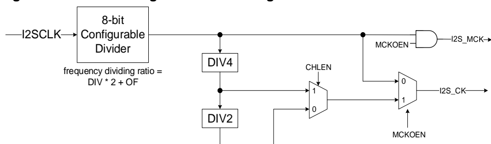
Figure 18-48. Block diagram of I2S clock generator
