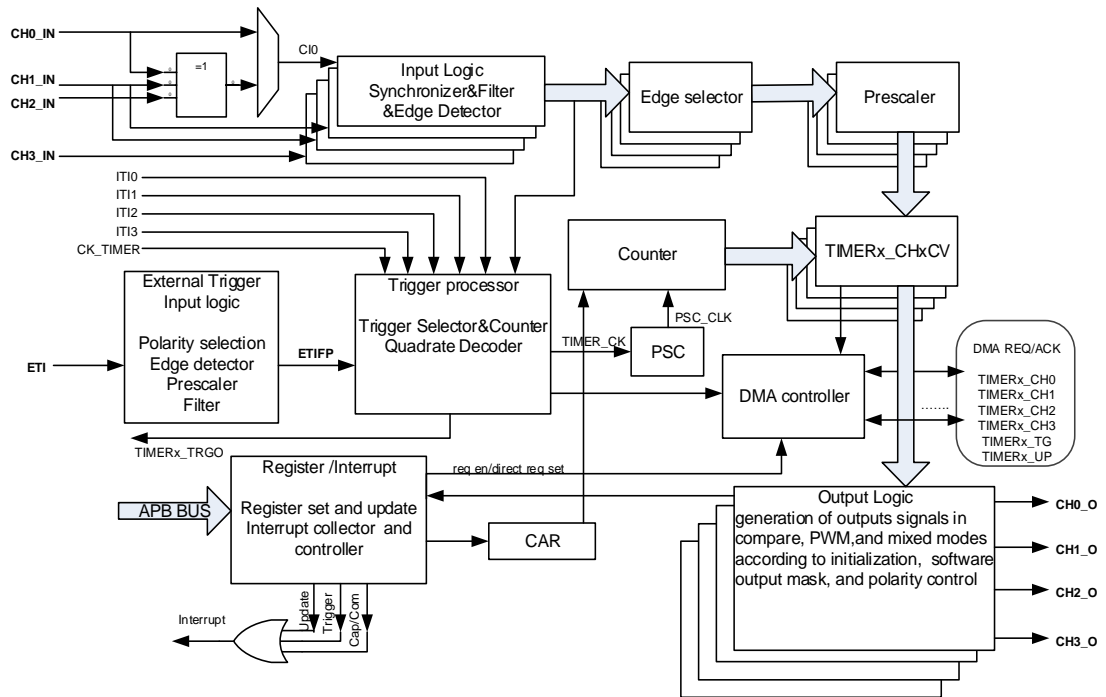
Figure 15-30. General Level 0 timer block diagram
