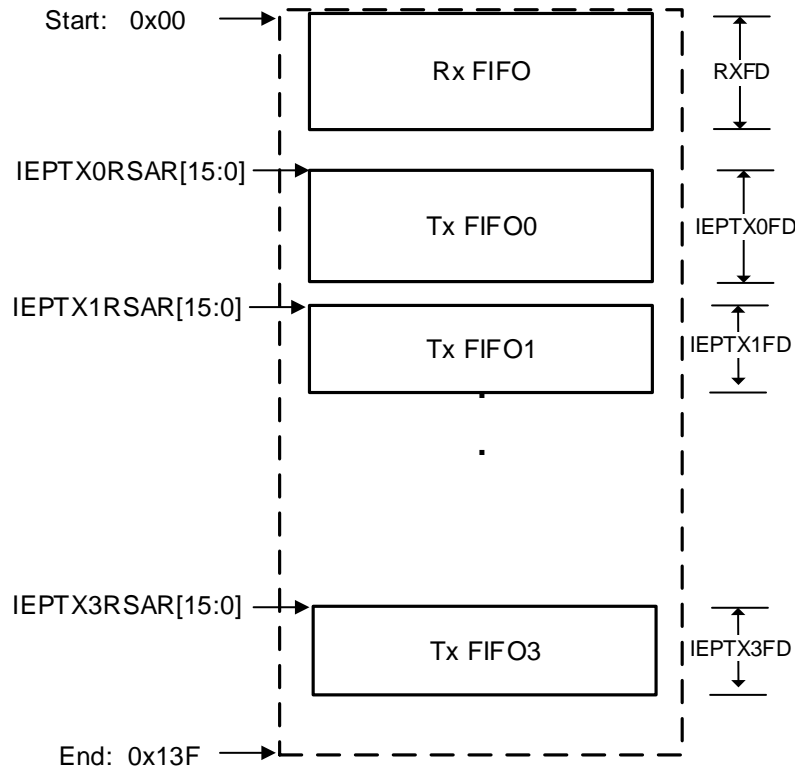
Figure 21-7. Device mode FIFO space in SRAM
