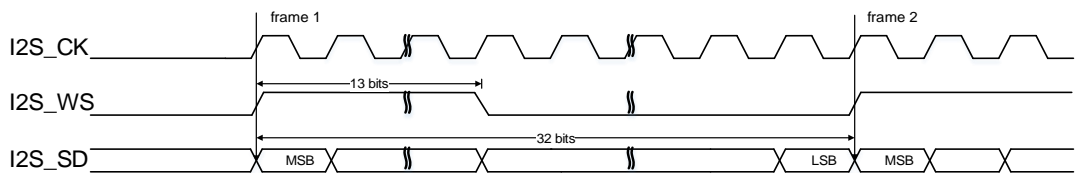
Figure 18-42. PCM standard long frame synchronization mode timing diagram (DTLEN=10, CHLEN=1, CKPL=0)
