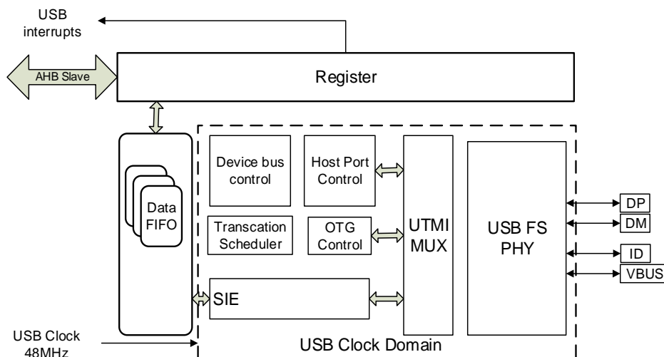
Figure 21-1. USBFS block diagram
