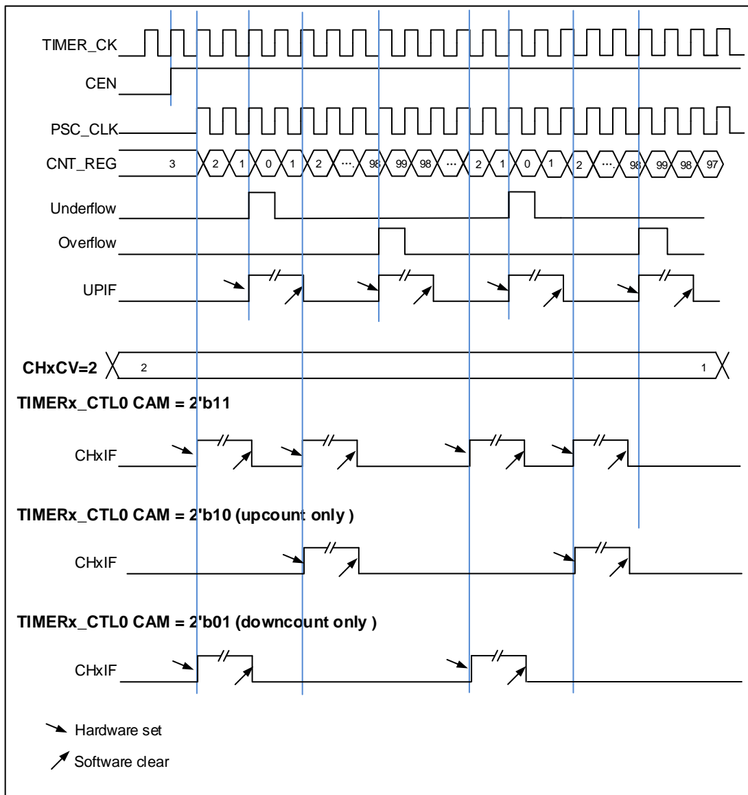
Figure 15-8. Timing chart of center-aligned counting mode
