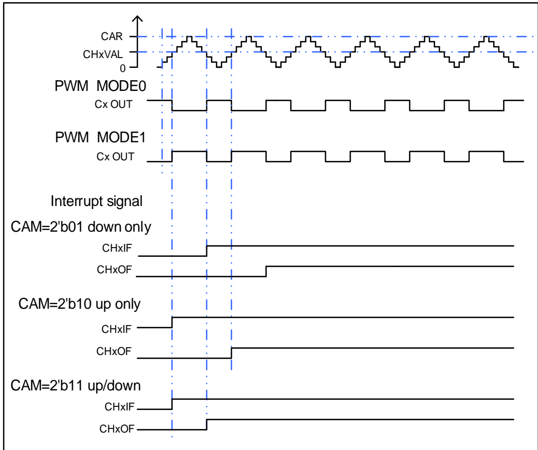
Figure 15-41. CAPWM timechart
