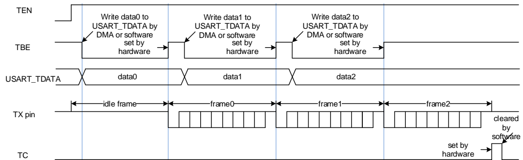
Figure 16-3.USART transmit procedure
