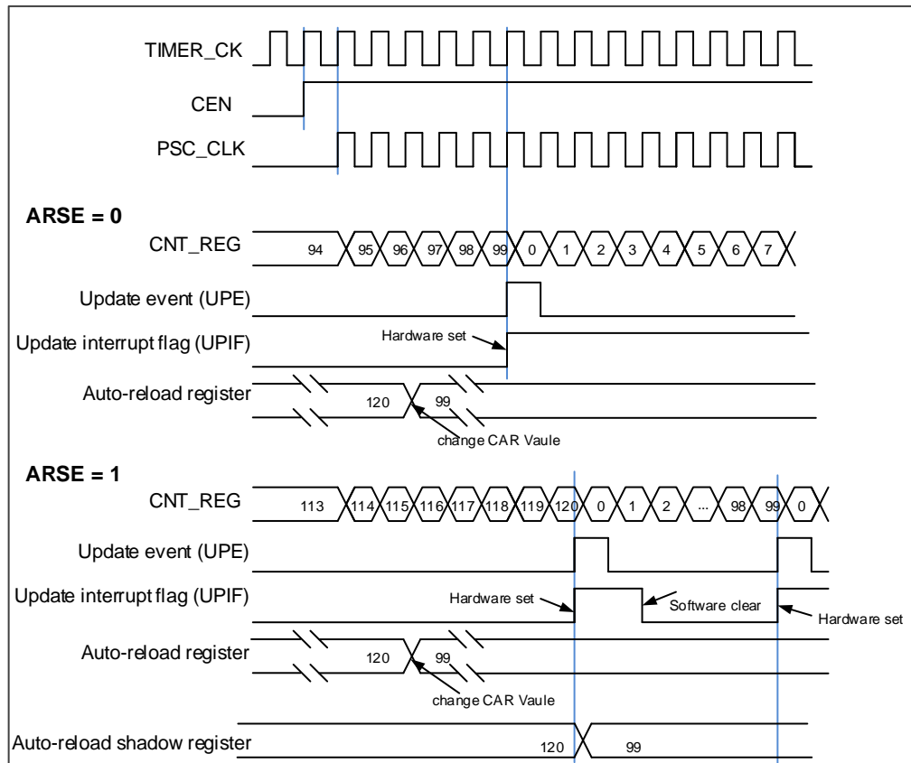
Figure 14-48. Timing chart of up counting mode, change TIMERx_CAR on the go
