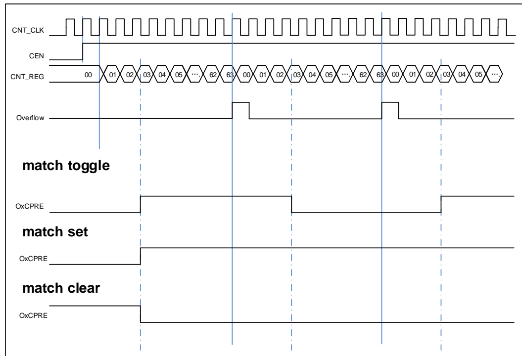
Figure 14-51. Output-compare in three modes
