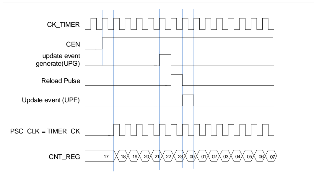
Figure 14-32. Timing chart of internal clock divided by 1
