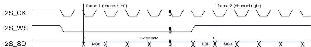
Figure 18-21. I2S Philips standard timing diagram (DTLEN=10, CHLEN=1, CKPL=1)
