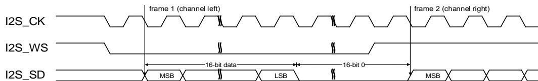
Figure 18-25. I2S Philips standard timing diagram (DTLEN=00, CHLEN=1, CKPL=1)
