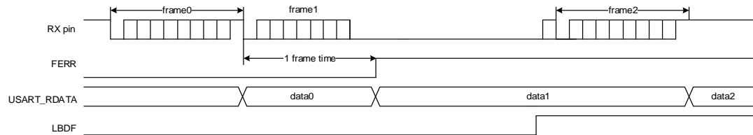
Figure 16-10. Break frame occurs during a frame
