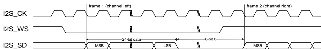
Figure 18-22. I2S Philips standard timing diagram (DTLEN=01, CHLEN=1, CKPL=0)
