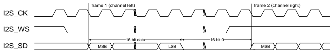
Figure 18-24. I2S Philips standard timing diagram (DTLEN=00, CHLEN=1, CKPL=0)
