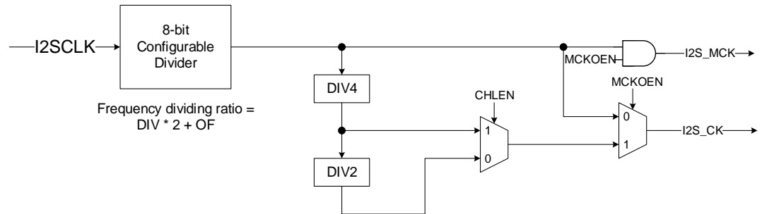
Figure 18-54. Block diagram of I2S clock generator
