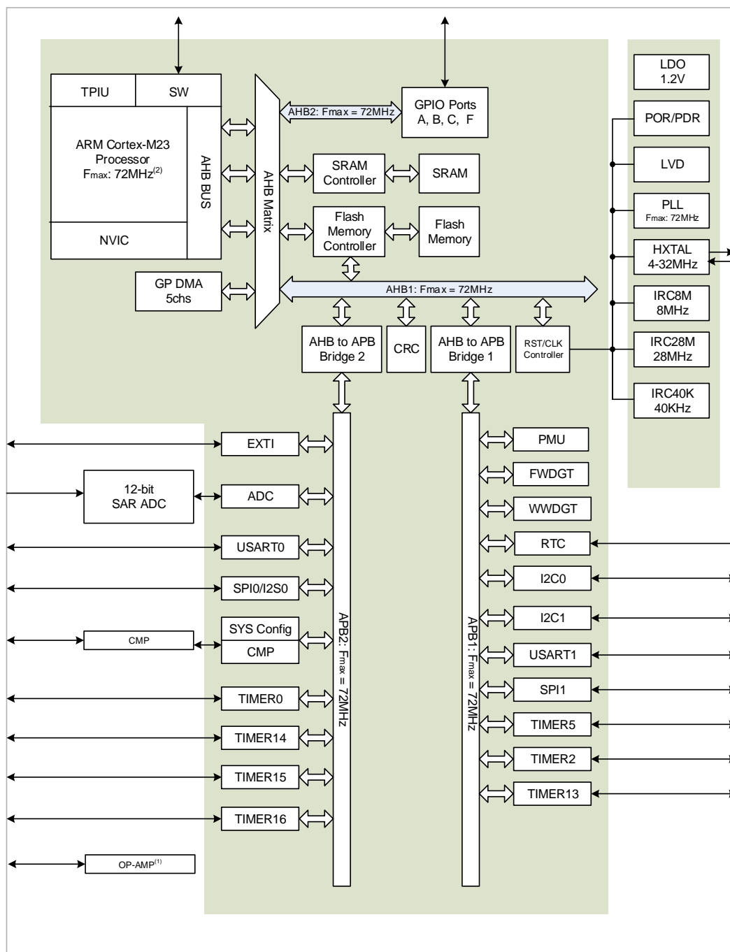
Figure 1-2. Series system architecture of GD32E23x series
