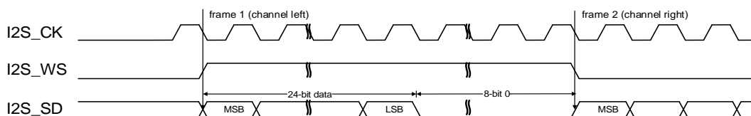
Figure 18-30. MSB justified standard timing diagram (DTLEN=01, CHLEN=1, CKPL=0)
