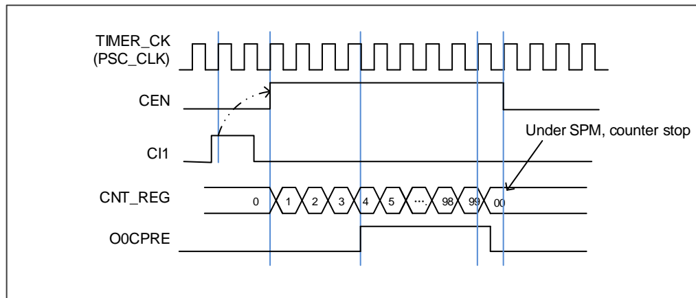
Figure 14-69. Single pulse mode TIMERx_CHxCV = 4 TIMERx_CAR=99
