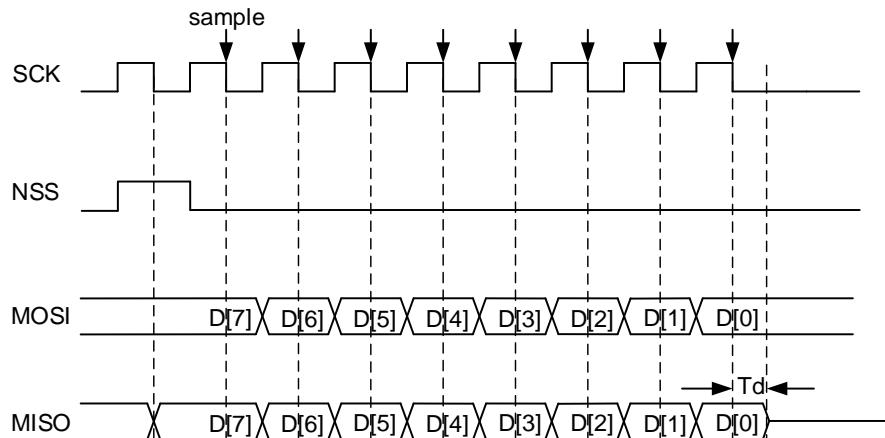
Figure 18-13. Timing diagram of TI slave mode
