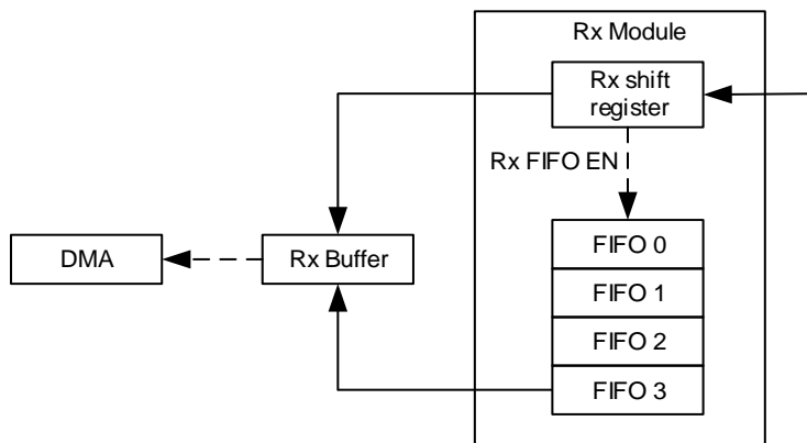
Figure 16-16. USART receive FIFO structure
