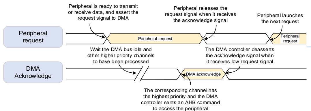
Figure 8-2. Handshake mechanism
