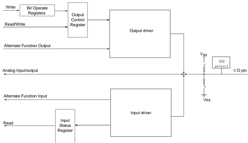
Figure 6-1. Basic structure of of a general-purpose I/O
