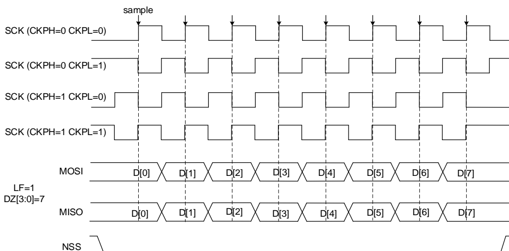
Figure 18-3. SPI1 timing diagram in normal mode
