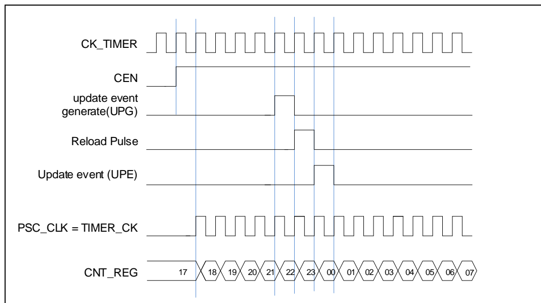
Figure 14-54. Timing chart of internal clock divided by 1
