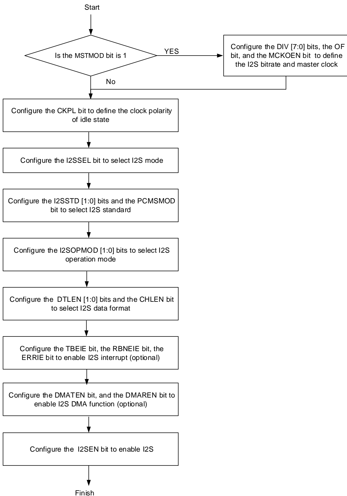
Figure 18-55. I2S initialization sequence
