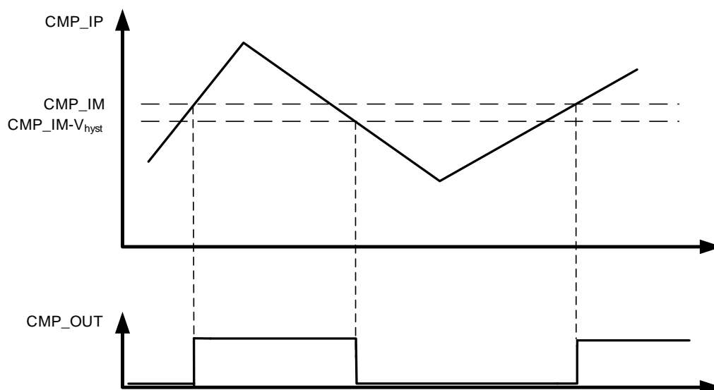
Figure 11-2. CMP hysteresis
