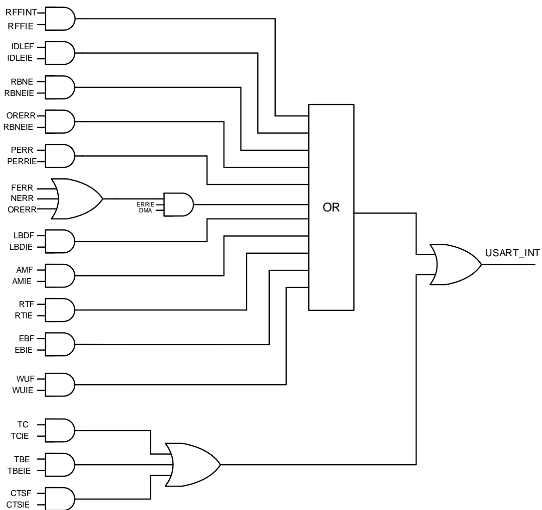
Figure 16-17. USART interrupt mapping diagram
