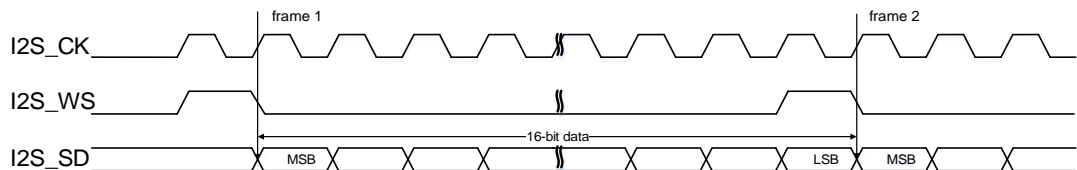
Figure 18-38. PCM standard short frame synchronization mode timing diagram (DTLEN=00, CHLEN=0, CKPL=0)
