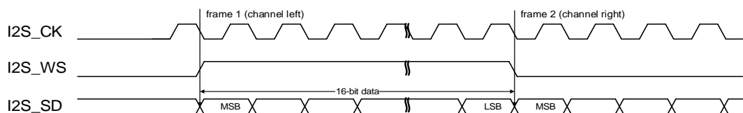
Figure 18-26. MSB justified standard timing diagram (DTLEN=00, CHLEN=0, CKPL=0)
