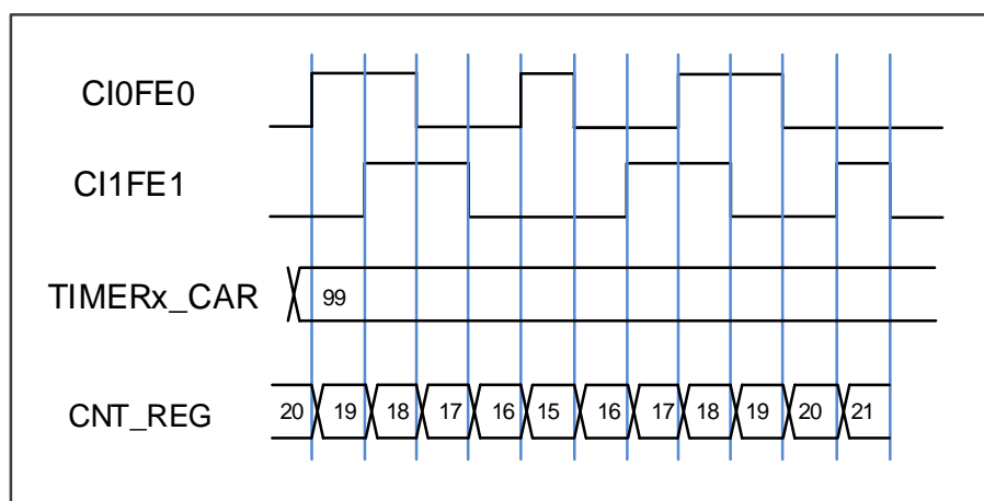
Figure 14-21. Counter behavior with CI0FE0 polarity inverted in mode 2
