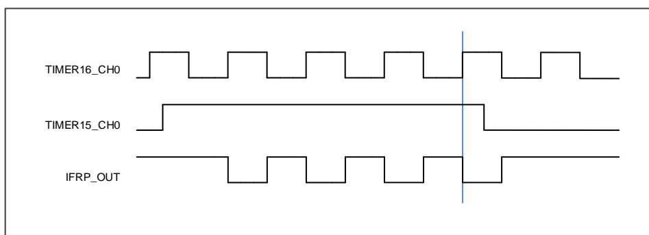
Figure 15-3. IFRP output timechart 3
