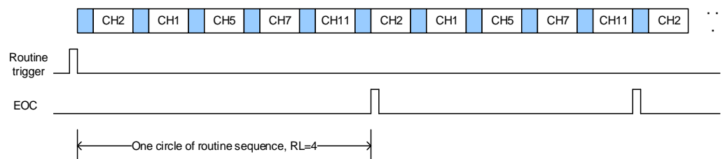
Figure 10-5. Scan operation mode, continuous enable
