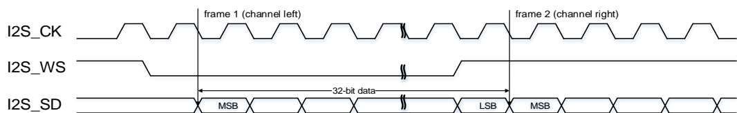
Figure 18-20. I2S Philips standard timing diagram (DTLEN=10, CHLEN=1, CKPL=0)
