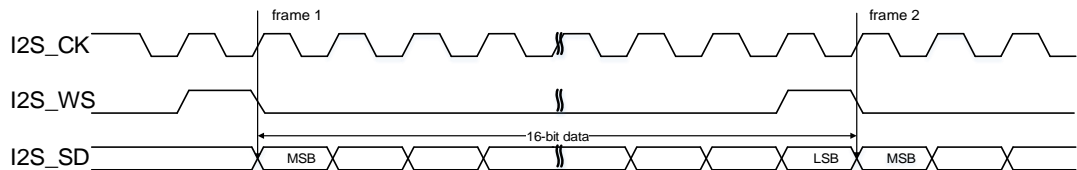
Figure 18-39. PCM standard short frame synchronization mode timing diagram (DTLEN=00, CHLEN=0, CKPL=1)
