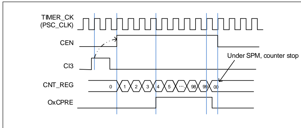
Figure 14-27. Single pulse mode TIMERx\_CHxCV=4 , TIMERx\_CAR=99
