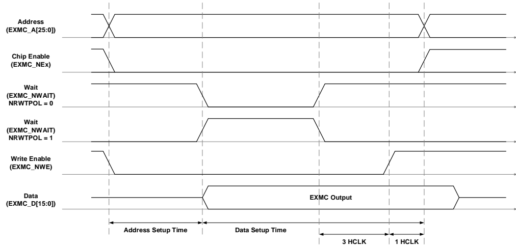
Figure 20-20. Write access timing diagram under async-wait signal assertion
