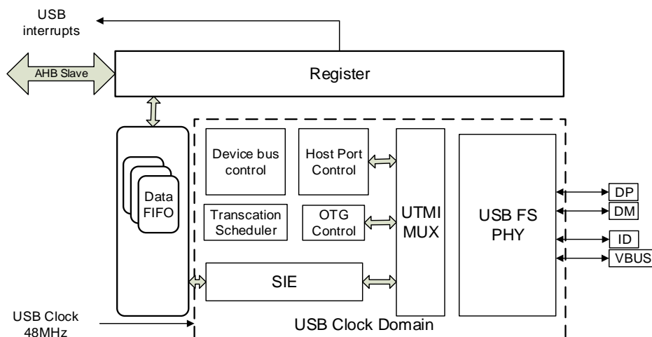
Figure 24-1. USBFS block diagram
