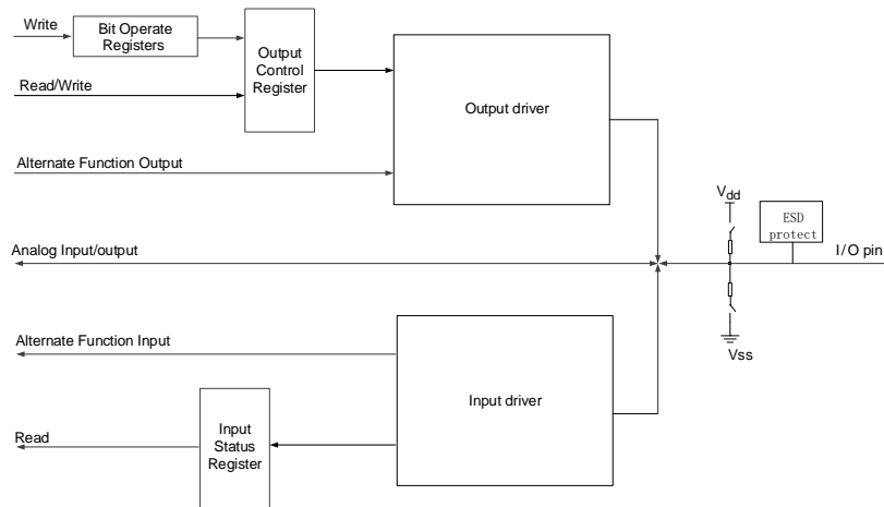
Figure 7-1. Basic structure of of a general-purpose I/O
