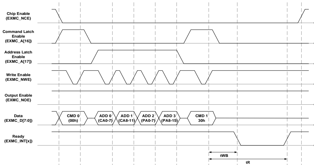
Figure 20-24. Access to none "NCE don't care" NAND Flash
