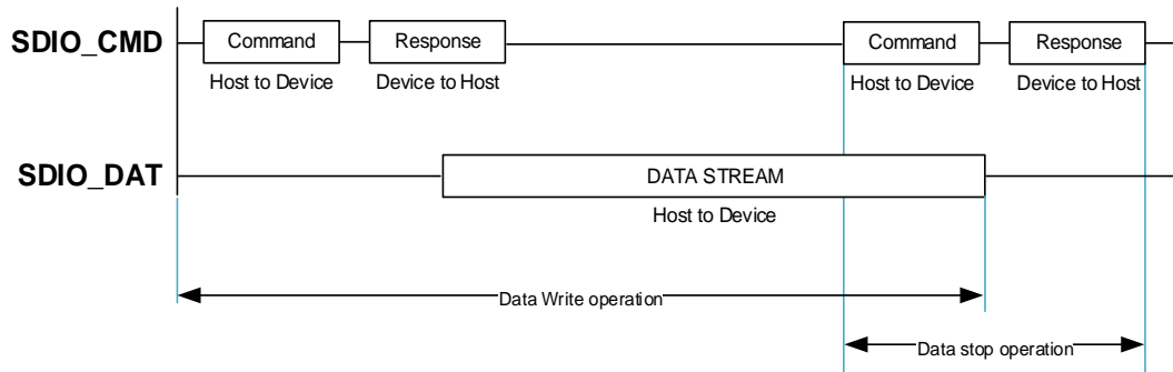
Figure 19-5. SDIO sequential write operation
