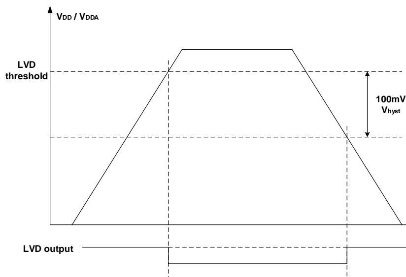
Figure 3-3. Waveform of the LVD threshold
