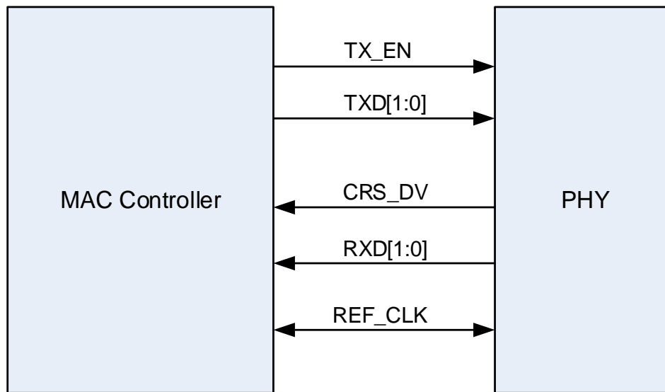
Figure 22-5. Reduced media-independent interface signals
