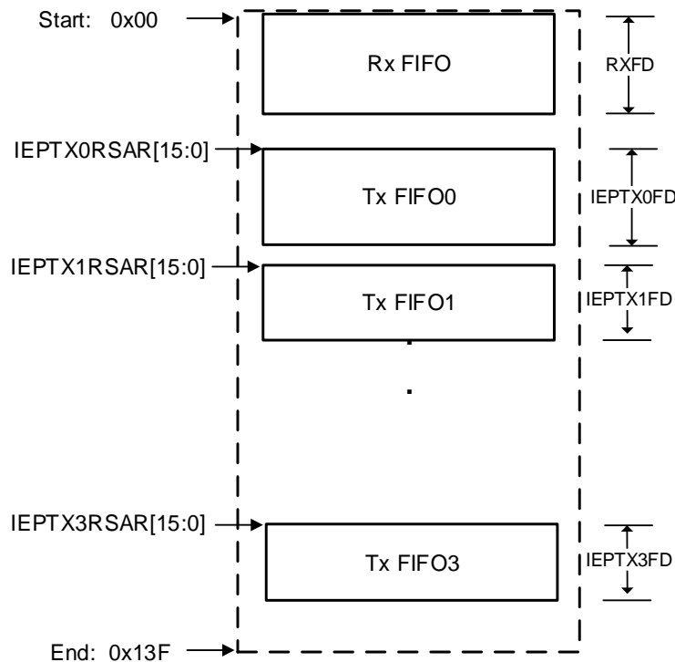
Figure 24-7. Device mode FIFO space in SRAM
