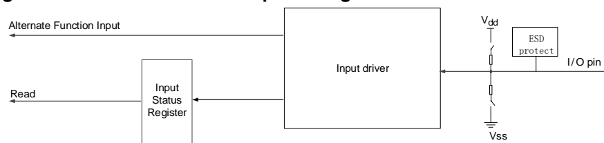
Figure 7-2. Basic structure of Input configuration
