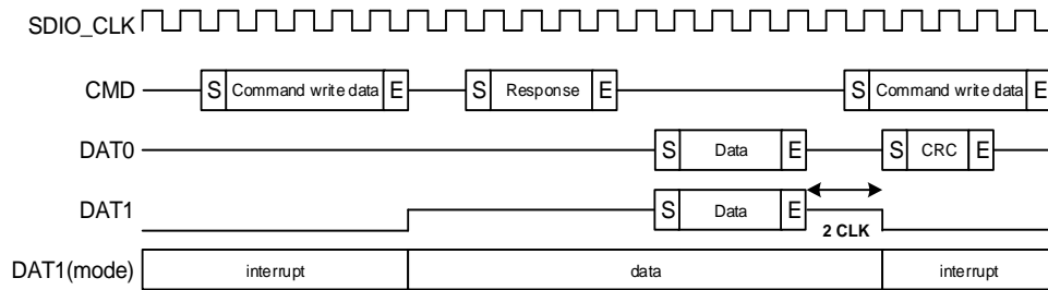
Figure 19-16. Write interrupt cycle timing
