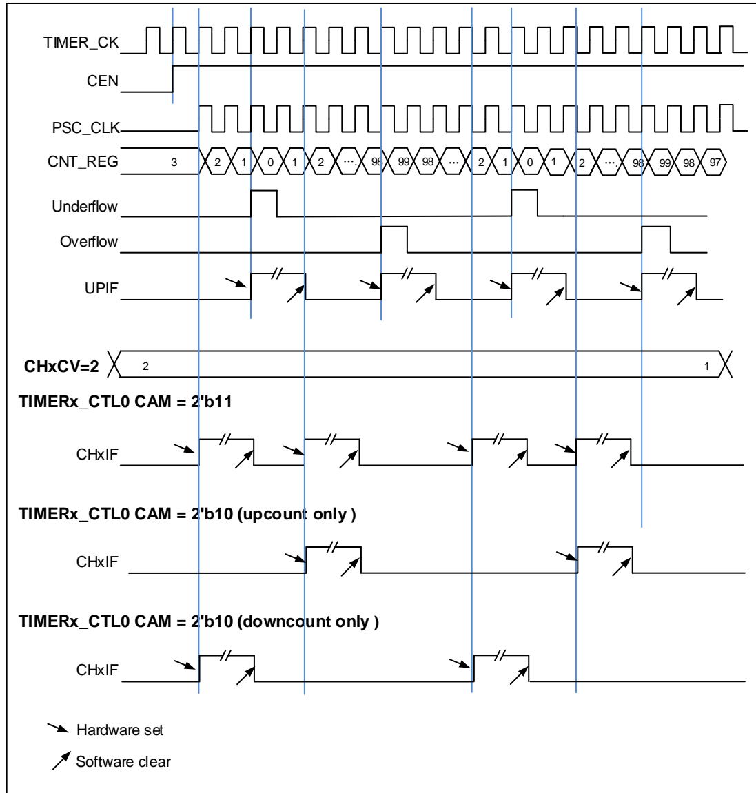
Figure 15-54. Timing chart of center-aligned counting mode
