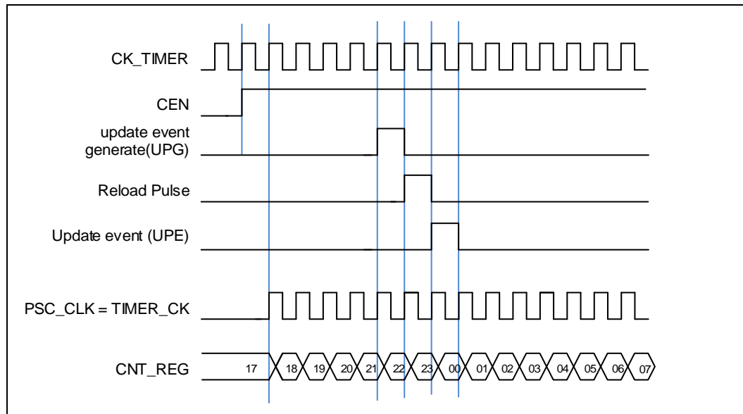
Figure 15-48. Timing chart of internal clock divided by 1
