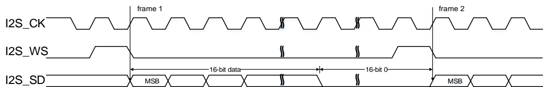
Figure 18-35. PCM standard short frame synchronization mode timing diagram (DTLEN=00, CHLEN=1, CKPL=1)
