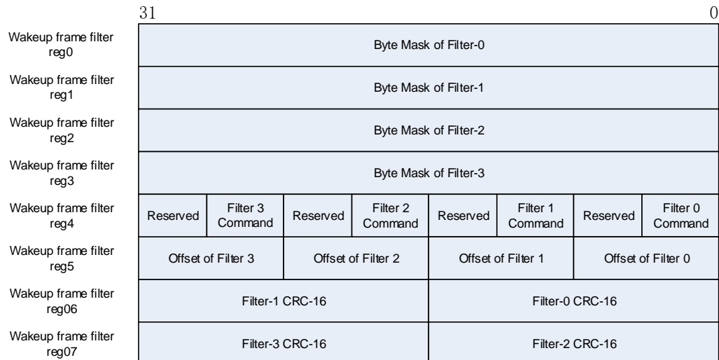
Figure 22-13. Wakeup frame filter register
