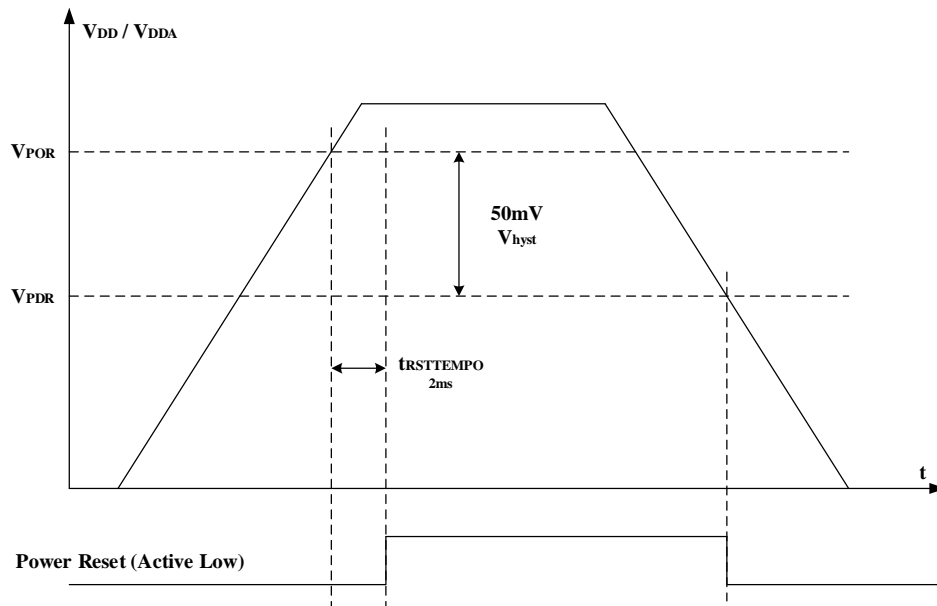
Figure 3-2. Waveform of the POR / PDR
