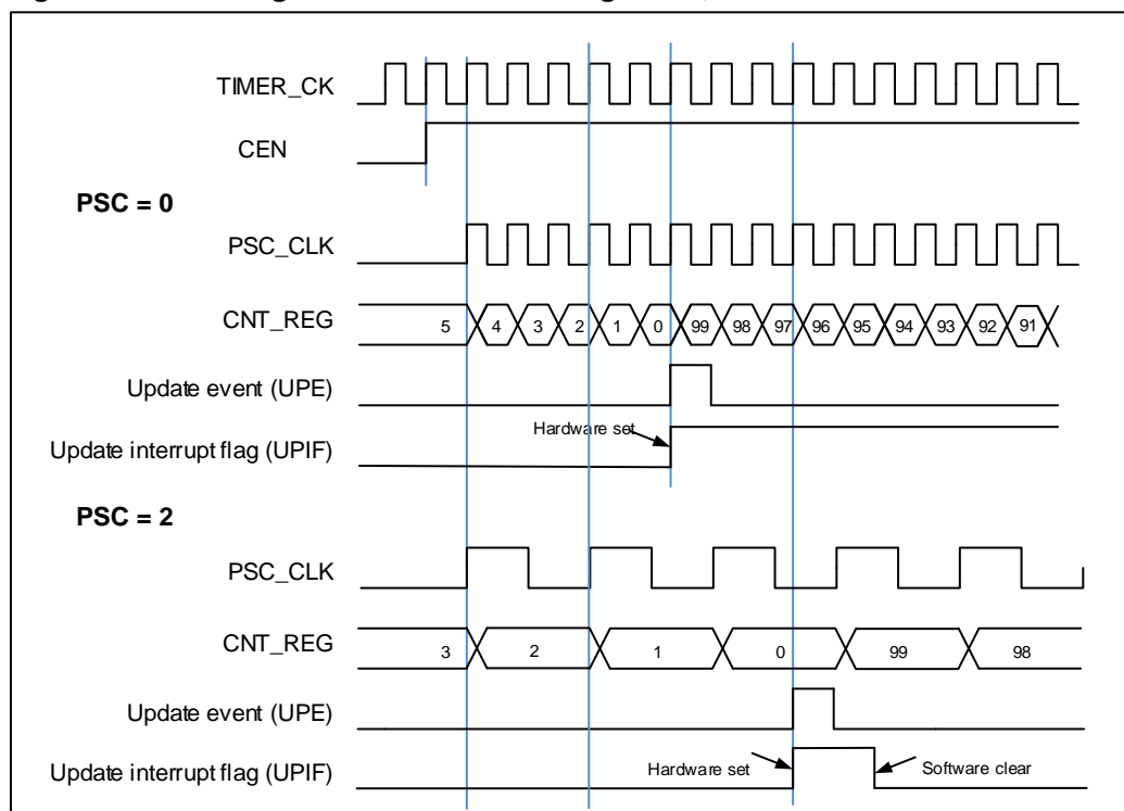
Figure 15-52. Timing chart of down counting mode, PSC=0/2
