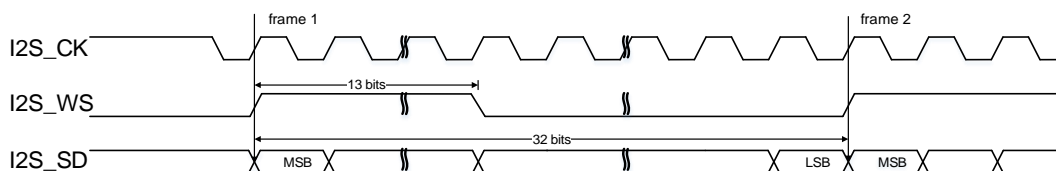
Figure 18-39. PCM standard long frame synchronization mode timing diagram (DTLEN=10, CHLEN=1, CKPL=1)
