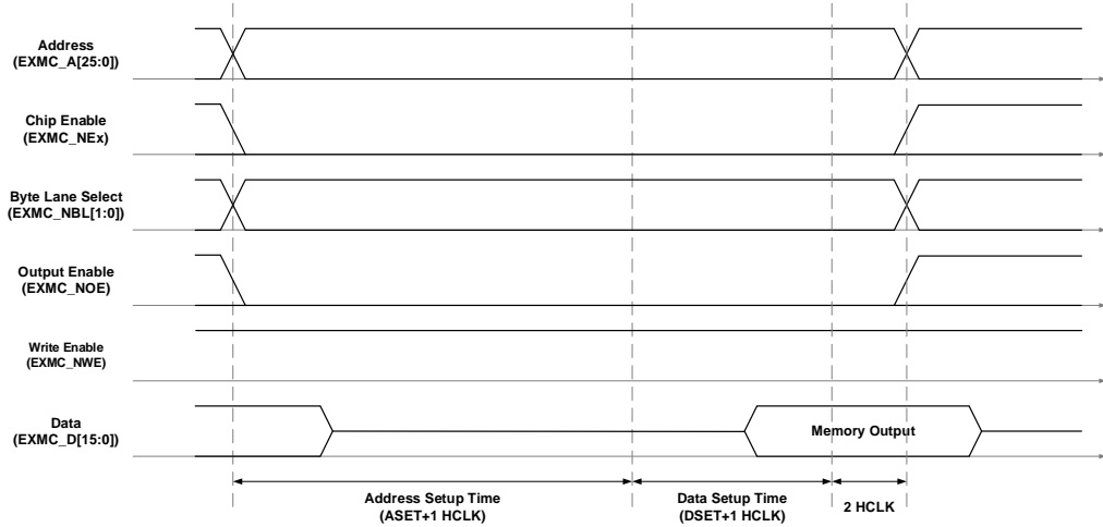
Figure 20-7. Mode 1 write access
