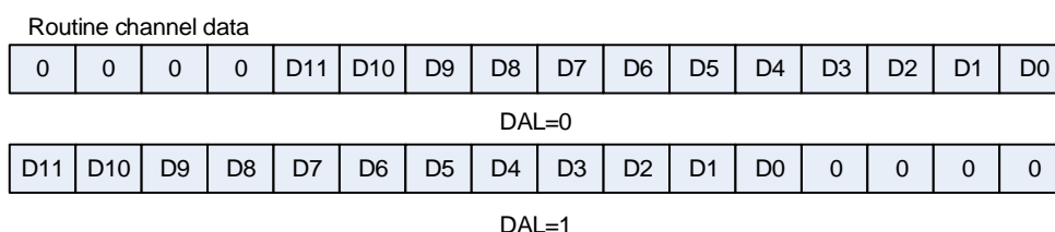
Figure 11-7. 12-bit Data storage mode
