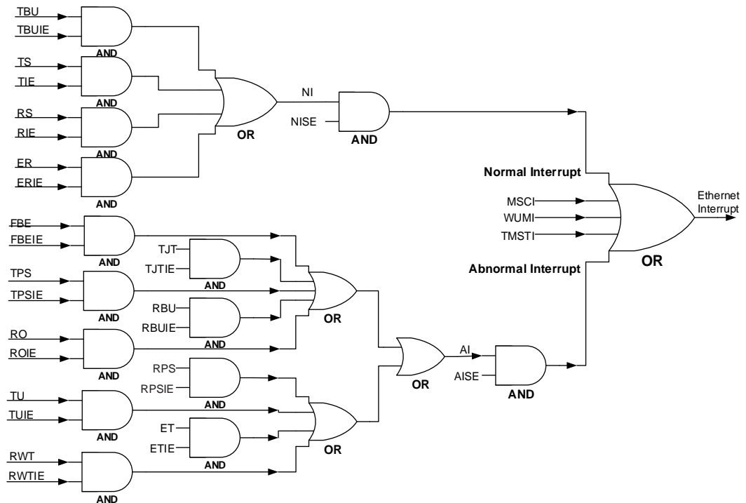
Figure 22-12. Ethernet interrupt scheme
