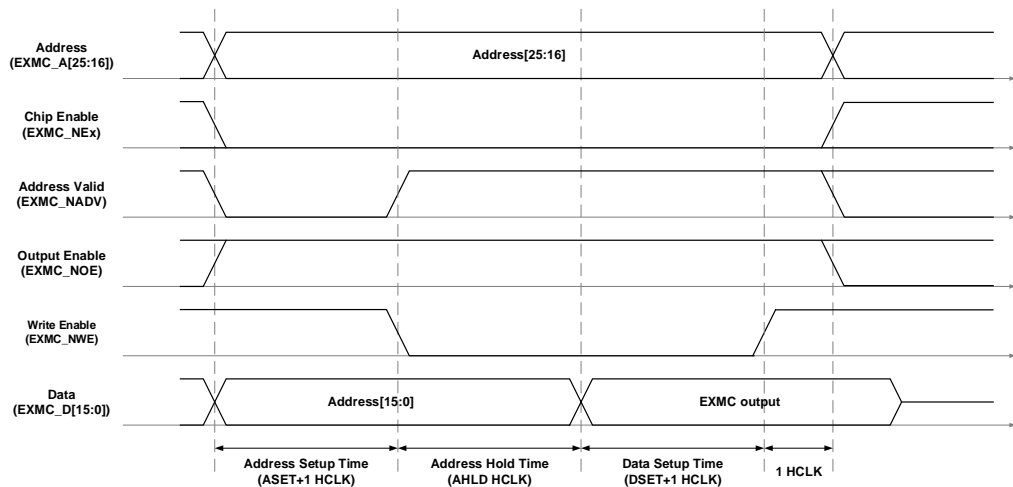
Figure 20-18. Multiplex mode write access
