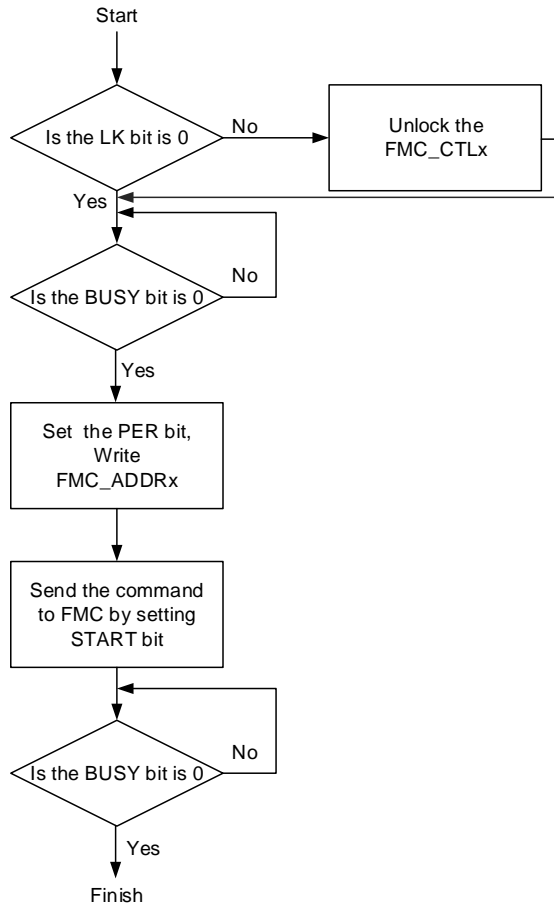
Figure 2-1. Process of page erase operation
