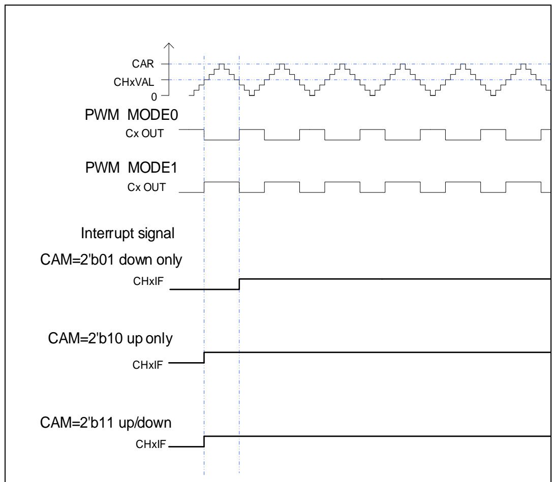
Figure 15-17. Timing chart of CAPWM
