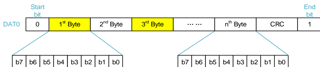
Figure 19-9. 1-bit data bus width
