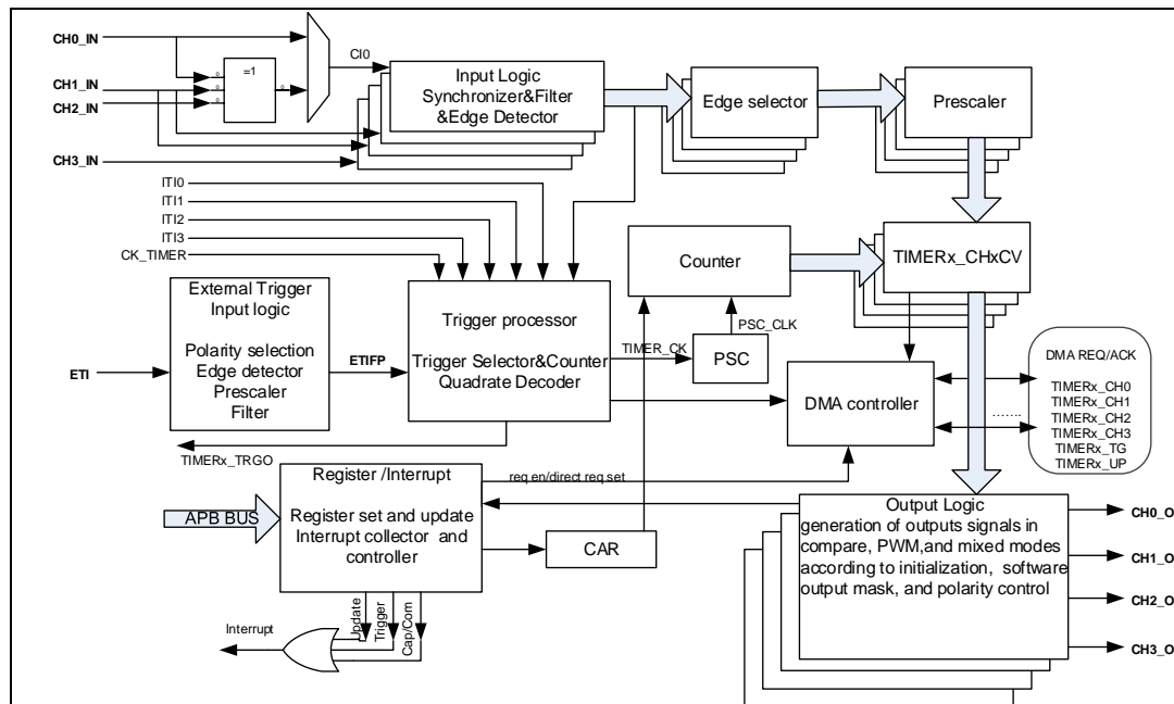
Figure 15-31. General Level 0 timer block diagram
