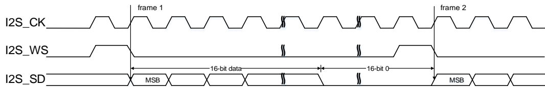
Figure 18-34. PCM standard short frame synchronization mode timing diagram (DTLEN=00, CHLEN=1, CKPL=0)
