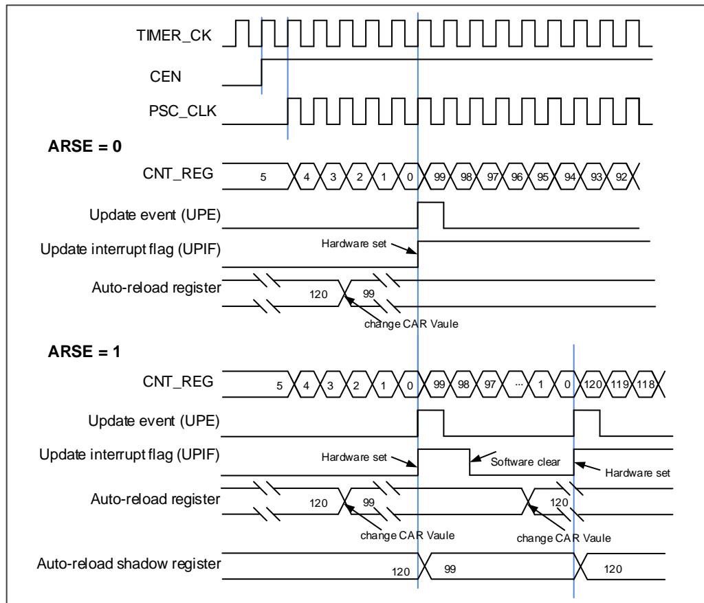
Figure 15-37. Timing chart of down counting mode, change TIMERx_CAR ongoing
