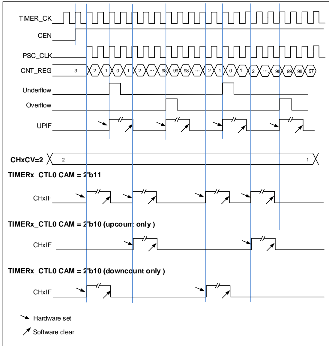
Figure 15-38. Timing chart of center-aligned counting mode
