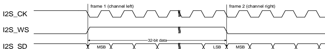
Figure 18-19. MSB justified standard timing diagram (DTLEN=10, CHLEN=1, CKPL=1)
