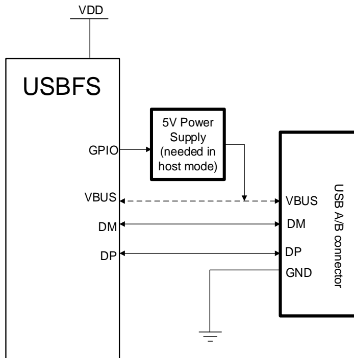
Figure 24-2. Connection with host or device mode
