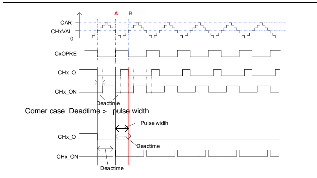
Figure 15-18. Channel output complementary PWM with dead-time insertion
