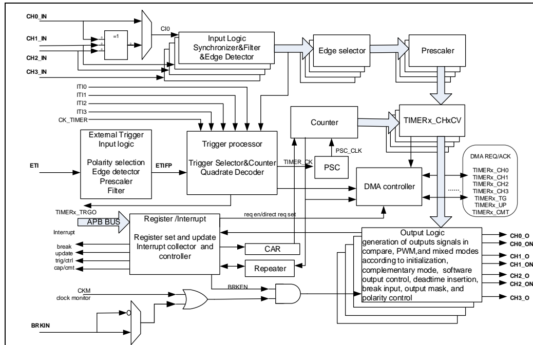
Figure 15-1. Advanced timer block diagram
