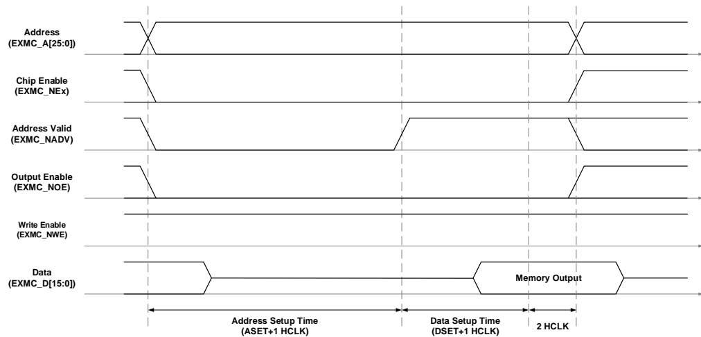
Figure 20-10. Mode 2/B read access
