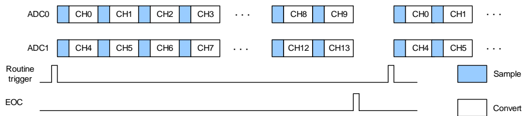
Figure 11-9. Routine parallel mode on 10 channels
