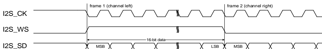
Figure 18-17. MSB justified standard timing diagram (DTLEN=00, CHLEN=0, CKPL=1)
