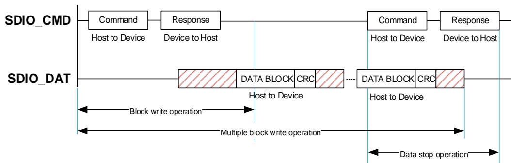
Figure 19-3. SDIO multiple blocks write operation
