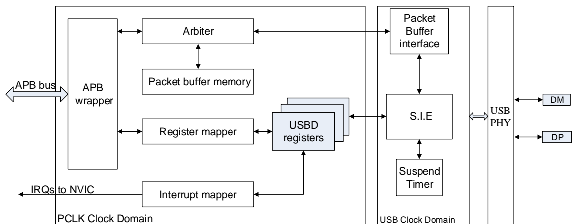
Figure 23-1. USBD block diagram
