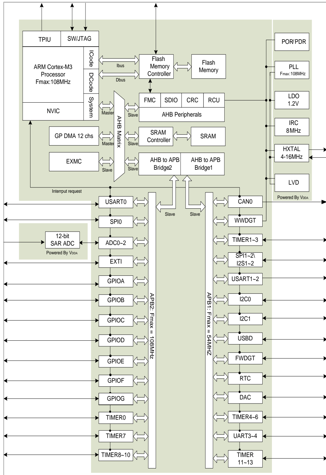
Figure 1-4. GD32F10x Extra-density series system architecture
