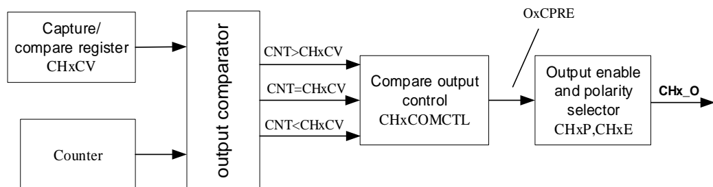
Figure 15-56. channel output compare principle (x=0,1)
