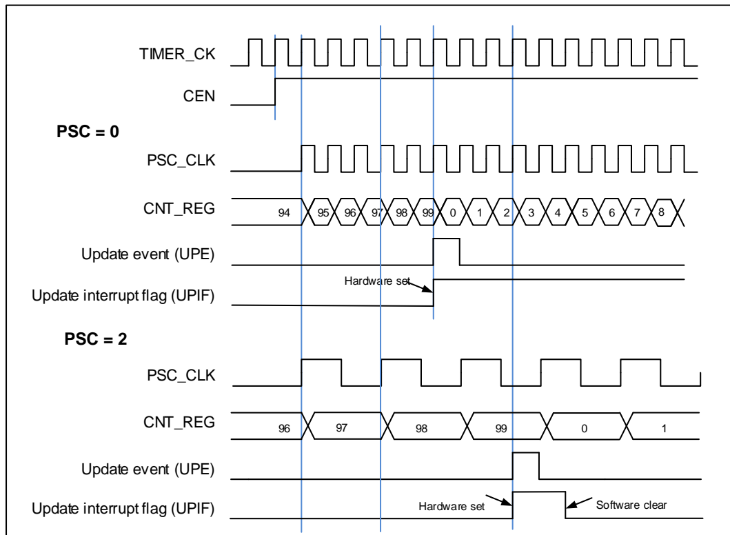
Figure 15-78. Timing chart of up counting mode, PSC=0/2
