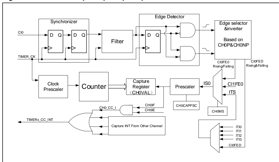
Figure 15-39. Channel input capture principle
