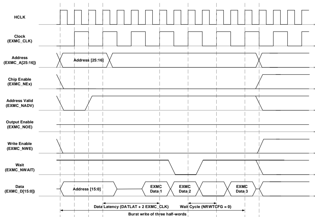
Figure 20-22. Write timing of synchronous multiplexed burst mode
