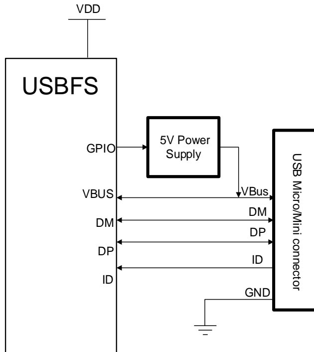
Figure 24-3. Connection with OTG mode
