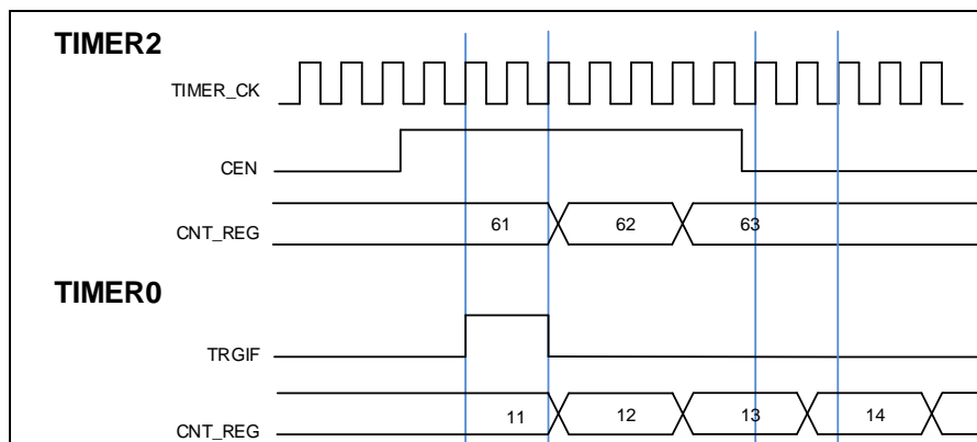
Figure 15-29. Triggering TIMER0 with enable signal of TIMER2
