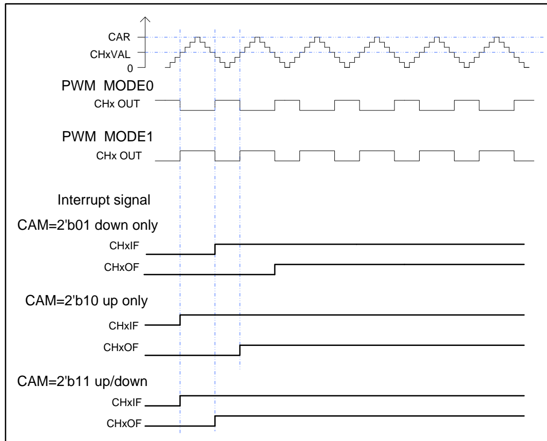
Figure 15-59. CAPWM timechart
