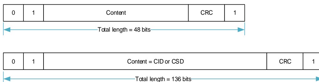
Figure 19-8. Response Token Format
