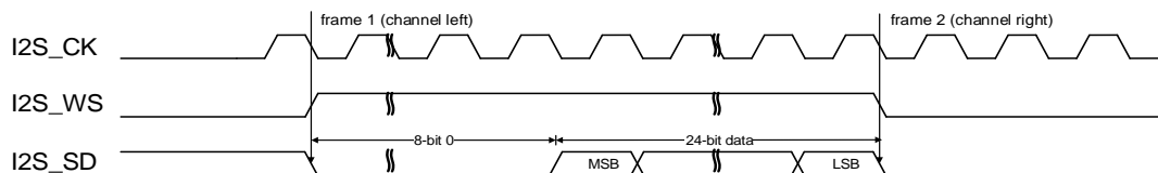
Figure 18-24. LSB justified standard timing diagram (DTLEN=01, CHLEN=1, CKPL=0)
