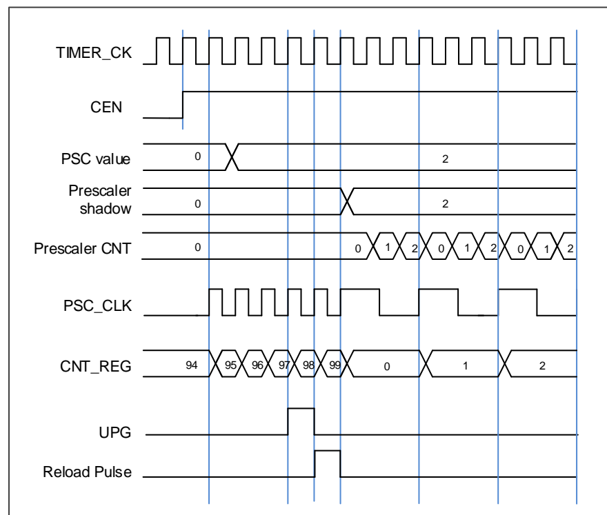
Figure 15-66. Timing chart of PSC value change from 0 to 2
