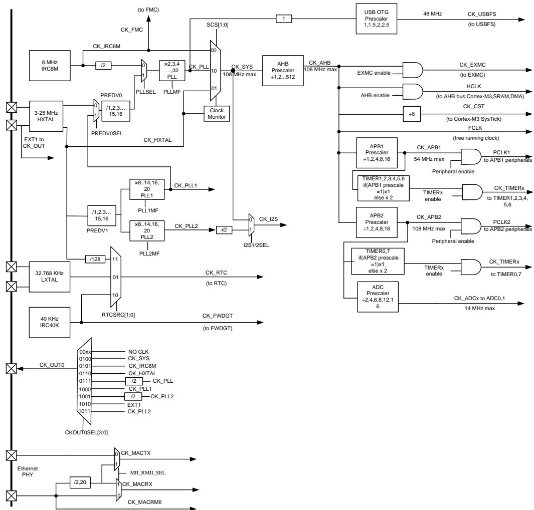
Figure 5-6. Clock tree
