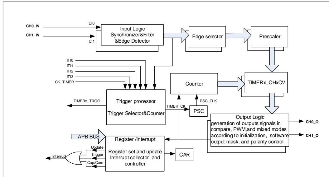
Figure 15-47. General level1 timer block diagram
