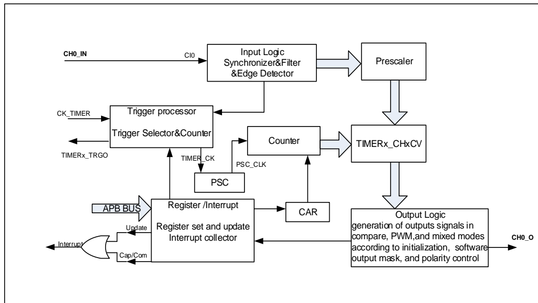
Figure 15-64. General level2 timer block diagram
