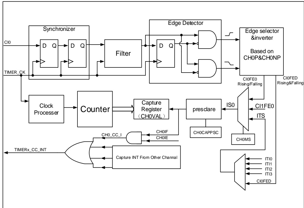
Figure 15-55. Channel input capture principle
