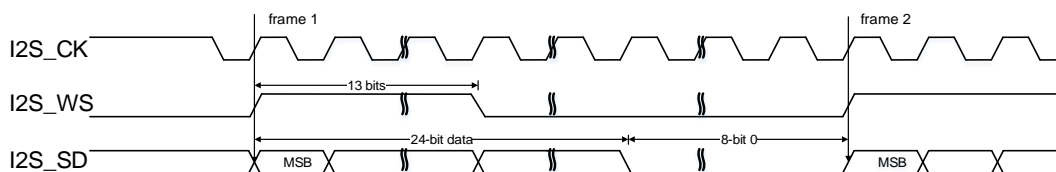
Figure 18-41. PCM standard long frame synchronization mode timing diagram (DTLEN=01, CHLEN=1, CKPL=1)
