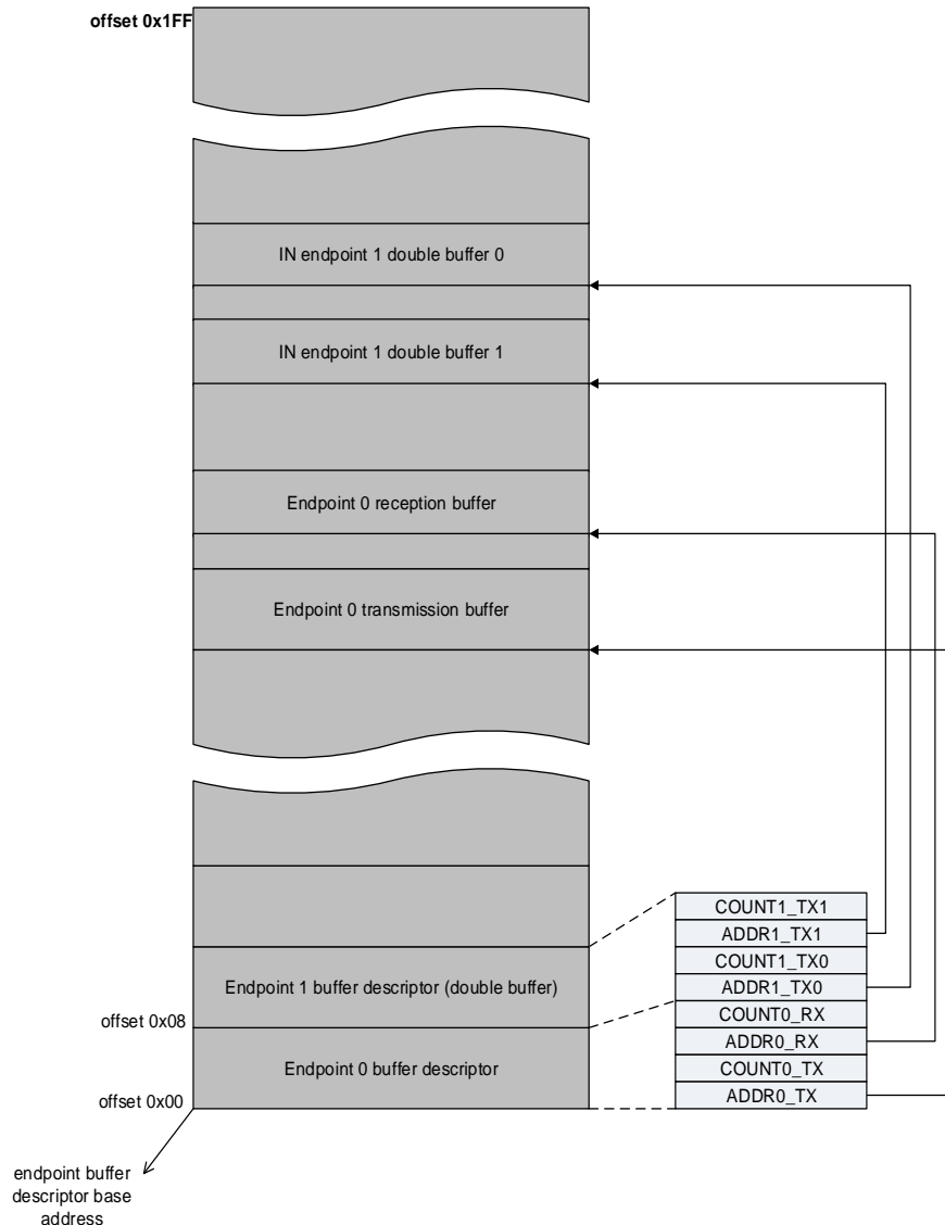
Figure 23-2. An example with buffer descriptor table usage (USB_D_BADDR = 0)
