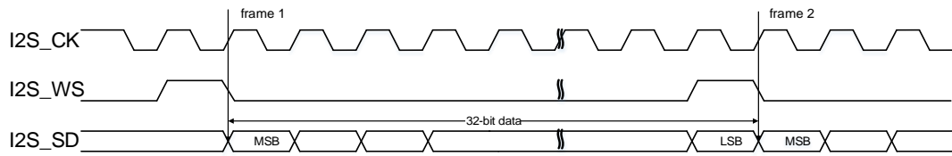
Figure 18-32. PCM standard short frame synchronization mode timing diagram (DTLEN=01, CHLEN=1, CKPL=0)
