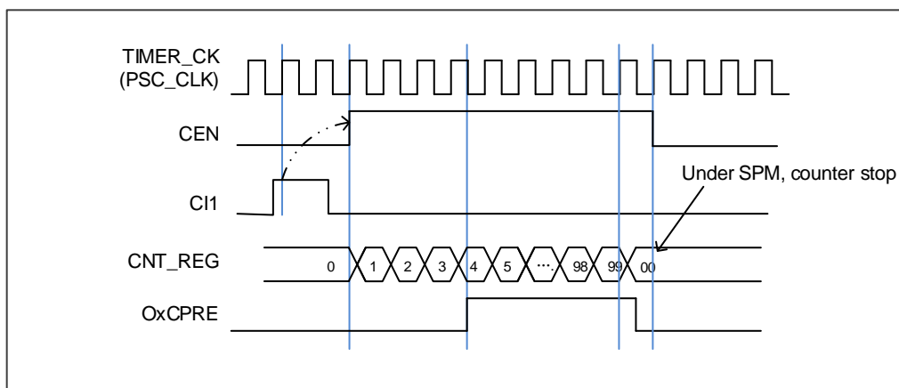
Figure 15-63. Single pulse mode TIMERx_CHxCV = 4 TIMERx_CAR=99
