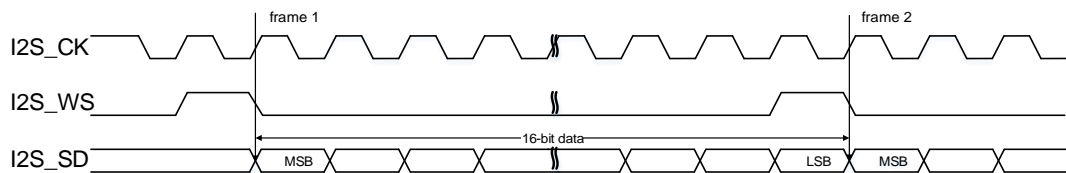
Figure 18-29. PCM standard short frame synchronization mode timing diagram (DTLEN=00, CHLEN=0, CKPL=1)
