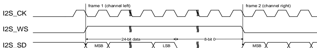
Figure 18-20. MSB justified standard timing diagram (DTLEN=01, CHLEN=1, CKPL=0)
