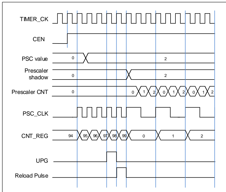
Figure 15-77. Timing chart of PSC value change from 0 to 2
