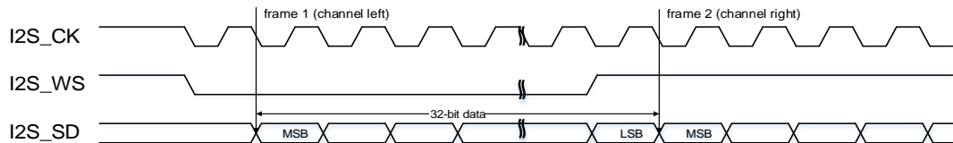
Figure 18-11. I2S Philips standard timing diagram (DTLEN=10, CHLEN=1, CKPL=1)
