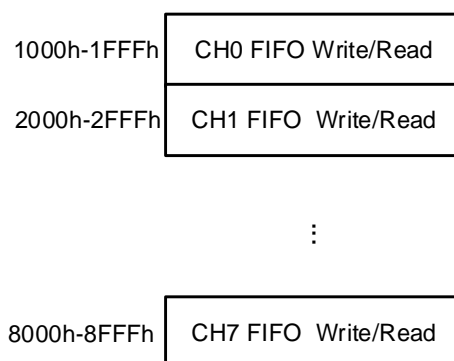
Figure 24-6. Host mode FIFO access register map
