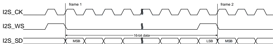
Figure 18-28. PCM standard short frame synchronization mode timing diagram (DTLEN=00, CHLEN=0, CKPL=0)
