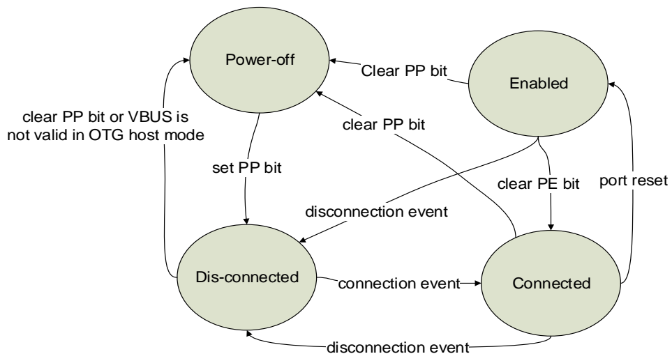
Figure 24-4. State transition diagram of host port
