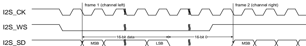
Figure 18-15. I2S Philips standard timing diagram (DTLEN=00, CHLEN=1, CKPL=1)
