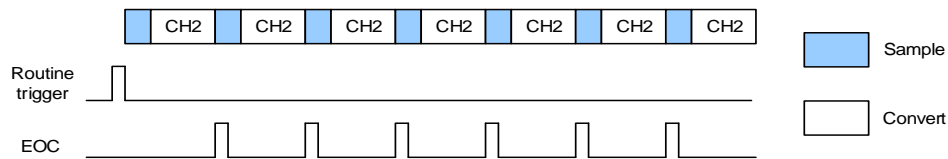
Figure 11-3. Continuous operation mode
