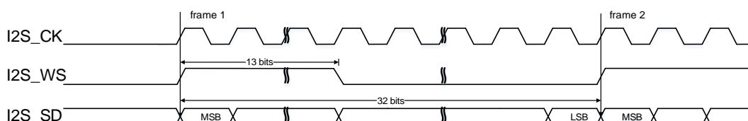
Figure 18-38. PCM standard long frame synchronization mode timing diagram (DTLEN=10, CHLEN=1, CKPL=0)
