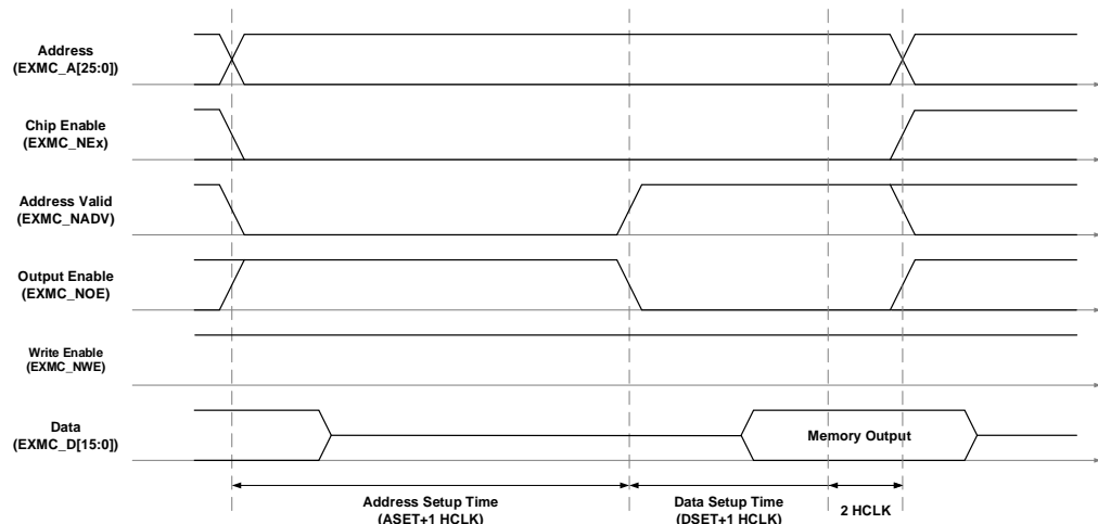
Figure 20-13. Mode C read access
