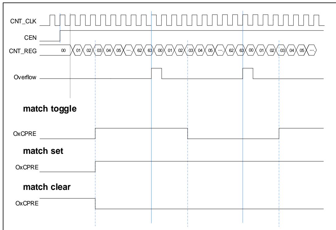
Figure 15-15. Output-compare in three modes
