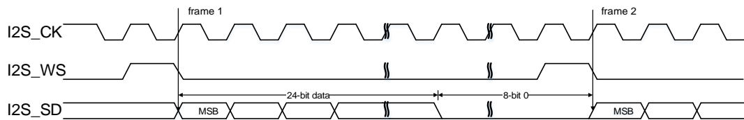
Figure 18-33. PCM standard short frame synchronization mode timing diagram (DTLEN=01, CHLEN=1, CKPL=1)
