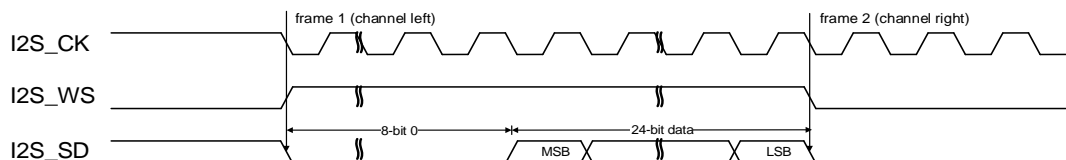
Figure 18-25. LSB justified standard timing diagram (DTLEN=01, CHLEN=1, CKPL=1)
