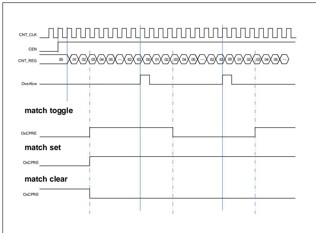
Figure 15-57. Output-compare under three modes
