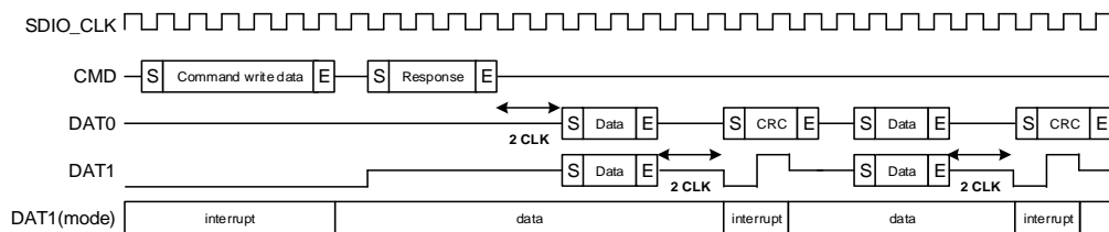
Figure 19-18. Multiple block 4-Bit write interrupt cycle timing
