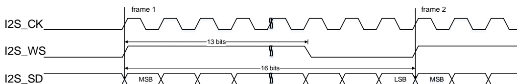
Figure 18-37. PCM standard long frame synchronization mode timing diagram (DTLEN=00, CHLEN=0, CKPL=1)
