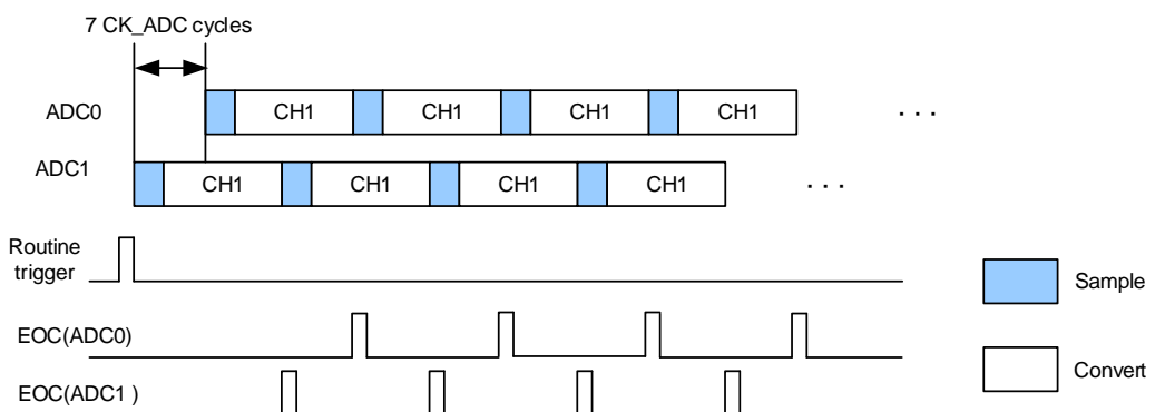
Figure 11-10. Routine follow-up fast mode (the CTN bit of ADCs are set)
