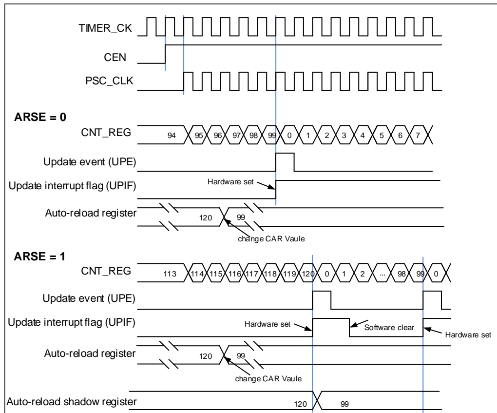
Figure 15-51. Timing chart of up counting mode, change TIMERx_CAR ongoing
