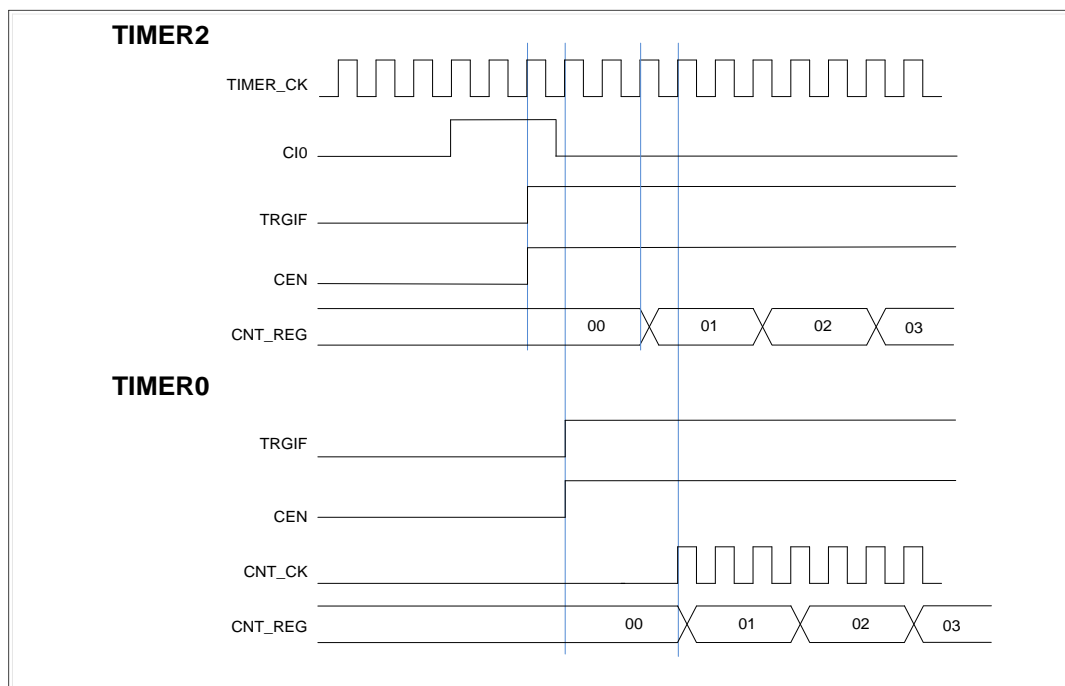
Figure 15-30. Triggering TIMER0 and TIMER2 with TIMER2's CI0 input
