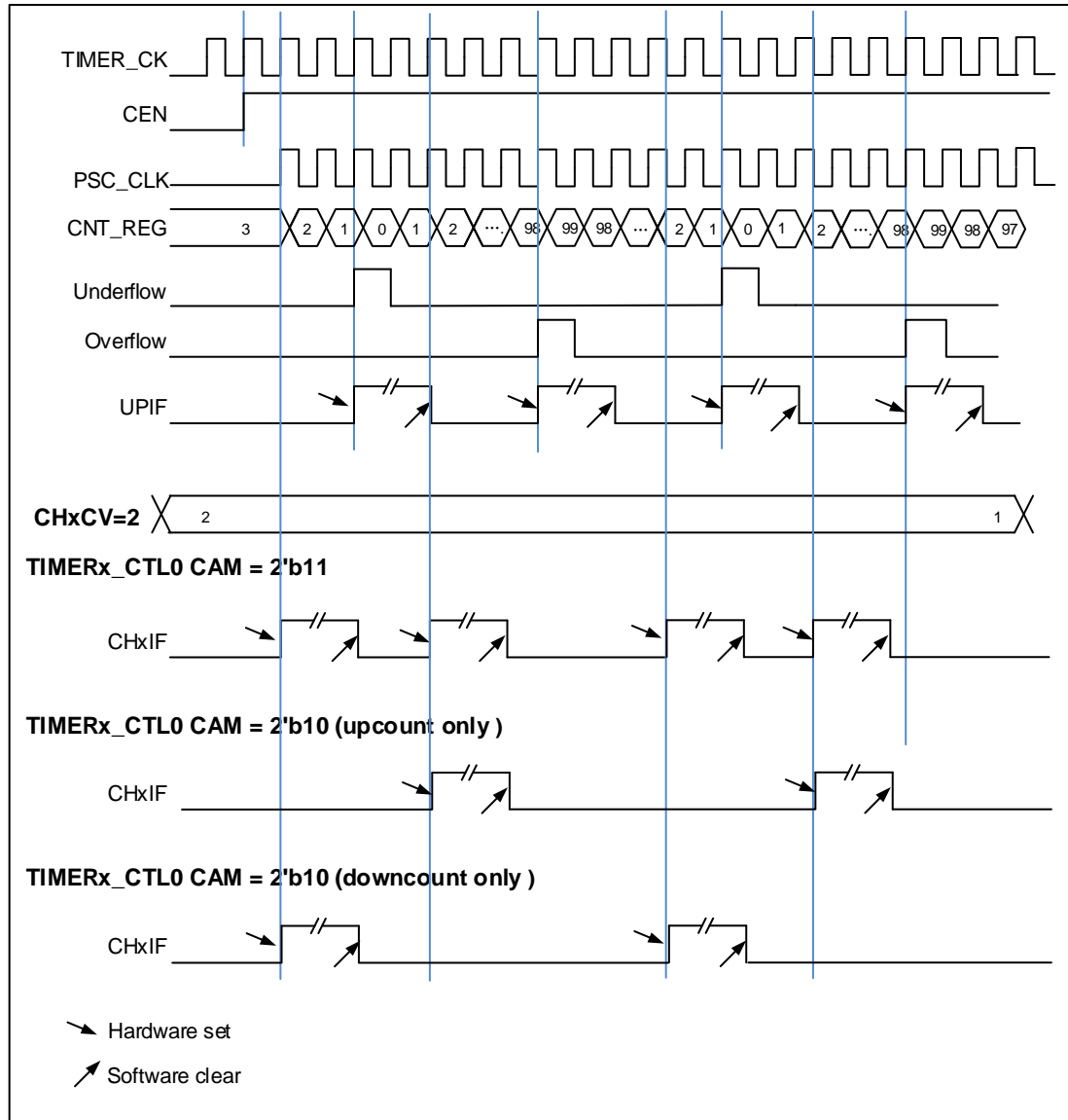
Figure 15-71. Center-aligned counter timechart
