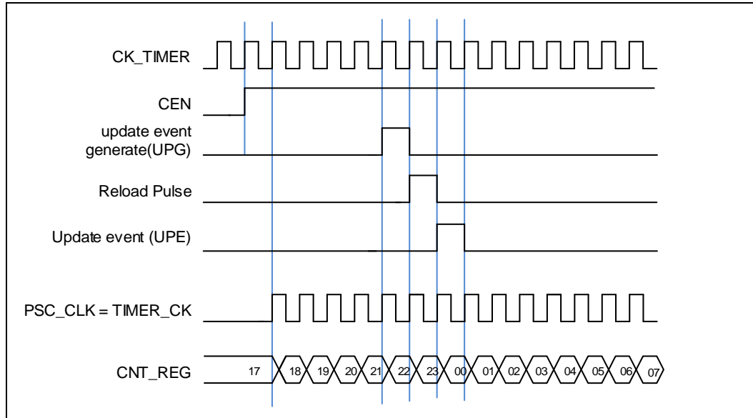
Figure 15-76. Timing chart of internal clock divided by 1
