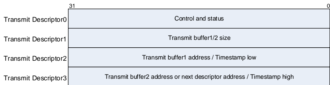
Figure 22-7. Transmit descriptor
