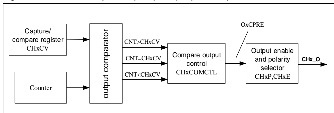
Figure 15-40. channel output compare principle (x=0,1,2,3)
