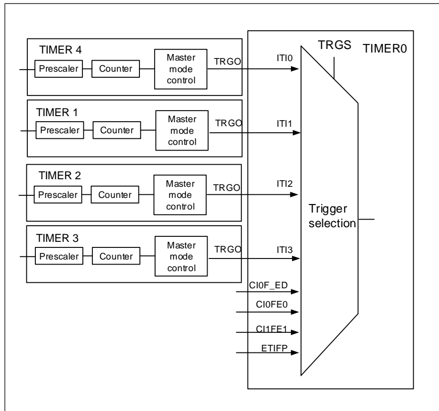
Figure 15-28. Timer0 master/slave mode timer example
