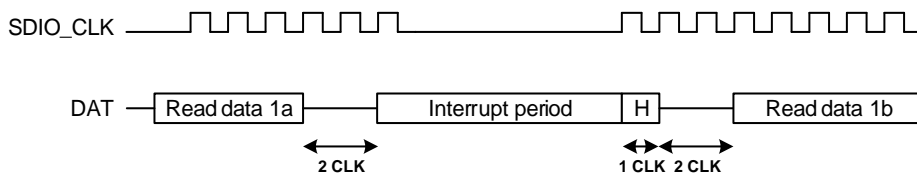
Figure 19-13. Read wait operation using SDIO_DAT[2]
