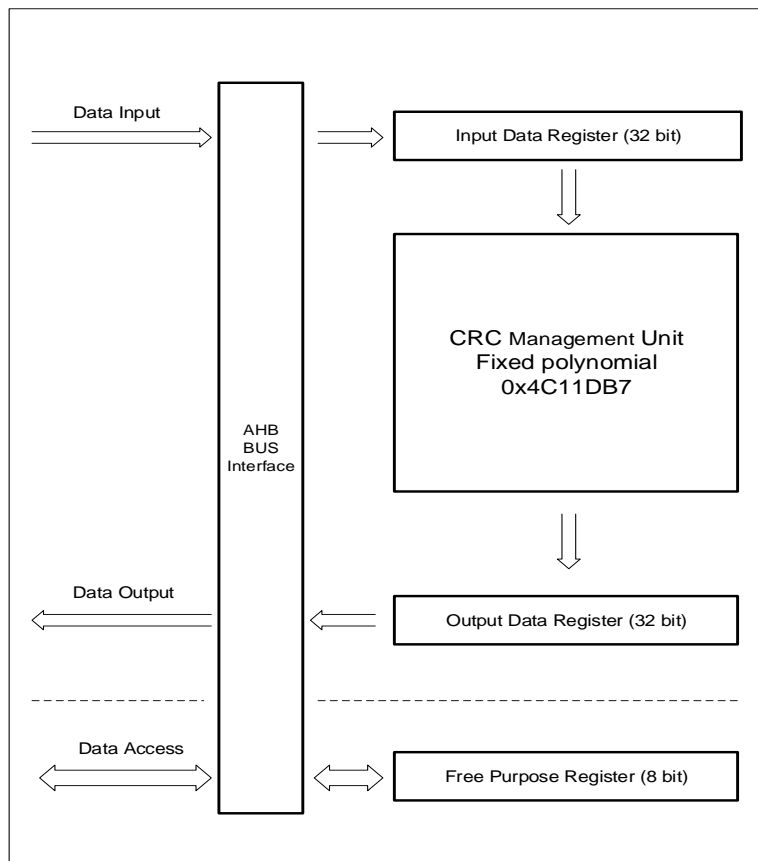
Figure 8-1. Block diagram of CRC management unit
