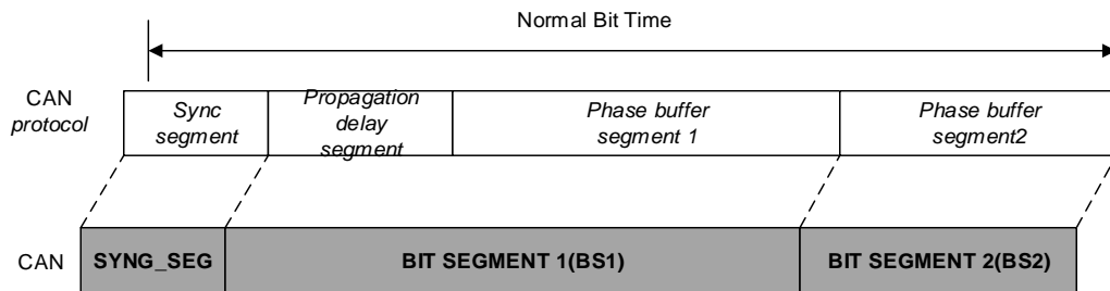
Figure 21-11. The bit time
