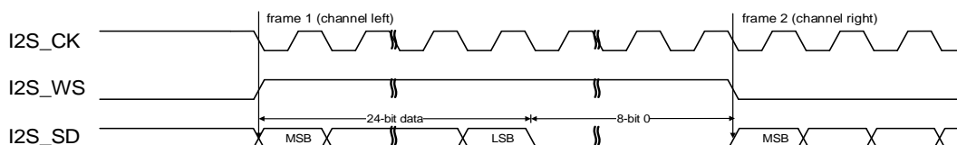
Figure 18-21. MSB justified standard timing diagram (DTLEN=01, CHLEN=1, CKPL=1)
