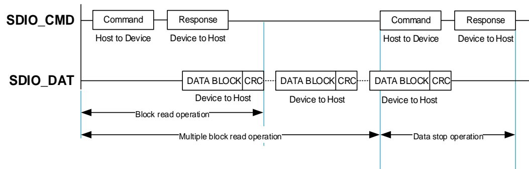
Figure 19-2. SDIO multiple blocks read operation
