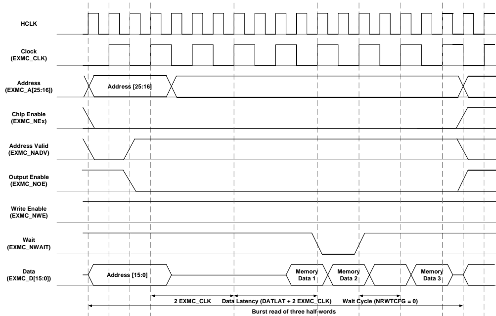
Figure 20-21. Read timing of synchronous multiplexed burst mode
