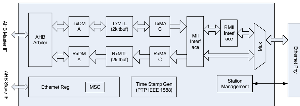
Figure 22-1. ENET module block diagram
