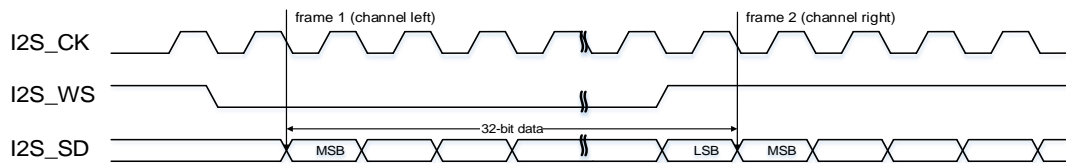
Figure 18-10. I2S Philips standard timing diagram (DTLEN=10, CHLEN=1, CKPL=0)
