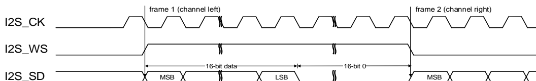
Figure 18-22. MSB justified standard timing diagram (DTLEN=00, CHLEN=1, CKPL=0)
