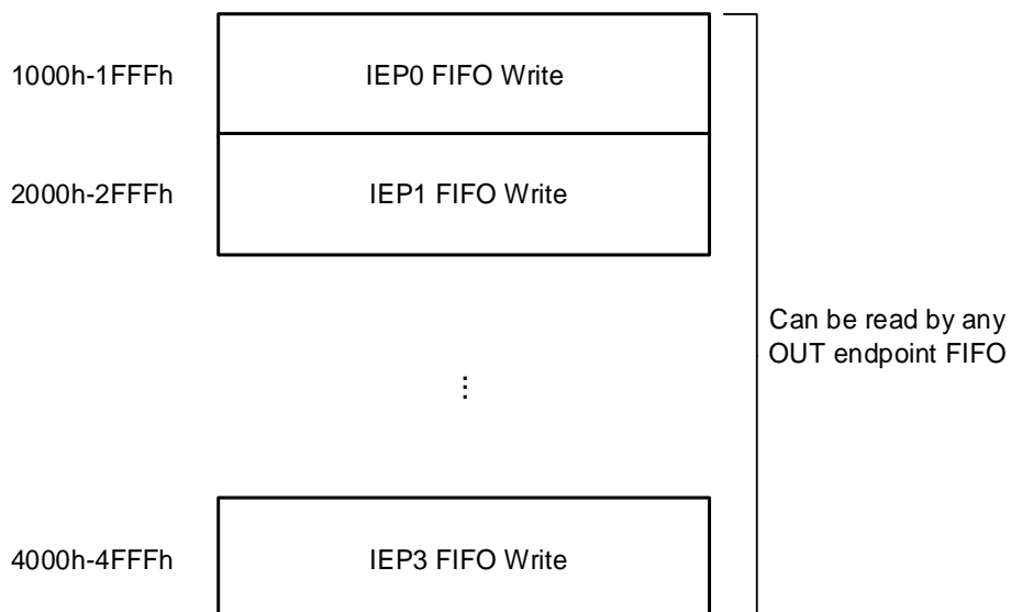
Figure 24-8. Device mode FIFO access register map
