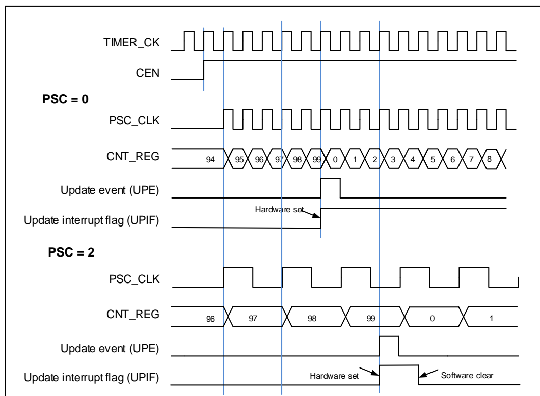
Figure 15-67. Up-counter timechart, PSC=0/2
