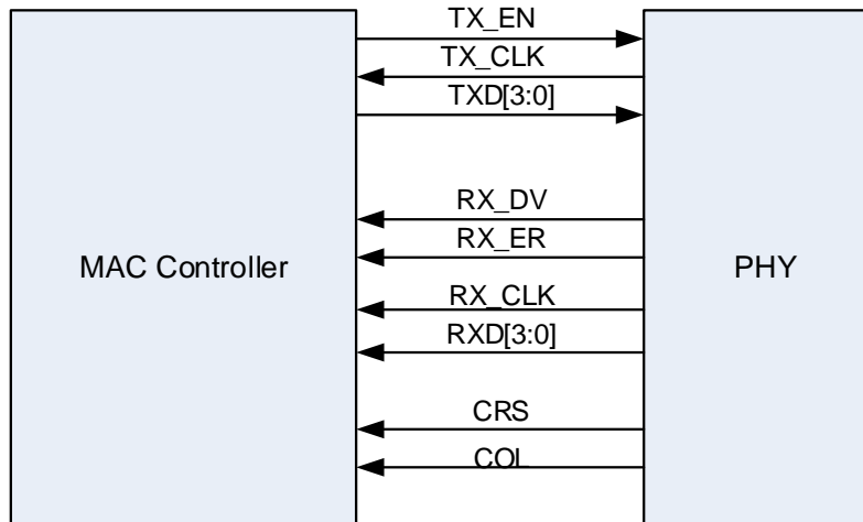
Figure 22-4. Media independent interface signals
