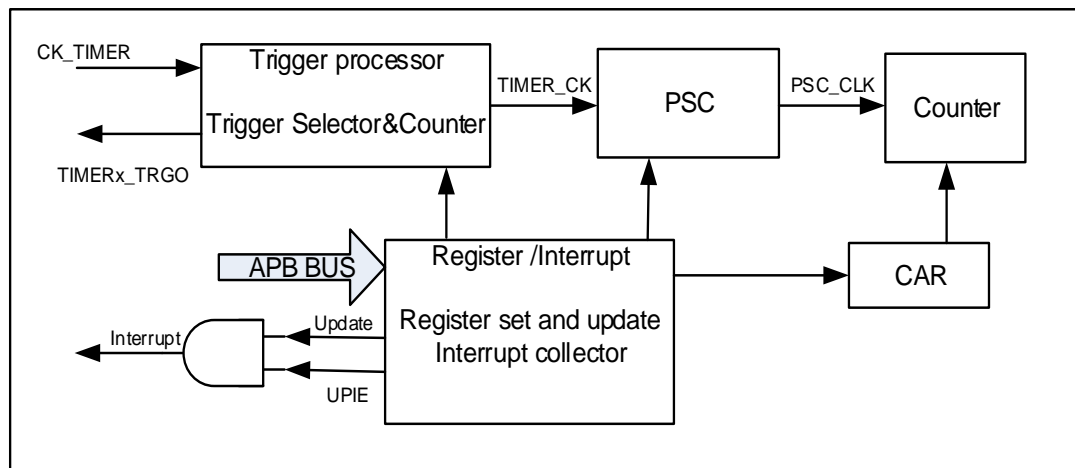
Figure 15-75. Basic timer block diagram
