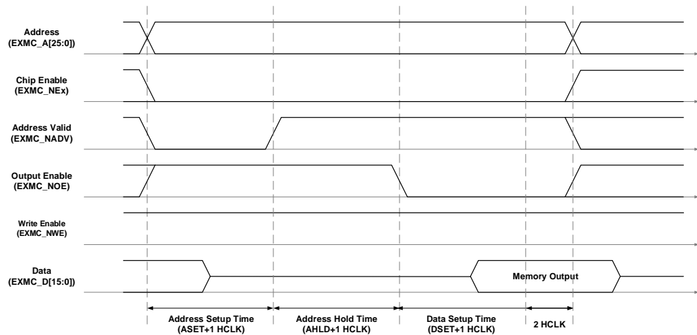
Figure 20-15. Mode D read access
