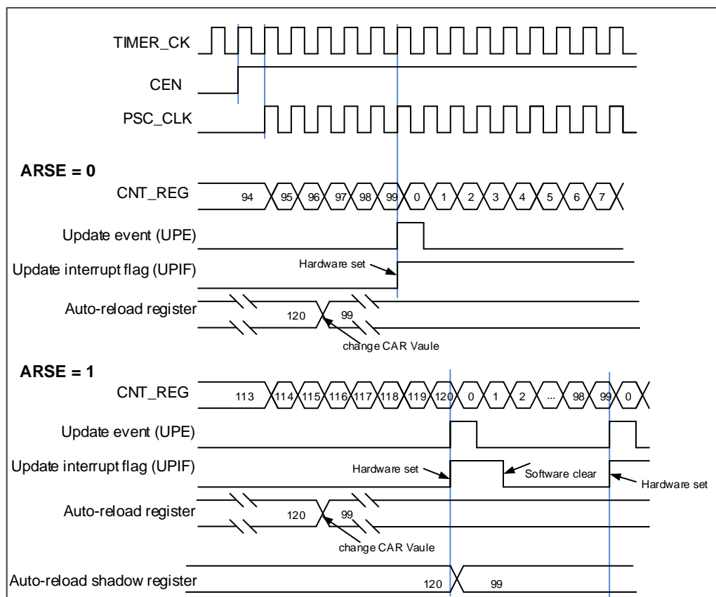
Figure 15-79. Timing chart of up counting mode, change TIMERx_CAR ongoing
