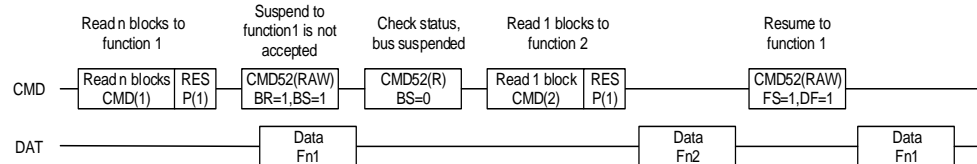
Figure 19-14. Function2 read cycle inserted during function1 multiple read cycle
