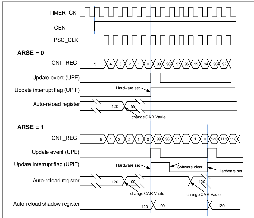
Figure 15-70. Down-counter timechart, change TIMERx_CAR on the go
