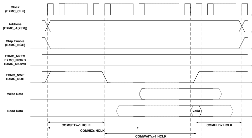
Figure 20-23. Access timing of common memory space of PC Card Controller
