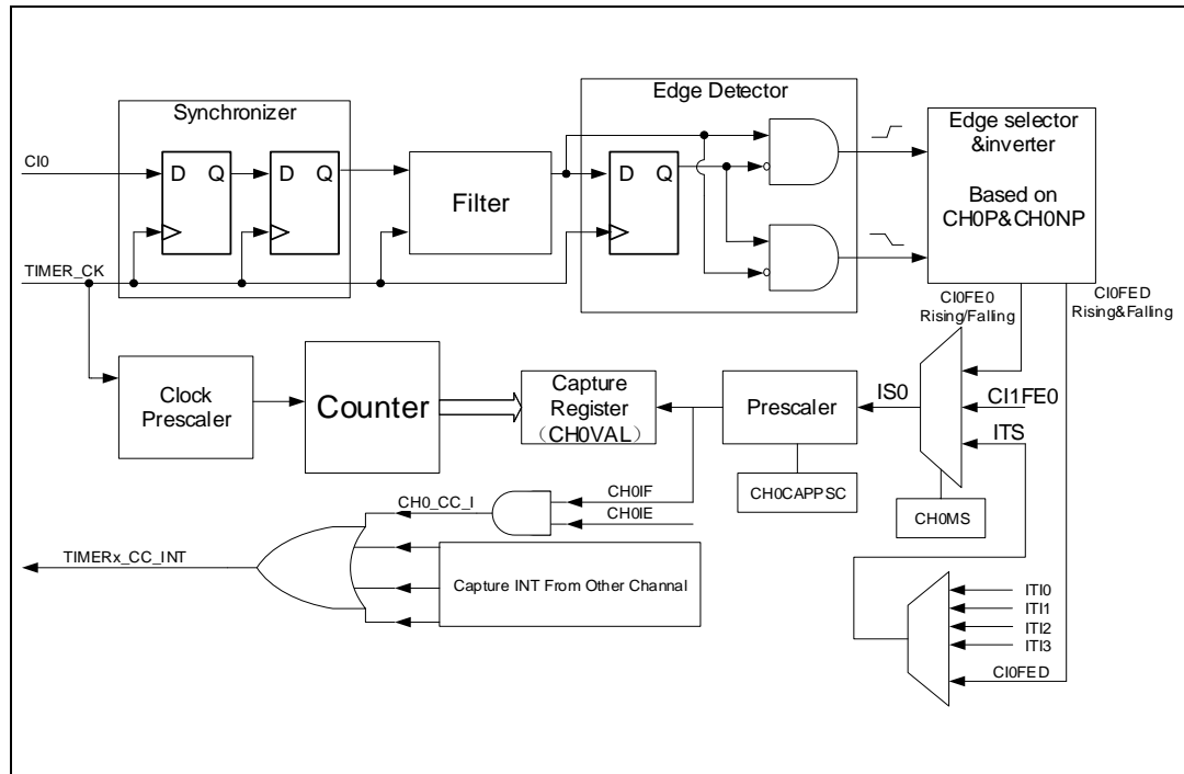
Figure 15-12. Channel input capture principle
