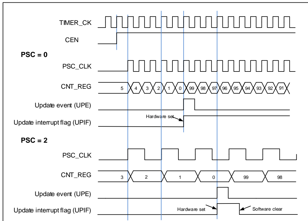
Figure 15-69. Down-counter timechart, PSC=0/2
