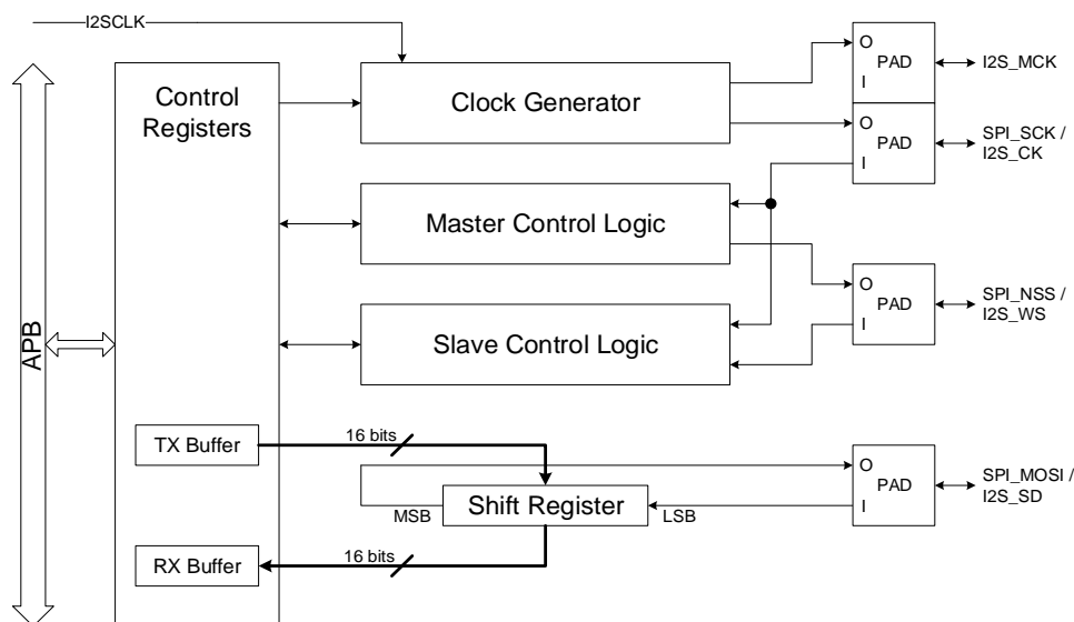
Figure 18-7. Block diagram of I2S
