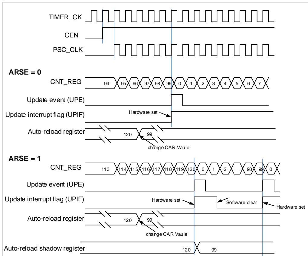
Figure 15-68. Up-counter timechart, change TIMERx_CAR on the go
