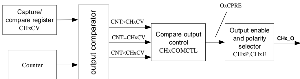
Figure 15-73. Channel output compare principle (x=0)
