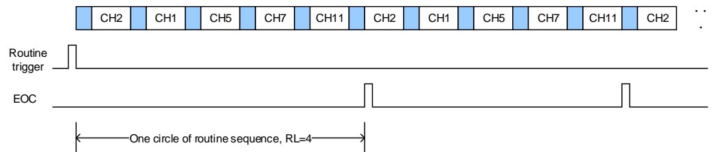
Figure 11-5. Scan operation mode, continuous enable
