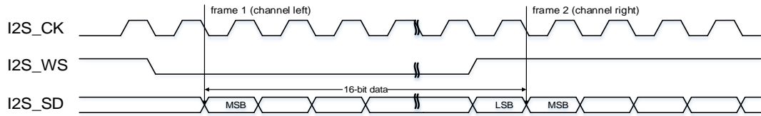
Figure 18-8. I2S Philips standard timing diagram (DTLEN=00, CHLEN=0, CKPL=0)
