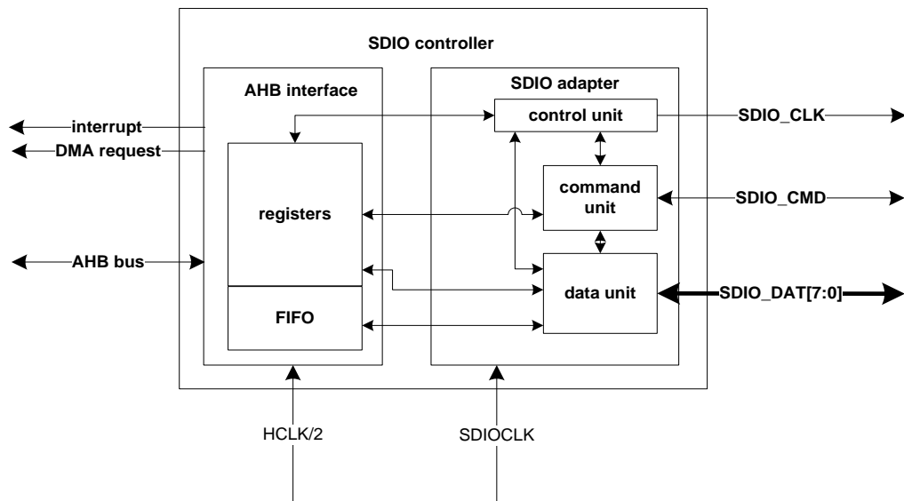
Figure 19-6. SDIO block diagram
