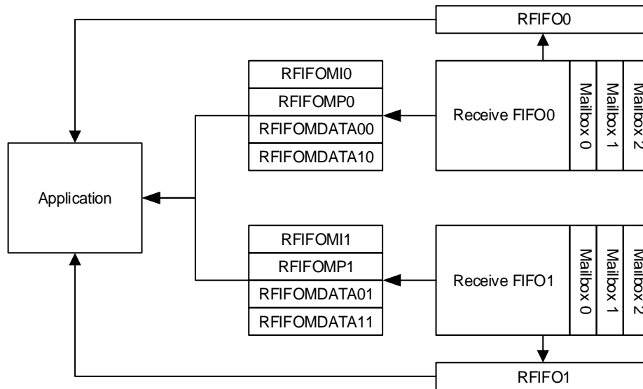
Figure 21-4. Reception register
