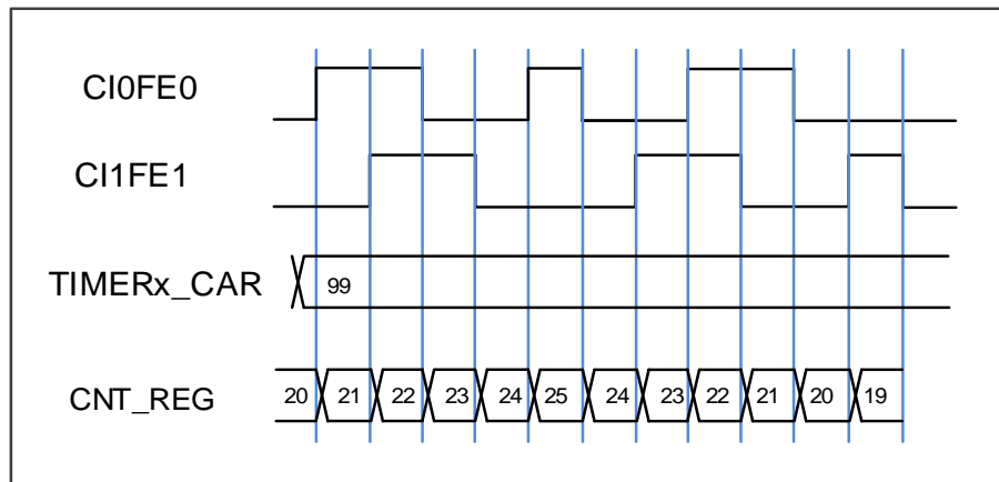
Figure 15-20. Counter behavior with CI0FE0 polarity non-inverted in mode 2
