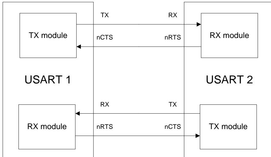
Figure 16-7. Hardware flow control between two USARTs
