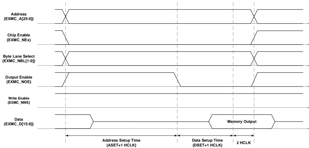
Figure 20-8. Mode A read access
