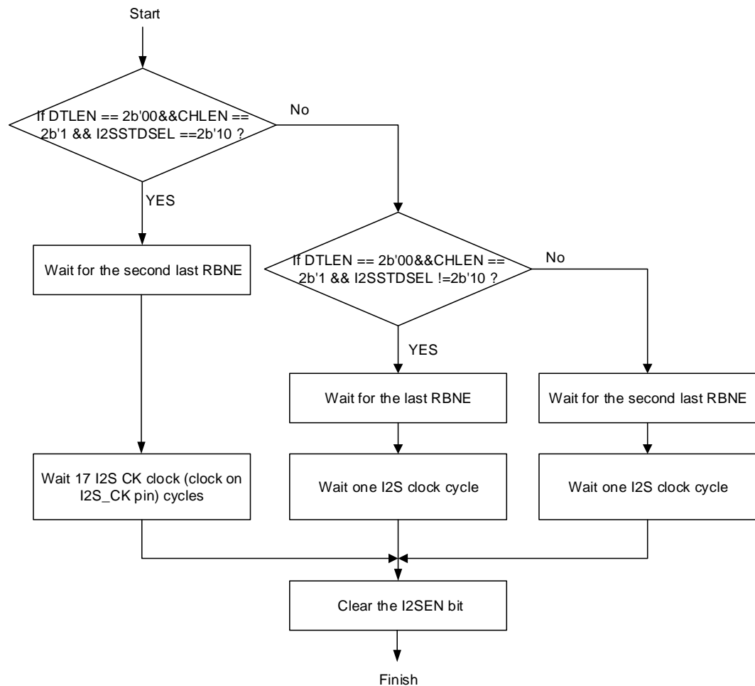
Figure 18-46. I2S master reception disabling sequence
