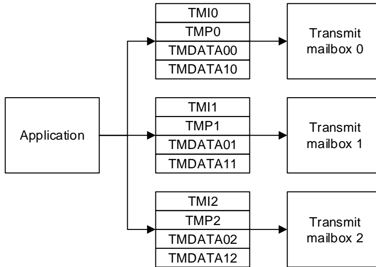
Figure 21-2. Transmission register
