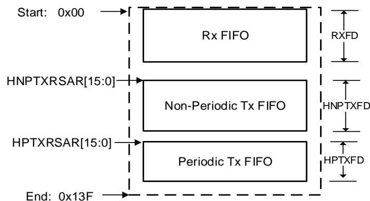
Figure 24-5. HOST mode FIFO space in SRAM
