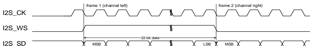
Figure 18-18. MSB justified standard timing diagram (DTLEN=10, CHLEN=1, CKPL=0)
