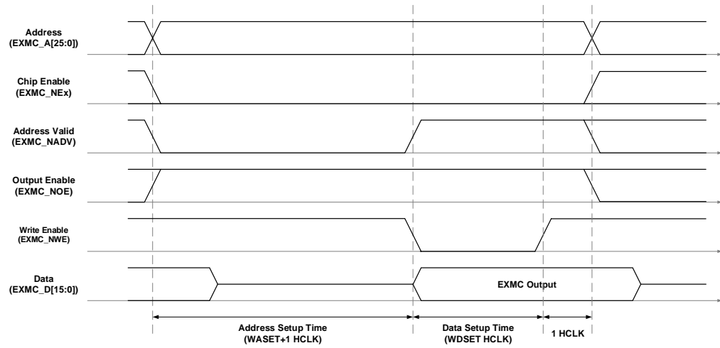
Figure 20-14. Mode C write access
