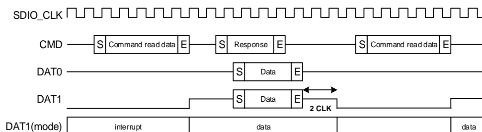
Figure 19-15. Read Interrupt cycle timing
