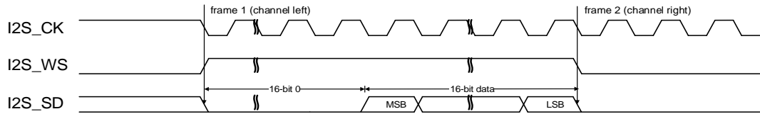
Figure 18-27. LSB justified standard timing diagram (DTLEN=00, CHLEN=1, CKPL=1)
