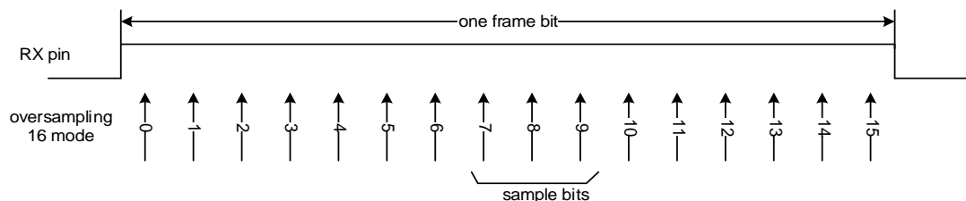
Figure 16-4. Oversampling method of a receive frame bit
