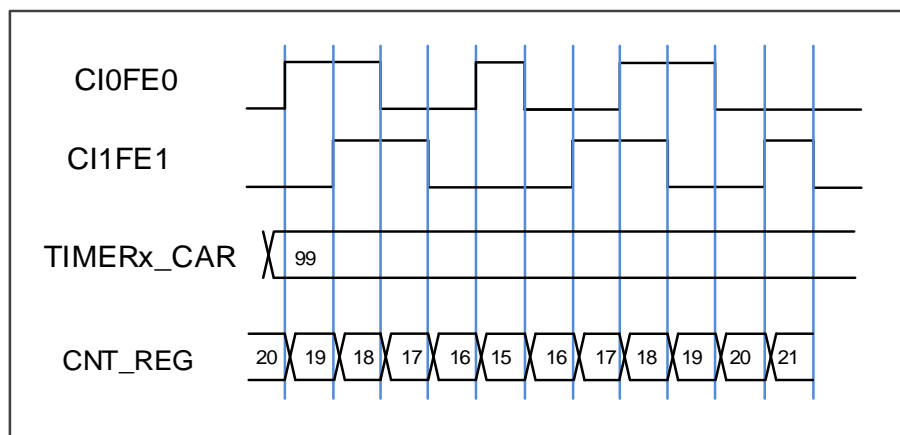
Figure 15-21. Counter behavior with CI0FE0 polarity inverted in mode 2
