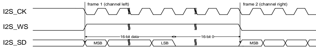
Figure 18-23. MSB justified standard timing diagram (DTLEN=00, CHLEN=1, CKPL=1)
