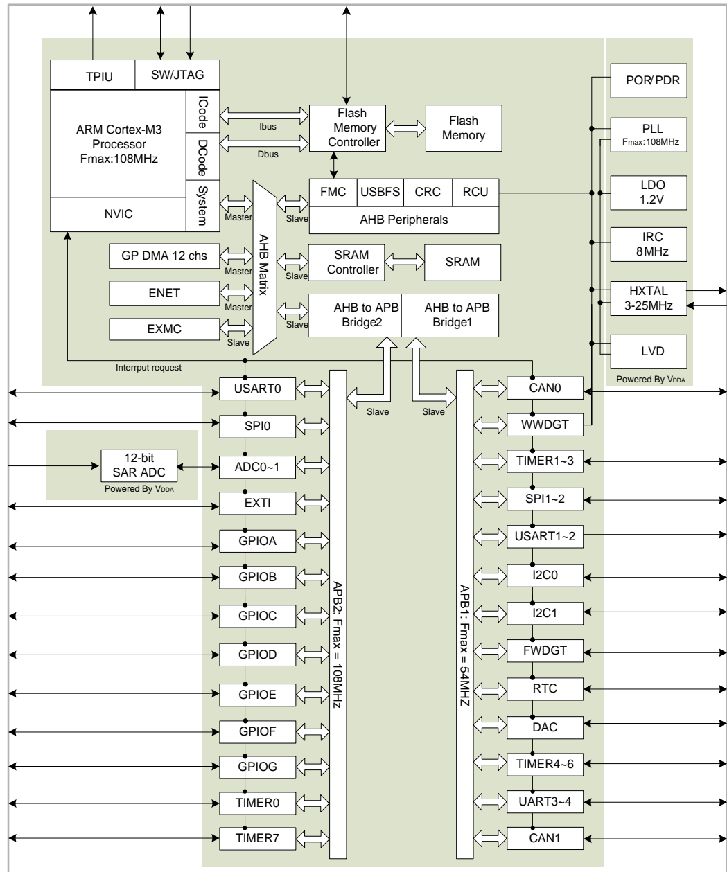
Figure 1-5. GD32F10x Connectivity line series system architecture
