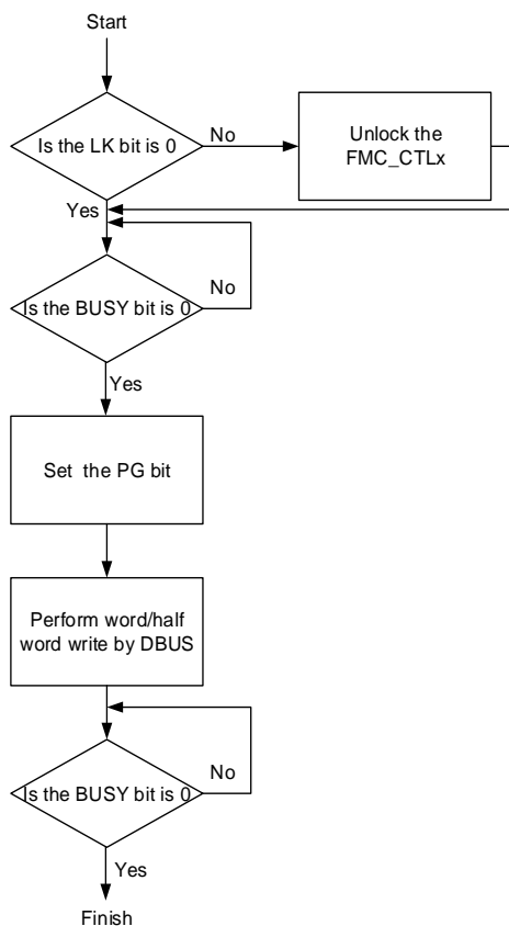
Figure 2-3. Process of word program operation
