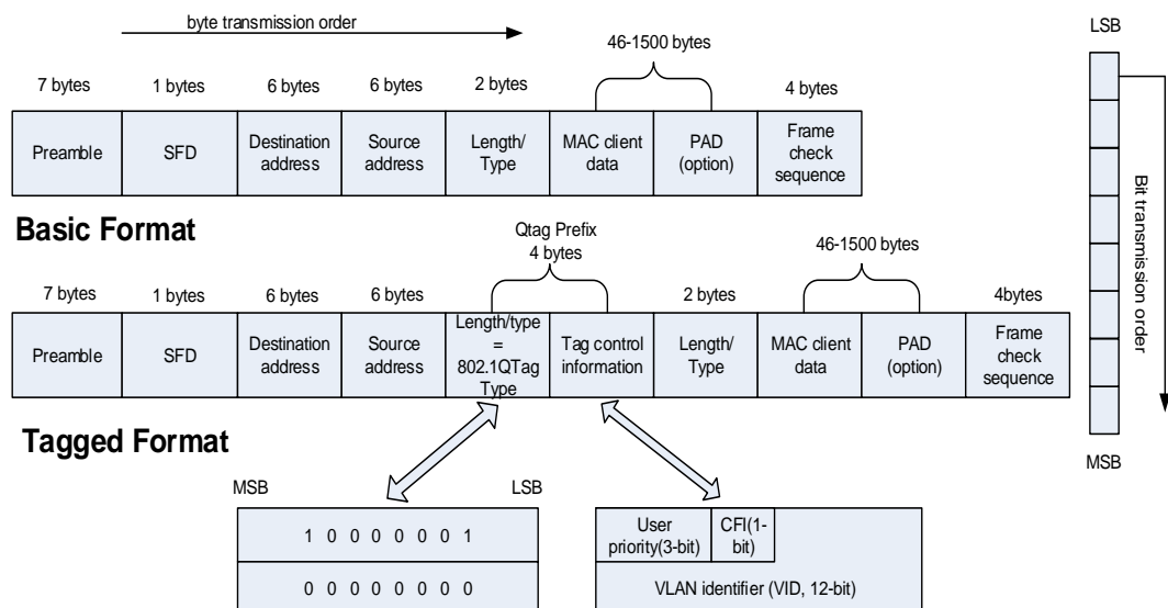
Figure 22-2. MAC/Tagged MAC frame format
