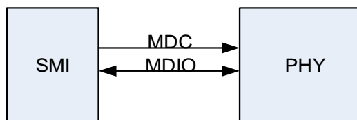
Figure 22-3. Station management interface signals
