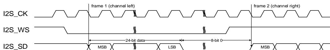
Figure 18-12. I2S Philips standard timing diagram (DTLEN=01, CHLEN=1, CKPL=0)
