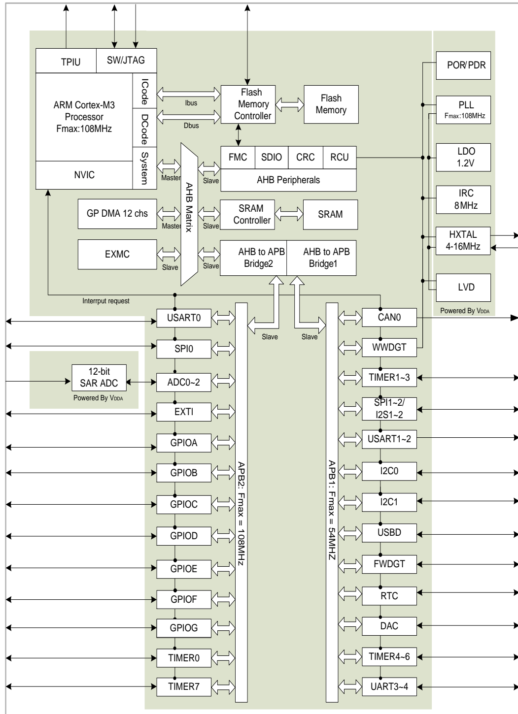
Figure 1-3. GD32F10x High-density series system architecture
