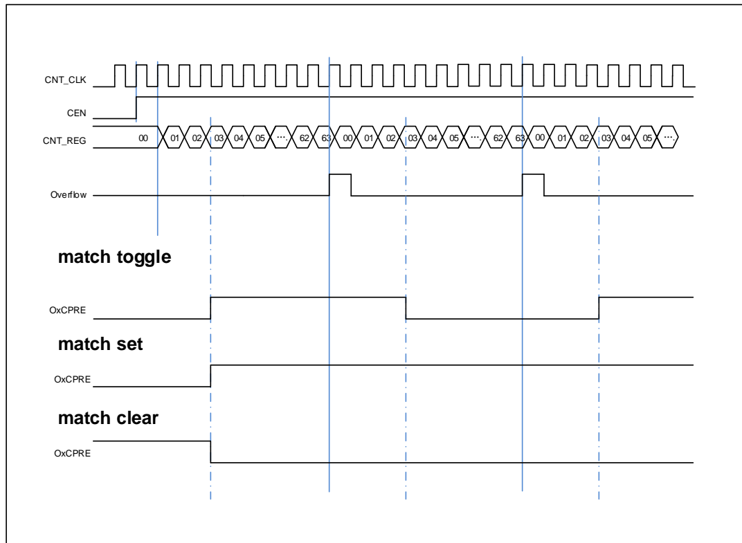
Figure 15-74. Output-compare under three modes
