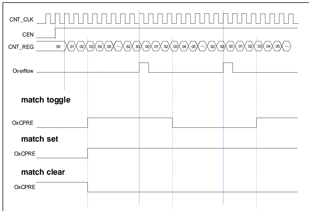
Figure 15-41. Output-compare in three modes
