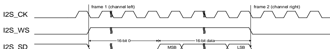
Figure 18-26. LSB justified standard timing diagram (DTLEN=00, CHLEN=1, CKPL=0)
