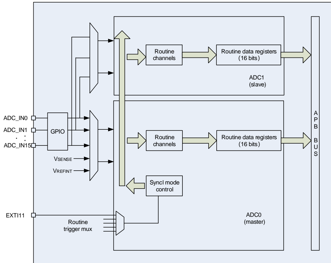
Figure 11-8. ADC sync block diagram
