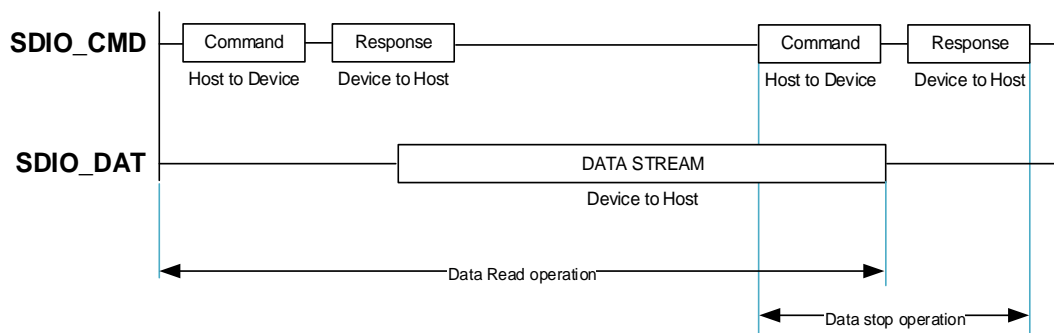
Figure 19-4. SDIO sequential read operation
