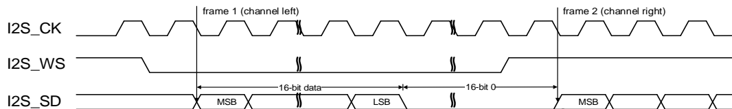
Figure 18-14. I2S Philips standard timing diagram (DTLEN=00, CHLEN=1, CKPL=0)
