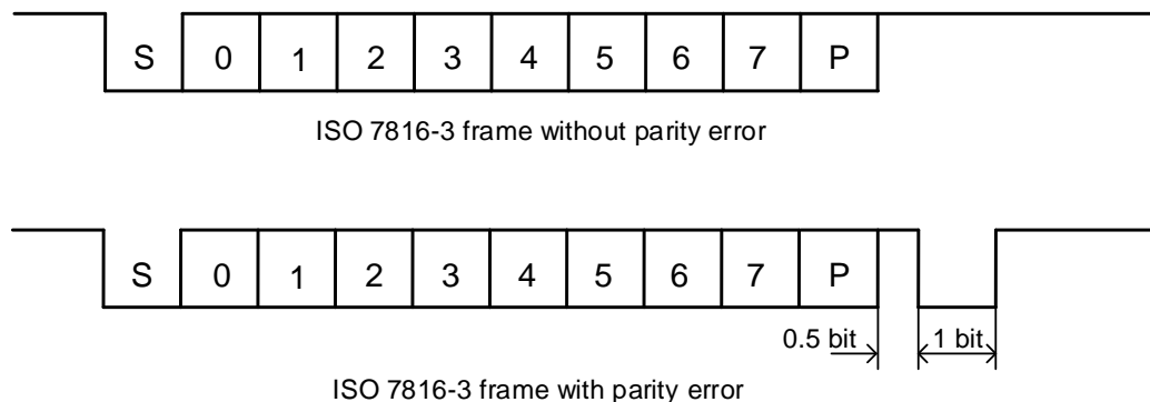
Figure 16-15. ISO7816-3 frame format
