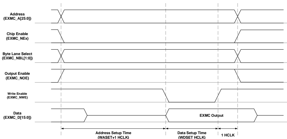
Figure 20-9. Mode A write access
