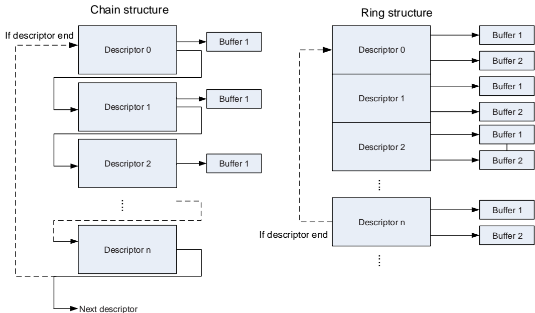
Figure 22-6. Descriptor ring and chain structure
