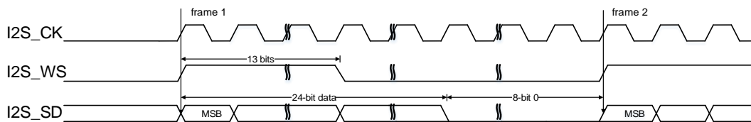
Figure 18-40. PCM standard long frame synchronization mode timing diagram (DTLEN=01, CHLEN=1, CKPL=0)
