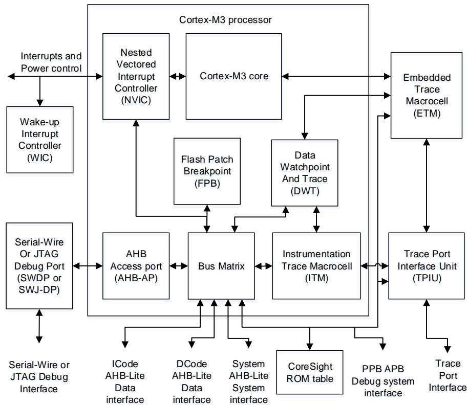
Figure 1-1. The structure of the Cortex®-M3 processor
