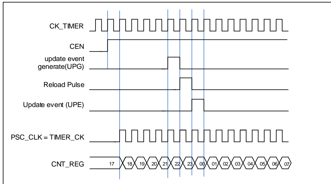
Figure 15-65. Timing chart of internal clock divided by 1
