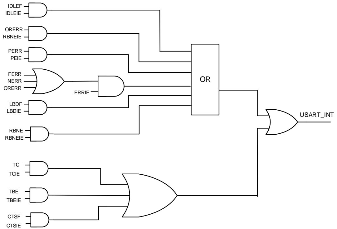
Figure 16-16. USART interrupt mapping diagram
