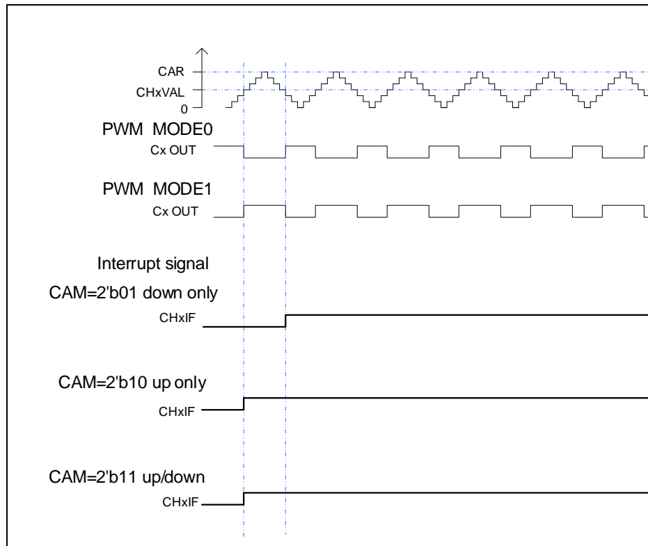
Figure 15-43. CAPWM timechart
