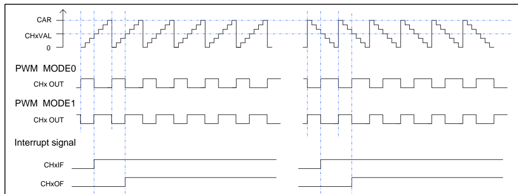
Figure 15-58. EAPWM timechart
