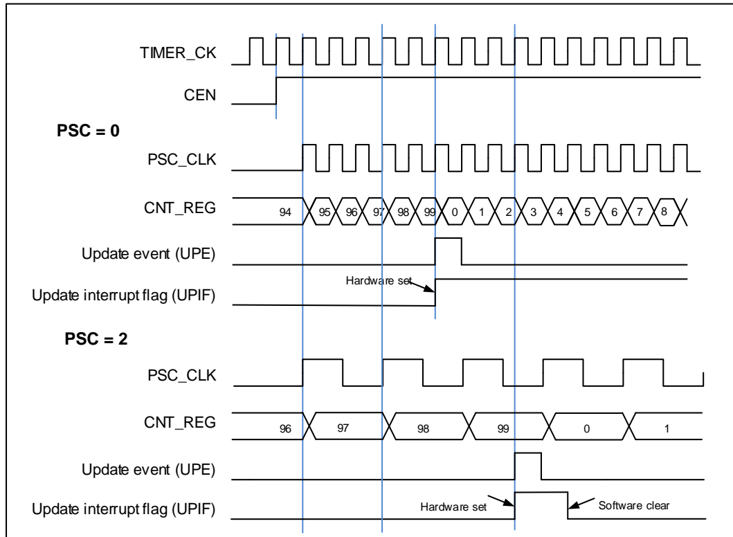
Figure 15-50. Timing chart of up counting mode, PSC=0/2
