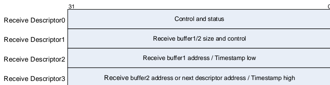
Figure 22-8. Receive descriptor
