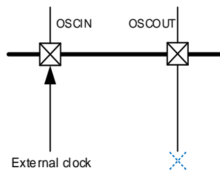
Figure 5-8. HXTAL clock source in bypass mode
