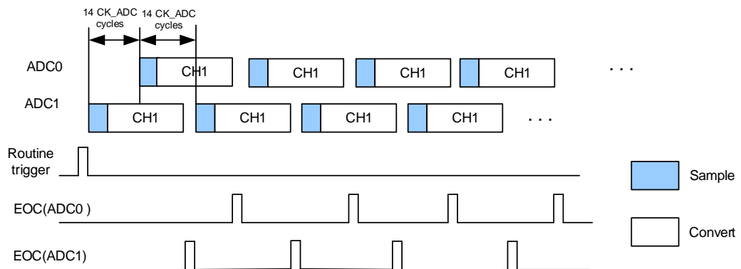
Figure 11-11. Routine follow-up slow mode
