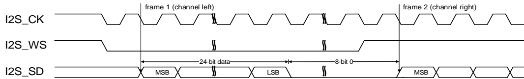
Figure 18-13. I2S Philips standard timing diagram (DTLEN=01, CHLEN=1, CKPL=1)
