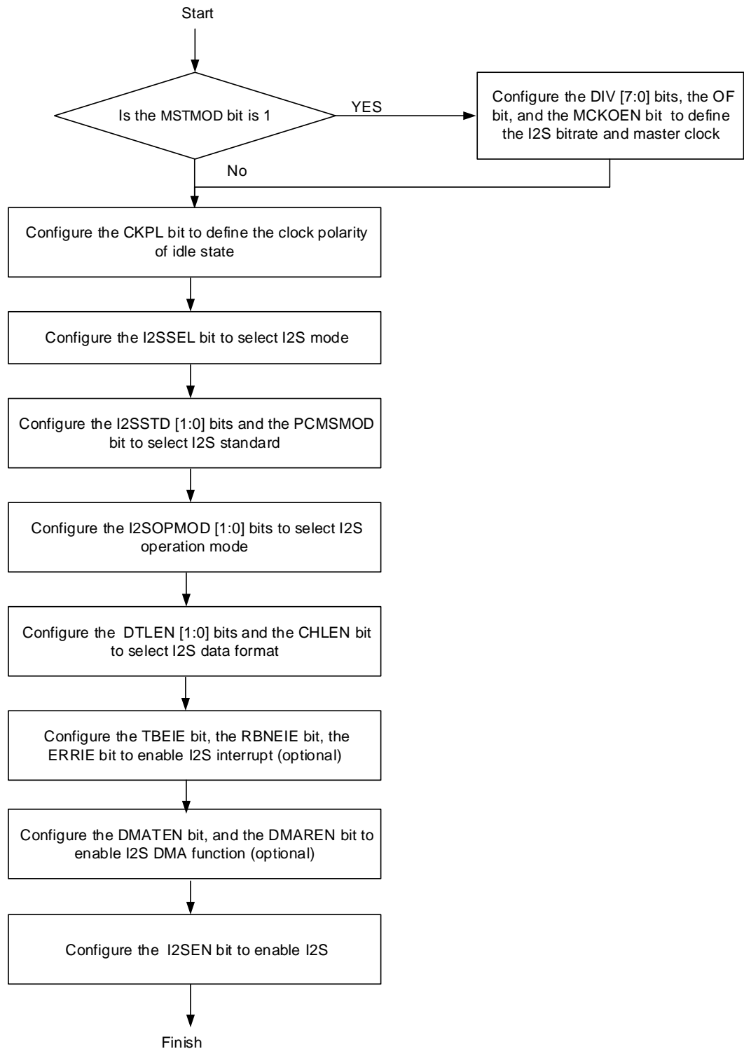
Figure 18-45. I2S initialization sequence
