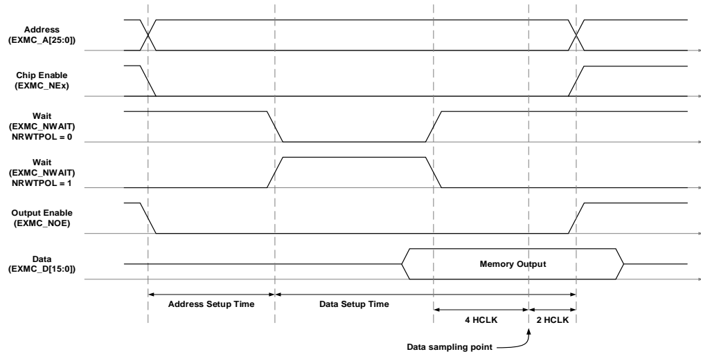
Figure 20-19. Read access timing diagram under async-wait signal assertion
