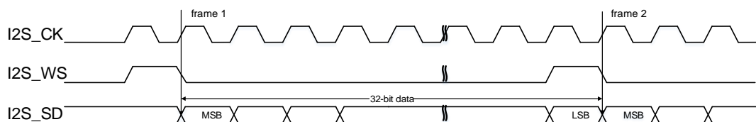
Figure 18-30. PCM standard short frame synchronization mode timing diagram (DTLEN=10, CHLEN=1, CKPL=0)
