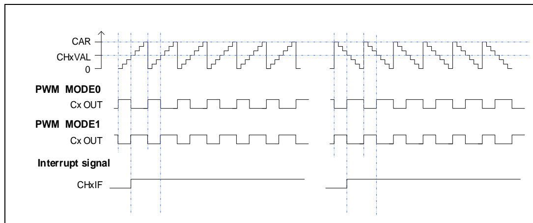
Figure 15-42. EAPWM timechart
