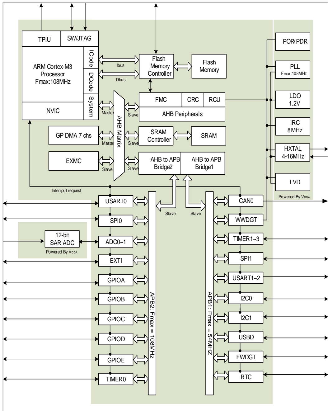
Figure 1-2. GD32F10x Medium-density series system architecture
