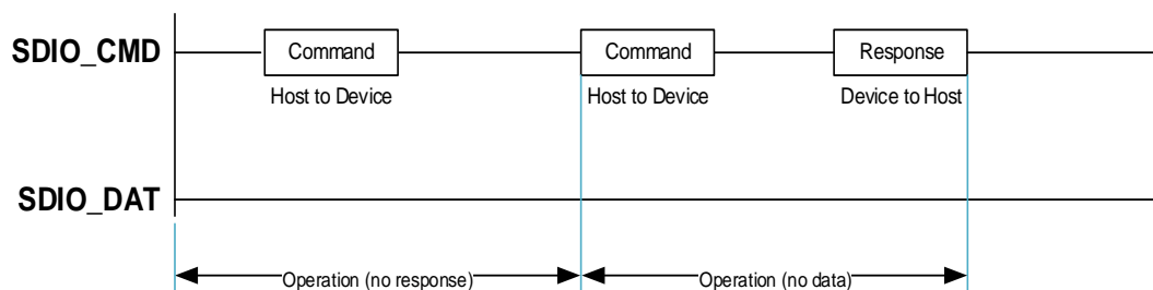
Figure 19-1. SDIO “no response” and “no data” operations
