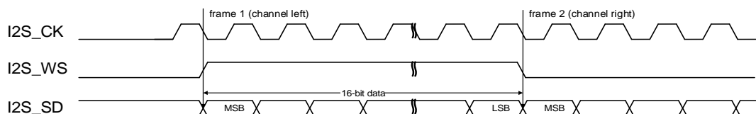
Figure 18-16. MSB justified standard timing diagram (DTLEN=00, CHLEN=0, CKPL=0)
