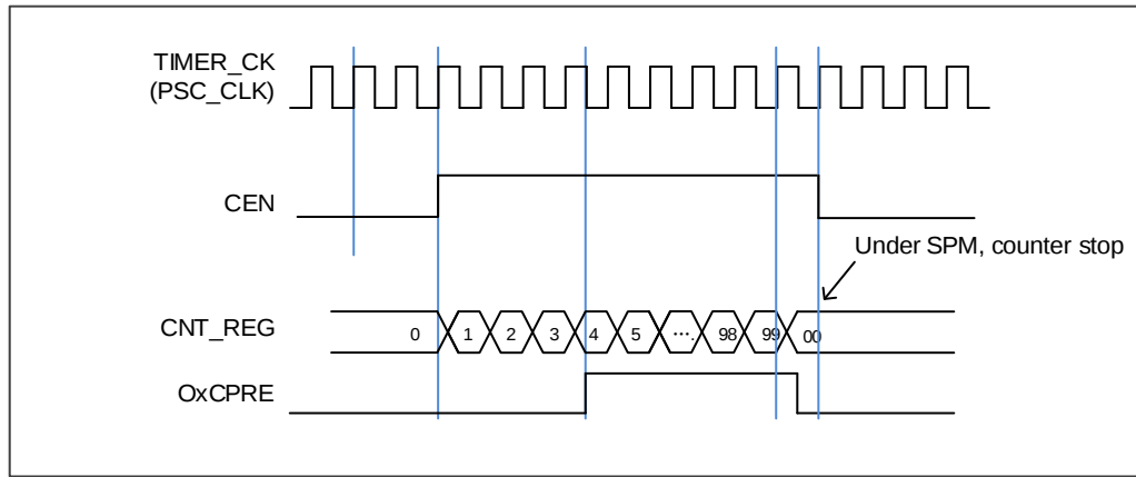
图 18-79. 单脉冲模式, TIMERx\_CHxCV = 4 TIMERx\_CAR = 99
