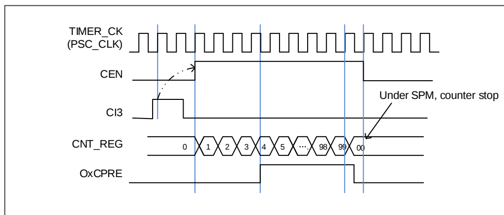
图 18-32. 单脉冲模式, TIMERx_CHxCV = 4 TIMERx_CAR=99
