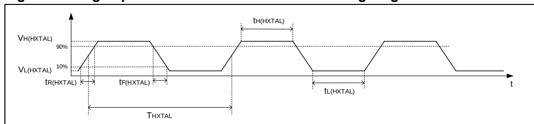
Figure 4-5. High-speed external clock source AC timing diagram
