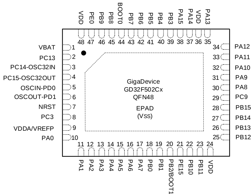
Figure 2-7. GD32F502Cx QFN48 pinouts
