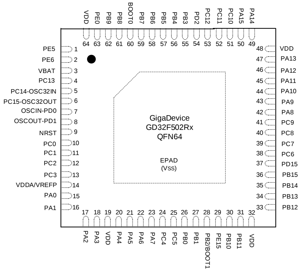
Figure 2-4. GD32F502Rx QFN64 pinouts
