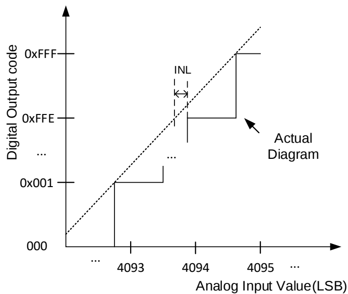
Figure 4-11. Integral linearity error (INL)
