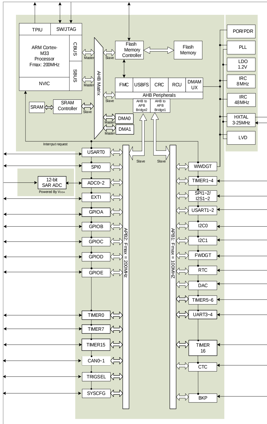
Figure 2-1. GD32F502xx block diagram
