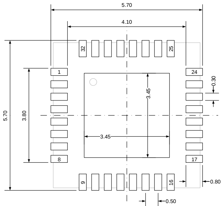
Figure 5-14. QFN32 recommended footprint
