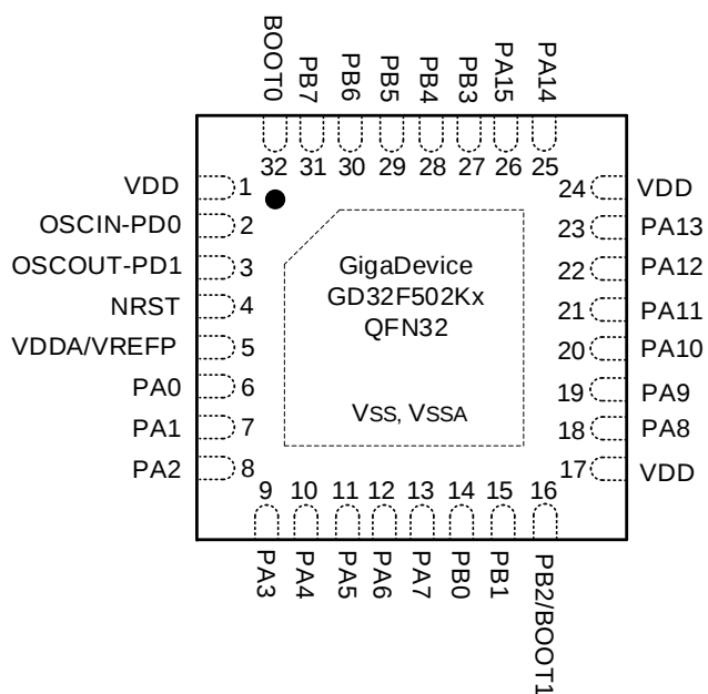
Figure 2-8. GD32F502Kx QFN32 pinouts
