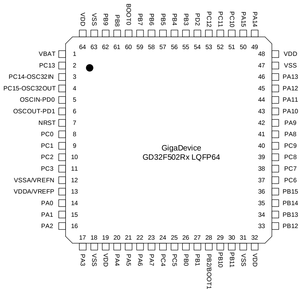
Figure 2-3. GD32F502Rx LQFP64 pinouts
