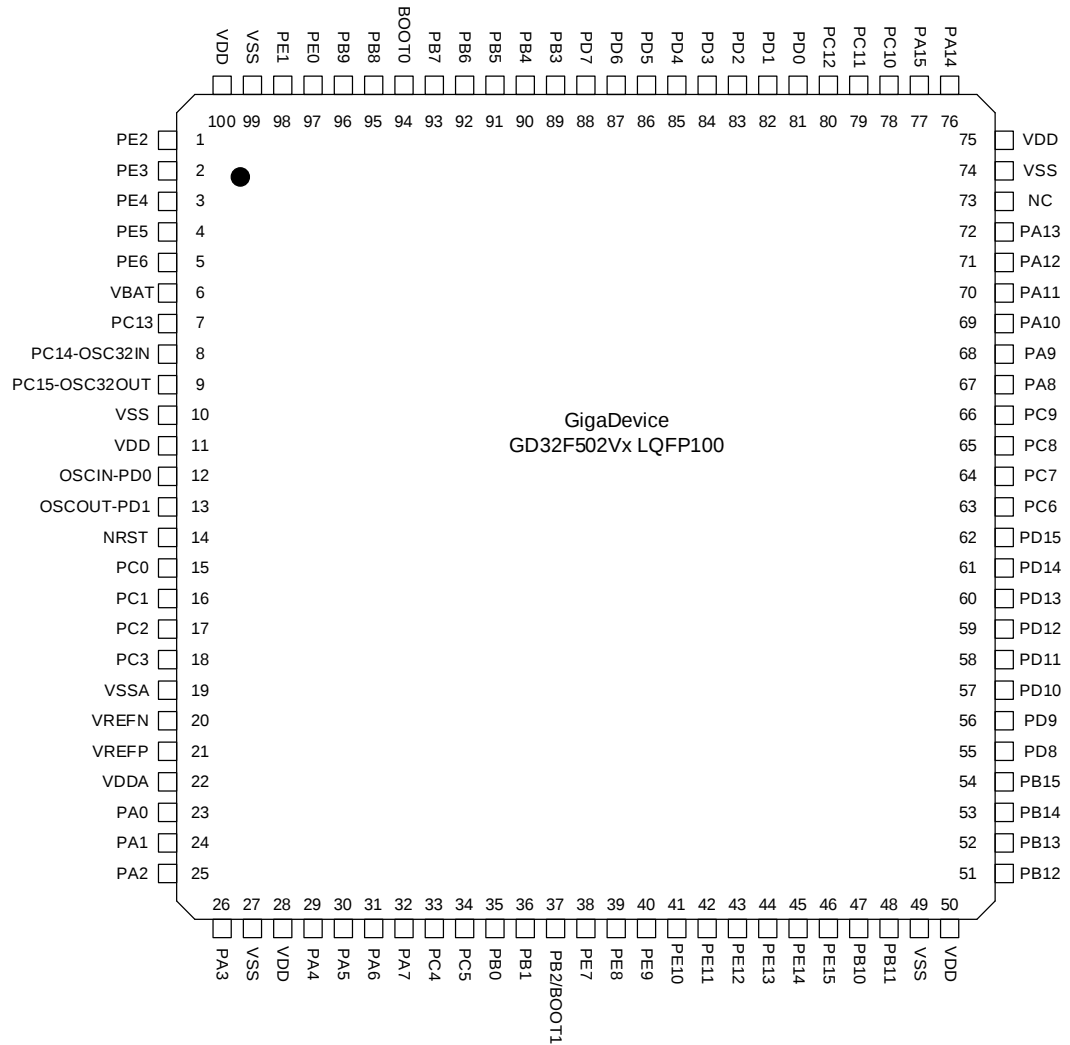
Figure 2-2. GD32F502Vx LQFP100 pinouts
