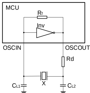
Figure 4-4. Internal structure diagram of OSCIN and OSCOUT pin
