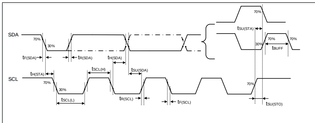
Figure 4-13. I2C bus timing diagram
