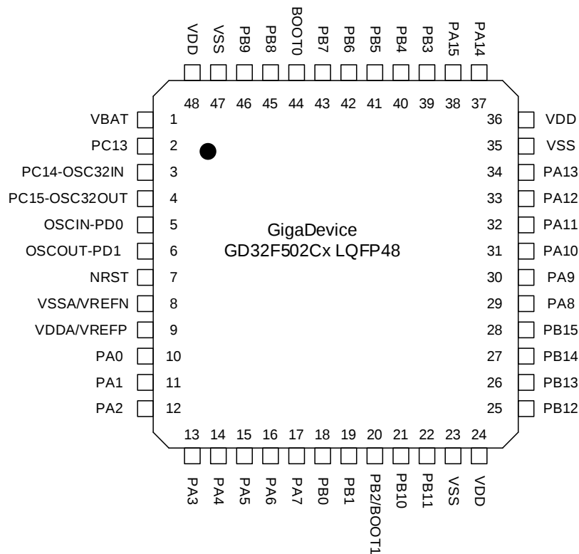
Figure 2-6. GD32F502Cx LQFP48 pinouts
