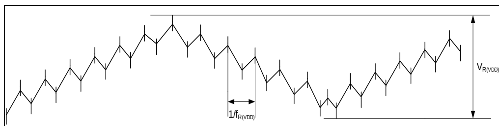
Figure 4-2. Rise and fall gradient and ripple frequency characteristics
