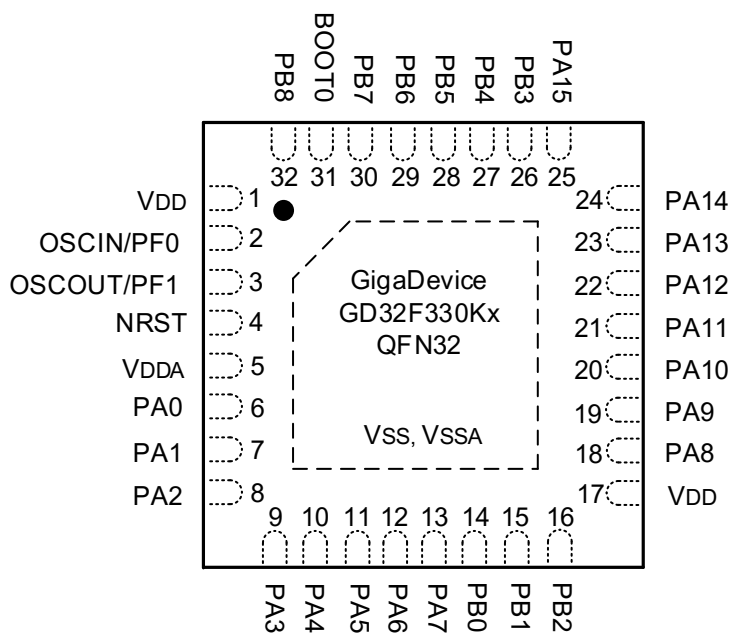
Figure 2-5. GD32F330Kx QFN32 pinouts
