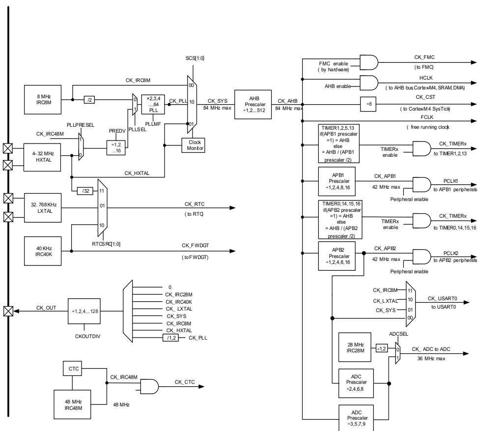
Figure 2-8. GD32F330xx clock tree
