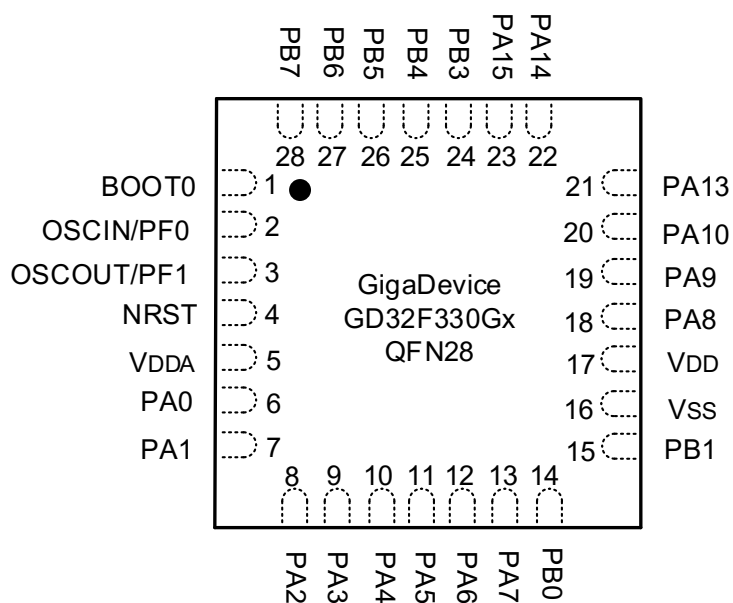
Figure 2-6. GD32F330Gx QFN28 pinouts
