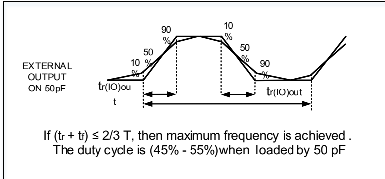
Figure 4-5. I/O port AC characteristics definition
