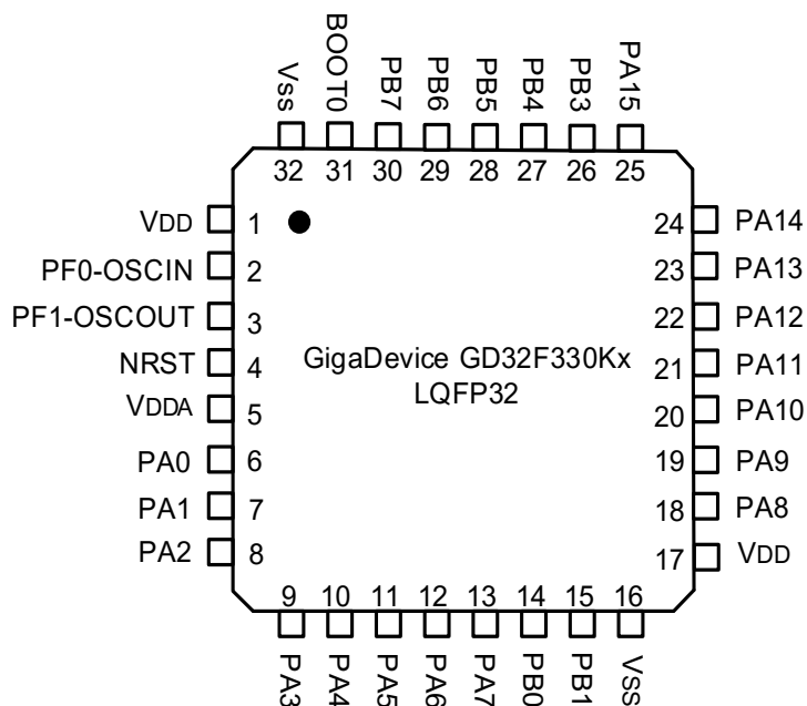
Figure 2-4. GD32F330Kx LQFP32 pinouts
