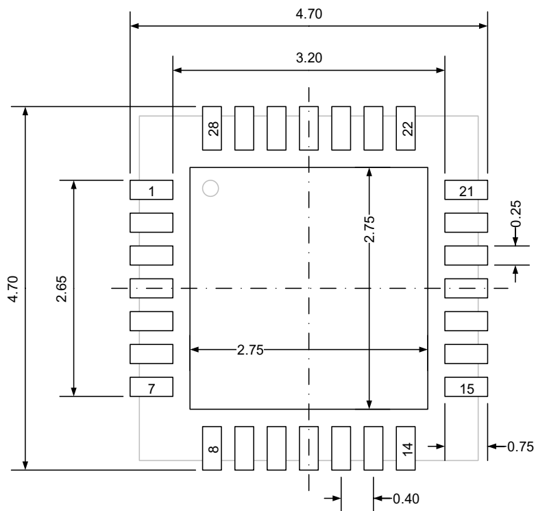
Figure 5-10. QFN28 recommended footprint
