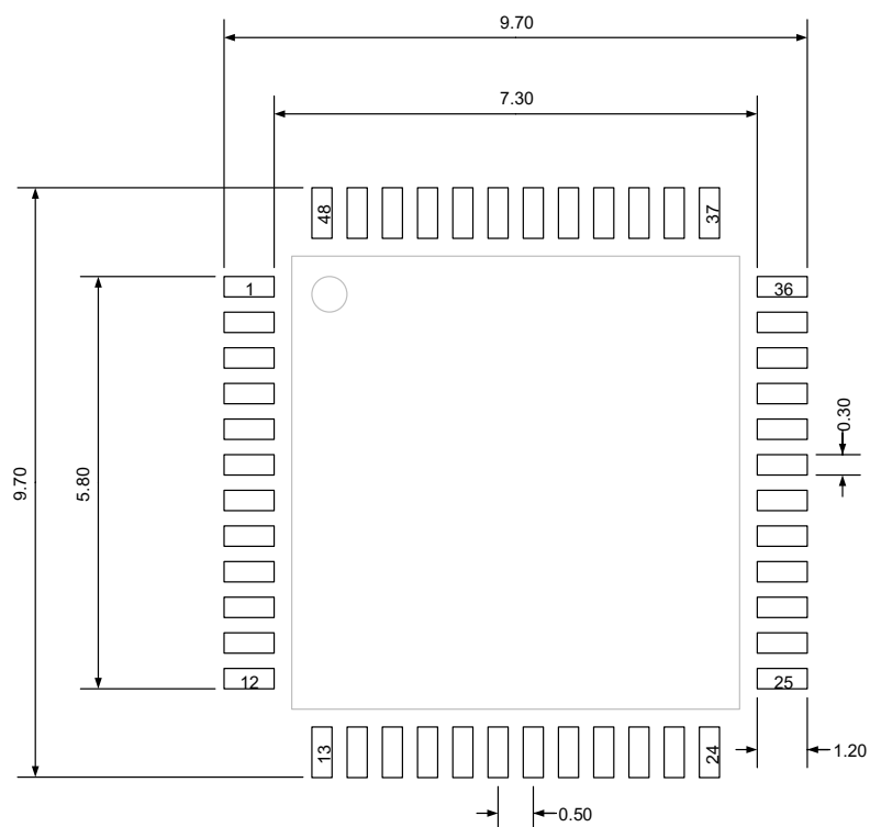
Figure 5-4. LQFP48 recommended footprint
