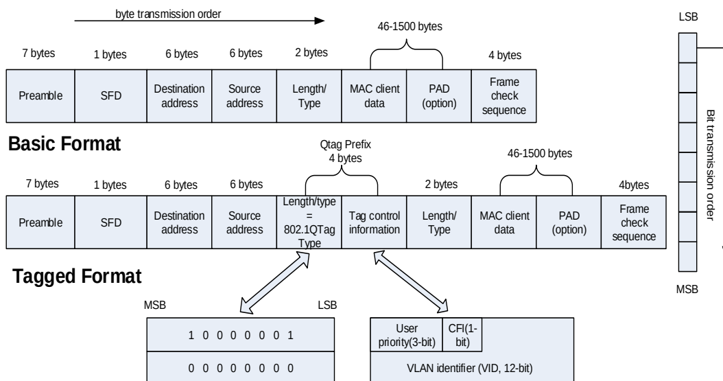
Figure 23-2. MAC/Tagged MAC frame format
