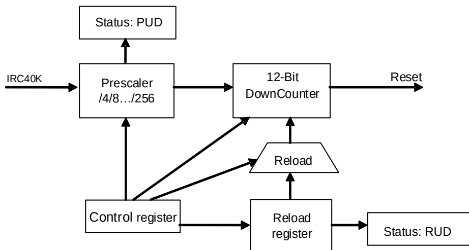
Figure 14-1. Free watchdog block diagram
