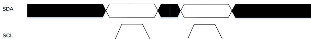
Figure 18-2. Data validation
