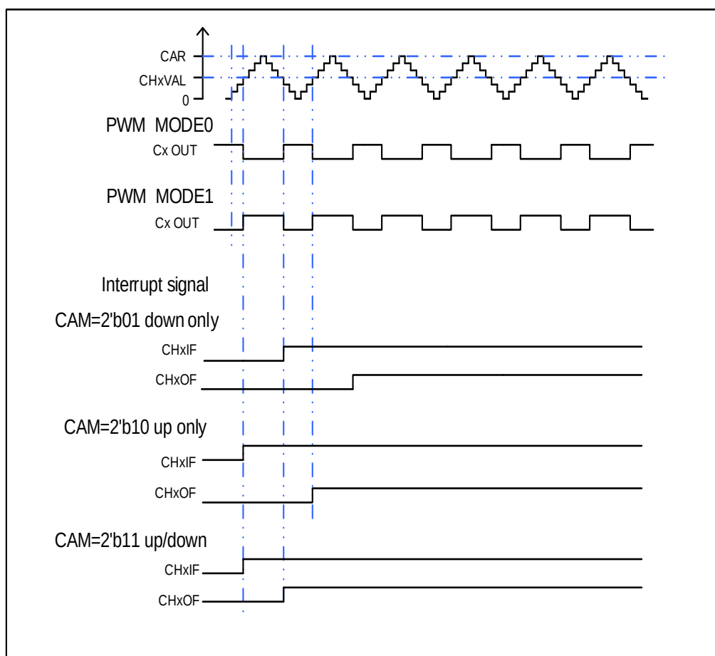
Figure 16-40. CAPWM timechart
