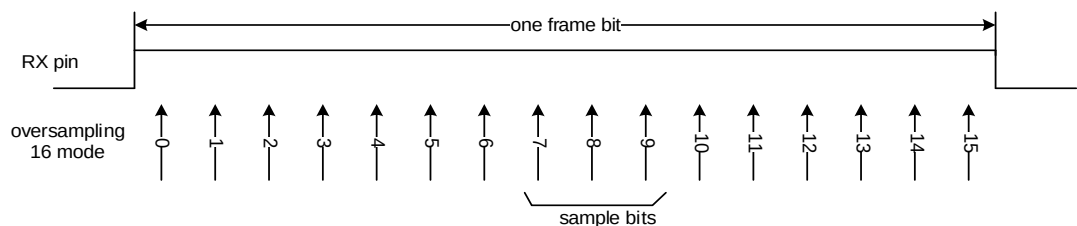
Figure 17-4. Receiving a frame bit by oversampling method
