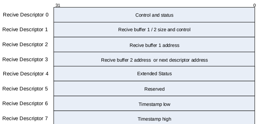
Figure 23-10. Receive descriptor in enhanced mode
