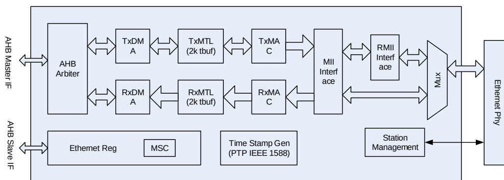
Figure 23-1. ENET module block diagram
