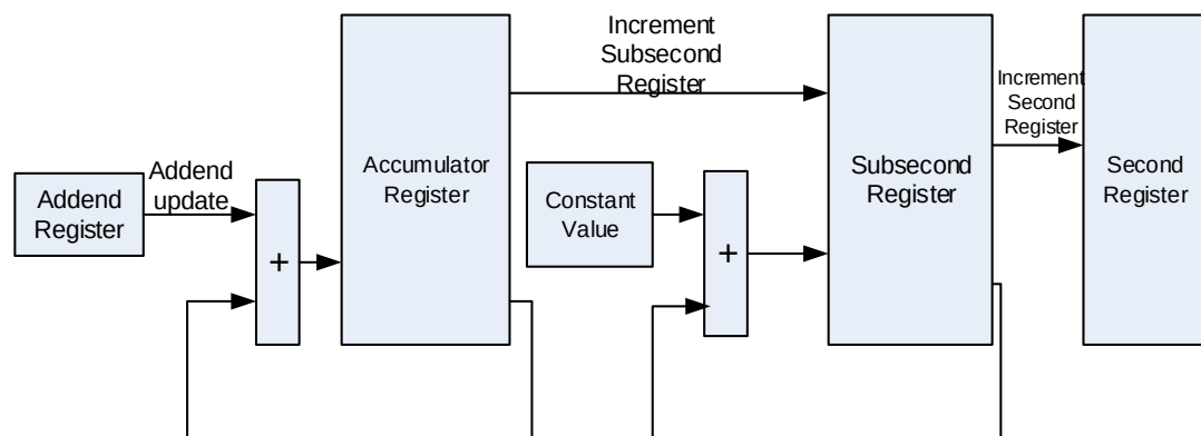
Figure 23-12. System time update using the fine correction method
