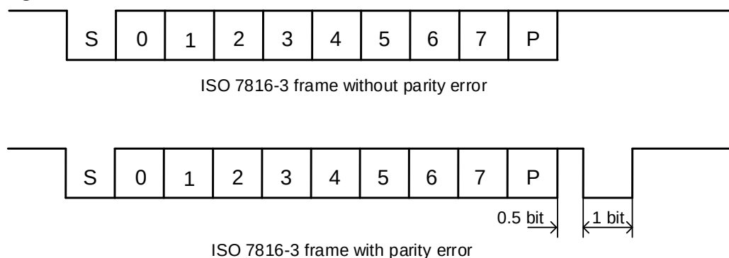
Figure 17-15. ISO7816-3 frame format
