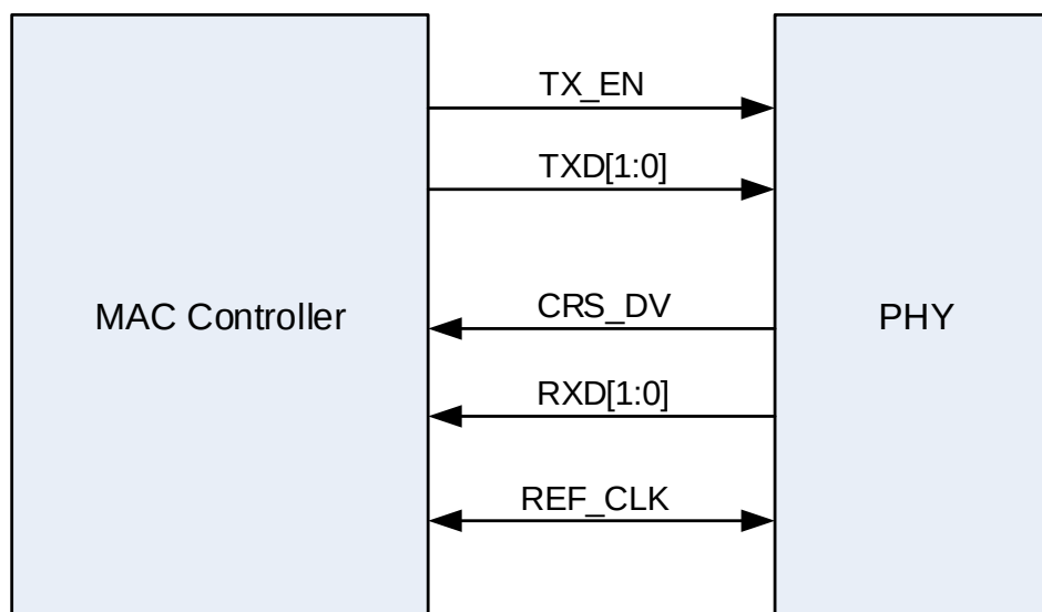
Figure 23-5. Reduced media-independent interface signals
