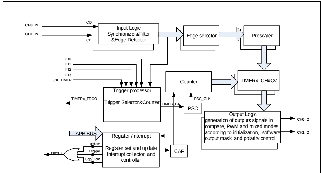
Figure 16-44. General level1 timer block diagram
