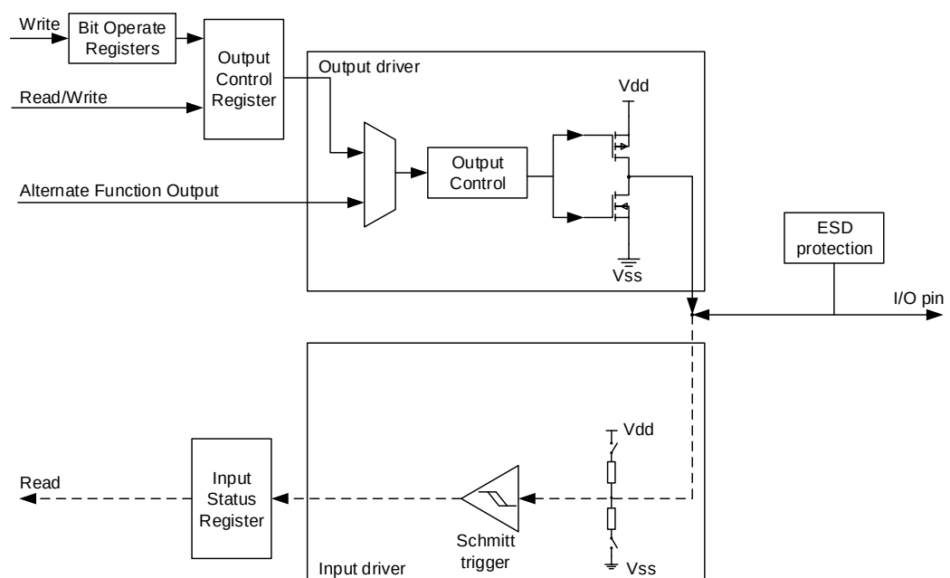
Figure 8-3. Output configuration
