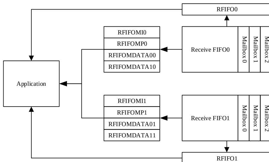
Figure 22-4. Reception register
