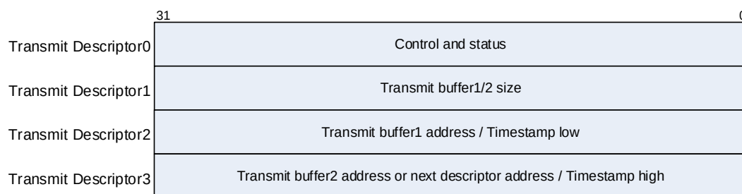
Figure 23-7. Transmit descriptor in normal mode
