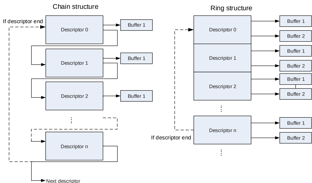
Figure 23-6. Descriptor ring and chain structure
