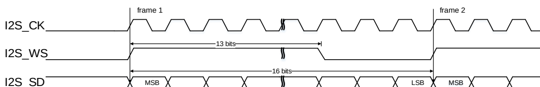
Figure19-44. PCM standard long frame synchronization mode timing diagram
