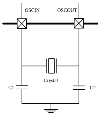
Figure 5-7. HXTAL clock source
