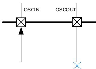
Figure 5-8. HXTAL clock source in bypass mode
