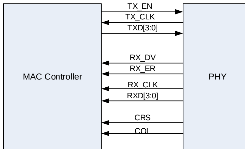
Figure 23-4. Media independent interface signals
