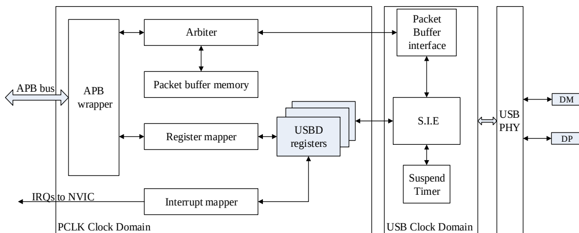
Figure 24-1. USB D block diagram
