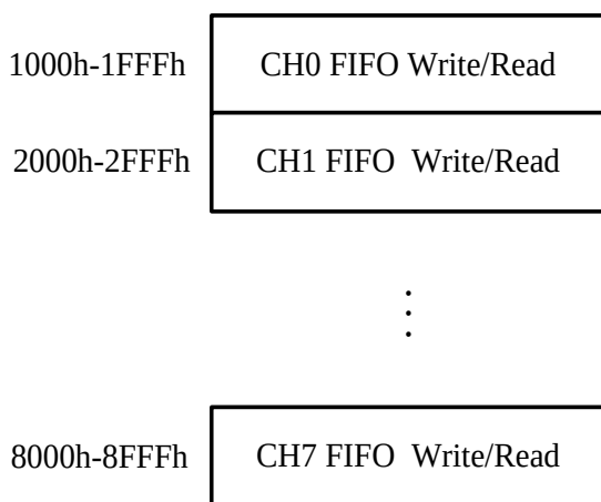
Figure 25-6. Host mode FIFO access register map
