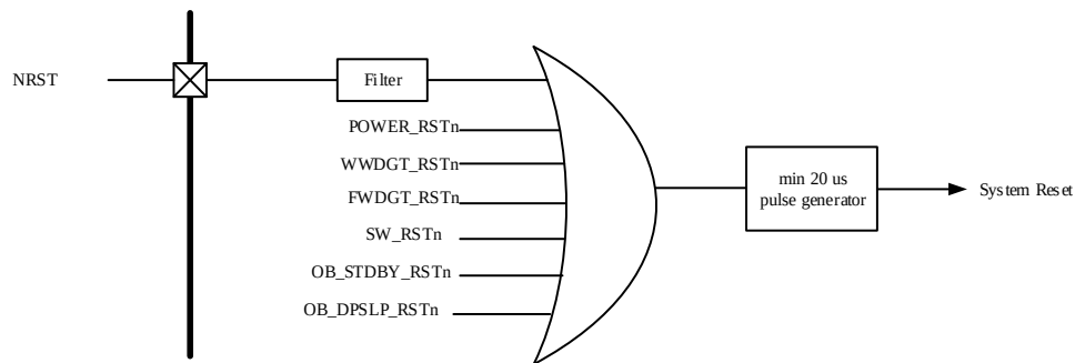
Figure 5-5. The system reset circuit
