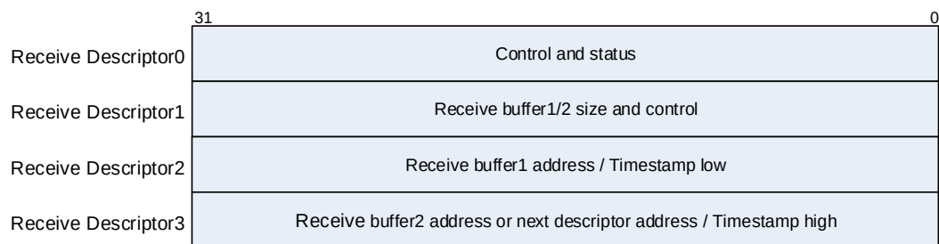
Figure 23-9. Receive descriptor in normal mode
