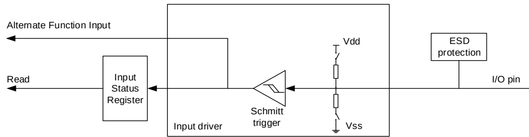
Figure 8-2. Input configuration
