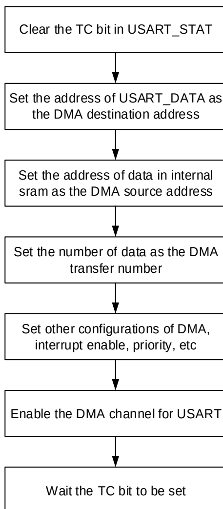
Figure 17-5. Configuration step when using DMA for USART transmission
