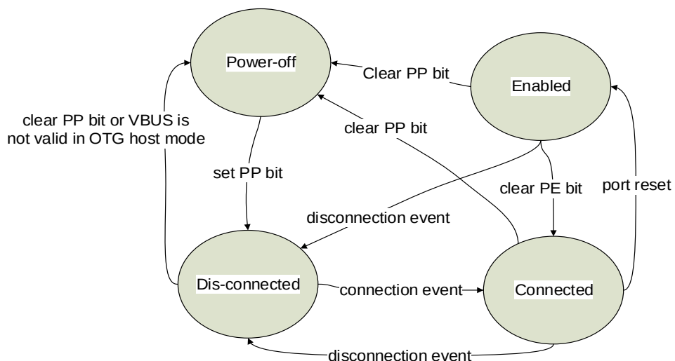
Figure 25-4. State transition diagram of host port
