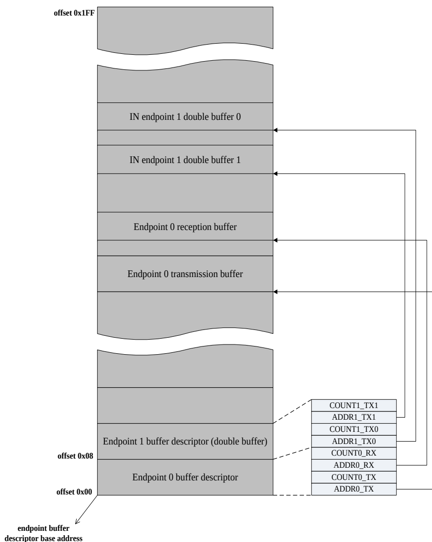
Figure 24-2. an example with buffer descriptor table usage (USB_D_BADDR = 0)
