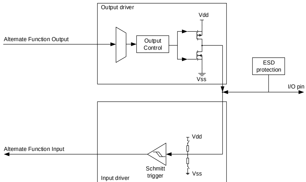
Figure 8-5. Alternate function configuration
