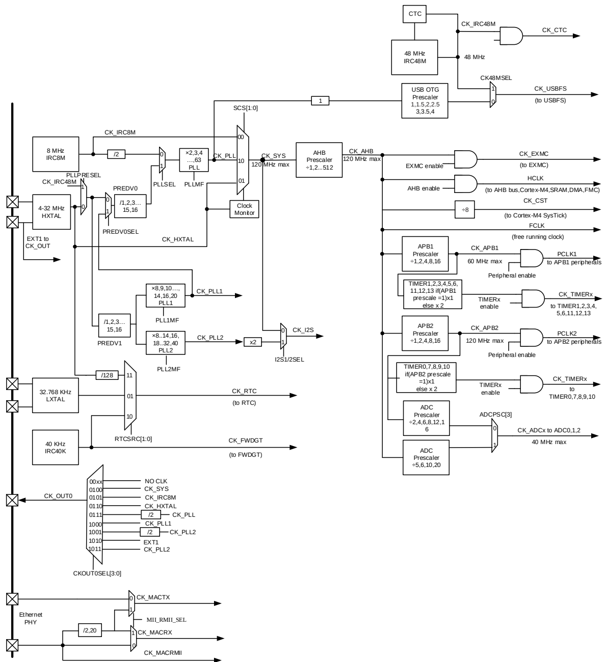
Figure 5-6. Clock tree
