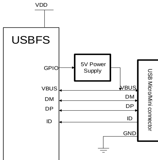
Figure 25-3. Connection with OTG mode
