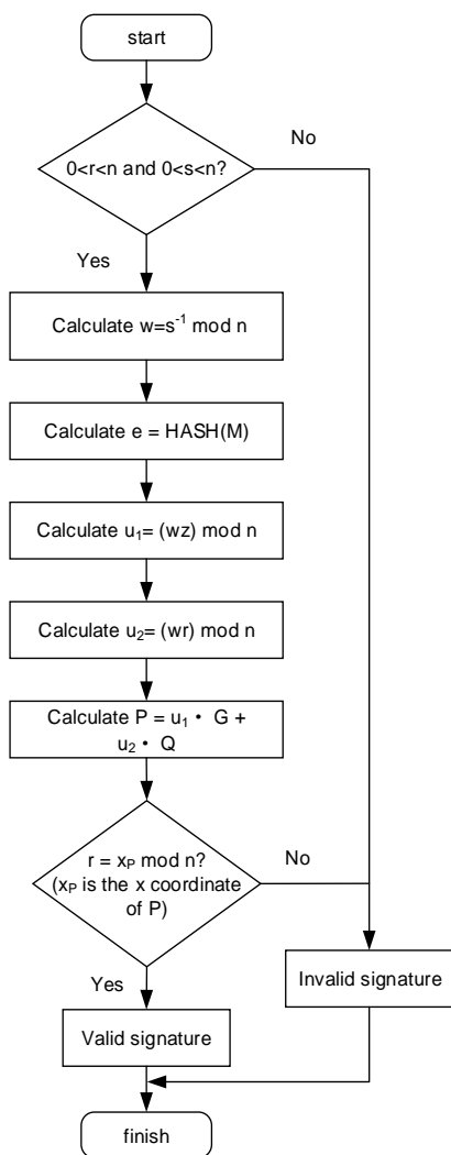
Figure 29-4. Flow chart of ECDSA verification
