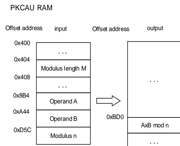
Figure 29-14. Montgomery multiplication
