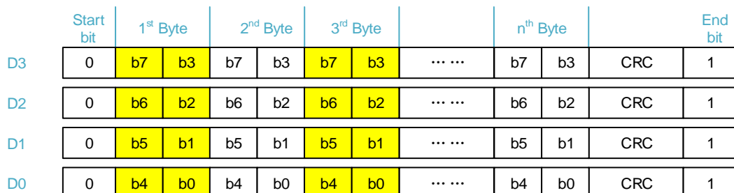
Figure 23-10. 4-bit data bus width
