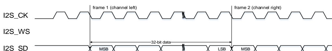
Figure 20-16. I2S Phillips standard timing diagram (DTLEN=10, CHLEN=1, CKPL=0)
