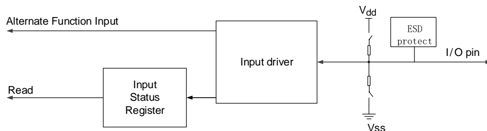
Figure 8-2. Basic structure of Input configuration
