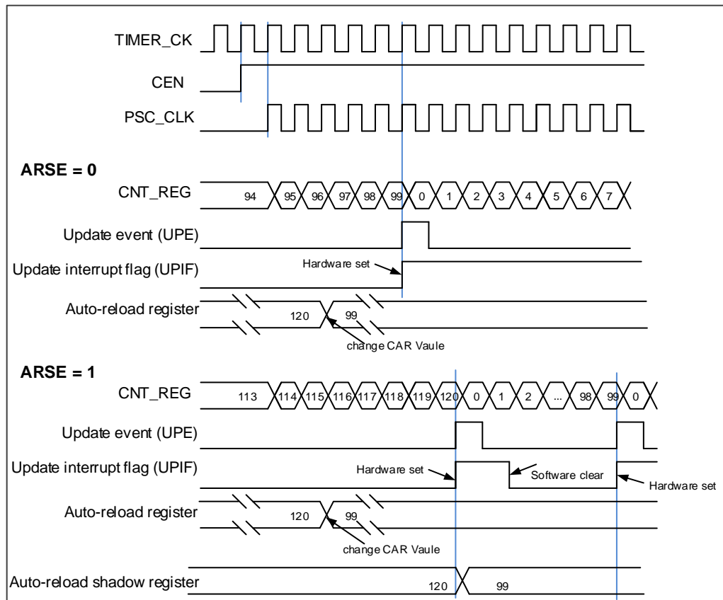
Figure 17-55. Up-counter timechart, change TIMERx_CAR on the go
