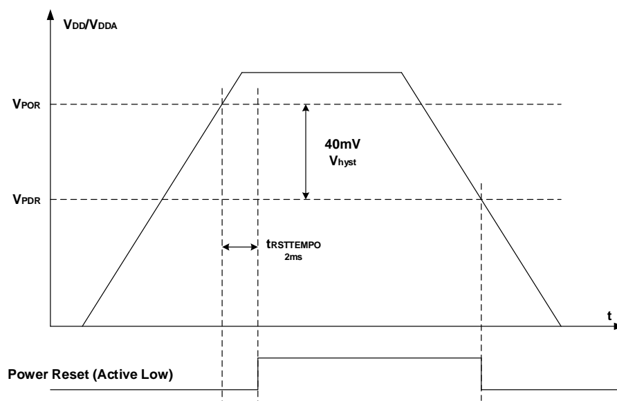
Figure 5-2. Waveform of the POR / PDR
