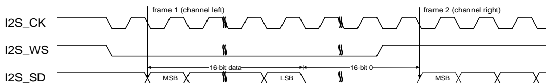
Figure 20-21. I2S Phillips standard timing diagram (DTLEN=00, CHLEN=1, CKPL=1)
