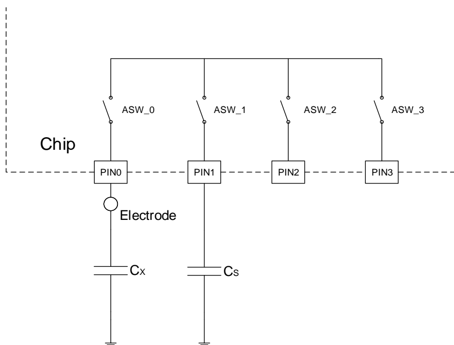
Figure 26-2. Block diagram of sample pin and channel pin
