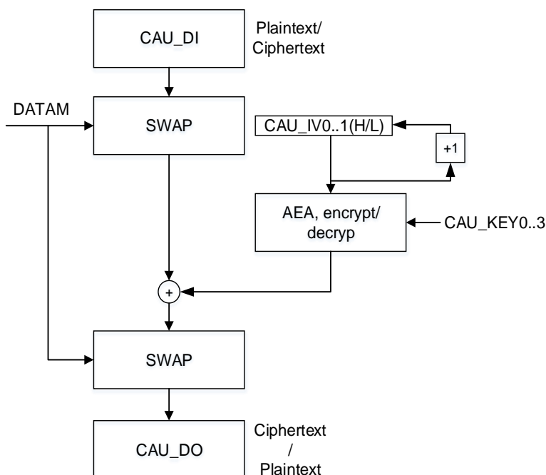
Figure 27-13. AES CTR encryption/decryption
