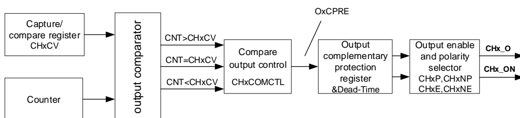
Figure 17-58. Channel output compare principle (with complementary output, x=0)
