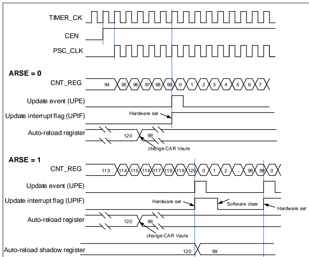
Figure 17-5. Timing chart of up counting mode, change TIMERx_CAR ongoing
