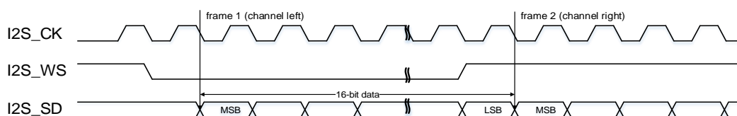
Figure 20-14. I2S Phillips standard timing diagram (DTLEN=00, CHLEN=0, CKPL=0)
