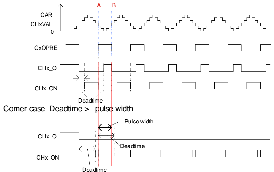
Figure 17-18. Complementary output with dead-time insertion.
