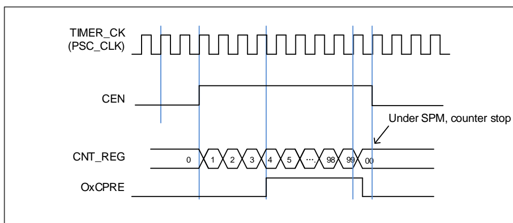
Figure 17-63. Single pulse mode TIMERx_CHxCV = 0x04 TIMERx_CAR=0x60
