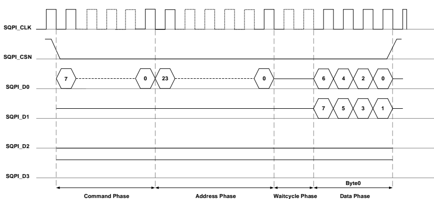
Figure 21-9. SQPI SSD Mode Timing
