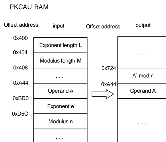
Figure 29-15. Modular exponentiation of normal mode
