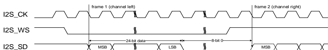
Figure 20-18. I2S Phillips standard timing diagram (DTLEN=01, CHLEN=1, CKPL=0)
