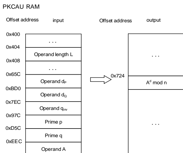
Figure 29-18. RSA CRT exponentiation
