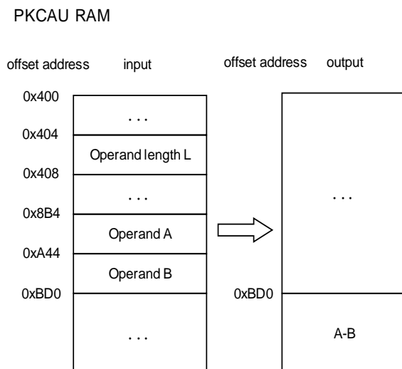
Figure 29-6. Arithmetic subtraction
