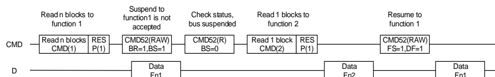
Figure 23-14. Function2 read cycle inserted during function1 multiple read cycle
