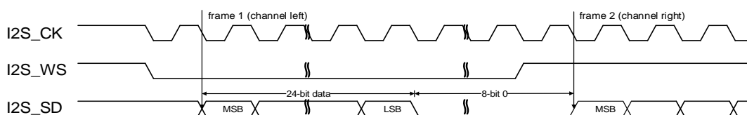
Figure 20-19. I2S Phillips standard timing diagram (DTLEN=01, CHLEN=1, CKPL=1)
