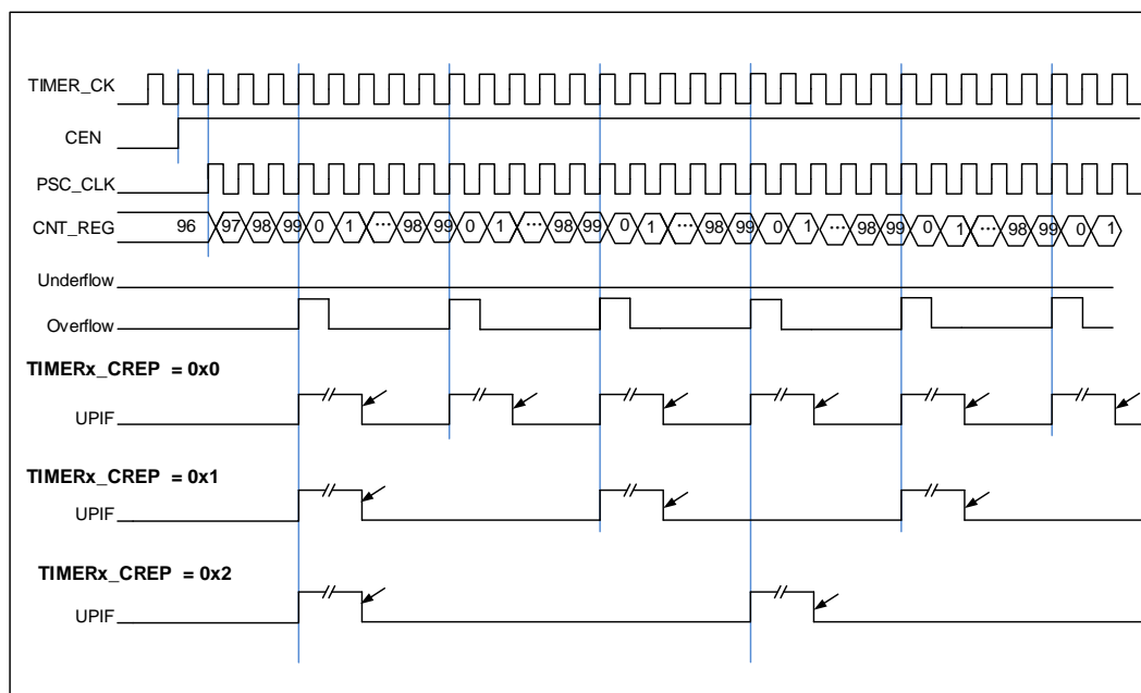
Figure 17-56. Repetition timechart for up-counter
