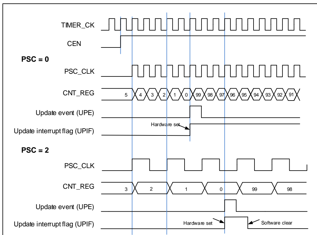
Figure 17-6. Timing chart of down counting mode, \text{PSC}=0/2
