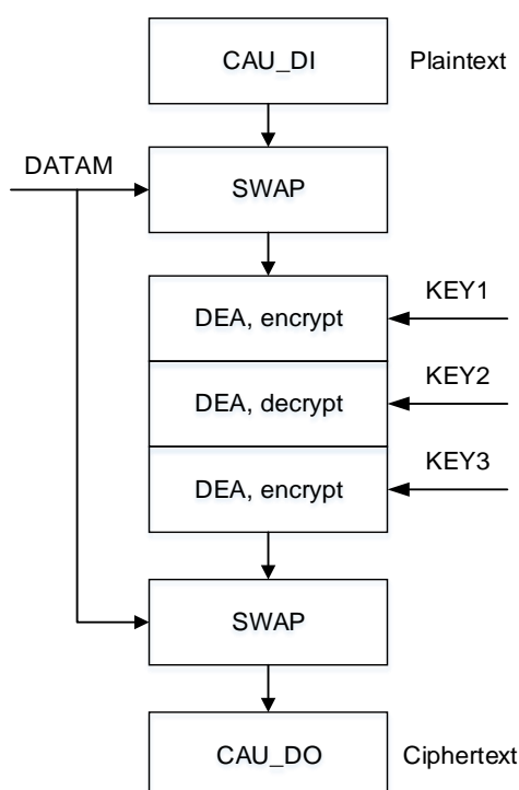
Figure 27-4. DES/TDES ECB encryption
