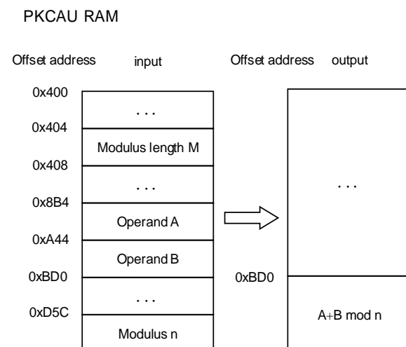
Figure 29-10. Modular addition
