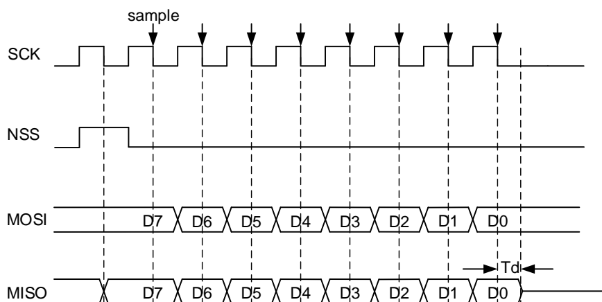
Figure 20-10. Timing diagram of TI slave mode
