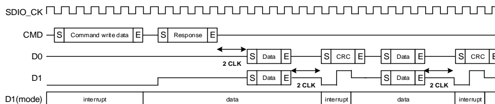
Figure 23-18. Multiple block 4-Bit write interrupt cycle timing
