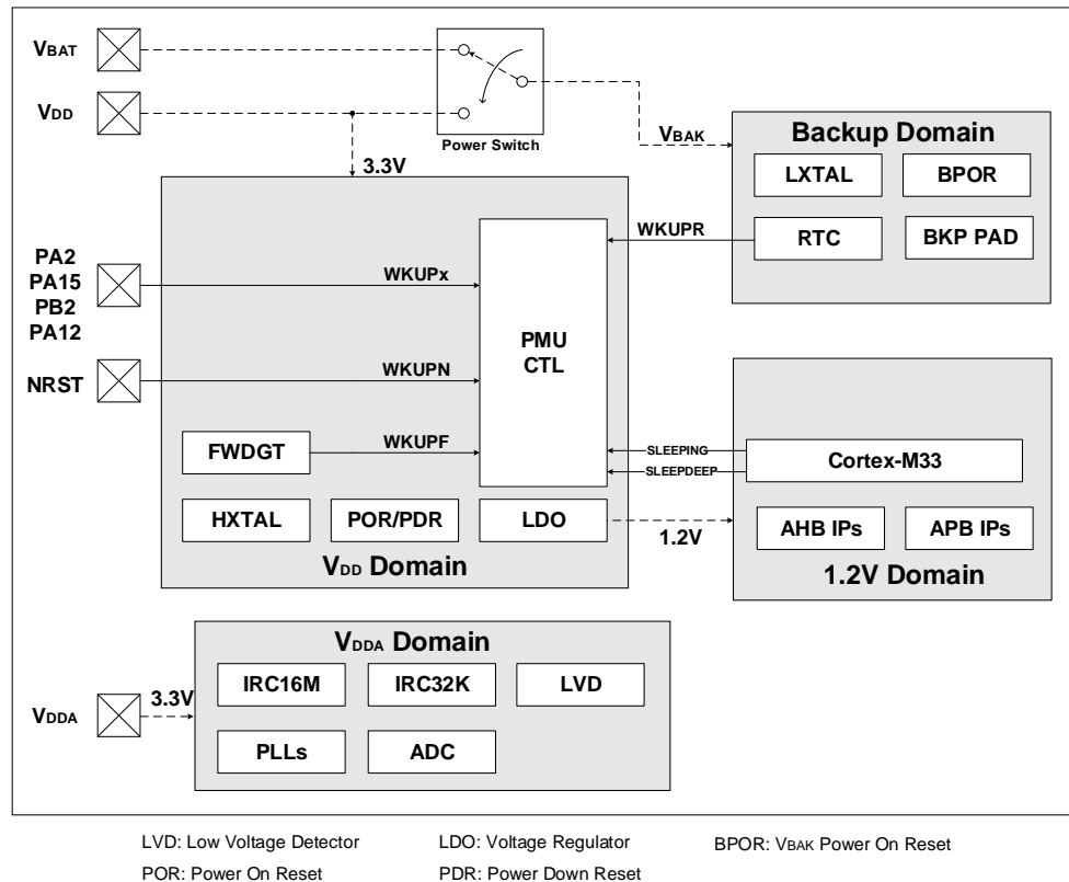
Figure 5-1. Power supply overview
