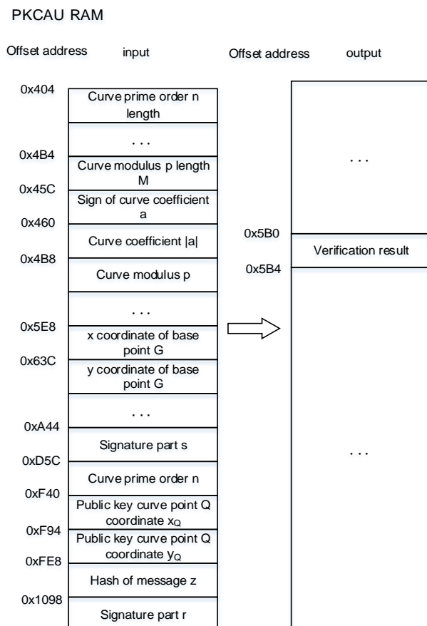
Figure 29-23. ECDSA verification
