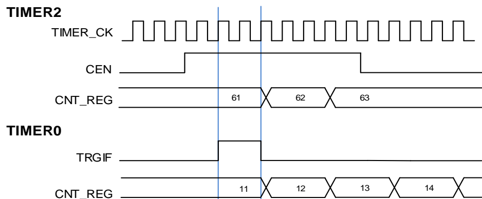
Figure 17-29. Trigger mode of TIMER0 controlled by enable signal of TIMER2
