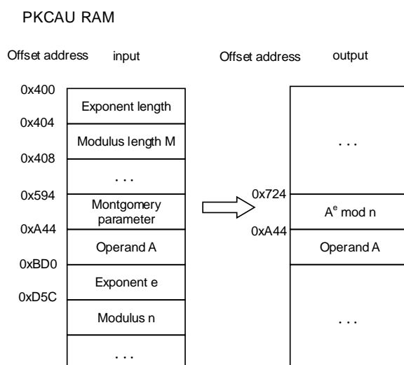
Figure 29-16. Modular exponentiation of fast mode
