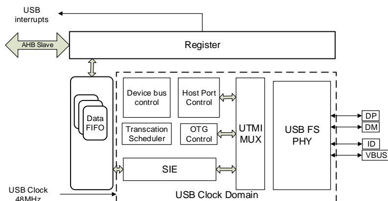
Figure 24-1. USBFS block diagram
