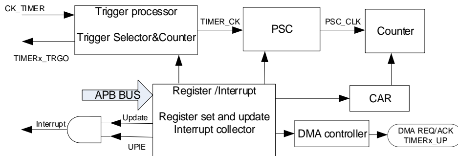
Figure 17-64. Basic timer block diagram
