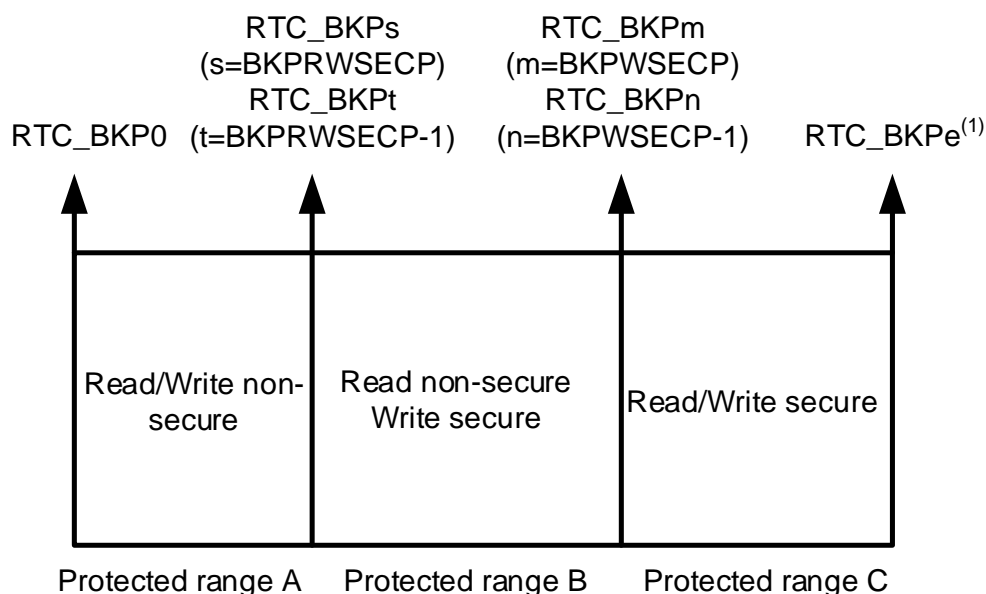
Figure 16-2. Backup registers secure protections configuration
