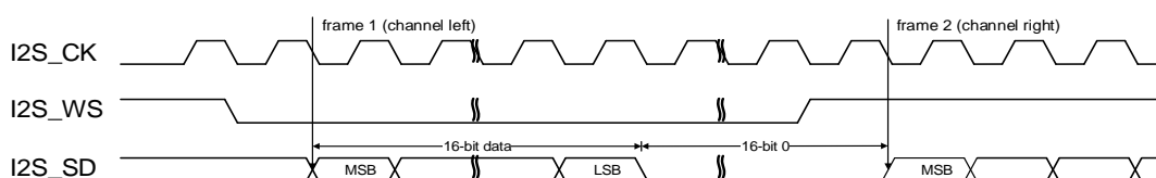
Figure 20-20. I2S Phillips standard timing diagram (DTLEN=00, CHLEN=1, CKPL=0)
