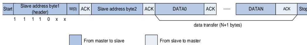
Figure 19-4. I2C communication flow with 10-bit address (Master Transmit)
