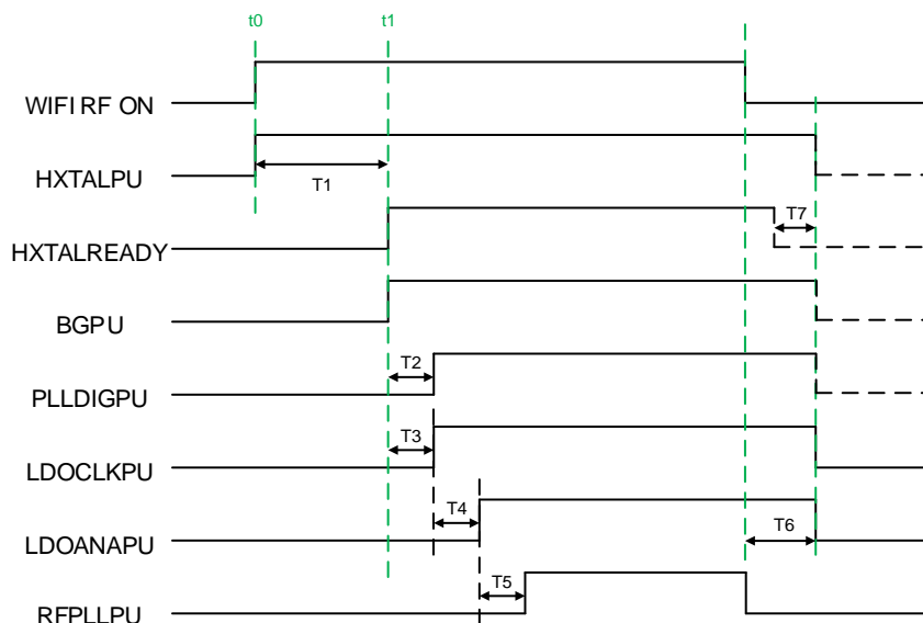
Figure 5-4. RF sequence
