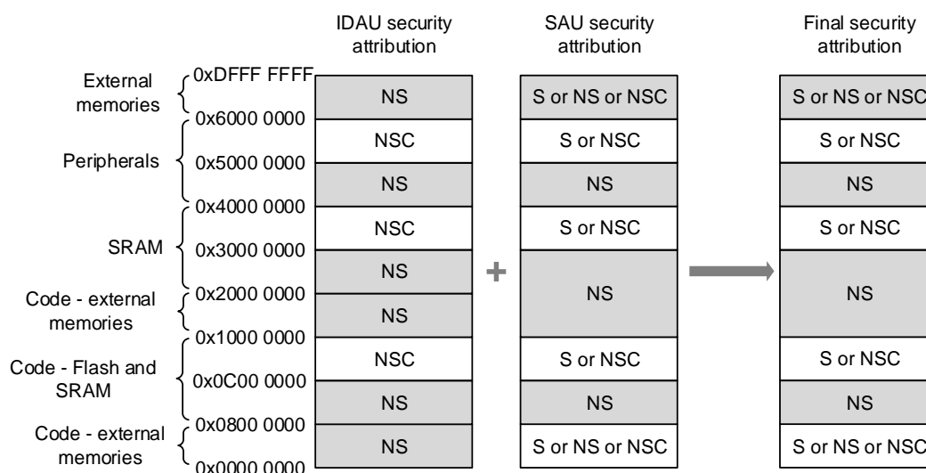
Figure 1-3. Example of memory map security attribution vs SAU configuration regions
