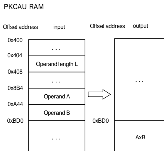
Figure 29-7. Arithmetic multiplication
