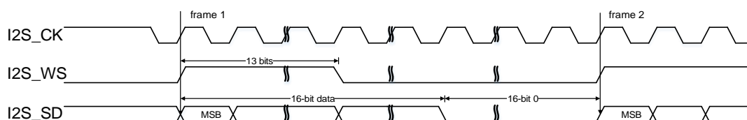
Figure 20-49. PCM standard long frame synchronization mode timing diagram (DTLEN=00, CHLEN=1, CKPL=1)
