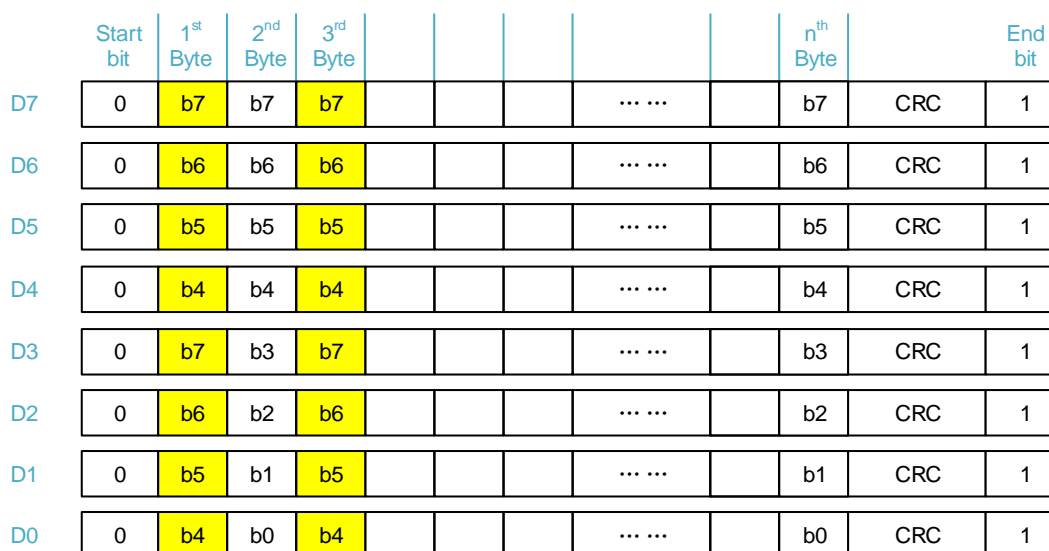
Figure 23-11. 8-bit data bus width
