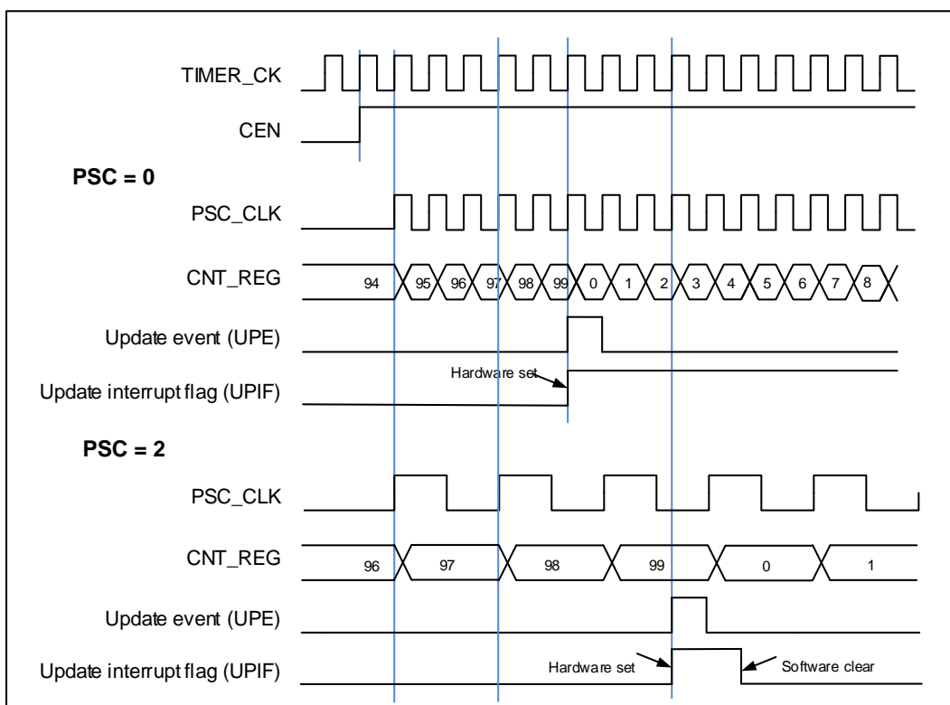
Figure 17-37. Timing chart of up counting mode, PSC=0/2
