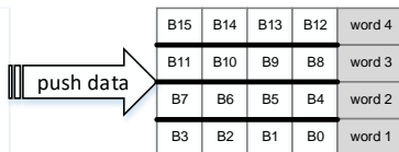
Figure 12-4. Data packing/unpacking when PWIDTH = '00'
