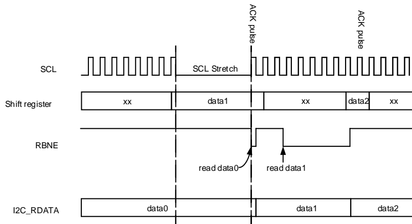
Figure 19-12. Data reception
