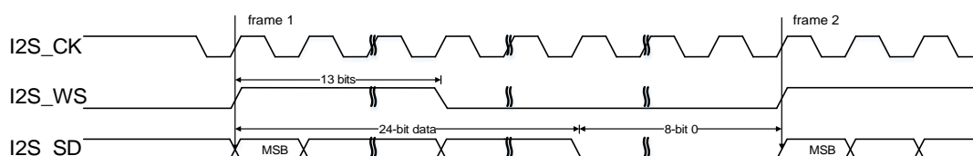
Figure 20-47. PCM standard long frame synchronization mode timing diagram (DTLEN=01, CHLEN=1, CKPL=1)
