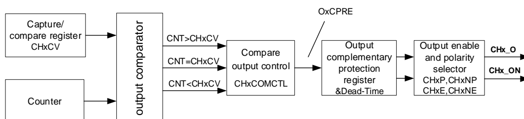
Figure 17-13. Channel output compare principle (with complementary output, x=0,1,2)
