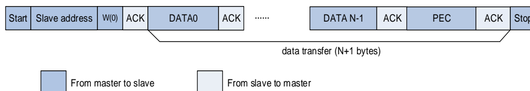
Figure 19-22. SMBus master transmitter and slave receiver communication flow
