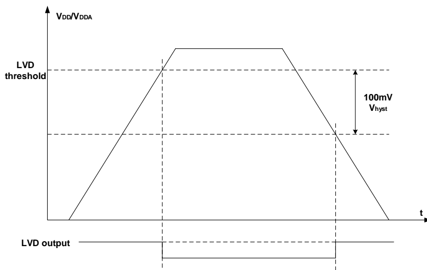
Figure 5-3. Waveform of the LVD threshold
