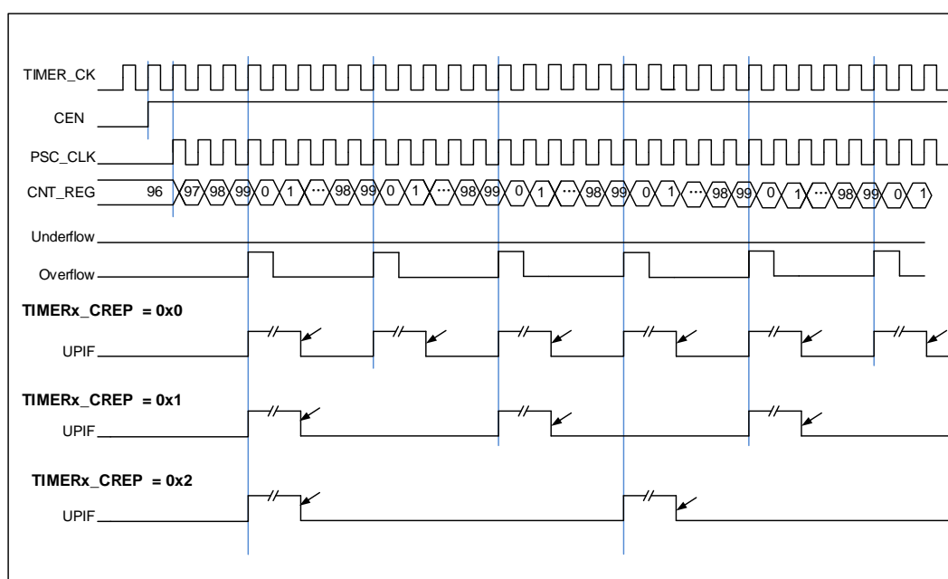
Figure 17-10. Repetition timechart for up-counter
