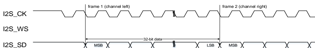
Figure 20-17. I2S Phillips standard timing diagram (DTLEN=10, CHLEN=1, CKPL=1)
