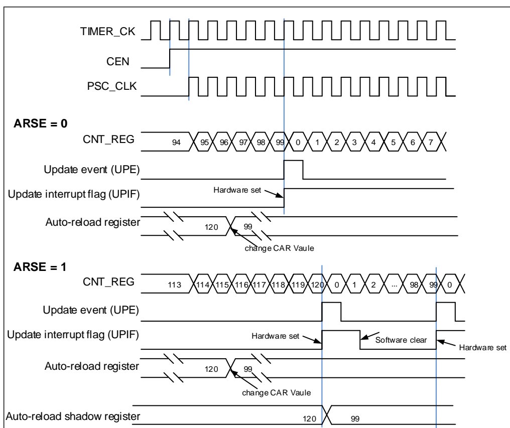
Figure 17-38. Timing chart of up counting mode, change TIMERx_CAR ongoing
