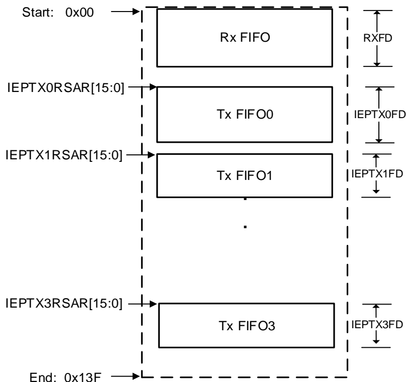
Figure 24-7. Device mode FIFO space in SRAM
