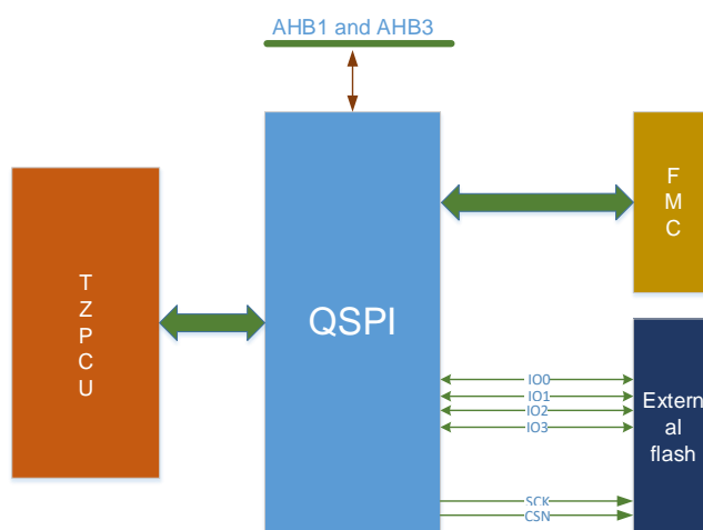
Figure 22-1. QSPI diagram
