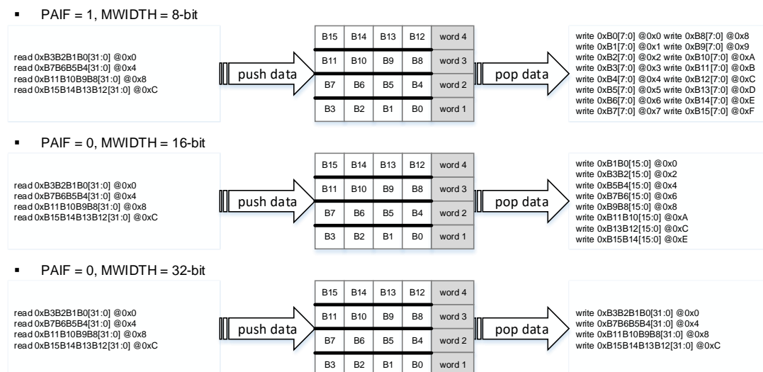
Figure 12-6. Data packing/unpacking when PWIDTH = '10'
