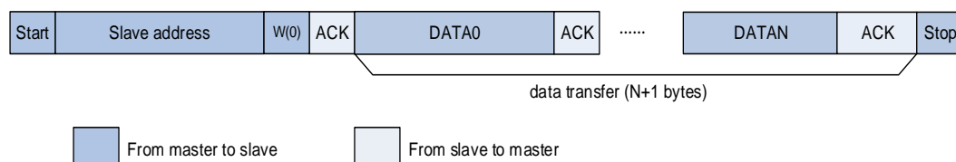
Figure 19-5. I2C communication flow with 7-bit address (Master Transmit)
