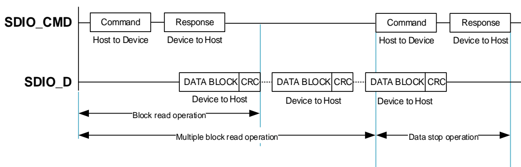
Figure 23-2. SDIO multiple blocks read operation
