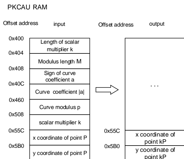
Figure 29-20. ECC scalar multiplication of normal mode
