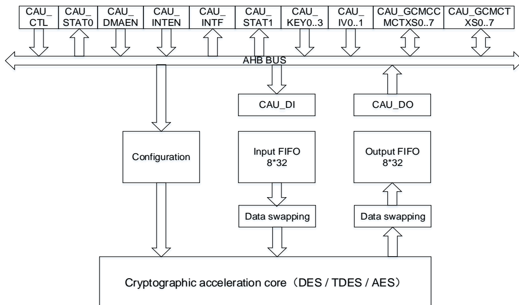
Figure 27-3. CAU diagram
