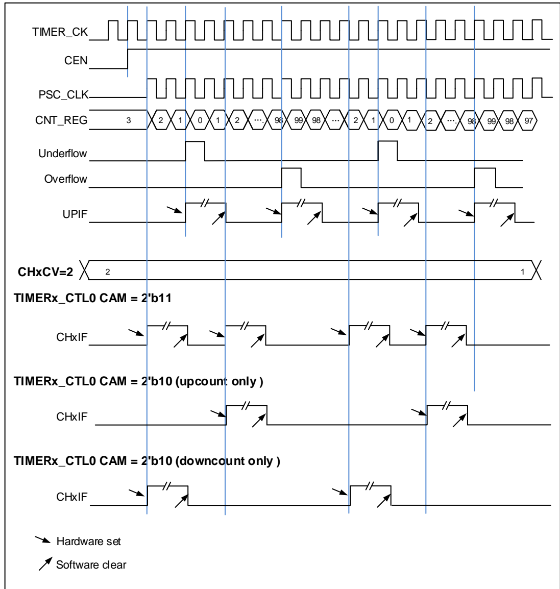
Figure 17-8. Timing chart of center-aligned counting mode
