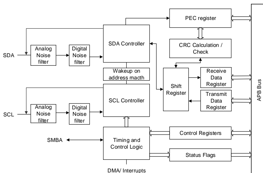
Figure 19-1. I2C module block diagram
