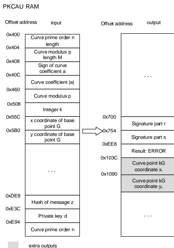
Figure 29-22. ECDSA sign
