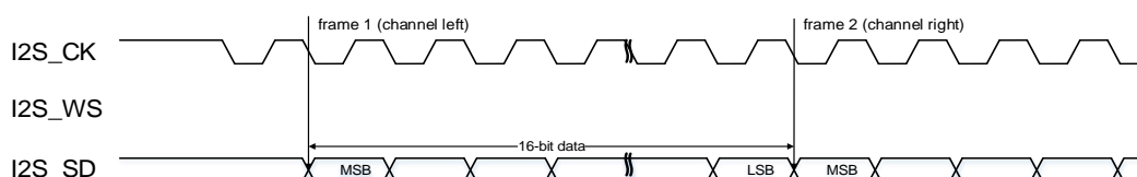
Figure 20-15. I2S Phillips standard timing diagram (DTLEN=00, CHLEN=0, CKPL=1)
