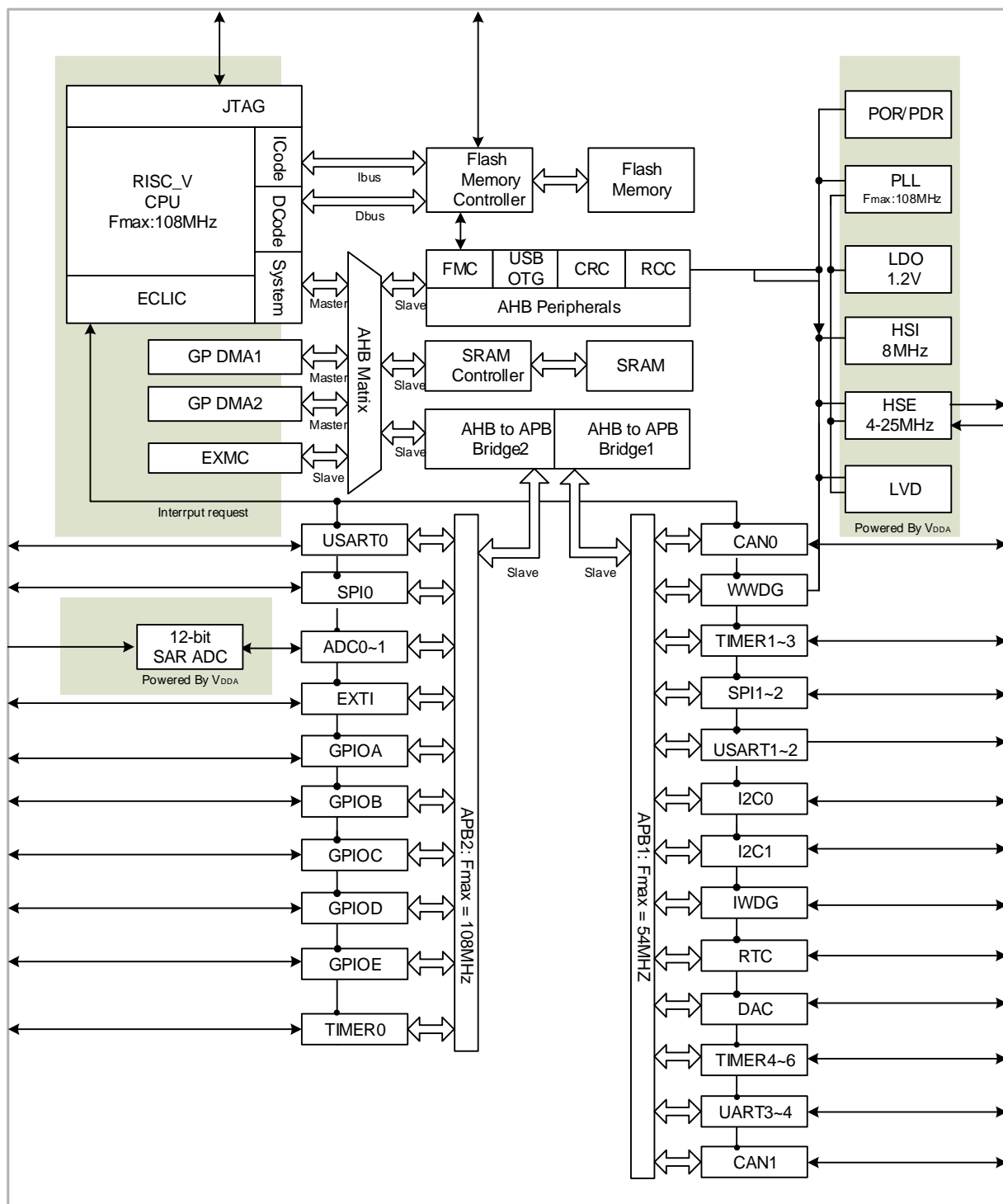
Figure 1-1. GD32VF103 system architecture
