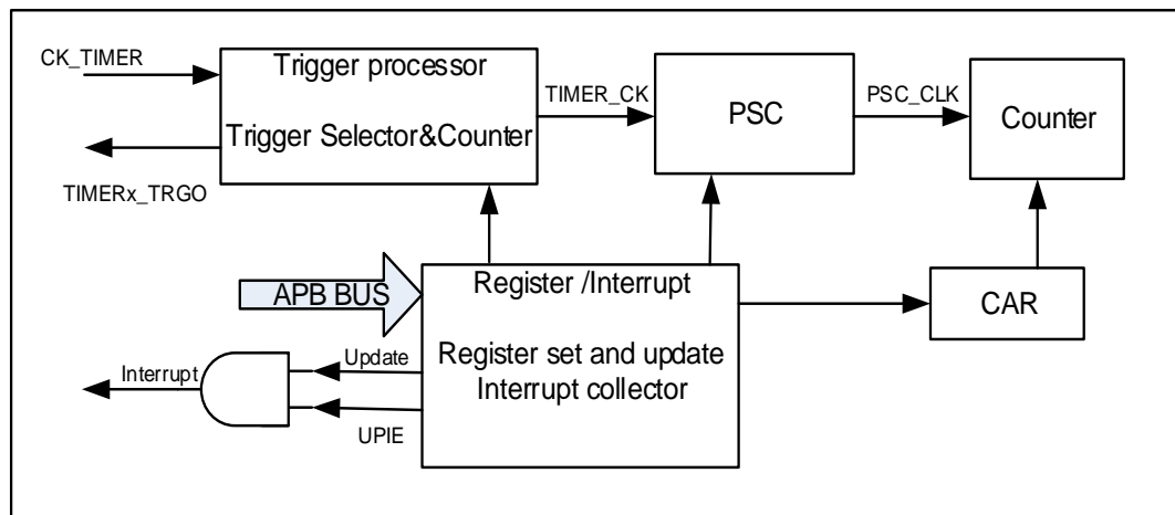
Figure 15-45. Basic timer block diagram
