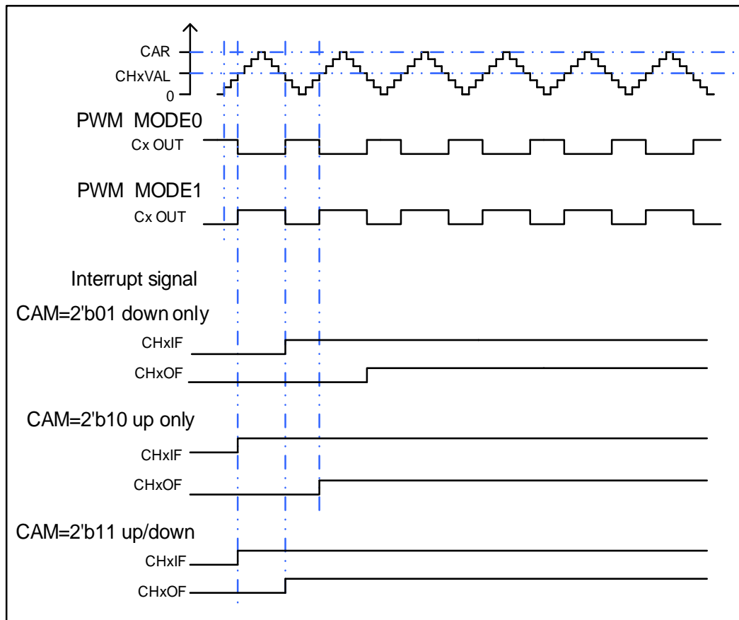
Figure 15-41. CAPWM timechart
