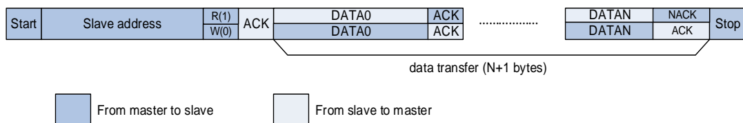
Figure 17-7. I2C communication flow with 10-bit address (Master Transmit)
