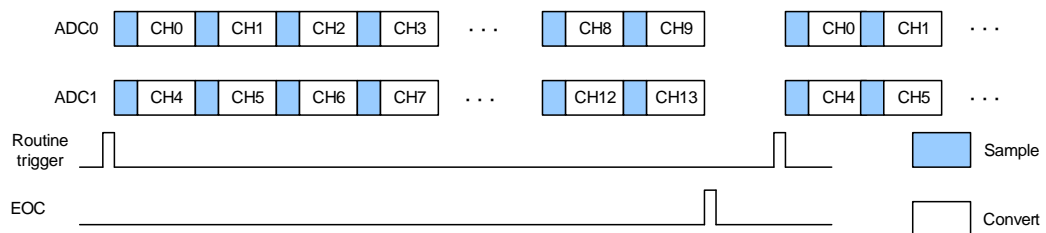
Figure 11-12. Routine parallel mode on 10 channels
