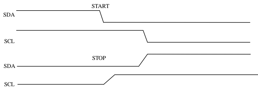
Figure 17-3. START and STOP condition
