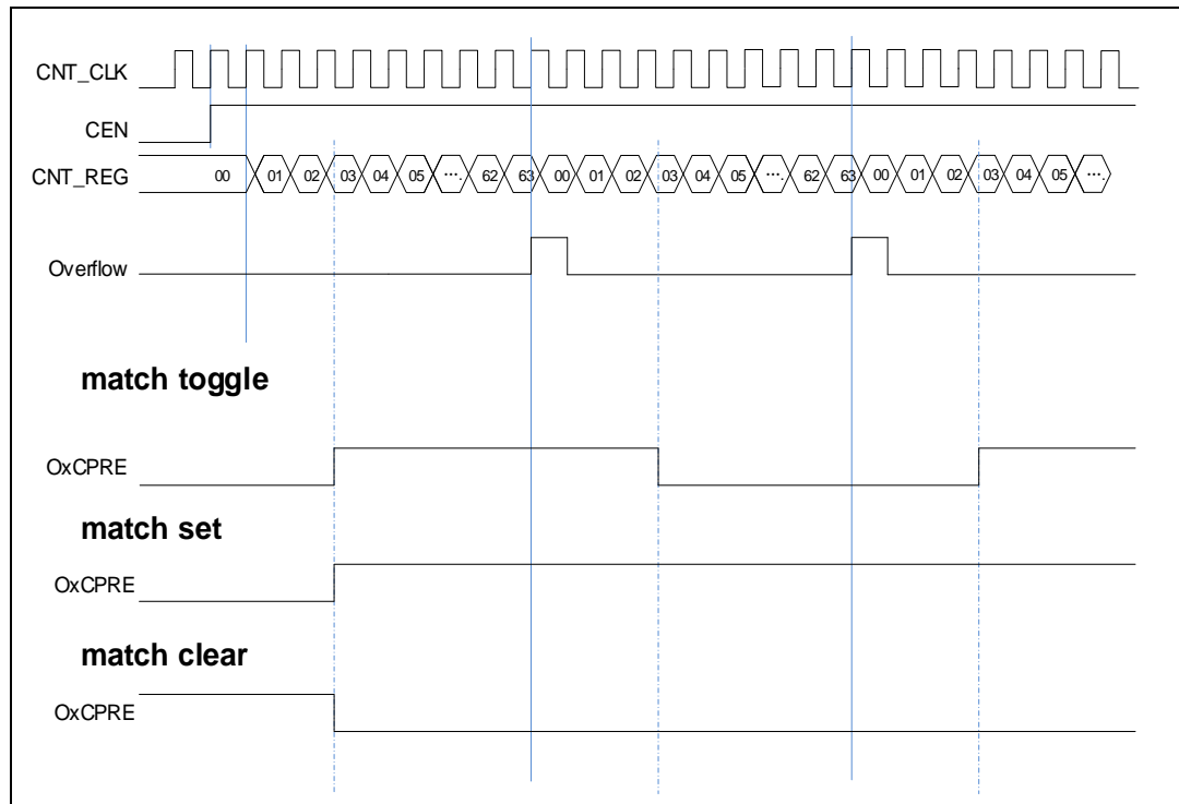
Figure 15-41. Output-compare in three modes
