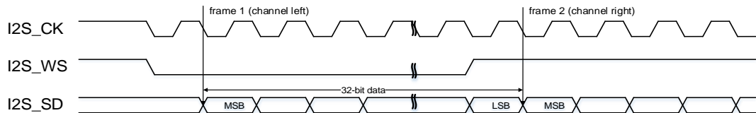
Figure 18-11. I2S Phillips standard timing diagram (DTLEN=10, CHLEN=1, CKPL=1)
