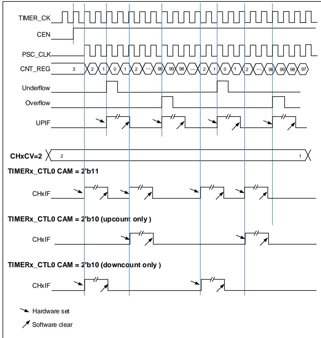
Figure 15-54. Timing chart of center-aligned counting mode
