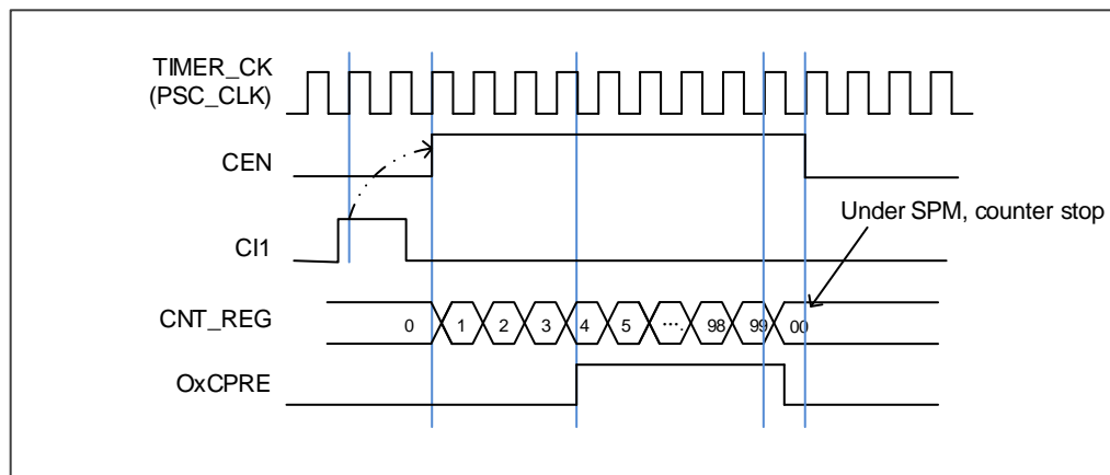
Figure 15-63. Single pulse mode TIMERx_CHxCV = 4 TIMERx_CAR=99
