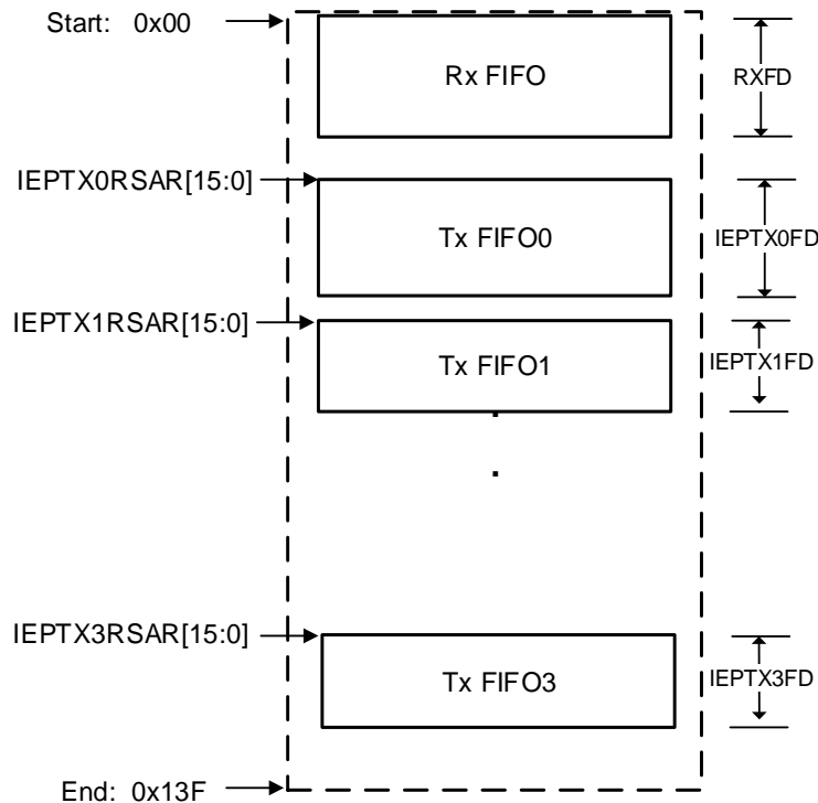
Figure 24-7. Device mode FIFO space in SRAM
