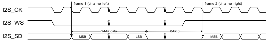
Figure 18-13. I2S Phillips standard timing diagram (DTLEN=01, CHLEN=1, CKPL=1)
