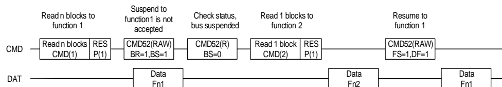
Figure 19-14. Function2 read cycle inserted during function1 multiple read cycle
