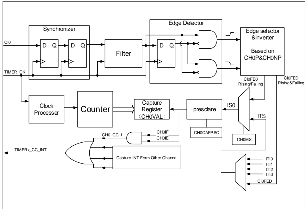
Figure 15-72. Channels input capture principle
