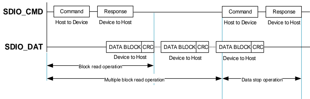
Figure 19-2. SDIO multiple blocks read operation
