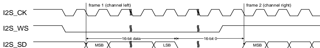
Figure 18-15. I2S Phillips standard timing diagram (DTLEN=00, CHLEN=1, CKPL=1)
