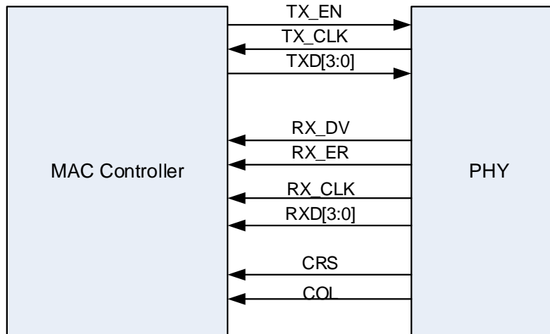
Figure 22-4. Media independent interface signals
