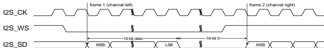
Figure 18-14. I2S Phillips standard timing diagram (DTLEN=00, CHLEN=1, CKPL=0)
