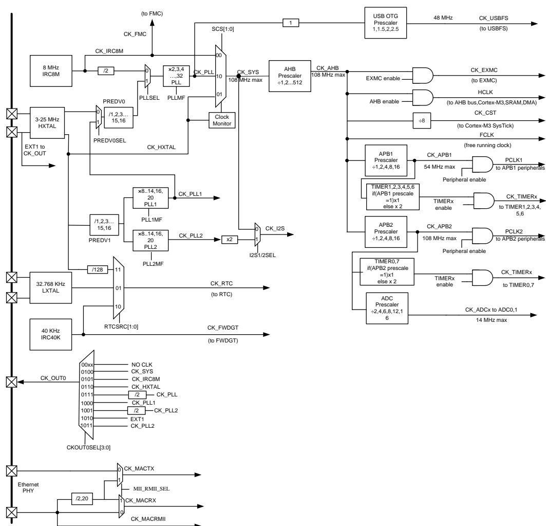
Figure 5-6. Clock tree
