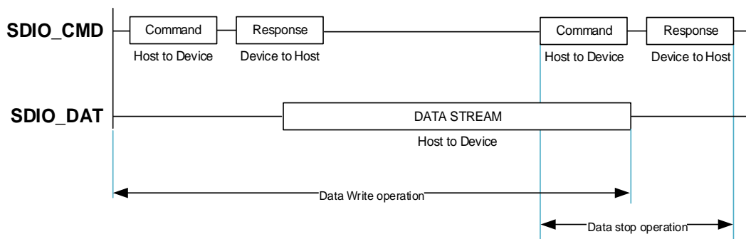
Figure 19-5. SDIO sequential write operation
