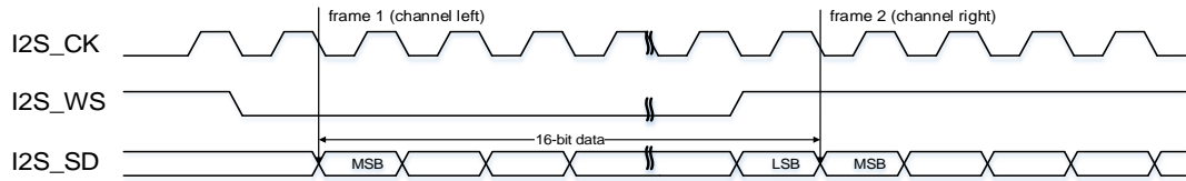
Figure 18-8. I2S Phillips standard timing diagram (DTLEN=00, CHLEN=0, CKPL=0)
