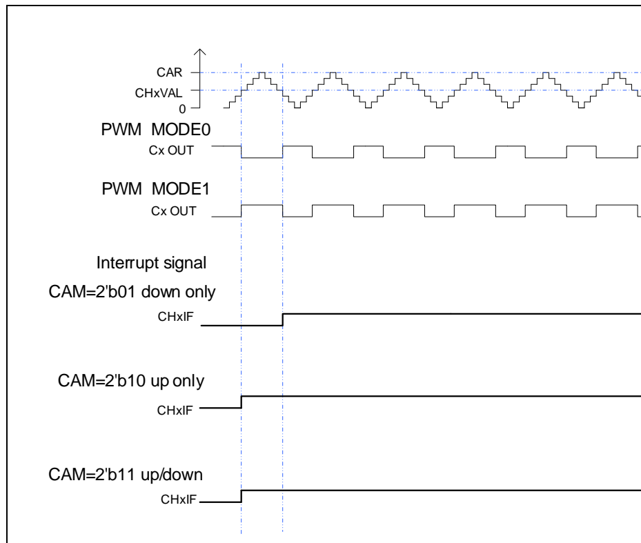
Figure 15-43. CAPWM timechart
