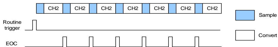
Figure 11-3. Continuous operation mode
