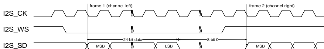
Figure 18-12. I2S Phillips standard timing diagram (DTLEN=01, CHLEN=1, CKPL=0)
