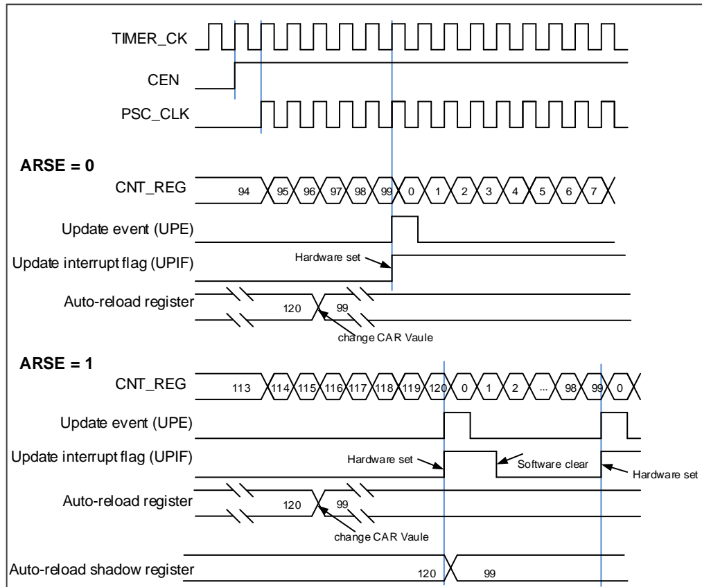
Figure 15-68. Up-counter timechart, change TIMERx_CAR on the go
