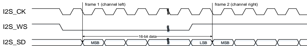
Figure 18-9. I2S Phillips standard timing diagram (DTLEN=00, CHLEN=0, CKPL=1)
