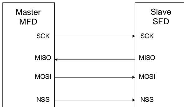
Figure 18-3. A typical full-duplex connection
