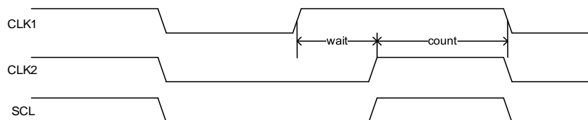
Figure 17-4. Clock synchronization
