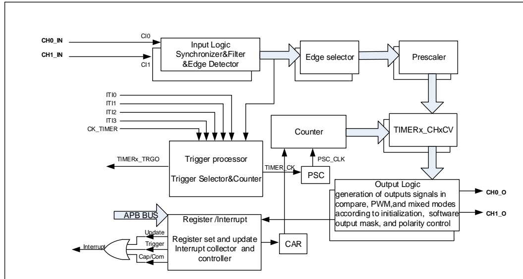
Figure 15-47. General level1 timer block diagram
