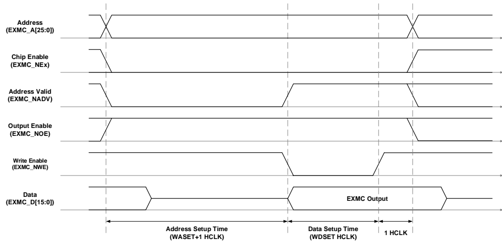
Figure 20-14. Mode C write access
