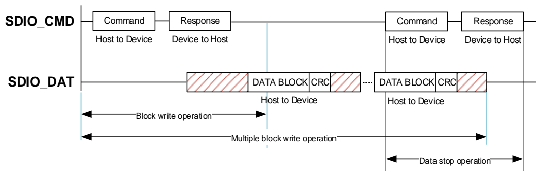
Figure 19-3. SDIO multiple blocks write operation
