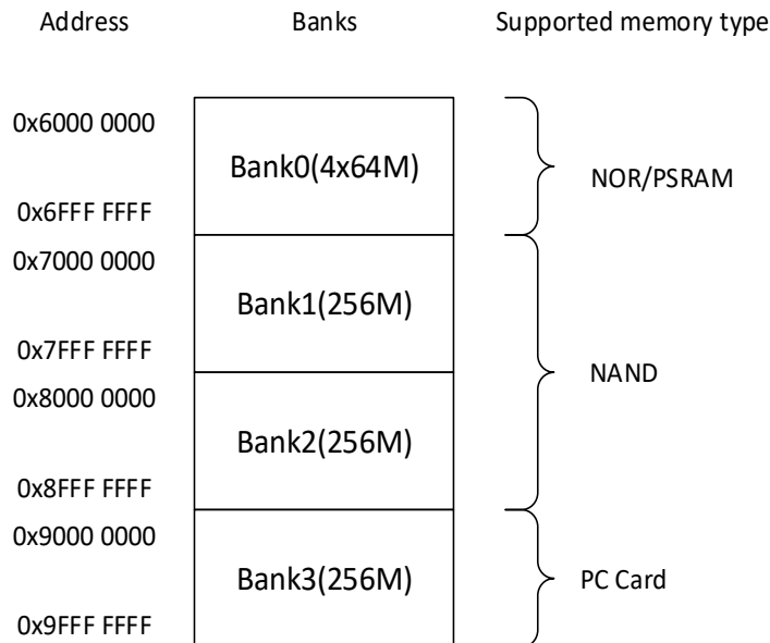
Figure 20-2. EXMC memory banks
