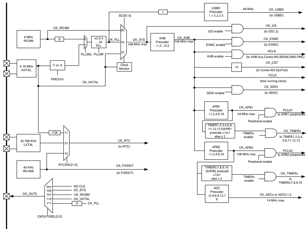
Figure 5-2. Clock tree
