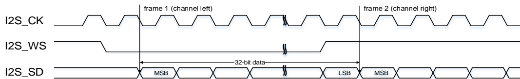
Figure 18-10. I2S Phillips standard timing diagram (DTLEN=10, CHLEN=1, CKPL=0)
