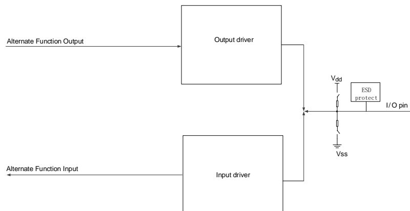
Figure 8-5. Basic structure of Alternate function configuration
