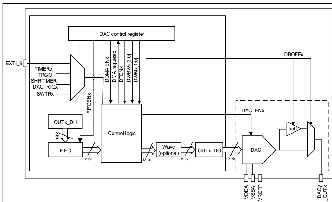
Figure 14-1. DAC block diagram
