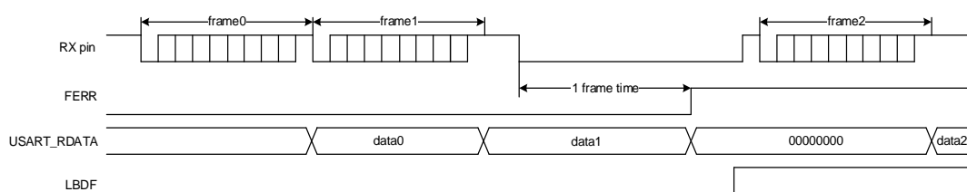
Figure 20-23. Break frame occurs during idle state
