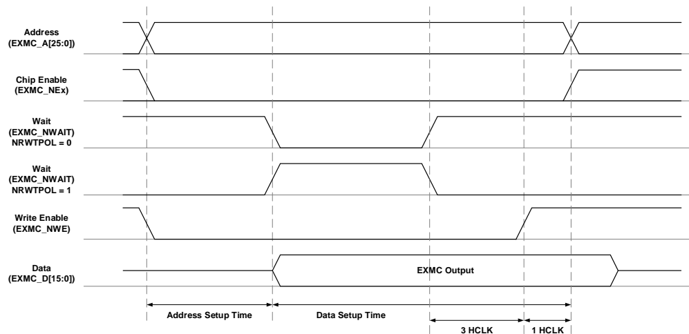
Figure 24-20. Write access timing diagram under async-wait signal assertion
