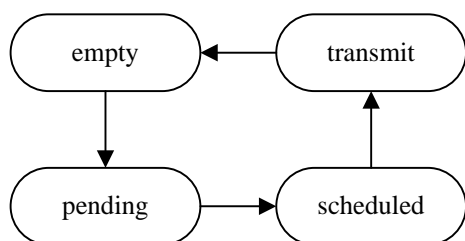
Figure 25-3. State of transmit mailbox
