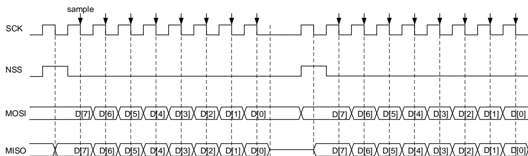
Figure 22-9. Timing diagram of TI master mode with continuous transfer
