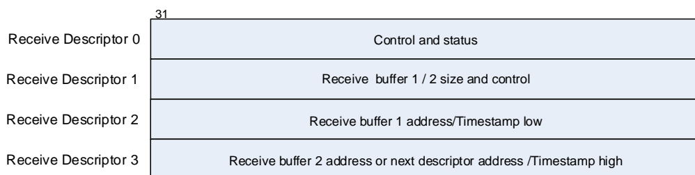
Figure 26-9. Receive descriptor in normal mode
