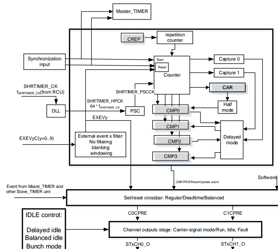
Figure 19-10. Slave_TIMERx diagram
