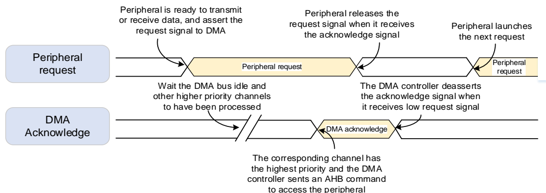
Figure 11-2. Handshake mechanism
