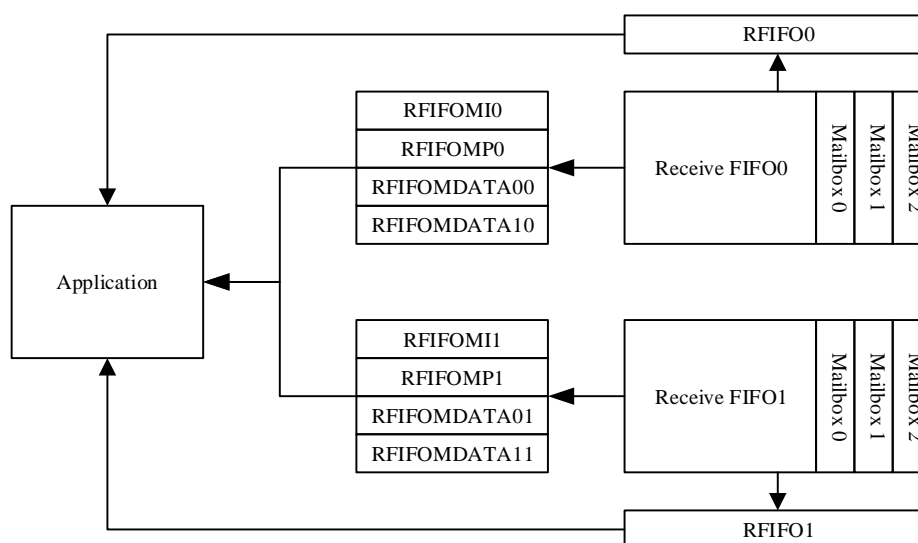
Figure 25-4. Reception register
