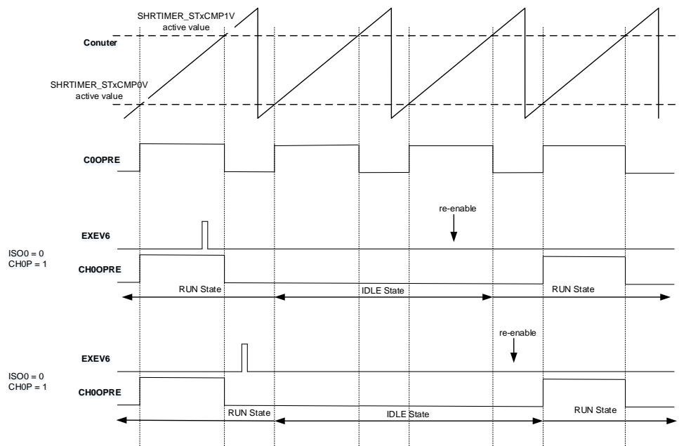
Figure 19-33. ISO0 = 1 and CHOP = 1 in delayed IDLE
