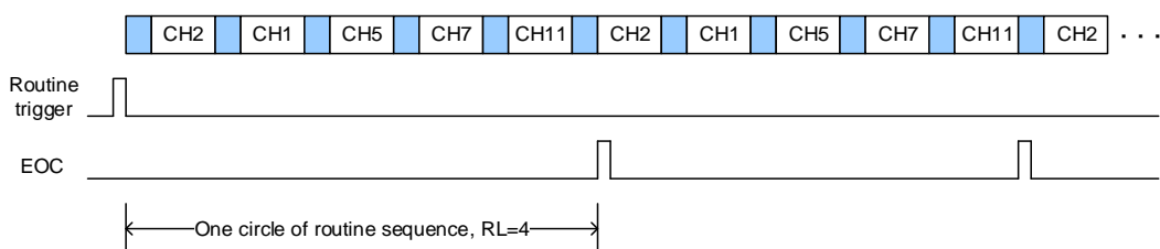
Figure 13-5. Scan operation mode, continuous operation mode enable
