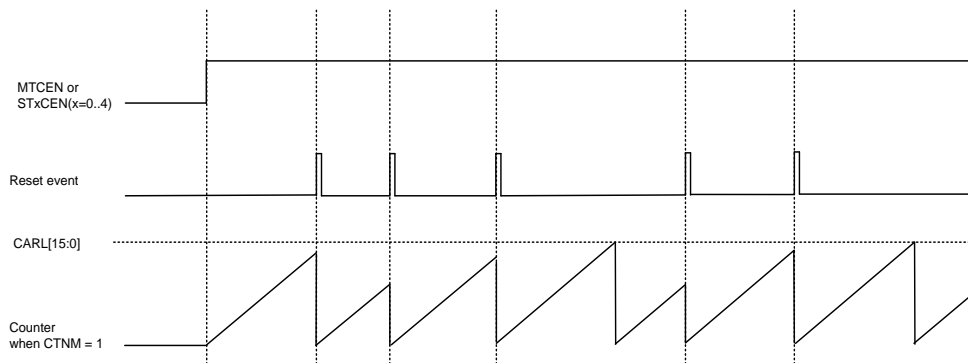
Figure 19-5. Counter behavior in continuous mode
