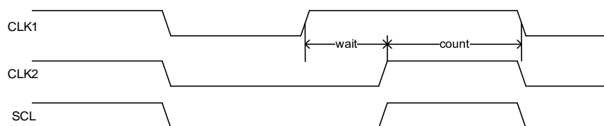
Figure 21-4. Clock synchronization
