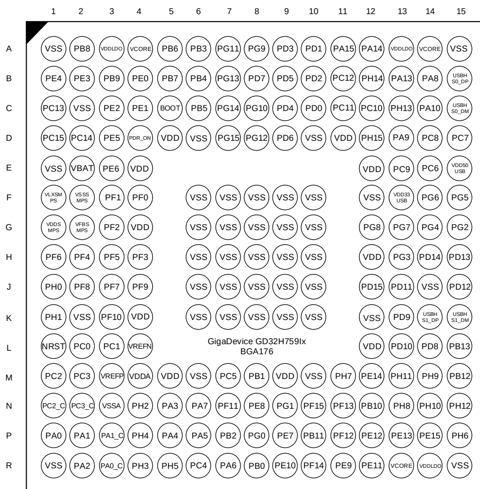
Figure 2-2. GD32H759xx BGA176 pinouts
