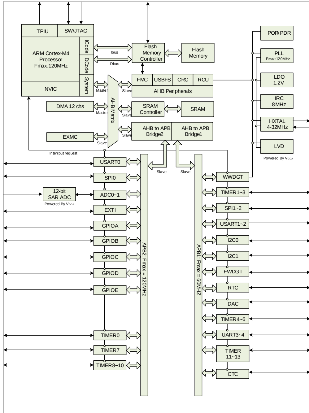
Figure 2-1.GD32E103xx block diagram
